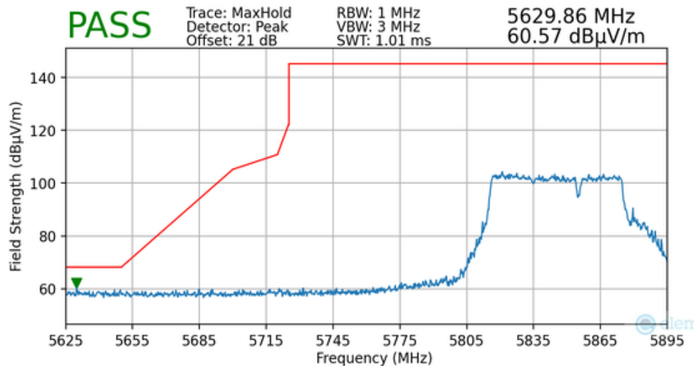
Plot 7-158. Radiated Lower Band Edge Plot MIMO (Peak – UNII Band 4 – Punctured)
