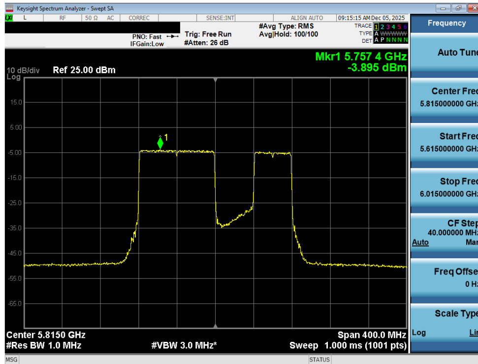
Plot 7-121. Power Spectral Density Plot MIMO ANT2 (160MHz BW 802.11be (40MHz Puncture) (UNII Band 3/4) – Ch. 163)
