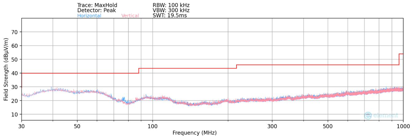
Plot 7-131. Radiated Spurious Plot below 1GHz MIMO 802.11b (2.4GHz – Ch. 6) + MIMO 802.11a (5GHz – Ch. 120)
