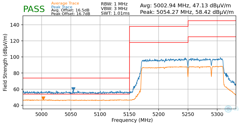
Plot 7-165. Radiated Lower Band Edge Plot MIMO (Average & Peak – UNII Band 1 – Punctured)
