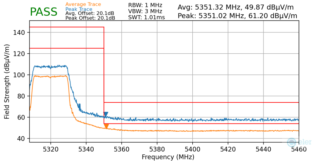
Plot 7-141. Radiated Upper Band Edge Plot MIMO with WCP (Average & Peak – UNII Band 2A)
