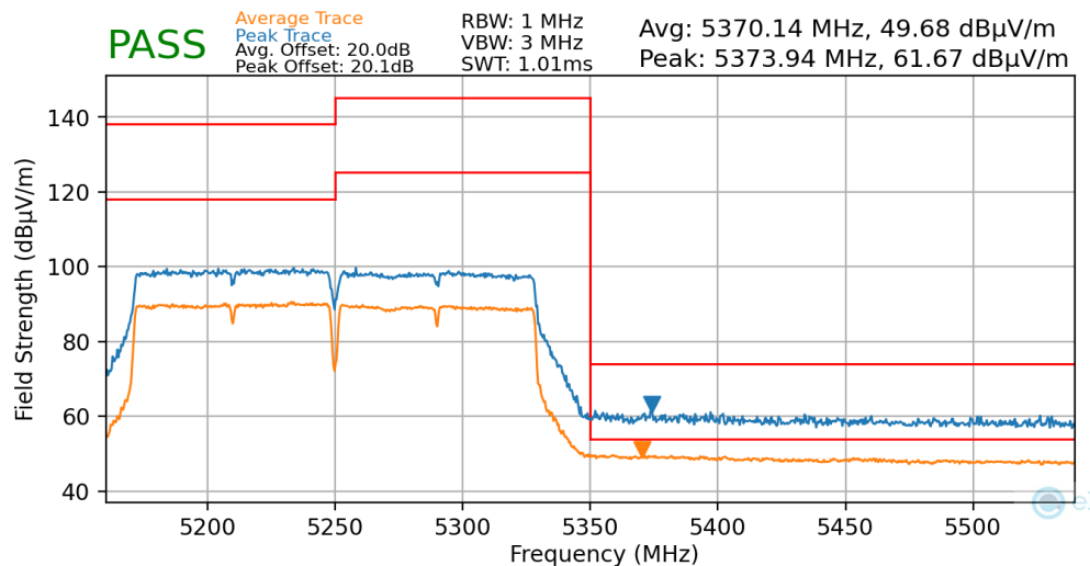
Plot 7-161. Radiated Upper Band Edge Plot MIMO (Average & Peak – UNII Band 2A)
