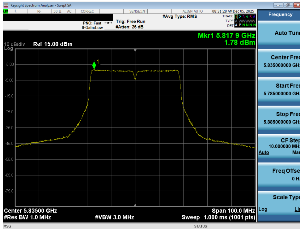
Plot 7-115. Power Spectral Density Plot MIMO ANT2 (40MHz BW 802.11n (UNII Band 3/4) – Ch. 167)
