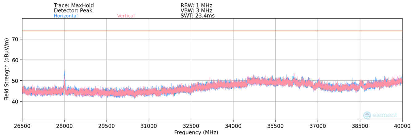
Plot 7-134. Radiated Spurious Plot below 26.5-40GHz MIMO 802.11b (2.4GHz – Ch.6) + MIMO 802.11a (5GHz – Ch. 120)
