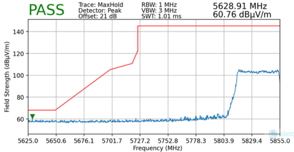
Plot 7-146. Radiated Lower Band Edge Plot MIMO (Peak – UNII Band 4)
