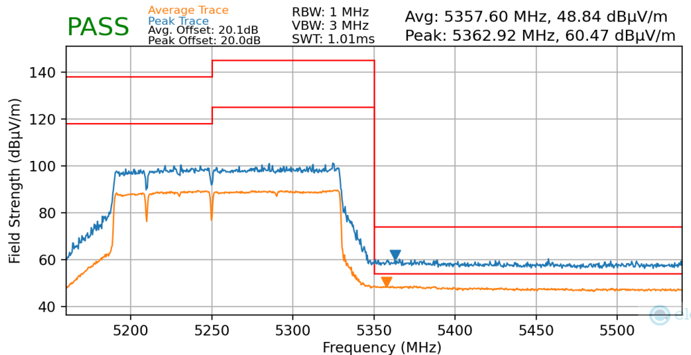
Plot 7-166. Radiated Upper Band Edge Plot MIMO (Average & Peak – UNII Band 2A – Punctured)
