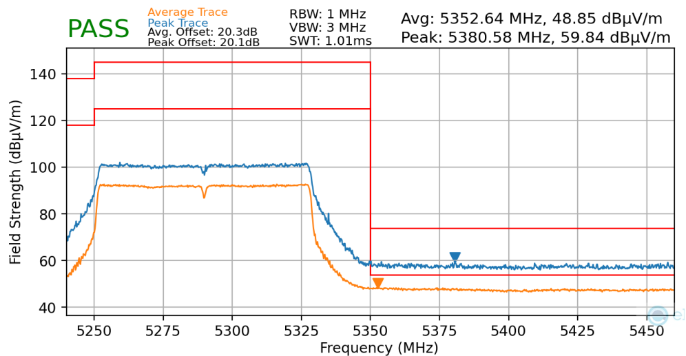
Plot 7-149. Radiated Upper Band Edge Plot MIMO (Average & Peak – UNII Band 2A)
