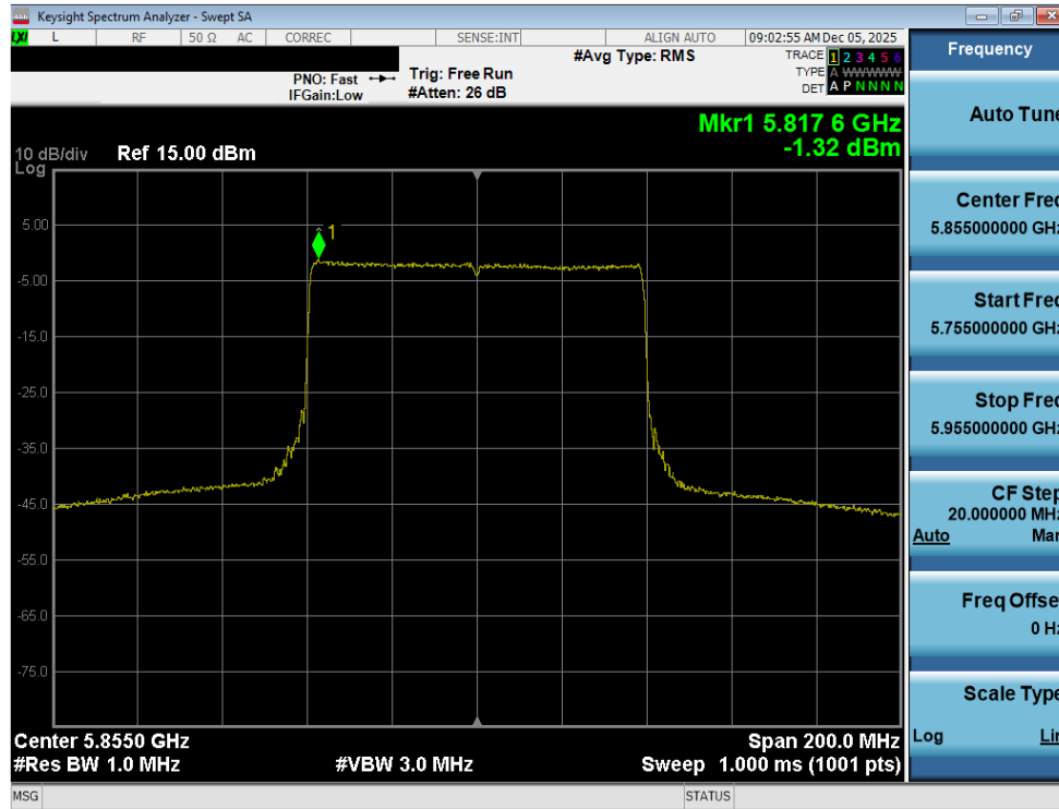
Plot 7-118. Power Spectral Density Plot MIMO ANT2 (80MHz BW 802.11be (UNII Band 3/4) – Ch. 171)
