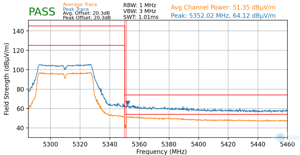
Plot 7-143. Radiated Upper Band Edge Plot MIMO (Average & Peak – UNII Band 2A)
