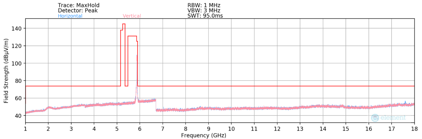
Plot 7-127. Radiated Spurious Plot above 1GHz MIMO (802.11a – UNII Band 4 Ch. 173)
