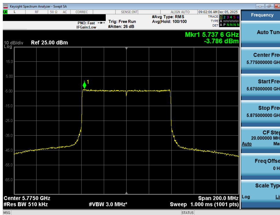
Plot 7-110. Power Spectral Density Plot MIMO ANT2 (80MHz BW 802.11be (UNII Band 3) – Ch. 155)
