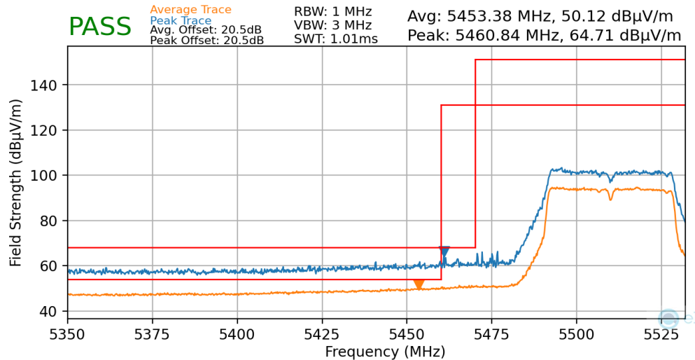
Plot 7-144. Radiated Lower Band Edge Plot MIMO (Average & Peak – UNII Band 2C)
