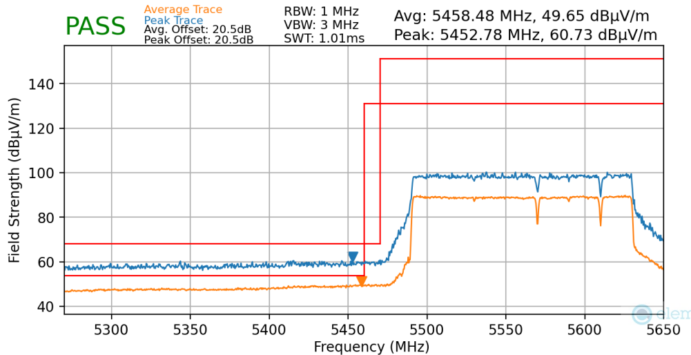
Plot 7-167. Radiated Lower Band Edge Plot MIMO (Average & Peak – UNII Band 2C – Punctured)
