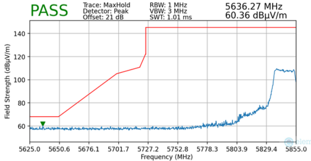
Plot 7-139. Radiated Lower Band Edge Plot MIMO (Peak – UNII Band 4)
