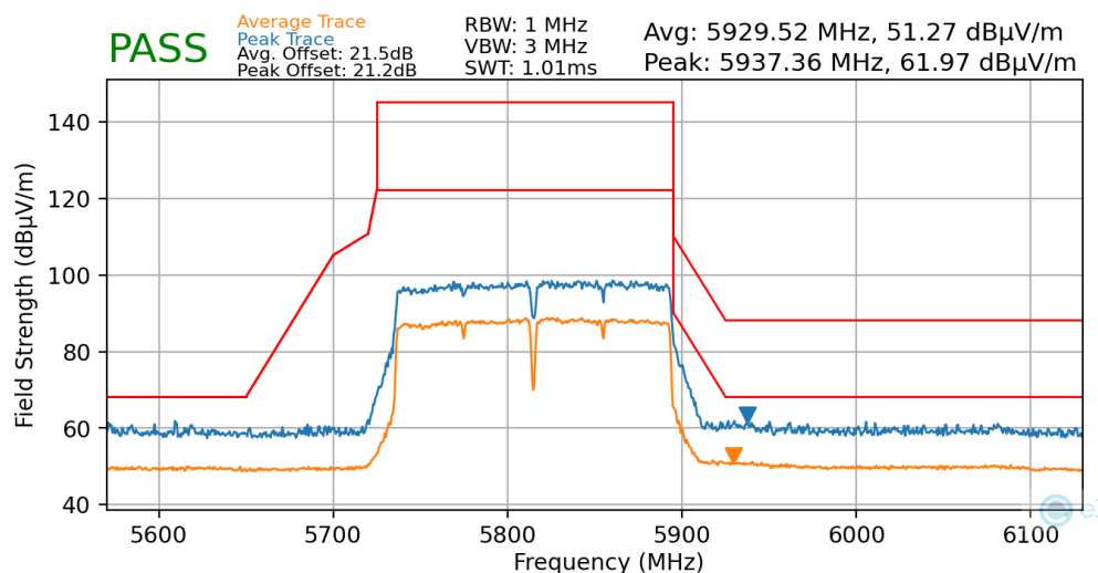
Plot 7-164. Radiated Upper Band Edge Plot MIMO (Average & Peak – UNII Band 4)
