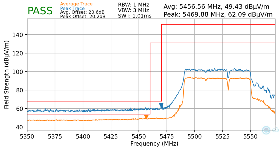
Plot 7-156. Radiated Lower Band Edge Plot MIMO (Average & Peak – UNII Band 2C – Punctured)
