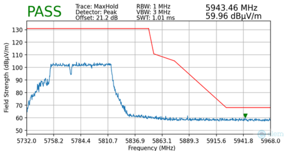
Plot 7-157. Radiated Upper Band Edge Plot MIMO (Peak – UNII Band 3 – Punctured)
