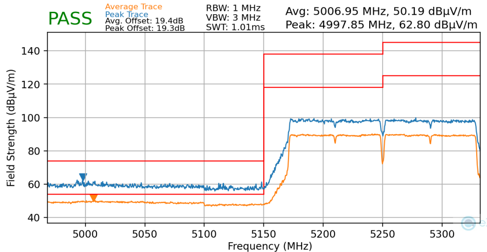
Plot 7-160. Radiated Lower Band Edge Plot MIMO (Average & Peak – UNII Band 1)
