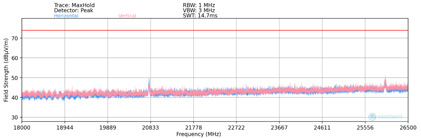
Plot 7-129. Radiated Spurious Plot 18GHz – 26.5GHz MIMO (802.11a)
