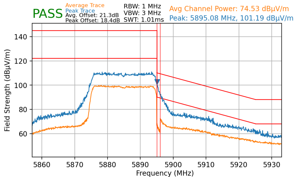
Plot 7-140. Radiated Upper Band Edge Plot MIMO (Average & Peak – UNII Band 4)
