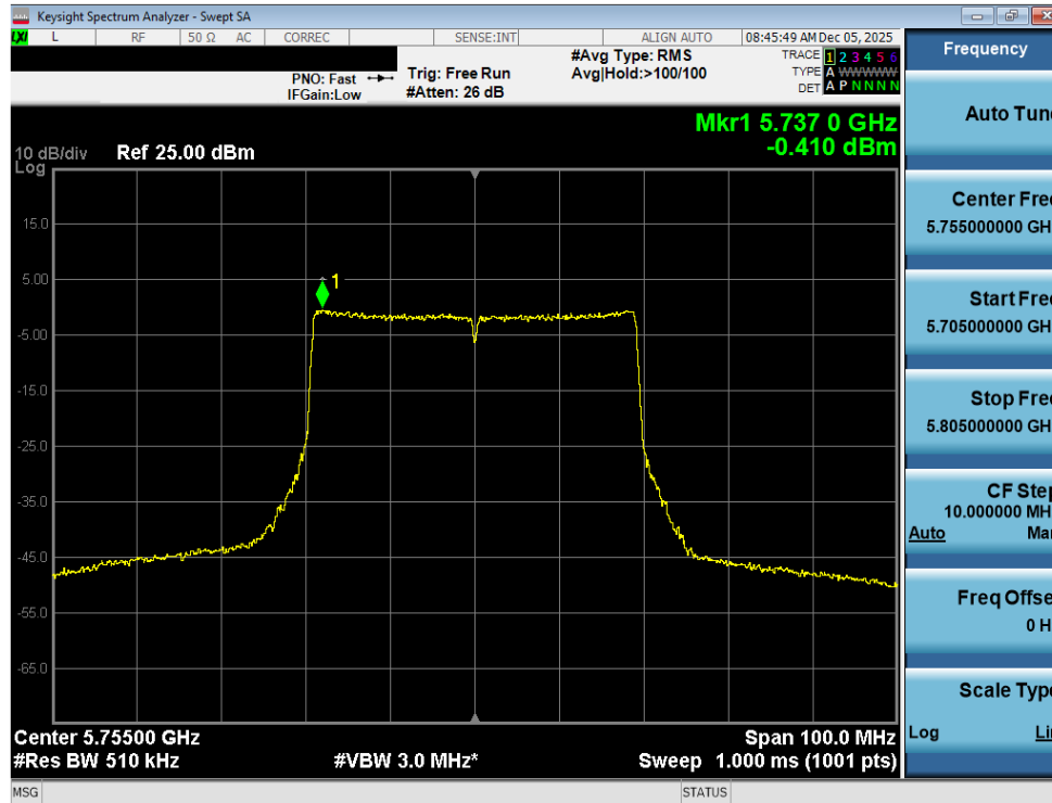
Plot 7-108. Power Spectral Density Plot MIMO ANT2 (40MHz BW 802.11be (UNII Band 3) – Ch. 151)
