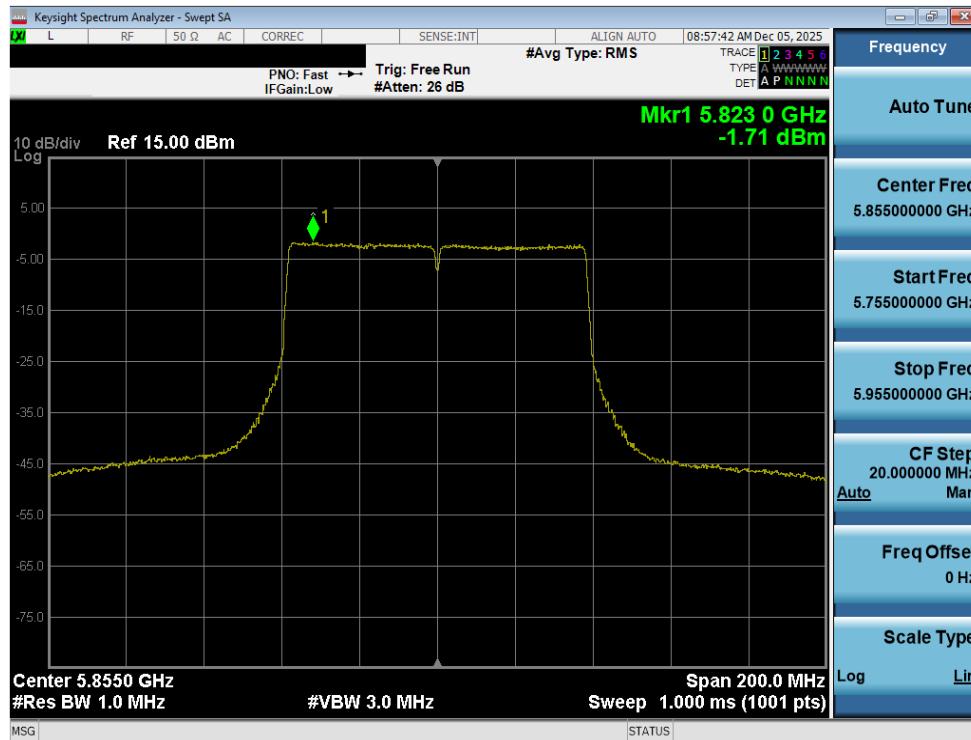
Plot 7-117. Power Spectral Density Plot MIMO ANT2 (80MHz BW 802.11ac (UNII Band 3/4) – Ch. 171)
