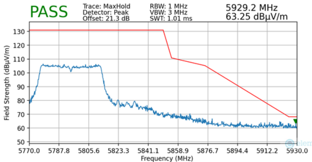
Plot 7-145. Radiated Upper Band Edge Plot MIMO (Peak – UNII Band 3)
