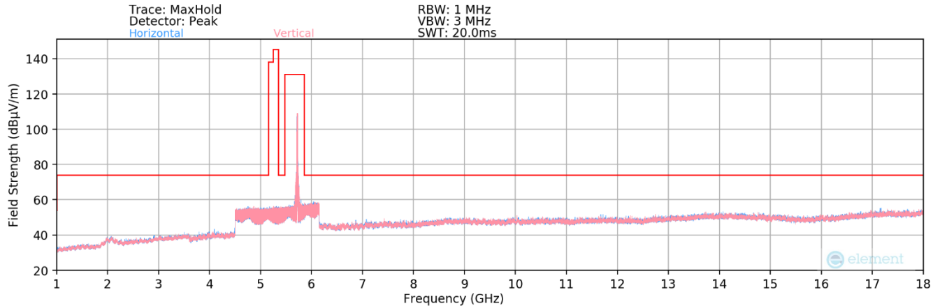
Plot 7-125. Radiated Spurious Plot above 1GHz MIMO (802.11a – UNII Band 2C Ch. 120)
