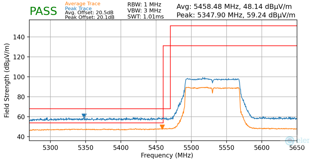
Plot 7-150. Radiated Lower Band Edge Plot MIMO (Average & Peak – UNII Band 2C)
