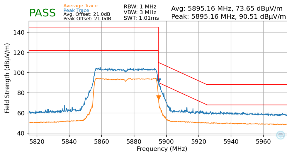
Plot 7-147. Radiated Upper Band Edge Plot MIMO (Average & Peak – UNII Band 4)
