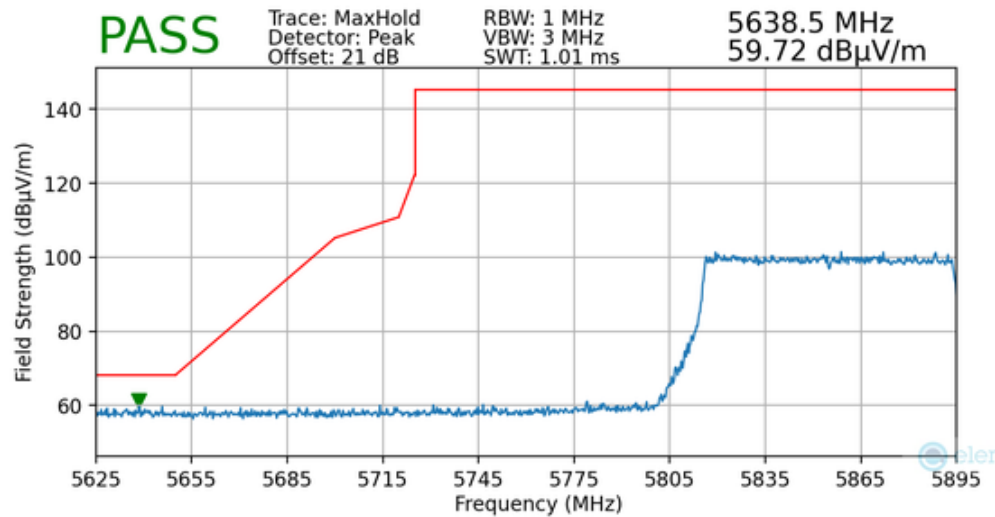
Plot 7-152. Radiated Lower Band Edge Plot MIMO (Peak – UNII Band 4)
