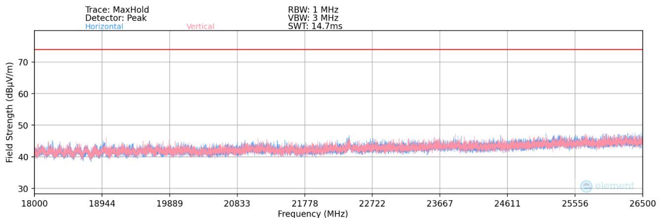
Plot 7-133. Radiated Spurious Plot below 18-26.5GHz MIMO 802.11b (2.4GHz – Ch.6) + MIMO 802.11a (5GHz – Ch. 120)
