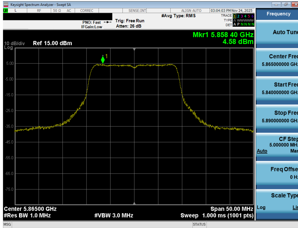
Plot 7-114. Power Spectral Density Plot MIMO ANT2 (20MHz BW 802.11be (UNII Band 4) – Ch. 173)
