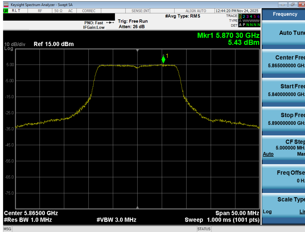
Plot 7-112. Power Spectral Density Plot MIMO ANT2 (802.11a (UNII Band 4) – Ch. 173)
