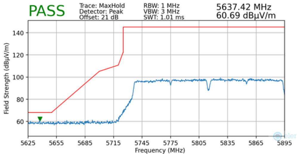
Plot 7-163. Radiated Lower Band Edge Plot MIMO (Peak – UNII Band 4)
