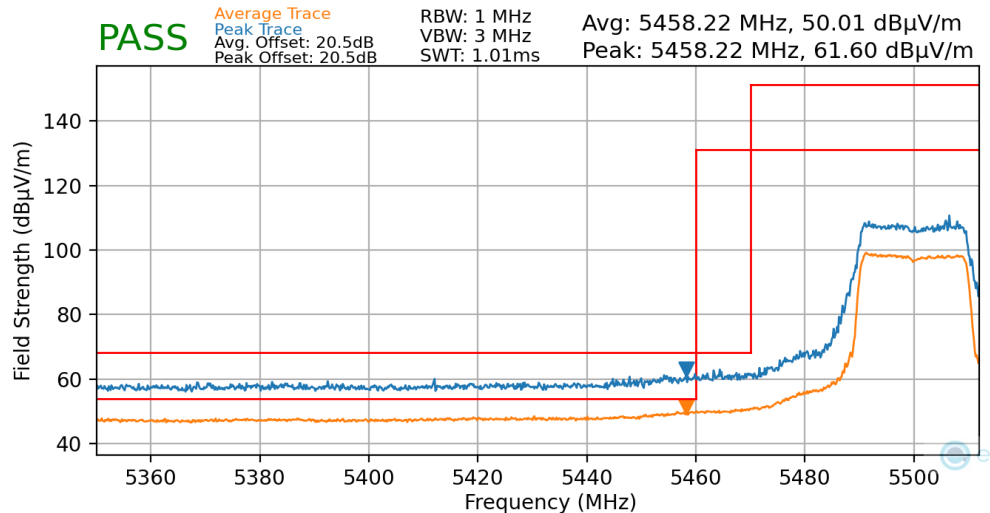
Plot 7-137. Radiated Lower Band Edge Plot MIMO (Average & Peak – UNII Band 2C)
