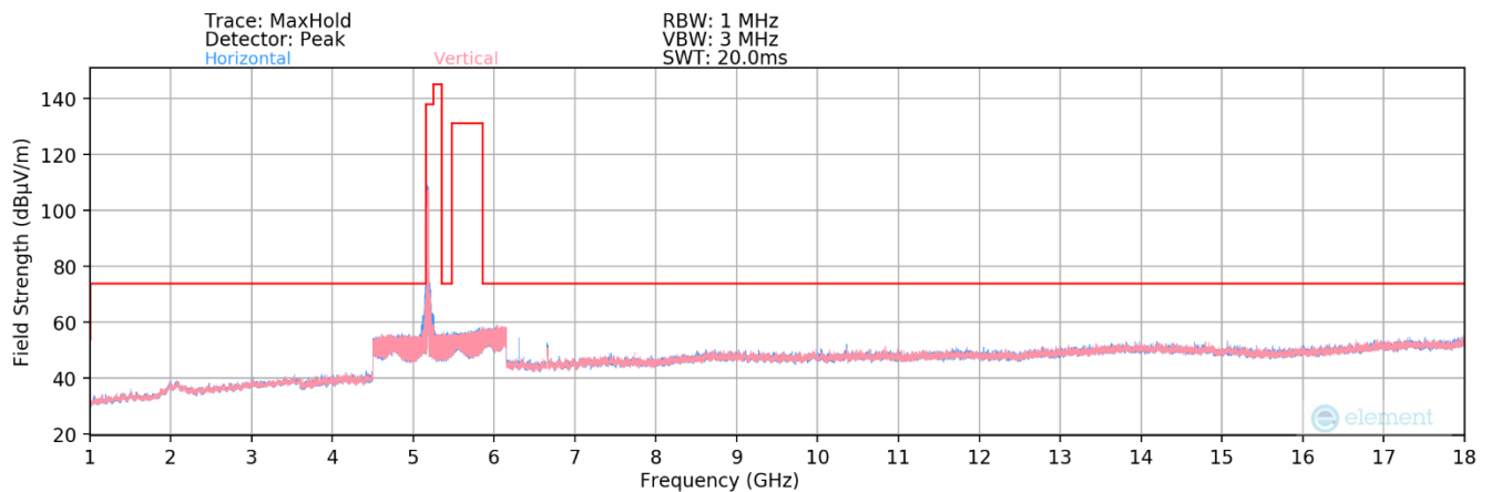
Plot 7-123. Radiated Spurious Plot above 1GHz MIMO (802.11a – UNII Band 1 Ch. 40)
