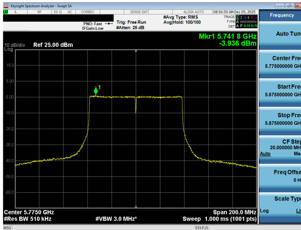
Plot 7-109. Power Spectral Density Plot MIMO ANT2 (80MHz BW 802.11ac (UNII Band 3) – Ch. 155)
