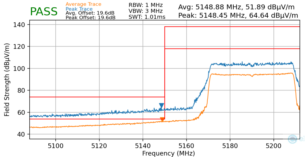
Plot 7-142. Radiated Lower Band Edge Plot MIMO (Average & Peak – UNII Band 1)
