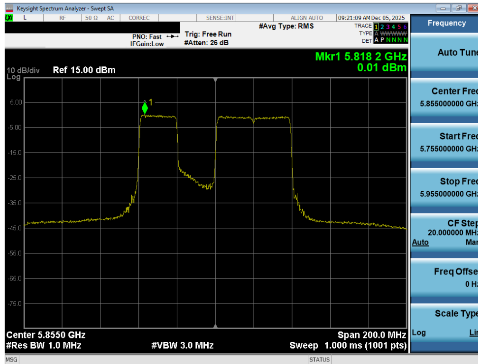
Plot 7-119. Power Spectral Density Plot MIMO ANT2 (80MHz BW 802.11be (20MHz Puncture) (UNII Band 3/4) – Ch. 171)
