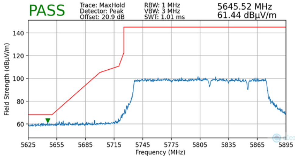
Plot 7-168. Radiated Lower Band Edge Plot MIMO (Peak – UNII Band 4 – Punctured)
