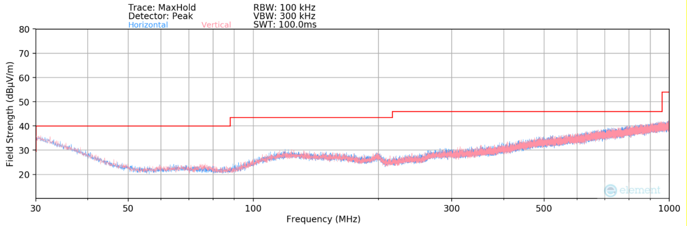
Plot 7-122. Radiated Spurious Plot below 1GHz MIMO (802.11a)
