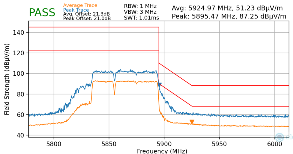
Plot 7-159. Radiated Upper Band Edge Plot MIMO (Average & Peak – UNII Band 4 – Punctured)
