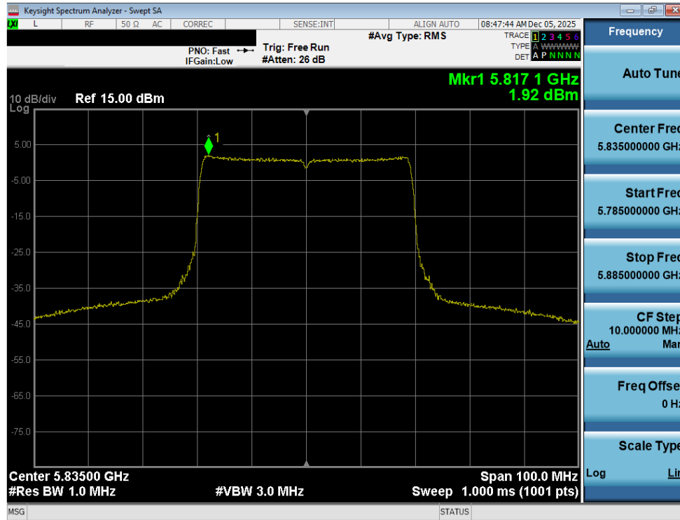
Plot 7-116. Power Spectral Density Plot MIMO ANT2 (40MHz BW 802.11be (UNII Band 3/4) – Ch. 167)
