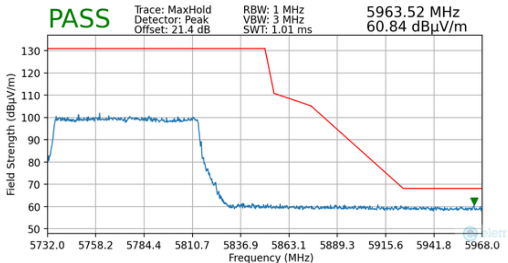
Plot 7-151. Radiated Upper Band Edge Plot MIMO (Peak – UNII Band 3)
