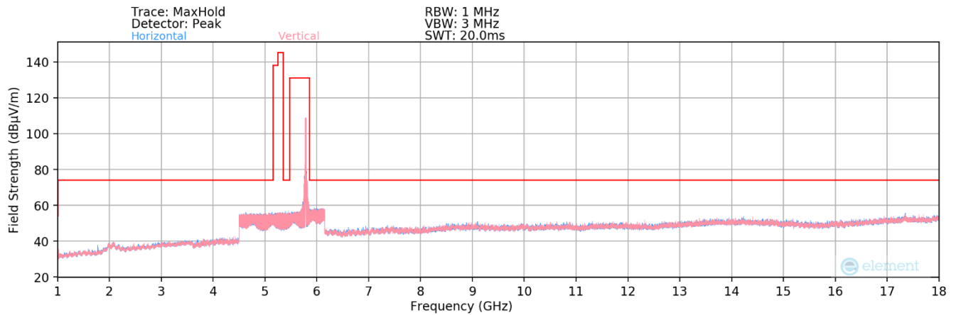
Plot 7-126. Radiated Spurious Plot above 1GHz MIMO (802.11a – UNII Band 3 Ch. 157)
