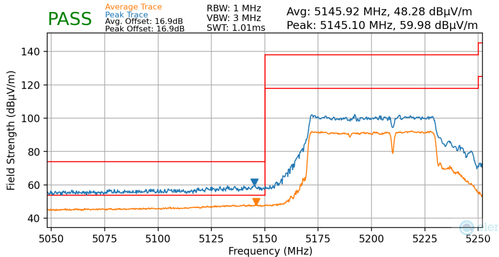
Plot 7-154. Radiated Lower Band Edge Plot MIMO (Average & Peak – UNII Band 1 - Punctured)
