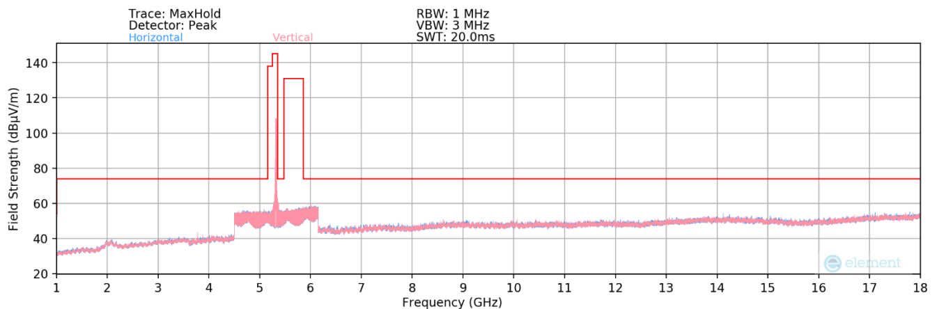
Plot 7-124. Radiated Spurious Plot above 1GHz MIMO (802.11a – UNII Band 2A Ch. 56)
