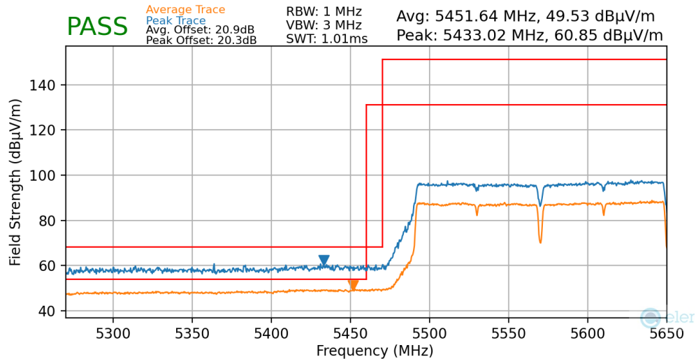
Plot 7-162. Radiated Lower Band Edge Plot MIMO (Average & Peak – UNII Band 2C)
