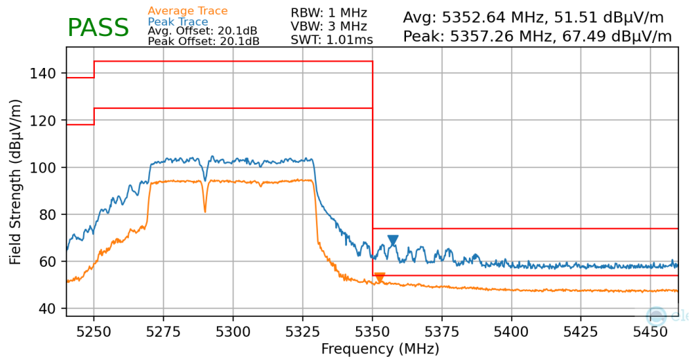
Plot 7-155. Radiated Upper Band Edge Plot MIMO (Average & Peak – UNII Band 2A – Punctured)
