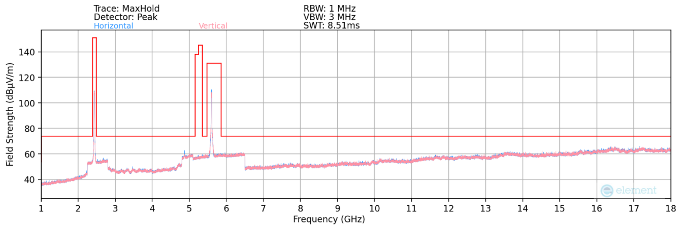
Plot 7-132. Radiated Spurious Plot below 1-18GHz MIMO 802.11b (2.4GHz – Ch.6) + MIMO 802.11a (5GHz – Ch. 120)
