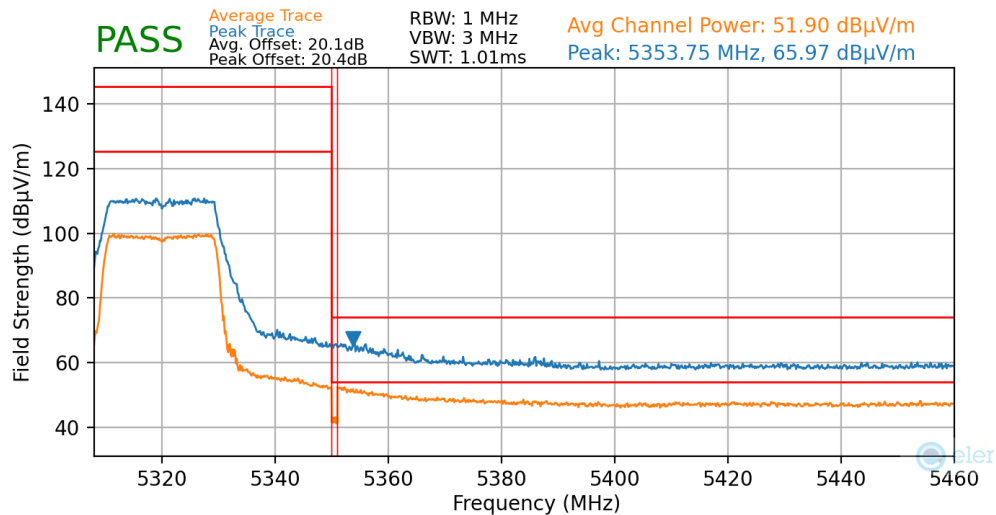
Plot 7-136. Radiated Upper Band Edge Plot MIMO (Average & Peak – UNII Band 2A)
