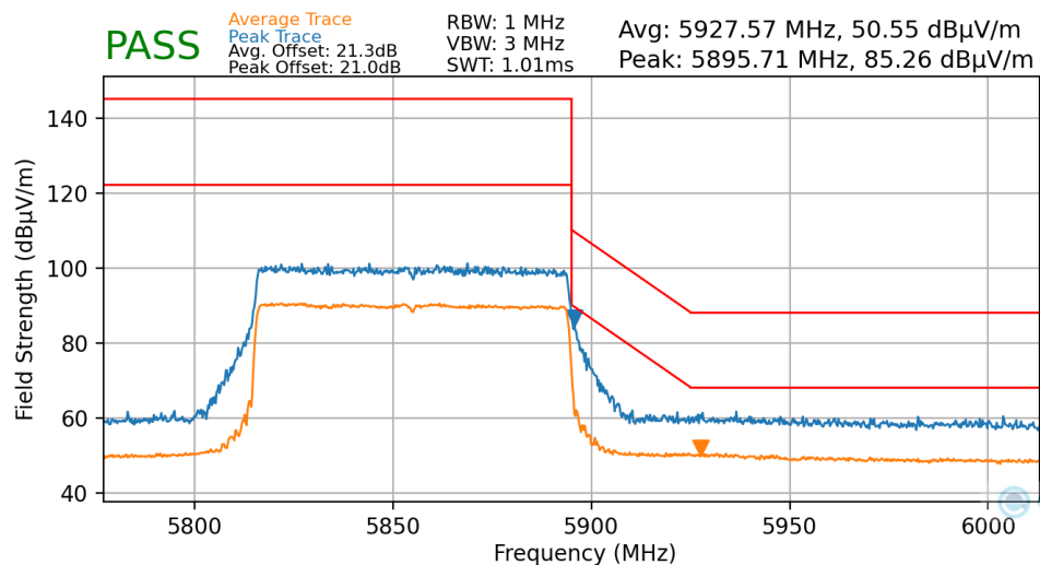
Plot 7-153. Radiated Upper Band Edge Plot MIMO (Average & Peak – UNII Band 4)
