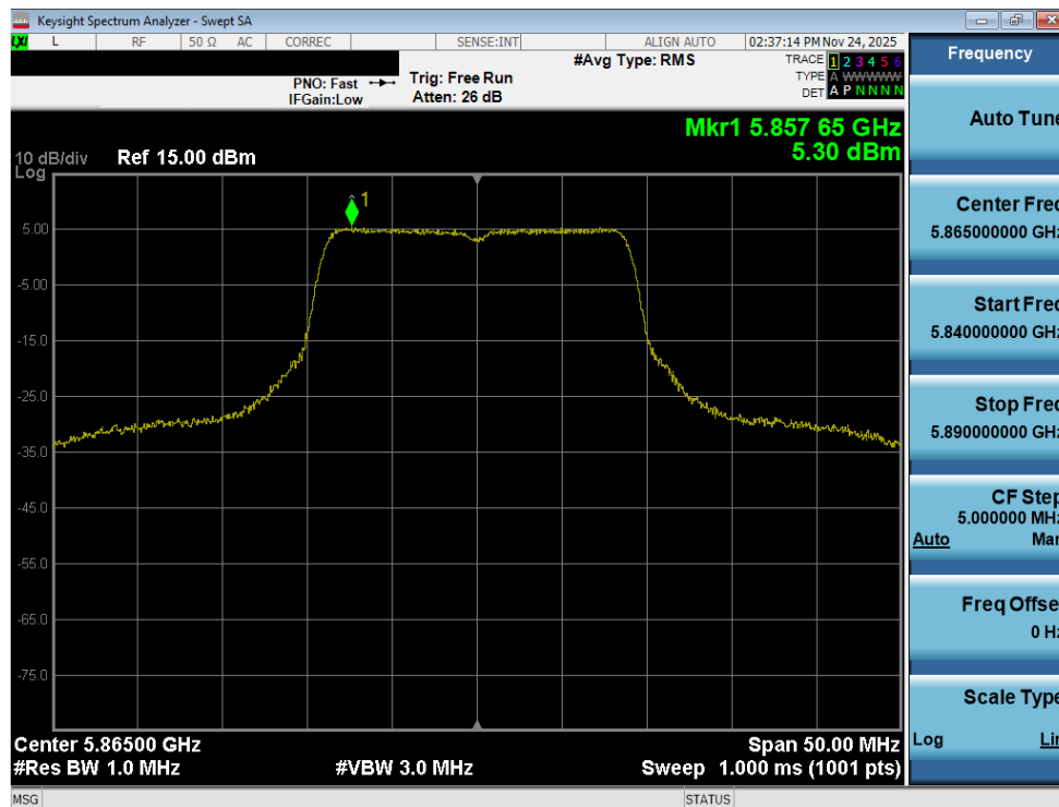
Plot 7-113. Power Spectral Density Plot MIMO ANT2 (20MHz BW 802.11n (UNII Band 4) – Ch. 173)
