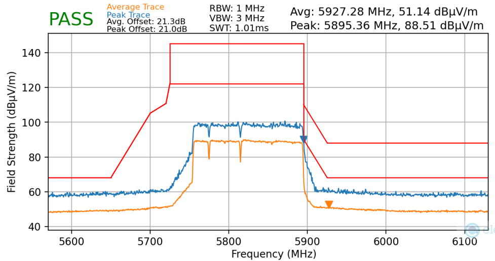
Plot 7-169. Radiated Upper Band Edge Plot MIMO (Average & Peak – UNII Band 4 – Punctured)
