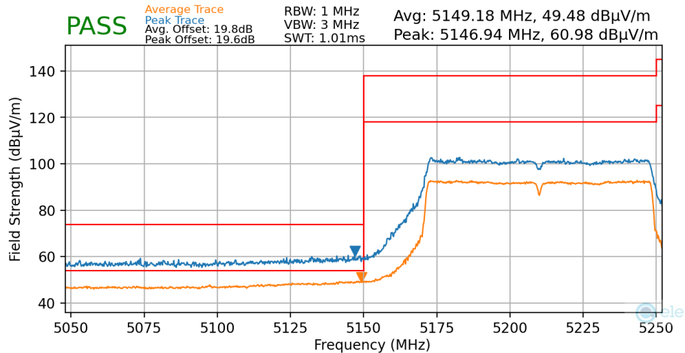
Plot 7-148. Radiated Lower Band Edge Plot MIMO (Average & Peak – UNII Band 1)
