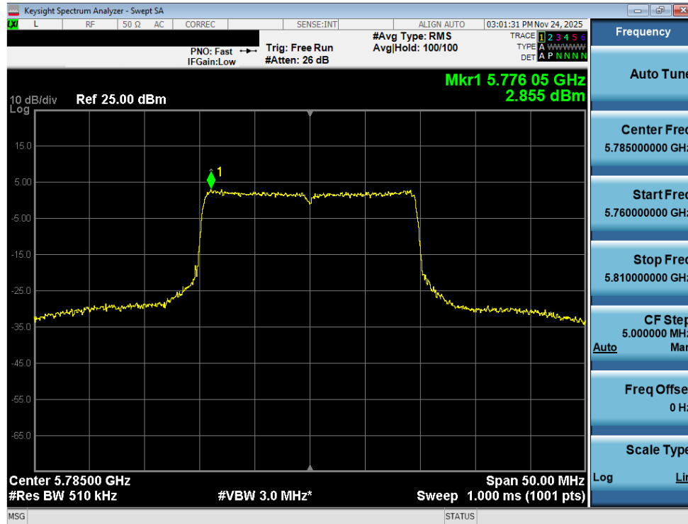
Plot 7-106. Power Spectral Density Plot MIMO ANT2 (20MHz BW 802.11be (UNII Band 3) – Ch. 157)
