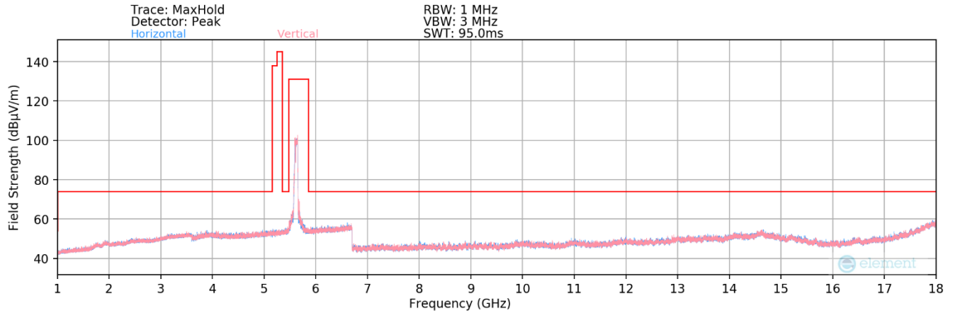
Plot 7-128. Radiated Spurious Plot above 1GHz MIMO (802.11be – UNII Band 2C Ch. 122 – Punctured)
