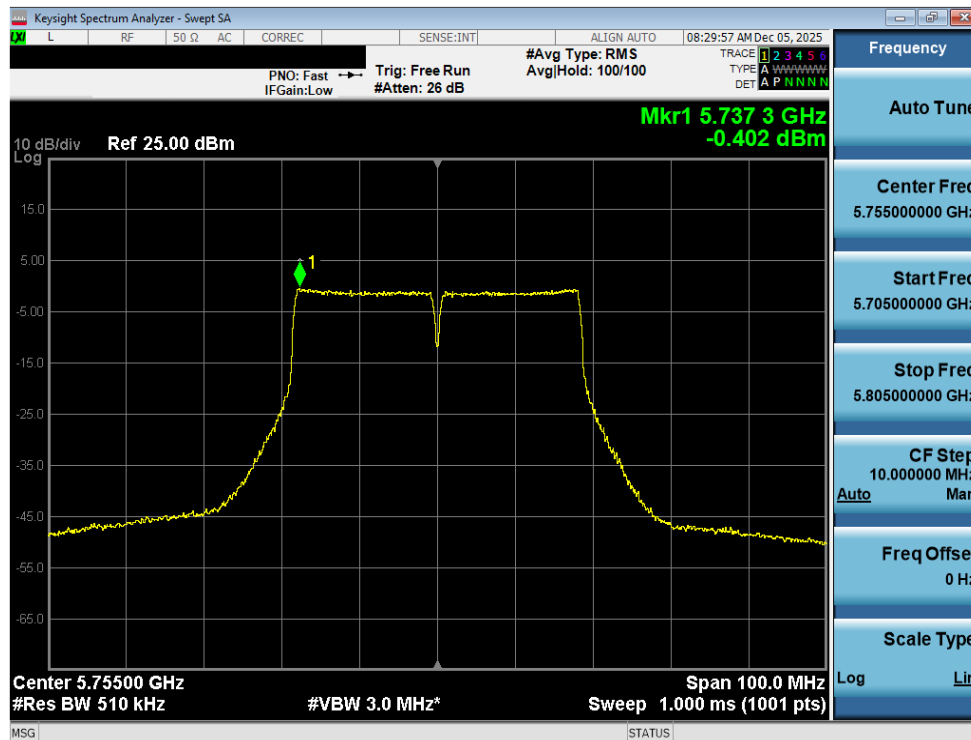
Plot 7-107. Power Spectral Density Plot MIMO ANT2 (40MHz BW 802.11n (UNII Band 3) – Ch. 151)
