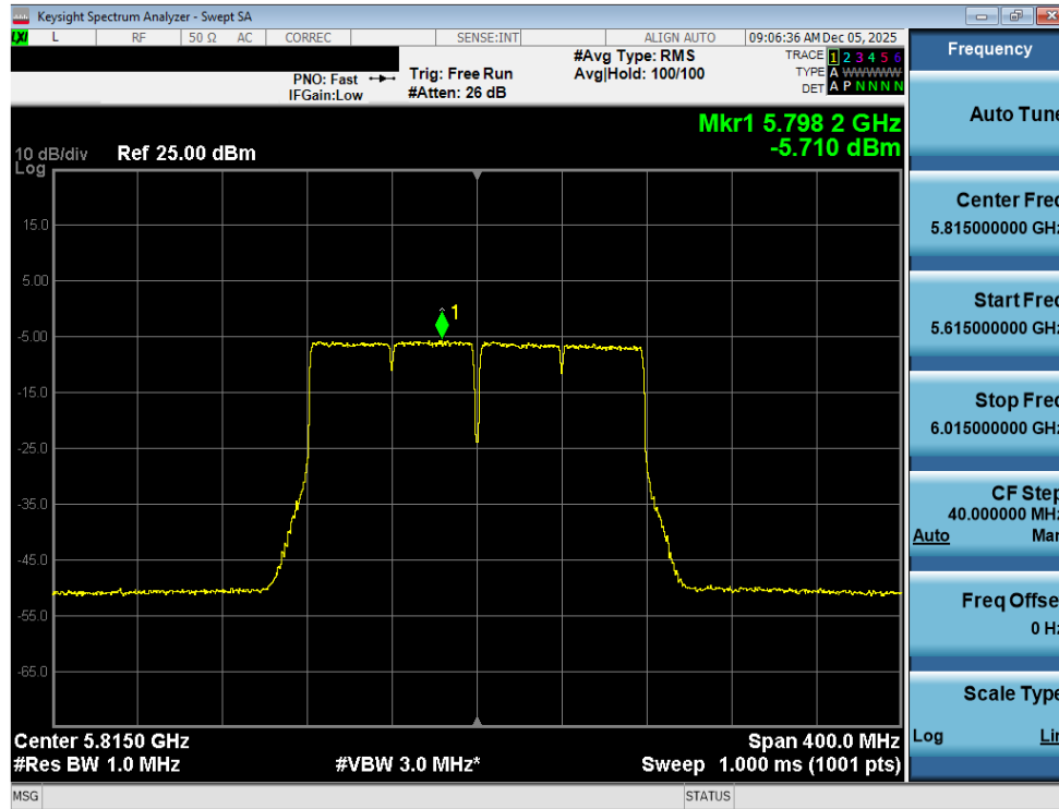
Plot 7-120. Power Spectral Density Plot MIMO ANT2 (160MHz BW 802.11ac (UNII Band 3/4) – Ch. 163)
