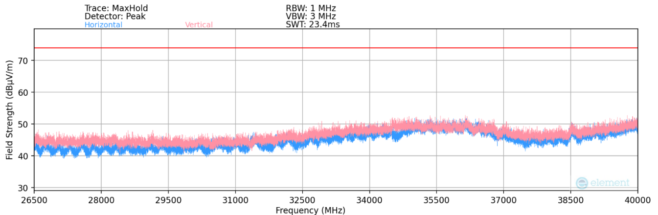
Plot 7-130. Radiated Spurious Plot 26.5GHz – 40GHz MIMO (802.11a)
