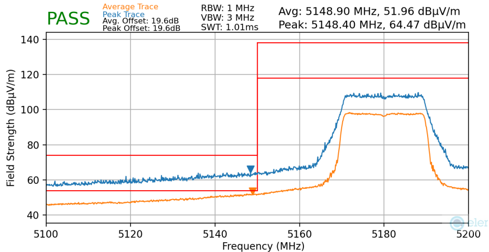
Plot 7-135. Radiated Lower Band Edge Plot MIMO (Average & Peak – UNII Band 1)
