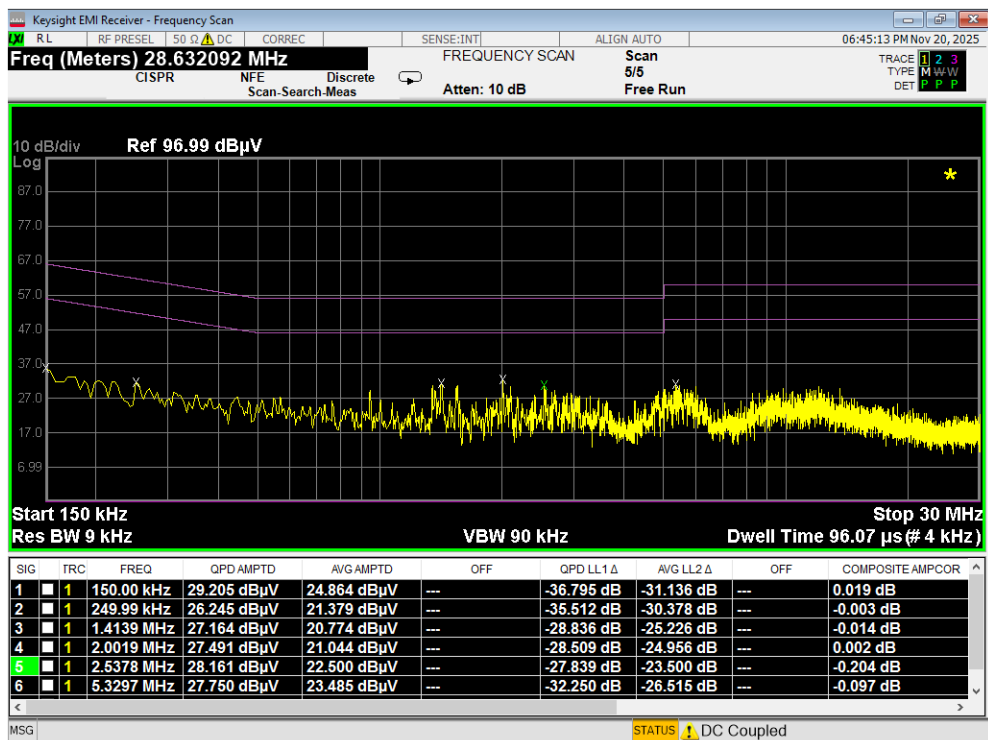
Plot 7-177. Line Conducted Plot with 802.11a UNII Band 3 (N)
