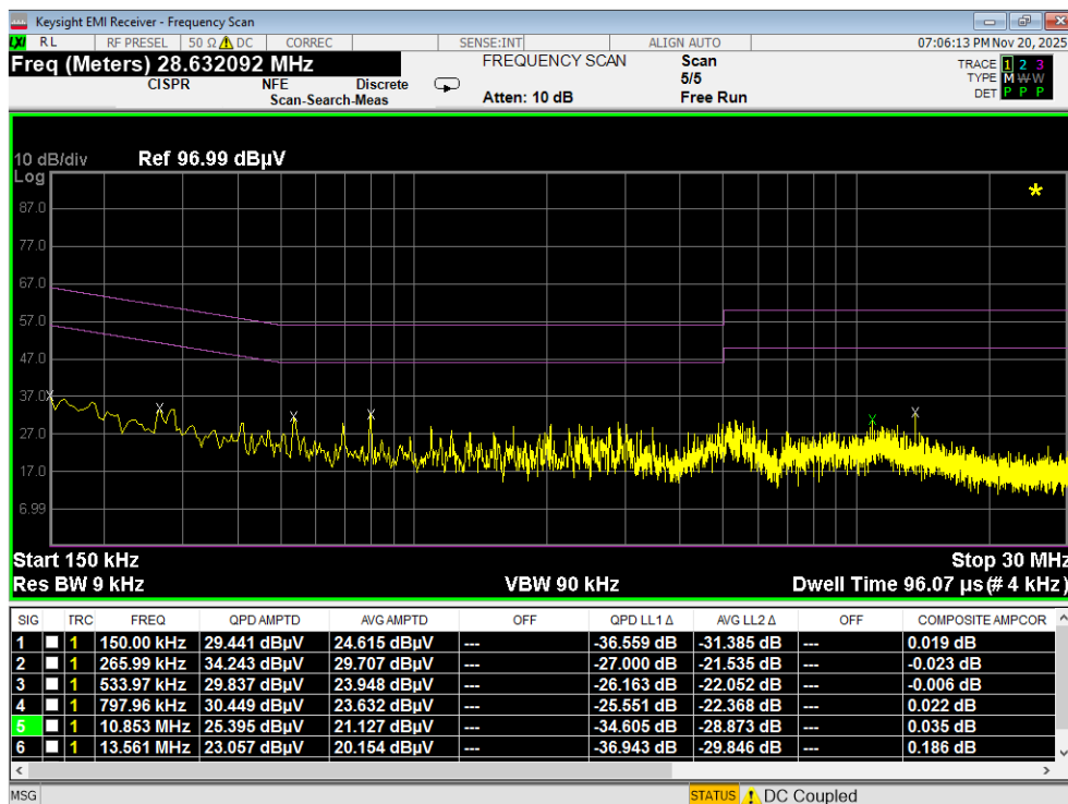
Plot 7-189. Line Conducted Plot with 802.11a UNII Band 4 (N) with WCP
