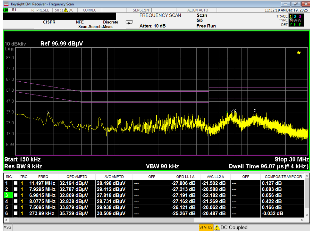
Plot 7-184. Line Conducted Plot with 802.11a UNII Band 2C (L1) with WCP
