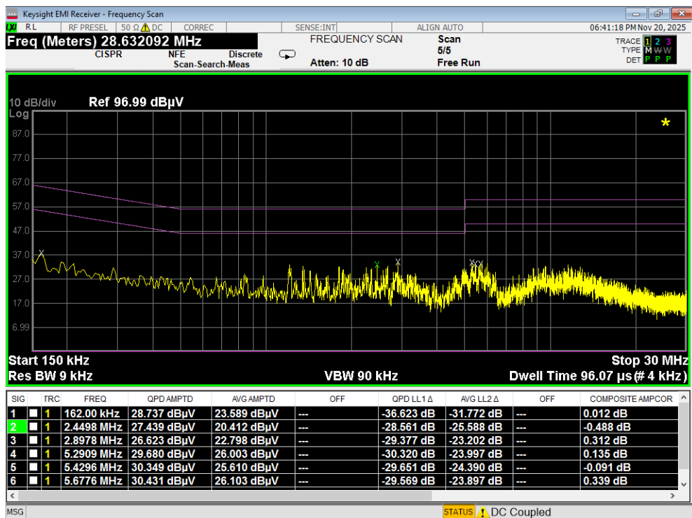
Plot 7-176. Line Conducted Plot with 802.11a UNII Band 3 (L1)
