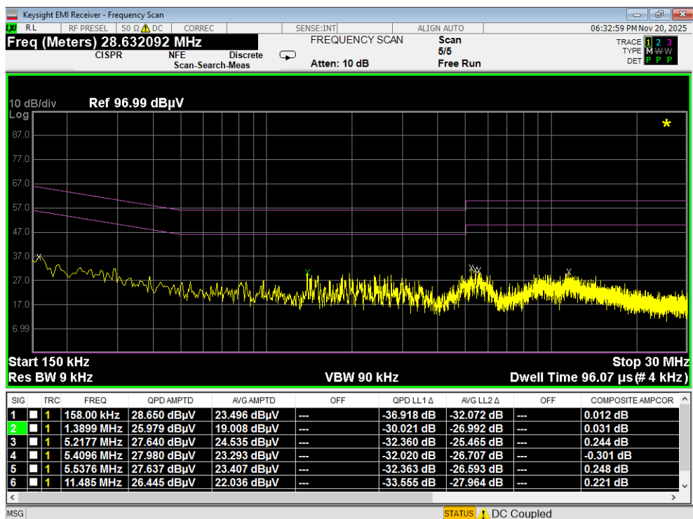
Plot 7-173. Line Conducted Plot with 802.11a UNII Band 2A (N)
