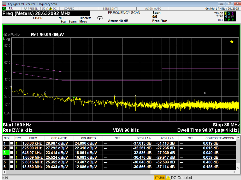
Plot 7-187. Line Conducted Plot with 802.11a UNII Band 3 (N) with WCP
