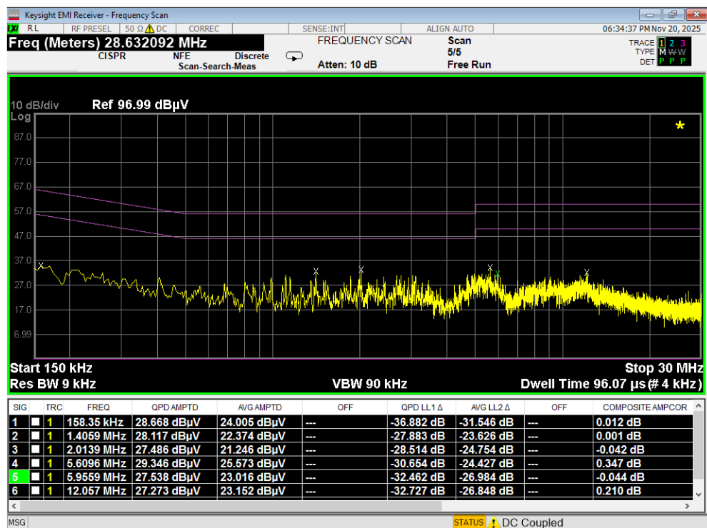
Plot 7-183. Line Conducted Plot with 802.11a UNII Band 2A (N) with WCP
