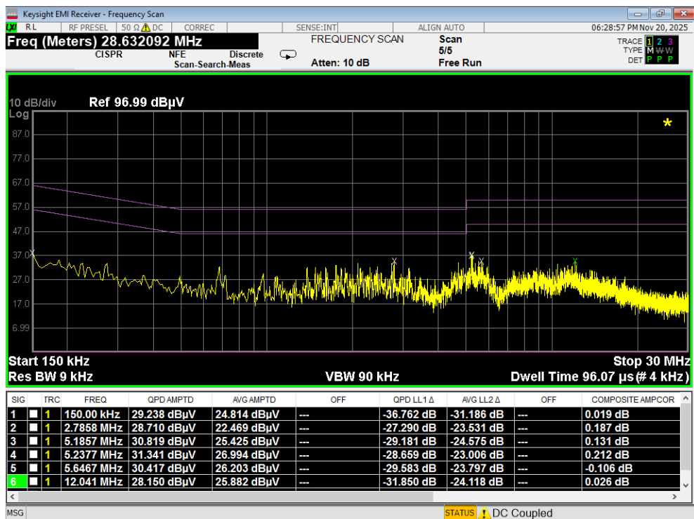
Plot 7-180. Line Conducted Plot with 802.11a UNII Band 1 (L1) with WCP
