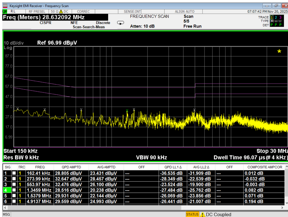
Plot 7-188. Line Conducted Plot with 802.11a UNII Band 4 (L1) with WCP
