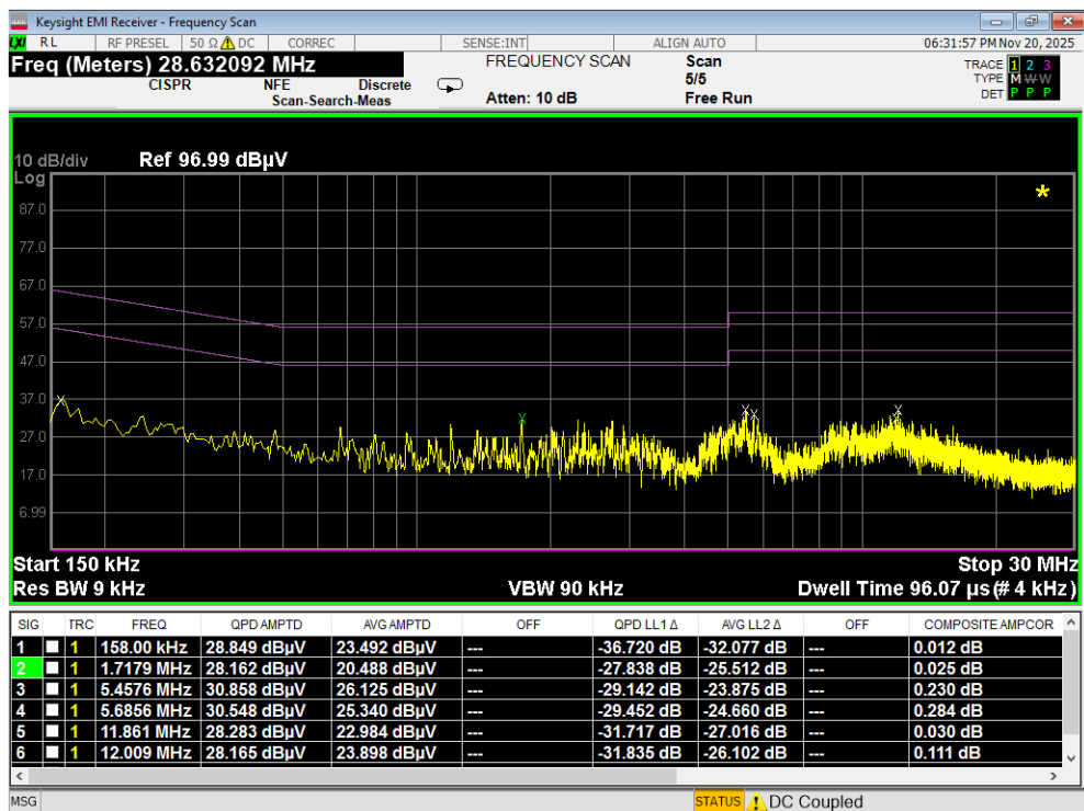
Plot 7-172. Line Conducted Plot with 802.11a UNII Band 2A (L1)
