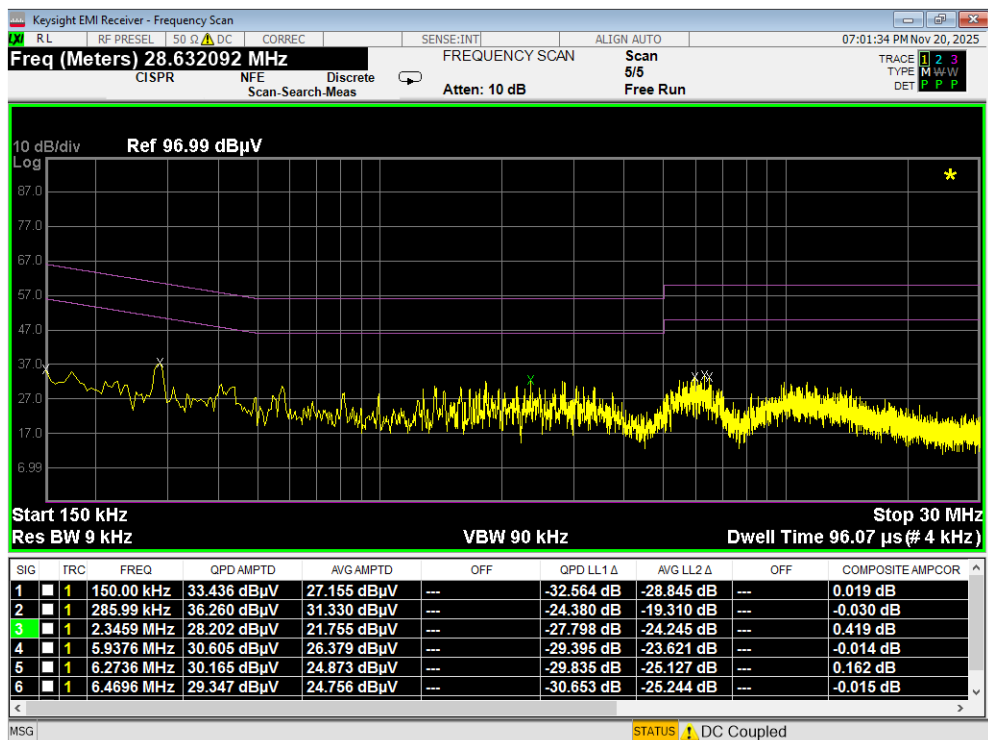
Plot 7-178. Line Conducted Plot with 802.11a UNII Band 4 (L1)
