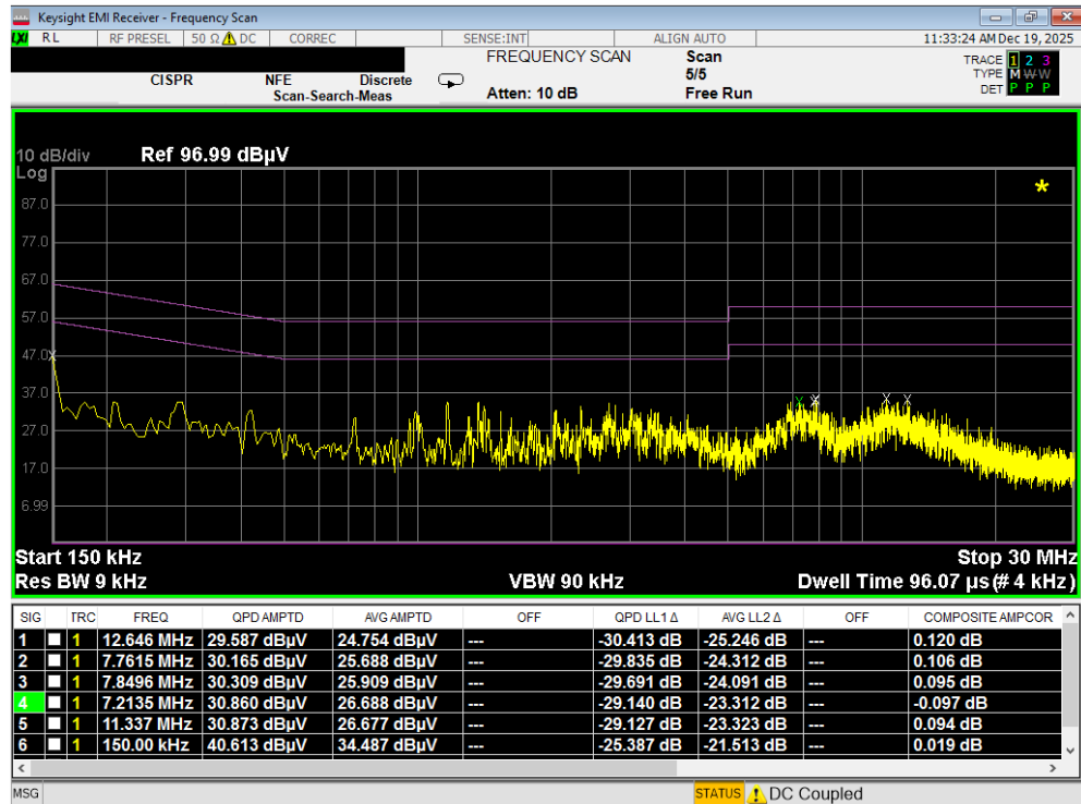
Plot 7-185. Line Conducted Plot with 802.11a UNII Band 2C (N) with WCP
