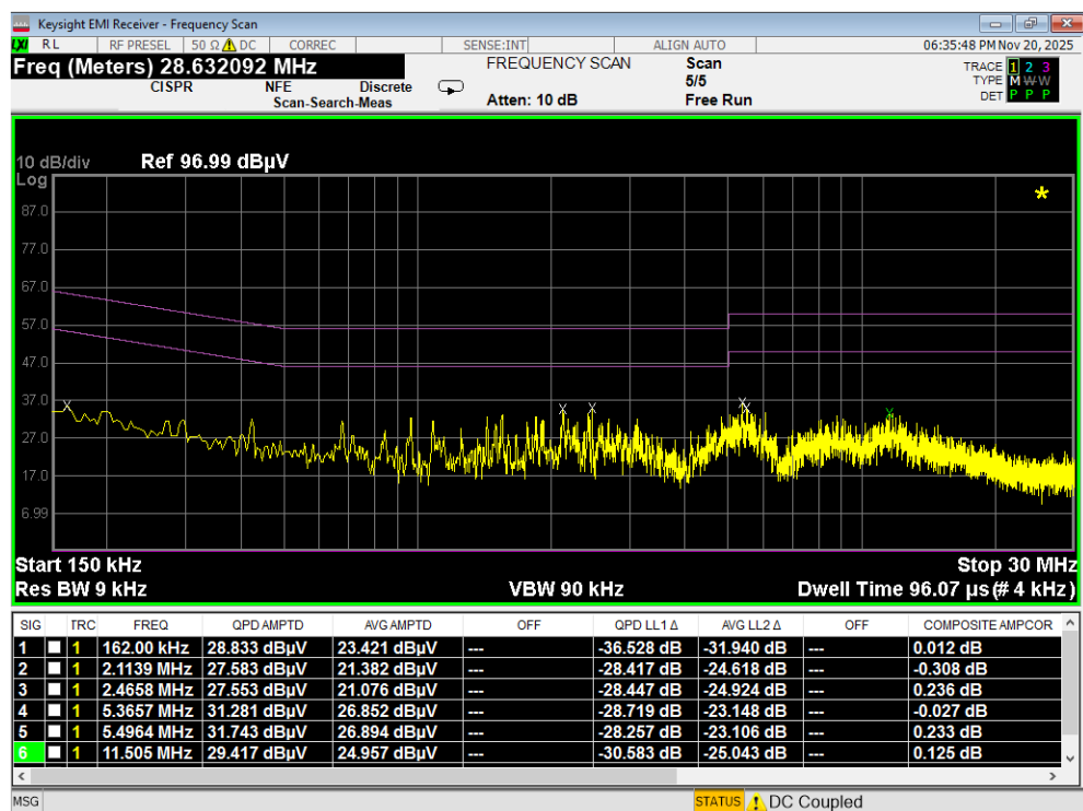
Plot 7-182. Line Conducted Plot with 802.11a UNII Band 2A (L1) with WCP
