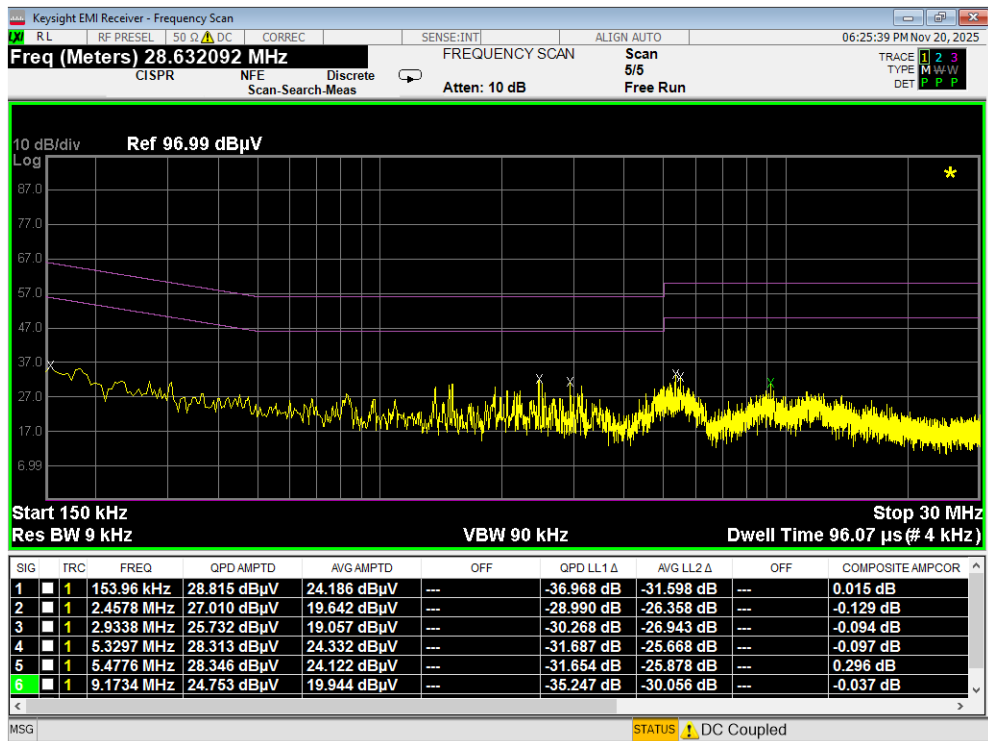
Plot 7-171. Line Conducted Plot with 802.11a UNII Band 1 (N)
