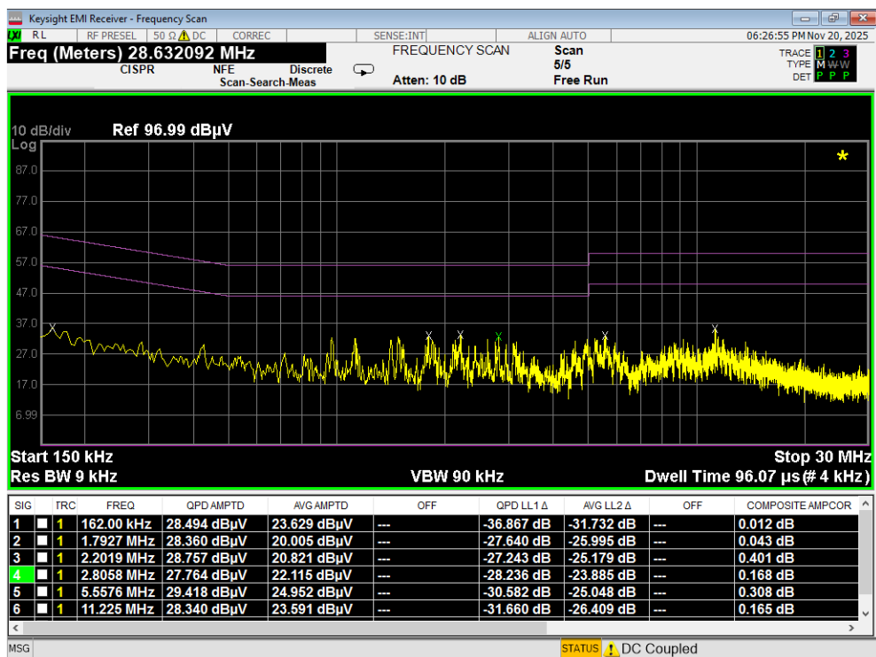
Plot 7-181. Line Conducted Plot with 802.11a UNII Band 1 (N) with WCP
