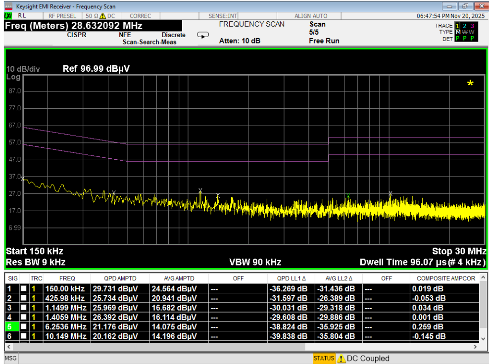
Plot 7-186. Line Conducted Plot with 802.11a UNII Band 3 (L1) with WCP
