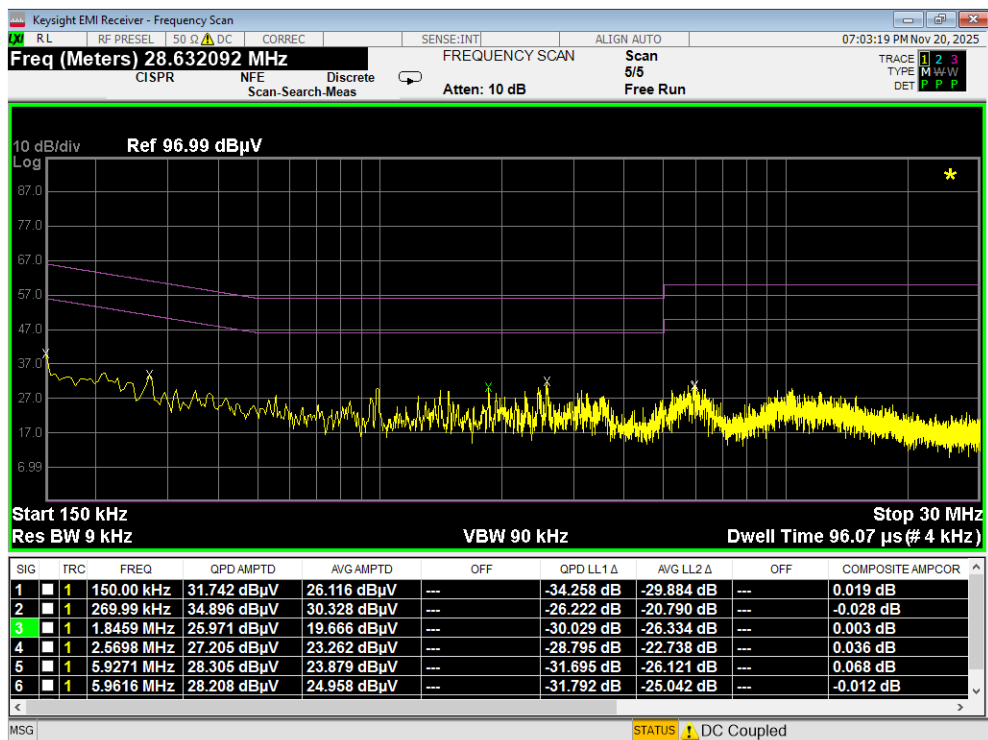
Plot 7-179. Line Conducted Plot with 802.11a UNII Band 4 (N)
