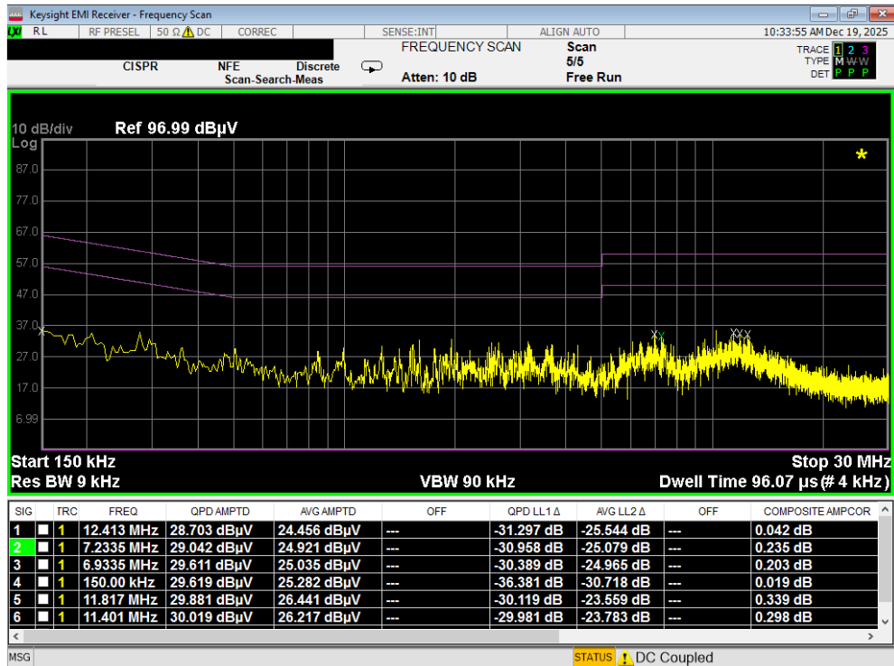
Plot 7-175. Line Conducted Plot with 802.11a UNII Band 2C (N)
