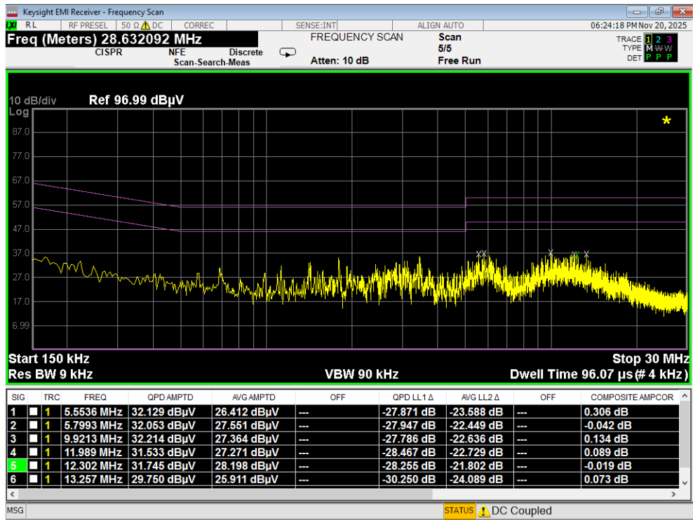
Plot 7-170. Line Conducted Plot with 802.11a UNII Band 1 (L1)
