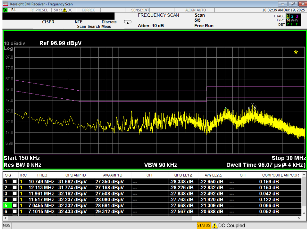
Plot 7-174. Line Conducted Plot with 802.11a UNII Band 2C (L1)
