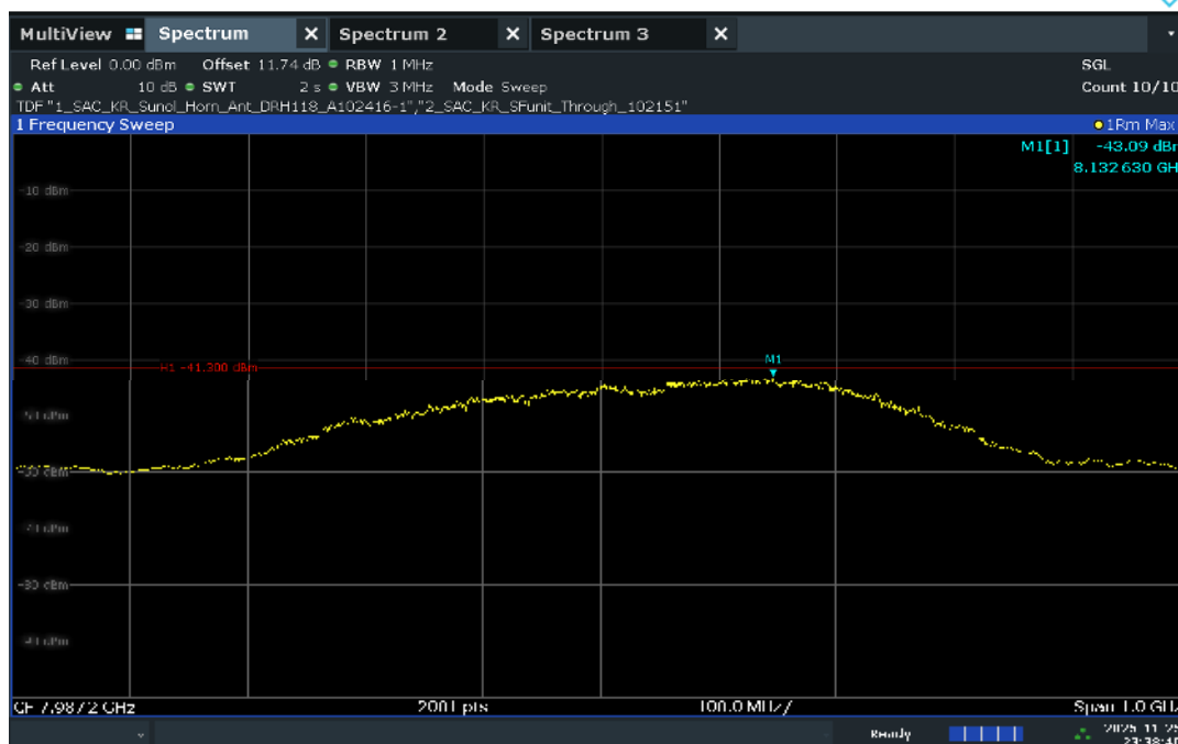
Plot 7-39. UWB Average Power Measurement - CH.9 – HPRF
