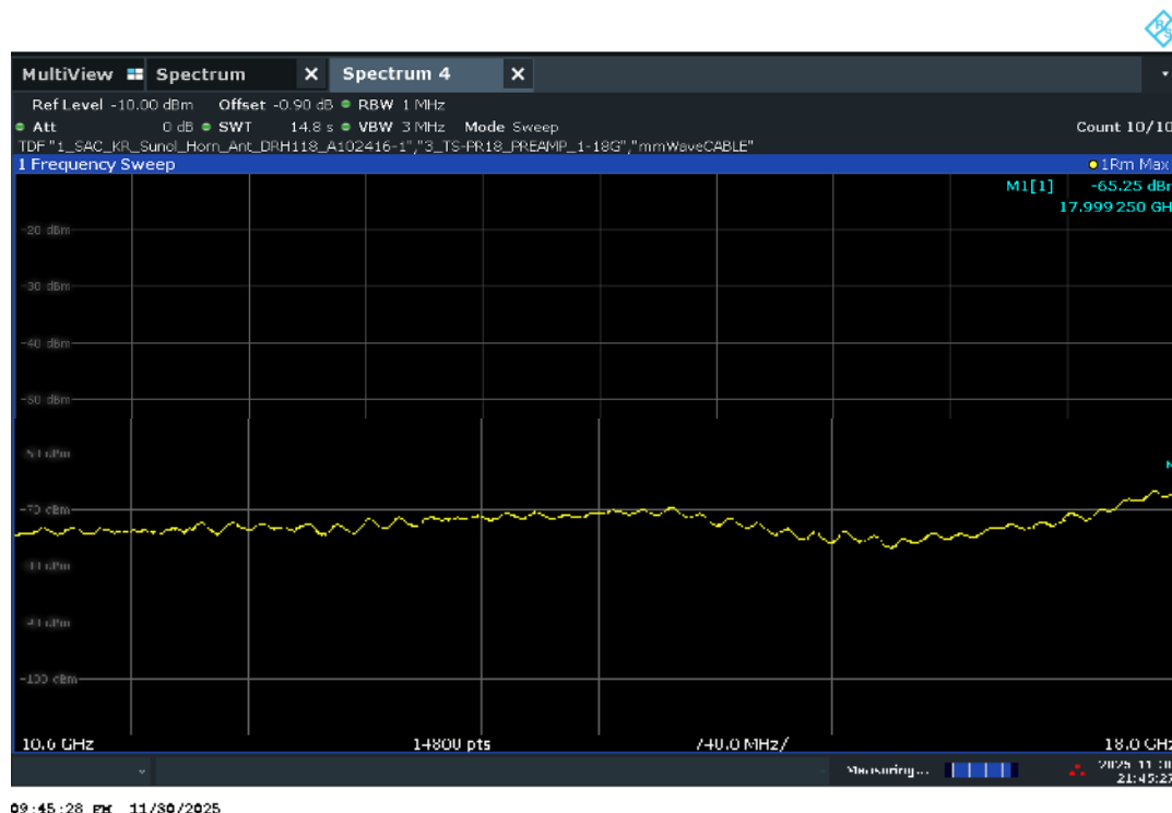
Plot 7-46. Radiated Spurious Pre-Scan 10600 - 18000 MHz - CH.9
