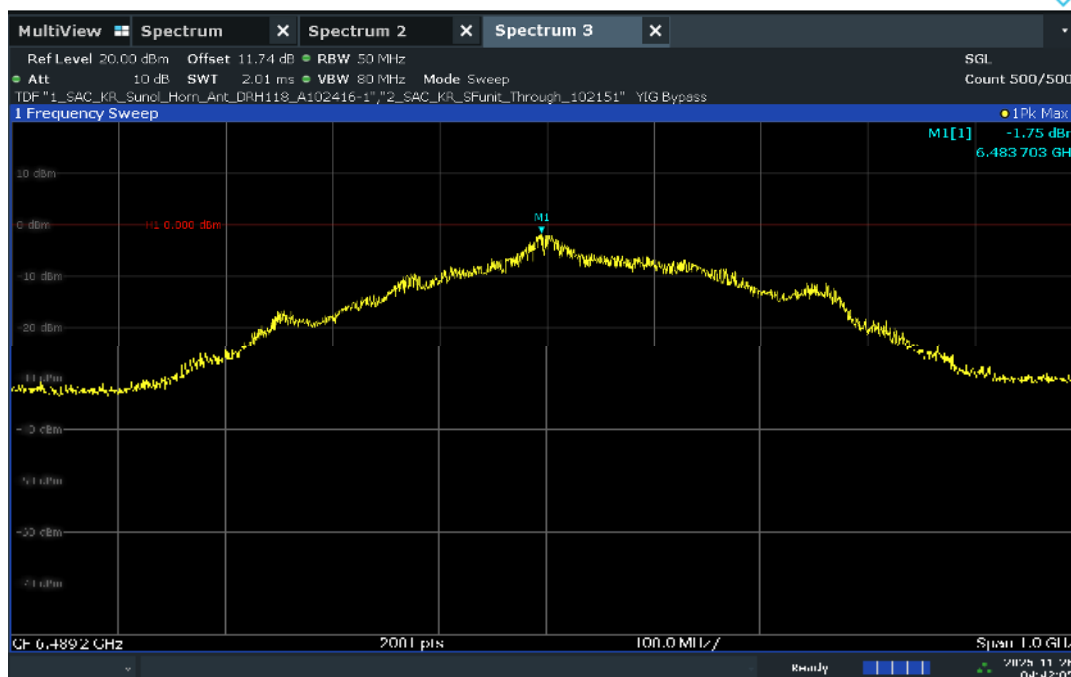
Plot 7-32. UWB Peak Power Measurement - CH.5 – BPRF
