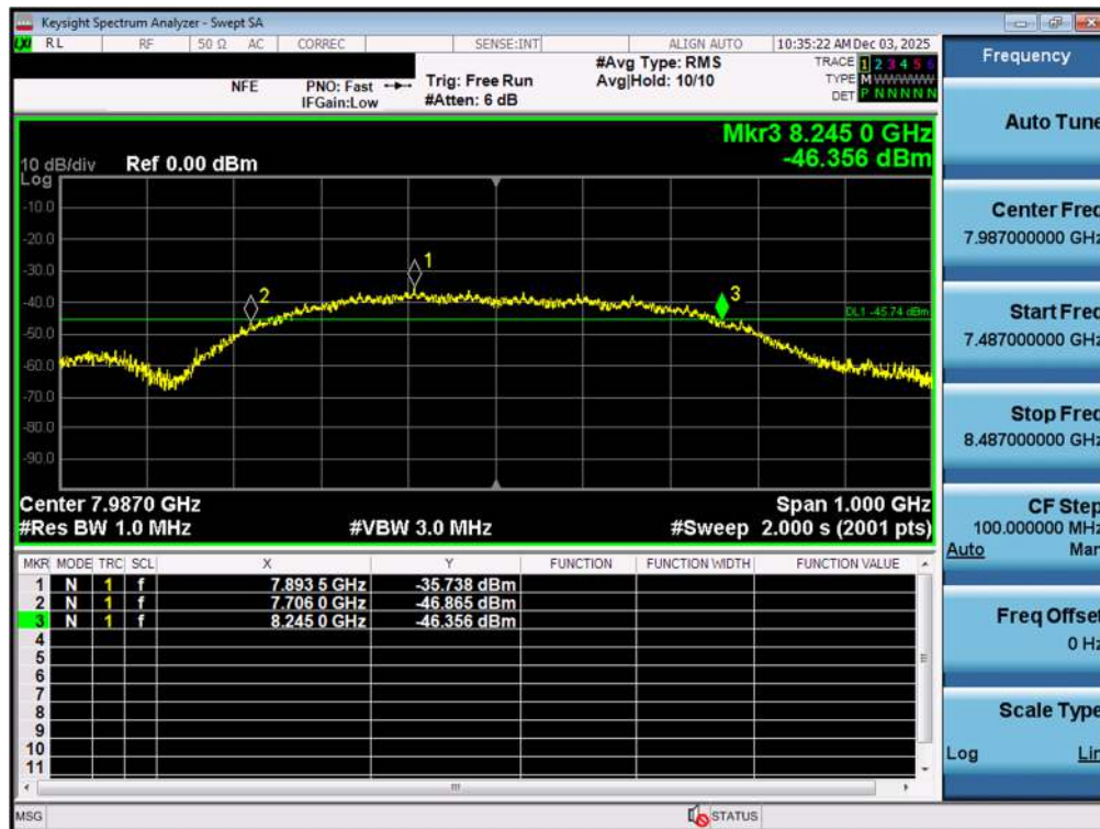
Plot 7-27. 10dBc Bandwidth – CH.9 – SP3 – Preamble 12
