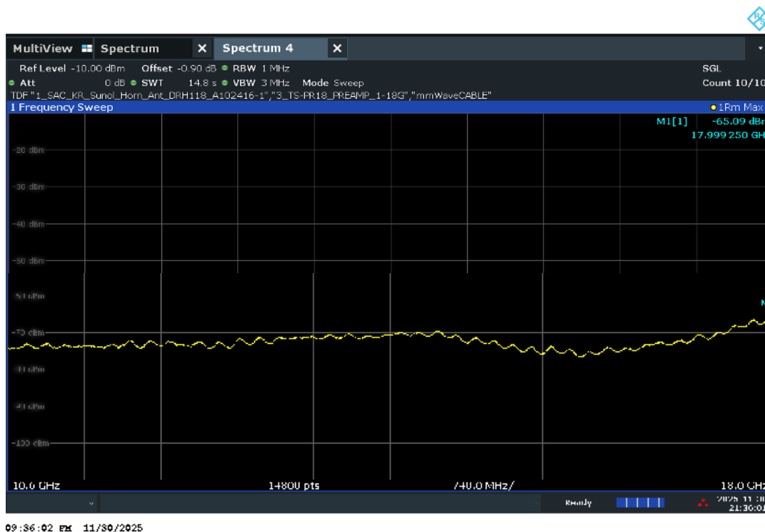
Plot 7-41. Radiated Spurious Pre-Scan 10600 - 18000 MHz - CH.5
