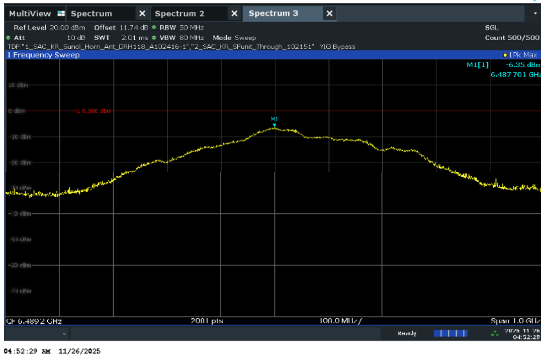
Plot 7-36. UWB Peak Power Measurement - CH.5 – HPRF
