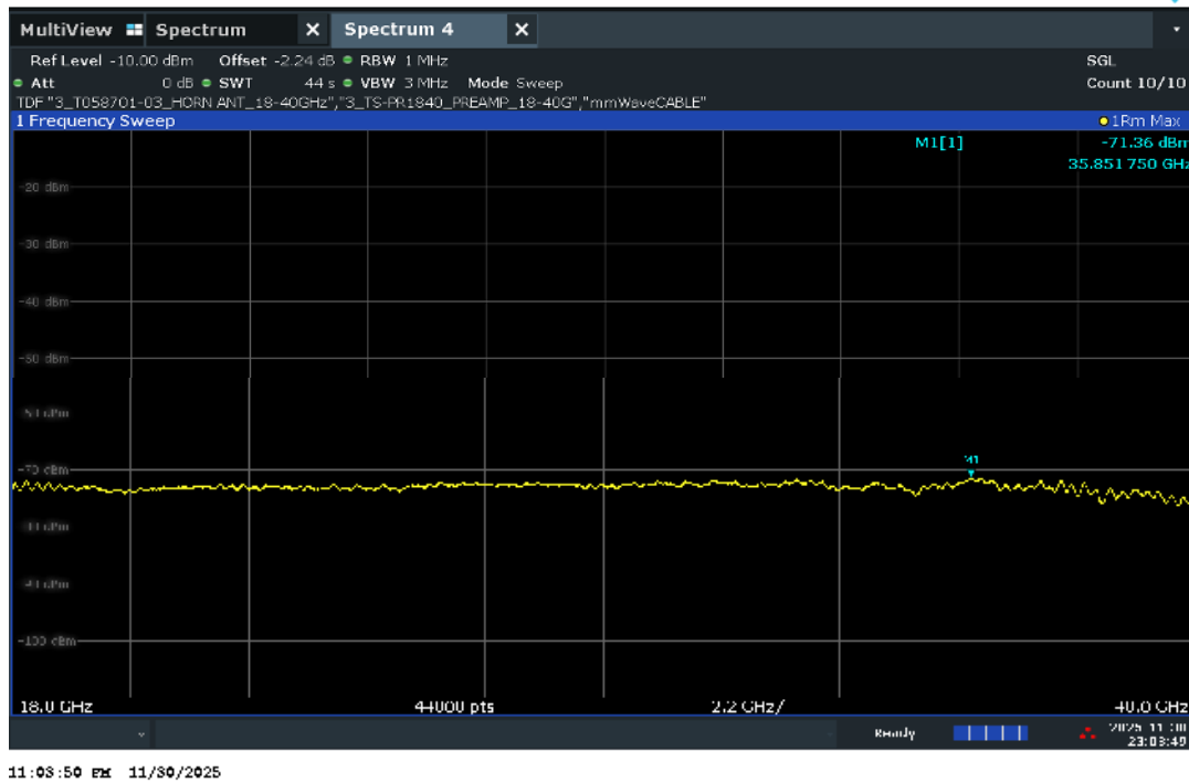
Plot 7-49. Radiated Spurious Pre-Scan 18 – 40 GHz - CH.9
