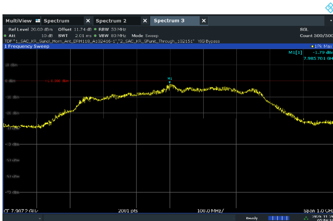
Plot 7-33. UWB Peak Power Measurement - CH.9 – BPRF
