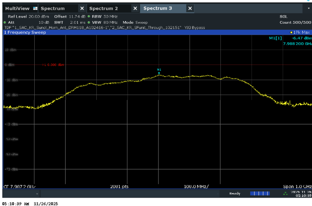
Plot 7-37. UWB Peak Power Measurement - CH.9 – HPRF
