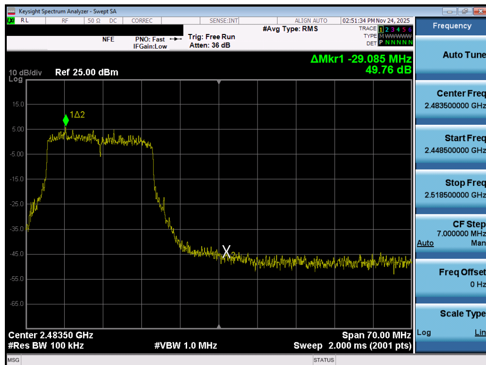
Plot 7-84. Band Edge Plot MIMO ANT2 (802.11ax/be (2.4GHz) – Ch. 11)
