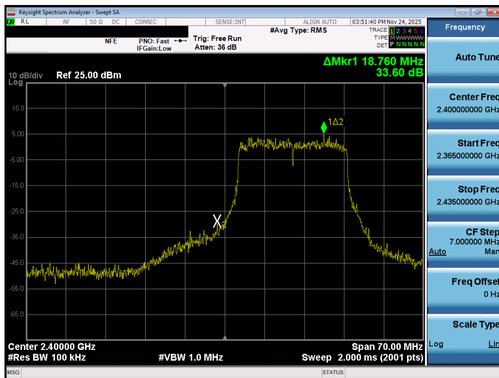
Plot 7-62. Band Edge Plot MIMO ANT1 (802.11ax/be (2.4GHz) – Ch. 1)
