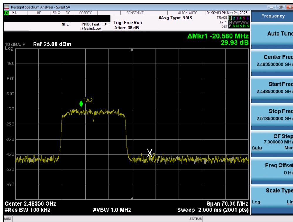
Plot 7-67. Band Edge Plot MIMO ANT1 (802.11ax/be (2.4GHz) – Ch. 13)
