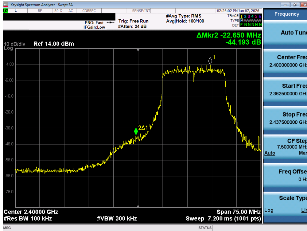
Plot 7-63. Band Edge Plot MIMO ANT1 (802.11ax/be (2.4GHz) – Ch. 2)
