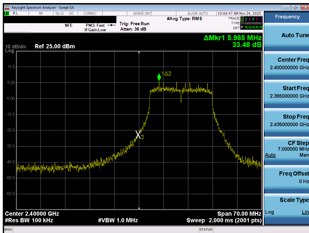
Plot 7-57. Band Edge Plot MIMO ANT1 (802.11n/ac (2.4GHz) – Ch. 1)
