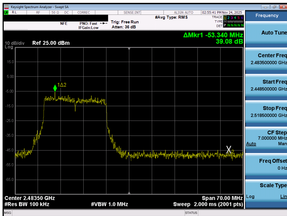
Plot 7-85. Band Edge Plot MIMO ANT2 (802.11ax/be (2.4GHz) – Ch. 12)
