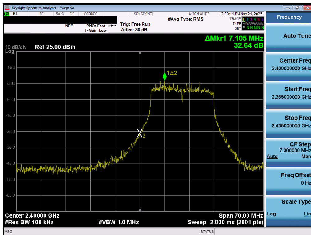
Plot 7-76. Band Edge Plot MIMO ANT2 (802.11n/ac (2.4GHz) – Ch. 1)
