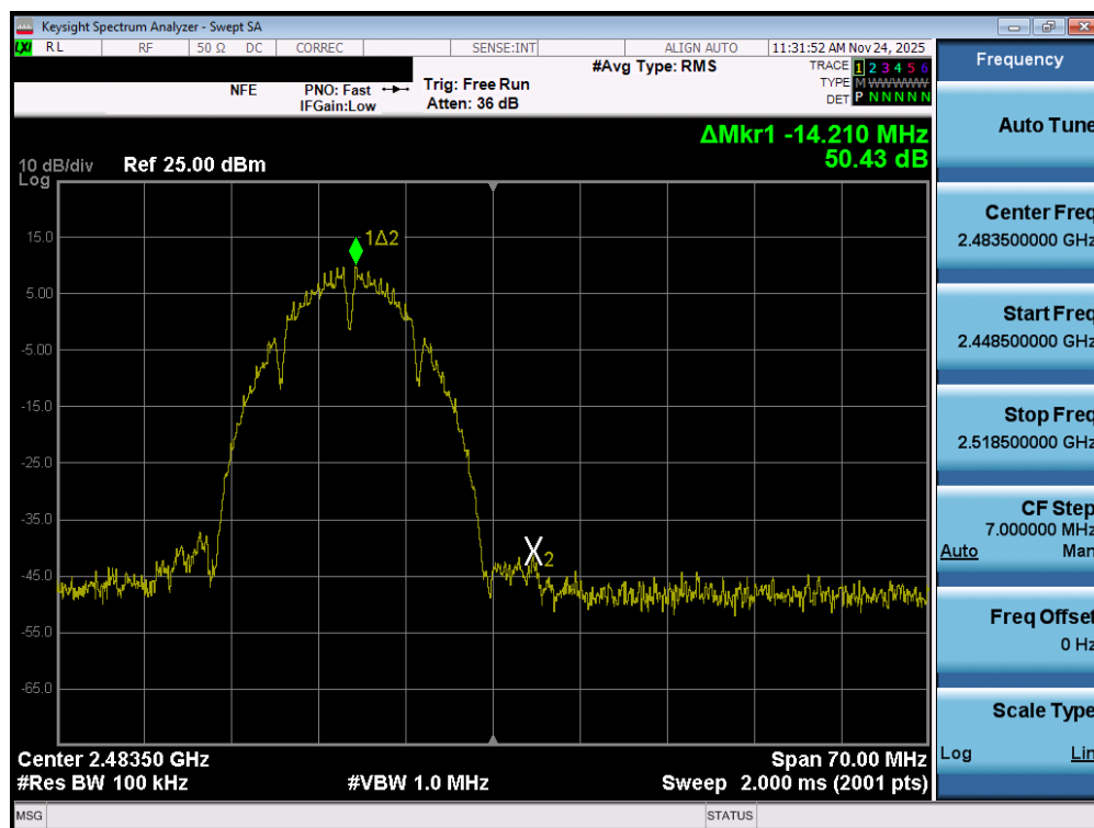
Plot 7-71. Band Edge Plot MIMO ANT2 (802.11b – Ch. 13)
