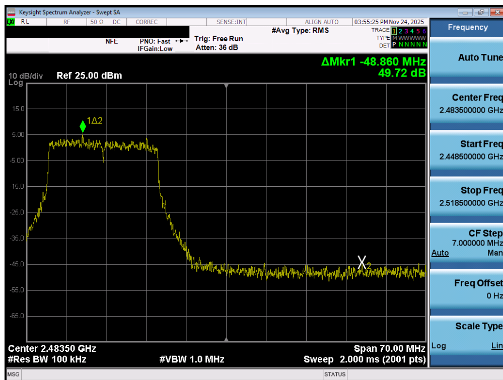
Plot 7-65. Band Edge Plot MIMO ANT1 (802.11ax/be (2.4GHz) – Ch. 11)
