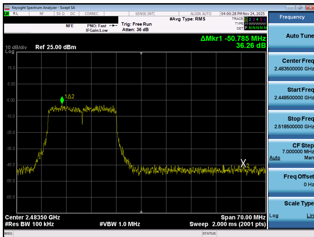
Plot 7-66. Band Edge Plot MIMO ANT1 (802.11ax/be (2.4GHz) – Ch. 12)
