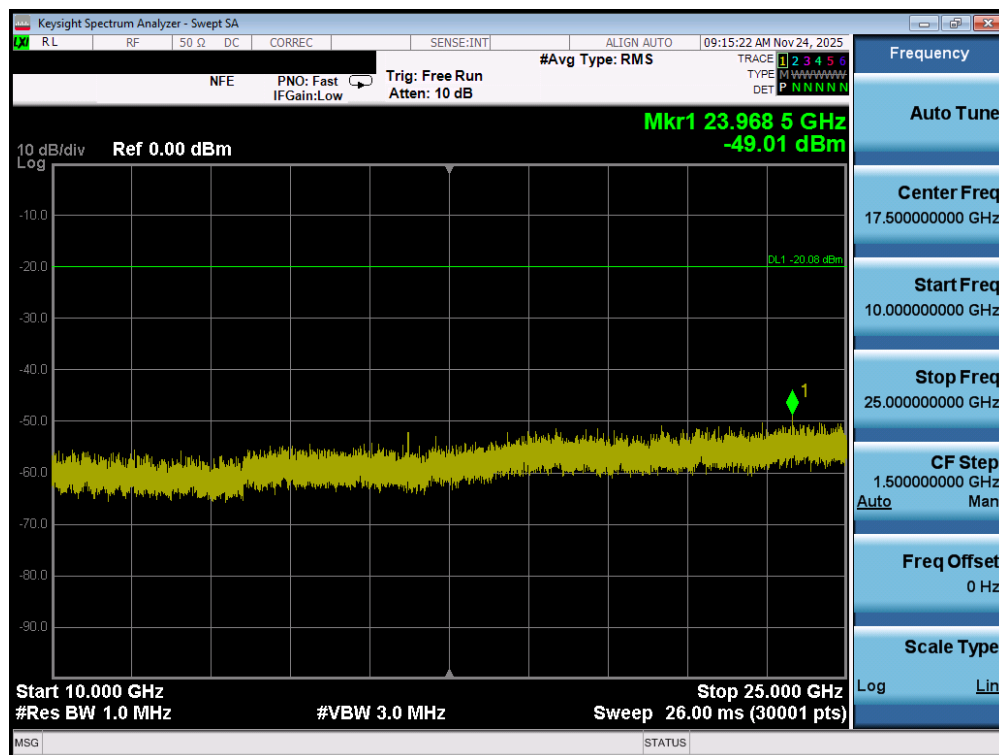
Plot 7-88. Conducted Spurious Plot MIMO ANT1 (802.11b – Ch. 1)
