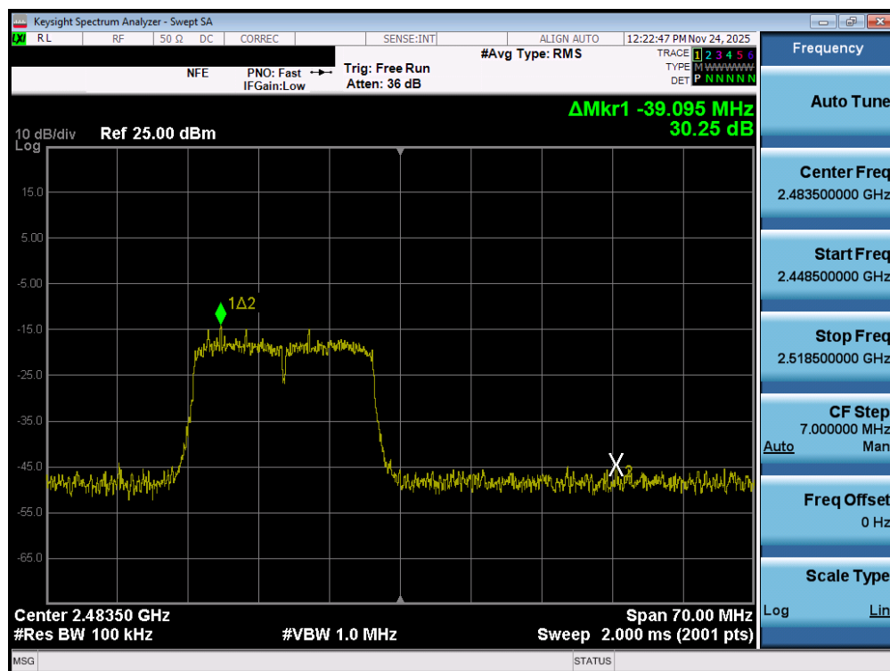
Plot 7-80. Band Edge Plot MIMO ANT2 (802.11n/ac (2.4GHz) – Ch. 13)
