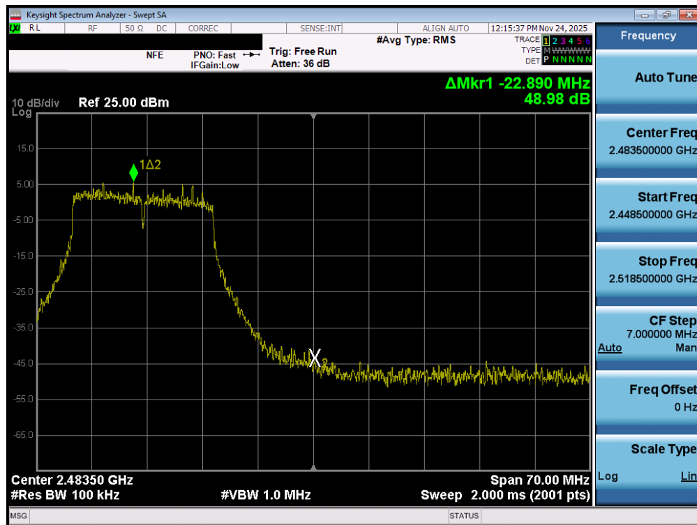
Plot 7-78. Band Edge Plot MIMO ANT2 (802.11n/ac (2.4GHz) – Ch. 11)
