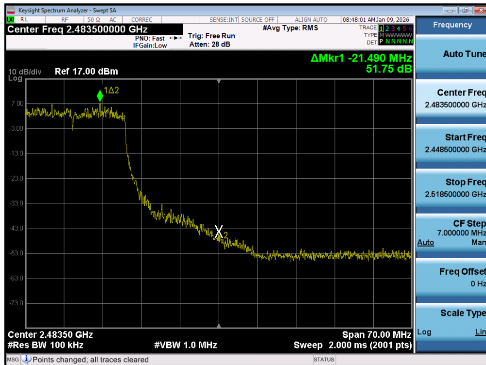
Plot 7-64. Band Edge Plot MIMO ANT1 (802.11ax/be (2.4GHz) – Ch. 10)
