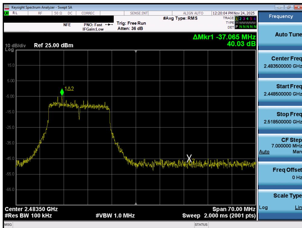
Plot 7-79. Band Edge Plot MIMO ANT2 (802.11n/ac (2.4GHz) – Ch. 12)
