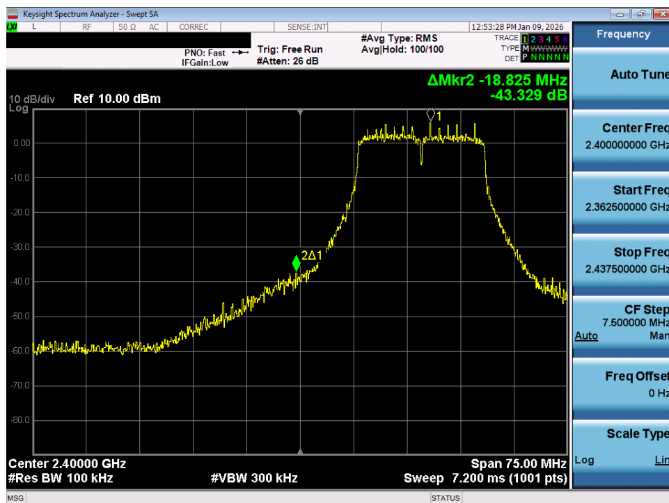
Plot 7-58. Band Edge Plot MIMO ANT1 (802.11n/ac (2.4GHz) – Ch. 2)
