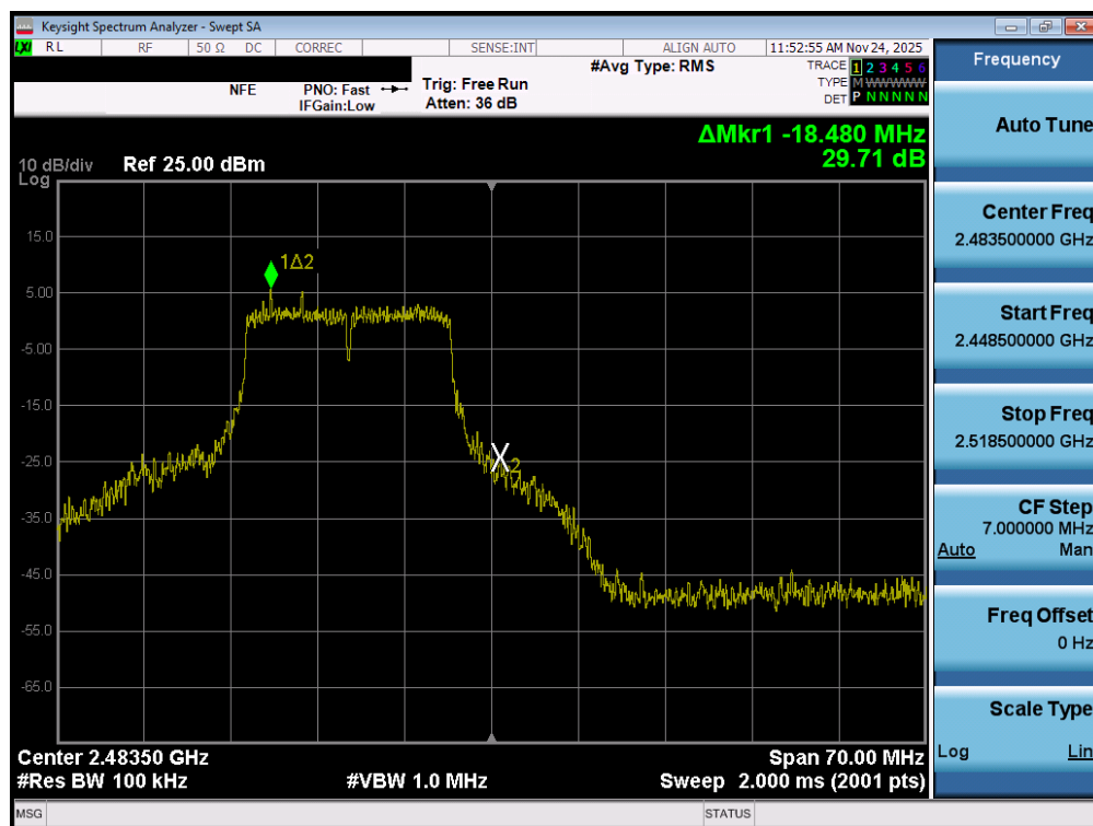
Plot 7-75. Band Edge Plot MIMO ANT2 (802.11g – Ch. 13)
