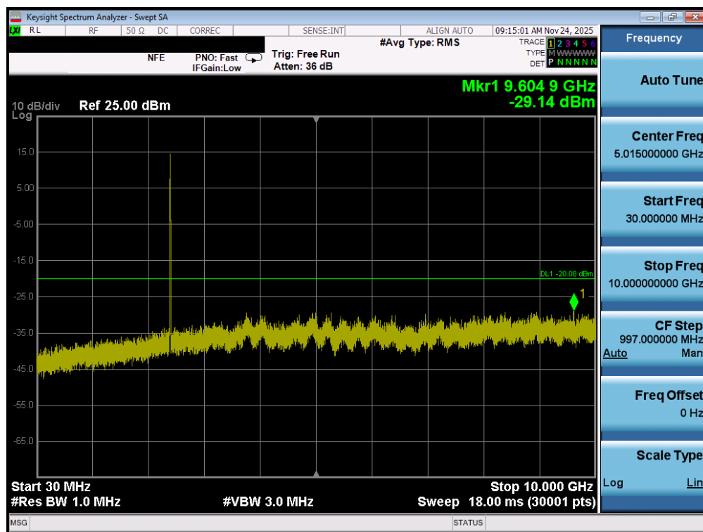
Plot 7-87. Conducted Spurious Plot MIMO ANT1 (802.11b – Ch. 1)
