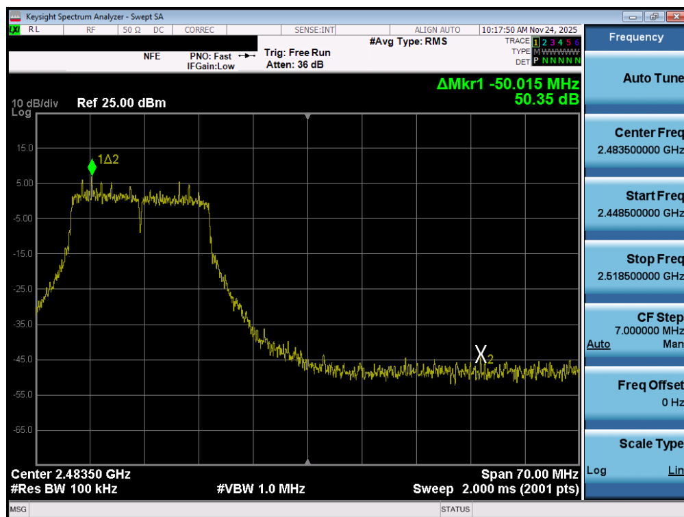
Plot 7-59. Band Edge Plot MIMO ANT1 (802.11n/ac (2.4GHz) – Ch. 11)
