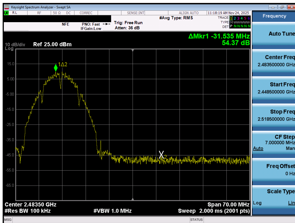
Plot 7-69. Band Edge Plot MIMO ANT2 (802.11b – Ch. 11)
