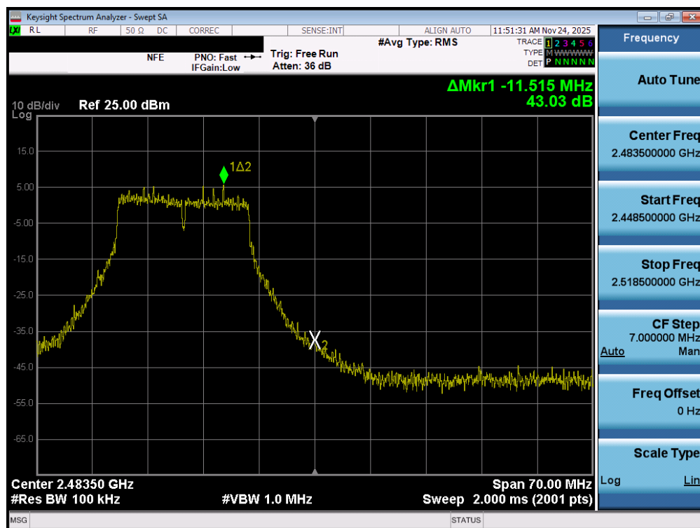
Plot 7-74. Band Edge Plot MIMO ANT2 (802.11g – Ch. 12)
