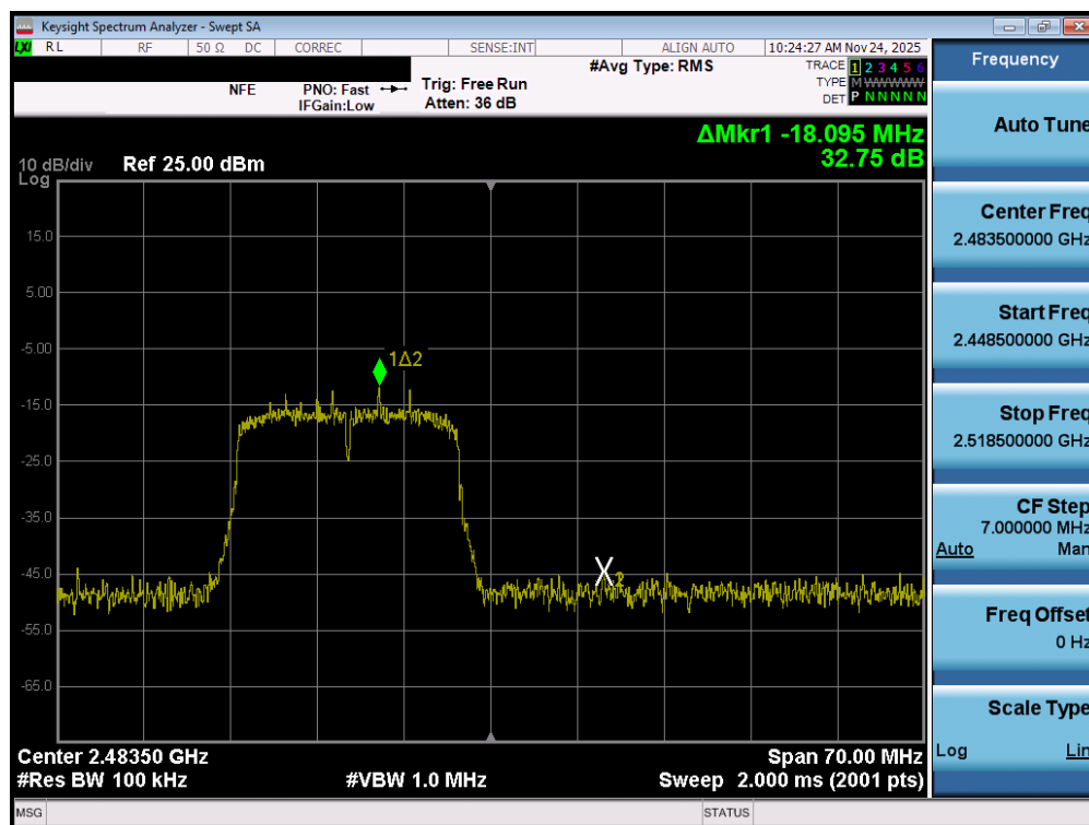
Plot 7-61. Band Edge Plot MIMO ANT1 (802.11n/ac (2.4GHz) – Ch. 13)
