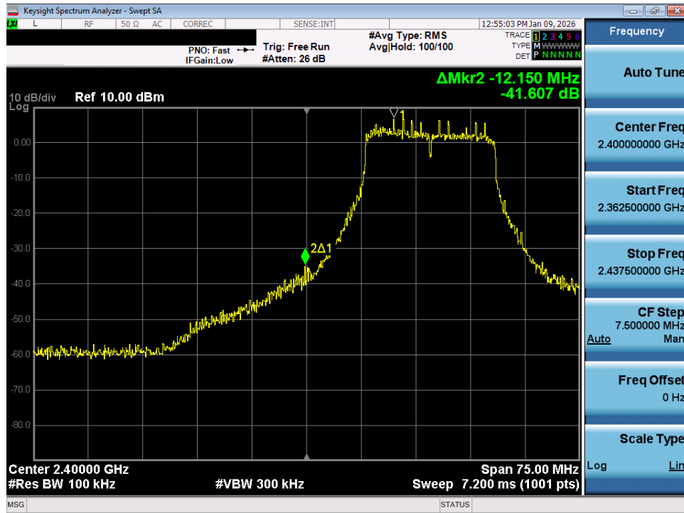
Plot 7-77. Band Edge Plot MIMO ANT2 (802.11n/ac (2.4GHz) – Ch. 2)
