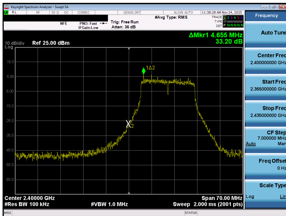
Plot 7-72. Band Edge Plot MIMO ANT2 (802.11g– Ch. 1)
