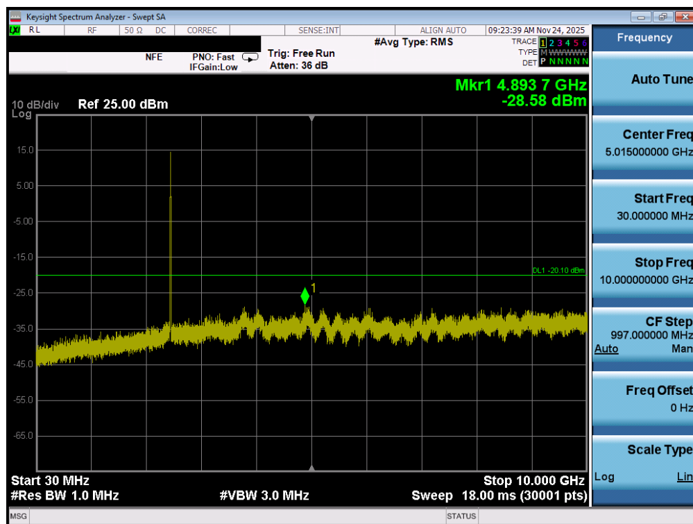
Plot 7-91. Conducted Spurious Plot MIMO ANT1 (802.11b – Ch. 11)
