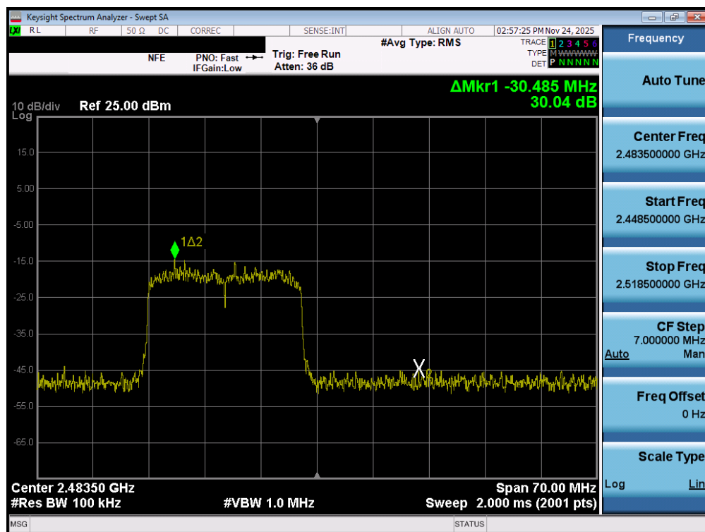
Plot 7-86. Band Edge Plot MIMO ANT2 (802.11ax/be (2.4GHz) – Ch. 13)
