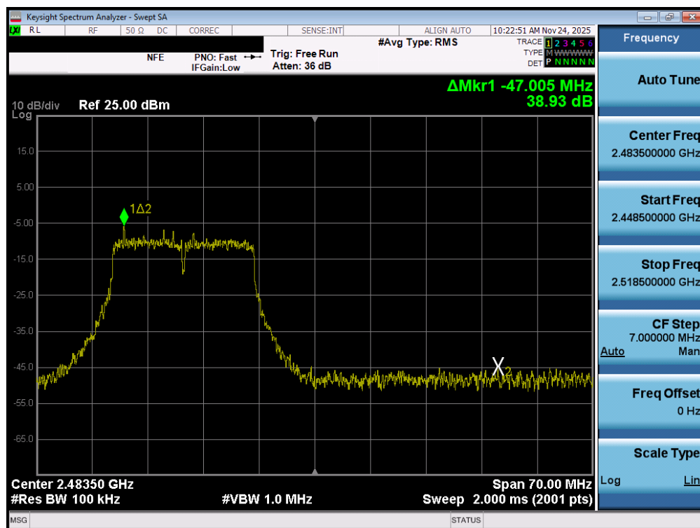
Plot 7-60. Band Edge Plot MIMO ANT1 (802.11n/ac (2.4GHz) – Ch. 12)
