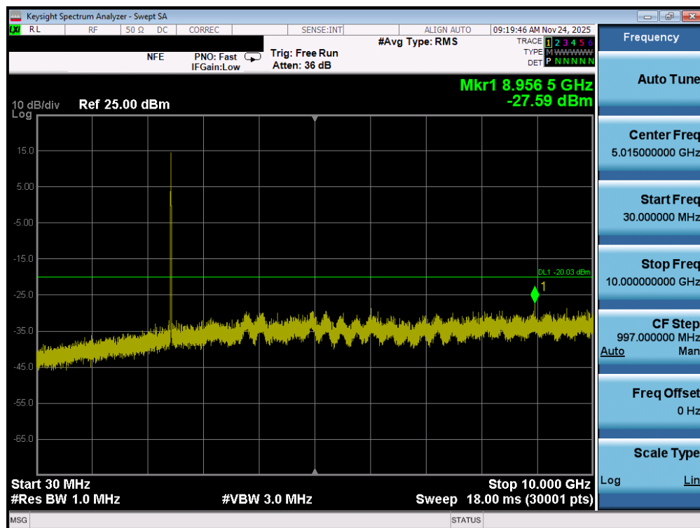
Plot 7-89. Conducted Spurious Plot MIMO ANT1 (802.11b – Ch. 6)
