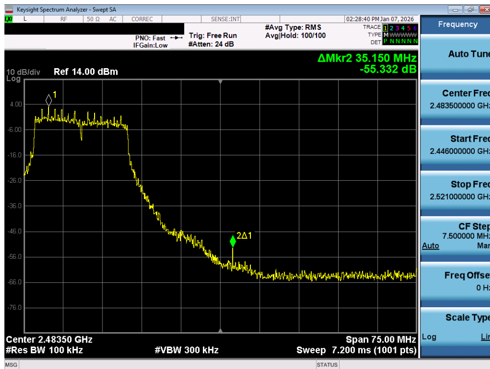
Plot 7-83. Band Edge Plot MIMO ANT2 (802.11ax/be (2.4GHz) – Ch. 10)
