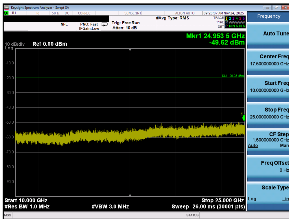
Plot 7-90. Conducted Spurious Plot MIMO ANT1 (802.11b – Ch. 6)
