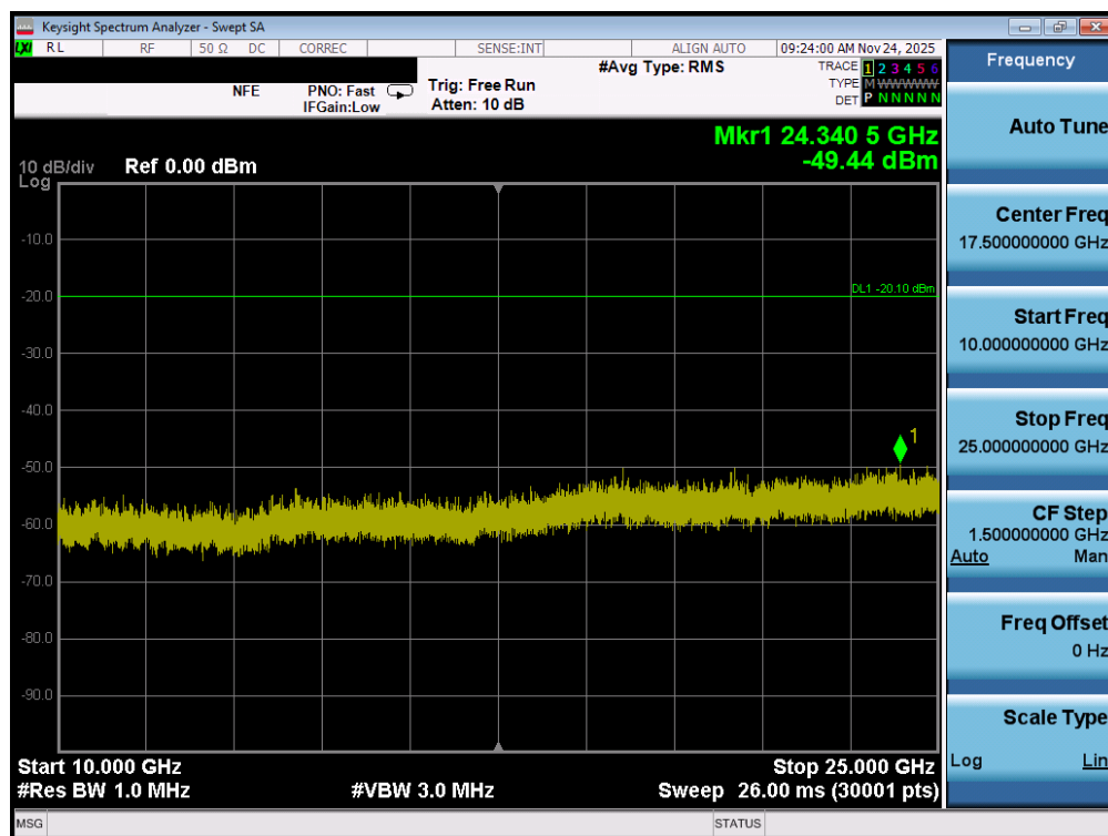
Plot 7-92. Conducted Spurious Plot MIMO ANT1 (802.11b – Ch. 11)
