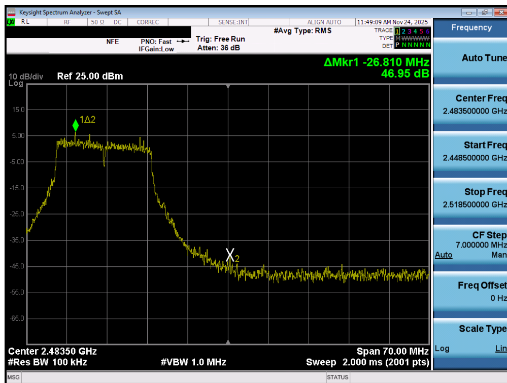
Plot 7-73. Band Edge Plot MIMO ANT2 (802.11g – Ch. 11)
