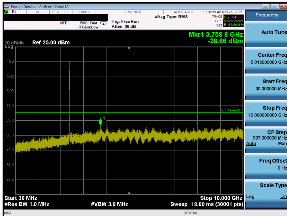
Plot 7-93. Conducted Spurious Plot MIMO ANT2 (802.11b – Ch. 1)
