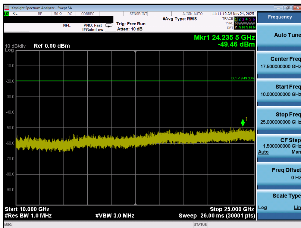
Plot 7-94. Conducted Spurious Plot MIMO ANT2 (802.11b – Ch. 1)
