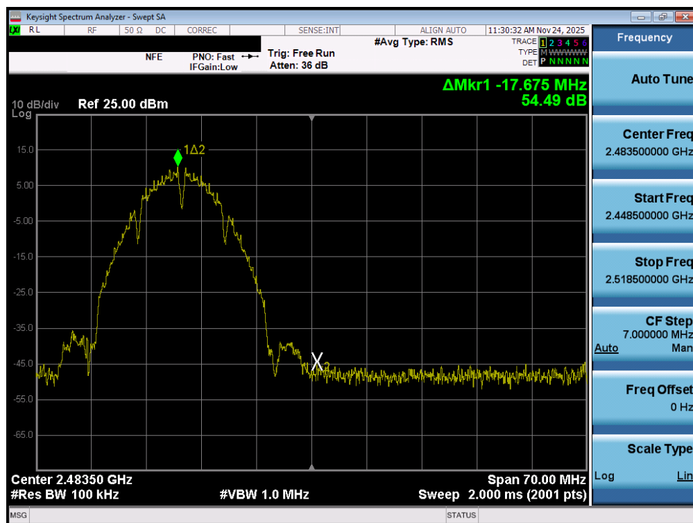
Plot 7-70. Band Edge Plot MIMO ANT2 (802.11b – Ch. 12)
