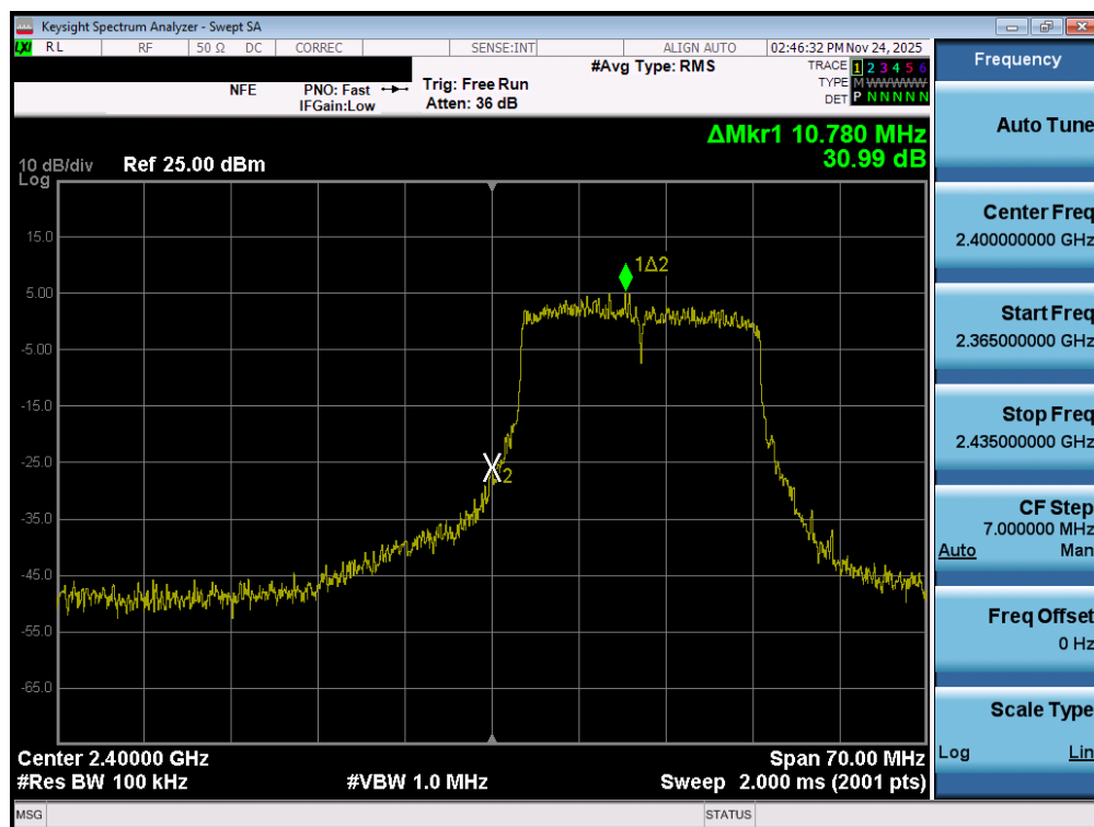
Plot 7-81. Band Edge Plot MIMO ANT2 (802.11ax/be (2.4GHz) – Ch. 1)
