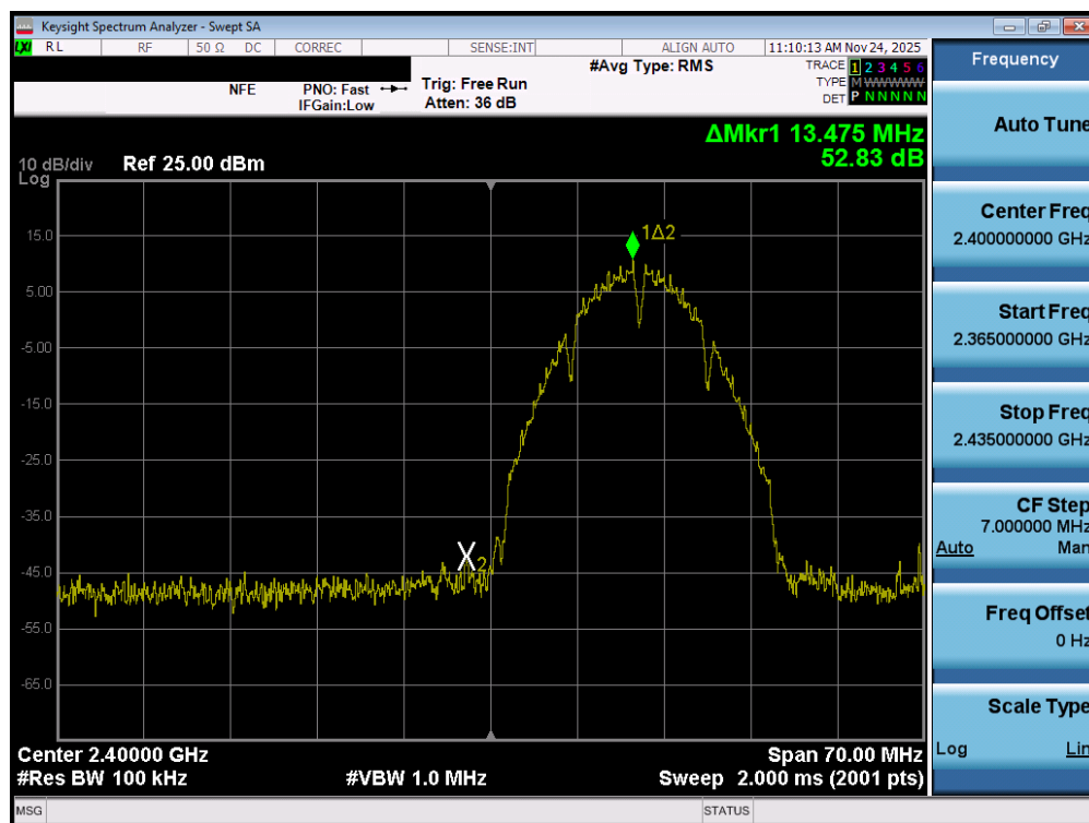
Plot 7-68. Band Edge Plot MIMO ANT2 (802.11b – Ch. 1)
