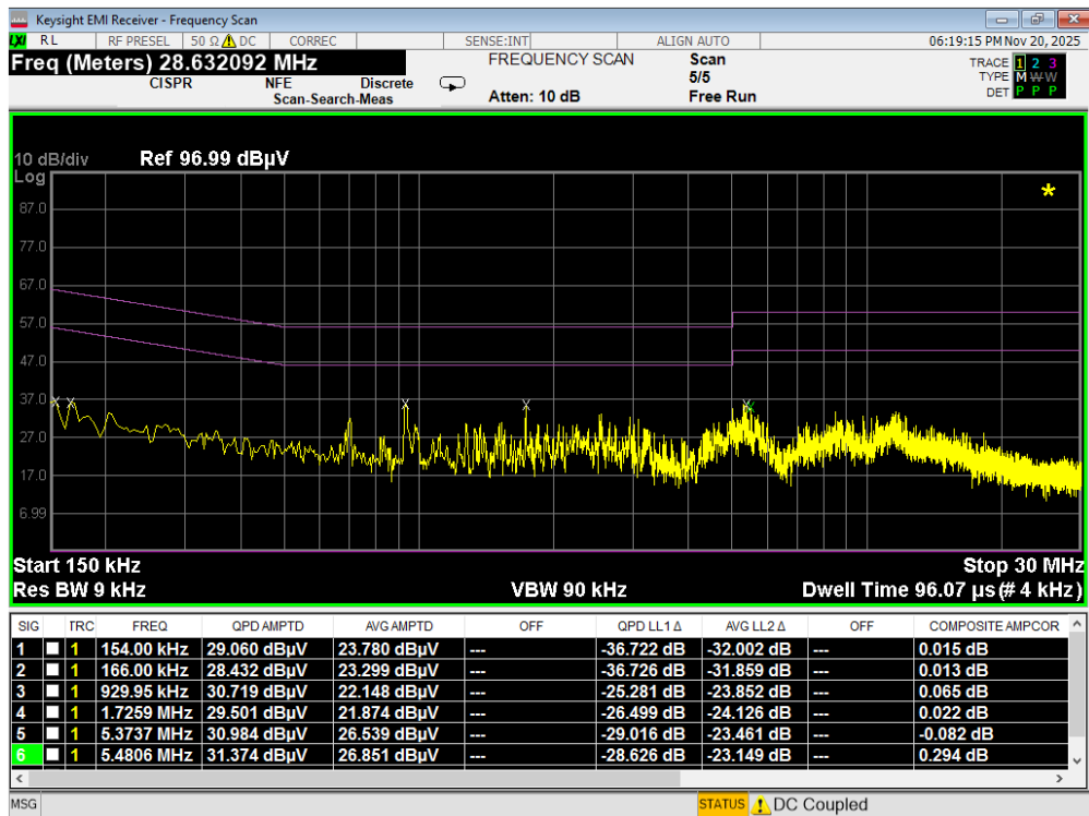
Plot 7-114. Line Conducted Plot with 802.11b (L1) – WCP
