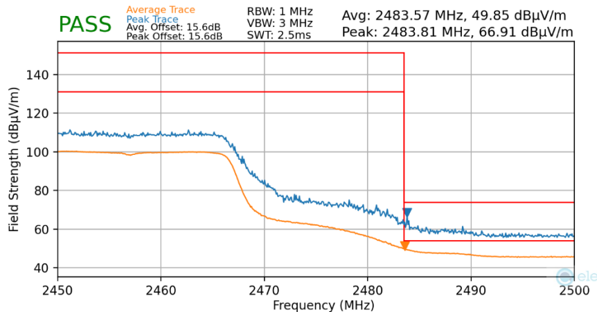
Plot 7-106. Radiated Restricted Upper Band Edge Measurement MIMO (Average & Peak)
