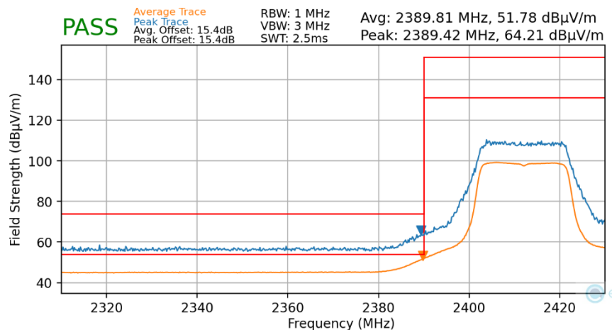
Plot 7-104. Radiated Restricted Lower Band Edge Measurement MIMO (Average & Peak)
