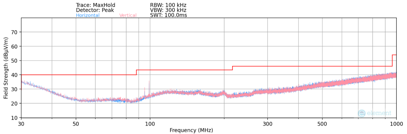
Plot 7-99. Radiated Spurious Plot below 1GHz MIMO
