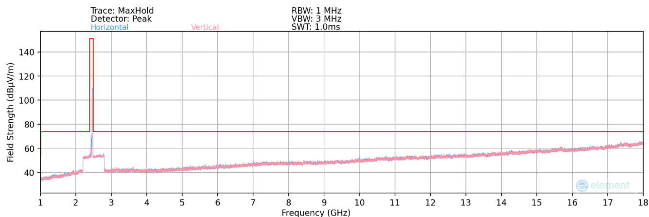
Plot 7-102. Radiated Spurious Plot above 1GHz MIMO (802.11b – Ch. 11)
