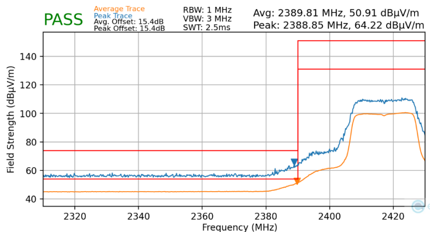
Plot 7-105. Radiated Restricted Lower Band Edge Measurement MIMO (Average & Peak)
