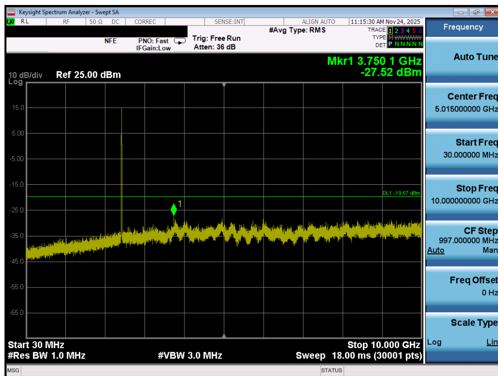
Plot 7-95. Conducted Spurious Plot MIMO ANT2 (802.11b – Ch. 6)
