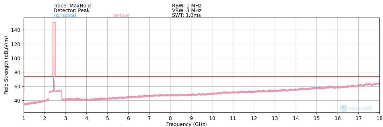
Plot 7-101. Radiated Spurious Plot above 1GHz MIMO (802.11b – Ch. 6)
