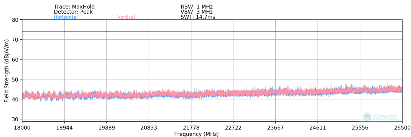
Plot 7-103. Radiated Spurious Plot above 18GHz MIMO
