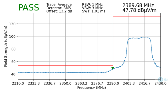
Plot 7-110. Radiated Restricted Lower Band Edge Measurement MIMO (Average) – WCP
