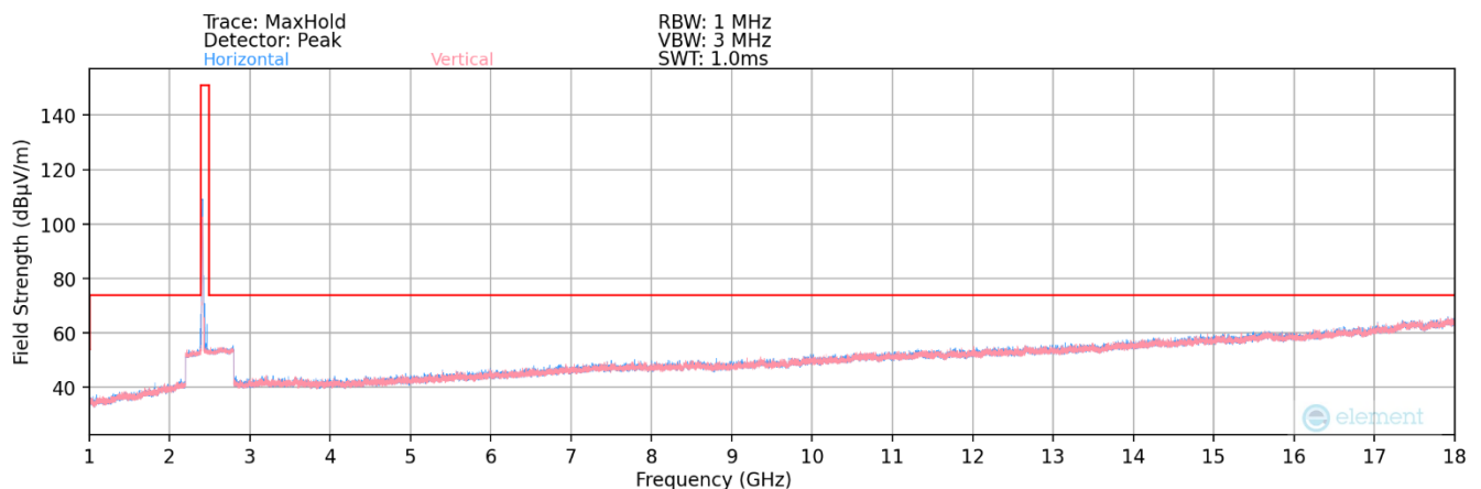
Plot 7-100. Radiated Spurious Plot above 1GHz MIMO (802.11b – Ch. 1)
