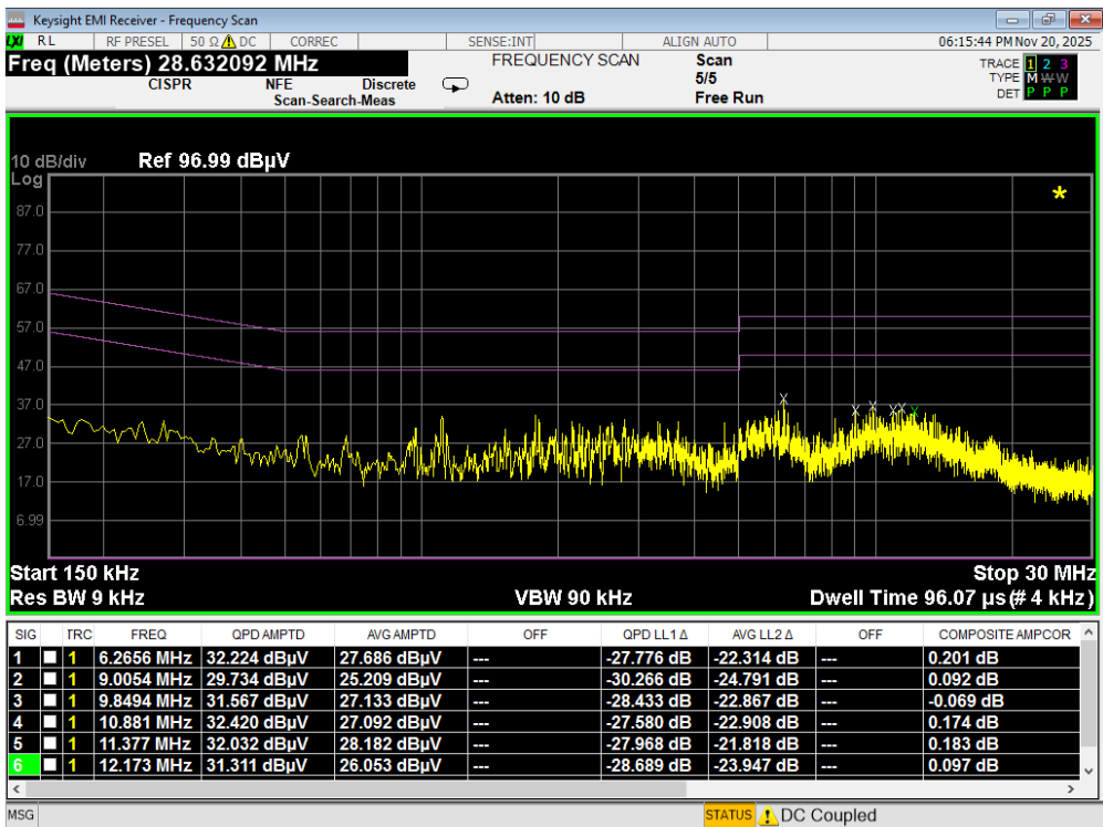
Plot 7-112. Line Conducted Plot with 802.11b (L1)
