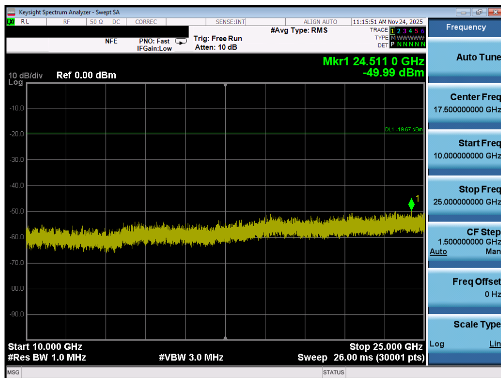
Plot 7-96. Conducted Spurious Plot MIMO ANT2 (802.11b – Ch. 6)
