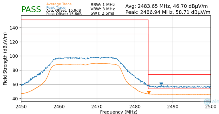
Plot 7-108. Radiated Restricted Upper Band Edge Measurement MIMO (Average & Peak)
