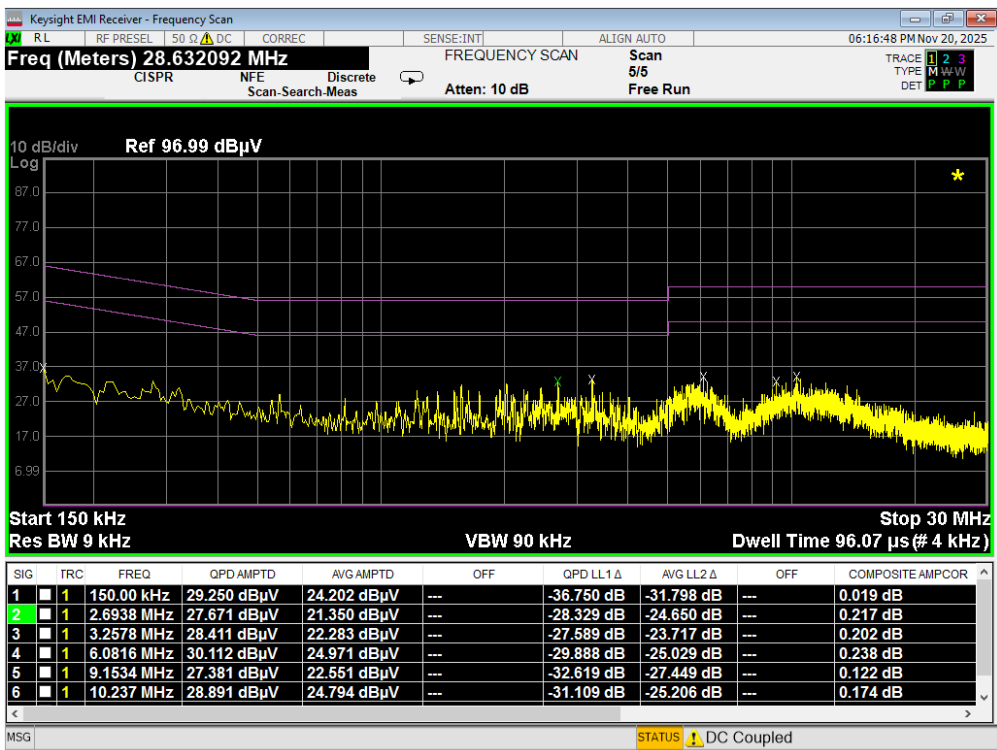
Plot 7-113. Line Conducted Plot with 802.11b (N)
