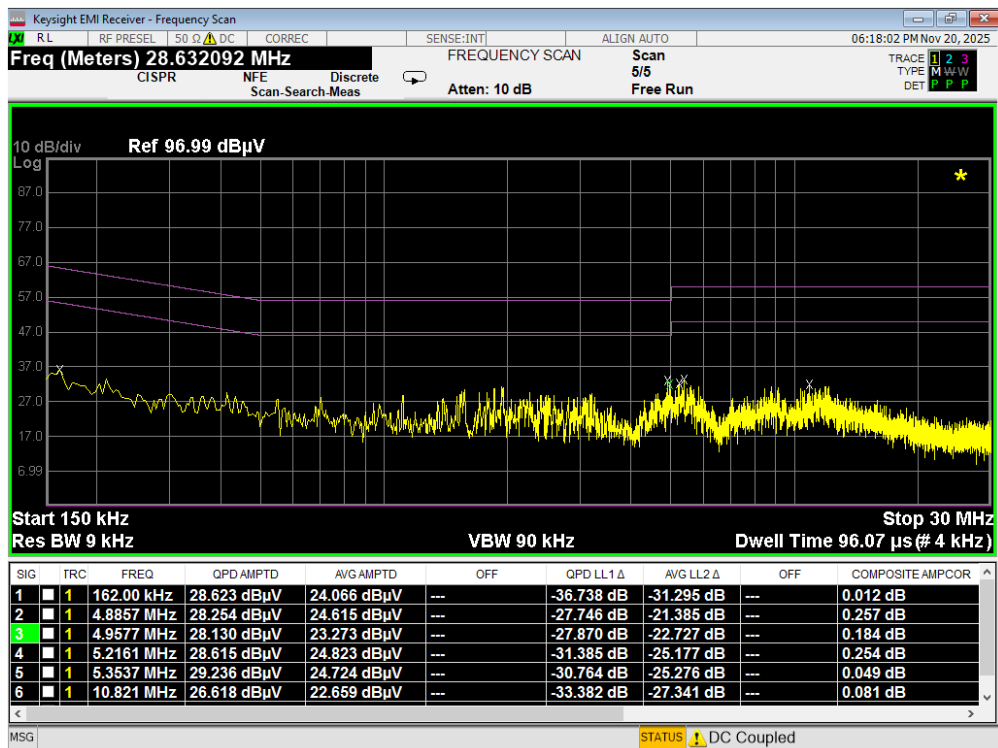
Plot 7-115. Line Conducted Plot with 802.11b (N) – WCP
