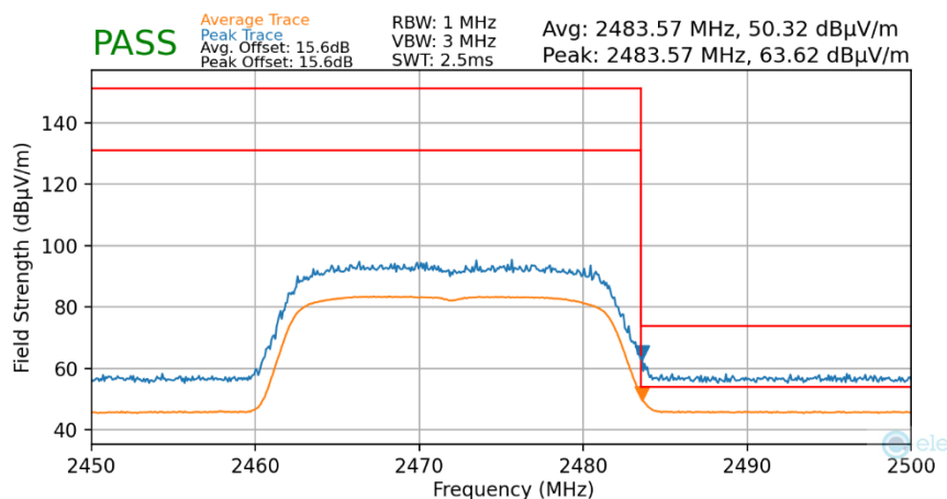
Plot 7-109. Radiated Restricted Upper Band Edge Measurement MIMO (Average & Peak)
