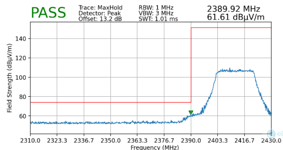
Plot 7-111. Radiated Restricted Lower Band Edge Measurement MIMO (Peak) – WCP
