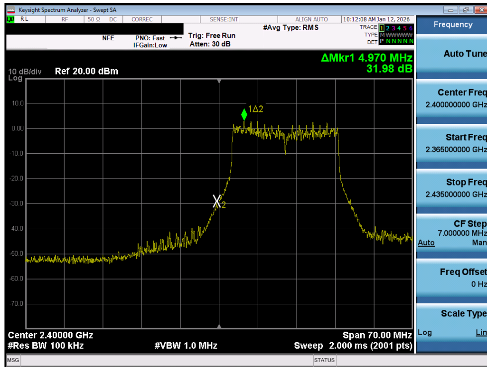
Plot 7-47. Band Edge Plot MIMO ANT2 (802.11ax/be OFDMA – 242 Tones – Ch. 1)
