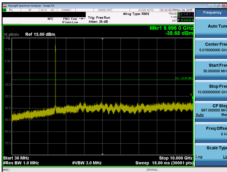
Plot 7-67. Conducted Spurious Plot MIMO ANT2 (802.11ax/be OFDMA – 26 Tones – Ch. 6)
