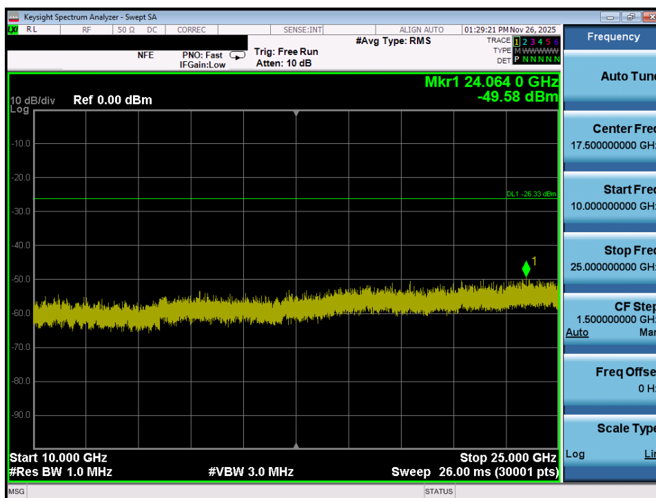
Plot 7-74. Conducted Spurious Plot MIMO ANT2 (802.11ax/be OFDMA – 242 Tones – Ch. 6)
