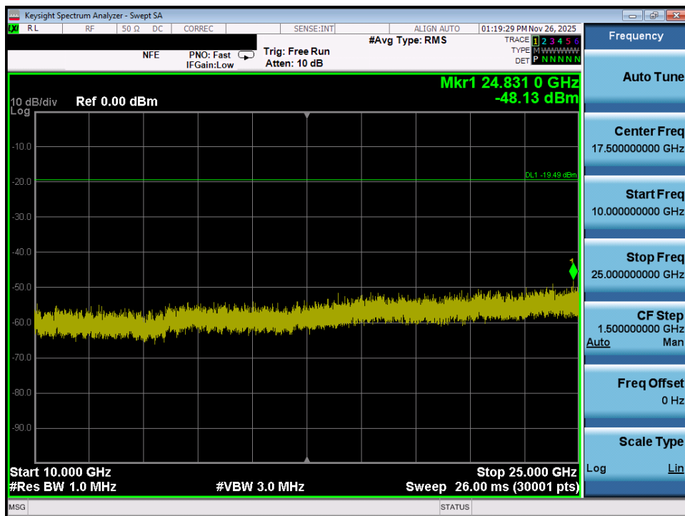
Plot 7-66. Conducted Spurious Plot MIMO ANT2 (802.11ax/be OFDMA – 26 Tones – Ch. 1)
