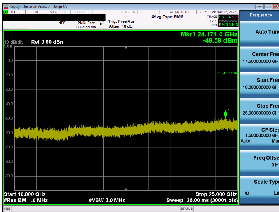
Plot 7-56. Conducted Spurious Plot MIMO ANT1 (802.11ax/be OFDMA – 26 Tones – Ch. 6)
