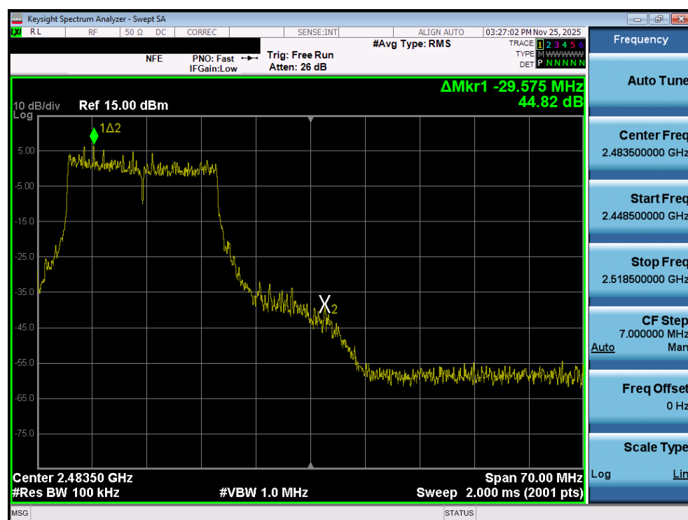
Plot 7-36. Band Edge Plot MIMO ANT1 (802.11ax/be OFDMA – 242 Tones – Ch. 11)
