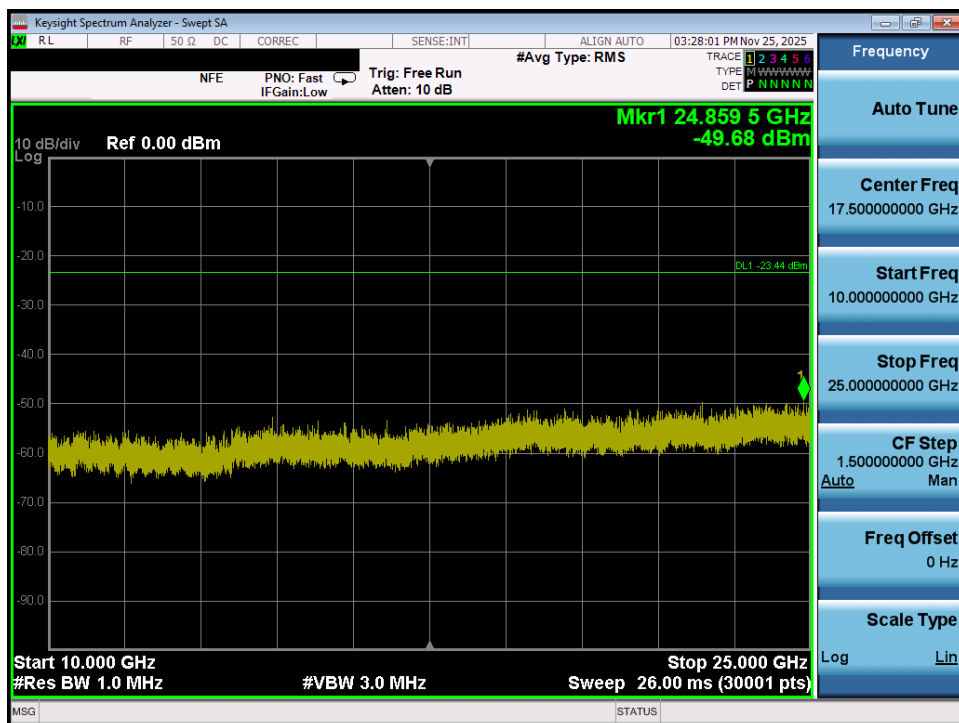
Plot 7-64. Conducted Spurious Plot MIMO ANT1 (802.11ax/be OFDMA – 242 Tones – Ch. 11)
