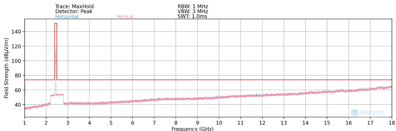
Plot 7-78. Radiated Spurious Plot above 1GHz MIMO (802.11ax OFDMA – 26 Tones – Ch. 6)
