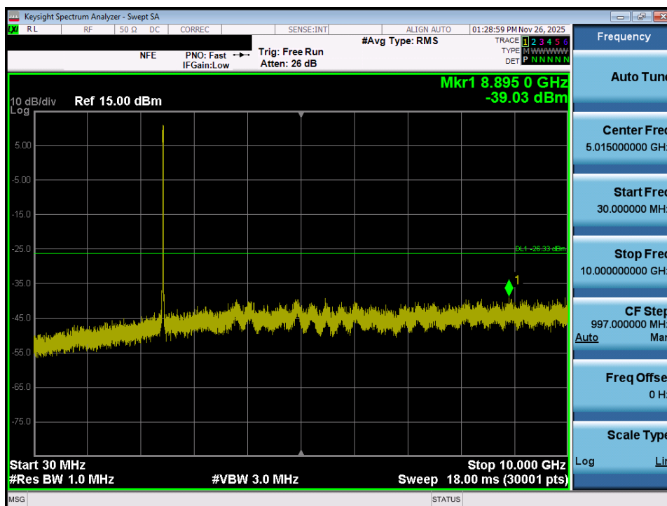
Plot 7-73. Conducted Spurious Plot MIMO ANT2 (802.11ax/be OFDMA – 242 Tones – Ch. 6)
