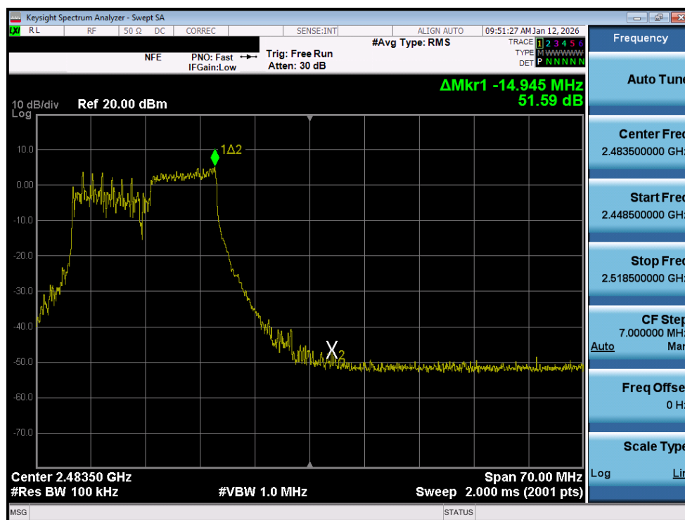
Plot 7-40. Band Edge Plot MIMO ANT2 (802.11ax/be OFDMA – 106 Tones – Ch. 11)
