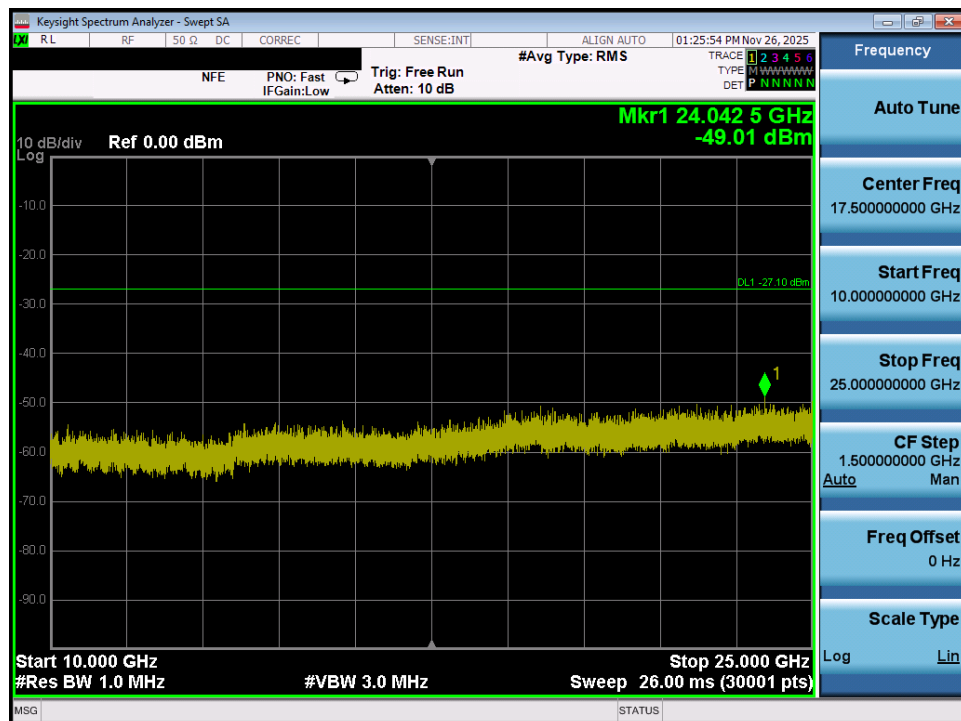
Plot 7-72. Conducted Spurious Plot MIMO ANT2 (802.11ax/be OFDMA – 242 Tones – Ch. 1)
