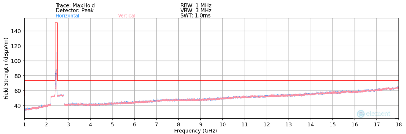
Plot 7-82. Radiated Spurious Plot above 1GHz MIMO (802.11ax OFDMA – 242 Tones – Ch. 6)
