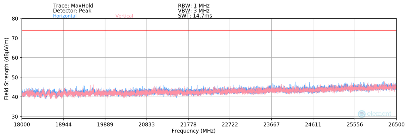
Plot 7-84. Radiated Spurious Plot above 18GHz MIMO (802.11ax OFDMA – 242 Tones)
