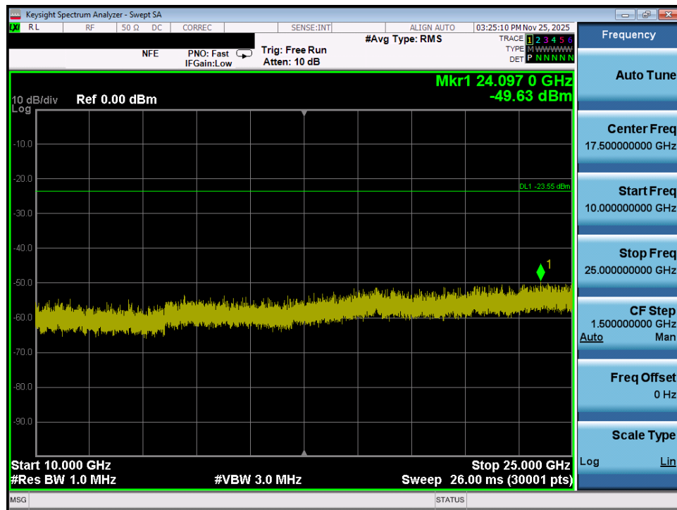
Plot 7-62. Conducted Spurious Plot MIMO ANT1 (802.11ax/be OFDMA – 242 Tones – Ch. 6)
