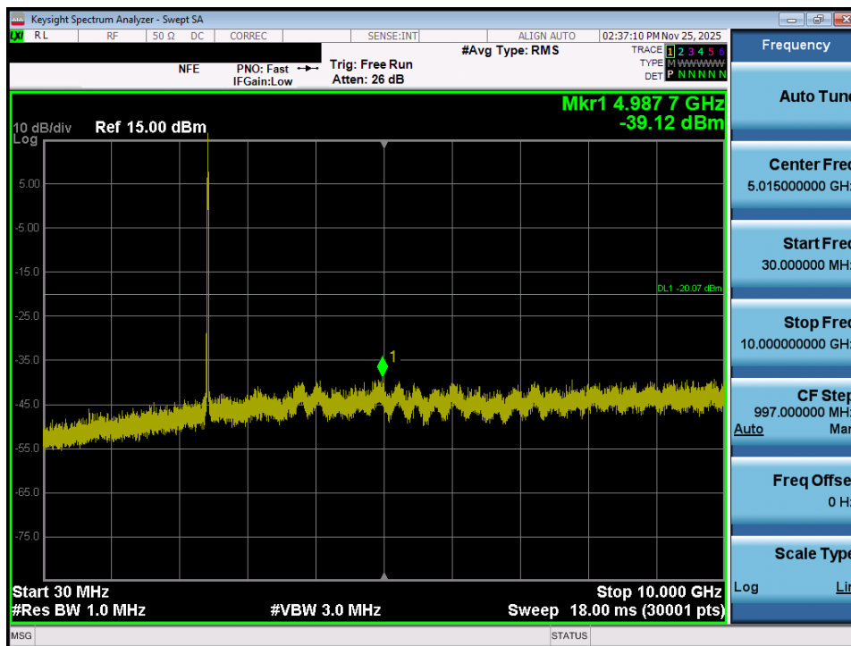
Plot 7-55. Conducted Spurious Plot MIMO ANT1 (802.11ax/be OFDMA – 26 Tones – Ch. 6)
