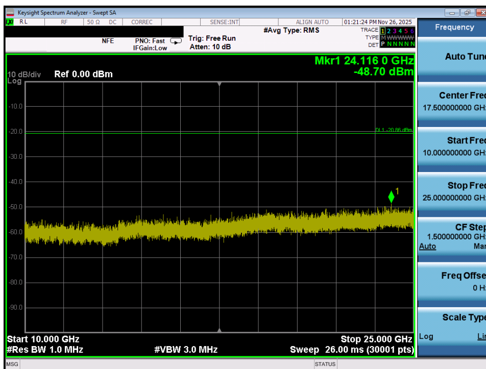
Plot 7-68. Conducted Spurious Plot MIMO ANT2 (802.11ax/be OFDMA – 26 Tones – Ch. 6)
