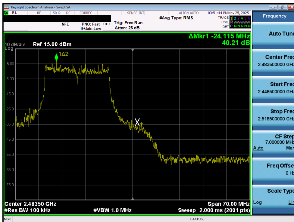
Plot 7-37. Band Edge Plot MIMO ANT1 (802.11ax/be OFDMA – 242 Tones – Ch. 12)
