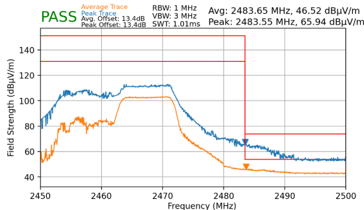
Plot 7-86. Radiated Restricted Upper Band Edge Measurement MIMO (Average & Peak – 106 Tones)
