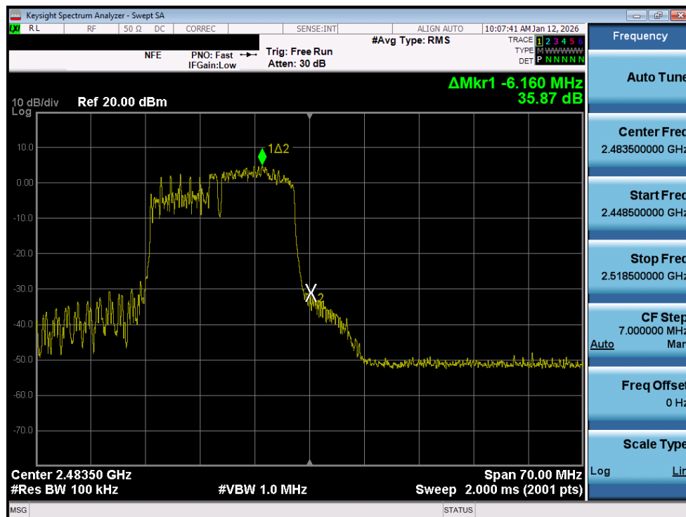
Plot 7-46. Band Edge Plot MIMO ANT12 (802.11be OFDMA – 106+26 Tones – Ch. 13)
