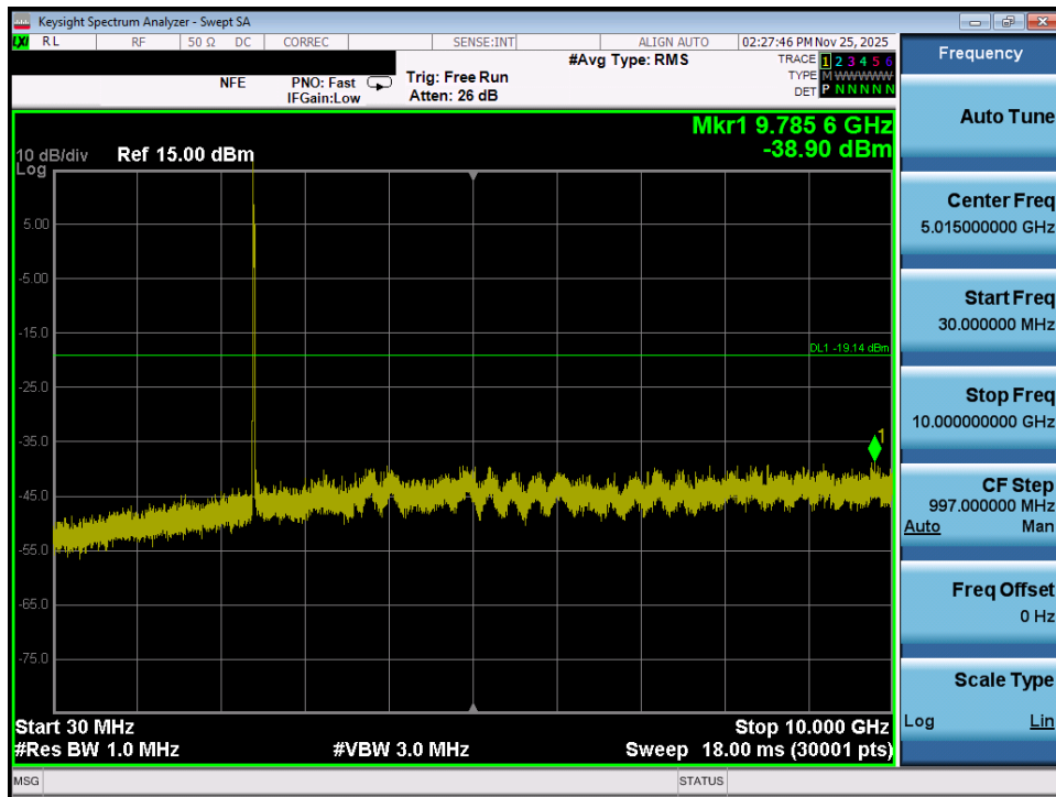
Plot 7-65. Conducted Spurious Plot MIMO ANT1 (802.11ax/be OFDMA – 26 Tones – Ch. 1)
