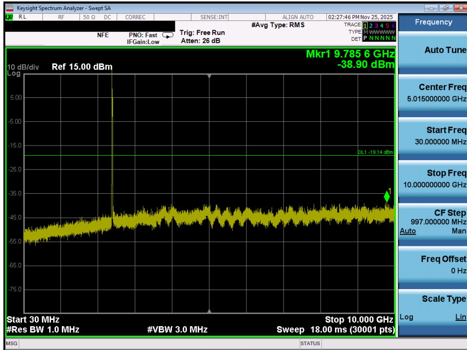
Plot 7-53. Conducted Spurious Plot MIMO ANT1 (802.11ax/be OFDMA – 26 Tones – Ch. 1)
