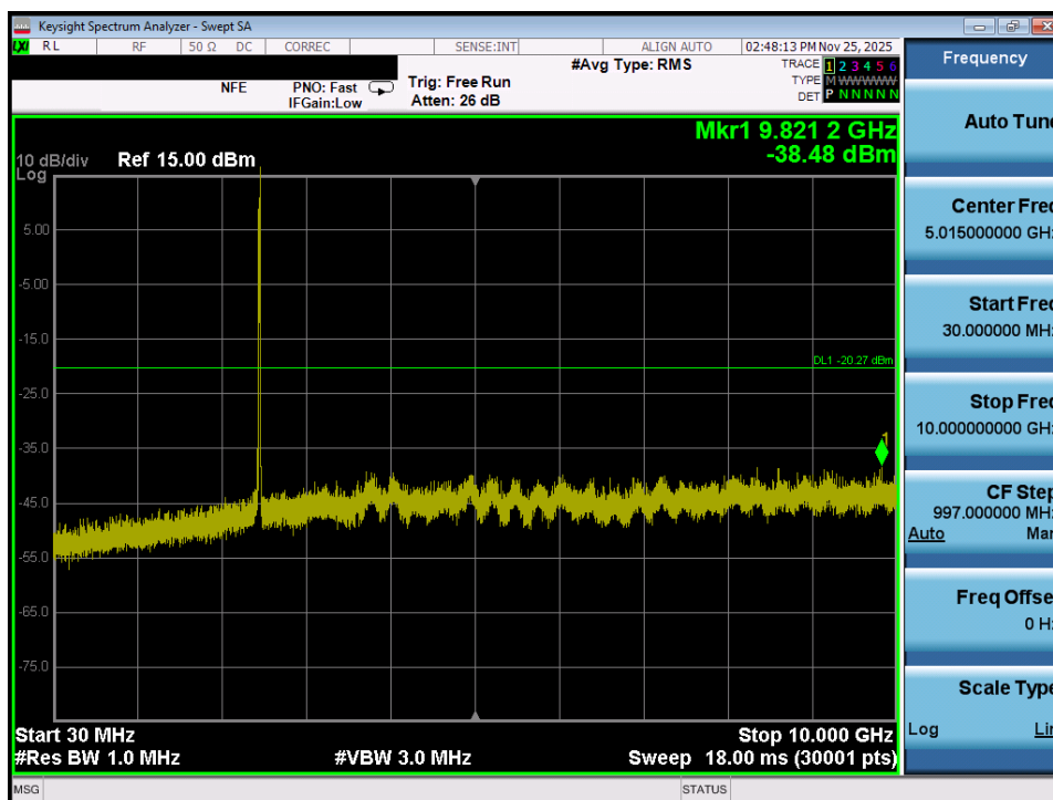
Plot 7-57. Conducted Spurious Plot MIMO ANT1 (802.11ax/be OFDMA – 26 Tones – Ch. 11)
