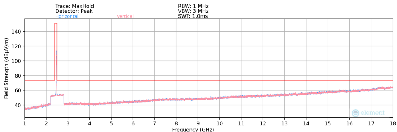
Plot 7-79. Radiated Spurious Plot above 1GHz MIMO (802.11ax OFDMA – 26 Tones – Ch. 11)
