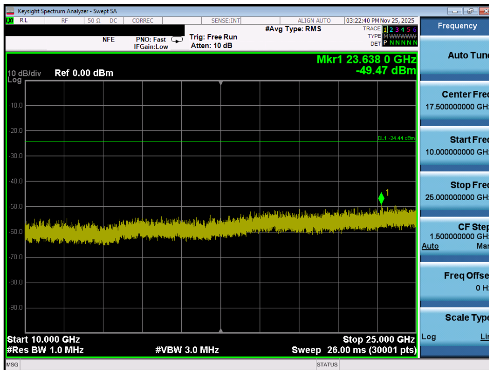
Plot 7-60. Conducted Spurious Plot MIMO ANT1 (802.11ax/be OFDMA – 242 Tones – Ch. 1)
