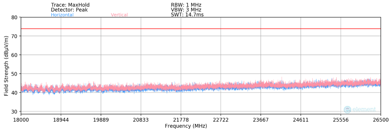
Plot 7-80. Radiated Spurious Plot above 18GHz MIMO (802.11ax OFDMA – 26 Tones)
