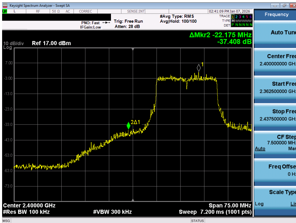
Plot 7-48. Band Edge Plot MIMO ANT2 (802.11ax/be OFDMA – 242 Tones – Ch. 2)
