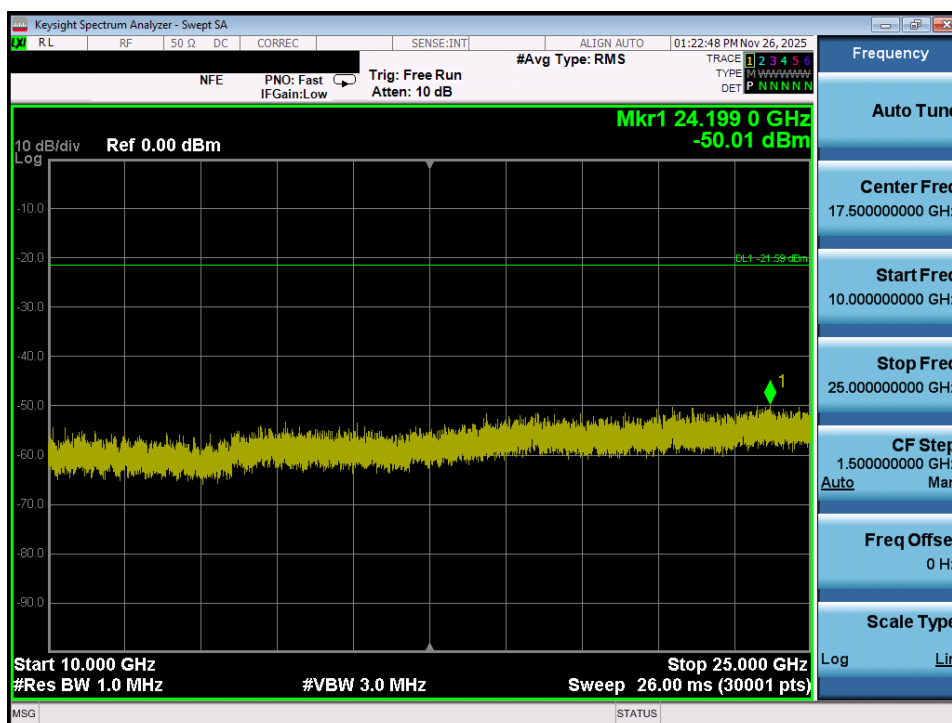
Plot 7-70. Conducted Spurious Plot MIMO ANT2 (802.11ax/be OFDMA – 26 Tones – Ch. 11)
