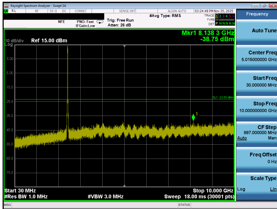
Plot 7-61. Conducted Spurious Plot MIMO ANT1 (802.11ax/be OFDMA – 242 Tones – Ch. 6)
