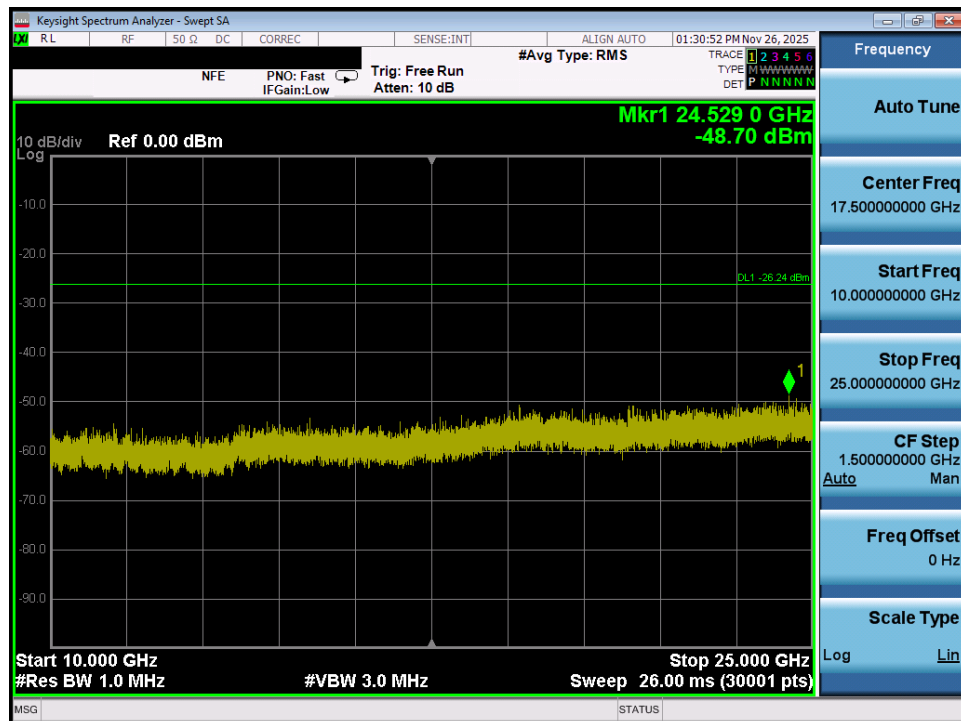
Plot 7-76. Conducted Spurious Plot MIMO ANT2 (802.11ax/be OFDMA – 242 Tones – Ch. 11)
