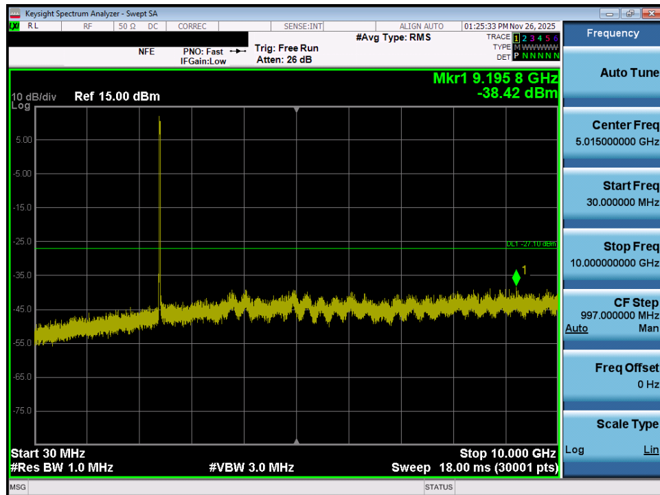
Plot 7-71. Conducted Spurious Plot MIMO ANT2 (802.11ax/be OFDMA – 242 Tones – Ch. 1)
