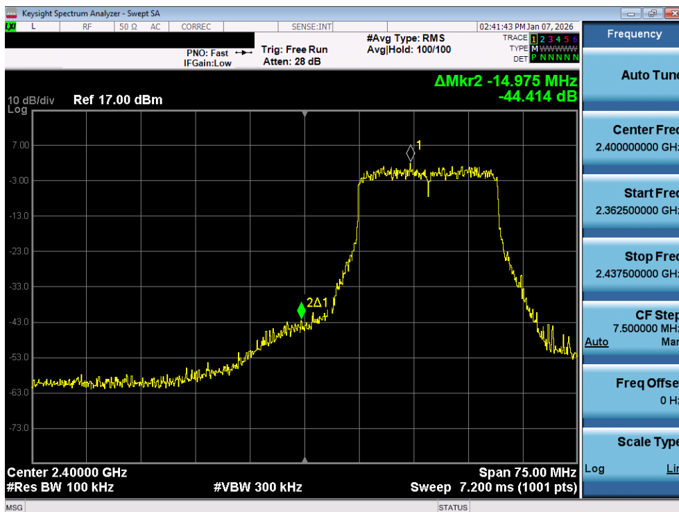
Plot 7-34. Band Edge Plot MIMO ANT1 (802.11ax/be OFDMA – 242 Tones – Ch. 2)
