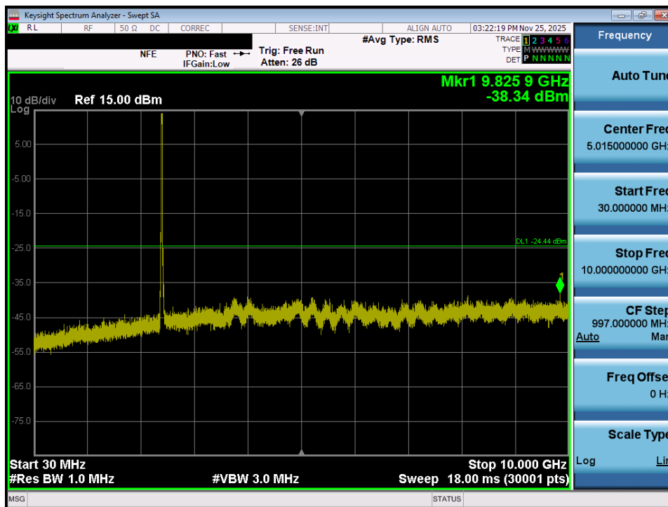
Plot 7-59. Conducted Spurious Plot MIMO ANT1 (802.11ax/be OFDMA – 242 Tones – Ch. 1)
