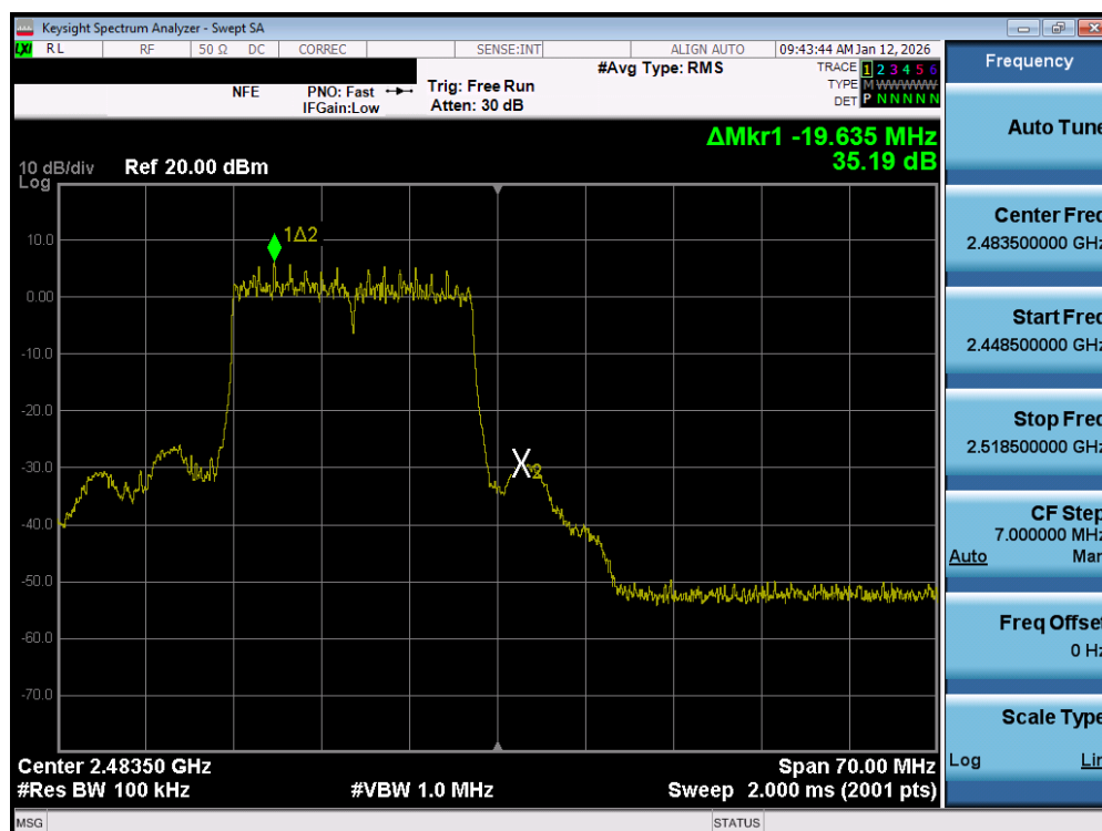
Plot 7-38. Band Edge Plot MIMO ANT1 (802.11ax/be OFDMA – 242 Tones – Ch. 13)
