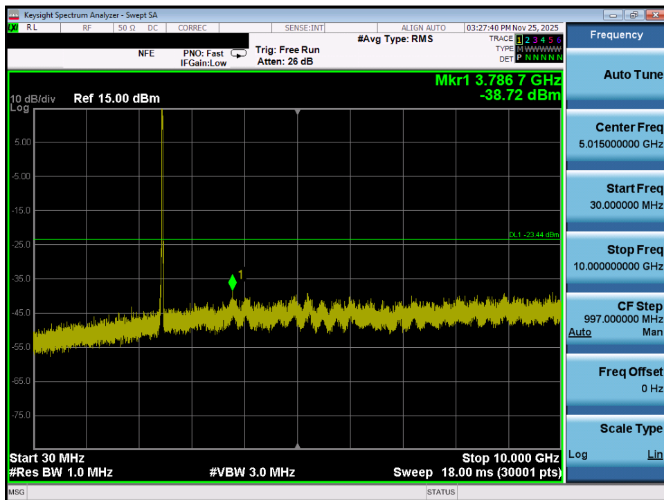
Plot 7-63. Conducted Spurious Plot MIMO ANT1 (802.11ax/be OFDMA – 242 Tones – Ch. 11)
