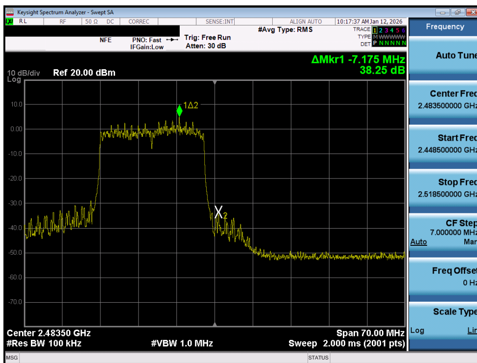
Plot 7-52. Band Edge Plot MIMO ANT2 (802.11ax/be OFDMA – 242 Tones – Ch. 13)
