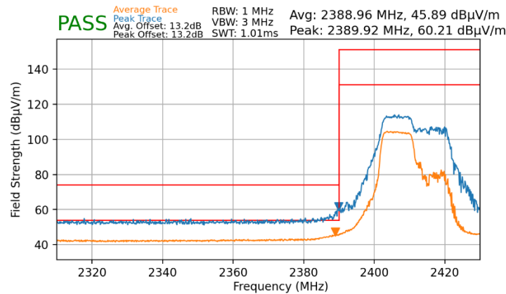
Plot 7-85. Radiated Restricted Lower Band Edge Measurement MIMO (Average & Peak – 106 Tones)
