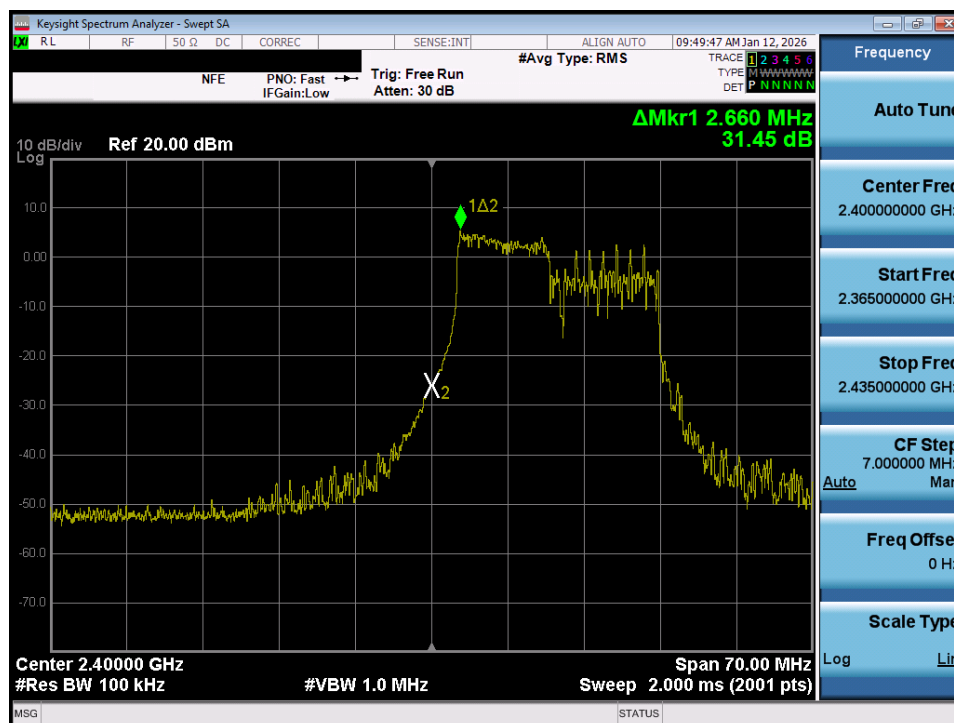
Plot 7-39. Band Edge Plot MIMO ANT2 (802.11ax/be OFDMA – 106 Tones – Ch. 1)
