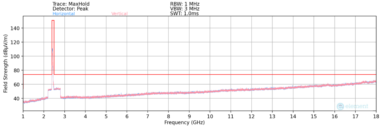
Plot 7-81. Radiated Spurious Plot above 1GHz MIMO (802.11ax OFDMA – 242 Tones – Ch. 1)
