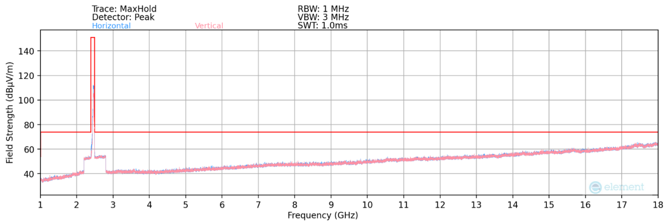
Plot 7-83. Radiated Spurious Plot above 1GHz MIMO (802.11ax OFDMA – 242 Tones – Ch. 11)
