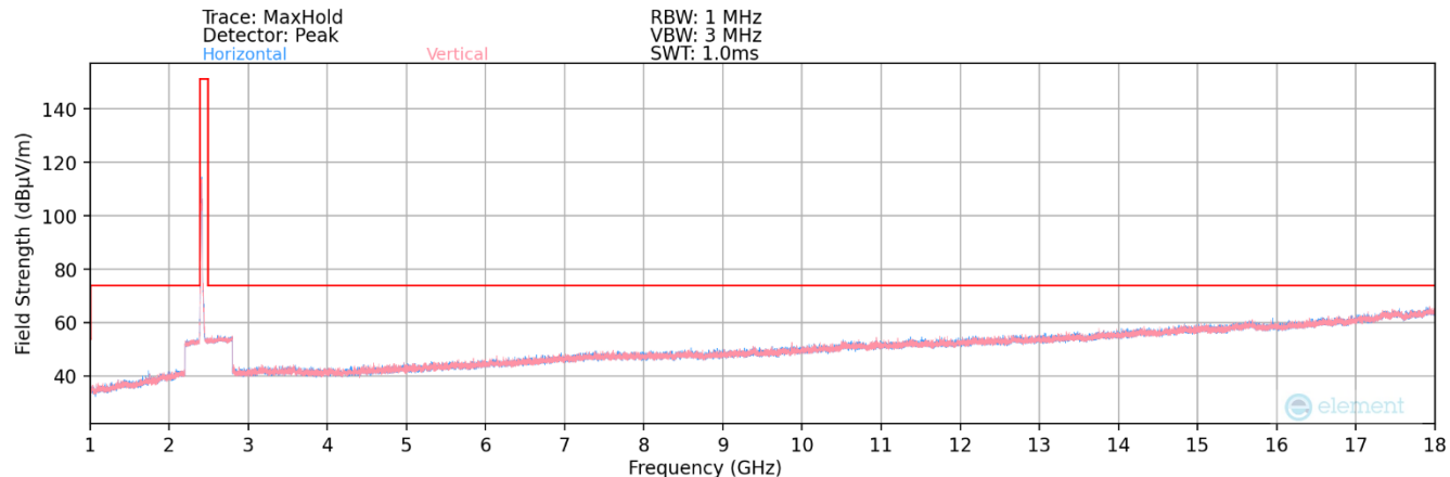
Plot 7-77. Radiated Spurious Plot above 1GHz MIMO (802.11ax OFDMA – 26 Tones – Ch. 1)
