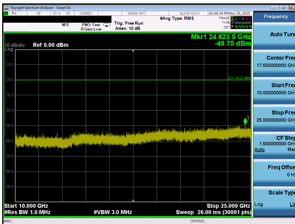
Plot 7-58. Conducted Spurious Plot MIMO ANT1 (802.11ax/be OFDMA – 26 Tones – Ch. 11)
