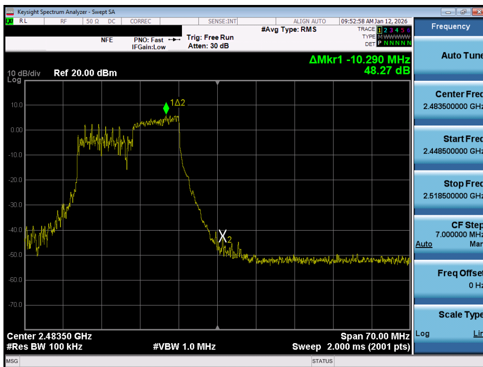
Plot 7-41. Band Edge Plot MIMO ANT2 (802.11ax/be OFDMA – 106 Tones – Ch. 12)
