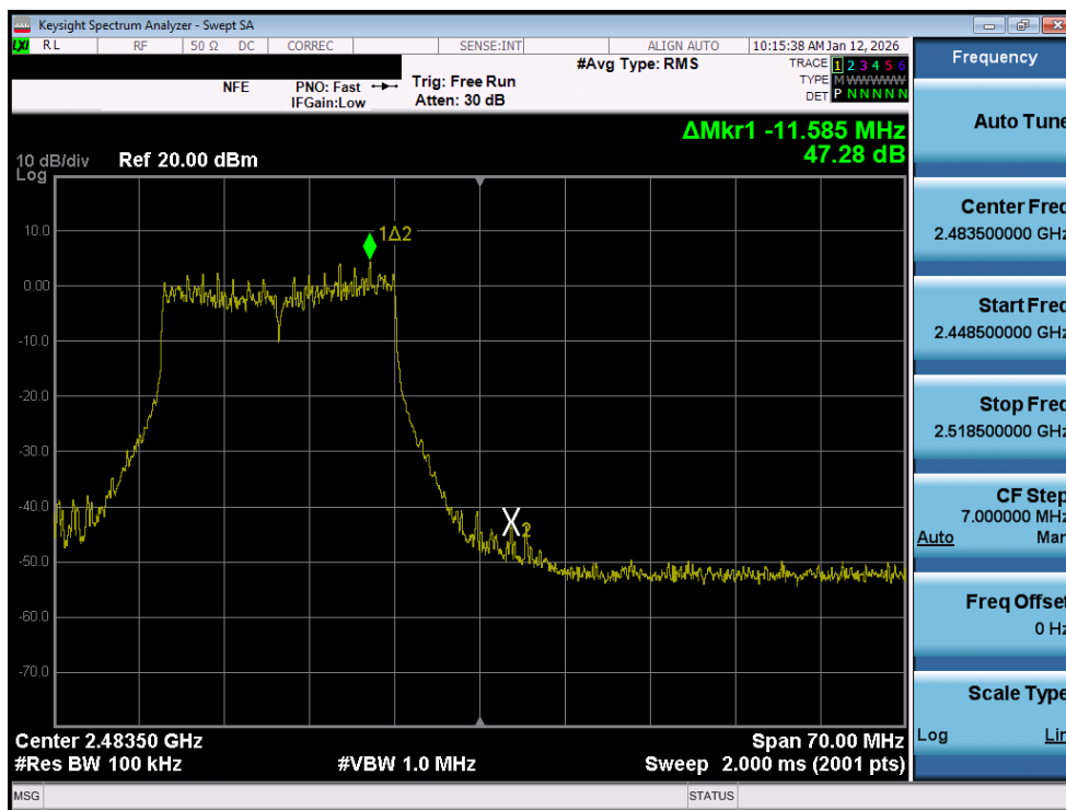
Plot 7-51. Band Edge Plot MIMO ANT2 (802.11ax/be OFDMA – 242 Tones – Ch. 12)
