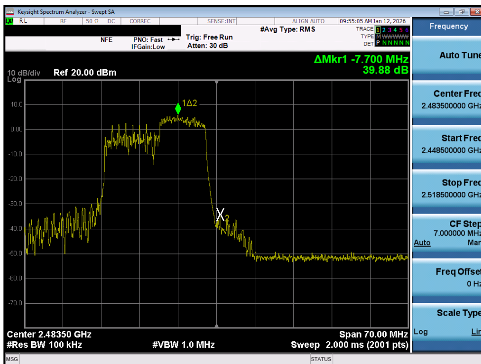
Plot 7-42. Band Edge Plot MIMO ANT2 (802.11ax/be OFDMA – 106 Tones – Ch. 13)
