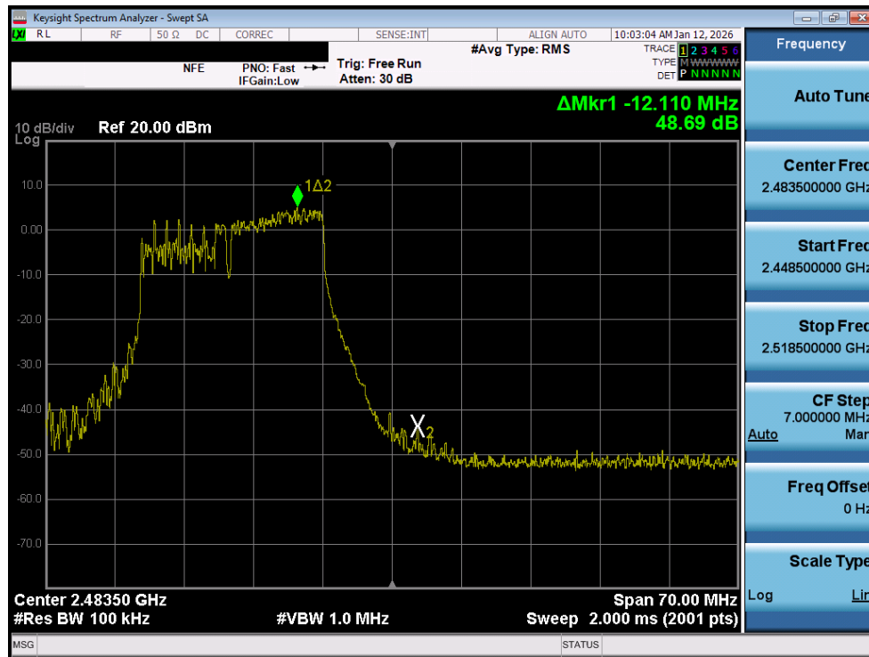
Plot 7-45. Band Edge Plot MIMO ANT2 (802.11be OFDMA – 106+26 Tones – Ch. 12)
