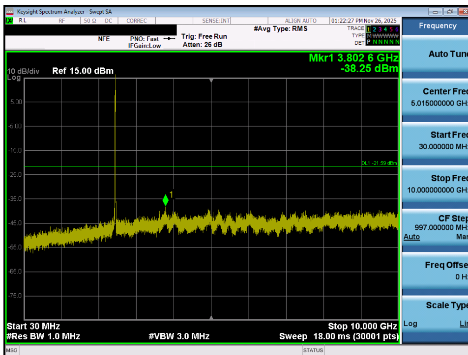
Plot 7-69. Conducted Spurious Plot MIMO ANT2 (802.11ax/be OFDMA – 26 Tones – Ch. 11)
