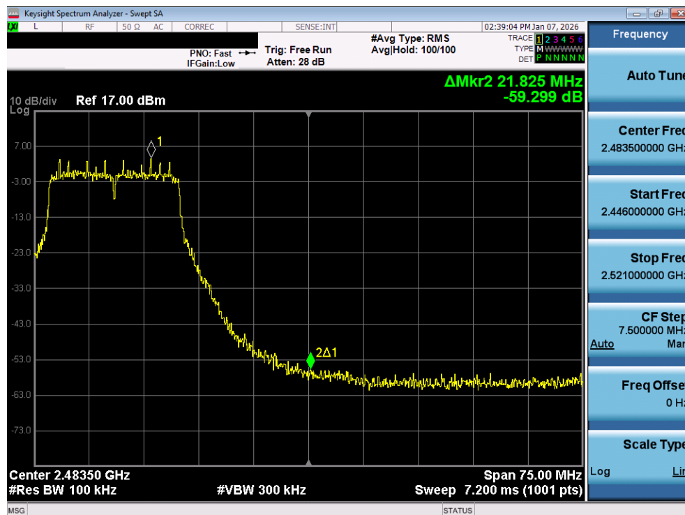
Plot 7-35. Band Edge Plot MIMO ANT1 (802.11ax/be OFDMA – 242 Tones – Ch. 10)
