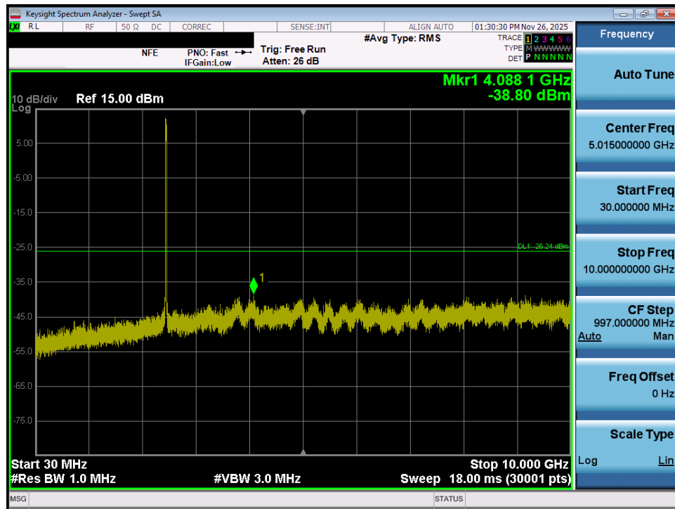
Plot 7-75. Conducted Spurious Plot MIMO ANT2 (802.11ax/be OFDMA – 242 Tones – Ch. 11)
