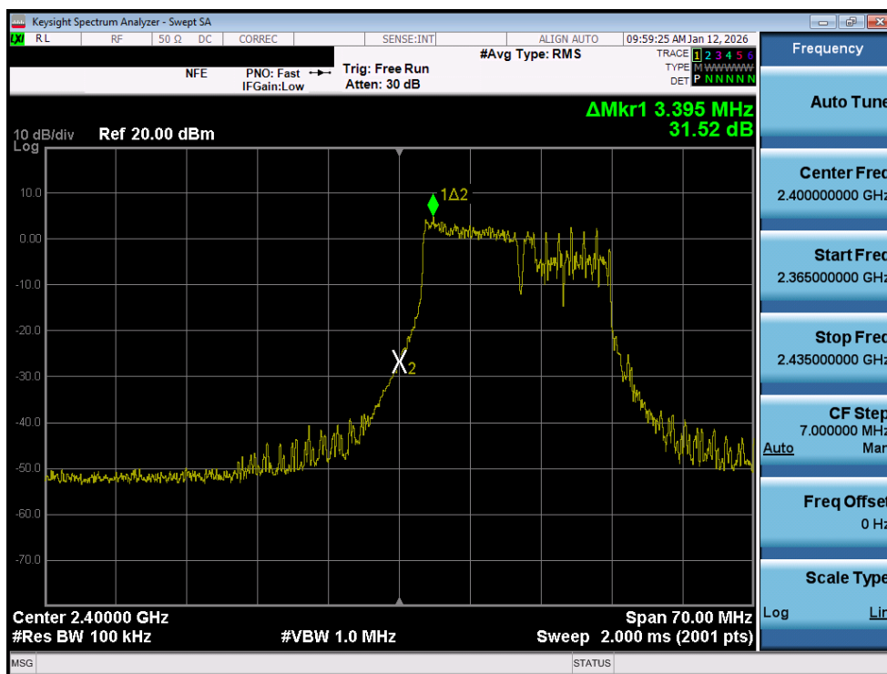
Plot 7-43. Band Edge Plot MIMO ANT2 (802.11be OFDMA – 106+26 Tones – Ch. 1)
