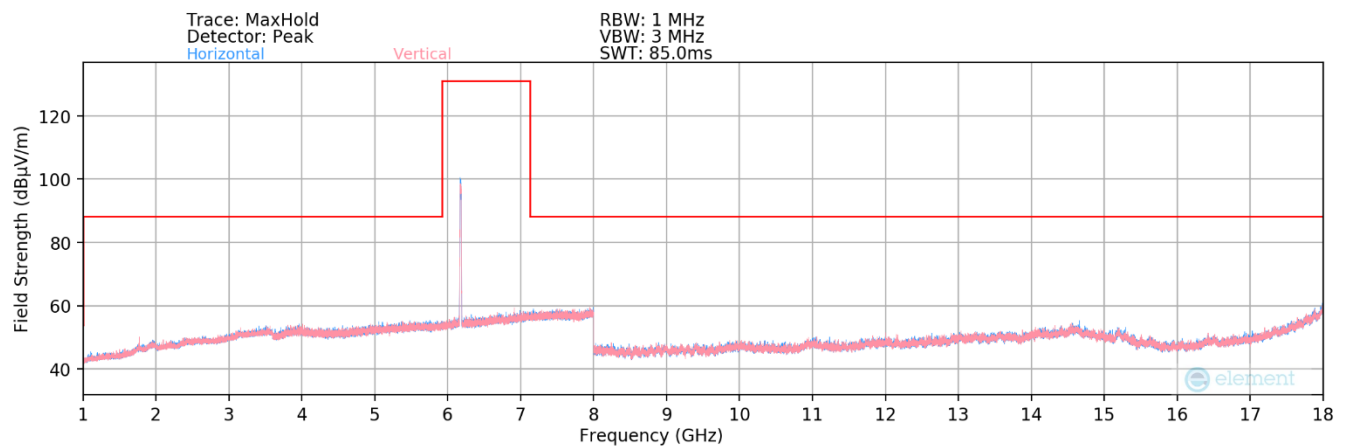
Plot 7-58. Radiated Spurious Plot 1GHz – 18GHz MIMO (802.11a – UNII Band 5 Ch. 45)
