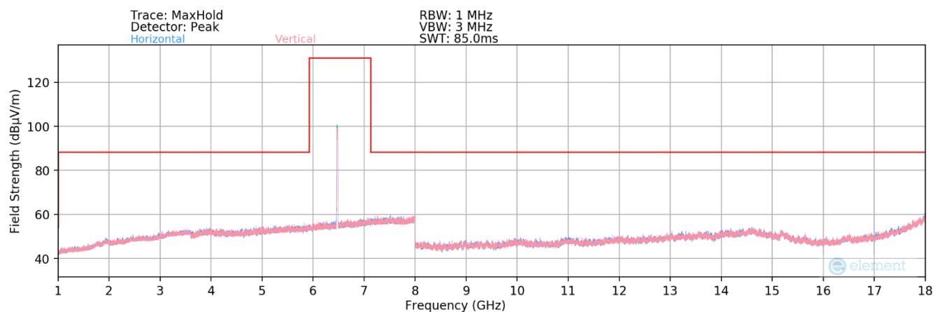
Plot 7-59. Radiated Spurious Plot 1GHz – 18GHz MIMO (802.11a – UNII Band 6 Ch. 105)
