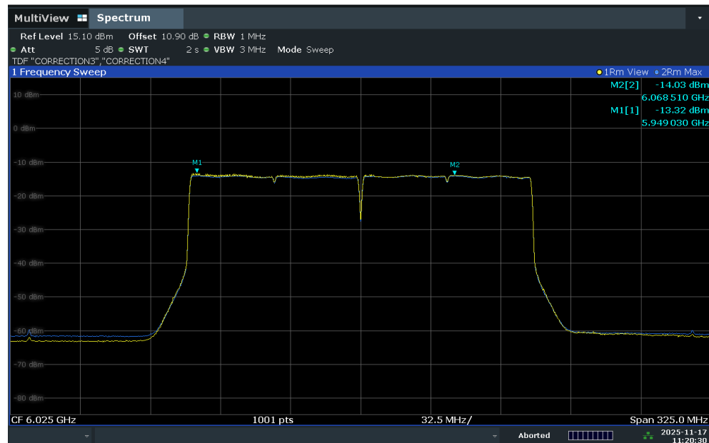
Plot 7-55. Power Spectral Density Plot – ANT1 (160MHz Bandwidth, RSSI level at -85dBm (yellow) and -27dBm (green))
