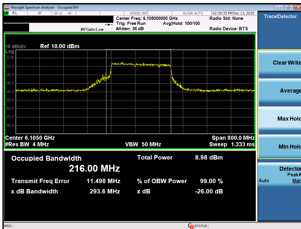
Plot 7-9. 26dB Bandwidth Plot MIMO ANT1 (320MHz 802.11be (UNII Band 5) – Ch. 31) – 40MHz Punctured - VLP
