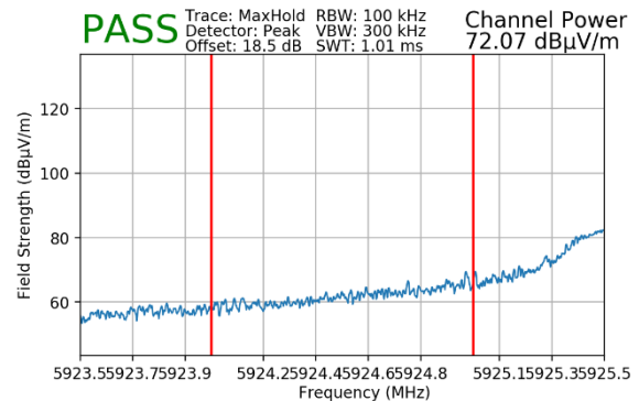
Plot 7-70. Radiated Lower Band Edge Plot MIMO (Peak – UNII Band 5) – WCP
