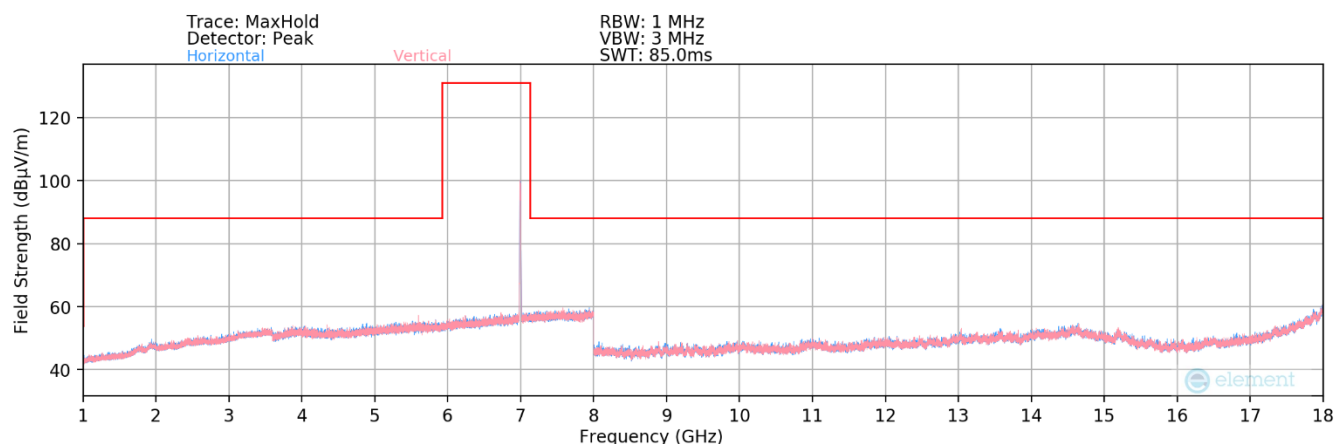
Plot 7-61. Radiated Spurious Plot 1GHz – 18GHz MIMO (802.11a – UNII Band 8 Ch. 209)
