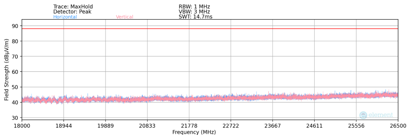
Plot 7-62. Radiated Spurious Plot 18GHz - 26.5GHz (802.11a) – Ch.149
