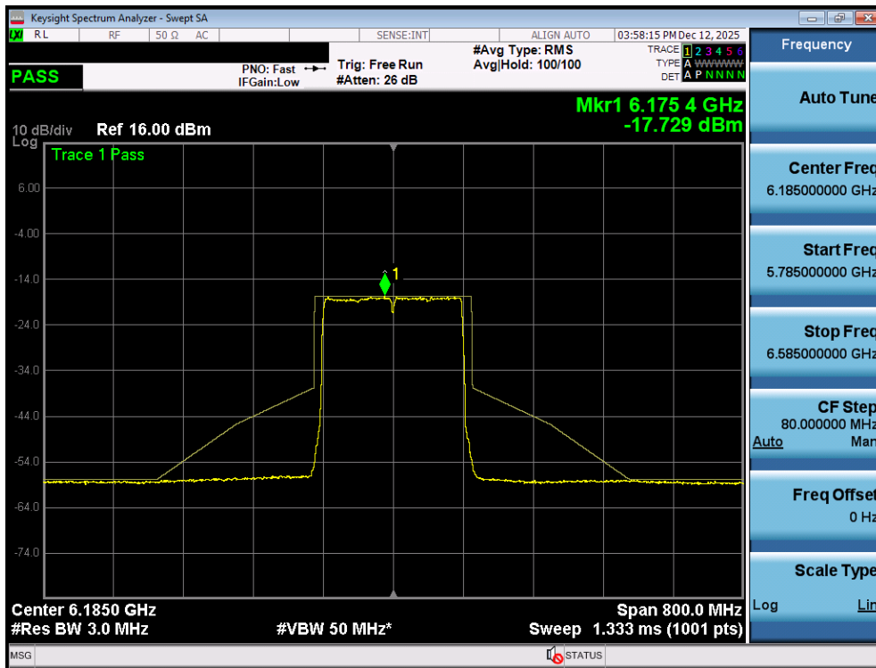
Plot 7-50. In Band Emissions Plot MIMO ANT2 (160MHz 802.11ax/be (UNII Band 5) – Ch. 47) - VLP
