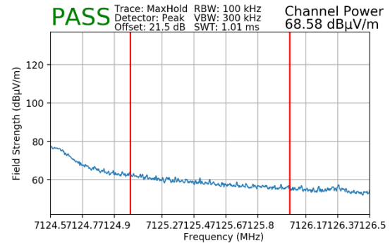
Plot 7-68. Radiated Upper Band Edge Plot MIMO (Peak – UNII Band 8)
