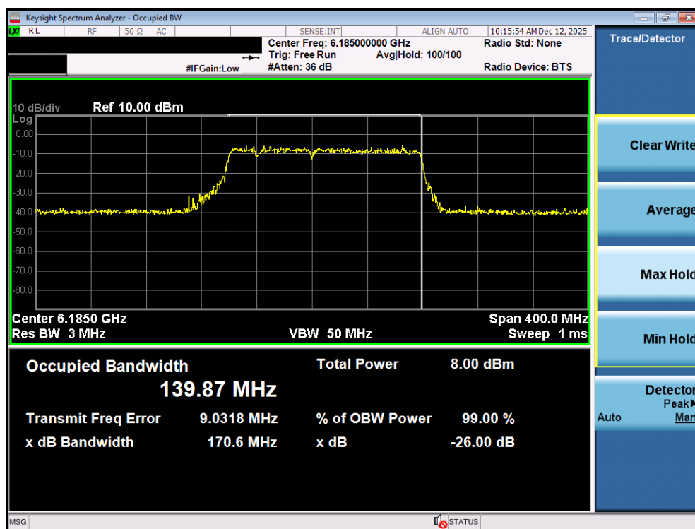
Plot 7-8. 26dB Bandwidth Plot MIMO ANT1 (160MHz 802.11be (UNII Band 5) – Ch. 47) – 20MHz Punctured - VLP
