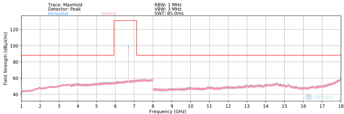
Plot 7-60. Radiated Spurious Plot 1GHz – 18GHz MIMO (802.11a – UNII Band 7 Ch. 149)
