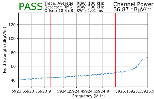
Plot 7-65. Radiated Lower Band Edge Plot MIMO (Average – UNII Band 5)
