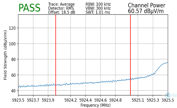
Plot 7-69. Radiated Lower Band Edge Plot MIMO (Average – UNII Band 5) – WCP
