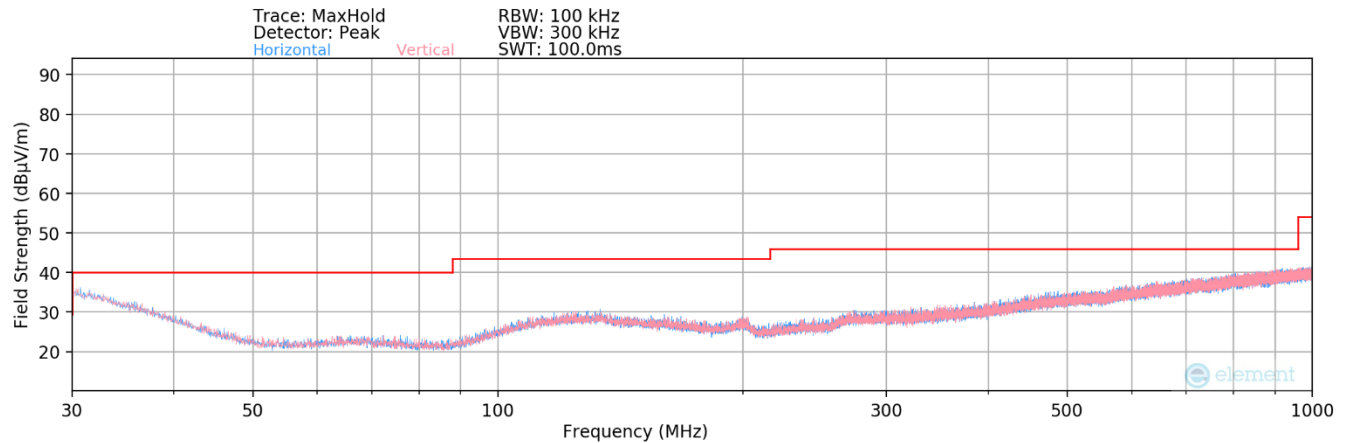
Plot 7-57. Radiated Spurious Plot below 1GHz MIMO (802.11a)
