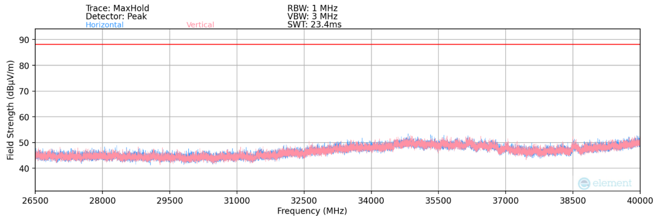
Plot 7-63. Radiated Spurious Plot 26.5GHz - 40GHz (802.11a) – Ch.149
