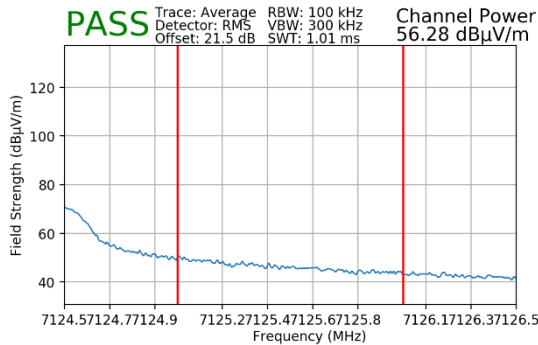
Plot 7-67. Radiated Upper Band Edge Plot MIMO (Average – UNII Band 8)
