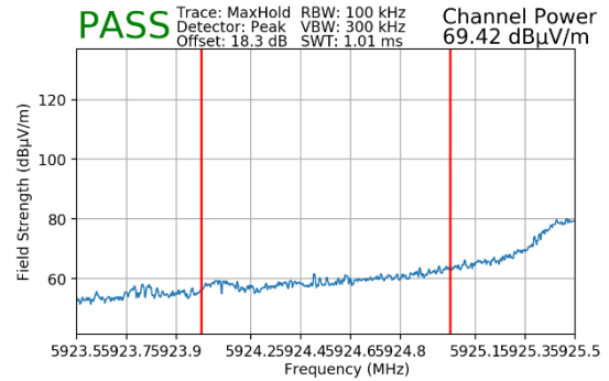
Plot 7-66. Radiated Lower Band Edge Plot MIMO (Peak – UNII Band 5)
