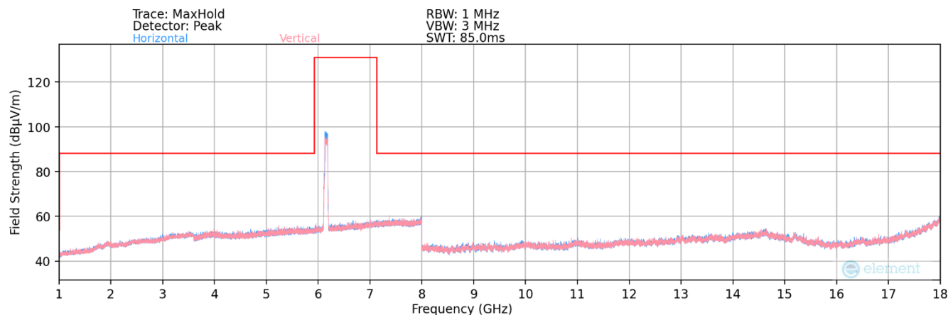
Plot 7-64. Radiated Spurious Plot 1GHz – 18GHz MIMO (802.11be – UNII Band 5 Ch. 39) – 20MHz Punctured
