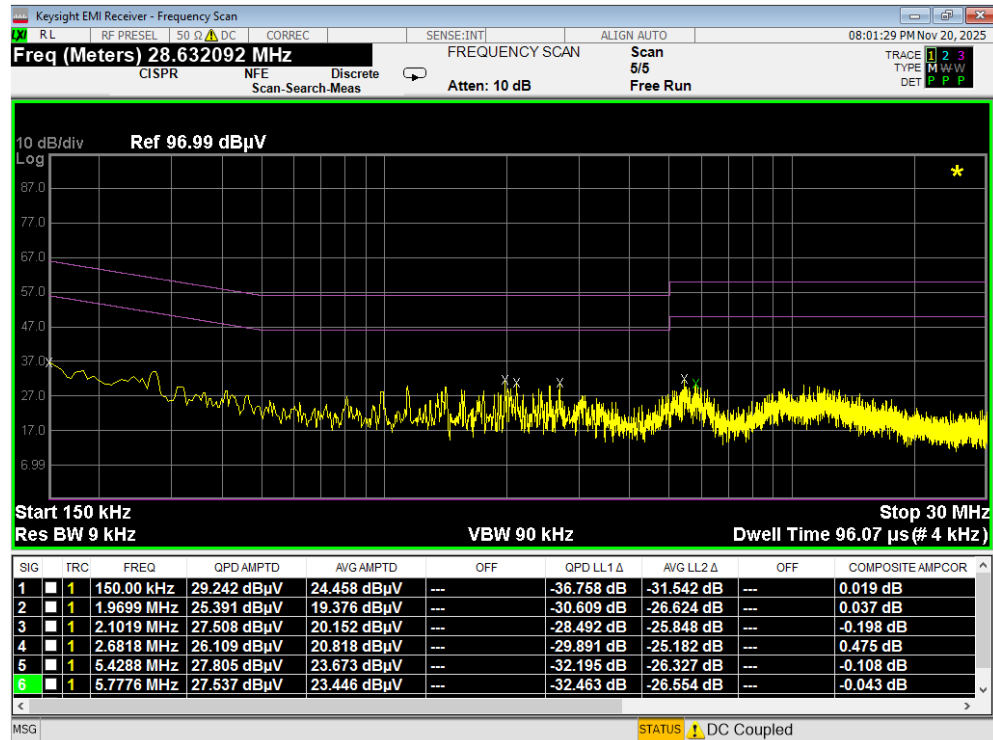
Plot 7-106. Line Conducted Plot with 802.11a UNII Band 8 (N)
