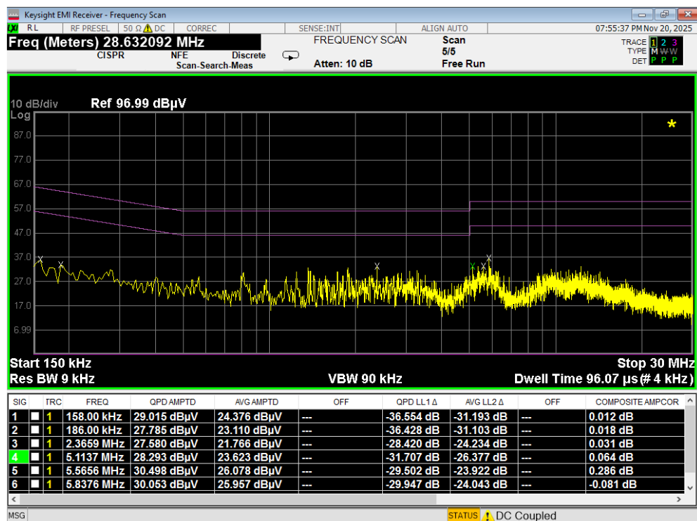
Plot 7-103. Line Conducted Plot with 802.11a UNII Band 7 (L1)
