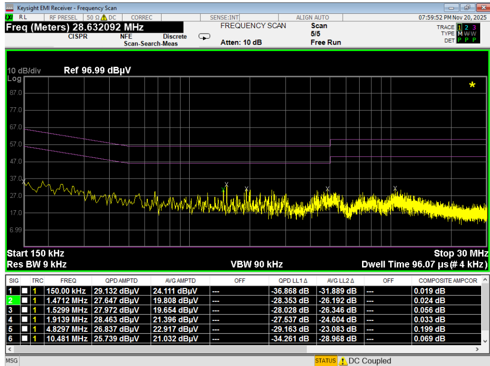
Plot 7-112. Line Conducted Plot with 802.11a UNII Band 7 (N) with WCP
