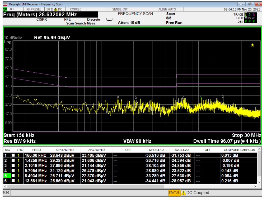
Plot 7-113. Line Conducted Plot with 802.11a UNII Band 8 (L1) with WCP
