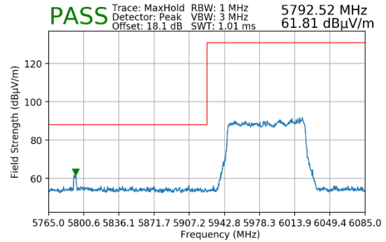
Plot 7-76. Radiated Lower Band Edge Plot MIMO (Peak – UNII Band 5)
