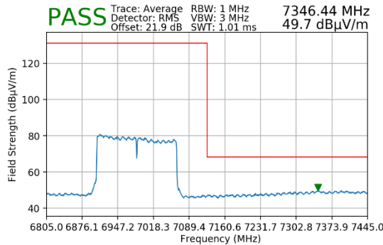
Plot 7-85. Radiated Upper Band Edge Plot MIMO (Average – UNII Band 8)
