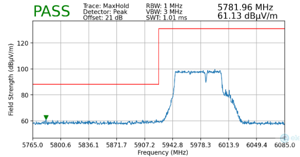
Plot 7-80. Radiated Lower Band Edge Plot MIMO (Peak – UNII Band 5)
