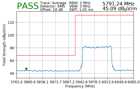
Plot 7-75. Radiated Lower Band Edge Plot MIMO (Average – UNII Band 5)
