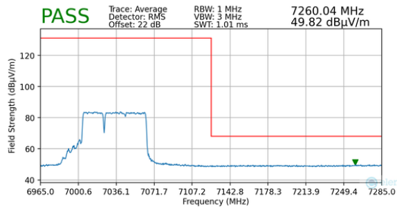
Plot 7-81. Radiated Upper Band Edge Plot MIMO (Average – UNII Band 8)
