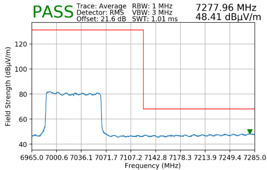
Plot 7-77. Radiated Upper Band Edge Plot MIMO (Average – UNII Band 8)
