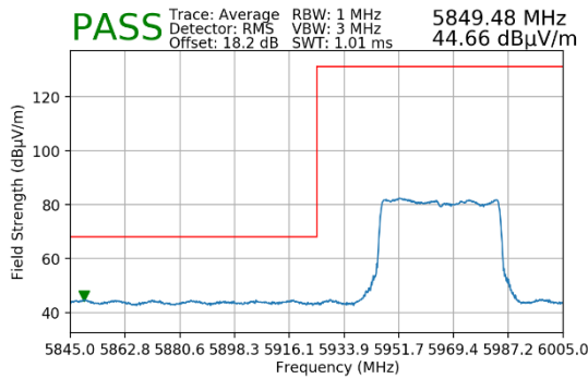
Plot 7-71. Radiated Lower Band Edge Plot MIMO (Average – UNII Band 5)
