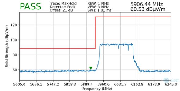
Plot 7-88. Radiated Lower Band Edge Plot MIMO (Peak – UNII Band 5)
