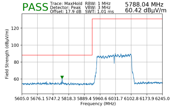
Plot 7-84. Radiated Lower Band Edge Plot MIMO (Peak – UNII Band 5)
