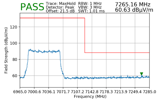
Plot 7-78. Radiated Upper Band Edge Plot MIMO (Peak – UNII Band 8)
