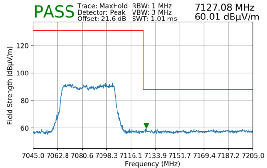
Plot 7-74. Radiated Upper Band Edge Plot MIMO (Peak – UNII Band 8)
