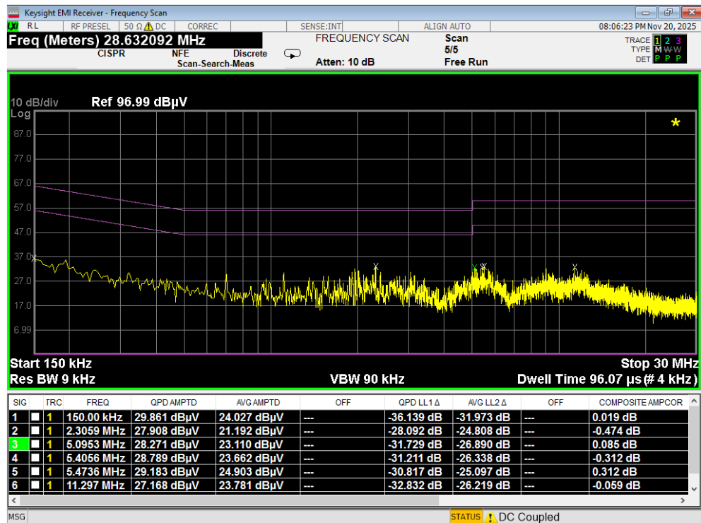
Plot 7-114. Line Conducted Plot with 802.11a UNII Band 8 (N) with WCP
