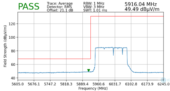
Plot 7-87. Radiated Lower Band Edge Plot MIMO (Average – UNII Band 5)
