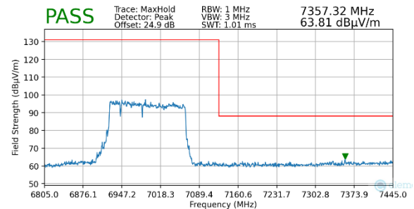
Plot 7-90. Radiated Upper Band Edge Plot MIMO (Peak – UNII Band 8)
