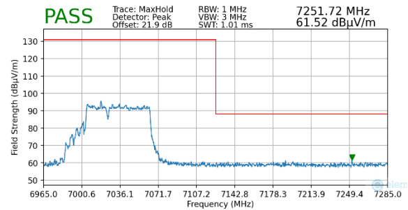
Plot 7-82. Radiated Upper Band Edge Plot MIMO (Peak – UNII Band 8)
