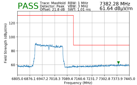
Plot 7-86. Radiated Upper Band Edge Plot MIMO (Peak – UNII Band 8)
