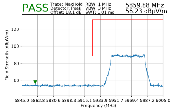
Plot 7-72. Radiated Lower Band Edge Plot MIMO (Peak – UNII Band 5)
