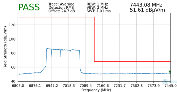
Plot 7-89. Radiated Upper Band Edge Plot MIMO (Average – UNII Band 8)
