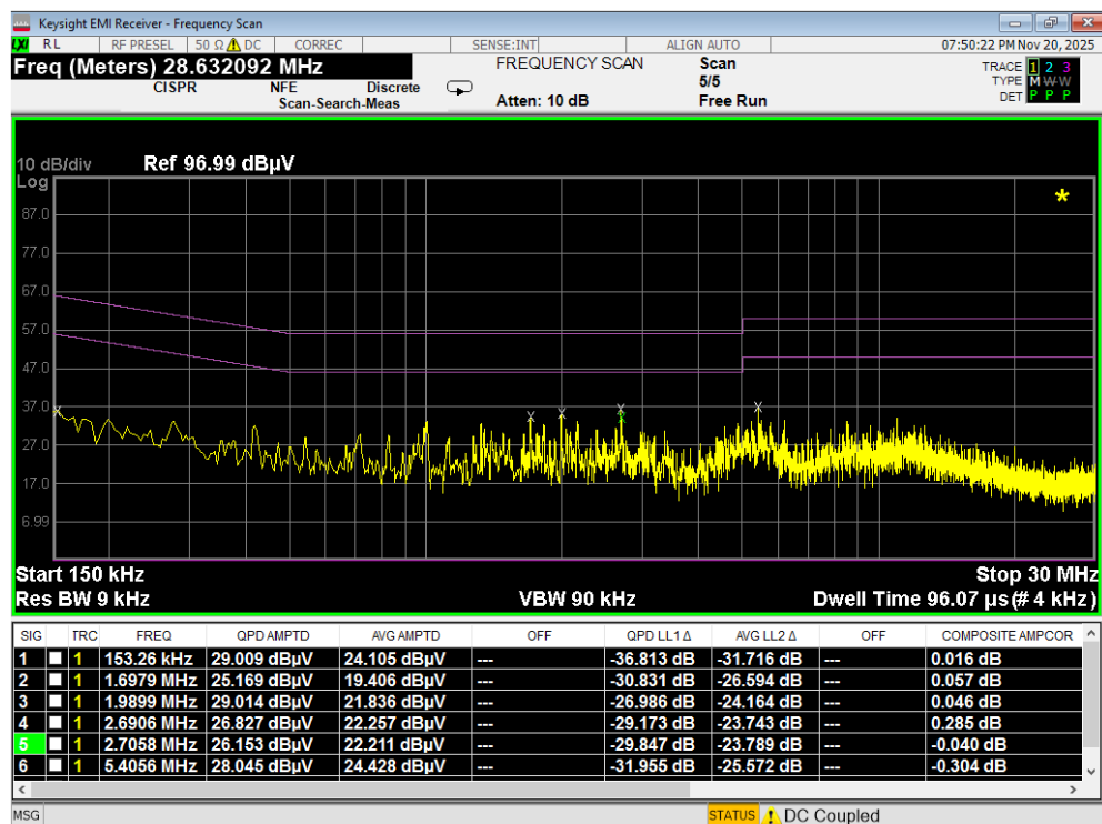
Plot 7-109. Line Conducted Plot with 802.11a UNII Band 6 (L1) with WCP
