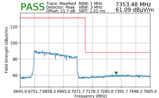
Plot 7-94. Radiated Upper Band Edge Plot MIMO (Peak – UNII Band 8)
