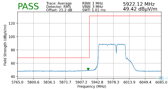
Plot 7-79. Radiated Lower Band Edge Plot MIMO (Average – UNII Band 5)
