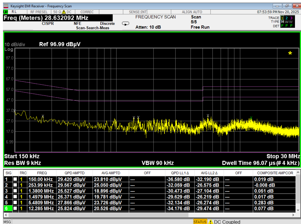
Plot 7-104. Line Conducted Plot with 802.11a UNII Band 7 (N)
