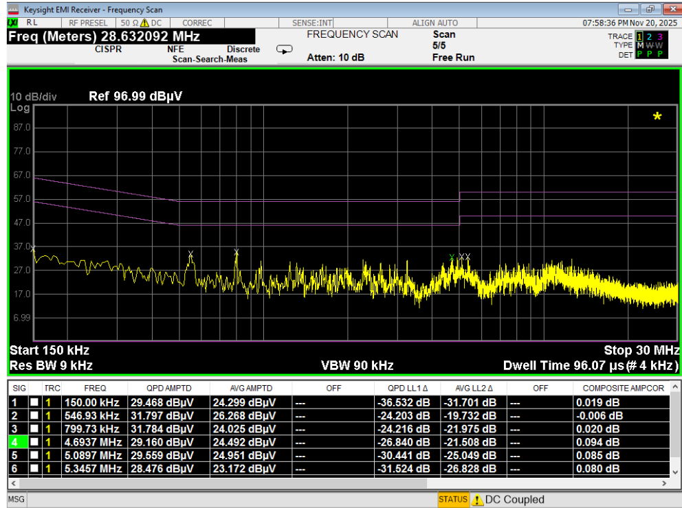
Plot 7-111. Line Conducted Plot with 802.11a UNII Band 7 (L1) with WCP
