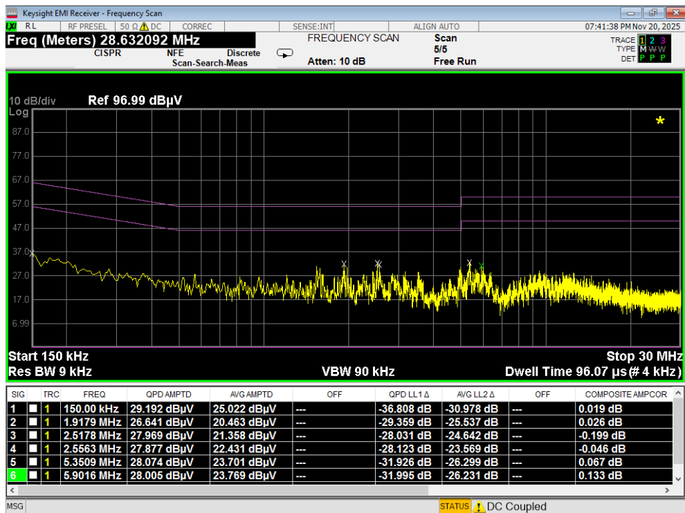
Plot 7-100. Line Conducted Plot with 802.11a UNII Band 5 (N)
