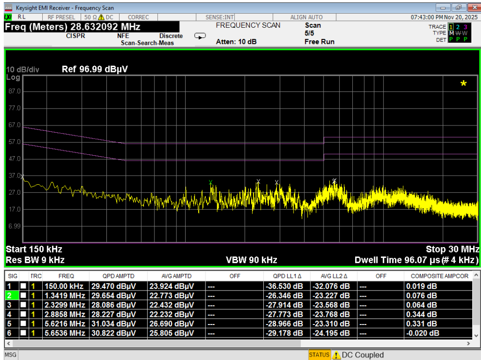
Plot 7-99. Line Conducted Plot with 802.11a UNII Band 5 (L1)
