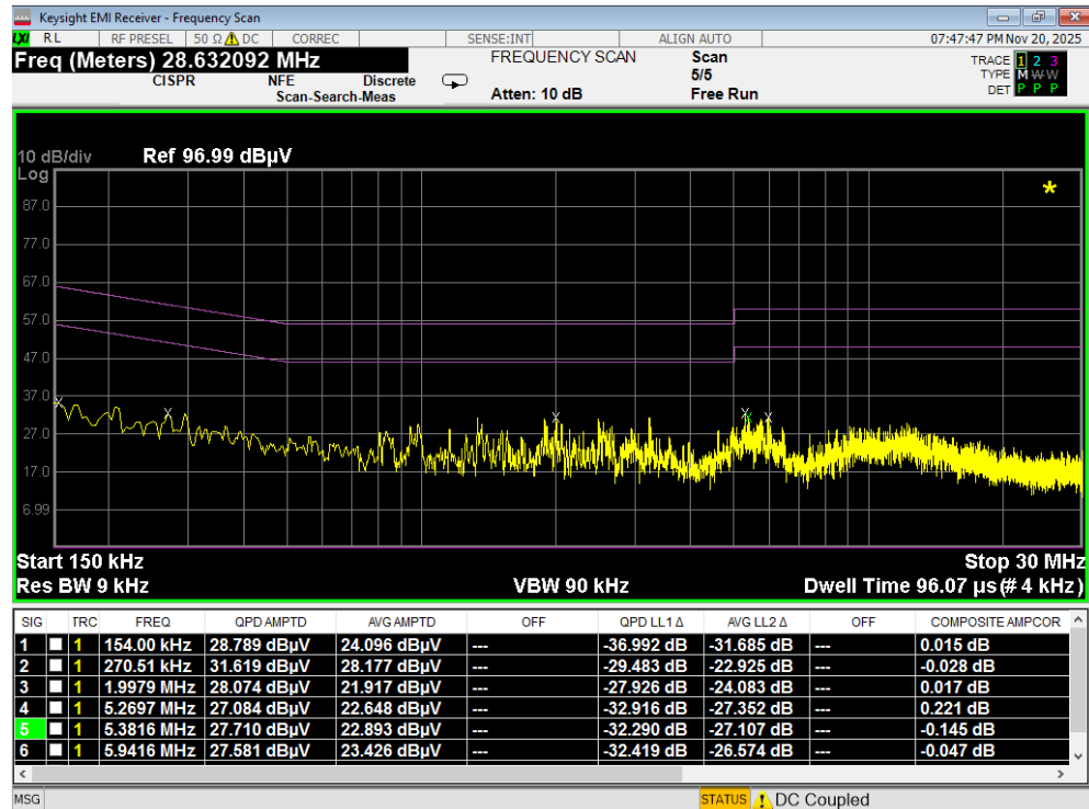
Plot 7-102. Line Conducted Plot with 802.11a UNII Band 6 (N)
