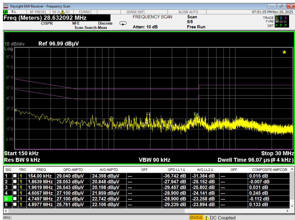
Plot 7-110. Line Conducted Plot with 802.11a UNII Band 6 (N) with WCP
