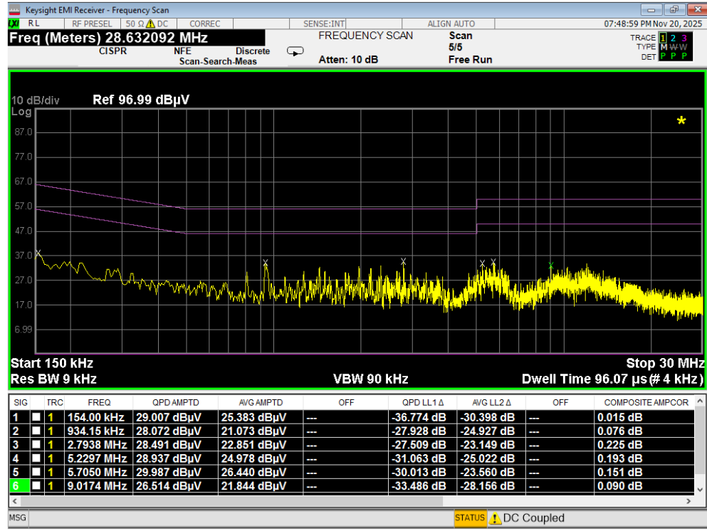
Plot 7-101. Line Conducted Plot with 802.11a UNII Band 6 (L1)
