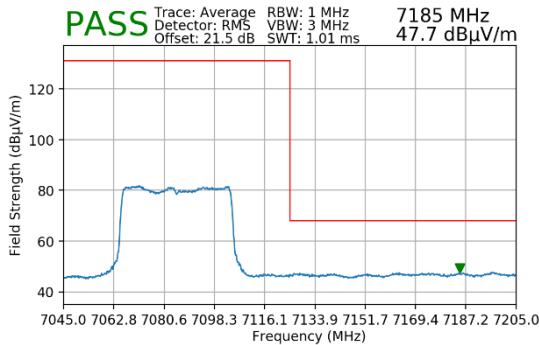
Plot 7-73. Radiated Upper Band Edge Plot MIMO (Average – UNII Band 8)
