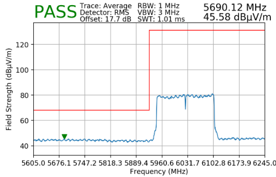
Plot 7-83. Radiated Lower Band Edge Plot MIMO (Average – UNII Band 5)
