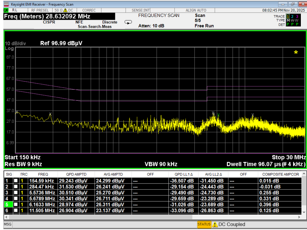
Plot 7-105. Line Conducted Plot with 802.11a UNII Band 8 (L1)
