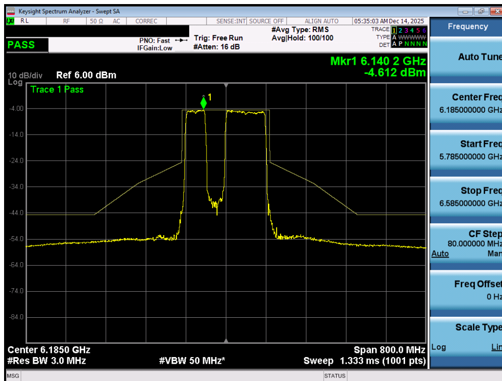
Plot 7-64. In Band Emissions Plot MIMO ANT1 (160MHz 802.11be (996+484 Tones) (UNII Band 5) – Ch. 47) VLP
