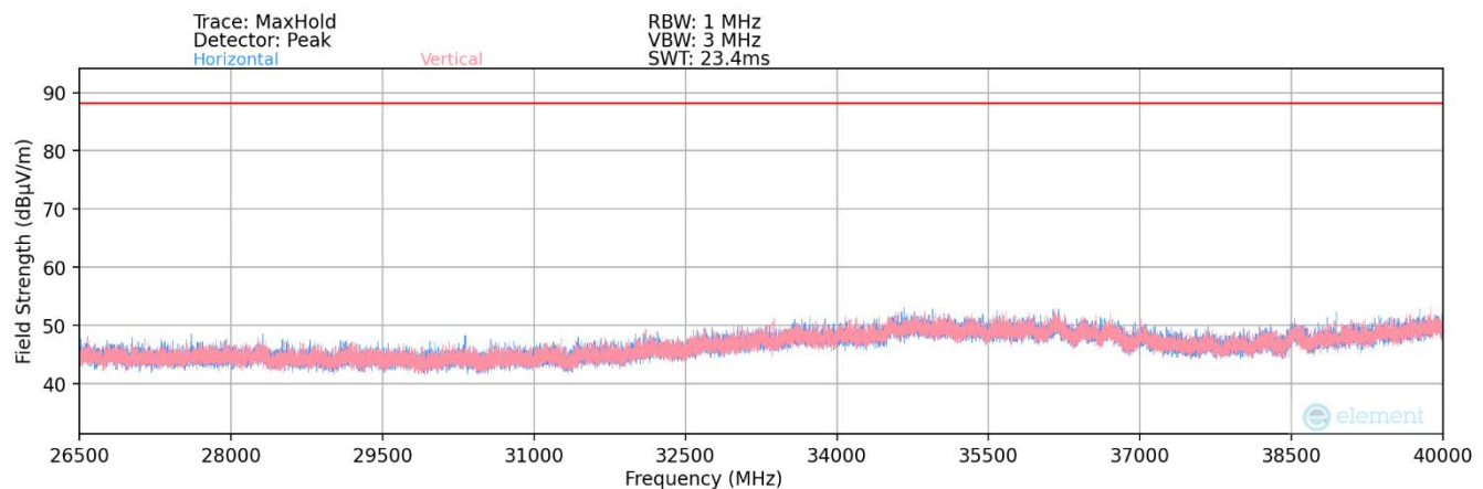
Plot 7-90. Radiated Spurious Plot 26.5GHz - 40GHz (802.11ax) – Ch. 149
