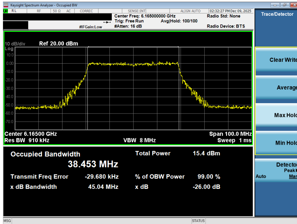
Plot 7-25. 26dB Bandwidth Plot MIMO ANT2 (40MHz 802.11ax/be (Full Tones) (UNII Band 5) – Ch. 43) - VLP
