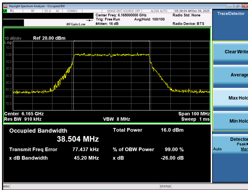
Plot 7-11. 26dB Bandwidth Plot MIMO ANT1 (40MHz 802.11ax/be (Full Tones) (UNII Band 5) – Ch. 43) - VLP
