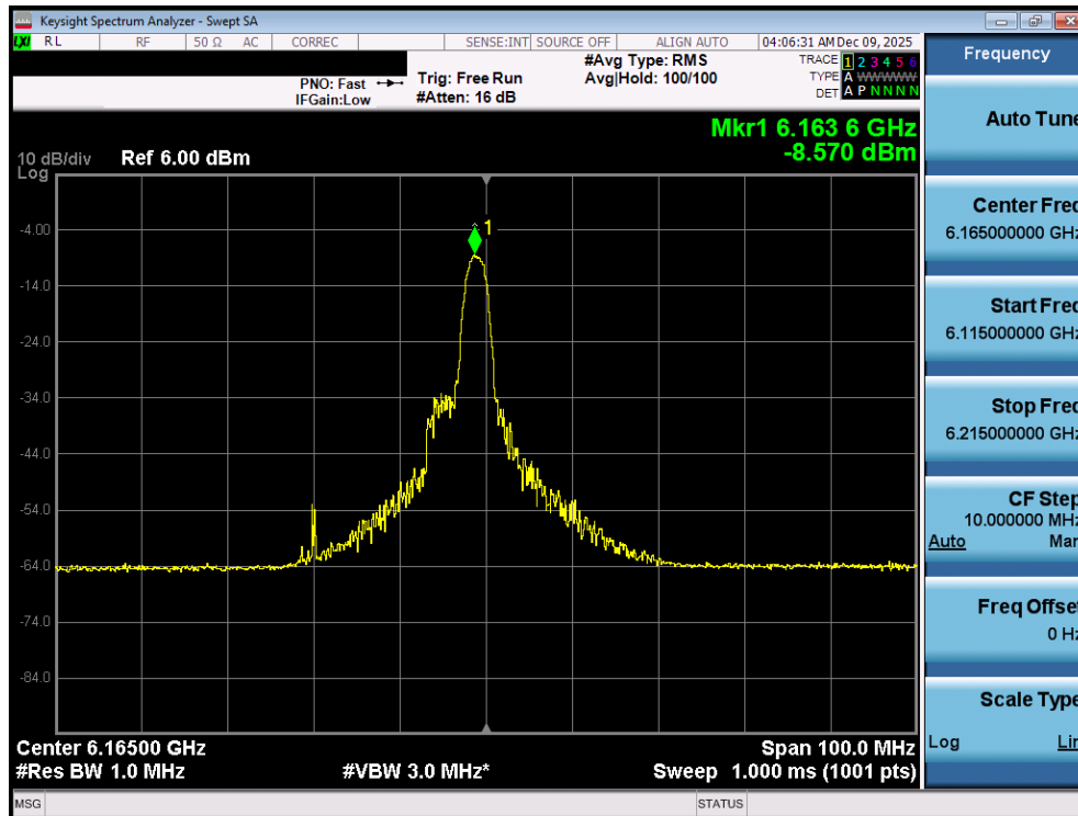
Plot 7-30. Power Spectral Density Plot MIMO ANT1 (40MHz 802.11ax/be (26 Tones) (UNII Band 5) – Ch. 43) - VLP
