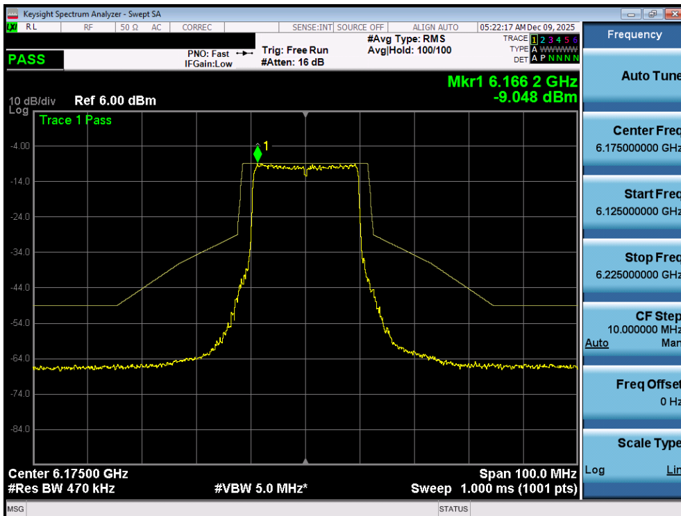
Plot 7-66. In Band Emissions Plot MIMO ANT1 (20MHz 802.11ax/be (Full Tones) (UNII Band 5) – Ch. 45) - VLP
