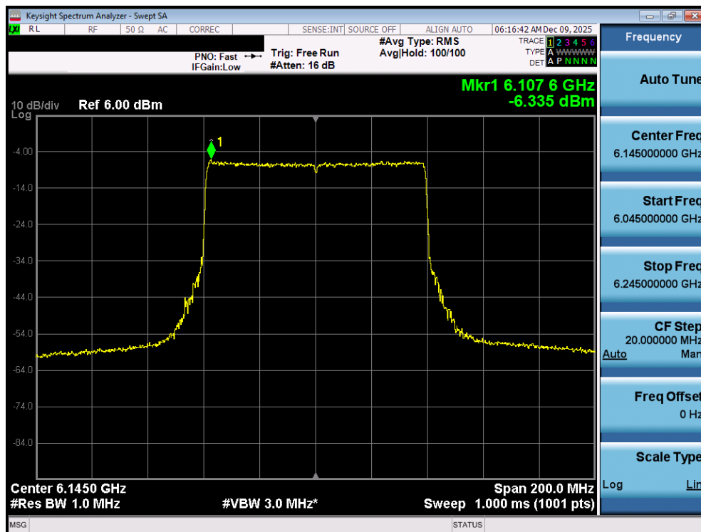
Plot 7-40. Power Spectral Density Plot MIMO ANT1 (80MHz 802.11ax/be (Full Tones) (UNII Band 5) – Ch. 39) - VLP
