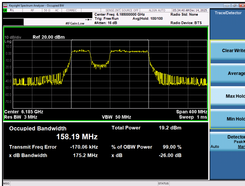
Plot 7-8. 26dB Bandwidth Plot MIMO ANT1 (160MHz 802.11be (996+484 Tones) (UNII Band 5) – Ch. 47) VLP
