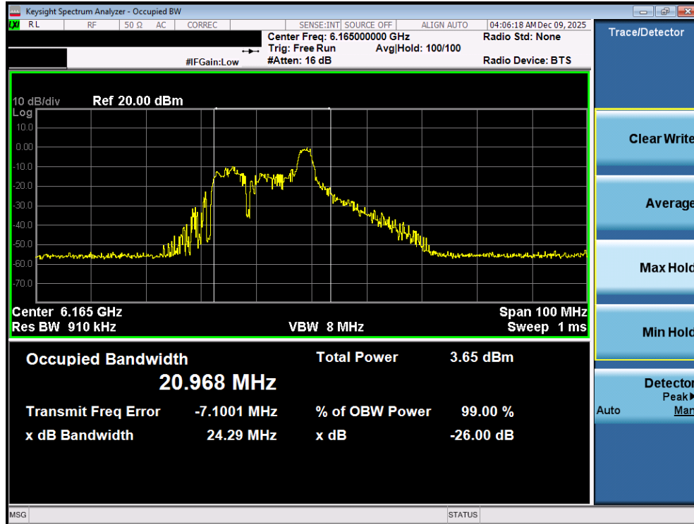
Plot 7-2. 26dB Bandwidth Plot MIMO ANT1 (40MHz 802.11ax/be (26 Tones) (UNII Band 5) – Ch. 43) - VLP
