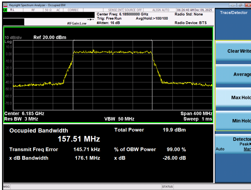
Plot 7-13. 26dB Bandwidth Plot MIMO ANT1 (160MHz 802.11ax/be (Full Tones) (UNII Band 5) – Ch. 47) - VLP
