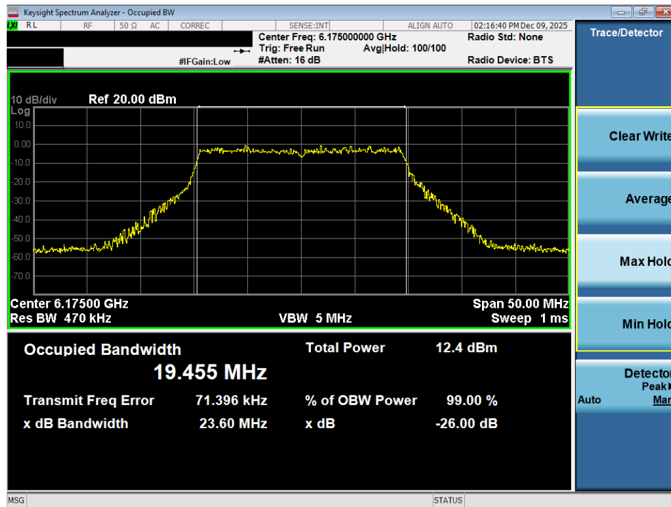
Plot 7-24. 26dB Bandwidth Plot MIMO ANT2 (20MHz 802.11ax/be (Full Tones) (UNII Band 5) – Ch. 45) - VLP
