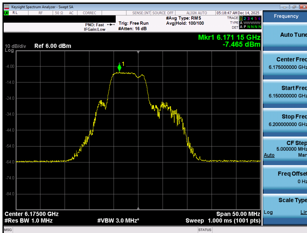
Plot 7-34. Power Spectral Density Plot MIMO ANT1 (20MHz 802.11be (52+26 Tones) (UNII Band 5) – Ch. 45) - VLP
