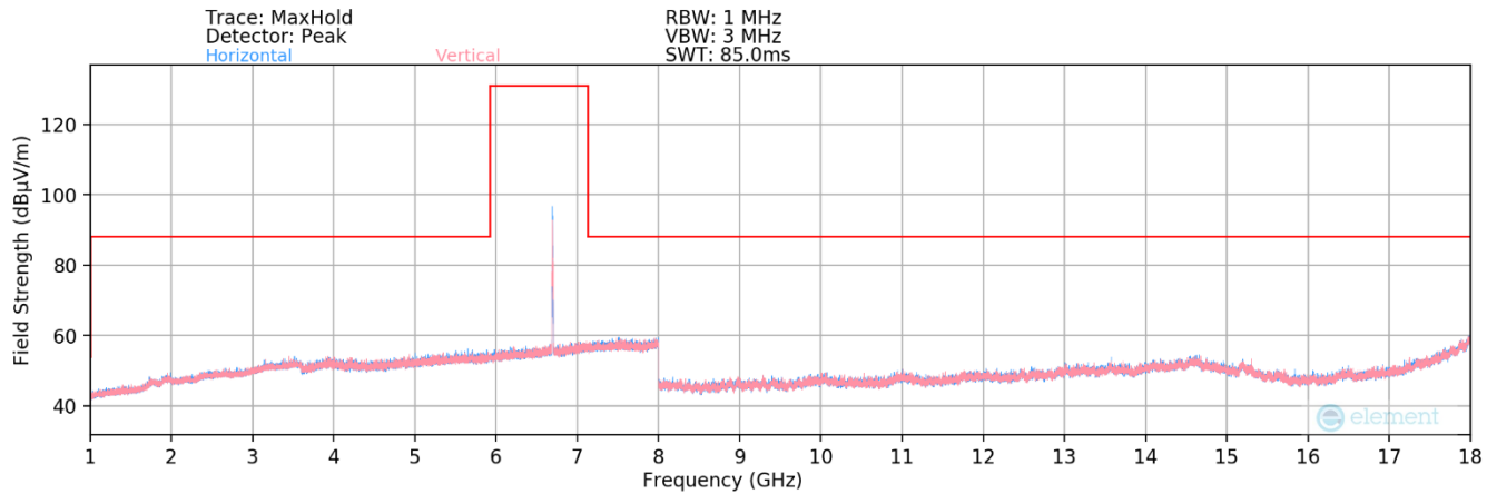
Plot 7-87. Radiated Spurious Plot 1GHz – 18GHz MIMO (802.11ax – UNII Band 7 Ch. 149)
