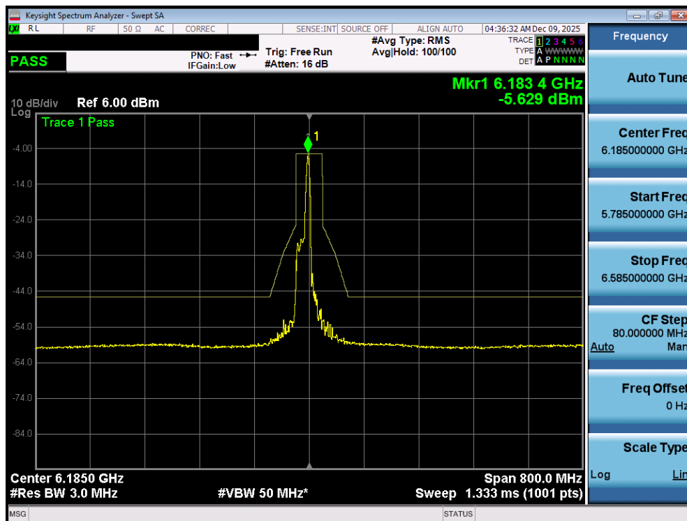
Plot 7-60. In Band Emissions Plot MIMO ANT1 (160MHz 802.11ax/be (26 Tones) (UNII Band 5) – Ch. 47) - VLP
