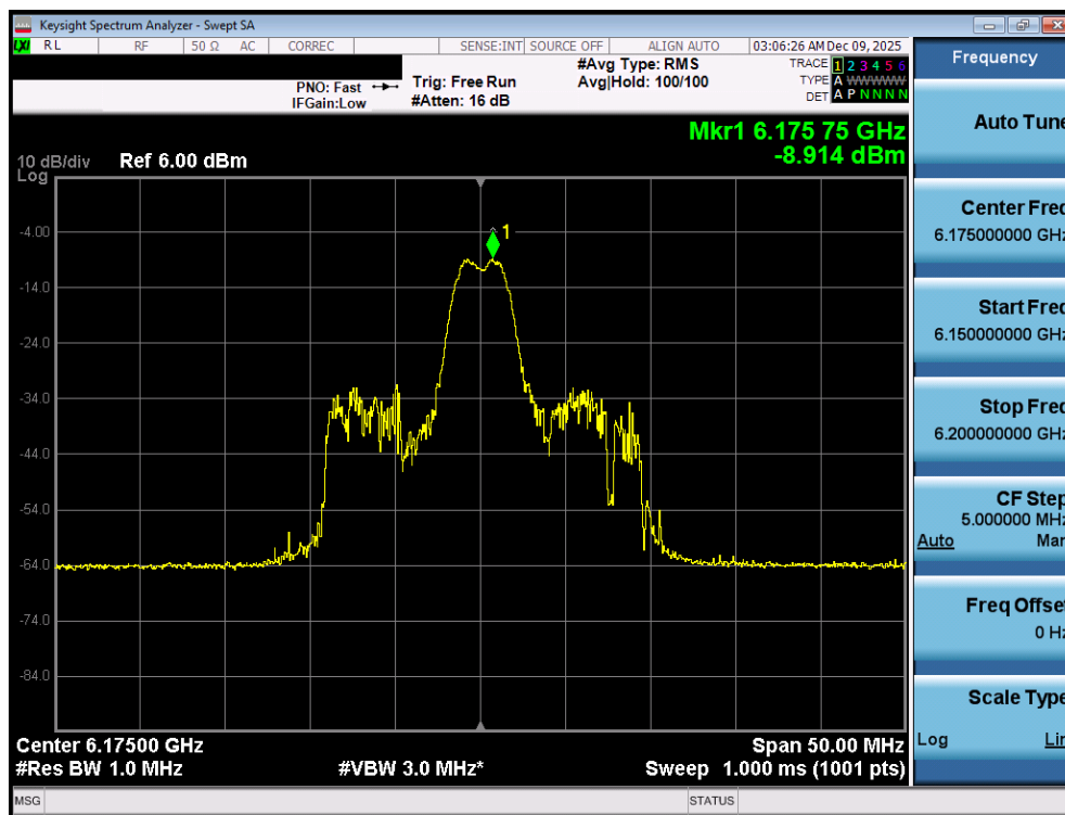
Plot 7-29. Power Spectral Density Plot MIMO ANT1 (20MHz 802.11ax/be (26 Tones) (UNII Band 5) – Ch. 45) - VLP
