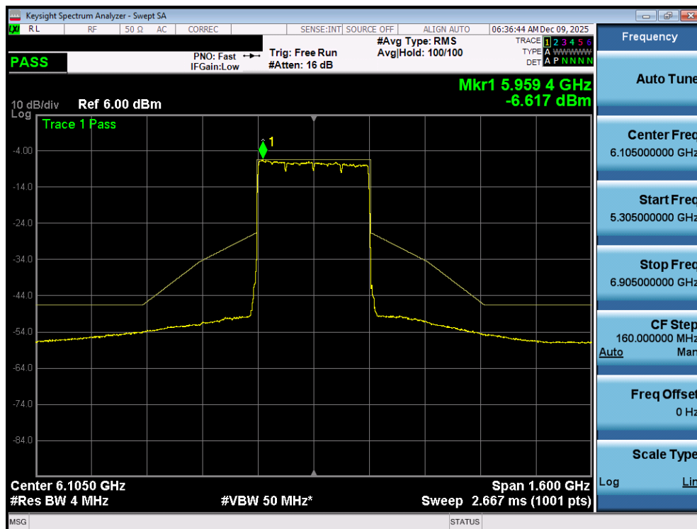
Plot 7-70. In Band Emissions Plot MIMO ANT1 (320MHz 802.11be (Full Tones) (UNII Band 5) – Ch. 31) - VLP
