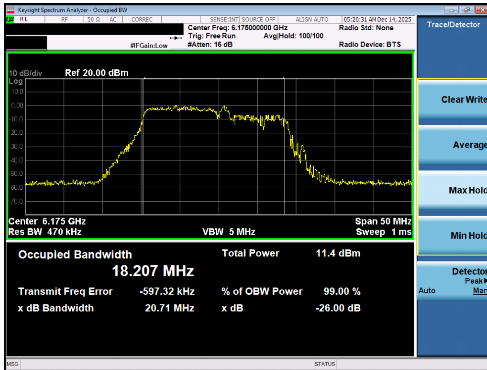
Plot 7-6. 26dB Bandwidth Plot MIMO ANT1 (20MHz 802.11be (106+26 Tones) (UNII Band 5) – Ch. 45) - VLP
