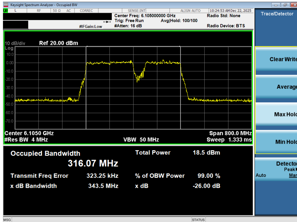
Plot 7-9. 26dB Bandwidth Plot MIMO ANT1 (320MHz 802.11be (3*996+484 Tones) (UNII Band 5) – Ch. 31) VLP
