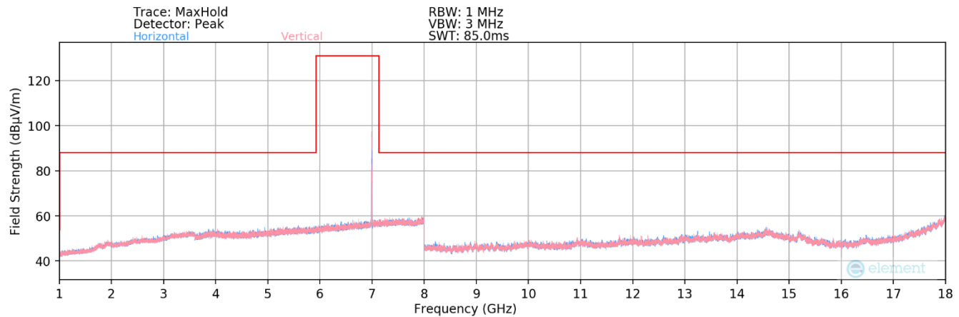
Plot 7-88. Radiated Spurious Plot 1GHz – 18GHz MIMO (802.11ax – U Band 8 Ch. 209)
