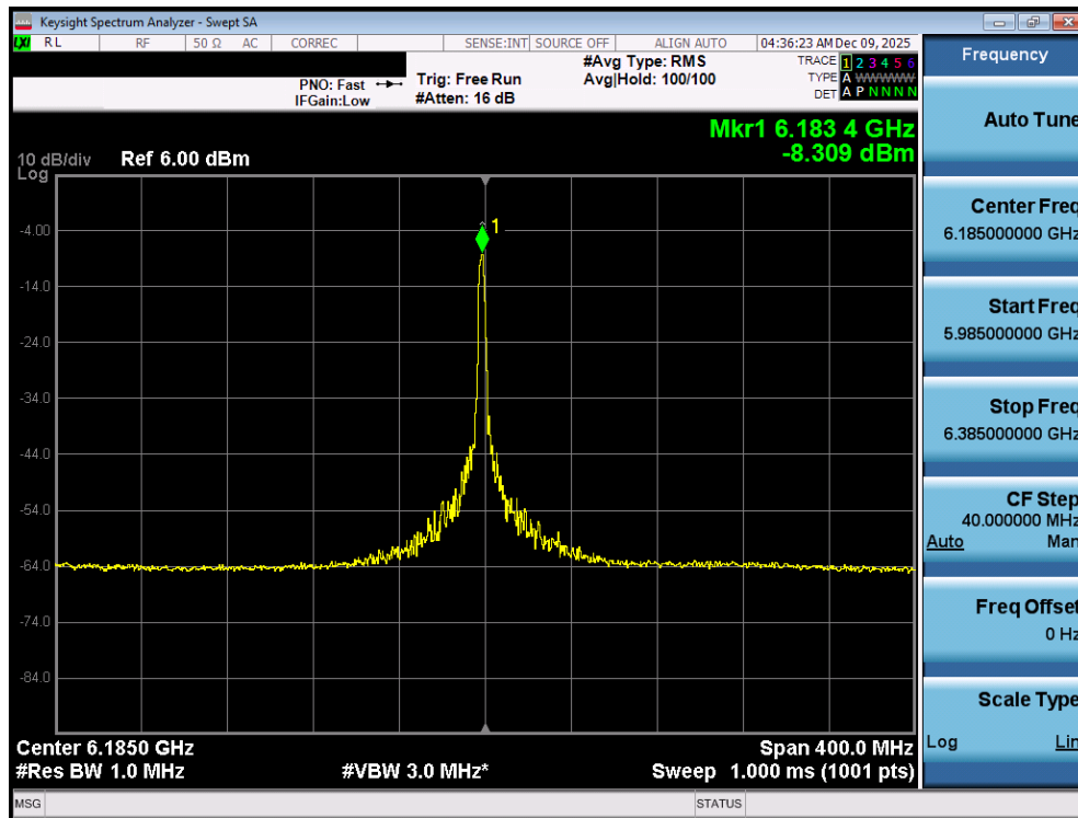
Plot 7-32. Power Spectral Density Plot MIMO ANT1 (160MHz 802.11ax/be (26 Tones) (UNII Band 5) – Ch. 47) - VLP
