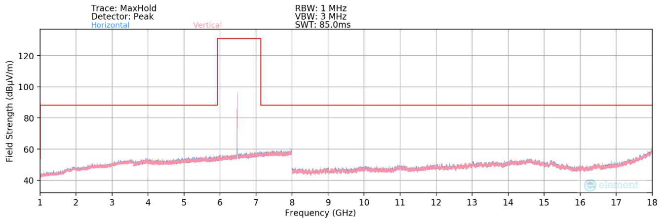
Plot 7-86. Radiated Spurious Plot 1GHz – 18GHz MIMO (802.11ax – UNII Band 6 Ch. 105)
