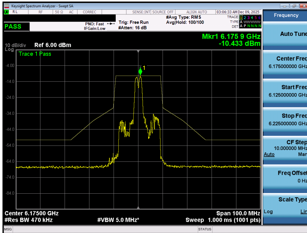
Plot 7-57. In Band Emissions Plot MIMO ANT1 (20MHz 802.11ax/be (26 Tones) (UNII Band 5) – Ch. 45) - VLP
