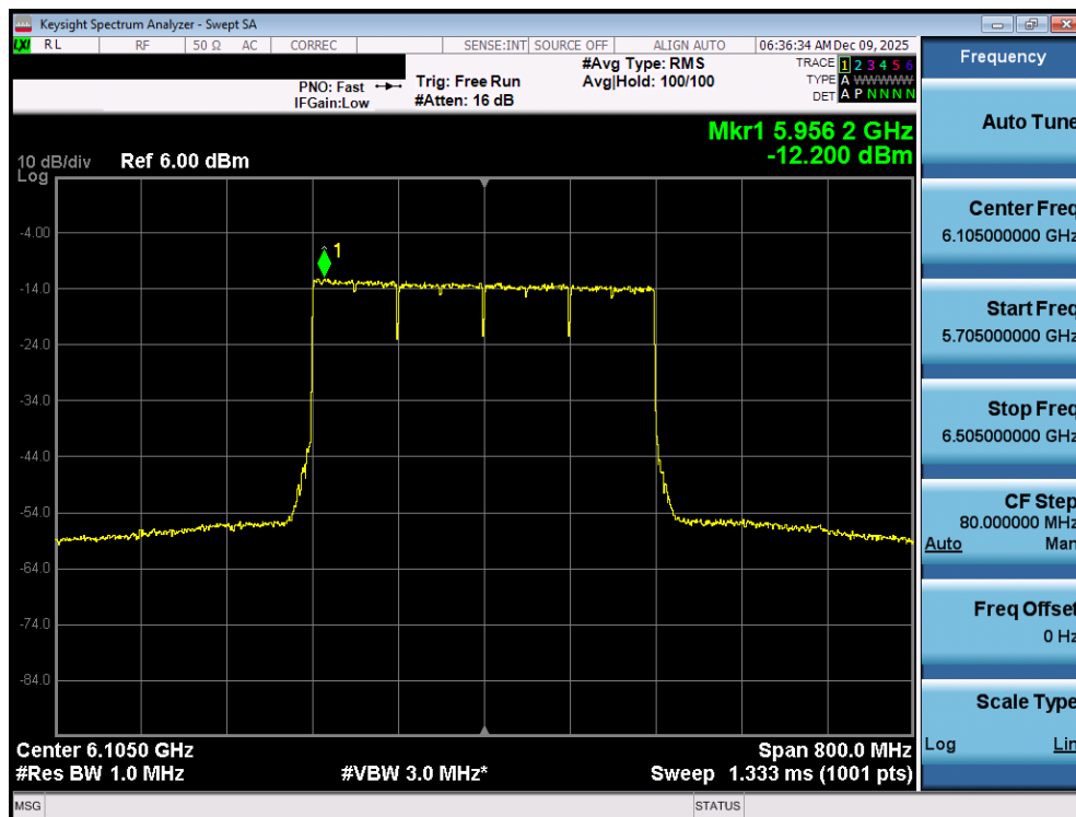
Plot 7-42. Power Spectral Density Plot MIMO ANT1 (320MHz 802.11be (Full Tones) (UNII Band 5) – Ch. 31) - VLP
