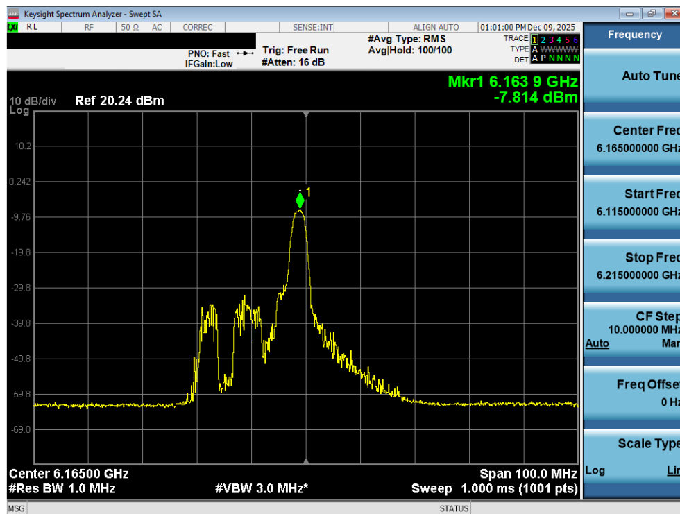
Plot 7-44. Power Spectral Density Plot MIMO ANT2 (40MHz 802.11ax/be (26 Tones) (UNII Band 5) – Ch. 43) - VLP
