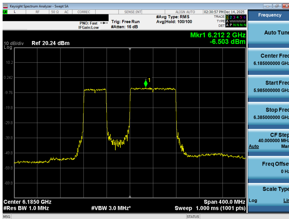
Plot 7-50. Power Spectral Density Plot MIMO ANT2 (160MHz 802.11be (996+484 Tones) (UNII Band 5) – Ch. 47) VLP
