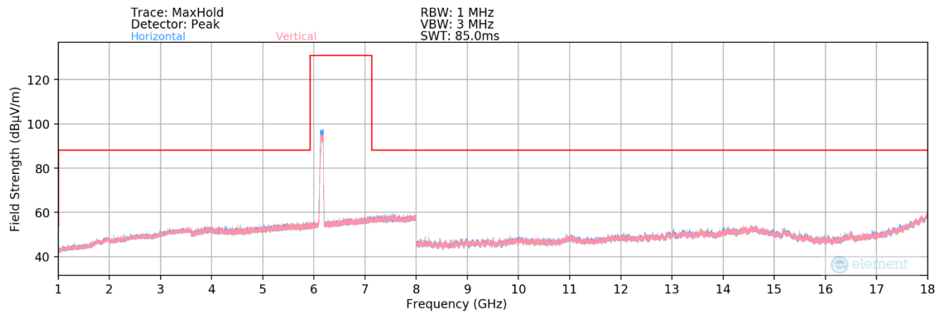
Plot 7-91. Radiated Spurious Plot 1GHz – 18GHz MIMO (802.11be – UNII Band 5 Ch. 39) – 484+242 Tones
