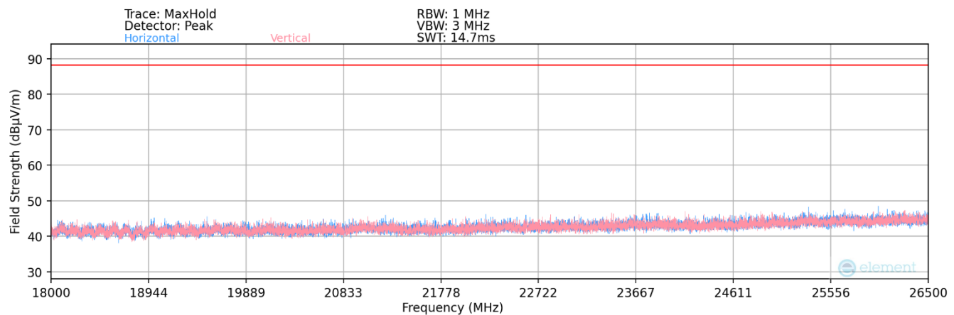
Plot 7-89. Radiated Spurious Plot 18GHz - 26.5GHz (802.11ax) – Ch. 149
