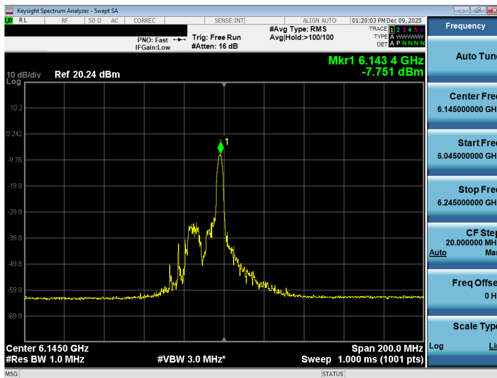
Plot 7-45. Power Spectral Density Plot MIMO ANT2 (80MHz 802.11ax/be (26 Tones) (UNII Band 5) – Ch. 39) - VLP
