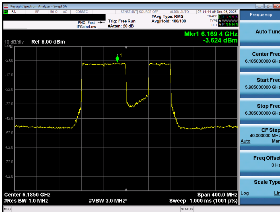
Plot 7-54. Power Spectral Density Plot MIMO ANT1 (160MHz 802.11be (996+484 Tones) (UNII Band 5) – Ch. 47) LPI
