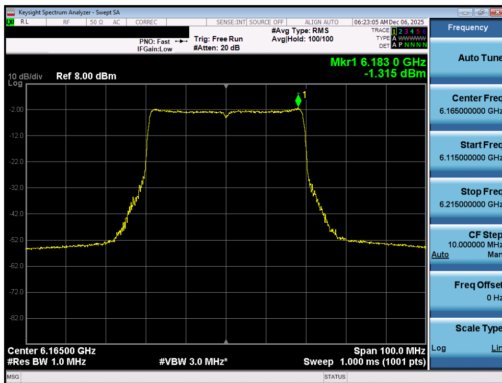
Plot 7-64. Power Spectral Density Plot MIMO ANT1 (40MHz 802.11ax/be (Full Tones) (UNII Band 5) – Ch. 43) - LPI
