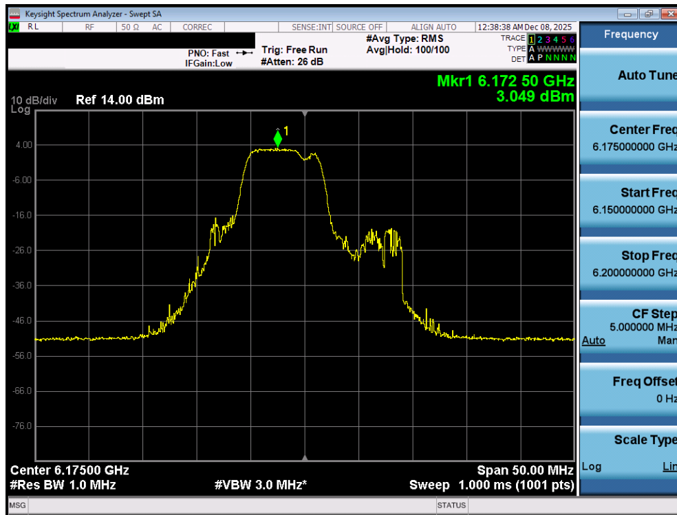
Plot 7-61. Power Spectral Density Plot MIMO ANT1 (20MHz 802.11be (52+26 Tones) (UNII Band 5) – Ch. 45) – SP
