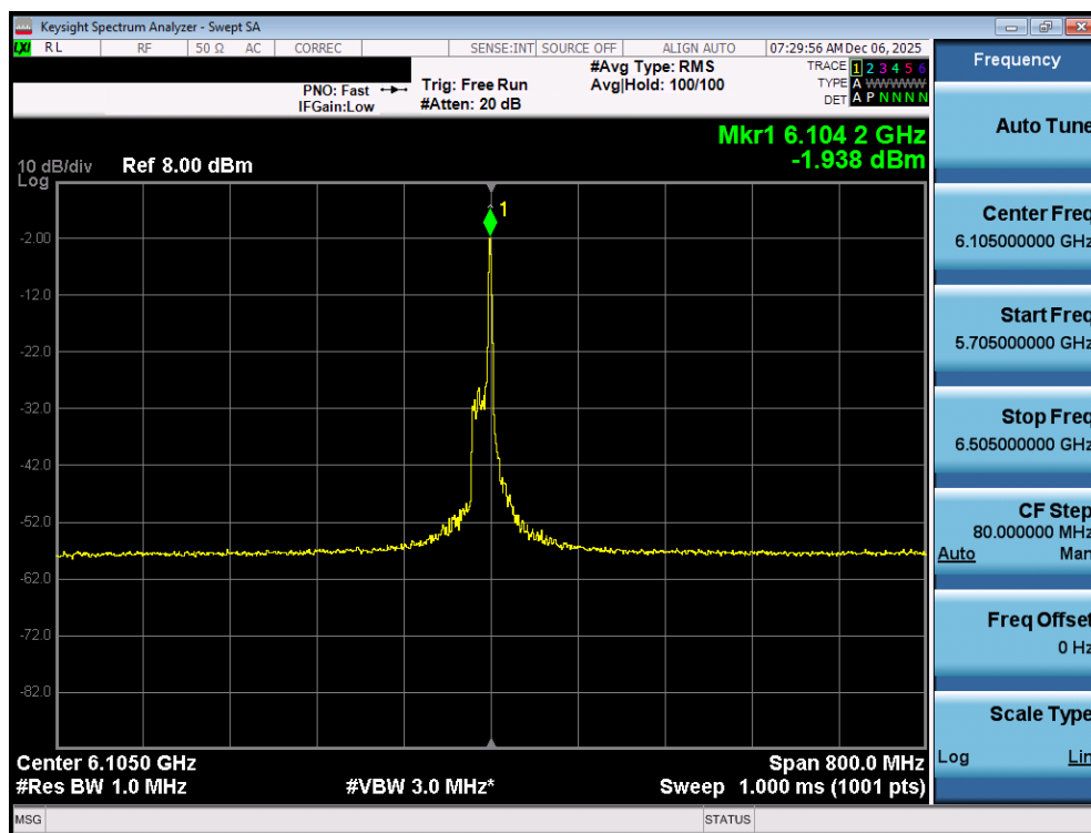
Plot 7-51. Power Spectral Density Plot MIMO ANT1 (320MHz 802.11be (26 Tones) (UNII Band 5) – Ch. 31) - LPI
