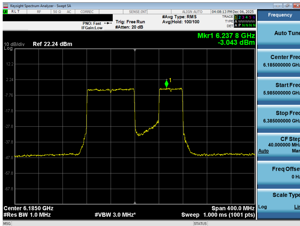
Plot 7-77. Power Spectral Density Plot MIMO ANT2 (160MHz 802.11be (996+484 Tones) (UNII Band 5) – Ch. 47) LPI
