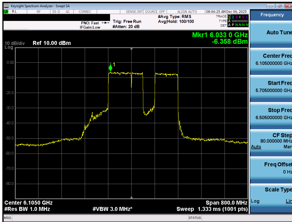
Plot 7-55. Power Spectral Density Plot MIMO ANT1 (320MHz 802.11be (2*996+484 Tones) (UNII Band 5) – Ch. 31) LPI
