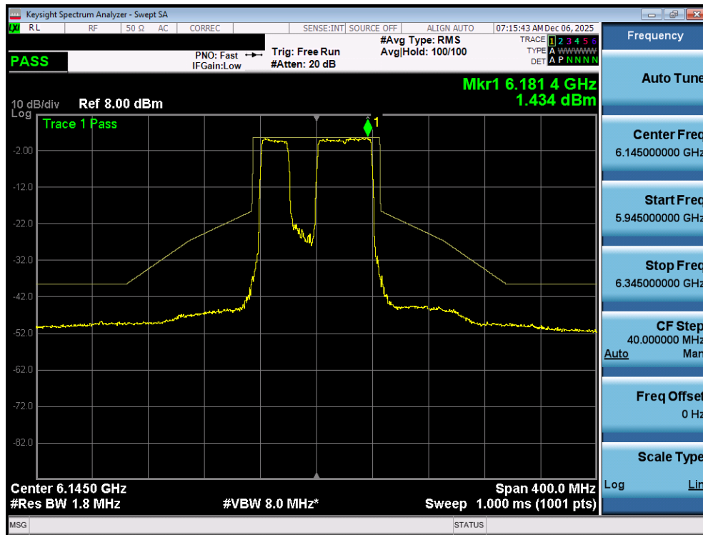
Plot 7-99. In Band Emissions Plot MIMO ANT1 (80MHz 802.11be (484+242 Tones) (UNII Band 5) – Ch. 39) LPI
