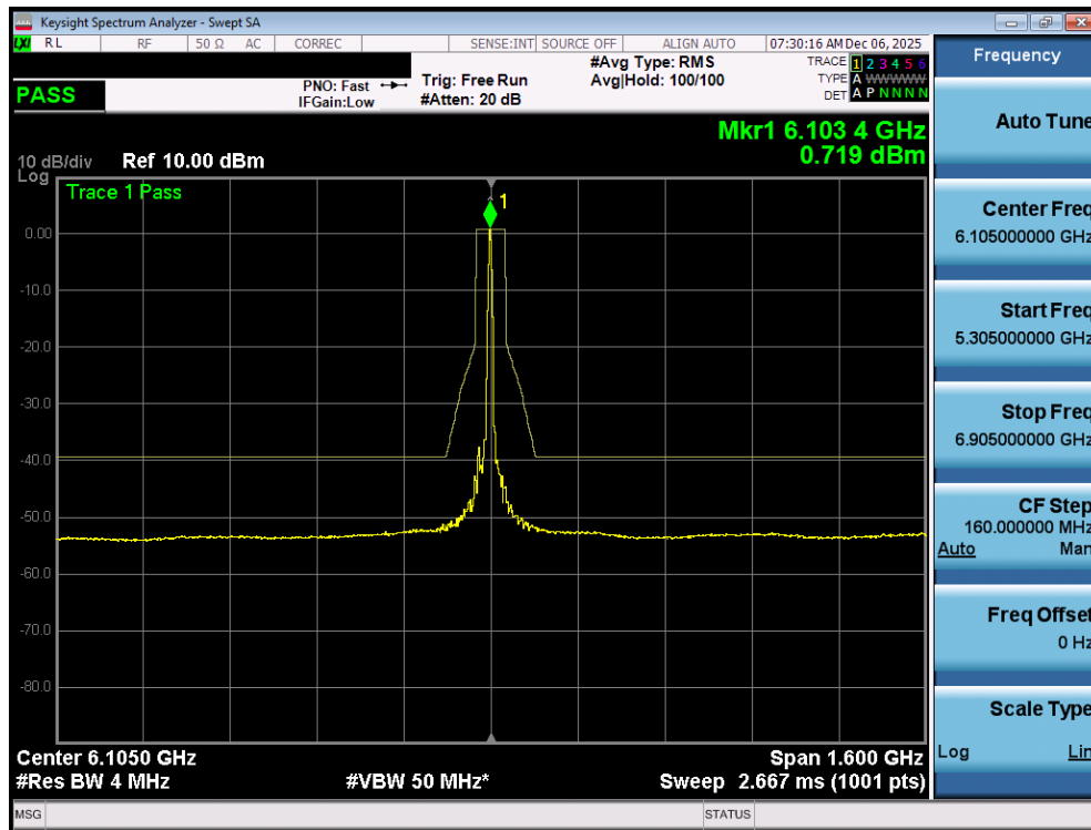
Plot 7-97. In Band Emissions Plot MIMO ANT1 (320MHz 802.11ax/be (26 Tones) (UNII Band 5) – Ch. 31) - LPI
