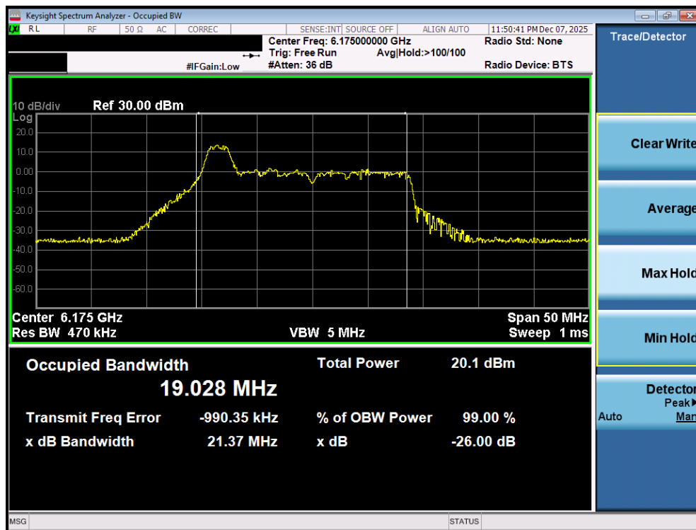
Plot 7-10. 26dB Bandwidth Plot MIMO ANT1 (20MHz 802.11ax/be (26 Tones) (UNII Band 5) – Ch. 45) – SP
