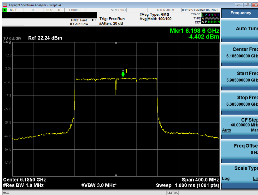
Plot 7-89. Power Spectral Density Plot MIMO ANT2 (160MHz 802.11ax/be (Full Tones) (UNII Band 5) – Ch. 47) - LPI
