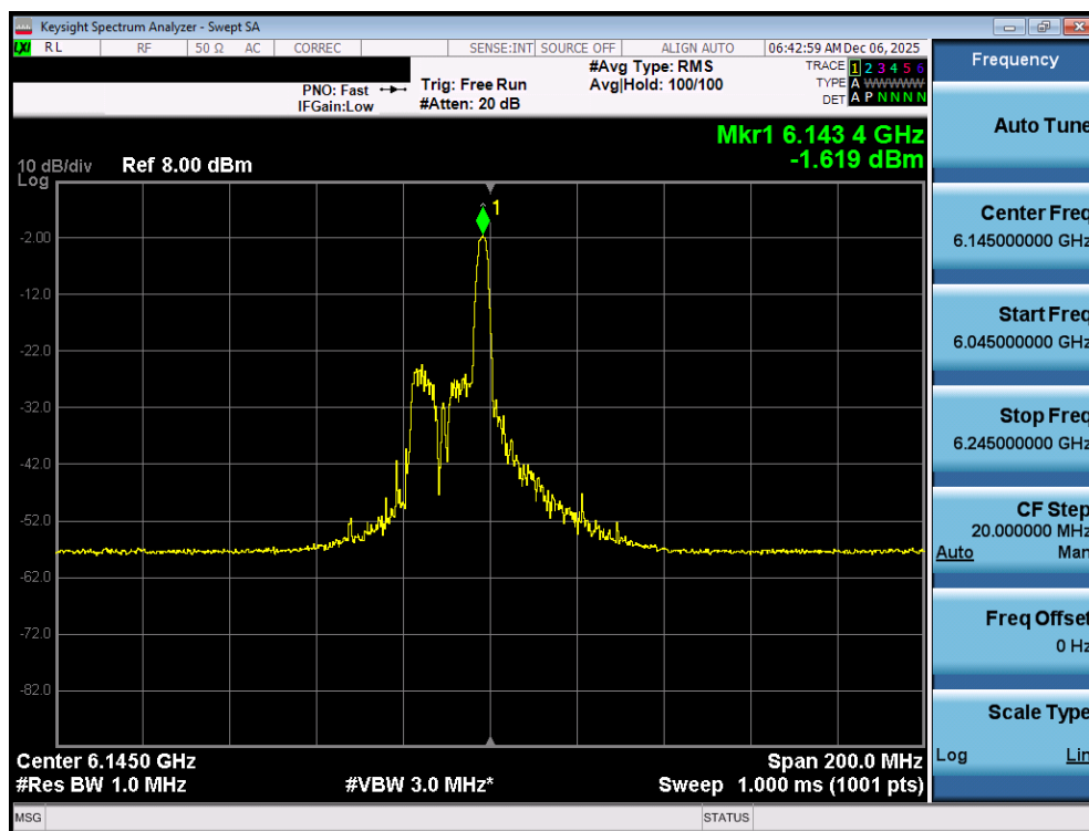
Plot 7-49. Power Spectral Density Plot MIMO ANT1 (80MHz 802.11ax/be (26 Tones) (UNII Band 5) – Ch. 39) - LPI
