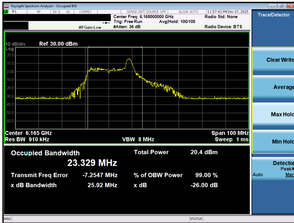
Plot 7-11. 26dB Bandwidth Plot MIMO ANT1 (40MHz 802.11ax/be (26 Tones) (UNII Band 5) – Ch. 43) - SP
