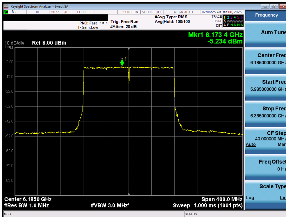
Plot 7-66. Power Spectral Density Plot MIMO ANT1 (160MHz 802.11ax/be (Full Tones) (UNII Band 5) – Ch. 47) - LPI
