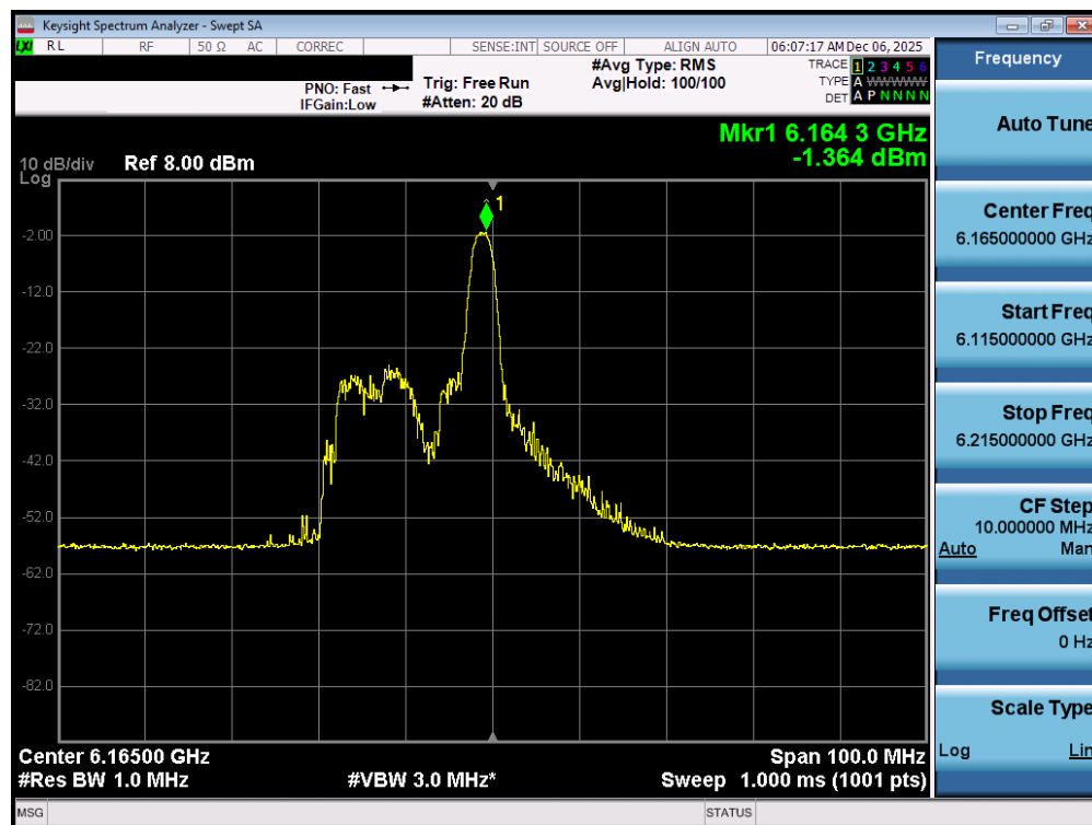
Plot 7-48. Power Spectral Density Plot MIMO ANT1 (40MHz 802.11ax/be (26 Tones) (UNII Band 5) – Ch. 43) - LPI
