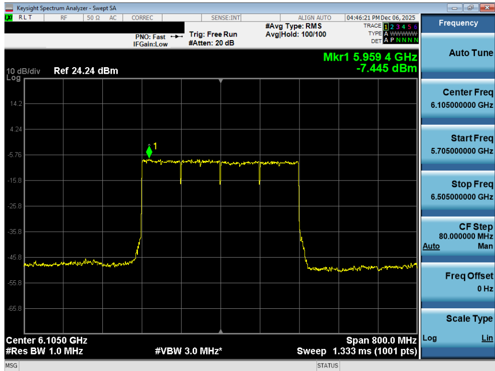
Plot 7-90. Power Spectral Density Plot MIMO ANT2 (320MHz 802.11be (Full Tones) (UNII Band 5) – Ch. 31) - LPI
