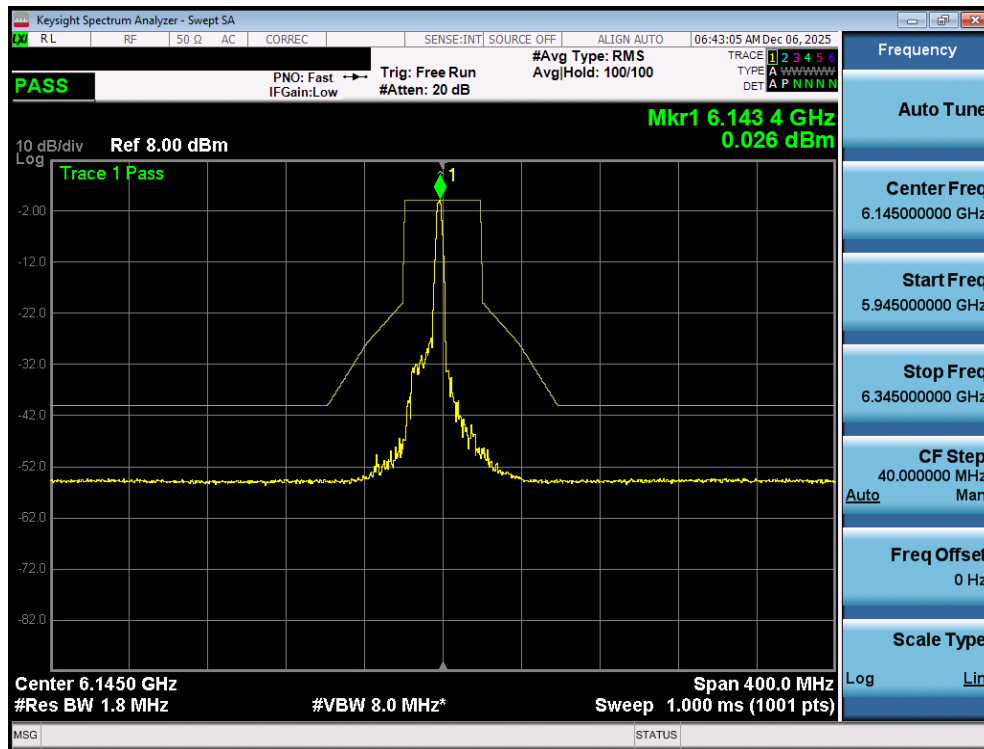
Plot 7-95. In Band Emissions Plot MIMO ANT1 (80MHz 802.11ax/be (26 Tones) (UNII Band 5) – Ch. 39) - LPI
