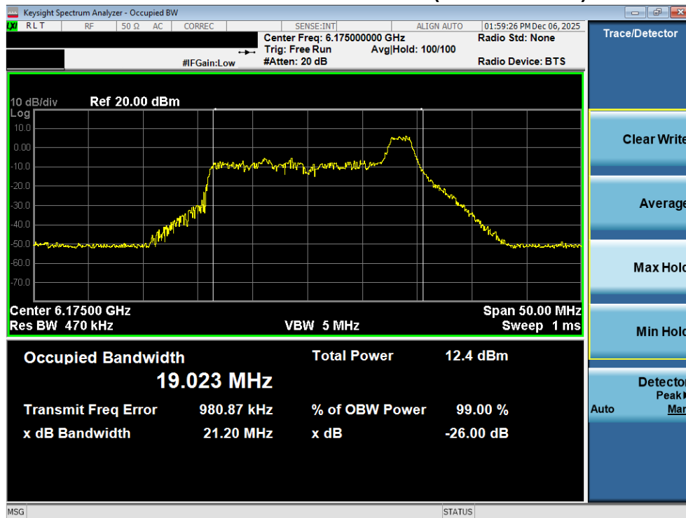
Plot 7-24. 26dB Bandwidth Plot MIMO ANT2 (20MHz 802.11ax/be (26 Tones) (UNII Band 5) – Ch. 45) - LPI
