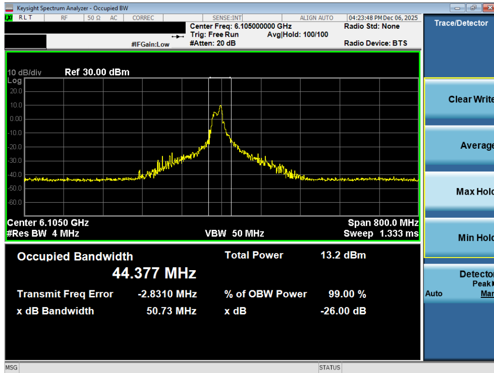
Plot 7-28. 26dB Bandwidth Plot MIMO ANT2 (320MHz 802.11ax/be (26 Tones) (UNII Band 5) – Ch. 31) - LPI
