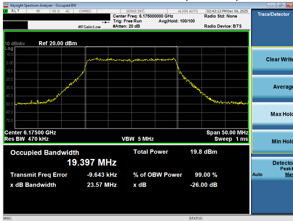
Plot 7-40. 26dB Bandwidth Plot MIMO ANT2 (20MHz 802.11ax/be (Full Tones) (UNII Band 5) – Ch. 45) - LPI
