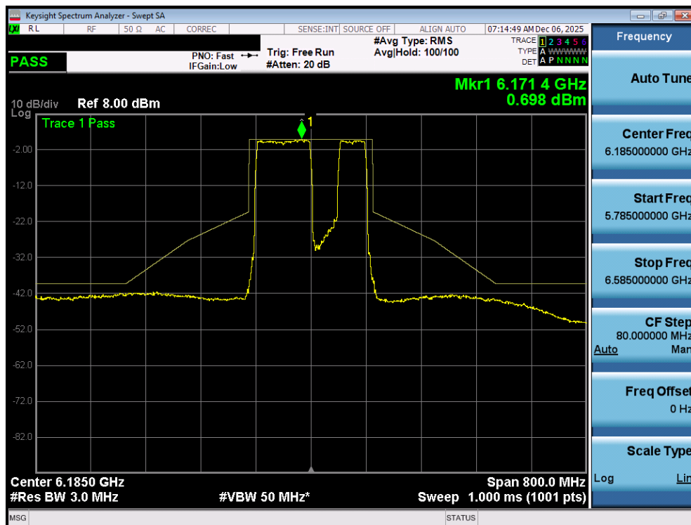
Plot 7-100. In Band Emissions Plot MIMO ANT1 (160MHz 802.11be (996+484 Tones) (UNII Band 5) – Ch. 47) LPI
