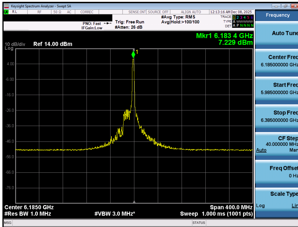
Plot 7-59. Power Spectral Density Plot MIMO ANT1 (160MHz 802.11ax/be (26 Tones) (UNII Band 5) – Ch. 47) - SP
