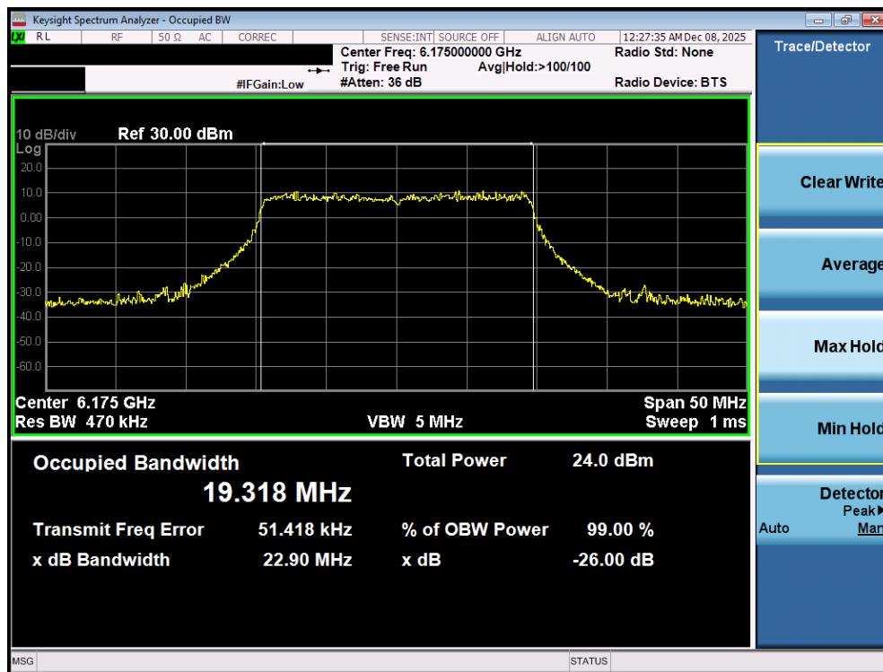
Plot 7-22. 26dB Bandwidth Plot MIMO ANT1 (20MHz 802.11ax/be (Full Tones) (UNII Band 5) – Ch. 45) - SP
