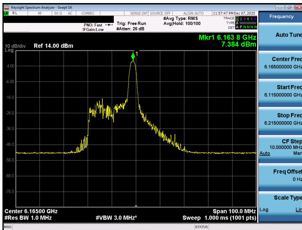
Plot 7-57. Power Spectral Density Plot MIMO ANT1 (40MHz 802.11ax/be (26 Tones) (UNII Band 5) – Ch. 43) - SP
