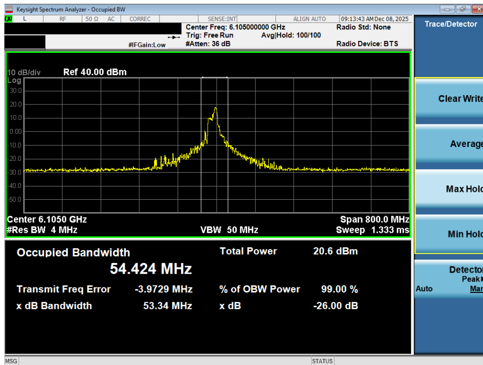
Plot 7-37. 26dB Bandwidth Plot MIMO ANT2 (320MHz 802.11ax/be (26 Tones) (UNII Band 5) – Ch. 31) - SP
