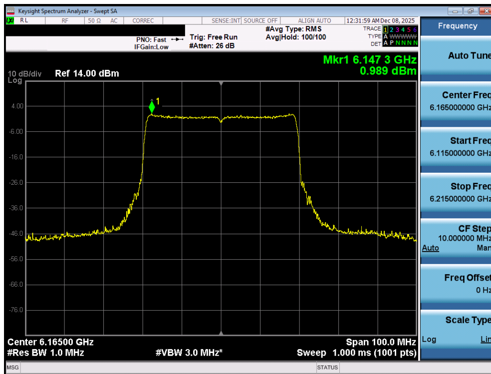
Plot 7-69. Power Spectral Density Plot MIMO ANT1 (40MHz 802.11ax/be (Full Tones) (UNII Band 5) – Ch. 43) - SP
