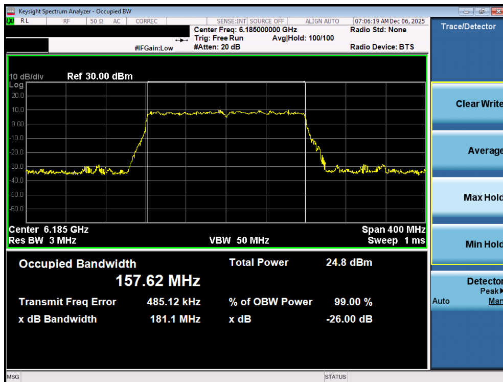
Plot 7-20. 26dB Bandwidth Plot MIMO ANT1 (160MHz 802.11ax/be (Full Tones) (UNII Band 5) – Ch. 47) - LPI
