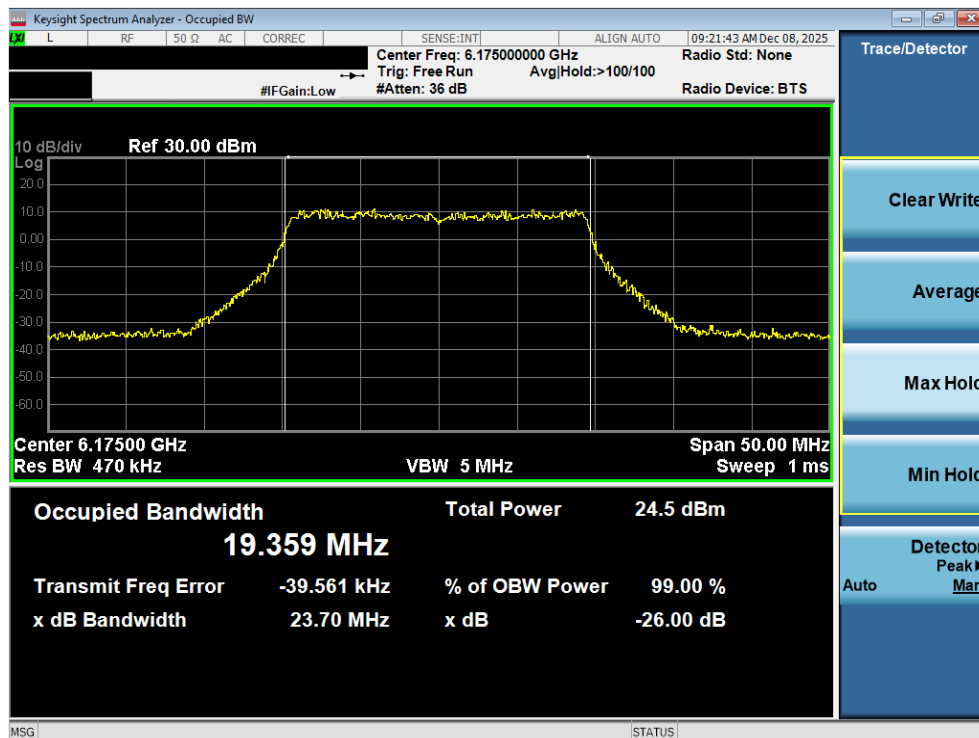
Plot 7-45. 26dB Bandwidth Plot MIMO ANT2 (20MHz 802.11ax/be (Full Tones) (UNII Band 5) – Ch. 45) - SP
