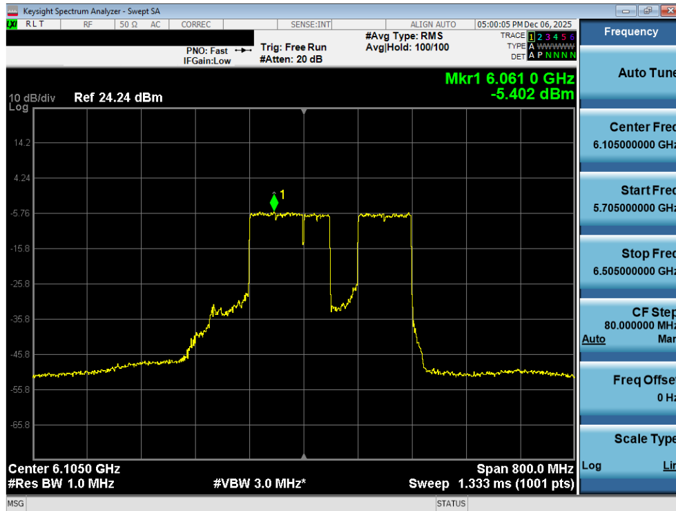
Plot 7-78. Power Spectral Density Plot MIMO ANT2 (320MHz 802.11be (2*996+484 Tones) (UNII Band 5) – Ch. 31) LPI
