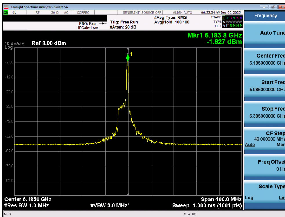
Plot 7-50. Power Spectral Density Plot MIMO ANT1 (160MHz 802.11ax/be (26 Tones) (UNII Band 5) – Ch. 47) - LPI
