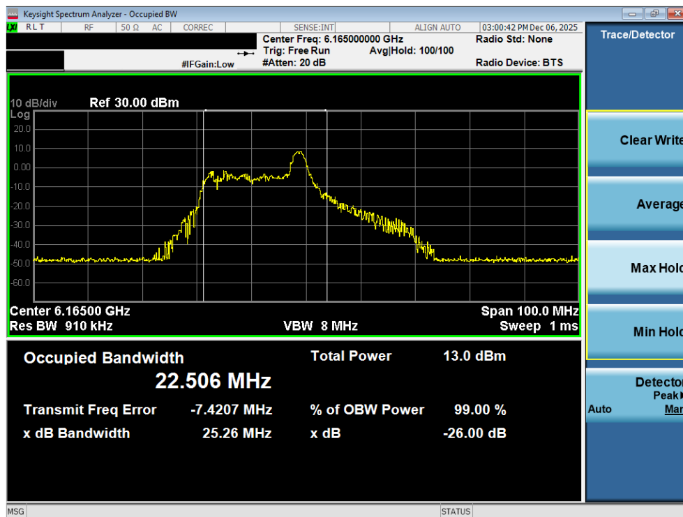
Plot 7-25. 26dB Bandwidth Plot MIMO ANT2 (40MHz 802.11ax/be (26 Tones) (UNII Band 5) – Ch. 43) - LPI
