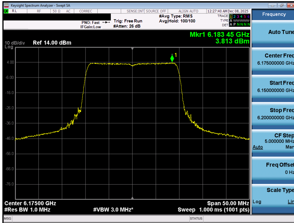
Plot 7-68. Power Spectral Density Plot MIMO ANT1 (20MHz 802.11ax/be (Full Tones) (UNII Band 5) – Ch. 45) - SP
