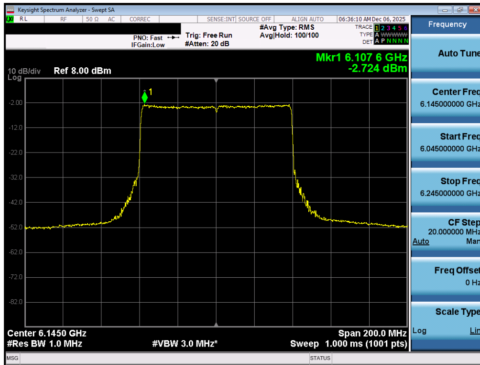
Plot 7-65. Power Spectral Density Plot MIMO ANT1 (80MHz 802.11ax/be (Full Tones) (UNII Band 5) – Ch. 39) - LPI
