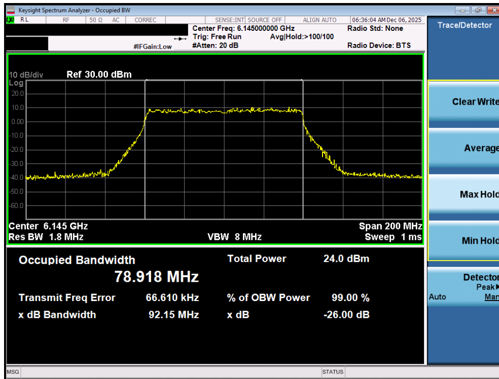
Plot 7-19. 26dB Bandwidth Plot MIMO ANT1 (80MHz 802.11ax/be (Full Tones) (UNII Band 5) – Ch. 39) - LPI
