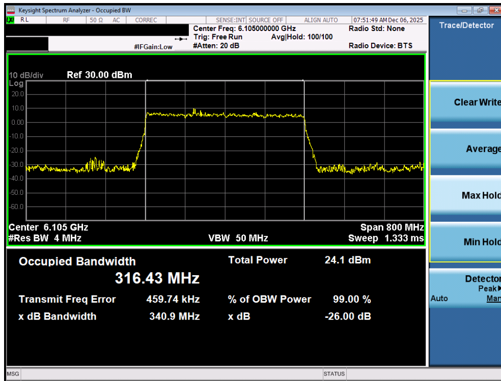
Plot 7-21. 26dB Bandwidth Plot MIMO ANT1 (320MHz 802.11be (Full Tones) (UNII Band 5) – Ch. 31) - LPI
