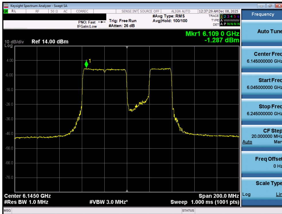
Plot 7-62. Power Spectral Density Plot MIMO ANT1 (80MHz 802.11be (484+242 Tones) (UNII Band 5) – Ch. 39) SP
