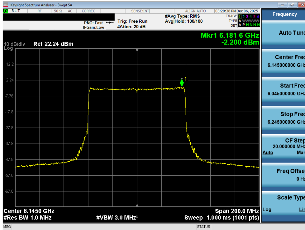
Plot 7-88. Power Spectral Density Plot MIMO ANT2 (80MHz 802.11ax/be (Full Tones) (UNII Band 5) – Ch. 39) - LPI
