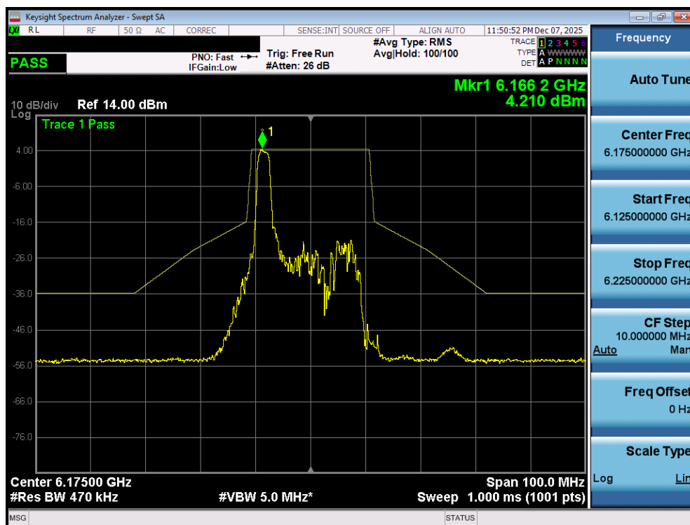
Plot 7-102. In Band Emissions Plot MIMO ANT1 (20MHz 802.11ax/be (26 Tones) (UNII Band 5) – Ch. 45) - SP
