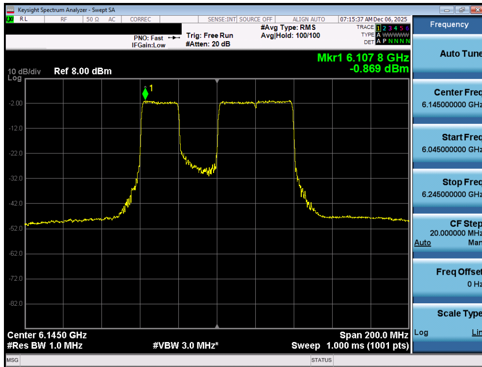
Plot 7-53. Power Spectral Density Plot MIMO ANT1 (80MHz 802.11be (484+242 Tones) (UNII Band 5) – Ch. 39) LPI
