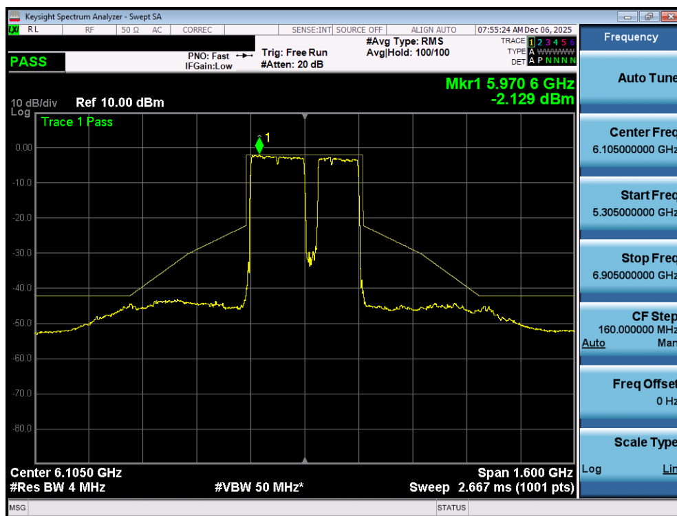
Plot 7-101. In Band Emissions Plot MIMO ANT1 (320MHz 802.11be (3*996+484 Tones) (UNII Band 5) – Ch. 31) LPI
