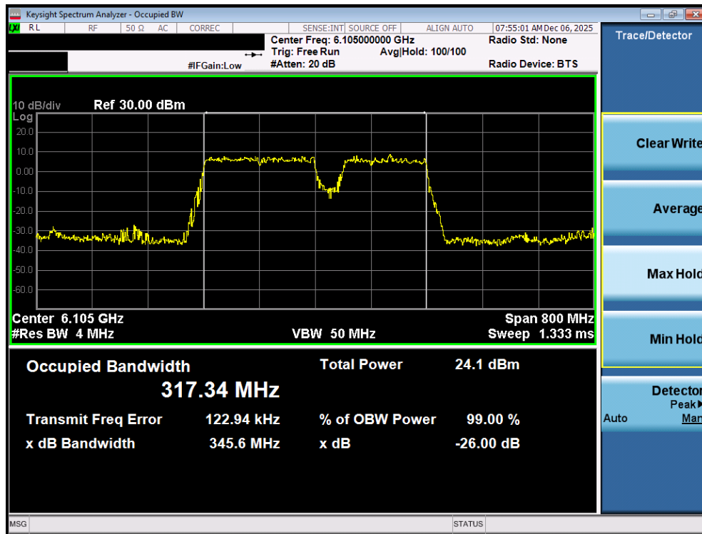
Plot 7-9. 26dB Bandwidth Plot MIMO ANT1 (320MHz 802.11be (3*996+484 Tones) (UNII Band 5) – Ch. 31) LPI/SP
