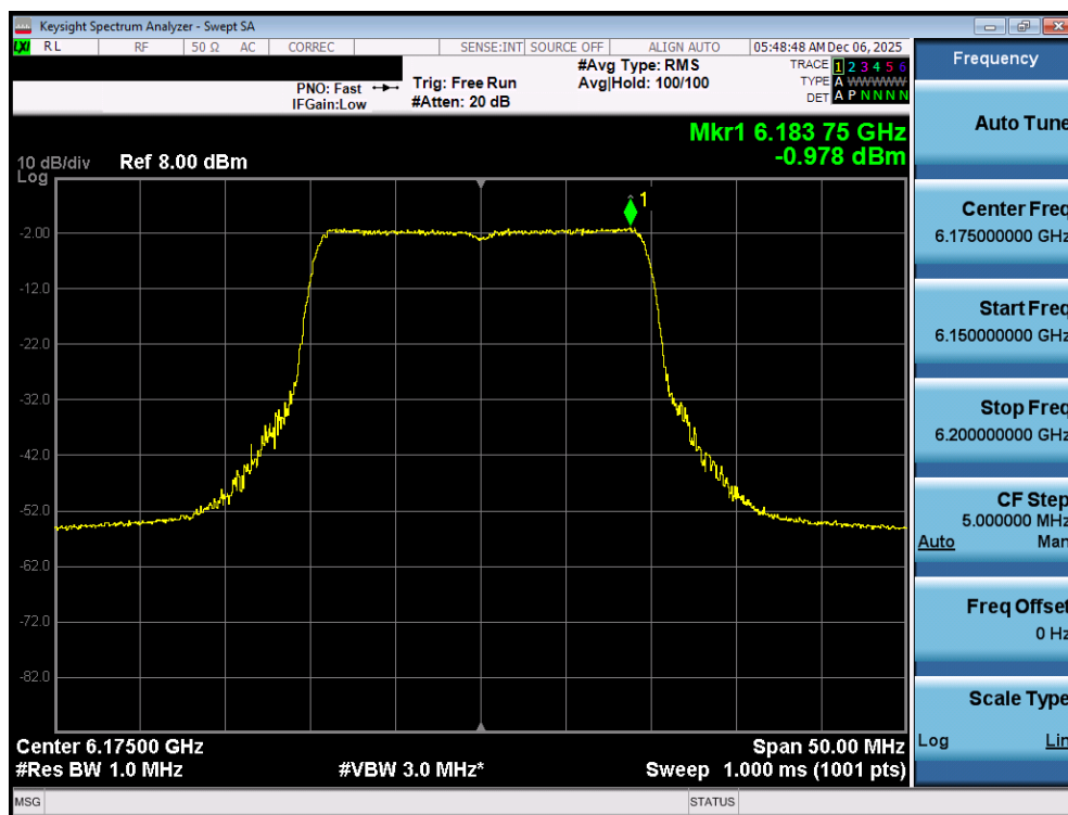
Plot 7-63. Power Spectral Density Plot MIMO ANT1 (20MHz 802.11ax/be (Full Tones) (UNII Band 5) – Ch. 45) - LPI
