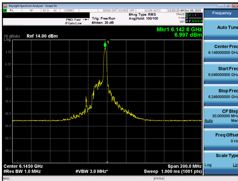
Plot 7-58. Power Spectral Density Plot MIMO ANT1 (80MHz 802.11ax/be (26 Tones) (UNII Band 5) – Ch. 39) – SP
