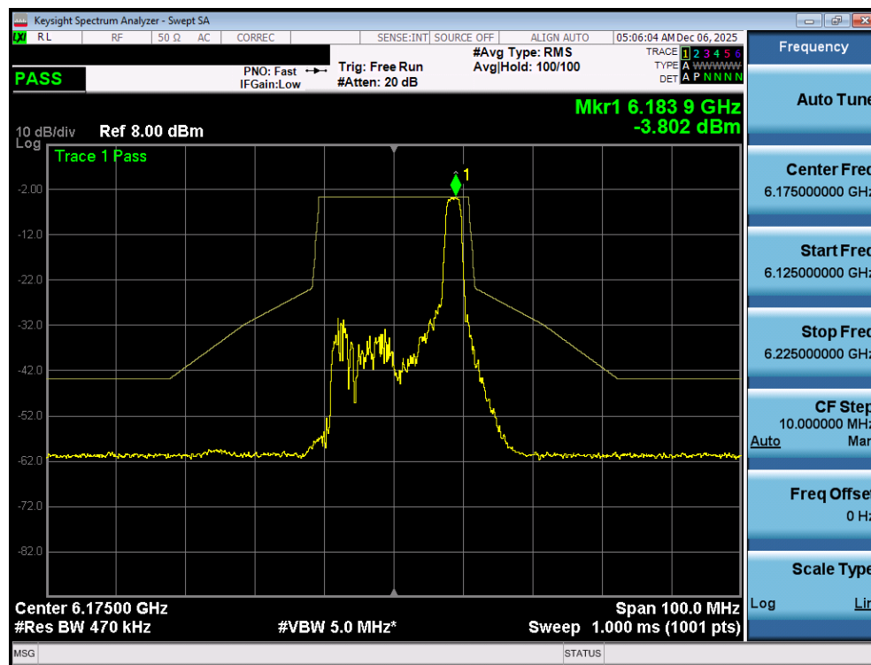
Plot 7-93. In Band Emissions Plot MIMO ANT1 (20MHz 802.11ax/be (26 Tones) (UNII Band 5) – Ch. 45) - LPI
