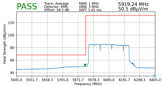
Plot 7-189. Radiated Lower Band Edge Plot MIMO (Average – UNII Band 5 – 3*996+484T)
