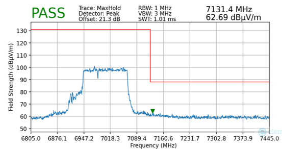
Plot 7-184. Radiated Upper Band Edge Plot MIMO (Peak – UNII Band 8 – 996+484T)
