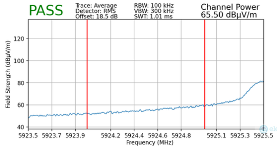
Plot 7-157. Radiated Lower Band Edge Plot MIMO (Average – UNII Band 5 – 106+26T)
