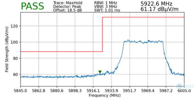
Plot 7-166. Radiated Lower Band Edge Plot MIMO (Peak – UNII Band 5 – 484T)
