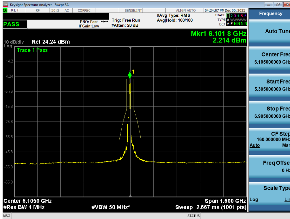
Plot 7-120. In Band Emissions Plot MIMO ANT2 (320MHz 802.11ax/be (26 Tones) (UNII Band 5) – Ch. 31) - LPI
