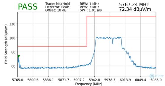
Plot 7-174. Radiated Lower Band Edge Plot MIMO (Peak – UNII Band 5 – 484+242T)
