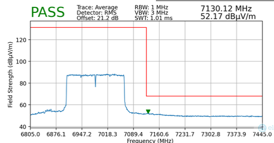
Plot 7-179. Radiated Upper Band Edge Plot MIMO (Average – UNII Band 8 – 2x996T)
