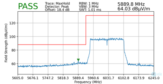
Plot 7-178. Radiated Lower Band Edge Plot MIMO (Peak – UNII Band 5 – 2x996T)
