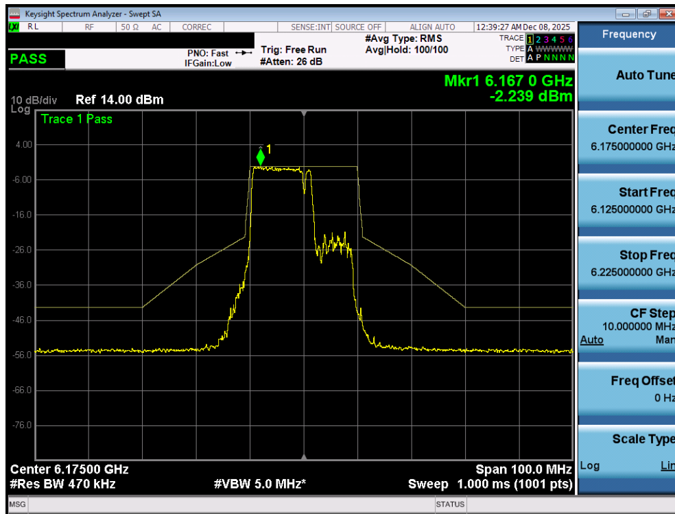
Plot 7-107. In Band Emissions Plot MIMO ANT1 (20MHz 802.11be (106+26 Tones) (UNII Band 5) – Ch. 45) - SP
