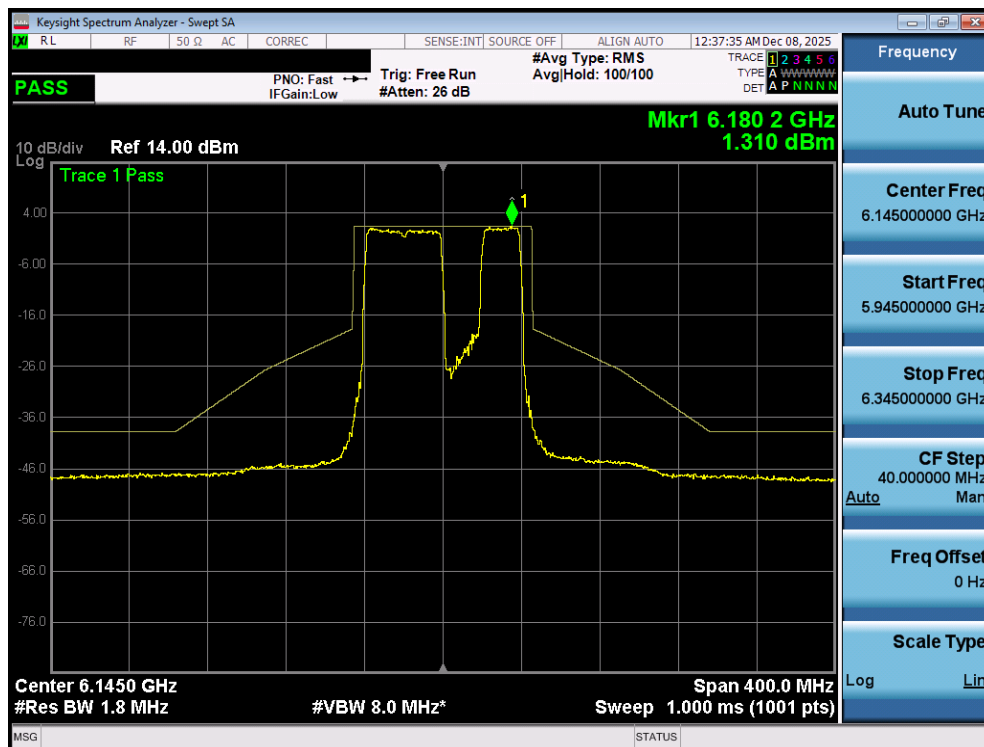
Plot 7-108. In Band Emissions Plot MIMO ANT1 (80MHz 802.11be (484+242 Tones) (UNII Band 5) – Ch. 39) SP
