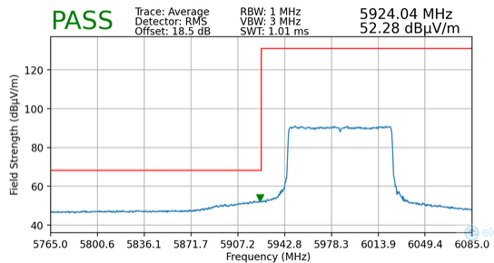
Plot 7-169. Radiated Lower Band Edge Plot MIMO (Average – UNII Band 5 – 996T)
