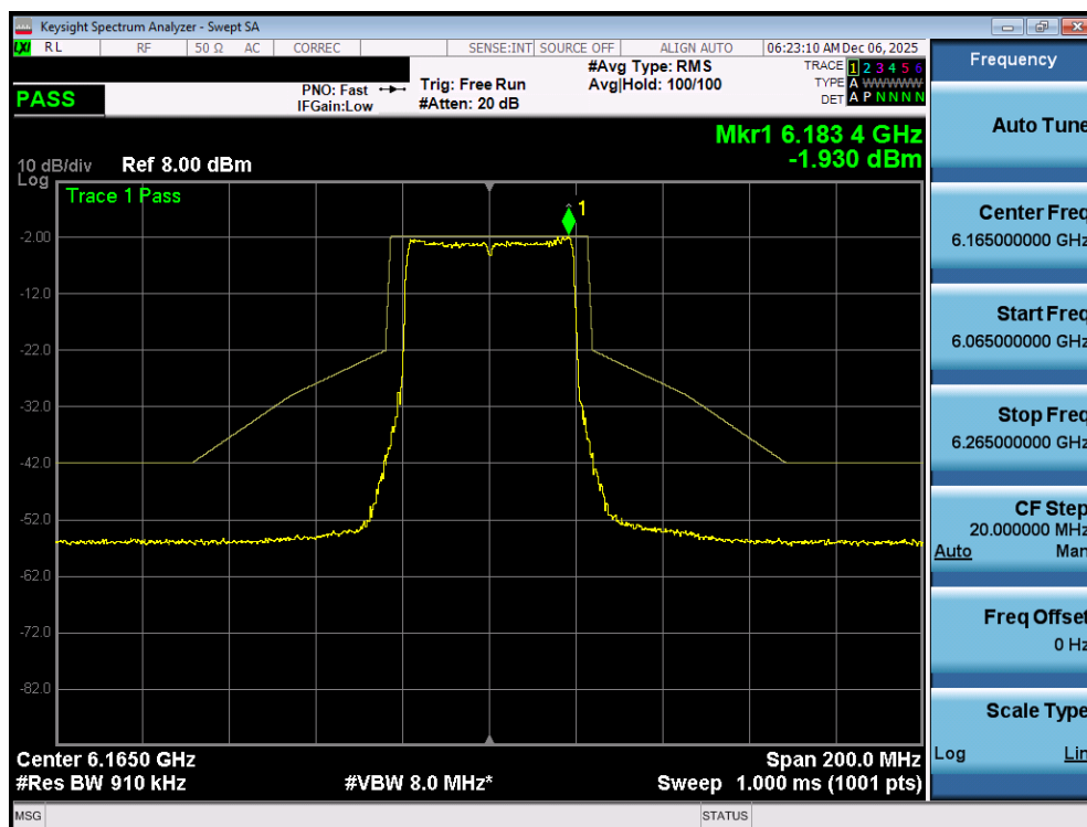
Plot 7-110. In Band Emissions Plot MIMO ANT1 (40MHz 802.11ax/be (Full Tones) (UNII Band 5) – Ch. 43) - LPI
