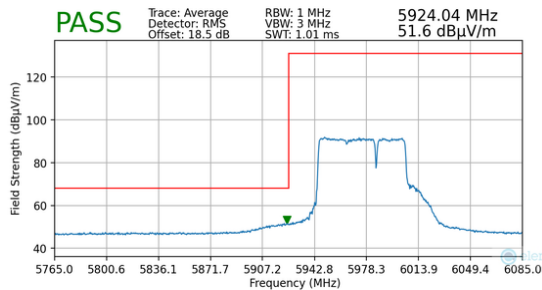
Plot 7-173. Radiated Lower Band Edge Plot MIMO (Average – UNII Band 5 – 484+242T)
