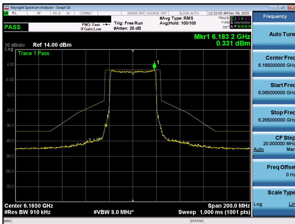
Plot 7-115. In Band Emissions Plot MIMO ANT1 (40MHz 802.11ax/be (Full Tones) (UNII Band 5) – Ch. 43) – SP
