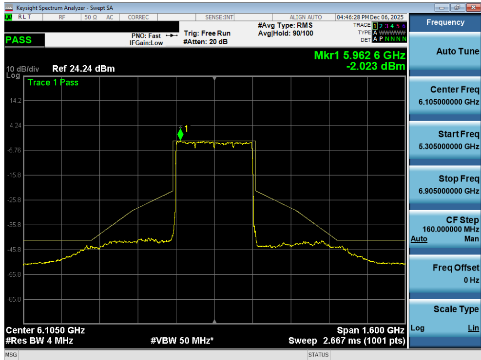
Plot 7-136. In Band Emissions Plot MIMO ANT2 (320MHz 802.11be (Full Tones) (UNII Band 5) – Ch. 31) - LPI
