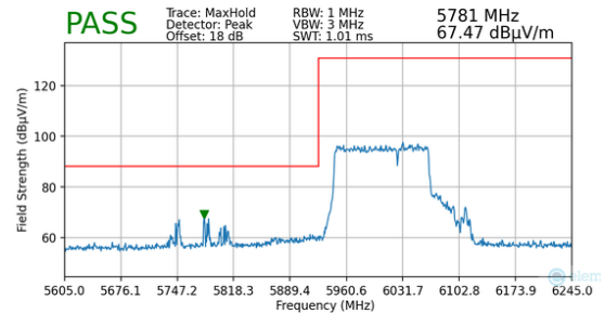
Plot 7-182. Radiated Lower Band Edge Plot MIMO (Peak – UNII Band 5 – 996+484T)
