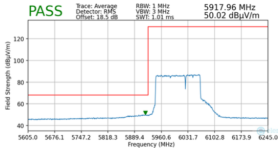
Plot 7-181. Radiated Lower Band Edge Plot MIMO (Average – UNII Band 5 – 996+484T)
