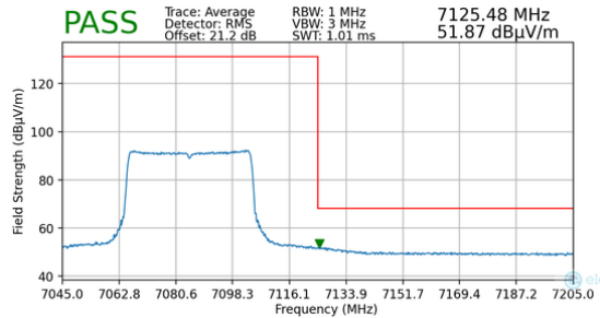
Plot 7-167. Radiated Upper Band Edge Plot MIMO (Average – UNII Band 8 – 484T)
