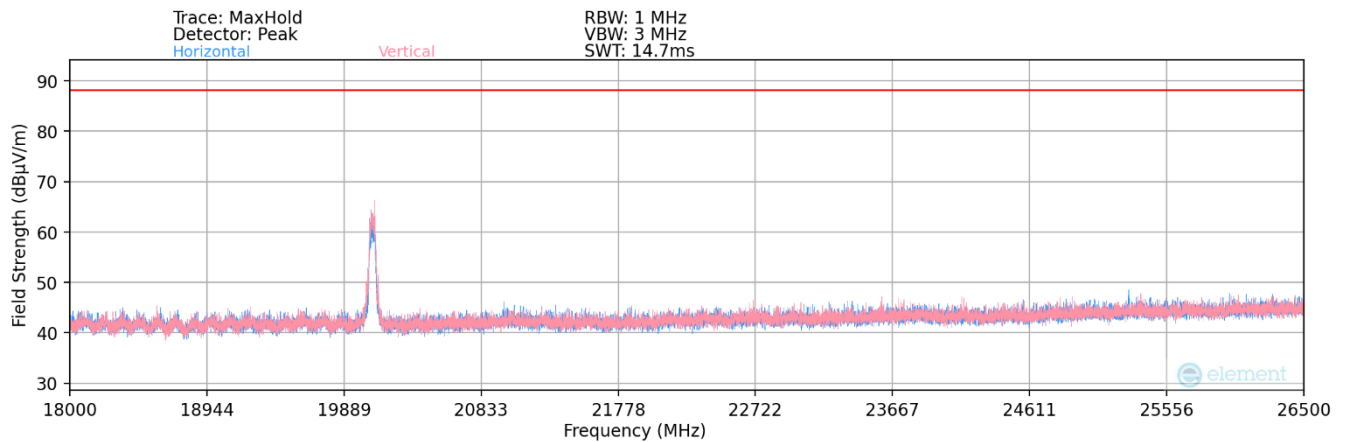
Plot 7-149. Radiated Spurious Plot 18GHz - 26.5GHz (802.11ax) – Ch.149
