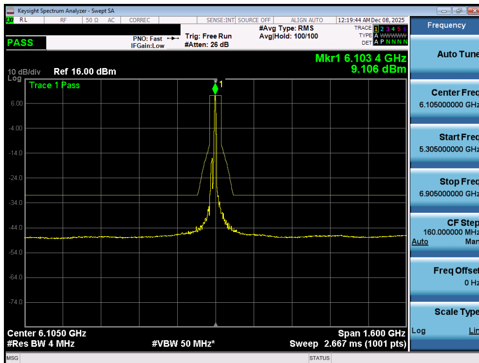
Plot 7-106. In Band Emissions Plot MIMO ANT1 (320MHz 802.11ax/be (26 Tones) (UNII Band 5) – Ch. 31) - SP
