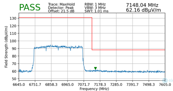
Plot 7-188. Radiated Upper Band Edge Plot MIMO (Peak – UNII Band 8 – 4*996T)
