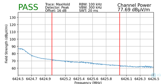
Plot 7-156. Radiated Upper Band Edge Plot MIMO (Peak – UNII Band 8 – 106T)
