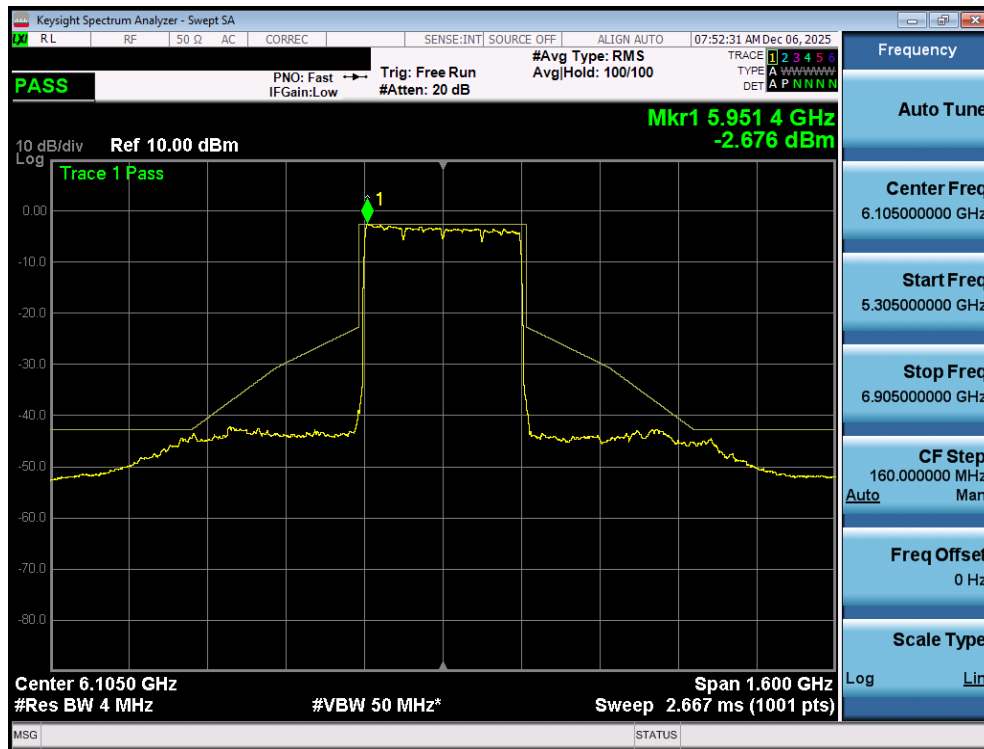
Plot 7-113. In Band Emissions Plot MIMO ANT1 (320MHz 802.11be (Full Tones) (UNII Band 5) – Ch. 31) - LPI
