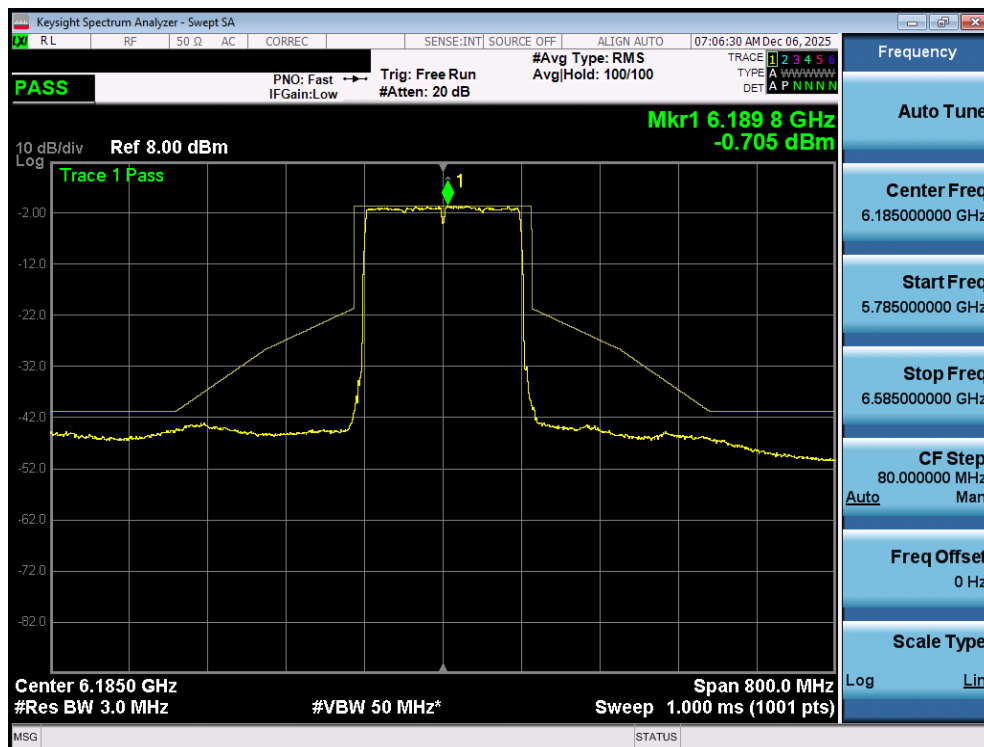
Plot 7-112. In Band Emissions Plot MIMO ANT1 (160MHz 802.11ax/be (Full Tones) (UNII Band 5) – Ch. 47) - LPI
