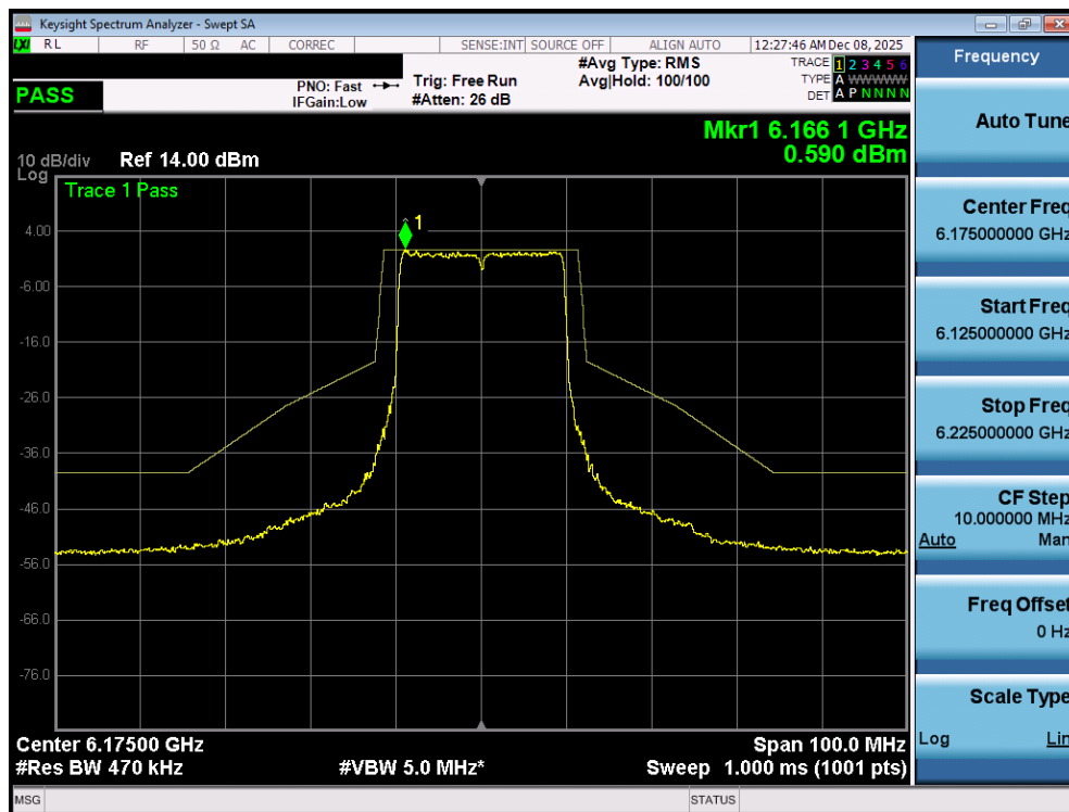
Plot 7-114. In Band Emissions Plot MIMO ANT1 (20MHz 802.11ax/be (Full Tones) (UNII Band 5) – Ch. 45) - SP
