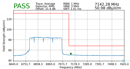
Plot 7-191. Radiated Upper Band Edge Plot MIMO (Average – UNII Band 8 – 3*996+484T)
