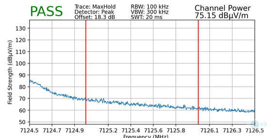
Plot 7-164. Radiated Upper Band Edge Plot MIMO (Peak – UNII Band 8 – 242T)
