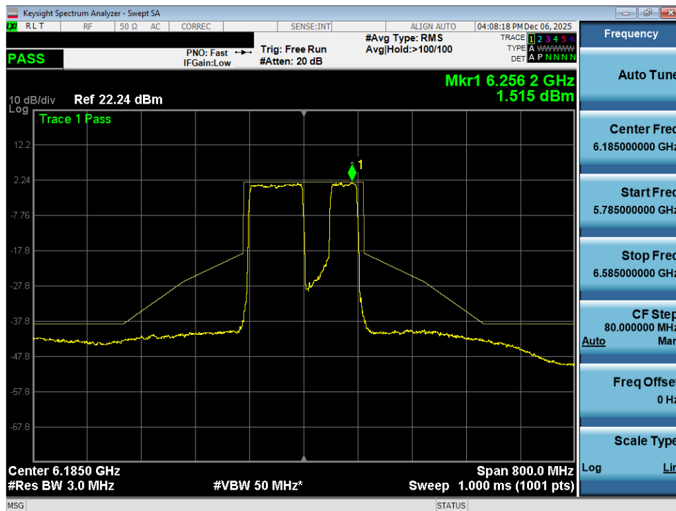
Plot 7-123. In Band Emissions Plot MIMO ANT2 (160MHz 802.11be (996+484 Tones) (UNII Band 5) – Ch. 47) LPI
