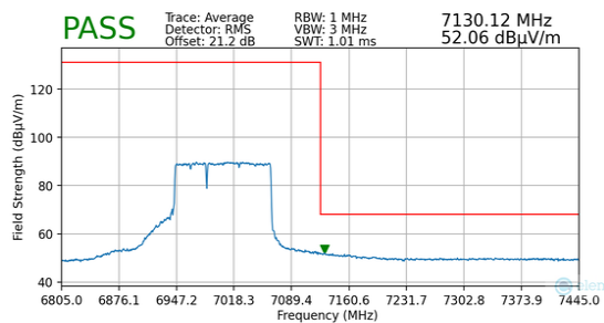
Plot 7-183. Radiated Upper Band Edge Plot MIMO (Average – UNII Band 8 – 996+484T)
