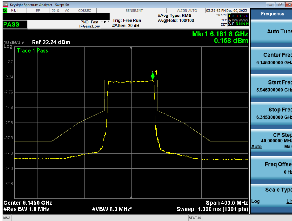
Plot 7-134. In Band Emissions Plot MIMO ANT2 (80MHz 802.11ax/be (Full Tones) (UNII Band 5) – Ch. 39) - LPI
