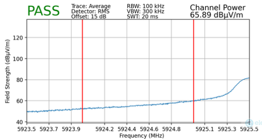
Plot 7-153. Radiated Lower Band Edge Plot MIMO (Average – UNII Band 5 – 106T)
