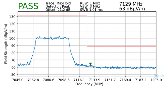
Plot 7-168. Radiated Upper Band Edge Plot MIMO (Peak – UNII Band 8 – 484T)
