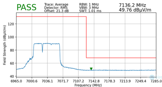
Plot 7-175. Radiated Upper Band Edge Plot MIMO (Average – UNII Band 8 – 484+242T)
