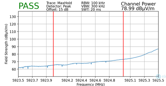
Plot 7-162. Radiated Lower Band Edge Plot MIMO (Peak – UNII Band 5 – 242T)
