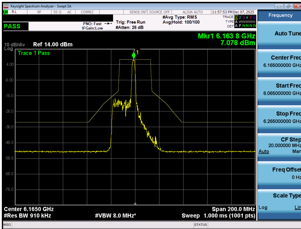
Plot 7-103. In Band Emissions Plot MIMO ANT1 (40MHz 802.11ax/be (26 Tones) (UNII Band 5) – Ch. 43) - SP
