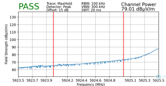
Plot 7-154. Radiated Lower Band Edge Plot MIMO (Peak – UNII Band 5 – 106T)
