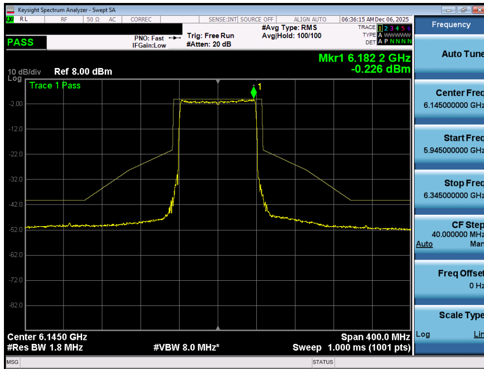
Plot 7-111. In Band Emissions Plot MIMO ANT1 (80MHz 802.11ax/be (Full Tones) (UNII Band 5) – Ch. 39) - LPI
