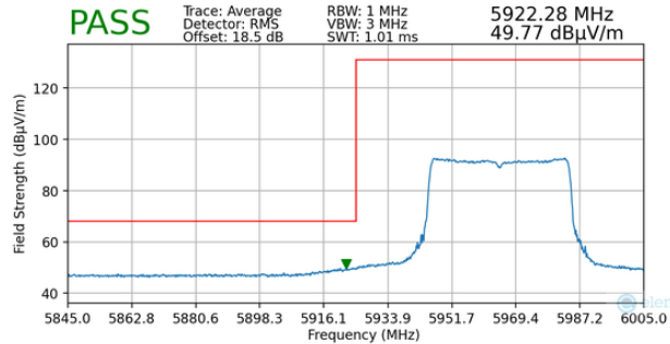
Plot 7-165. Radiated Lower Band Edge Plot MIMO (Average – UNII Band 5 – 484T)
