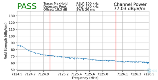
Plot 7-160. Radiated Upper Band Edge Plot MIMO (Peak – UNII Band 8 – 106+26T)
