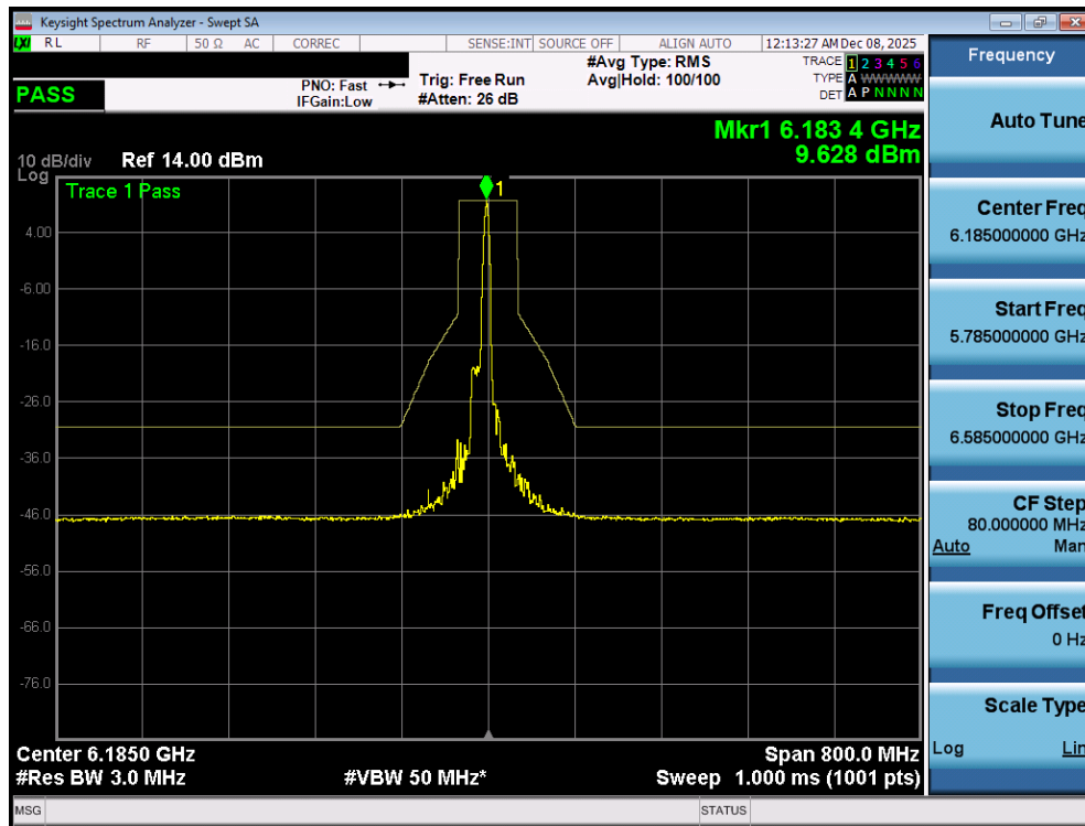
Plot 7-105. In Band Emissions Plot MIMO ANT1 (160MHz 802.11ax/be (26 Tones) (UNII Band 5) – Ch. 47) - SP
