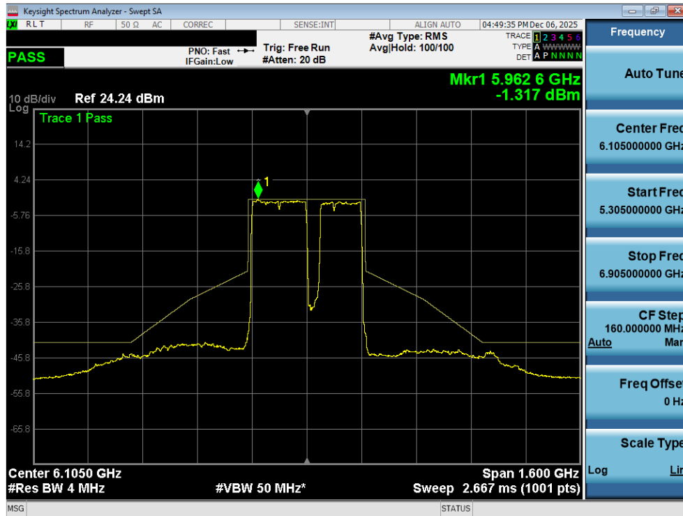
Plot 7-124. In Band Emissions Plot MIMO ANT2 (320MHz 802.11be (3*996+484 Tones) (UNII Band 5) – Ch. 31) LPI
