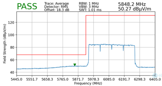
Plot 7-185. Radiated Lower Band Edge Plot MIMO (Average – UNII Band 5 – 4*996T)
