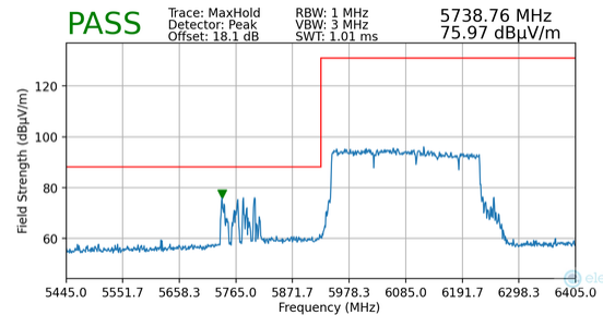
Plot 7-190. Radiated Lower Band Edge Plot MIMO (Peak – UNII Band 5 – 3*996+484T)
