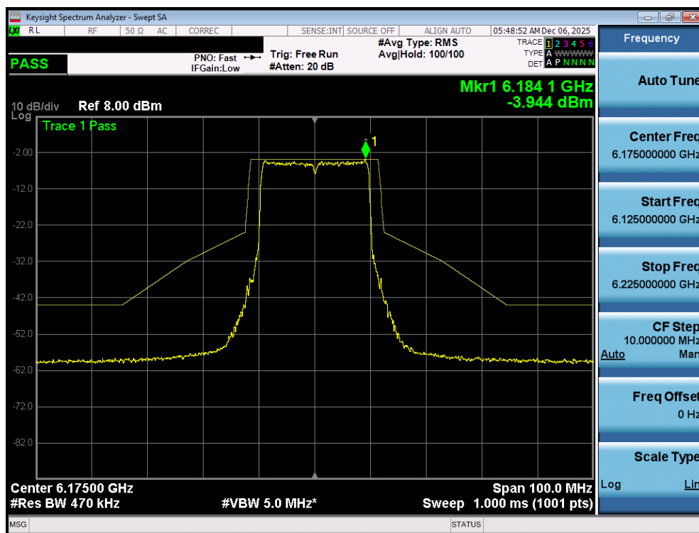
Plot 7-109. In Band Emissions Plot MIMO ANT1 (20MHz 802.11ax/be (Full Tones) (UNII Band 5) – Ch. 45) - LPI
