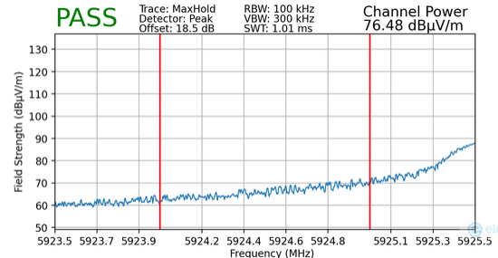
Plot 7-158. Radiated Lower Band Edge Plot MIMO (Peak – UNII Band 5 – 106+26T)
