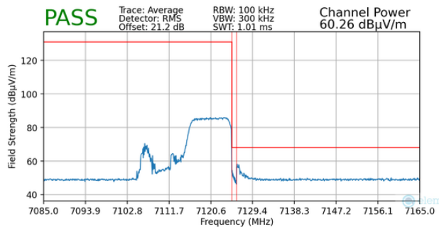
Plot 7-159. Radiated Upper Band Edge Plot MIMO (Average – UNII Band 8 – 106+26T)
