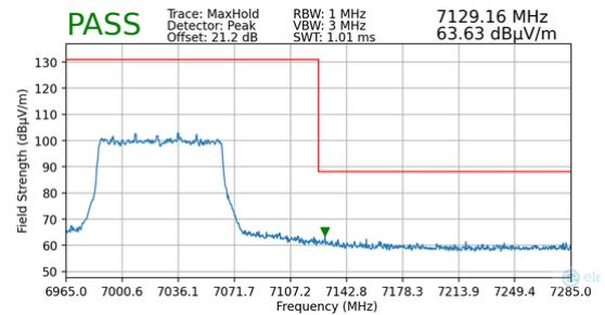
Plot 7-172. Radiated Upper Band Edge Plot MIMO (Peak – UNII Band 8 – 996T)
