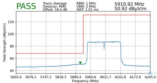
Plot 7-177. Radiated Lower Band Edge Plot MIMO (Average – UNII Band 5 – 2x996T)
