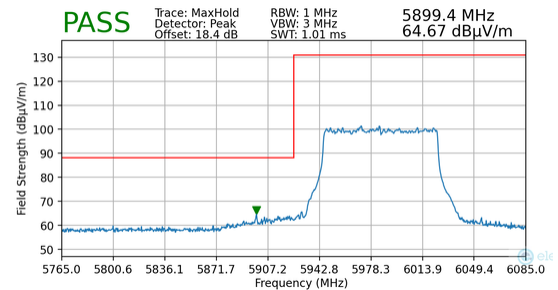
Plot 7-170. Radiated Lower Band Edge Plot MIMO (Peak – UNII Band 5 – 996T)
