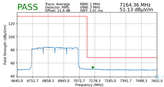
Plot 7-187. Radiated Upper Band Edge Plot MIMO (Average – UNII Band 8 – 4*996T)
