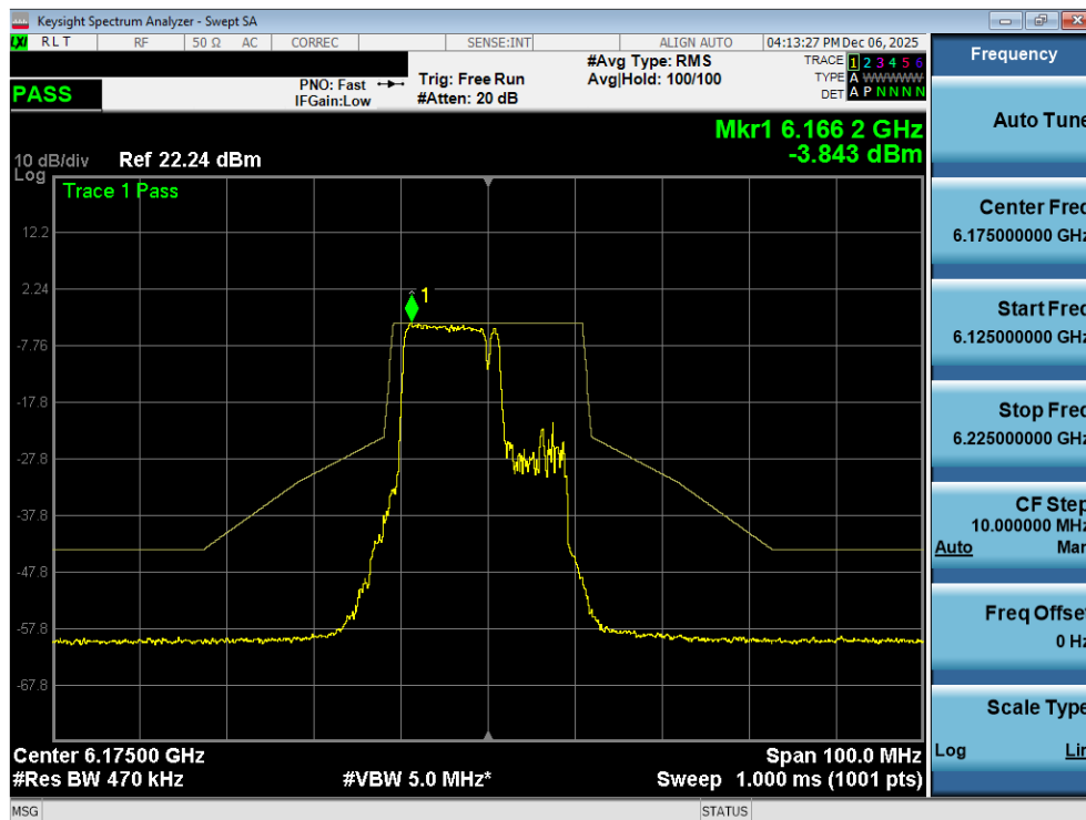
Plot 7-121. In Band Emissions Plot MIMO ANT2 (20MHz 802.11be (106+26 Tones) (UNII Band 5) – Ch. 45) - LPI
