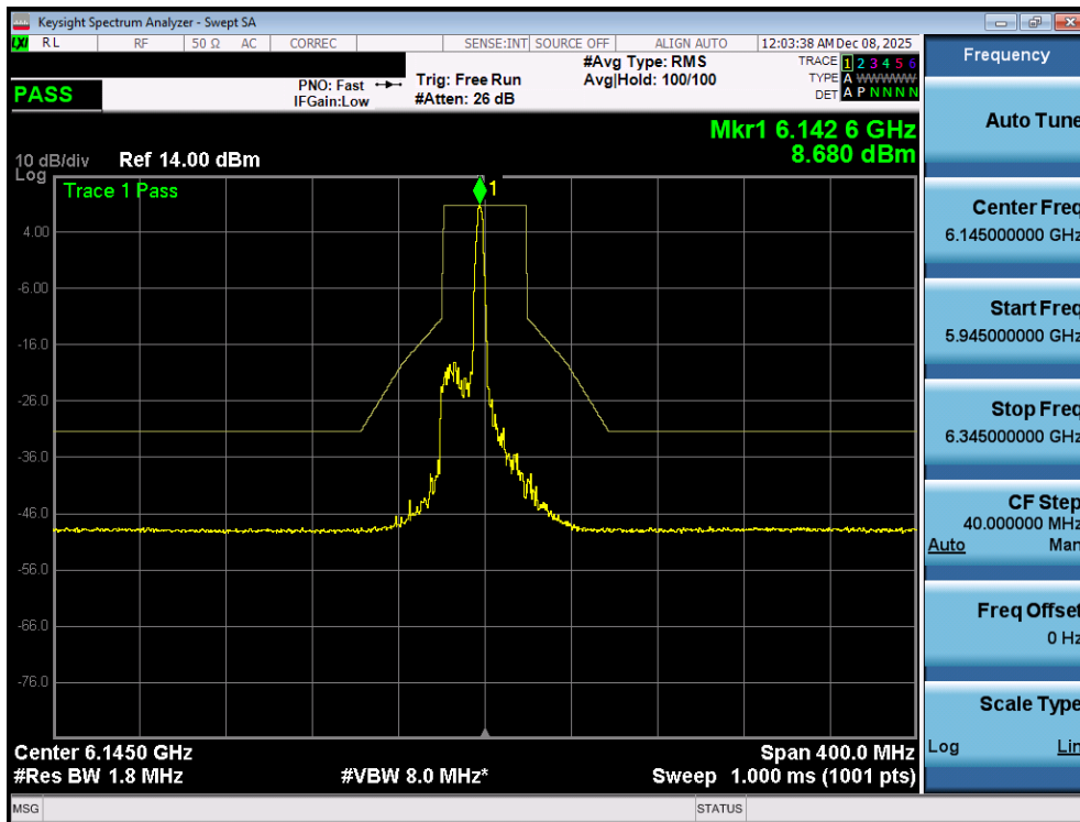
Plot 7-104. In Band Emissions Plot MIMO ANT1 (80MHz 802.11ax/be (26 Tones) (UNII Band 5) – Ch. 39) - SP
