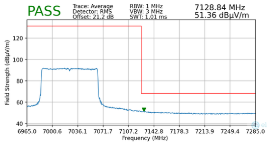
Plot 7-171. Radiated Upper Band Edge Plot MIMO (Average – UNII Band 8 – 996T)
