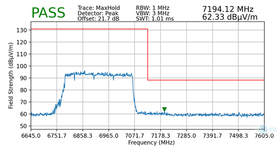
Plot 7-192. Radiated Upper Band Edge Plot MIMO (Peak – UNII Band 8 – 3*996+484T)
