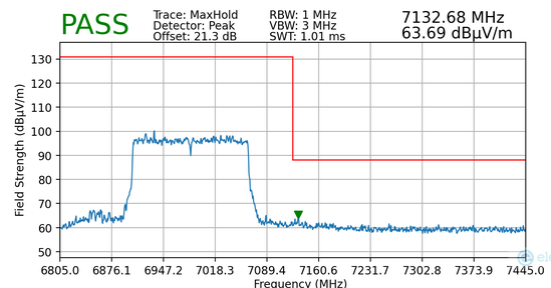
Plot 7-180. Radiated Upper Band Edge Plot MIMO (Peak – UNII Band 8 – 2x996T)
