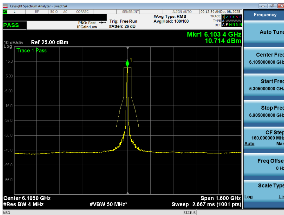
Plot 7-129. In Band Emissions Plot MIMO ANT2 (320MHz 802.11ax/be (26 Tones) (UNII Band 5) – Ch. 31) - SP
