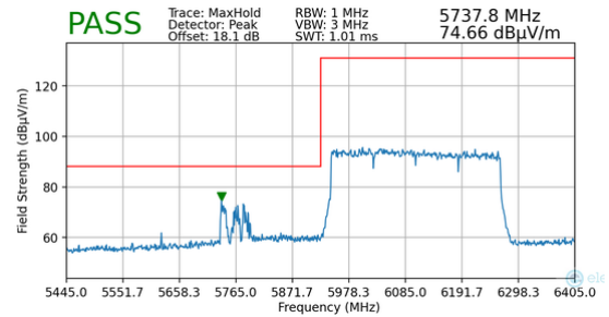
Plot 7-186. Radiated Lower Band Edge Plot MIMO (Peak – UNII Band 5 – 4*996T)
