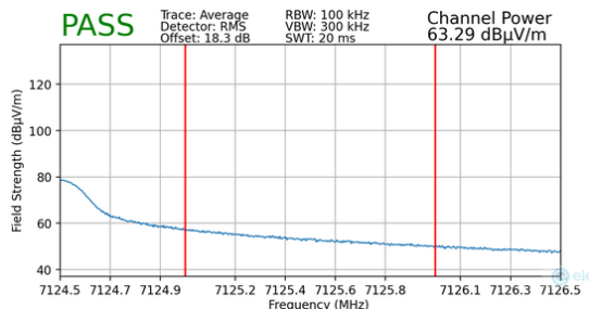
Plot 7-163. Radiated Upper Band Edge Plot MIMO (Average – UNII Band 8 – 242T)
