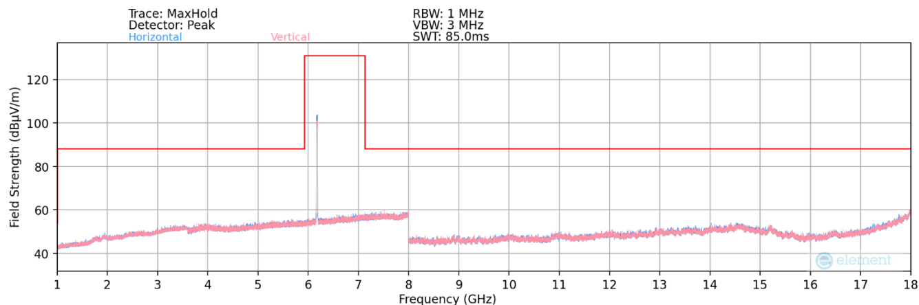
Plot 7-151. Radiated Spurious Plot 1GHz – 18GHz MIMO (802.11be – UNII Band 5 Ch. 45) – 52+26 Tones
