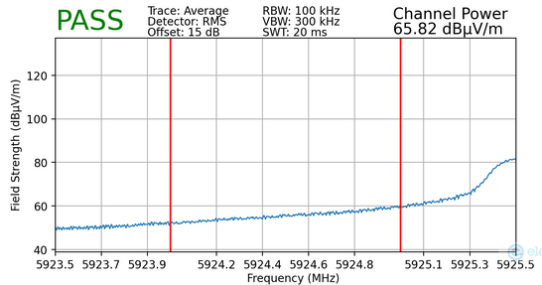
Plot 7-161. Radiated Lower Band Edge Plot MIMO (Average – UNII Band 5 – 242T)
