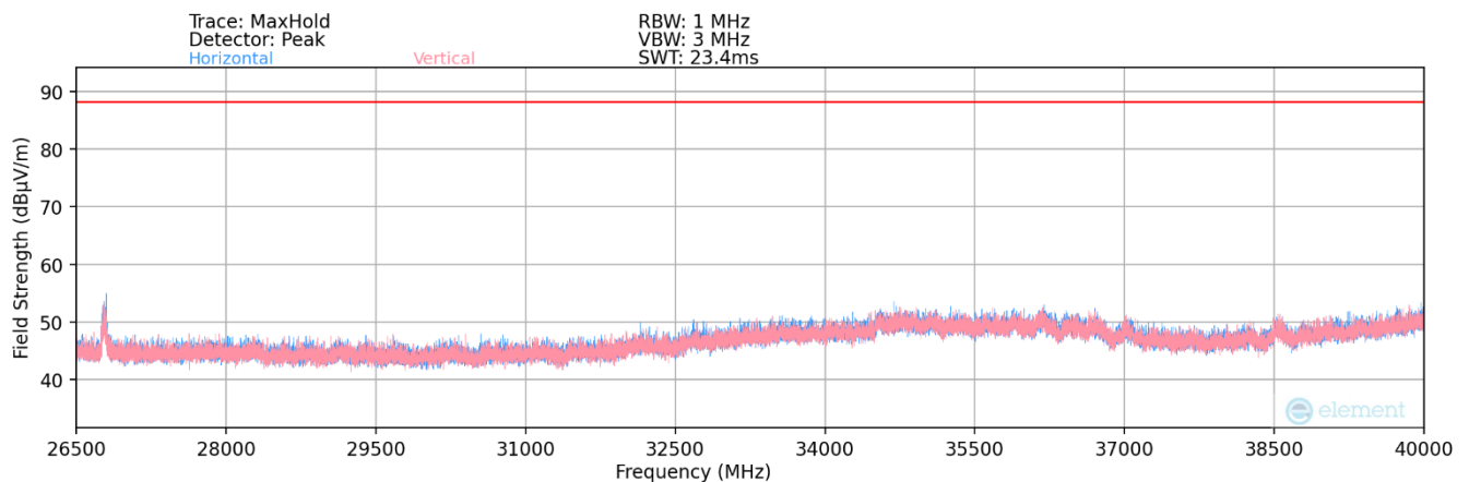
Plot 7-150. Radiated Spurious Plot 26.5GHz - 40GHz (802.11ax) – Ch.149
