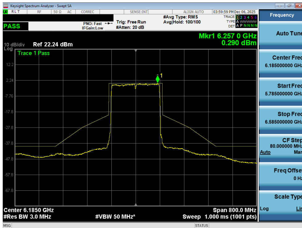
Plot 7-135. In Band Emissions Plot MIMO ANT2 (160MHz 802.11ax/be (Full Tones) (UNII Band 5) – Ch. 47) - LPI
