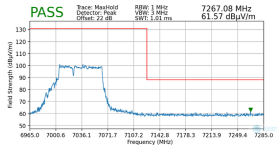
Plot 7-176. Radiated Upper Band Edge Plot MIMO (Peak – UNII Band 8 – 484+242T)
