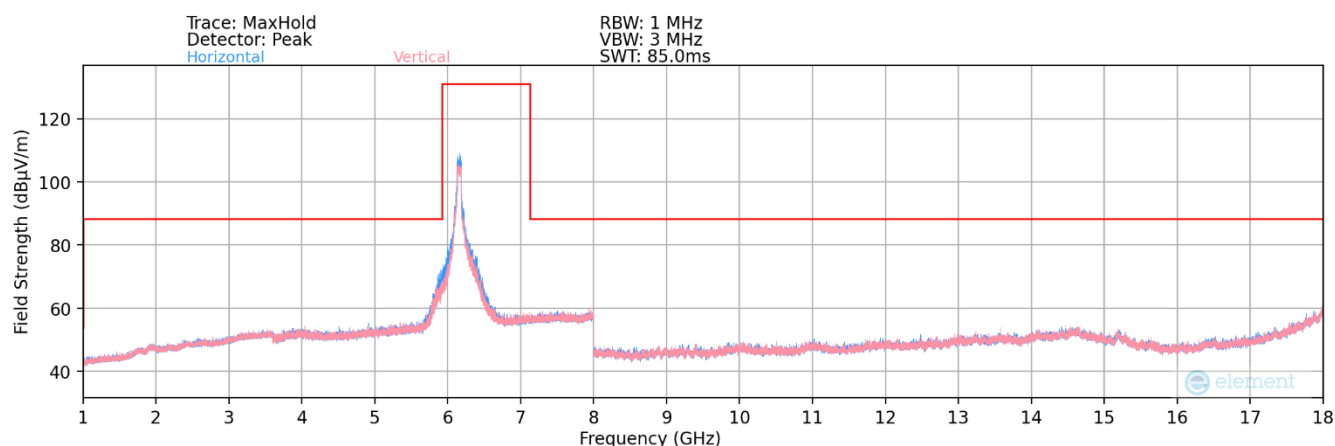
Plot 7-152. Radiated Spurious Plot 1GHz – 18GHz MIMO (802.11be – UNII Band 5 Ch. 39) – 484+242 Tones
