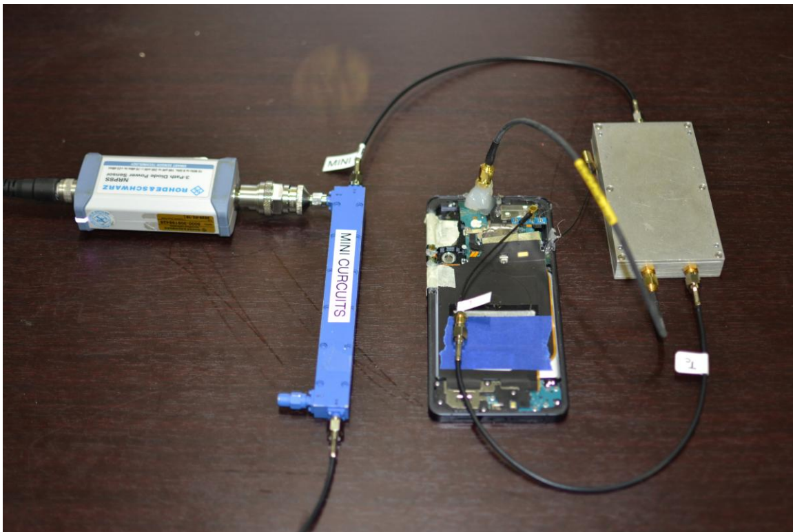
Test Setup Photo 4 – Conducted Test Setup (Figure 5.2-1b)
