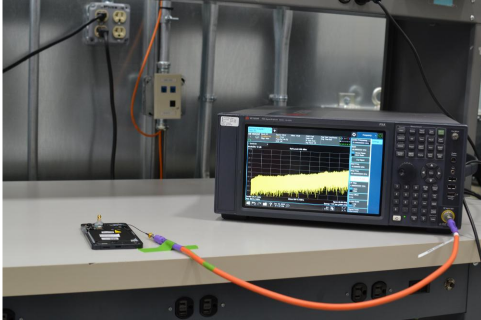
Figure 13. Conducted Test Setup
