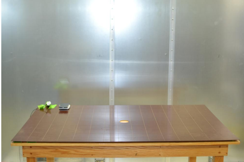
Figure 11. Test Setup – ACLC– <30MHz – with WCP
