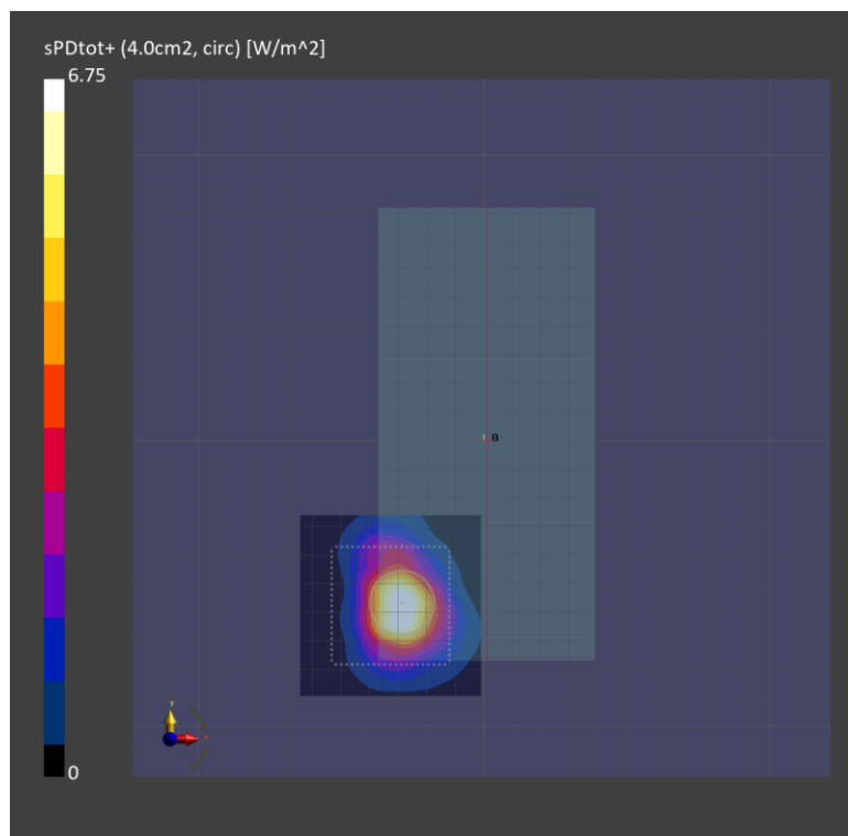
Figure D-3 4cm 2 -averaged power density distribution measured at input.power.limit of 9.9 dBm on the Right Surface n261 beam ID 5.
