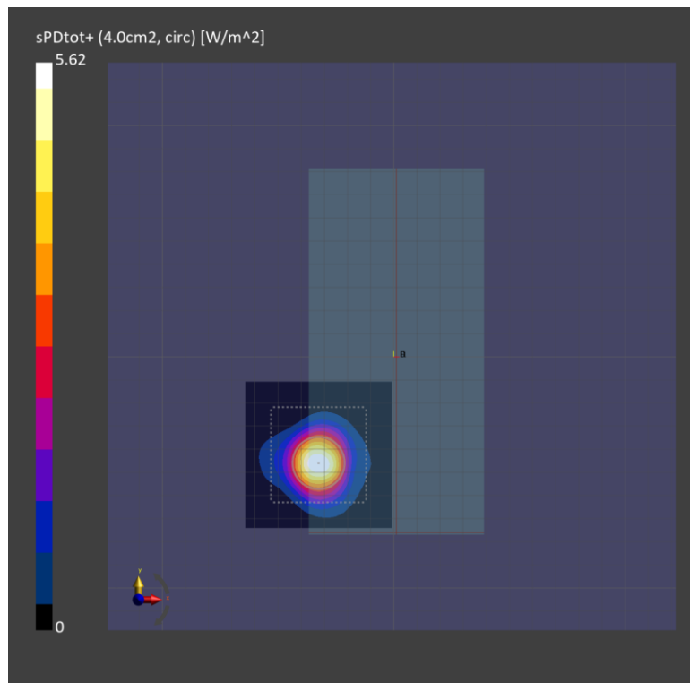
Figure D-2 4cm 2 -averaged power density distribution measured at input.power.limit of 3.6 dBm on the Rear Surface n261 beam ID 19.
