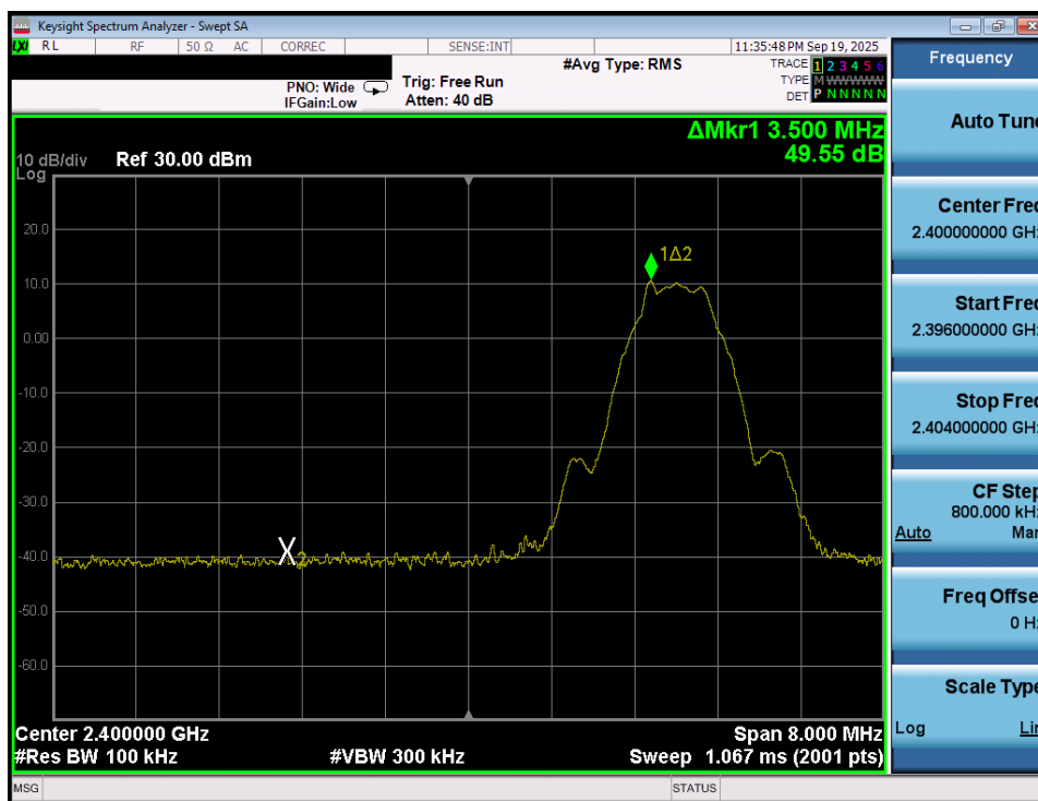
Plot 7-111. Band Edge Plot (Bluetooth (LE), 500kbps – Ch. 37) – Ant 1
