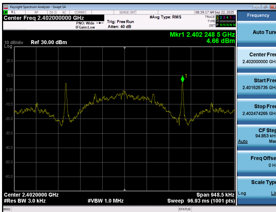
Plot 7-85. Power Spectral Density Plot (Bluetooth (LE), 125kbps – Ch. 37) – Ant 2
