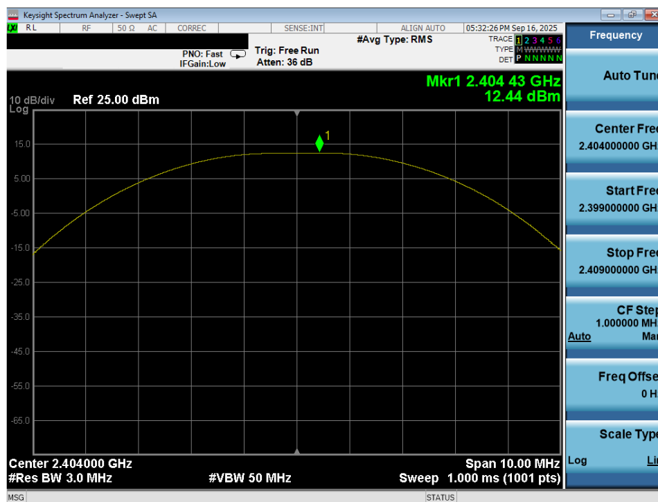
Plot 7-70. Peak Power Plot (Bluetooth (LE), 2Mbps – Ch. 0) – Dual Ant 2
