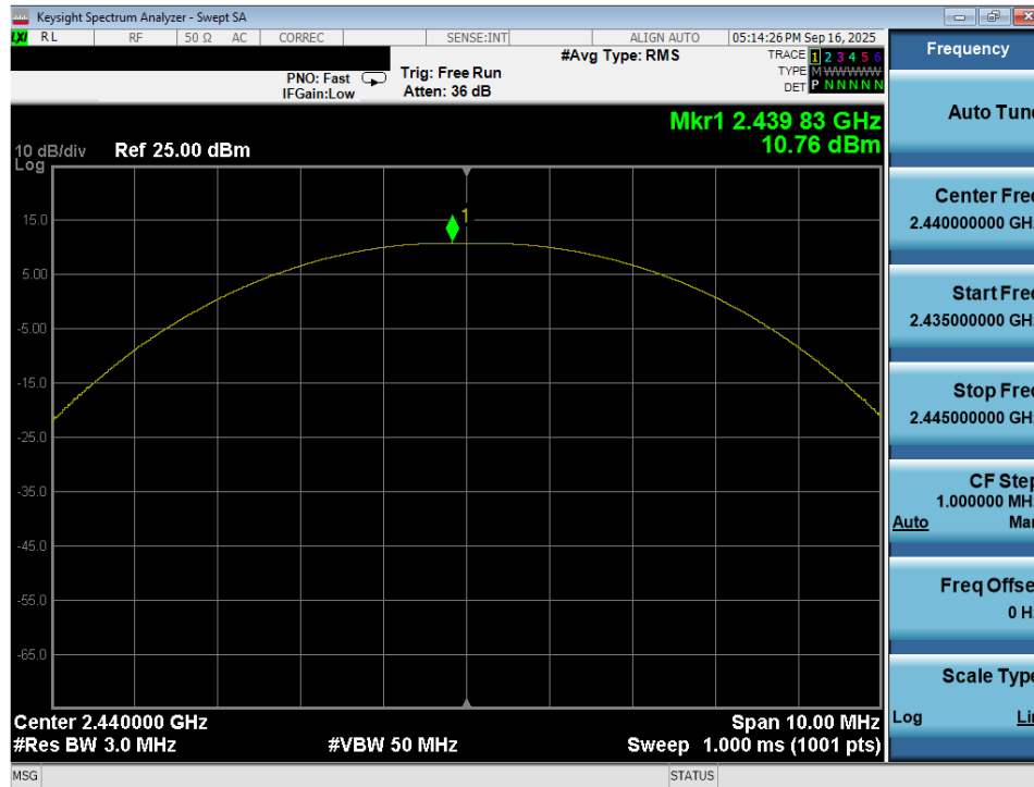
Plot 7-41. Peak Power Plot (Bluetooth (LE), 500kbps – Ch. 17) – Ant 1
