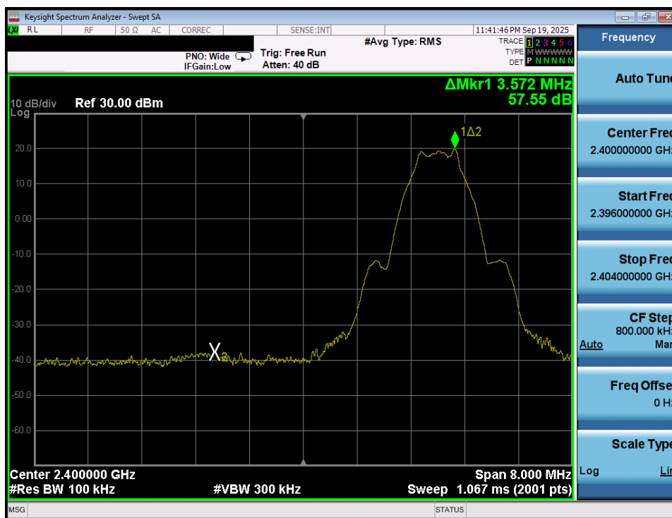
Plot 7-113. Band Edge Plot (Bluetooth (LE), 1Mbps - Ch. 37) - Ant 1
