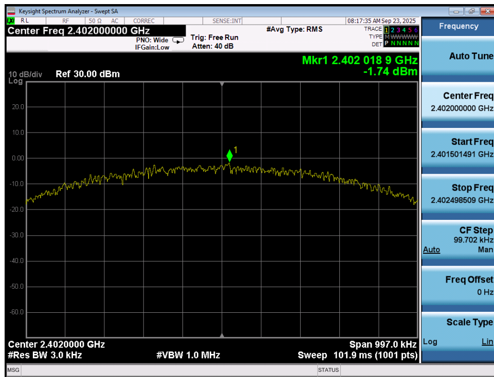
Plot 7-97. Power Spectral Density Plot (Bluetooth (LE), 1Mbps – Ch. 37) – Dual Ant 1
