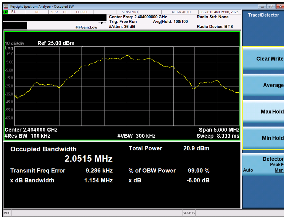
Plot 7-28. 6dB Bandwidth Plot (Bluetooth (LE), 2Mbps – Ch. 0) – Dual Ant 1
