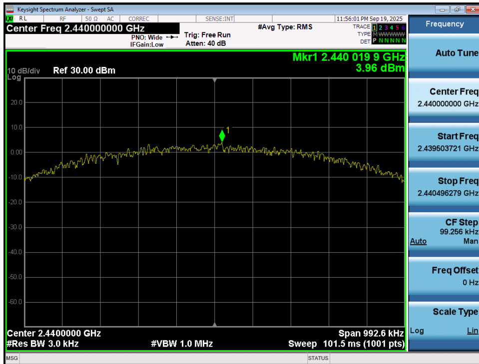
Plot 7-80. Power Spectral Density Plot (Bluetooth (LE), 1Mbps – Ch. 17) – Ant 1
