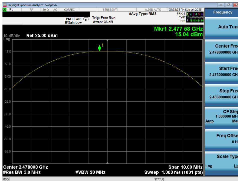
Plot 7-66. Peak Power Plot (Bluetooth (LE), 2Mbps – Ch. 36) – Dual Ant 1
