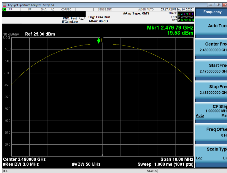
Plot 7-45. Peak Power Plot (Bluetooth (LE), 1Mbps – Ch. 39) – Ant 1
