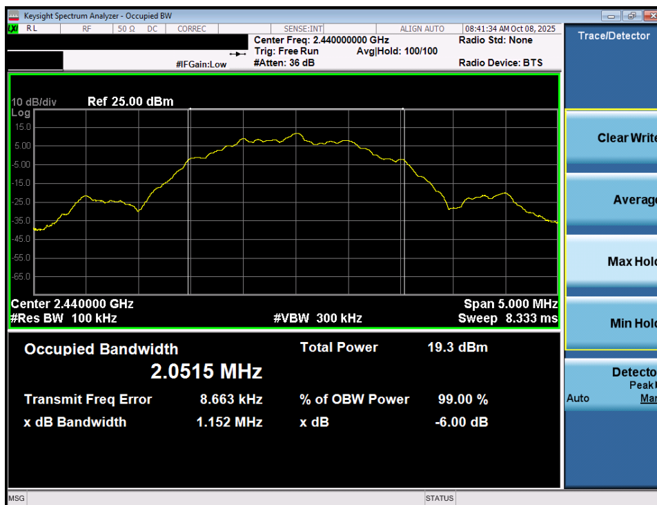
Plot 7-35. 6dB Bandwidth Plot (Bluetooth (LE), 2Mbps – Ch. 17) – Dual Ant 2
