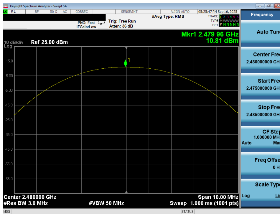
Plot 7-51. Peak Power Plot (Bluetooth (LE), 125kbps – Ch. 39) – Ant 2
