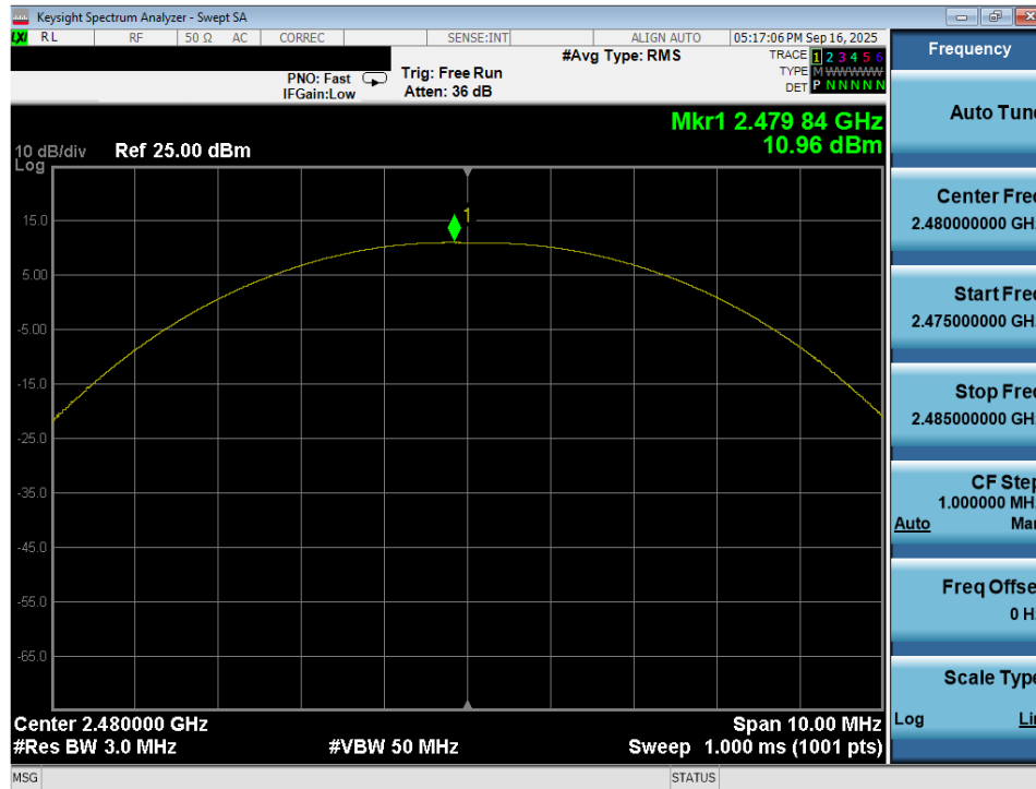
Plot 7-39. Peak Power Plot (Bluetooth (LE), 125kbps – Ch. 39) – Ant 1
