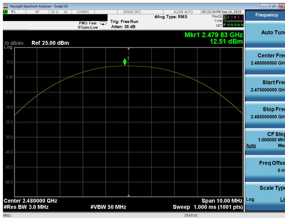
Plot 7-69. Peak Power Plot (Bluetooth (LE), 1Mbps – Ch. 39) – Dual Ant 2
