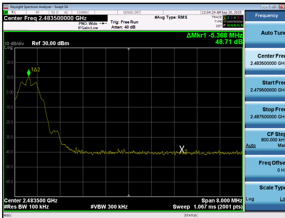
Plot 7-110. Band Edge Plot (Bluetooth (LE), 125kbps – Ch. 39) – Ant 1
