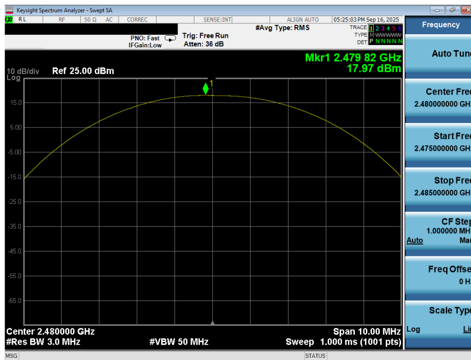
Plot 7-57. Peak Power Plot (Bluetooth (LE), 1Mbps – Ch. 39) – Ant 2
