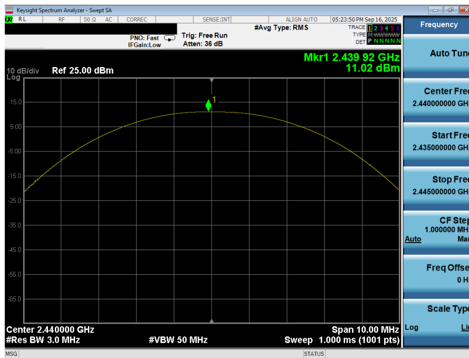
Plot 7-53. Peak Power Plot (Bluetooth (LE), 500kbps – Ch. 17) – Ant 2
