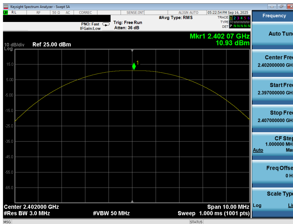
Plot 7-52. Peak Power Plot (Bluetooth (LE), 500kbps – Ch. 37) – Ant 2
