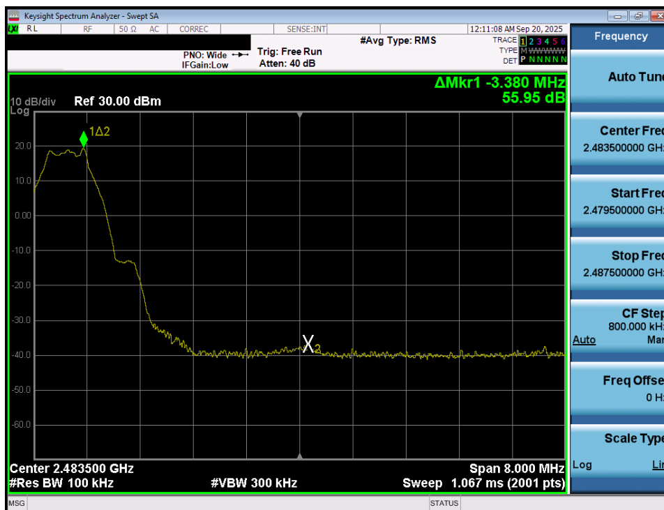
Plot 7-114. Band Edge Plot (Bluetooth (LE), 1Mbps - Ch. 39) - Ant 1
