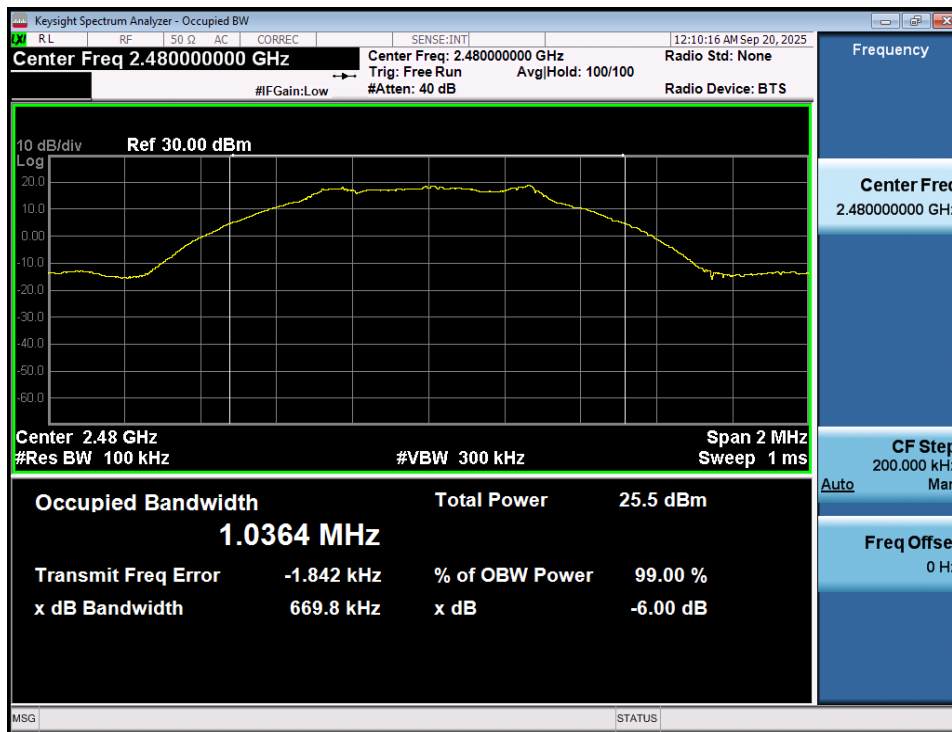
Plot 7-9. 6dB Bandwidth Plot (Bluetooth (LE), 1Mbps – Ch. 39) – Ant 1
