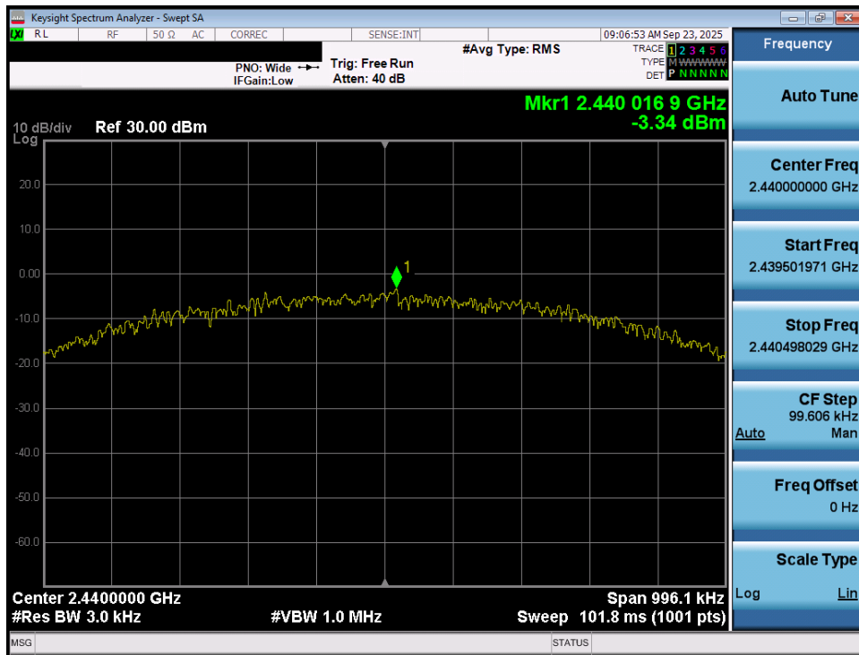
Plot 7-104. Power Spectral Density Plot (Bluetooth (LE), 1Mbps – Ch. 17) – Dual Ant 2
