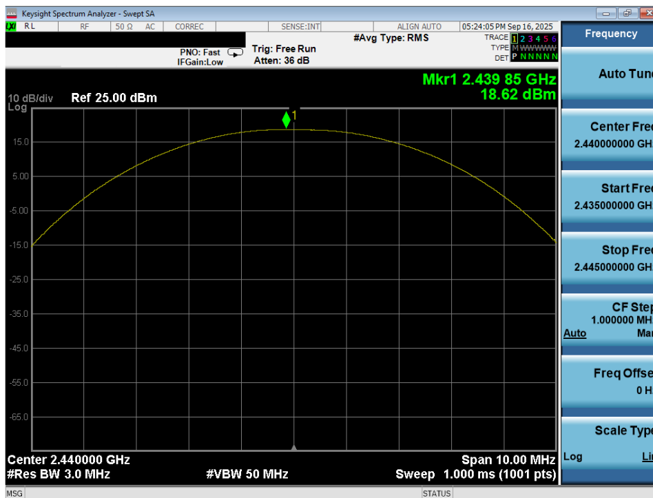
Plot 7-56. Peak Power Plot (Bluetooth (LE), 1Mbps – Ch. 17) – Ant 2
