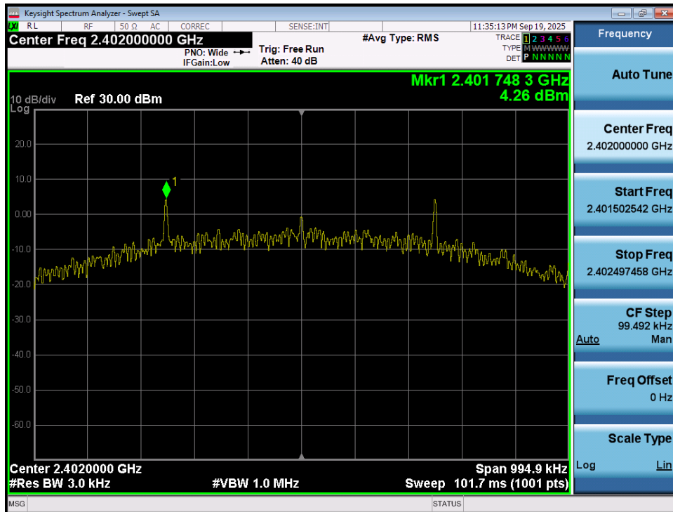
Plot 7-76. Power Spectral Density Plot (Bluetooth (LE), 500kbps – Ch. 37) – Ant 1
