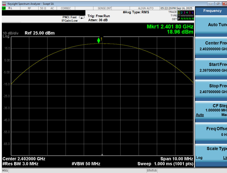
Plot 7-55. Peak Power Plot (Bluetooth (LE), 1Mbps – Ch. 37) – Ant 2
