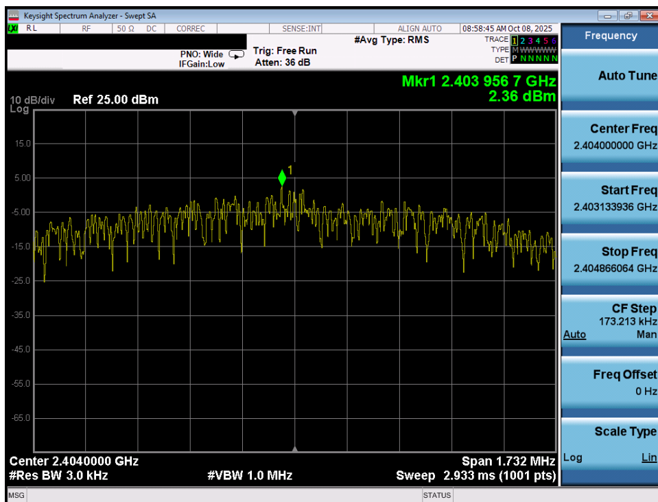
Plot 7-82. Power Spectral Density Plot (Bluetooth (LE), 2Mbps – Ch. 0) – Ant 1
