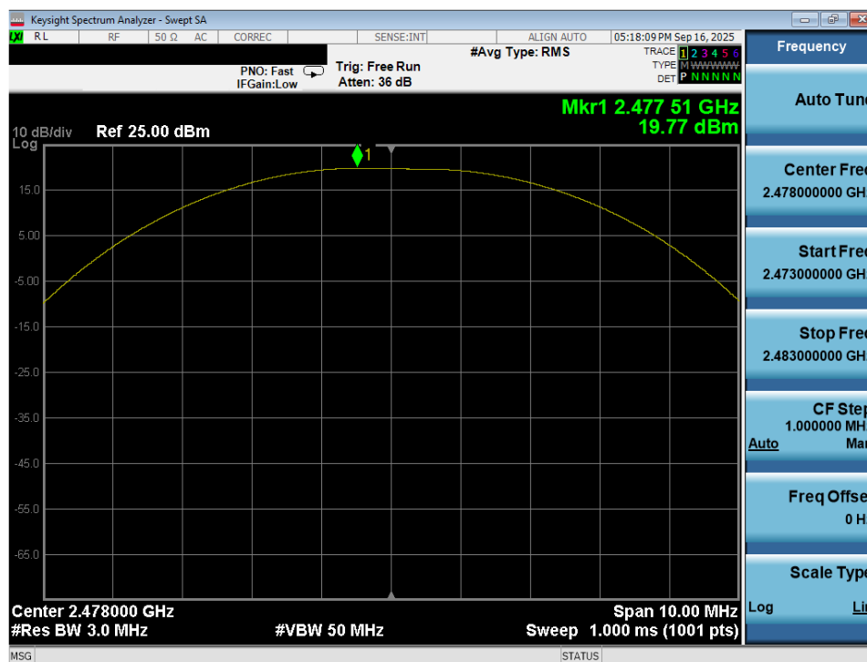
Plot 7-48. Peak Power Plot (Bluetooth (LE), 2Mbps – Ch. 36) – Ant 1
