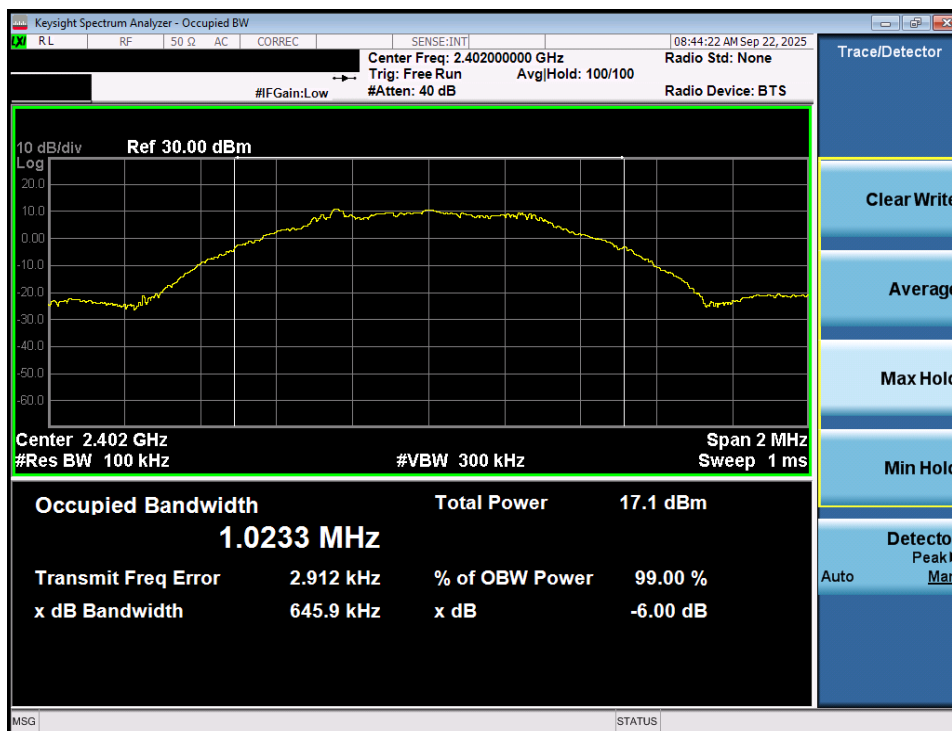
Plot 7-16. 6dB Bandwidth Plot (Bluetooth (LE), 500kbps – Ch. 37) – Ant 2
