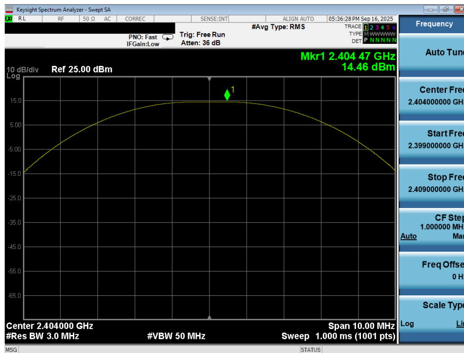
Plot 7-64. Peak Power Plot (Bluetooth (LE), 2Mbps – Ch. 0) – Dual Ant 1
