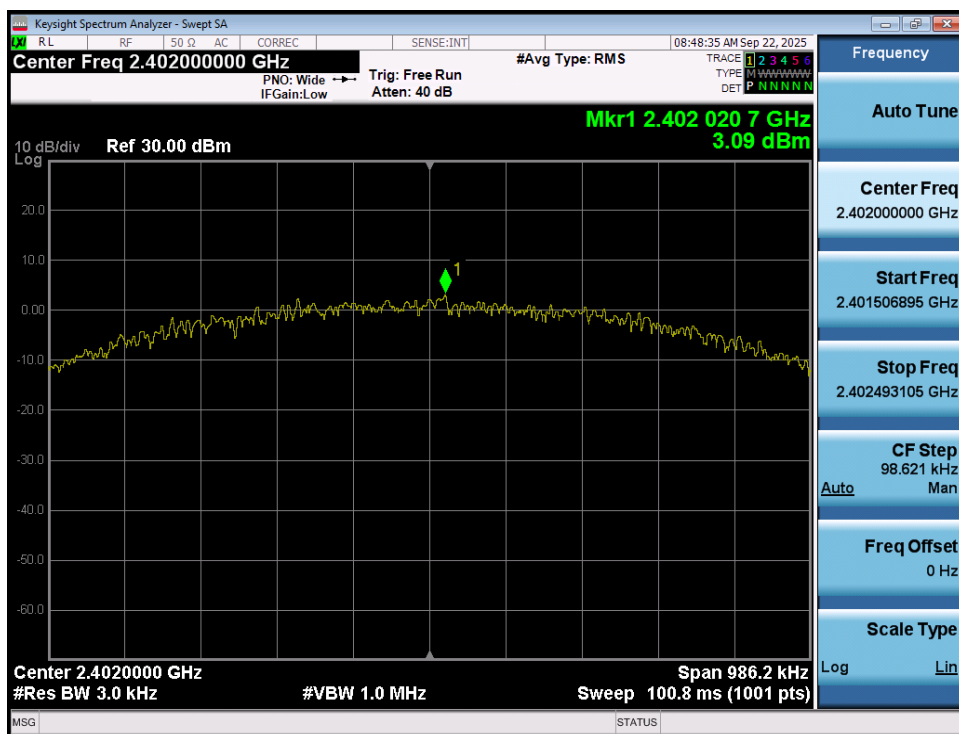
Plot 7-91. Power Spectral Density Plot (Bluetooth (LE), 1Mbps – Ch. 37) – Ant 2
