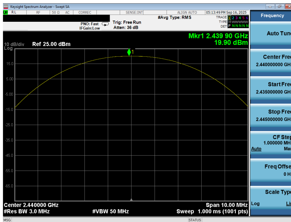
Plot 7-44. Peak Power Plot (Bluetooth (LE), 1Mbps – Ch. 17) – Ant 1
