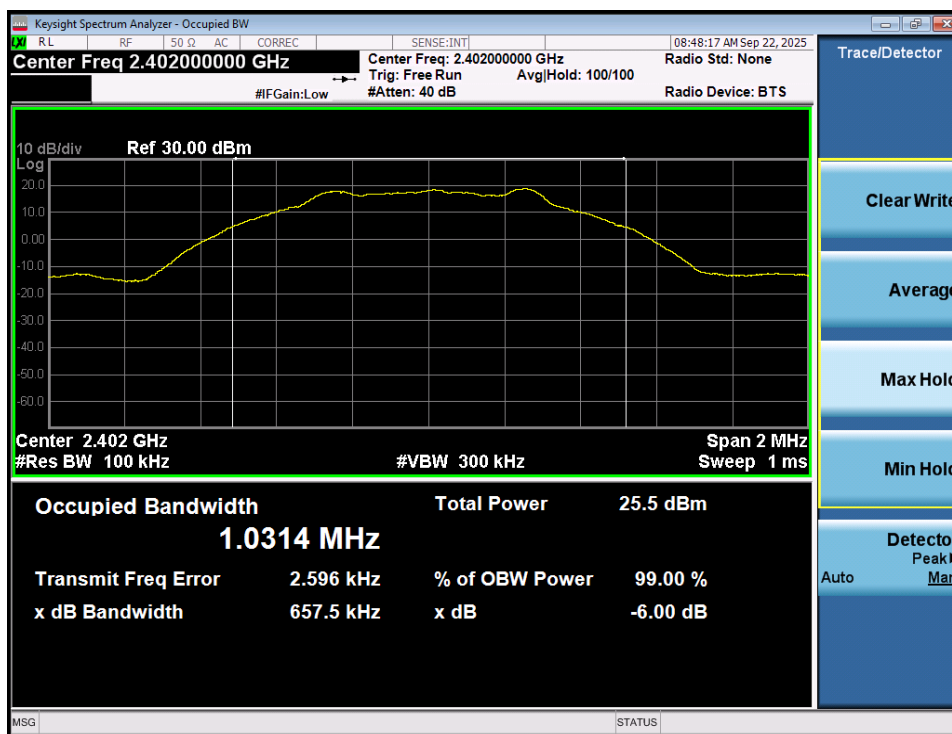
Plot 7-19. 6dB Bandwidth Plot (Bluetooth (LE), 1Mbps – Ch. 37) – Ant 2
