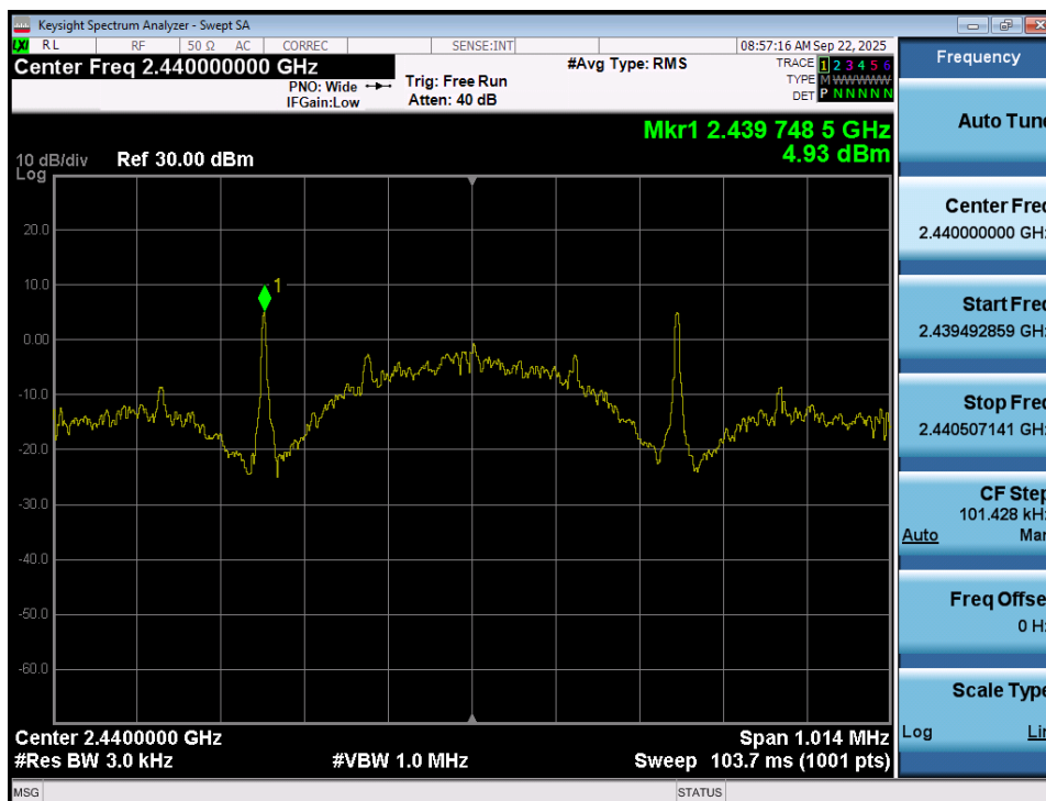
Plot 7-86. Power Spectral Density Plot (Bluetooth (LE), 125kbps – Ch. 17) – Ant 2
