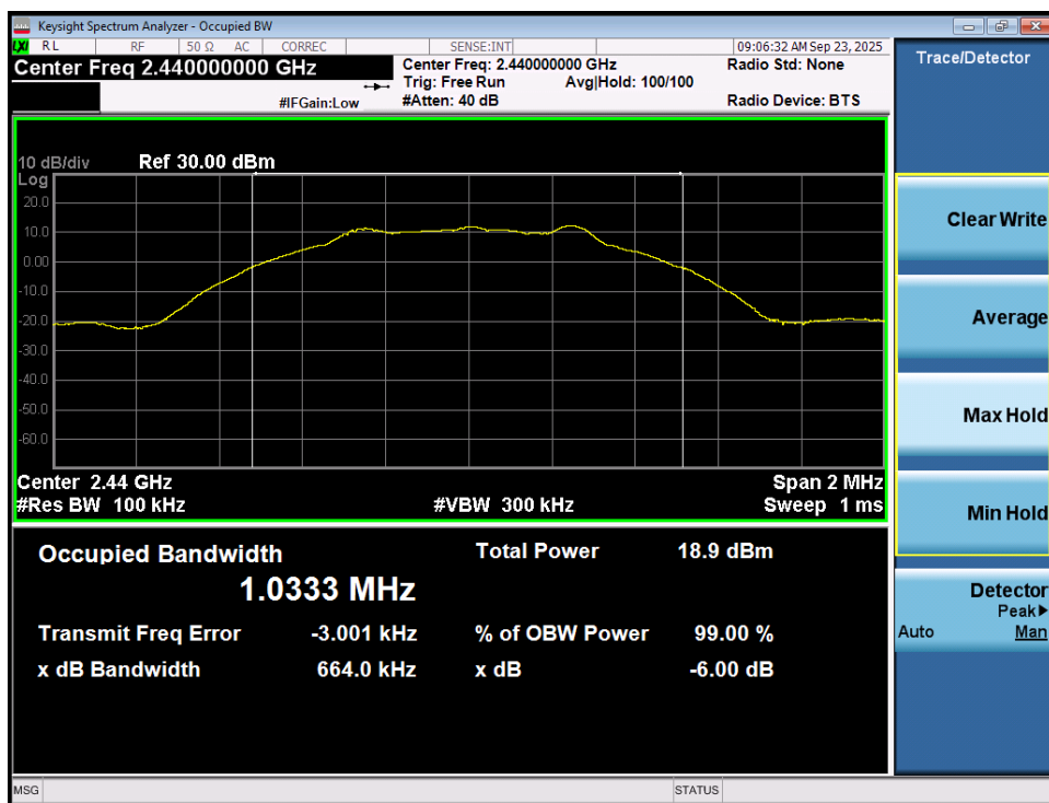
Plot 7-32. 6dB Bandwidth Plot (Bluetooth (LE), 1Mbps – Ch. 17) – Dual Ant 2
