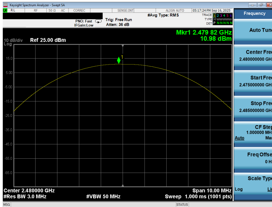
Plot 7-42. Peak Power Plot (Bluetooth (LE), 500kbps – Ch. 39) – Ant 1
