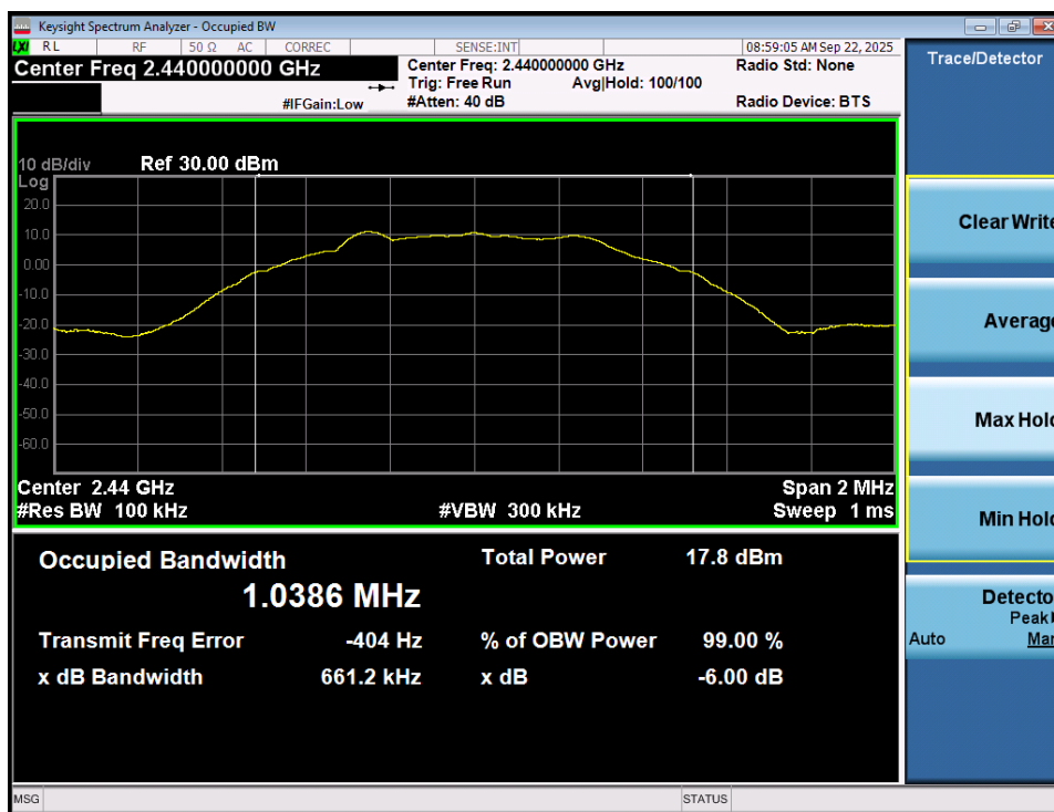
Plot 7-17. 6dB Bandwidth Plot (Bluetooth (LE), 500kbps – Ch. 17) – Ant 2
