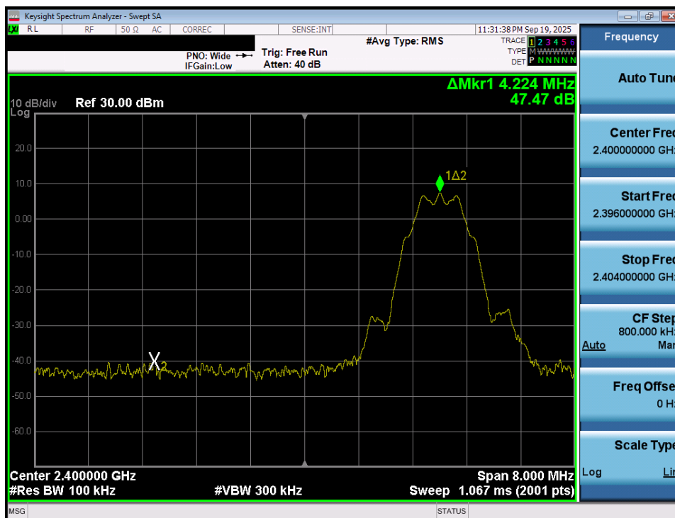
Plot 7-109. Band Edge Plot (Bluetooth (LE), 125kbps – Ch. 37) – Ant 1
