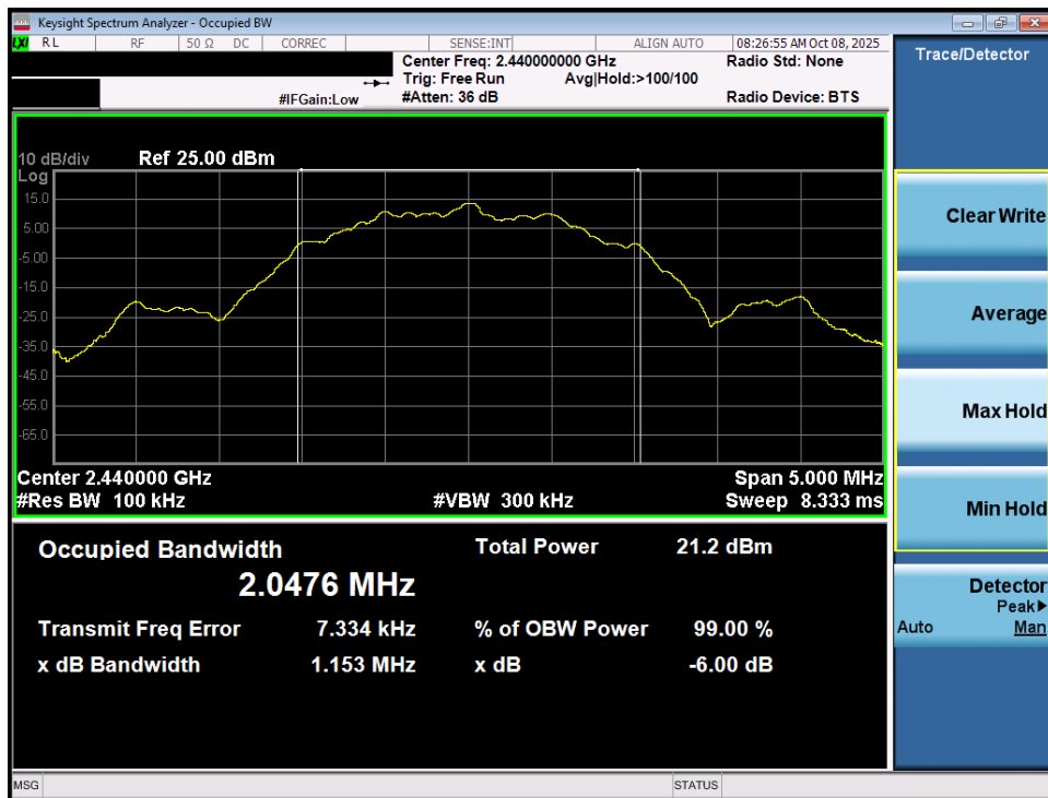
Plot 7-29. 6dB Bandwidth Plot (Bluetooth (LE), 2Mbps – Ch. 17) – Dual Ant 1
