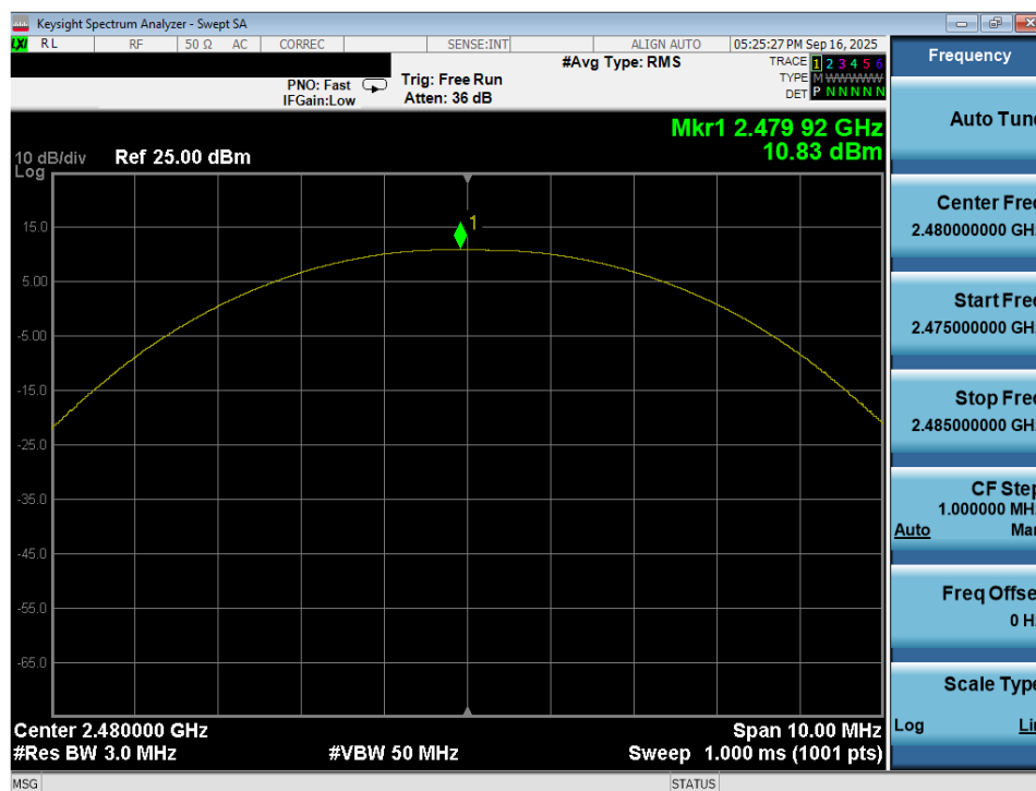
Plot 7-54. Peak Power Plot (Bluetooth (LE), 500kbps – Ch. 39) – Ant 2
