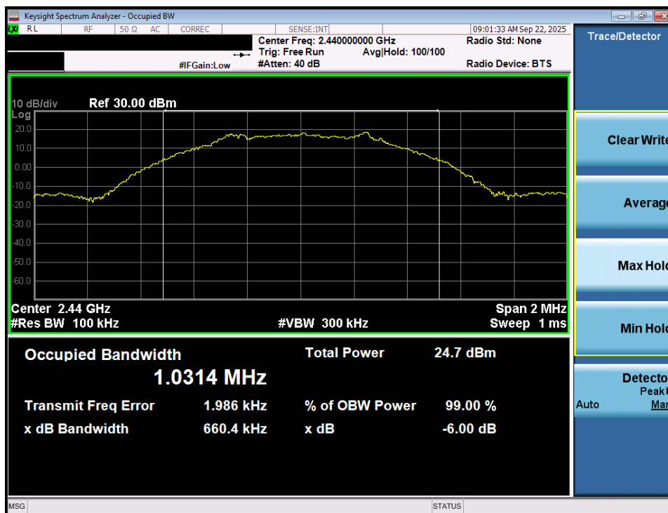
Plot 7-20. 6dB Bandwidth Plot (Bluetooth (LE), 1Mbps – Ch. 17) – Ant 2
