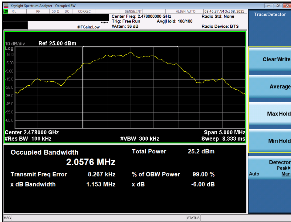
Plot 7-24. 6dB Bandwidth Plot (Bluetooth (LE), 2Mbps – Ch. 36) – Ant 2
