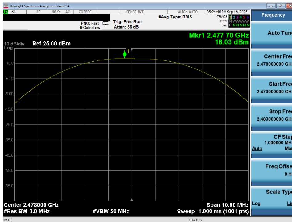
Plot 7-60. Peak Power Plot (Bluetooth (LE), 2Mbps – Ch. 36) – Ant 2
