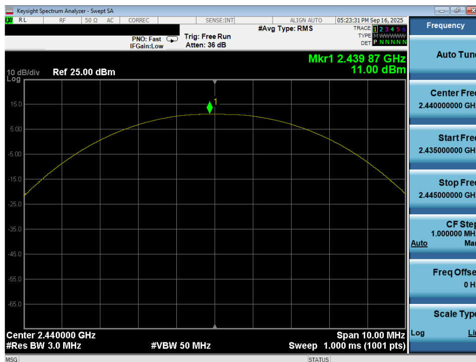
Plot 7-50. Peak Power Plot (Bluetooth (LE), 125kbps – Ch. 17) – Ant 2
