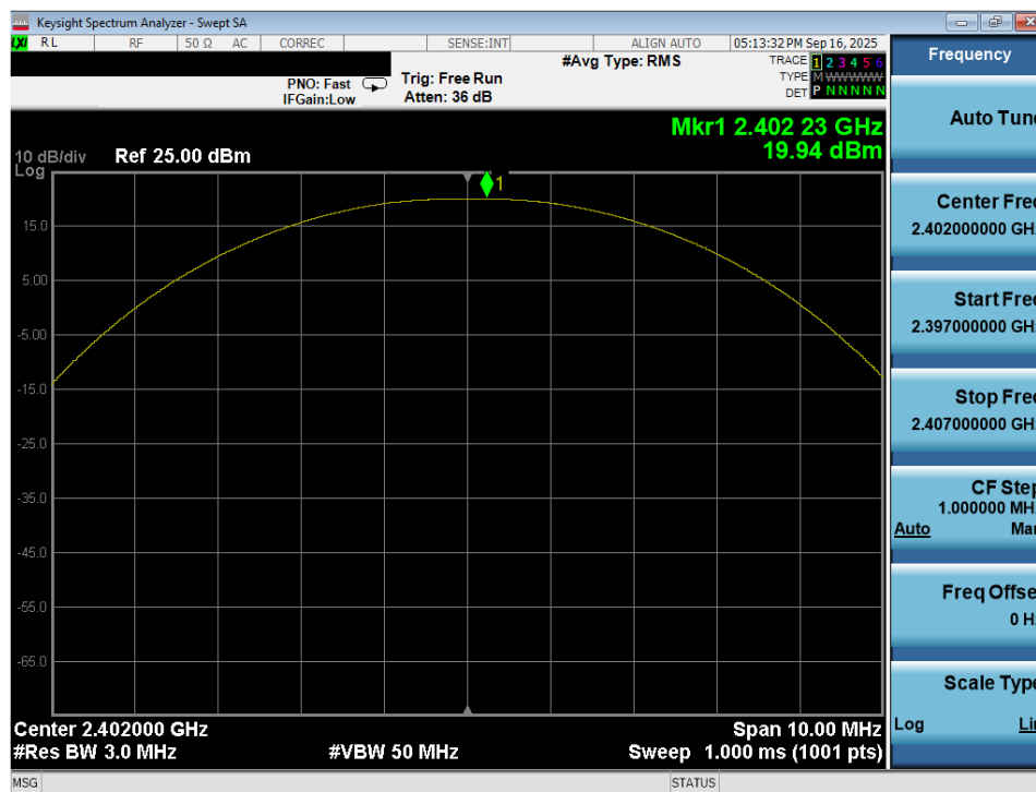
Plot 7-43. Peak Power Plot (Bluetooth (LE), 1Mbps – Ch. 37) – Ant 1
