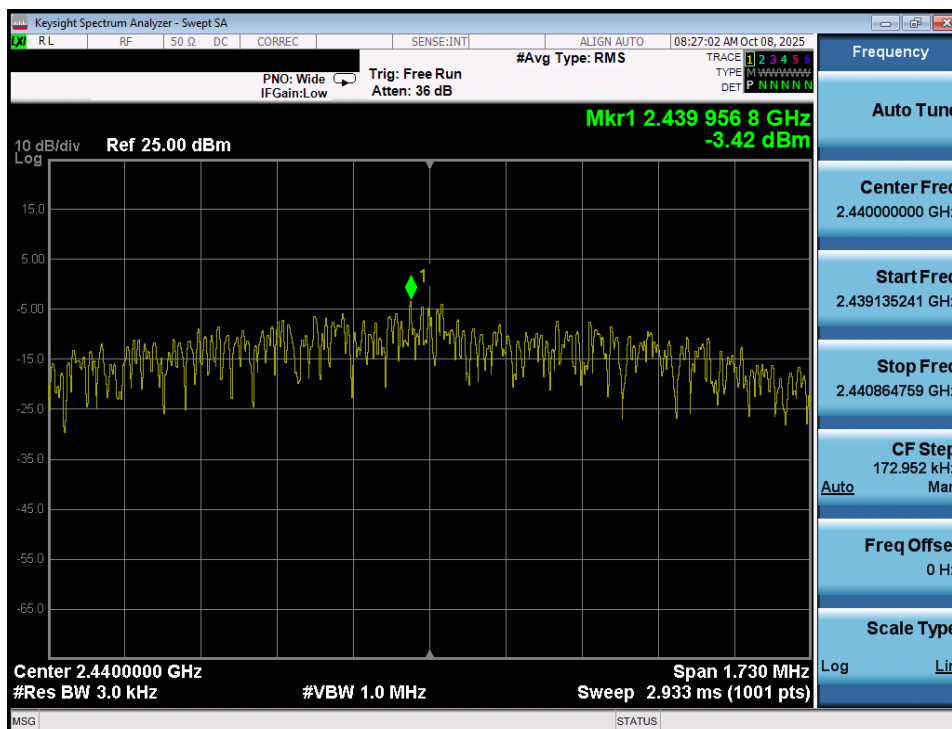
Plot 7-101. Power Spectral Density Plot (Bluetooth (LE), 2Mbps – Ch. 17) – Dual Ant 1
