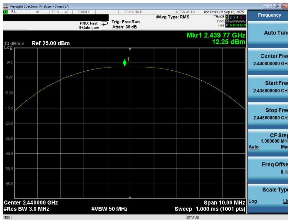
Plot 7-71. Peak Power Plot (Bluetooth (LE), 2Mbps – Ch. 17) – Dual Ant 2
