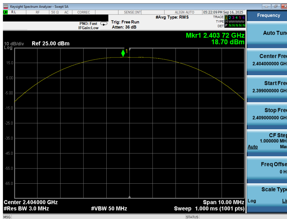
Plot 7-58. Peak Power Plot (Bluetooth (LE), 2Mbps – Ch. 0) – Ant 2
