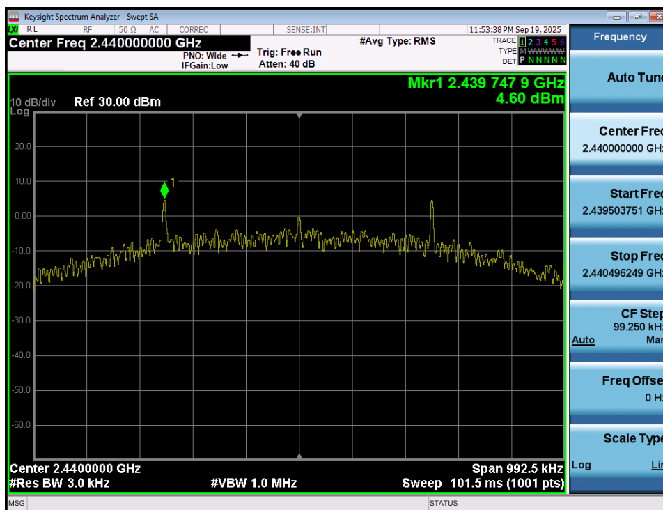
Plot 7-77. Power Spectral Density Plot (Bluetooth (LE), 500kbps – Ch. 17) – Ant 1
