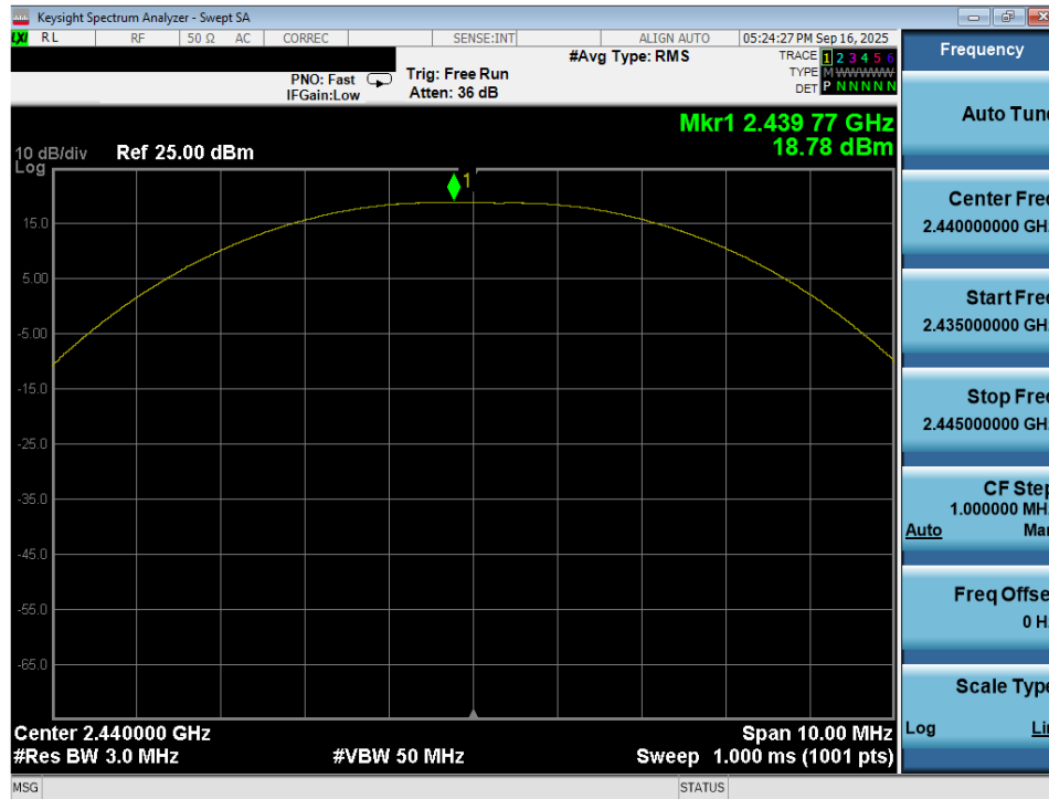
Plot 7-59. Peak Power Plot (Bluetooth (LE), 2Mbps – Ch. 17) – Ant 2
