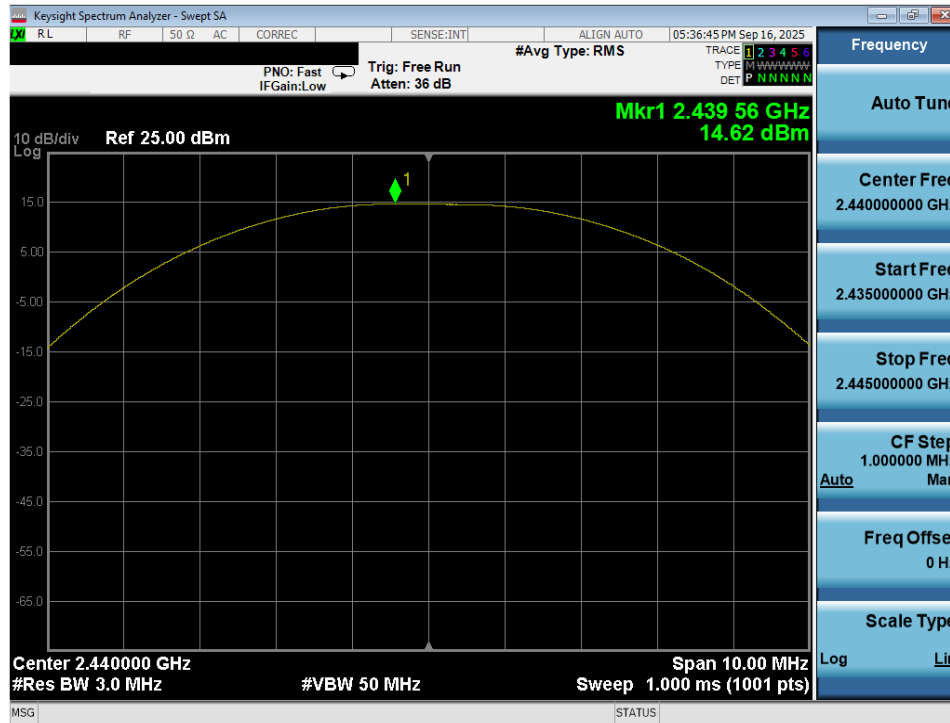
Plot 7-65. Peak Power Plot (Bluetooth (LE), 2Mbps – Ch. 17) – Dual Ant 1
