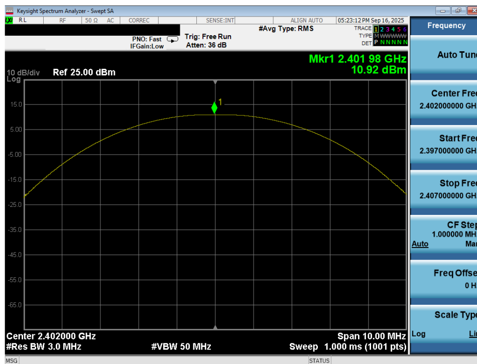
Plot 7-49. Peak Power Plot (Bluetooth (LE), 125kbps – Ch. 37) – Ant 2
