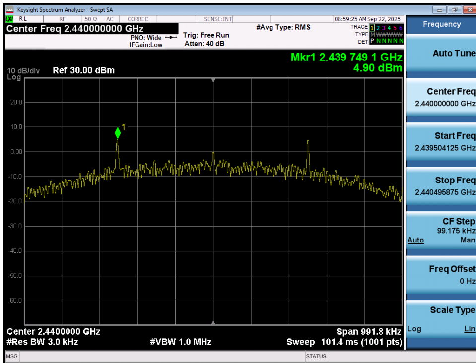
Plot 7-89. Power Spectral Density Plot (Bluetooth (LE), 500kbps – Ch. 17) – Ant 2
