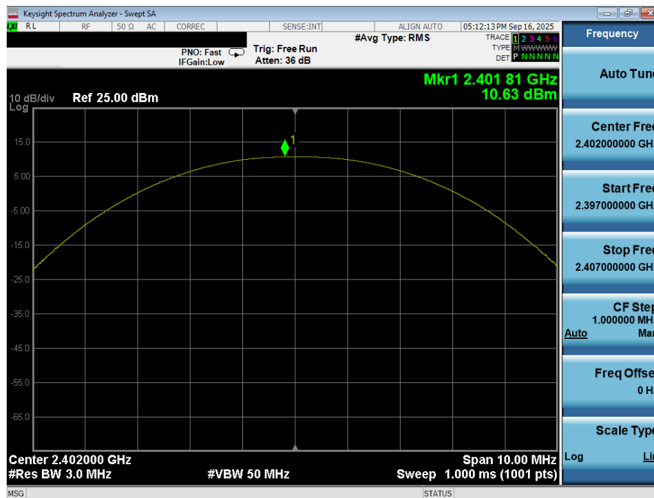
Plot 7-40. Peak Power Plot (Bluetooth (LE), 500kbps – Ch. 37) – Ant 1
