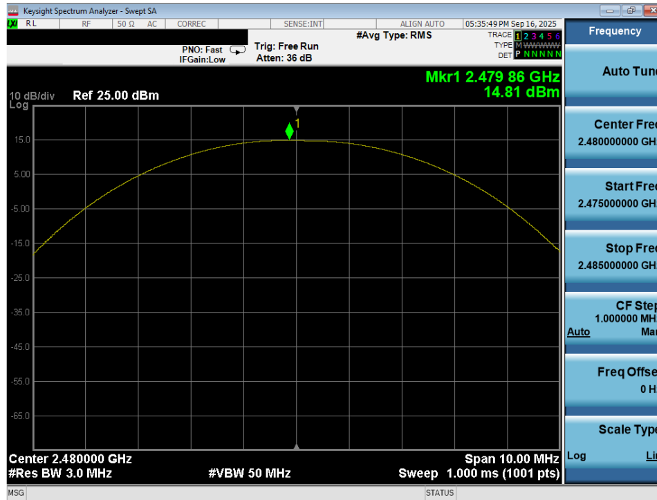
Plot 7-63. Peak Power Plot (Bluetooth (LE), 1Mbps – Ch. 39) – Dual Ant 1
