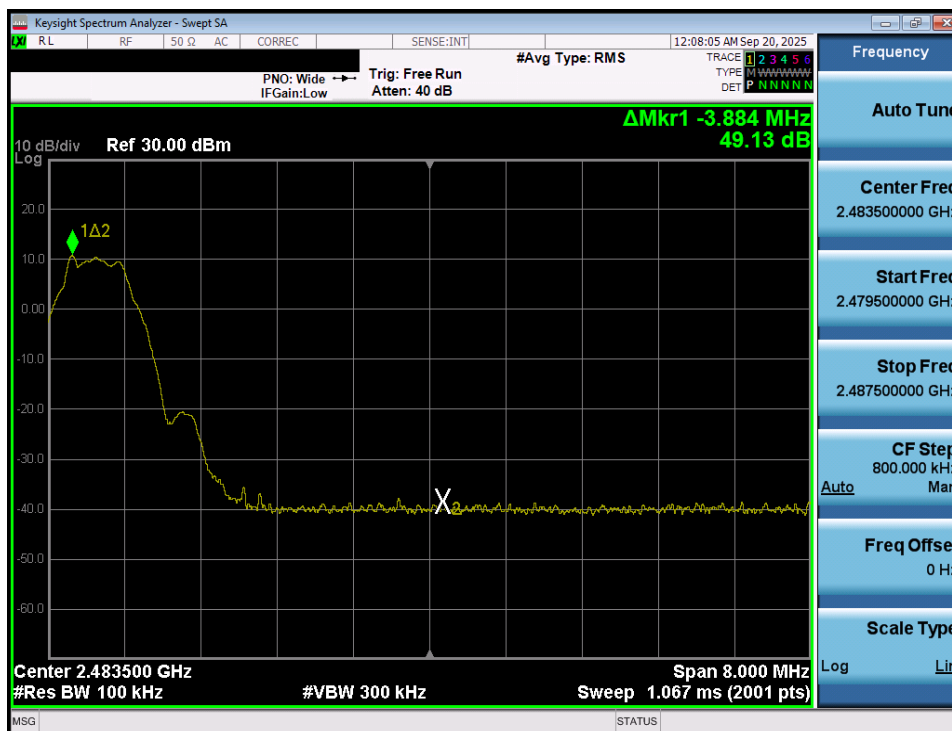
Plot 7-112. Band Edge Plot (Bluetooth (LE), 500kbps – Ch. 39) – Ant 1
