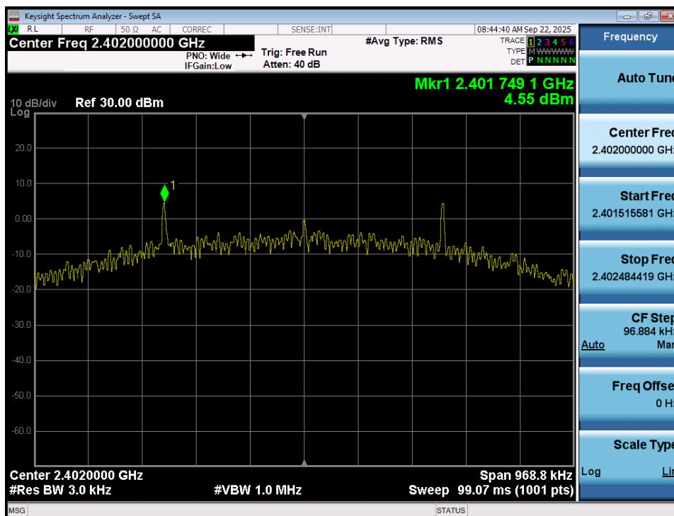
Plot 7-88. Power Spectral Density Plot (Bluetooth (LE), 500kbps – Ch. 37) – Ant 2
