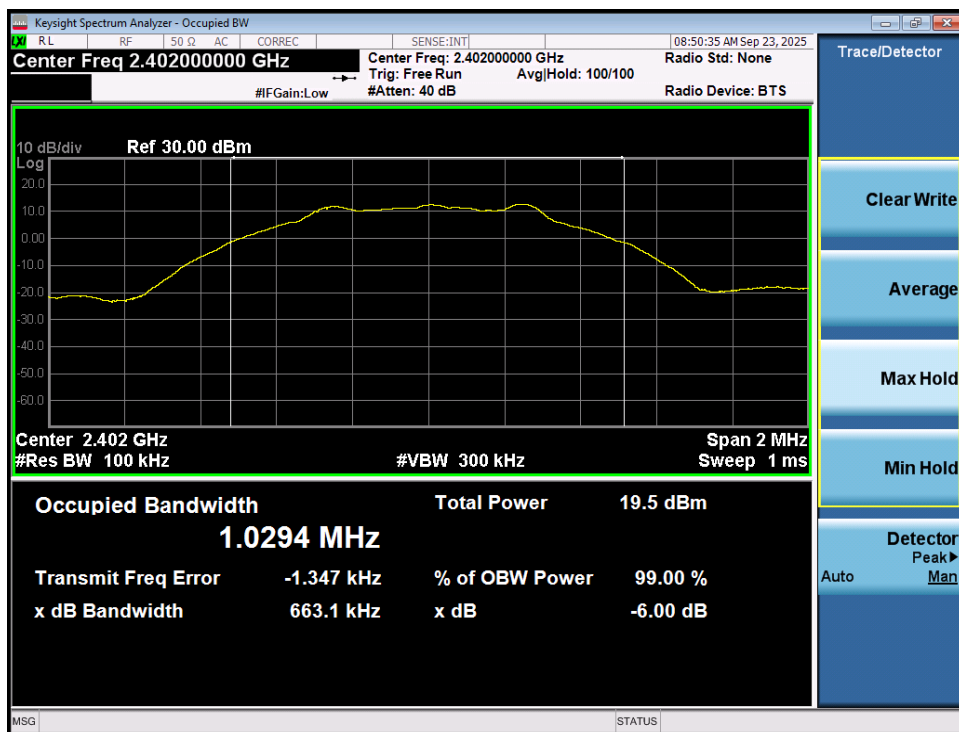
Plot 7-31. 6dB Bandwidth Plot (Bluetooth (LE), 1Mbps – Ch. 37) – Dual Ant 2
