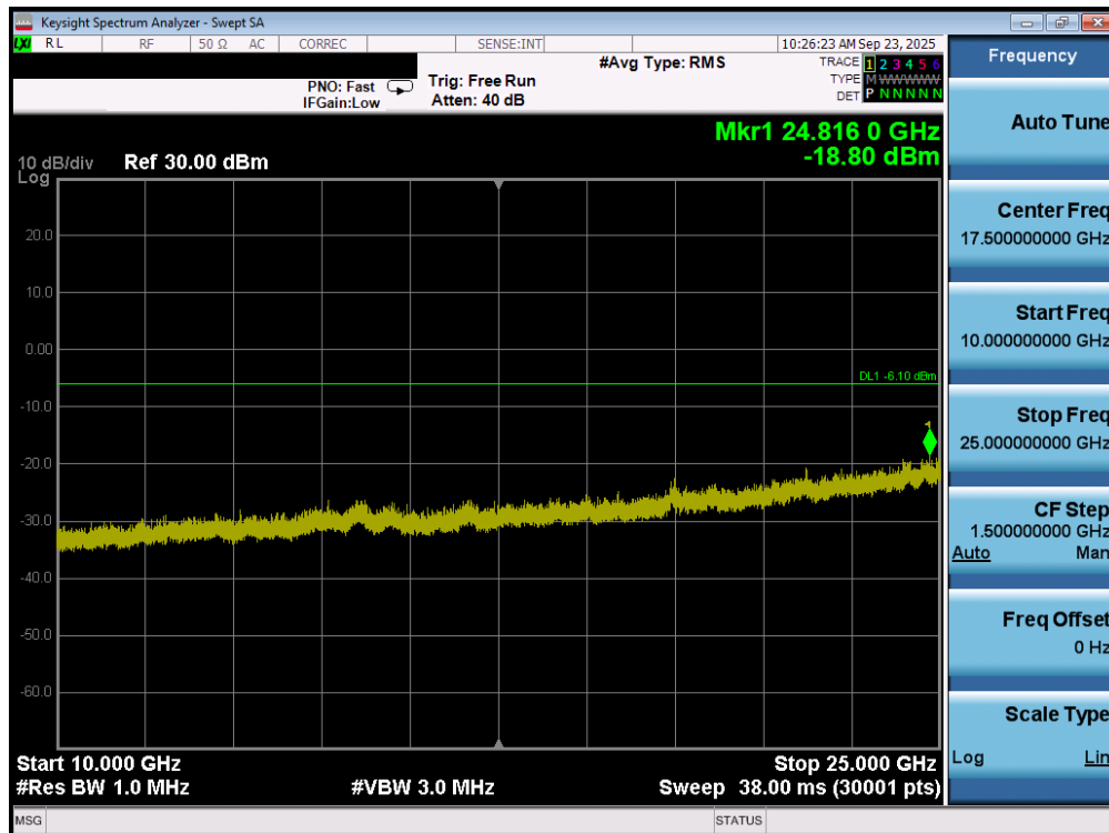
Plot 7-154. Conducted Spurious Plot (Bluetooth, 3Mbps – Ch. 0) – Dual Ant 1
