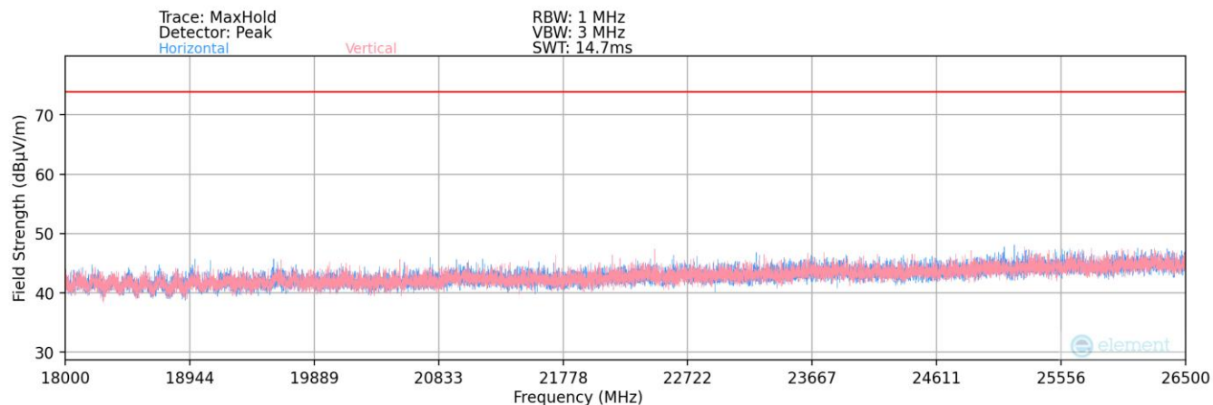
Plot 7-176. Radiated Spurious Plot above 18GHz – Dual
