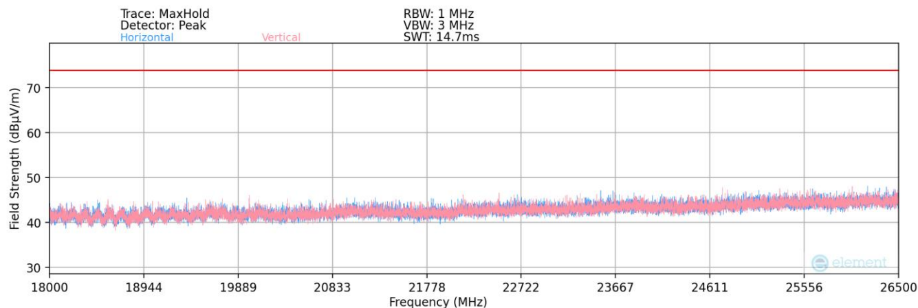
Plot 7-168. Radiated Spurious Plot above 18GHz – Ant 1
