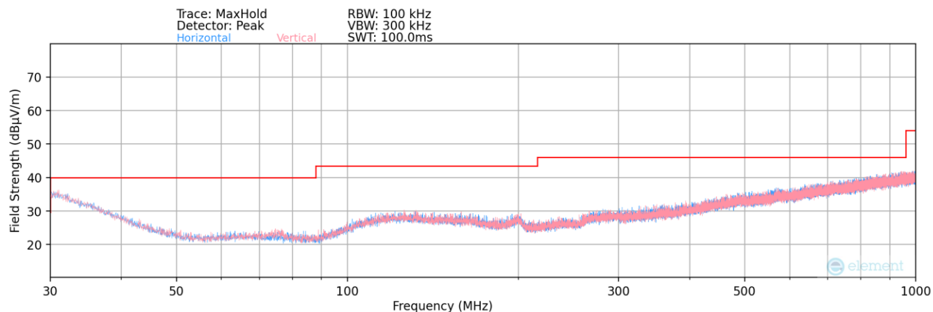
Plot 7-191. Radiated Spurious Plot below 1GHz – Dual
