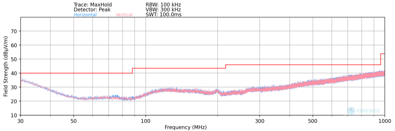
Plot 7-189. Radiated Spurious Plot below 1GHz – Ant 1
