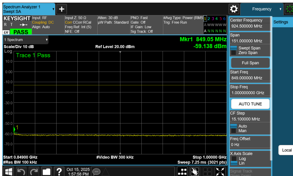
Plot 7-103. Conducted Spurious Plot (NR Band n5 - 20.0MHz - 1 RB - High Channel - Ant2)
