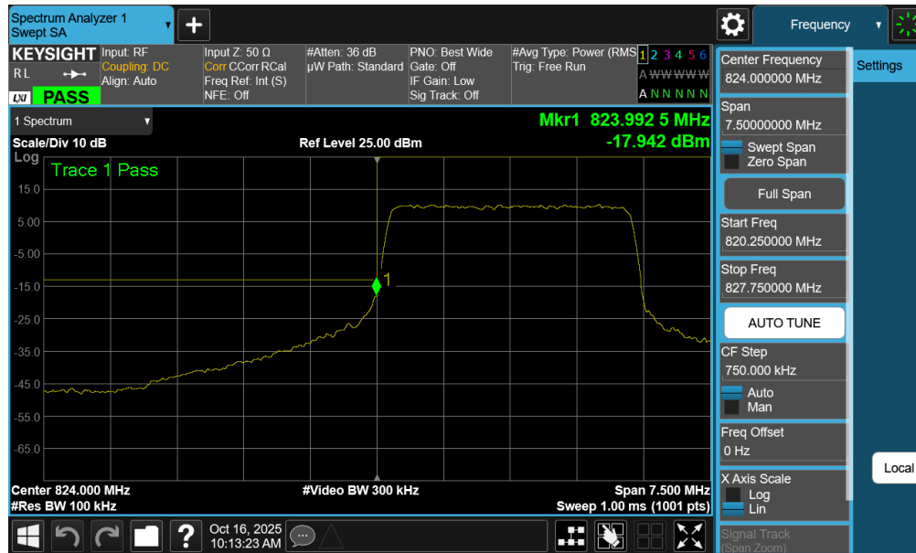
Plot 7-129. Lower Band Edge Plot (LTE Band 26/5 - 3MHz QPSK - Full RB - Ant1)
