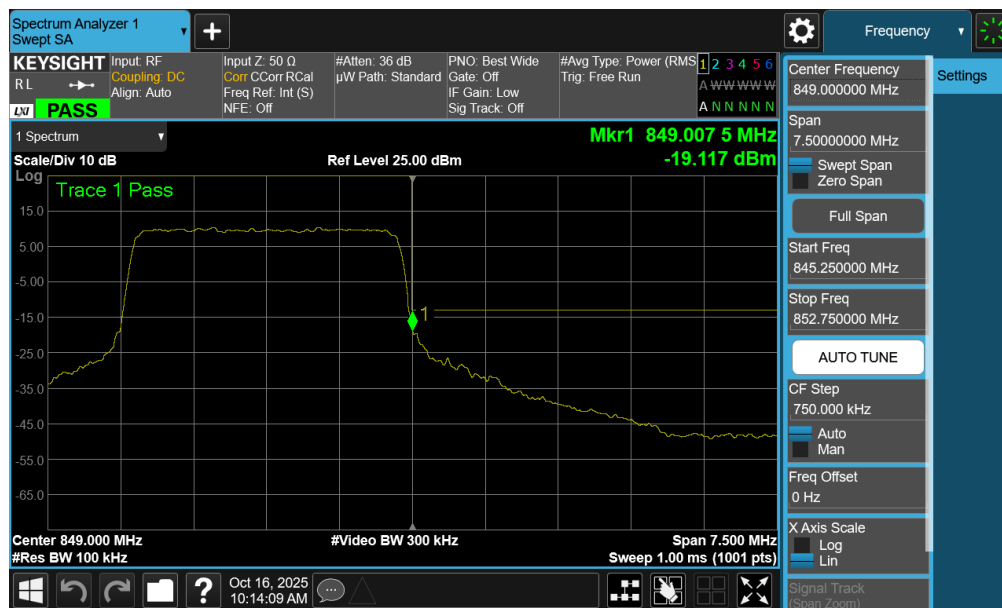
Plot 7-130. Upper Band Edge Plot (LTE Band 26/5 - 3MHz QPSK - Full RB - Ant1)
