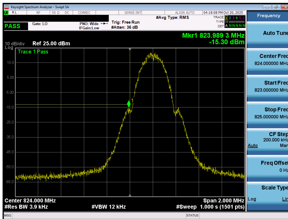
Plot 7-141. Lower Band Edge Plot (GPRS Cell – Ch. 128 – Ant1)
