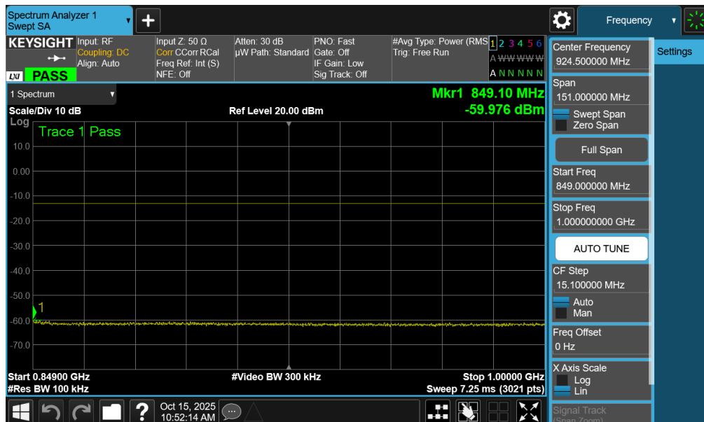
Plot 7-67. Conducted Spurious Plot (NR Band n5 - 20.0MHz - 1 RB - High Channel - Ant1)
