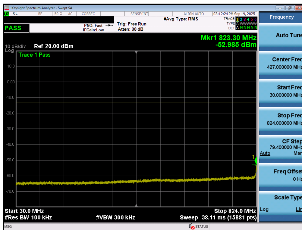
Plot 7-81. Conducted Spurious Plot (WCDMA Ch. 4183 – Ant1)
