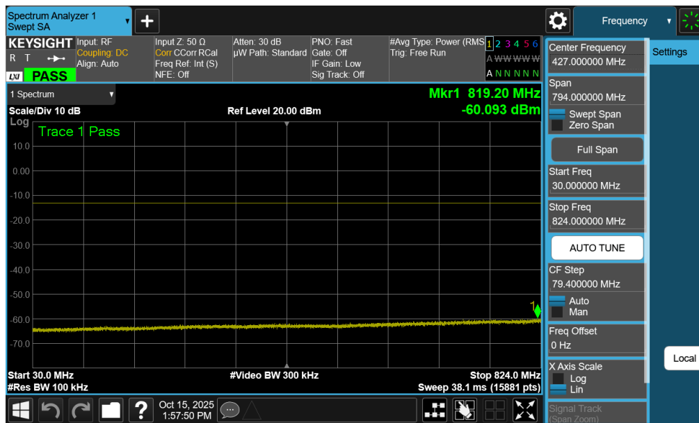
Plot 7-102. Conducted Spurious Plot (NR Band n5 - 20.0MHz - 1 RB - High Channel - Ant2)
