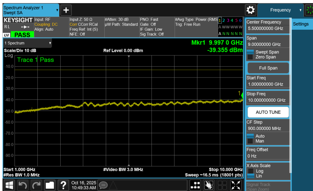
Plot 7-95. Conducted Spurious Plot (LTE Band 26/5 - 15MHz QPSK - 1 RB - High Channel – Ant2)
