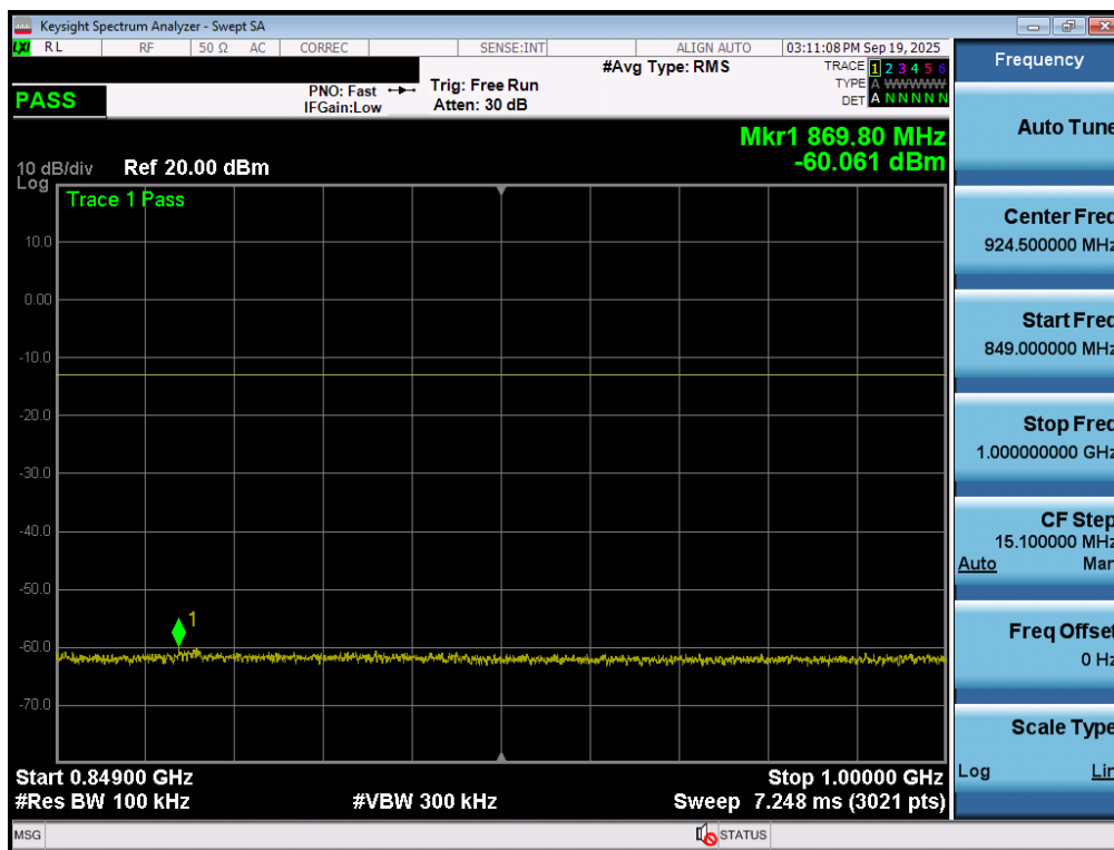
Plot 7-79. Conducted Spurious Plot (WCDMA Ch. 4132 – Ant1)
