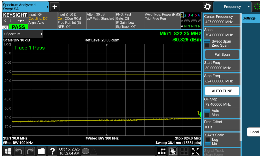
Plot 7-66. Conducted Spurious Plot (NR Band n5 - 20.0MHz - 1 RB - High Channel - Ant1)
