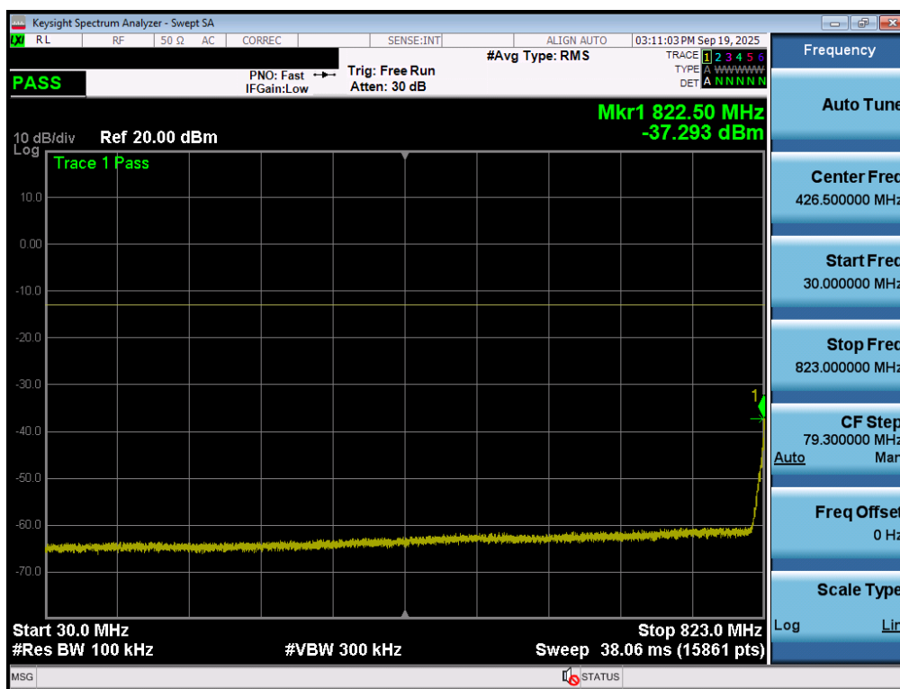
Plot 7-78. Conducted Spurious Plot (WCDMA Ch. 4132 – Ant1)
