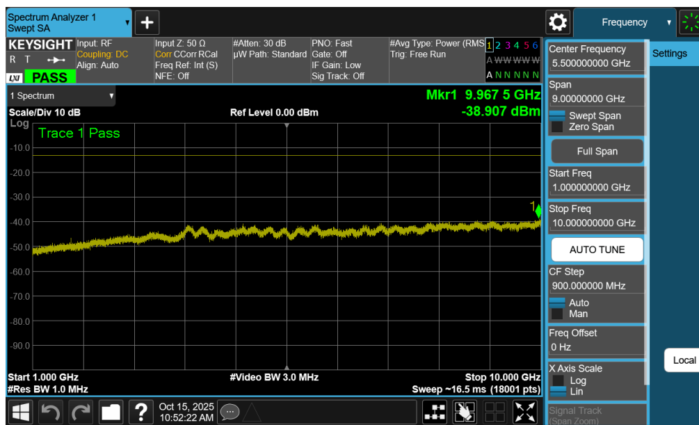
Plot 7-68. Conducted Spurious Plot (NR Band n5 - 20.0MHz - 1 RB - High Channel - Ant1)
