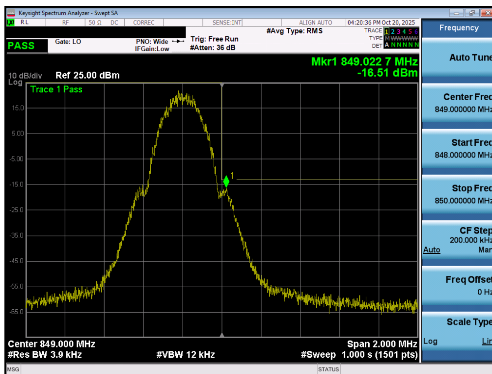
Plot 7-142. Upper Band Edge Plot (GPRS Cell – Ch. 251 – Ant1)
