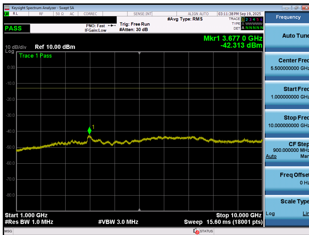
Plot 7-80. Conducted Spurious Plot (WCDMA Ch. 4132 – Ant1)
