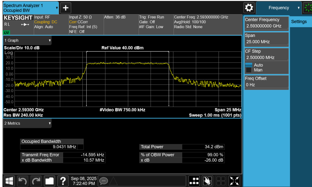
Plot 7-5. Occupied Bandwidth Plot (LTE Band 41PC2 - 10MHz QPSK - Full RB - Ant1)
