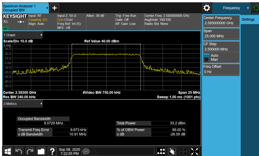
Plot 7-6. Occupied Bandwidth Plot (LTE Band 41PC2 - 10MHz 16-QAM - Full RB - Ant1)
