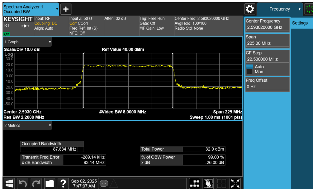
Plot 7-22. Occupied Bandwidth Plot (NR Band n41 PC2 – 90MHz 16-QAM – Full RB – Default – Ant1)
