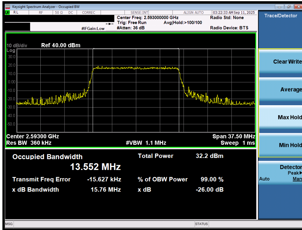
Plot 7-11. Occupied Bandwidth Plot (LTE Band 41(PC3) - 15MHz QPSK - Full RB - Ant1)
