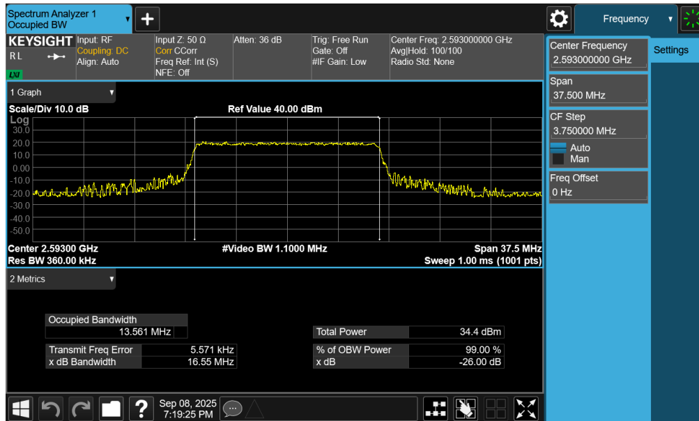
Plot 7-3. Occupied Bandwidth Plot (LTE Band 41PC2 - 15MHz QPSK - Full RB - Ant1)
