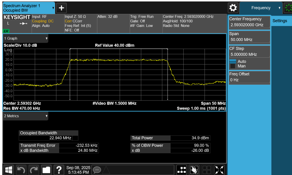
Plot 7-47. Occupied Bandwidth Plot (NR Band n41 PC2 – 25MHz \pi/2 BPSK – Full RB – Default – Ant1)
