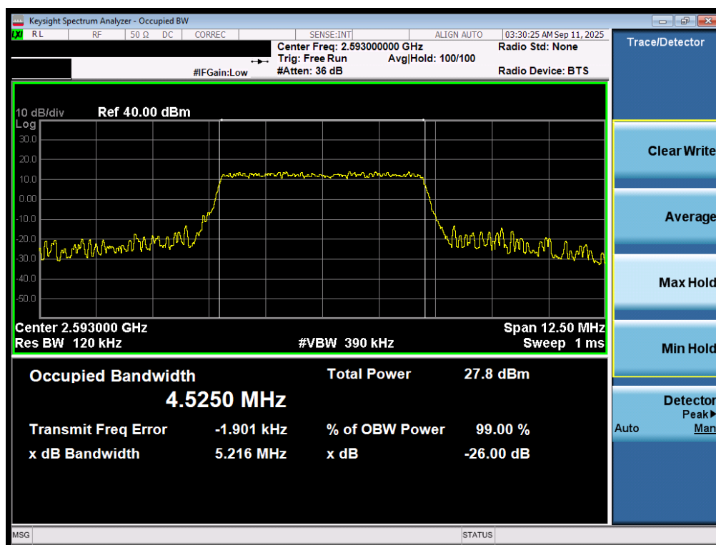
Plot 7-16. Occupied Bandwidth Plot (LTE Band 41(PC3) - 5MHz 16-QAM - Full RB - Ant1)
