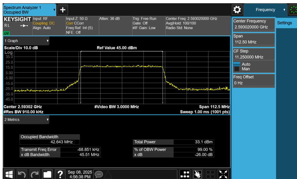
Plot 7-36. Occupied Bandwidth Plot (NR Band n41 PC2 – 45MHz QPSK – Full RB – Default – Ant1)
