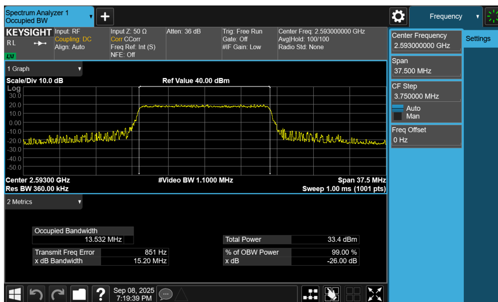
Plot 7-4. Occupied Bandwidth Plot (LTE Band 41PC2 - 15MHz 16-QAM - Full RB - Ant1)
