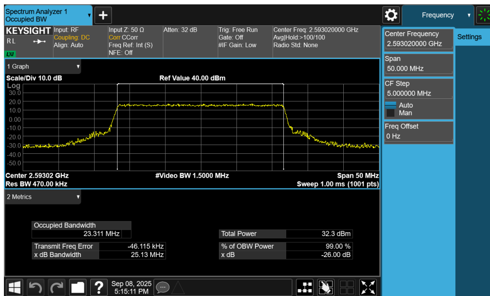
Plot 7-48. Occupied Bandwidth Plot (NR Band n41 PC2 – 25MHz QPSK – Full RB – Default – Ant1)
