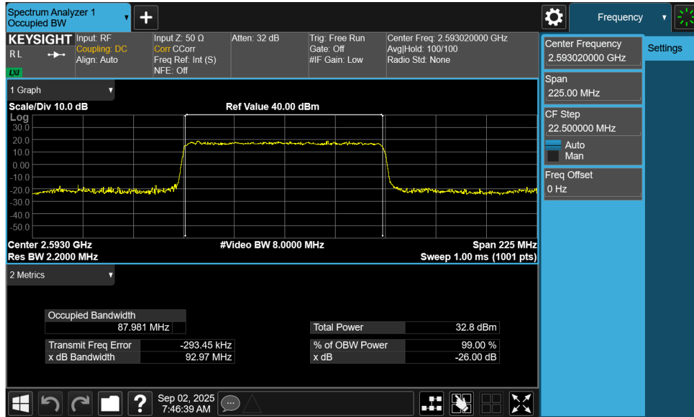
Plot 7-21. Occupied Bandwidth Plot (NR Band n41 PC2 – 90MHz QPSK – Full RB – Default – Ant1)
