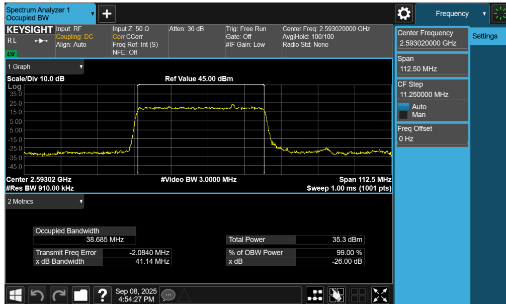
Plot 7-35. Occupied Bandwidth Plot (NR Band n41 PC2 – 45MHz \pi/2 BPSK – Full RB – Default – Ant1)
