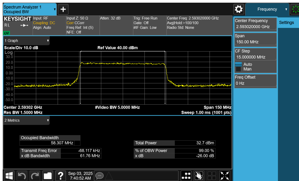
Plot 7-72. Occupied Bandwidth Plot (NR Band n41 PC2 – 60MHz QPSK – Full RB – Switch – Ant1)
