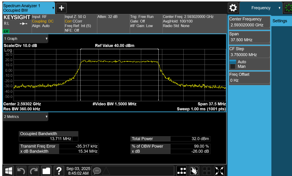
Plot 7-97. Occupied Bandwidth Plot (NR Band n41 PC2 – 15MHz 16-QAM – Full RB – Switch – Ant1)
