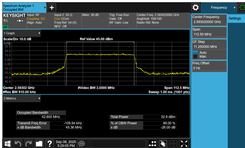
Plot 7-78. Occupied Bandwidth Plot (NR Band n41 PC2 – 45MHz QPSK – Full RB – Switch – Ant1)
