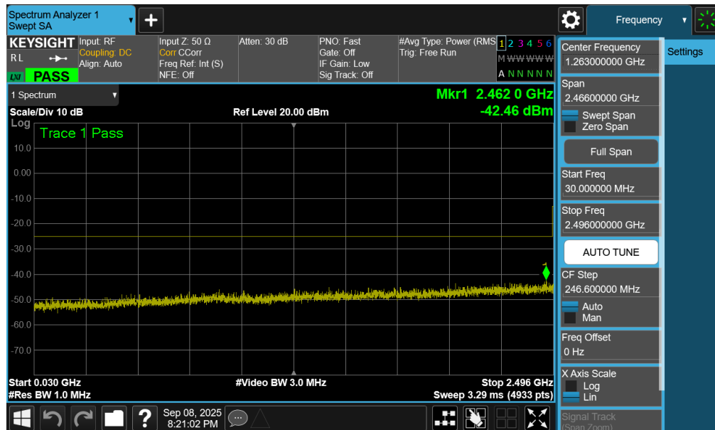
Plot 7-129. Conducted Spurious Plot (LTE Band 41PC2 - 20MHz QPSK - RB Size 1, RB Offset 0 - High Channel - Ant2)
