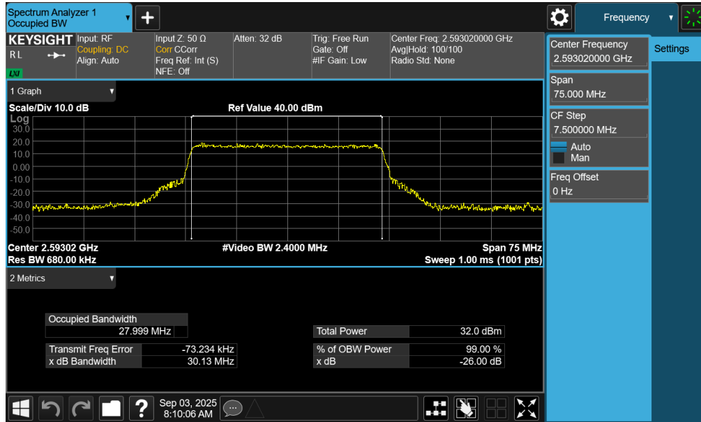
Plot 7-87. Occupied Bandwidth Plot (NR Band n41 PC2 – 30MHz QPSK – Full RB – Switch – Ant1)
