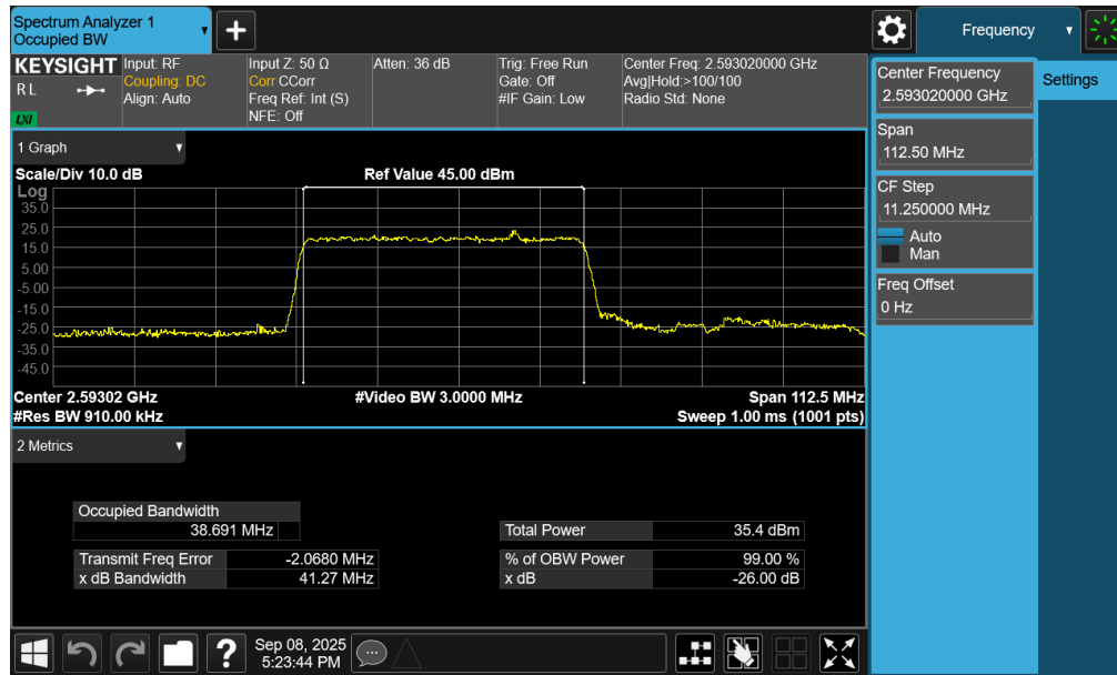
Plot 7-77. Occupied Bandwidth Plot (NR Band n41 PC2 – 45MHz \pi/2 BPSK – Full RB – Switch – Ant1)
