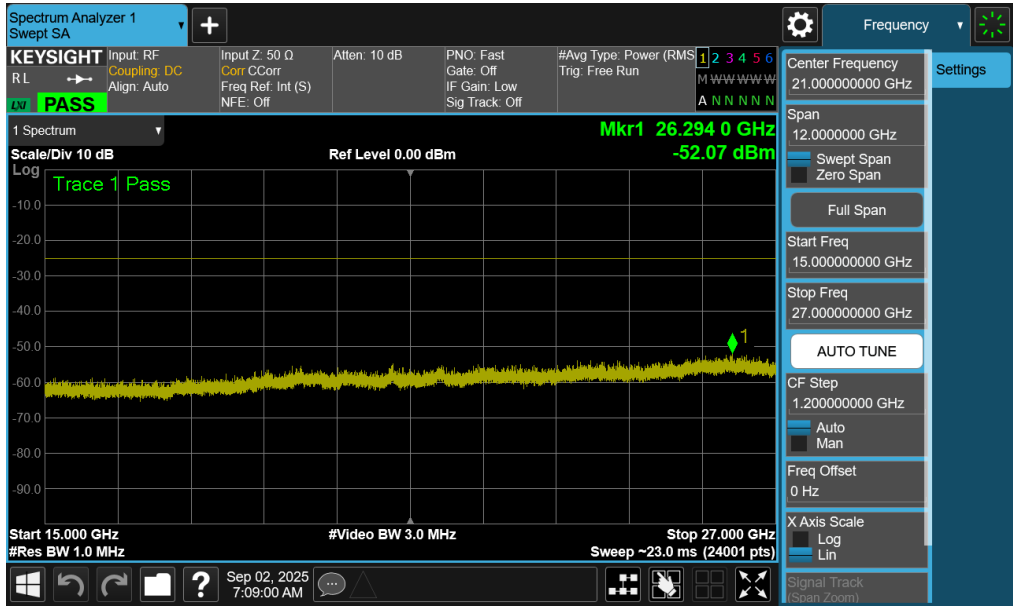
Plot 7-125. Conducted Spurious Plot (NR Band n41PC2 - 100MHz QPSK - RB Size 1, RB Offset 0 - Mid Channel Ant1)
