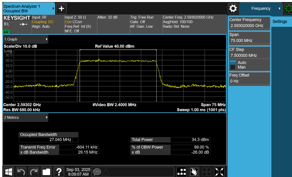
Plot 7-86. Occupied Bandwidth Plot (NR Band n41 PC2 – 30MHz \pi/2 BPSK – Full RB – Switch – Ant1)
