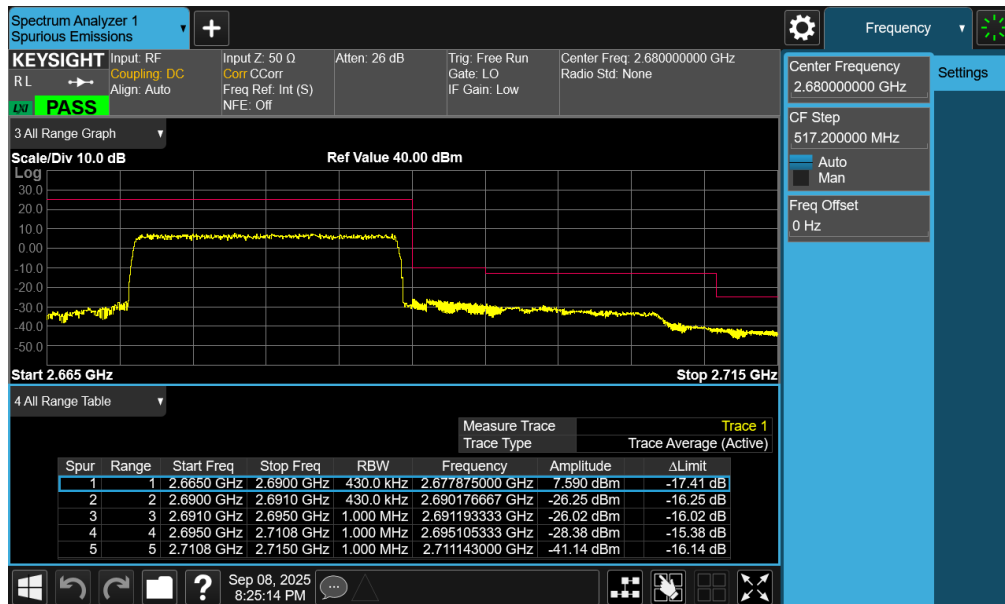
Plot 7-144. Upper ACP Plot (LTE Band 41(PC2) - 20MHz QPSK – Full RB - Ant2)
