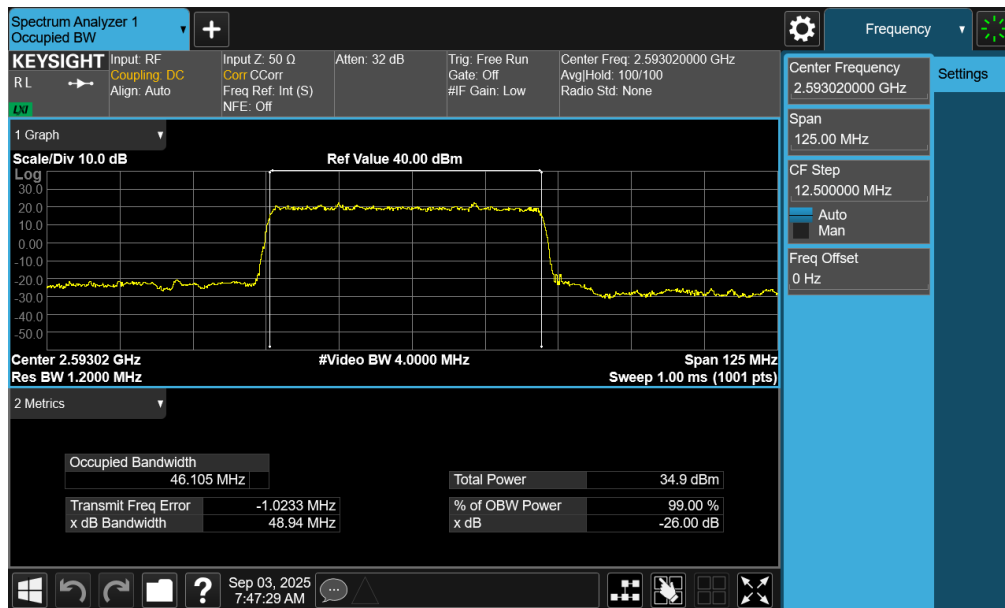
Plot 7-74. Occupied Bandwidth Plot (NR Band n41 PC2 – 50MHz \pi/2 BPSK – Full RB – Switch – Ant1)
