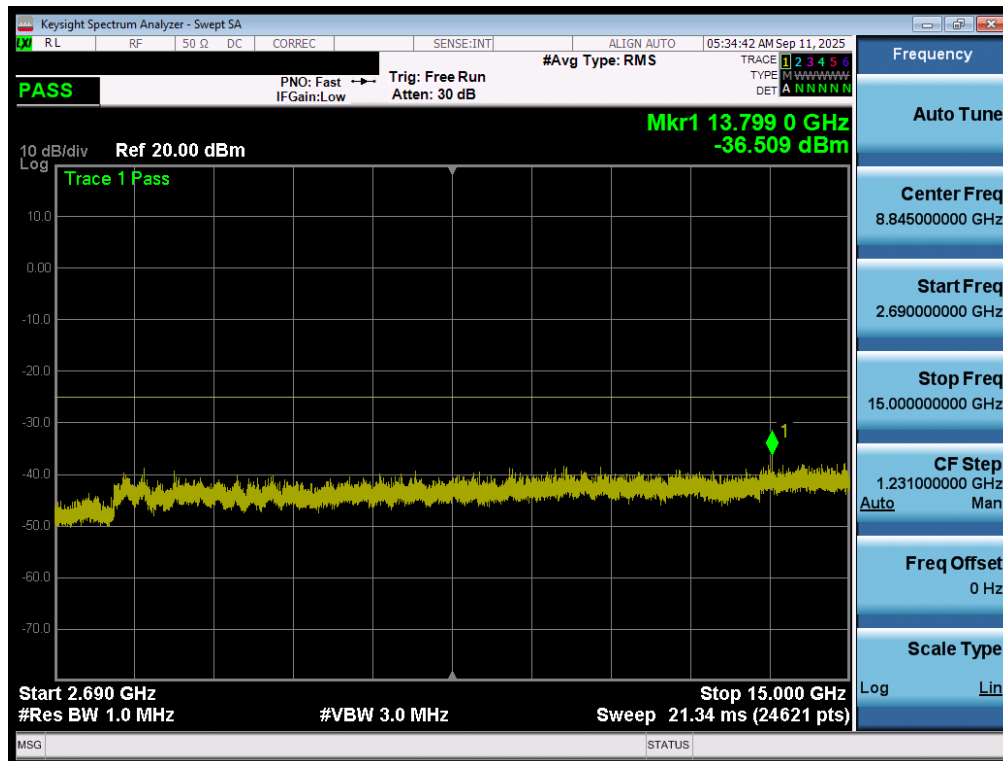
Plot 7-133. Conducted Spurious Plot (LTE Band 41(PC3) - 20MHz QPSK - RB Size 1, RB Offset 0 - Mid Channel - Ant2)
