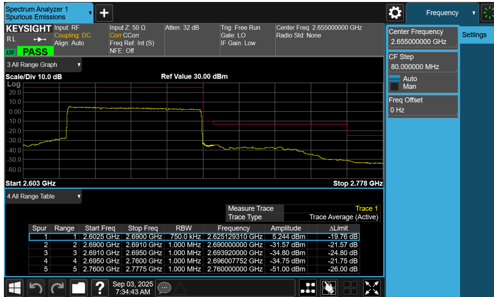
Plot 7-142. Upper ACP Plot (NR Band n41PC2 - 70MHz CP-OFDM-QPSK – Full RB - Ant1)
