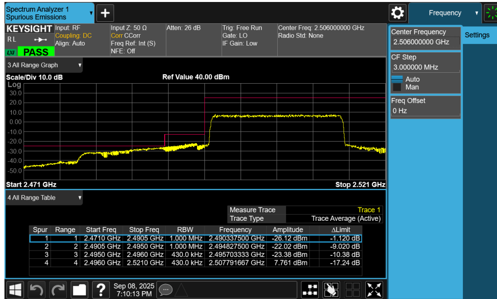
Plot 7-135. Lower ACP Plot (LTE Band 41(PC2) - 20MHz QPSK – Full RB - Ant1)
