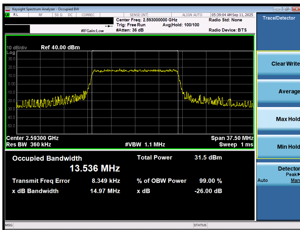
Plot 7-111. Occupied Bandwidth Plot (LTE Band 41(PC3) - 15MHz QPSK - Full RB - Ant2)
