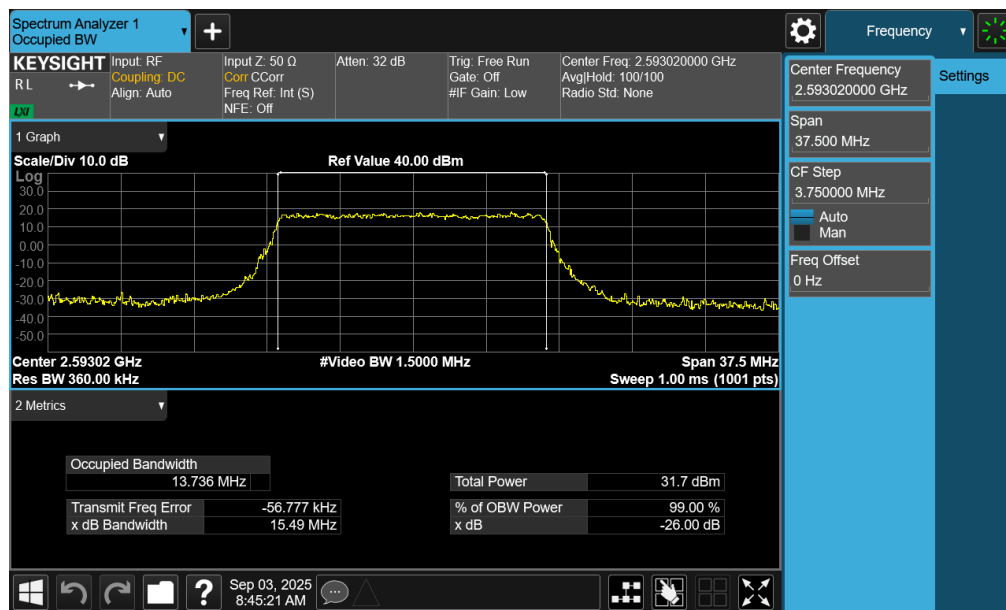
Plot 7-96. Occupied Bandwidth Plot (NR Band n41 PC2 – 15MHz QPSK – Full RB – Switch – Ant1)
