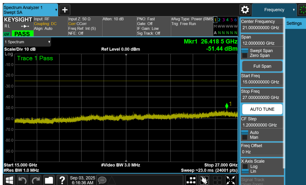
Plot 7-128. Conducted Spurious Plot (NR Band n41PC2 - 100MHz QPSK - RB Size 1, RB Offset 0 - Mid Channel Ant1)
