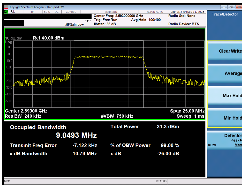
Plot 7-113. Occupied Bandwidth Plot (LTE Band 41(PC3) - 10MHz QPSK - Full RB - Ant2)
