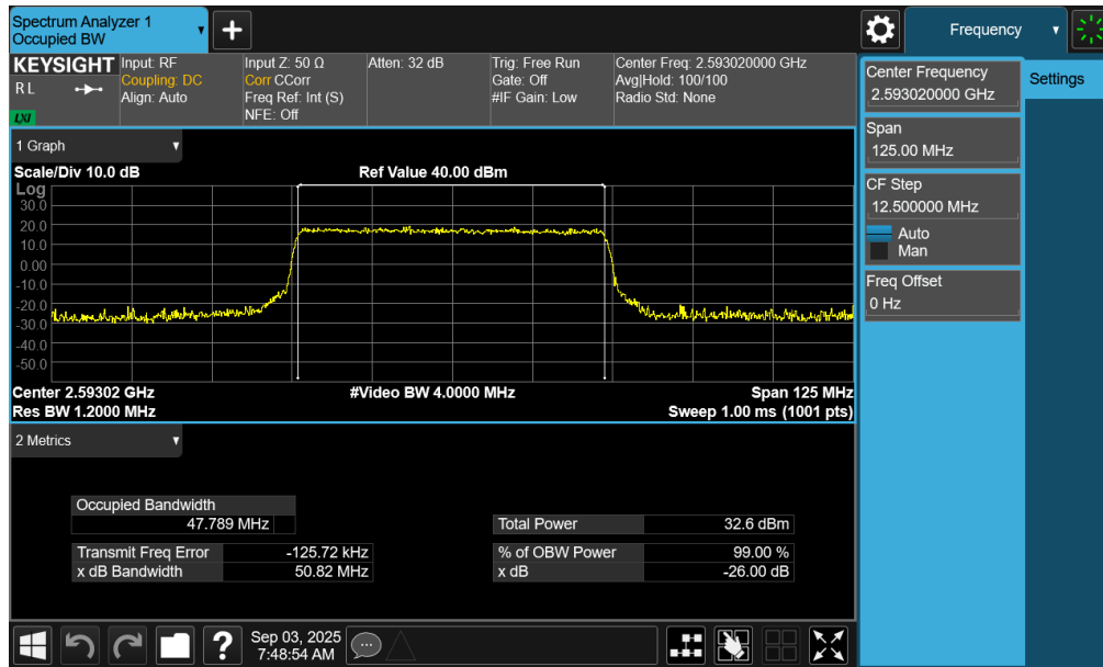
Plot 7-75. Occupied Bandwidth Plot (NR Band n41 PC2 – 50MHz QPSK – Full RB – Switch – Ant1)
