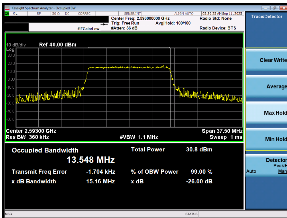
Plot 7-112. Occupied Bandwidth Plot (LTE Band 41(PC3) - 15MHz 16-QAM - Full RB - Ant2)
