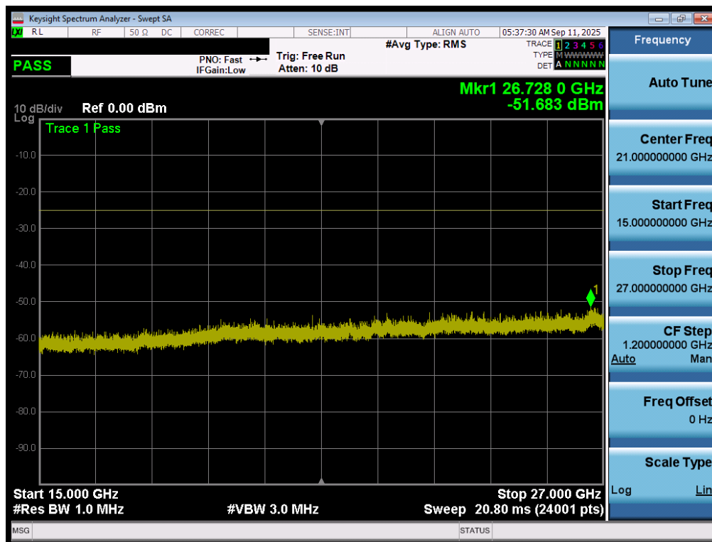
Plot 7-134. Conducted Spurious Plot (LTE Band 41(PC3) - 20MHz QPSK - RB Size 1, RB Offset 0 - Mid Channel - Ant2)
