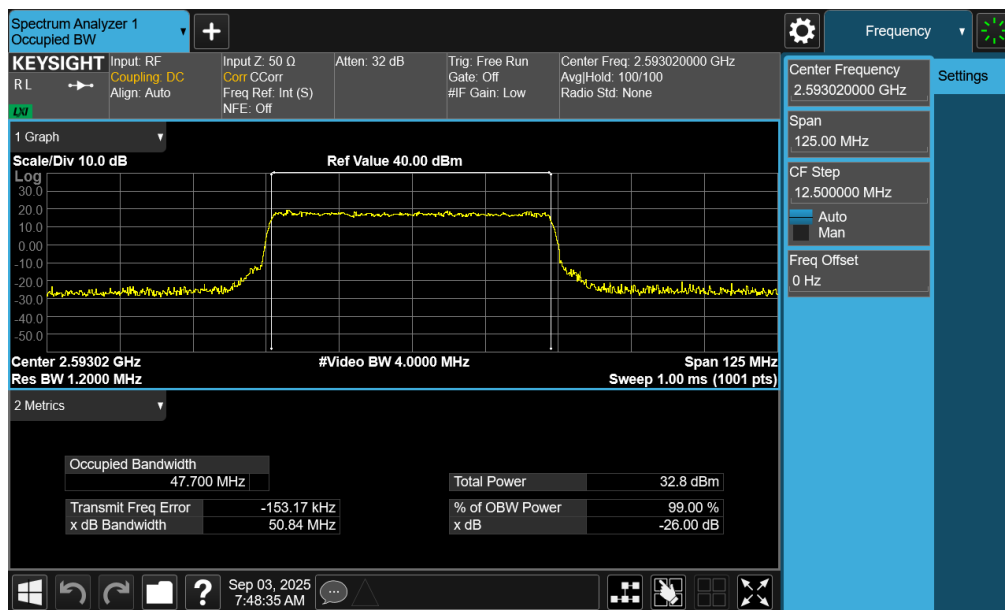
Plot 7-76. Occupied Bandwidth Plot (NR Band n41 PC2 – 50MHz 16-QAM – Full RB – Switch – Ant1)
