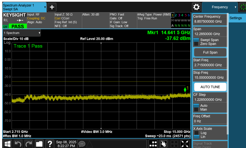
Plot 7-130. Conducted Spurious Plot (LTE Band 41PC2 - 20MHz QPSK - RB Size 1, RB Offset 0 - High Channel - Ant2)
