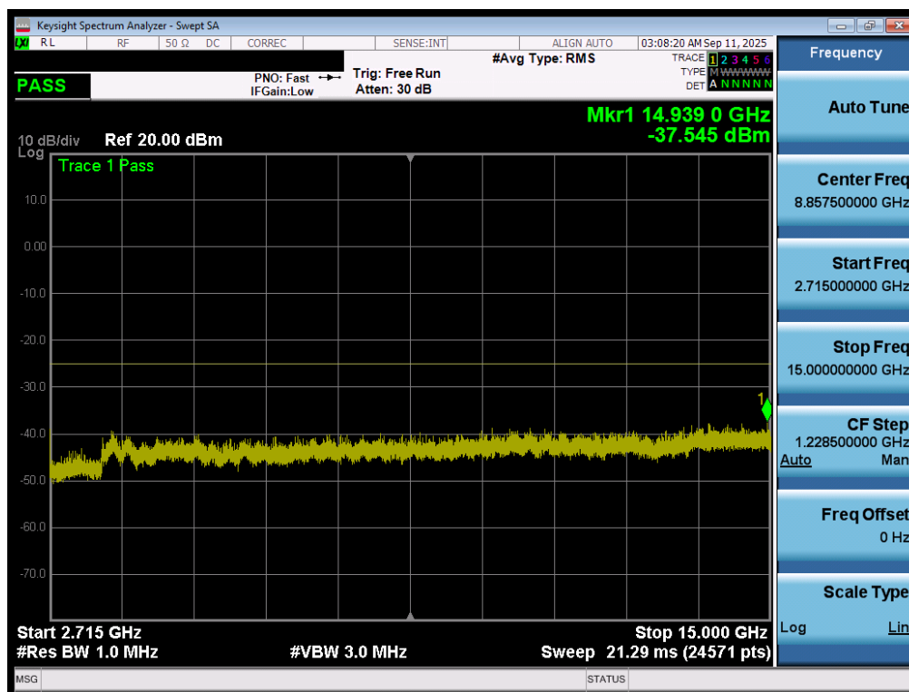
Plot 7-121. Conducted Spurious Plot (LTE Band 41(PC3)- 20MHz QPSK - RB Size 1, RB Offset 0 - High Channel - Ant1)
