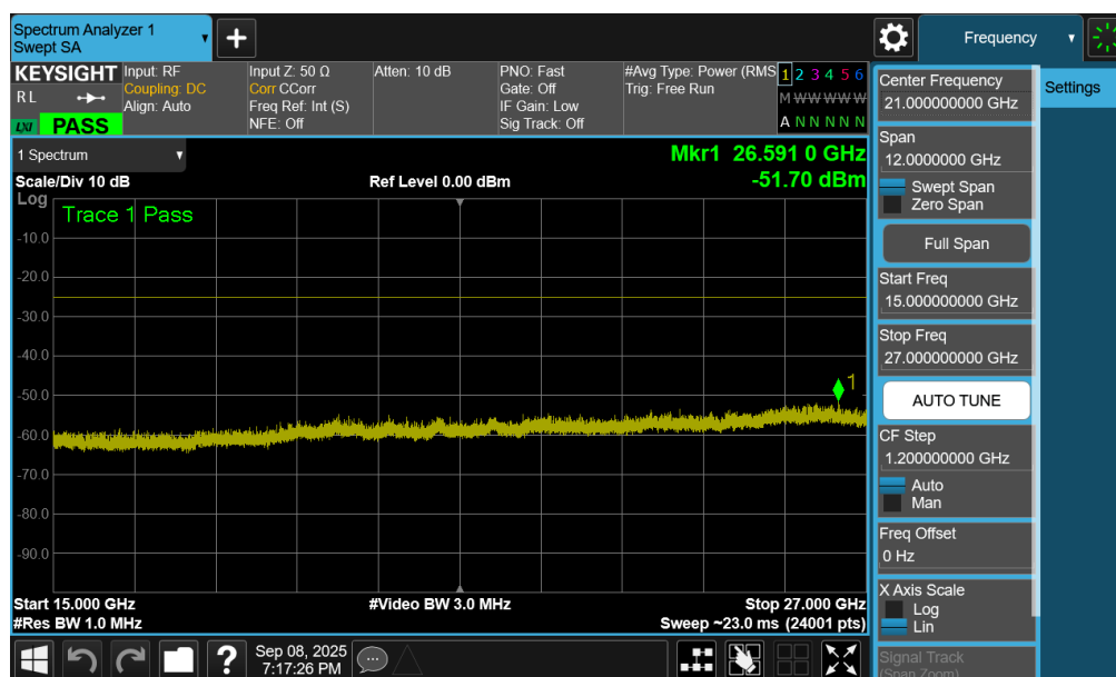
Plot 7-119. Conducted Spurious Plot (LTE Band 41PC2 - 20MHz QPSK - RB Size 1, RB Offset 0 - High Channel - Ant1)
