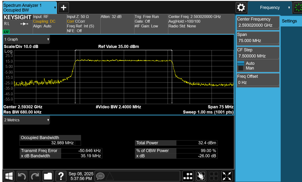
Plot 7-85. Occupied Bandwidth Plot (NR Band n41 PC2 – 35MHz 16-QAM – Full RB – Switch – Ant1)
