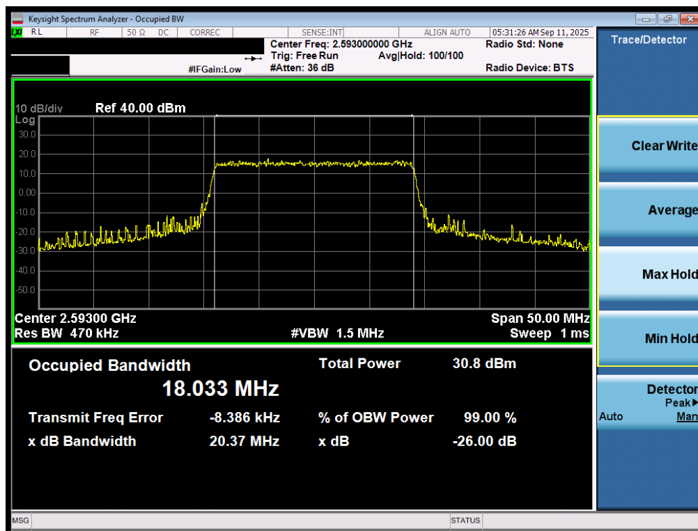
Plot 7-110. Occupied Bandwidth Plot (LTE Band 41(PC3) - 20MHz 16-QAM - Full RB - Ant2)
