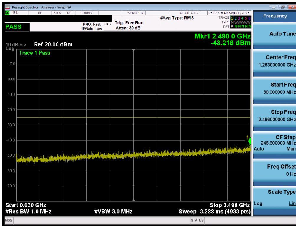
Plot 7-132. Conducted Spurious Plot (LTE Band 41(PC3) - 20MHz QPSK - RB Size 1, RB Offset 0 - Mid Channel - Ant2)
