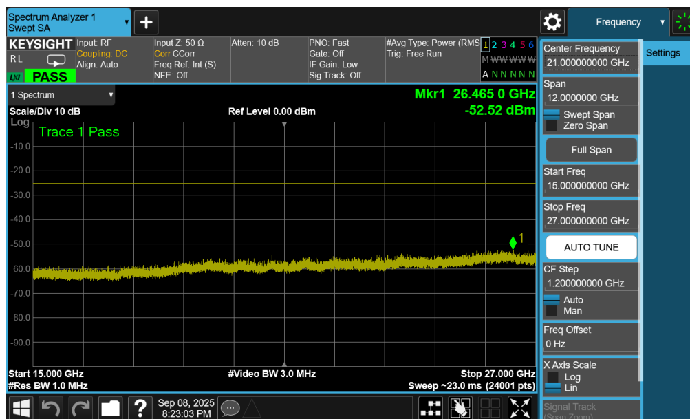
Plot 7-131. Conducted Spurious Plot (LTE Band 41PC2 - 20MHz QPSK - RB Size 1, RB Offset 0 - High Channel - Ant2)
