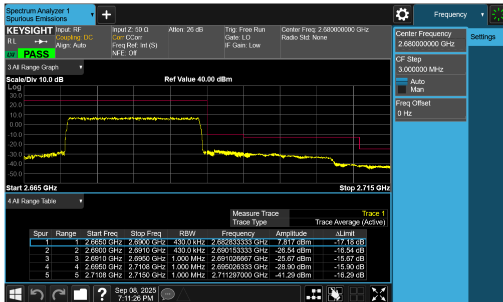
Plot 7-136. Upper ACP Plot (LTE Band 41(PC2) - 20MHz QPSK – Full RB - Ant1)
