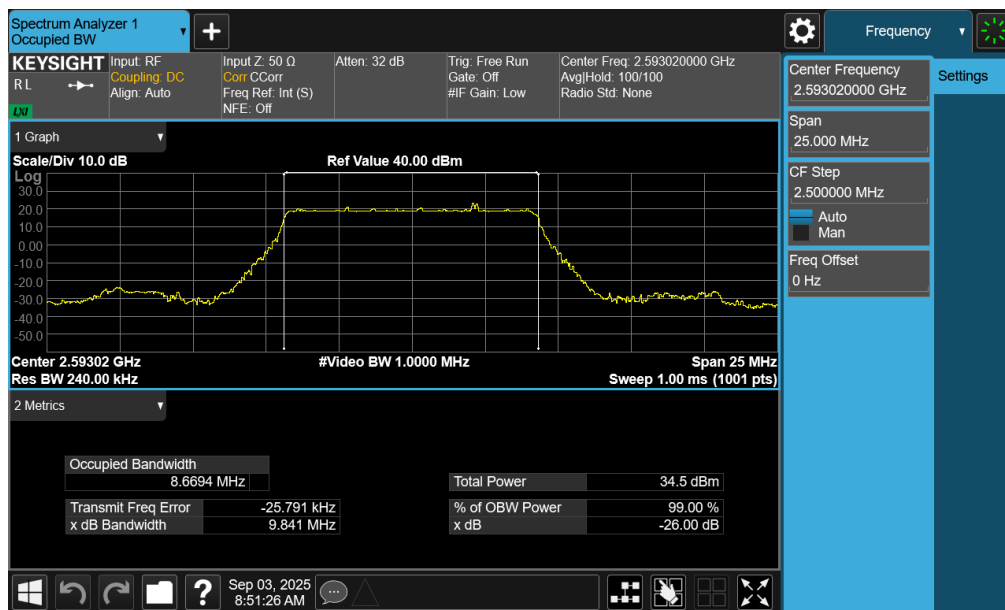
Plot 7-98. Occupied Bandwidth Plot (NR Band n41 PC2 – 10MHz \pi/2 BPSK – Full RB – Switch – Ant1)
