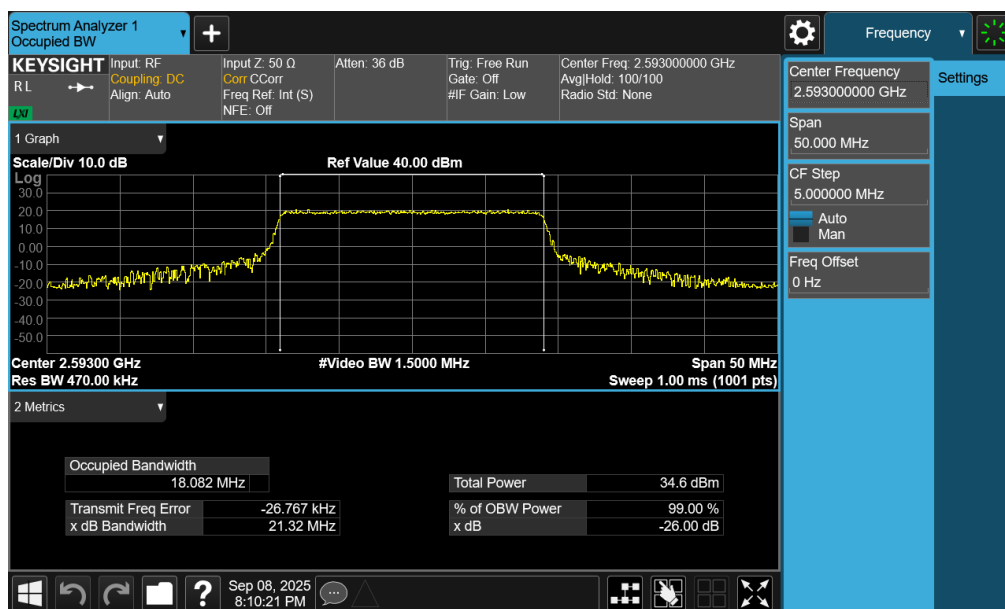
Plot 7-101. Occupied Bandwidth Plot (LTE Band 41PC2 - 20MHz QPSK - Full RB - Ant2)
