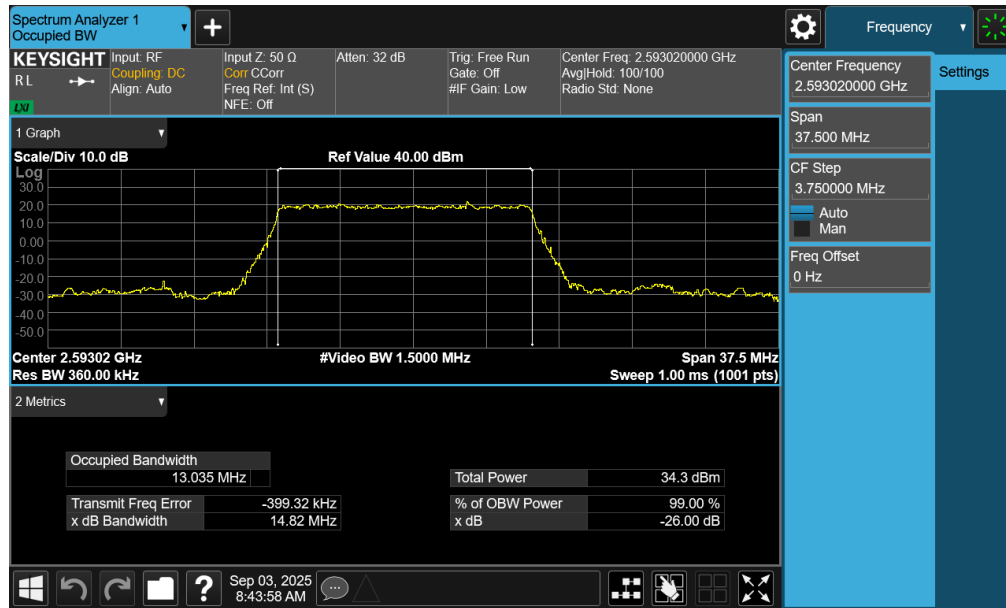
Plot 7-95. Occupied Bandwidth Plot (NR Band n41 PC2 – 15MHz \pi/2 BPSK – Full RB – Switch – Ant1)
