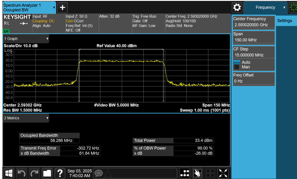
Plot 7-73. Occupied Bandwidth Plot (NR Band n41 PC2 – 60MHz 16-QAM – Full RB – Switch – Ant1)
