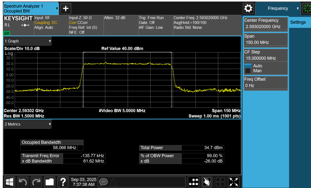
Plot 7-71. Occupied Bandwidth Plot (NR Band n41 PC2 – 60MHz \pi/2 BPSK – Full RB – Switch – Ant1)
