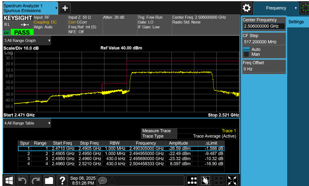
Plot 7-143. Lower ACP Plot (LTE Band 41(PC2) - 20MHz QPSK – Full RB - Ant2)
