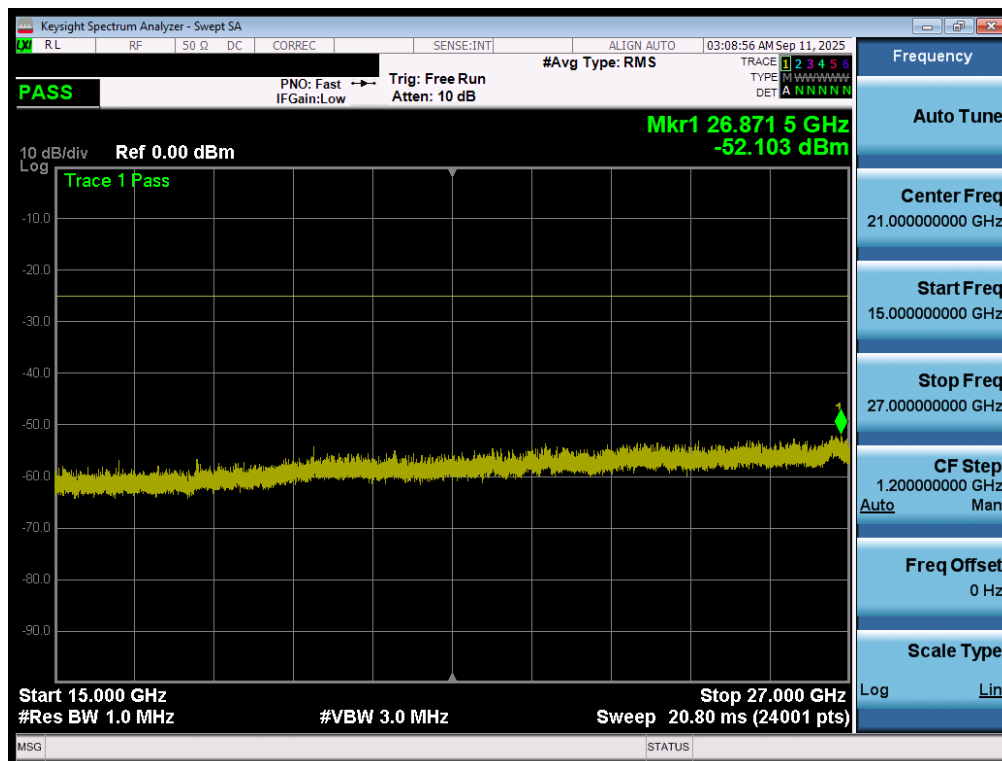
Plot 7-122. Conducted Spurious Plot (LTE Band 41(PC3)- 20MHz QPSK - RB Size 1, RB Offset 0 - High Channel - Ant1)
