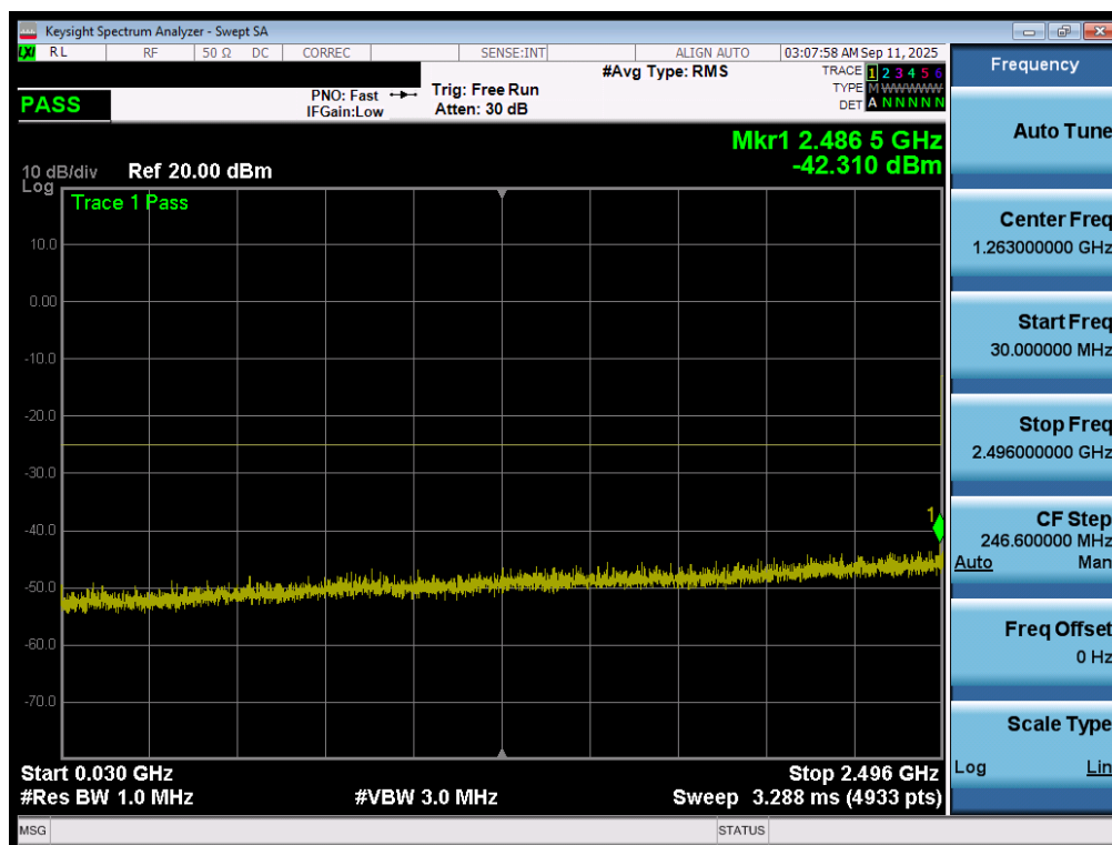
Plot 7-120. Conducted Spurious Plot (LTE Band 41(PC3)- 20MHz QPSK - RB Size 1, RB Offset 0 - High Channel - Ant1)
