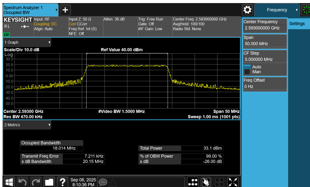
Plot 7-102. Occupied Bandwidth Plot (LTE Band 41PC2 - 20MHz 16-QAM - Full RB - Ant2)
