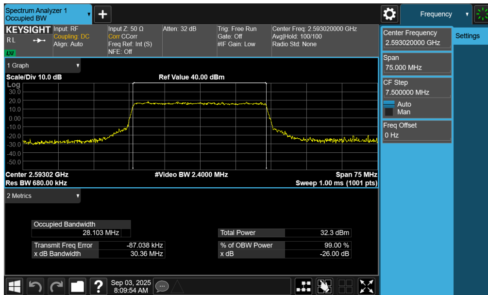
Plot 7-88. Occupied Bandwidth Plot (NR Band n41 PC2 – 30MHz 16-QAM – Full RB – Switch – Ant1)
