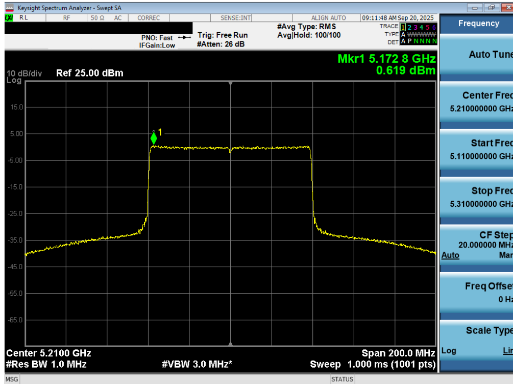
Plot 7-97. Power Spectral Density Plot MIMO ANT2 (80MHz BW 802.11be (UNII Band 1) – Ch. 42)
