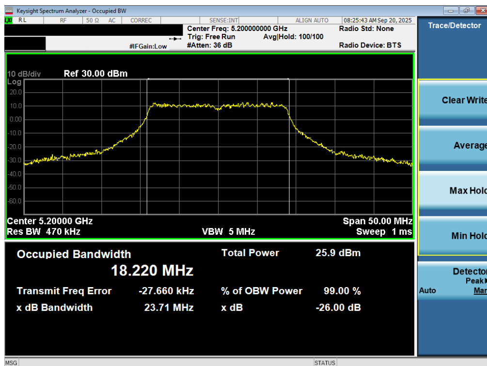
Plot 7-13. 26dB Bandwidth Plot MIMO ANT2 (20MHz BW 802.11n (UNII Band 1) – Ch. 40)
