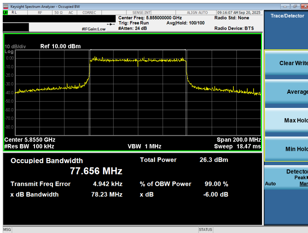
Plot 7-55. 6dB Bandwidth Plot MIMO ANT2 (80MHz BW 802.11be (UNII Band 3/4) – Ch. 171)
