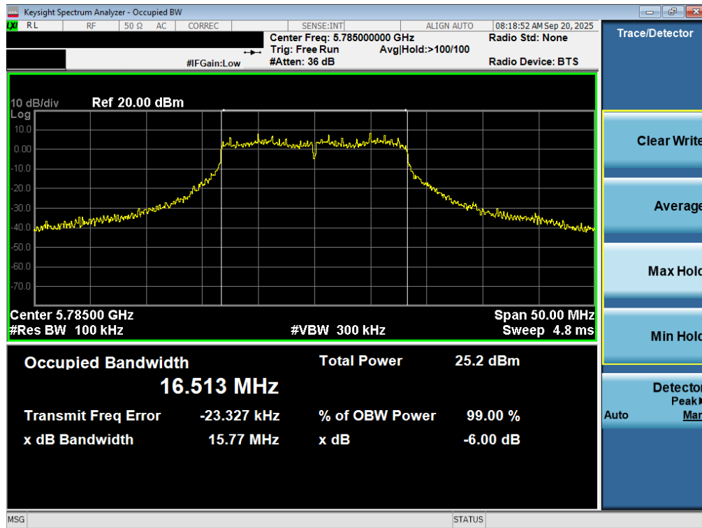
Plot 7-42. 6dB Bandwidth Plot MIMO ANT2 (802.11a (UNII Band 3) – Ch. 157)
