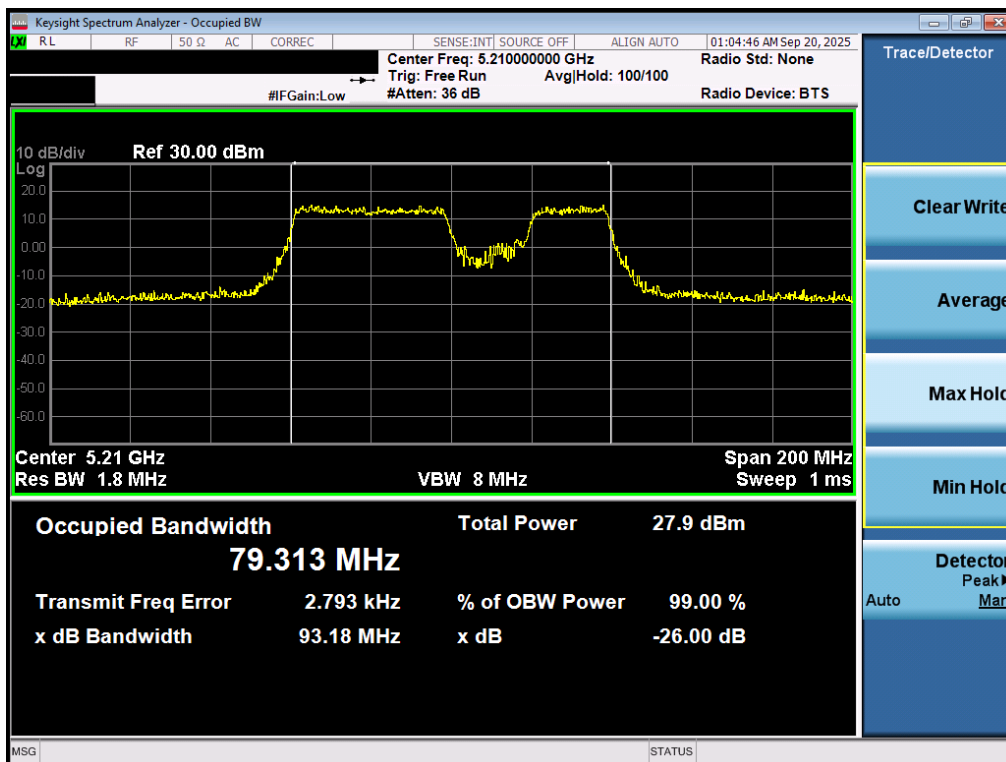
Plot 7-10. 26dB Bandwidth Plot MIMO ANT1 (80MHz BW 802.11be – 20MHz Puncture (UNII Band 1) – Ch. 42)
