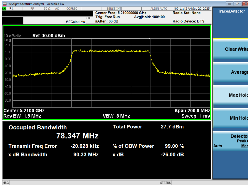
Plot 7-18. 26dB Bandwidth Plot MIMO ANT2 (80MHz BW 802.11be (UNII Band 1) – Ch. 42)
