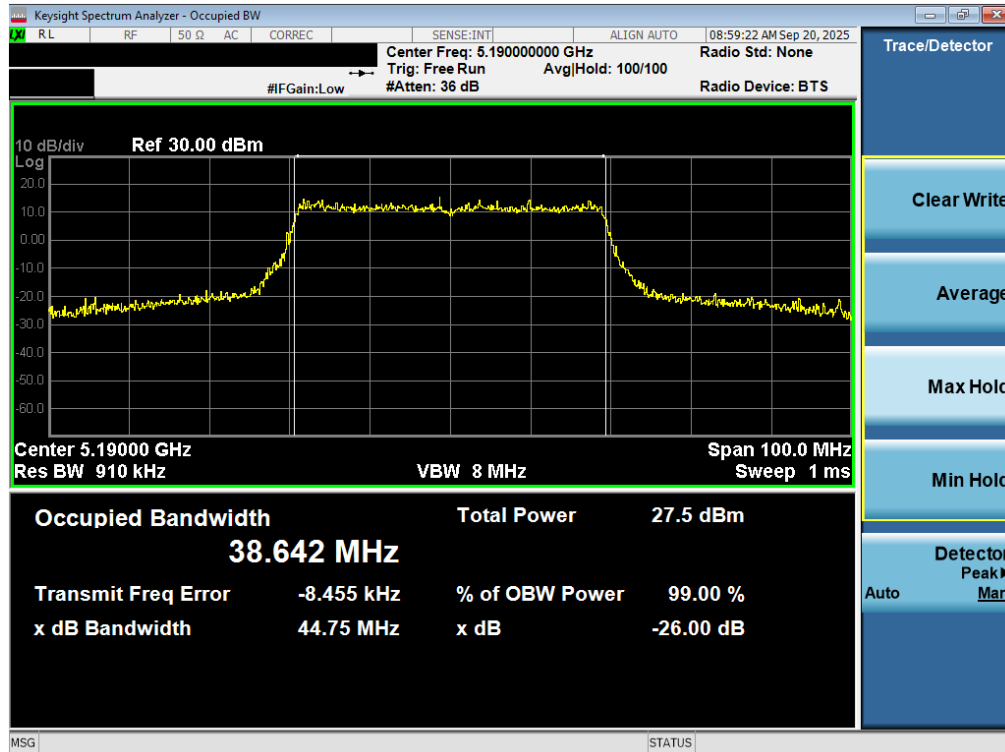
Plot 7-16. 26dB Bandwidth Plot MIMO ANT2 (40MHz BW 802.11be (UNII Band 1) – Ch. 38)
