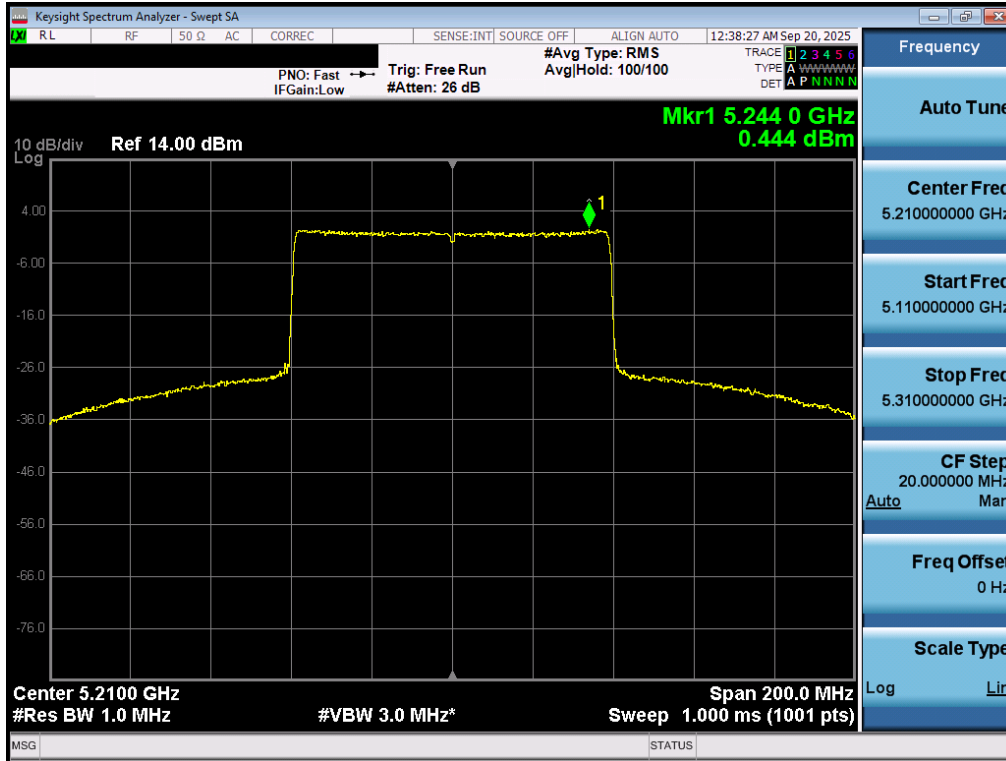
Plot 7-67. Power Spectral Density Plot MIMO ANT1 (80MHz BW 802.11be (UNII Band 1) – Ch. 42)
