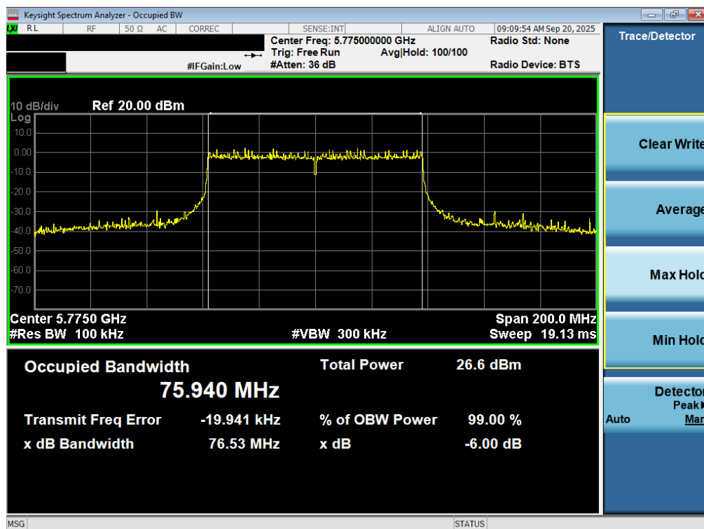
Plot 7-47. 6dB Bandwidth Plot MIMO ANT2 (80MHz BW 802.11ac (UNII Band 3) – Ch. 155)
