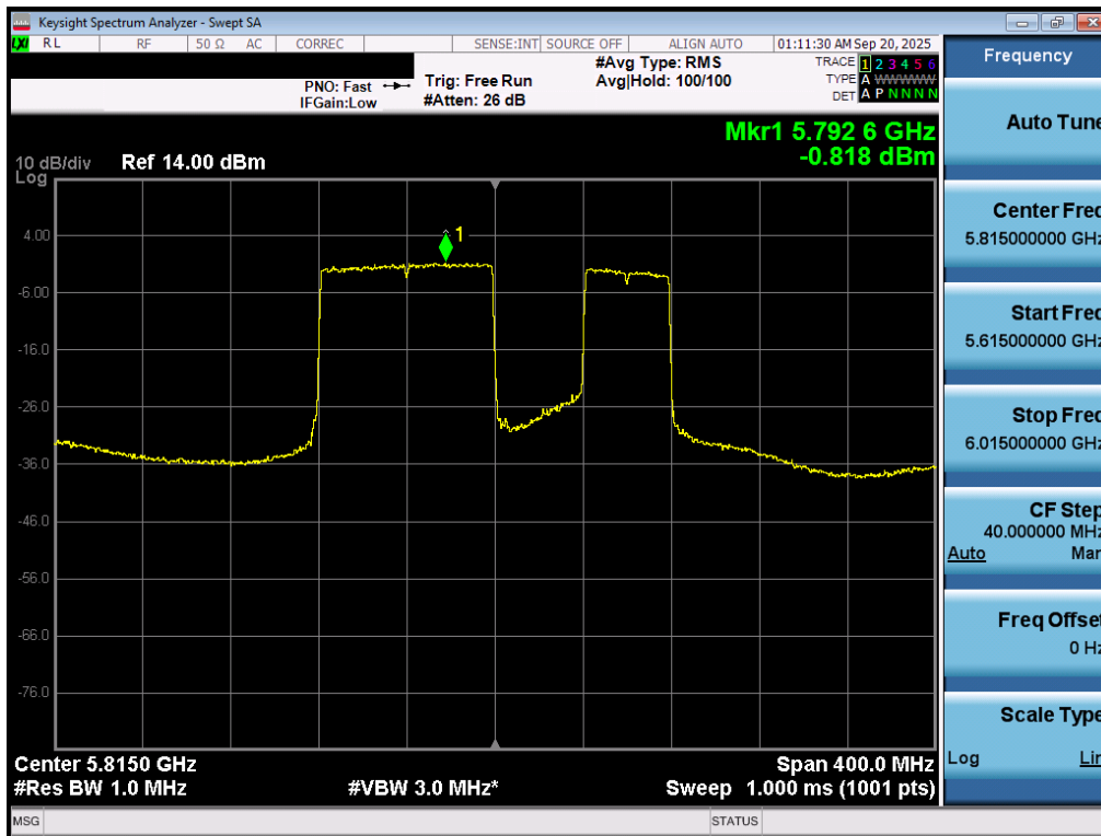
Plot 7-90. Power Spectral Density Plot MIMO ANT1 (160MHz BW 802.11be – 40MHz Puncture (UNII Band 3/4) – Ch. 163)
