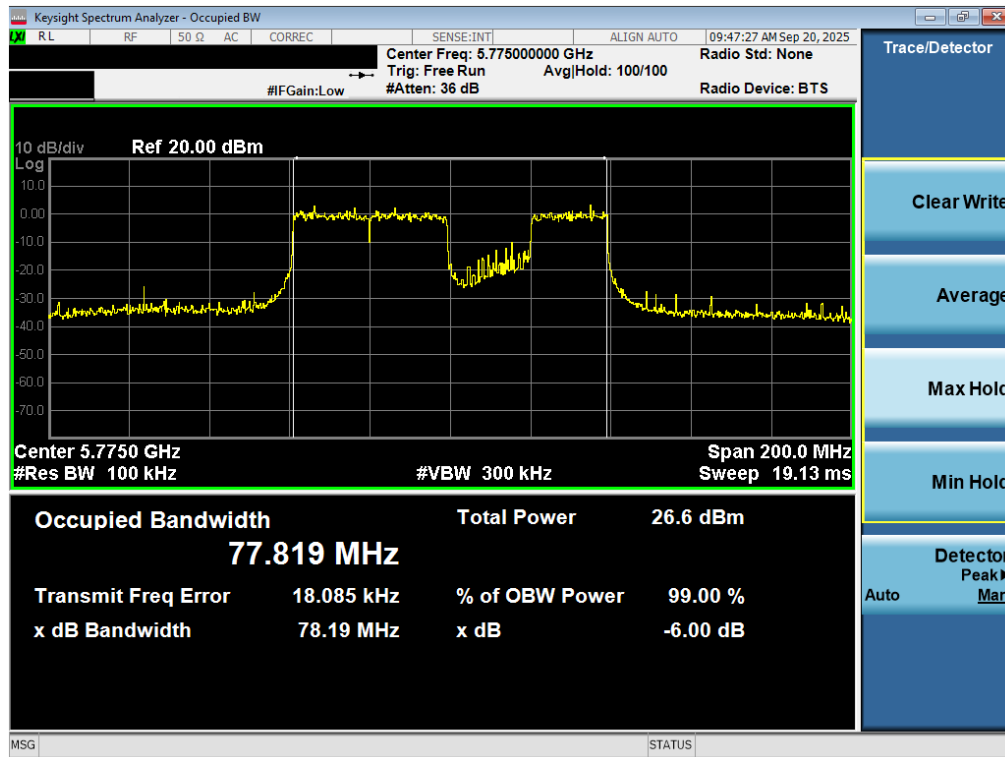
Plot 7-58. 6dB Bandwidth Plot MIMO ANT2 (80MHz BW 802.11be – 20MHz Puncture (UNII Band 3) – Ch. 155)
