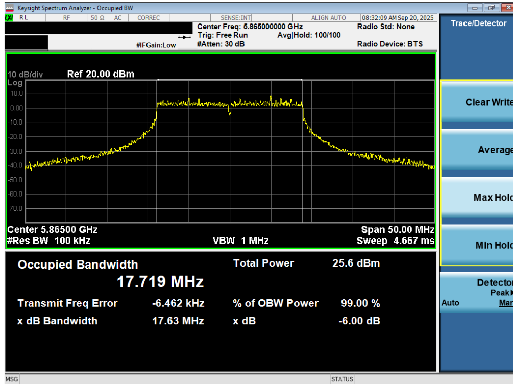
Plot 7-50. 6dB Bandwidth Plot MIMO ANT2 (20MHz BW 802.11n (UNII Band 3/4) – Ch. 173)
