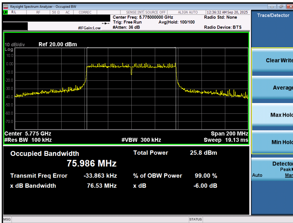
Plot 7-28. 6dB Bandwidth Plot MIMO ANT1 (80MHz BW 802.11ac (UNII Band 3) – Ch. 155)
