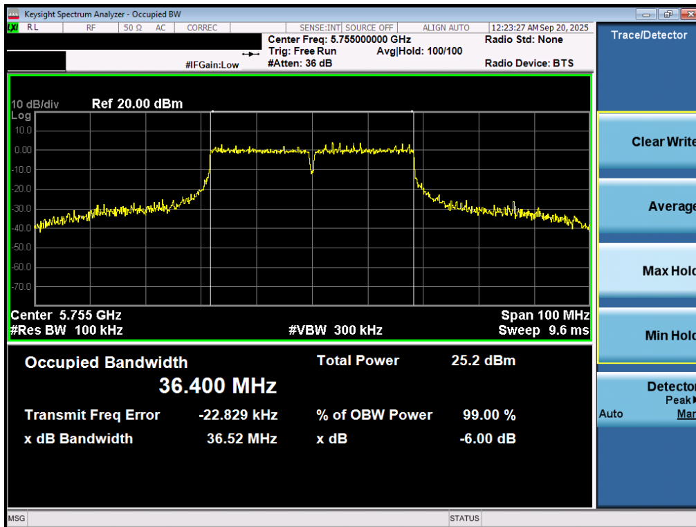
Plot 7-26. 6dB Bandwidth Plot MIMO ANT1 (40MHz BW 802.11n (UNII Band 3) – Ch. 151)
