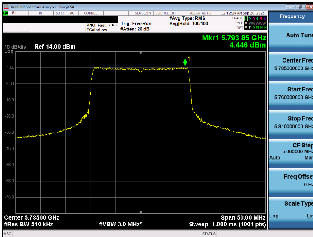
Plot 7-74. Power Spectral Density Plot MIMO ANT1 (20MHz BW 802.11be (UNII Band 3) – Ch. 157)
