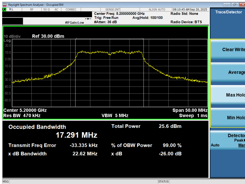
Plot 7-12. 26dB Bandwidth Plot MIMO ANT2 (802.11a (UNII Band 1) – Ch. 40)
