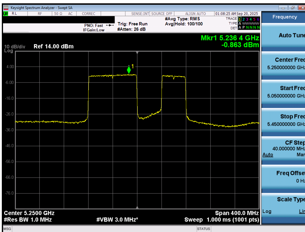
Plot 7-101. Power Spectral Density Plot MIMO ANT2 (160MHz BW 802.11be – 40MHz Puncture (UNII Band 1/2A) – Ch. 50)
