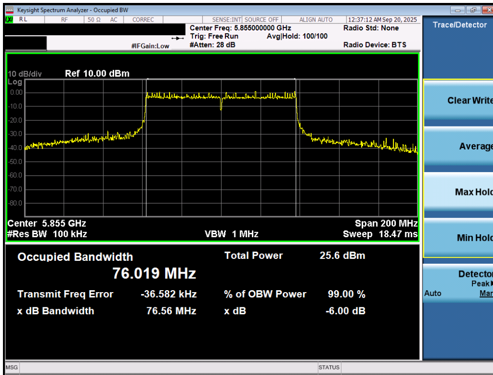
Plot 7-35. 6dB Bandwidth Plot MIMO ANT1 (80MHz BW 802.11ac (UNII Band 3/4) – Ch. 171)
