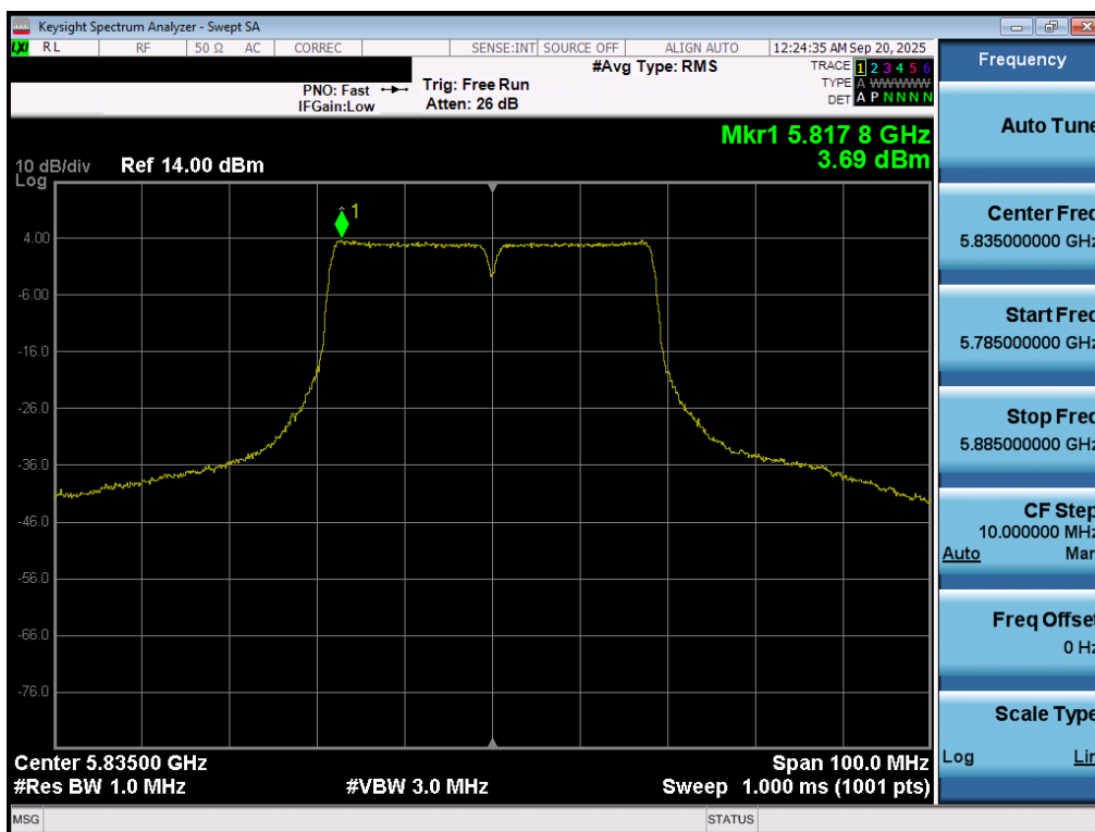
Plot 7-83. Power Spectral Density Plot MIMO ANT1 (40MHz BW 802.11n (UNII Band 3/4) – Ch. 167)
