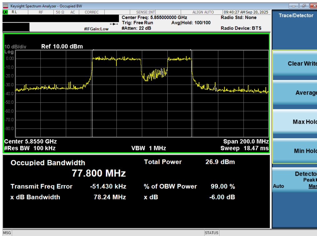
Plot 7-59. 6dB Bandwidth Plot MIMO ANT2 (80MHz BW 802.11be – 20MHz Puncture (UNII Band 3/4) – Ch. 171)
