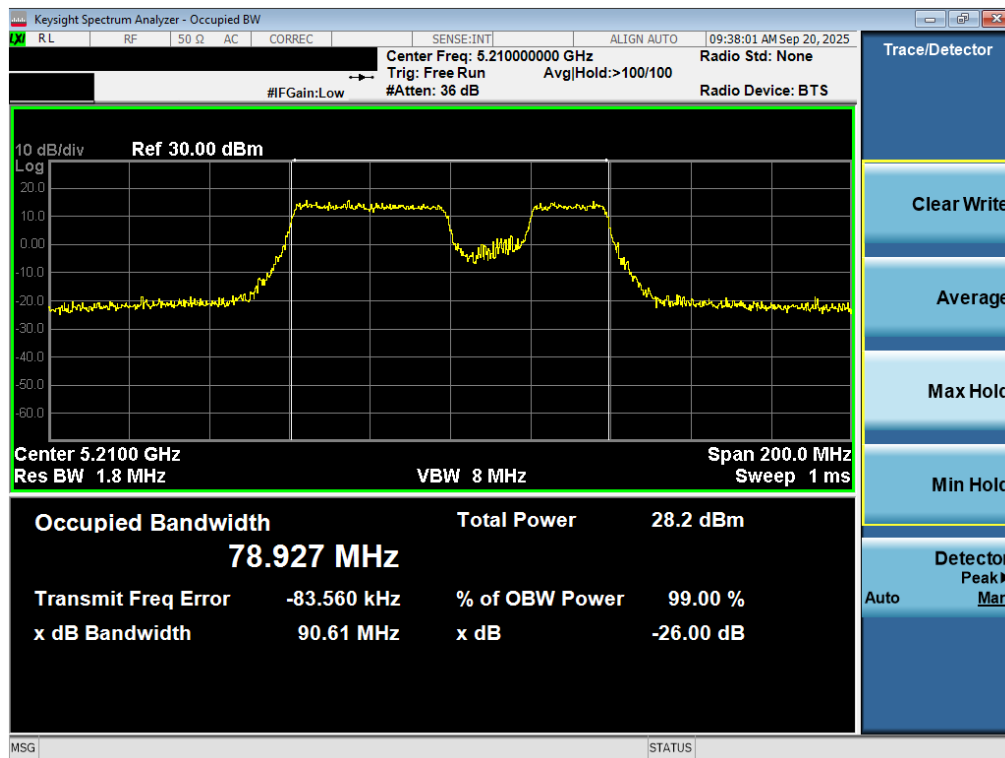
Plot 7-21. 26dB Bandwidth Plot MIMO ANT2 (80MHz BW 802.11be – 20MHz Puncture (UNII Band 1) – Ch. 42)
