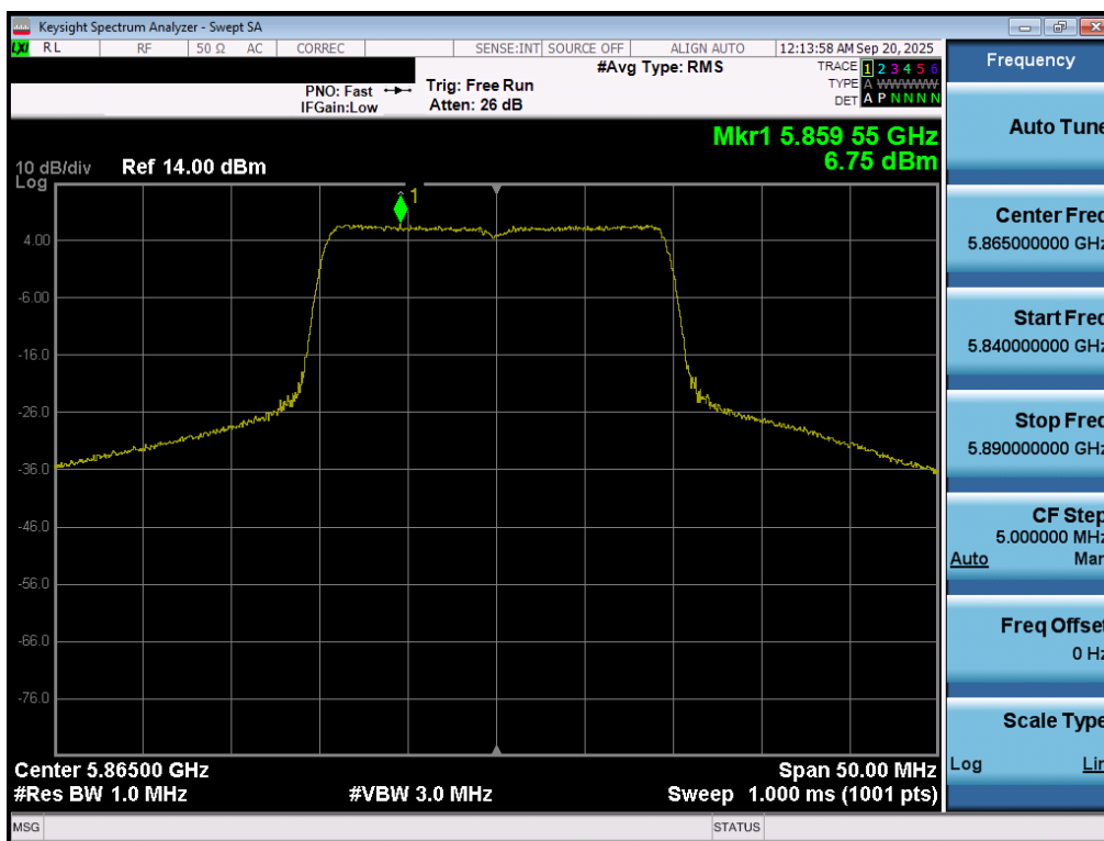
Plot 7-82. Power Spectral Density Plot MIMO ANT1 (20MHz BW 802.11be (UNII Band 4) – Ch. 173)
