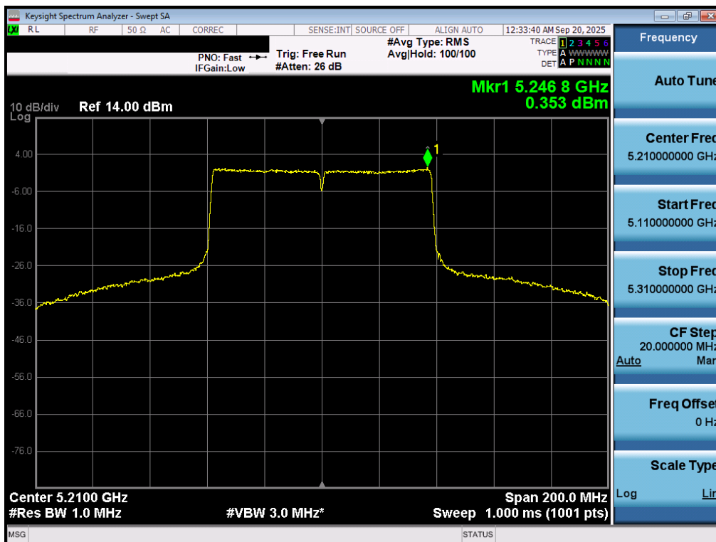
Plot 7-66. Power Spectral Density Plot MIMO ANT1 (80MHz BW 802.11ac (UNII Band 1) – Ch. 42)
