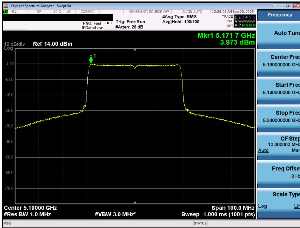
Plot 7-65. Power Spectral Density Plot MIMO ANT1 (40MHz BW 802.11be (UNII Band 1) – Ch. 38)
