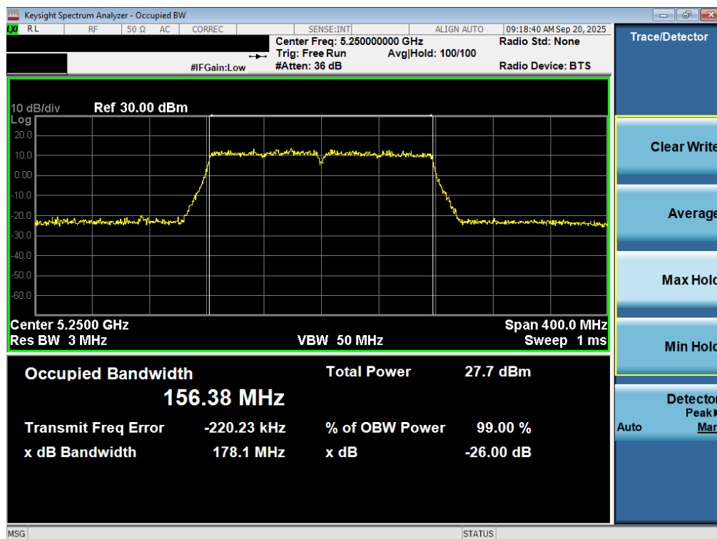
Plot 7-19. 26dB Bandwidth Plot MIMO ANT2 (160MHz BW 802.11ac (UNII Band 1/2A) – Ch. 50)
