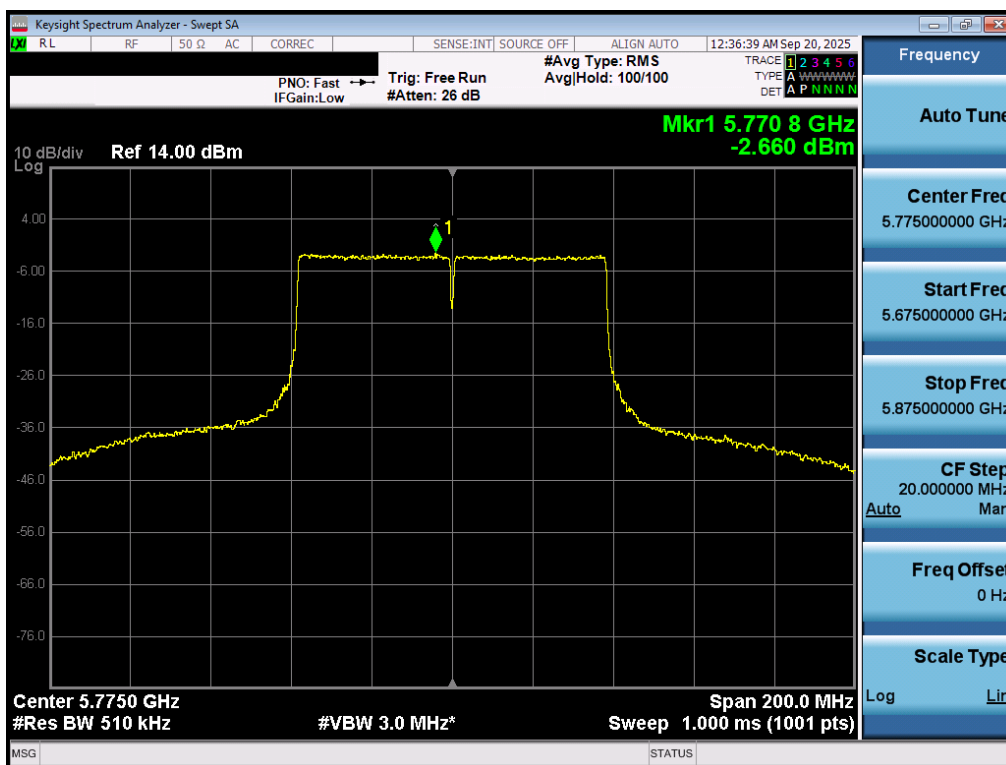
Plot 7-77. Power Spectral Density Plot MIMO ANT1 (80MHz BW 802.11ac (UNII Band 3) – Ch. 155)
