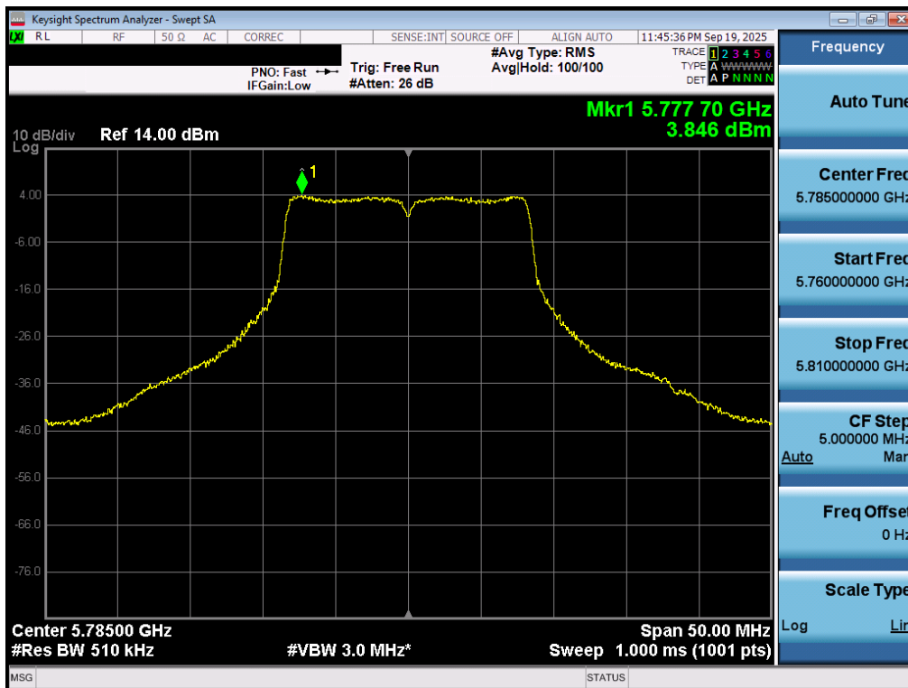
Plot 7-72. Power Spectral Density Plot MIMO ANT1 (802.11a (UNII Band 3) – Ch. 157)
