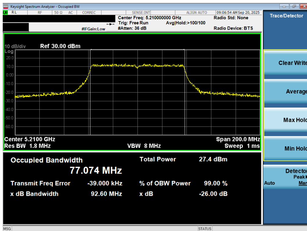
Plot 7-17. 26dB Bandwidth Plot MIMO ANT2 (80MHz BW 802.11ac (UNII Band 1) – Ch. 42)
