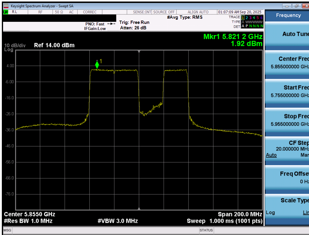
Plot 7-89. Power Spectral Density Plot MIMO ANT1 (80MHz BW 802.11be – 20MHz Puncture (UNII Band 3/4) – Ch. 171)
