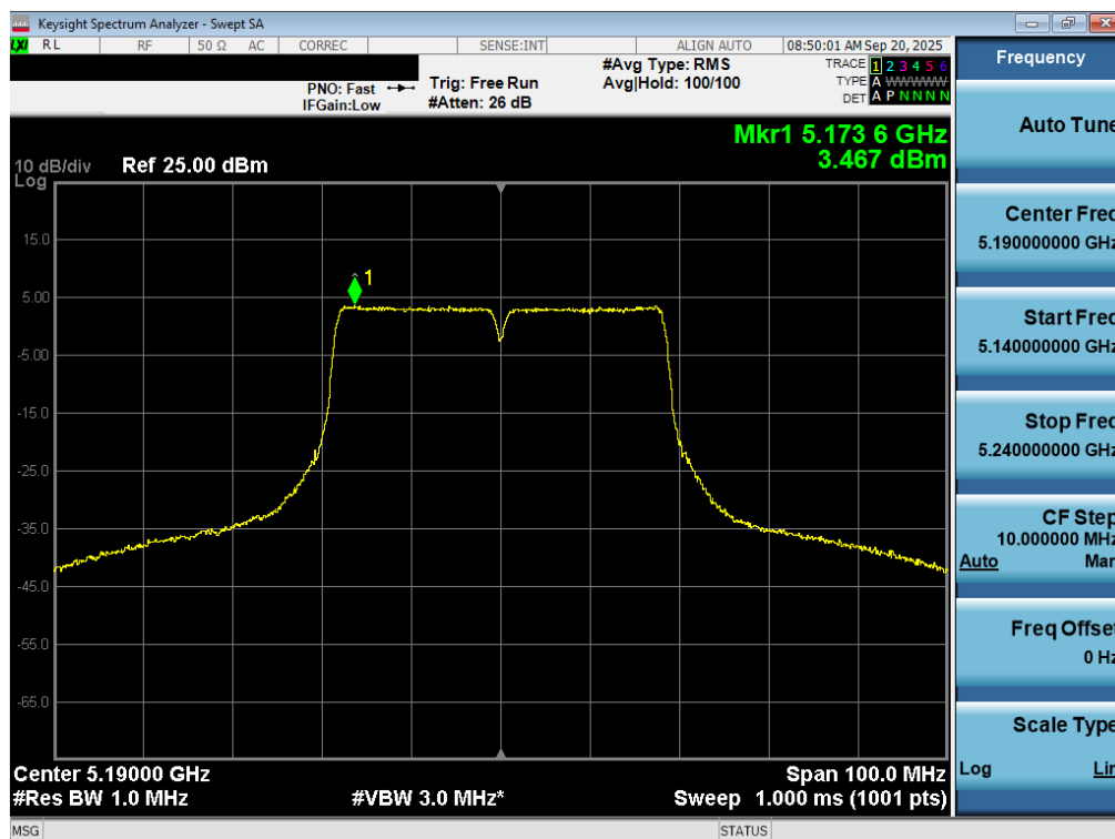
Plot 7-94. Power Spectral Density Plot MIMO ANT2 (40MHz BW 802.11n (UNII Band 1) – Ch. 38)
