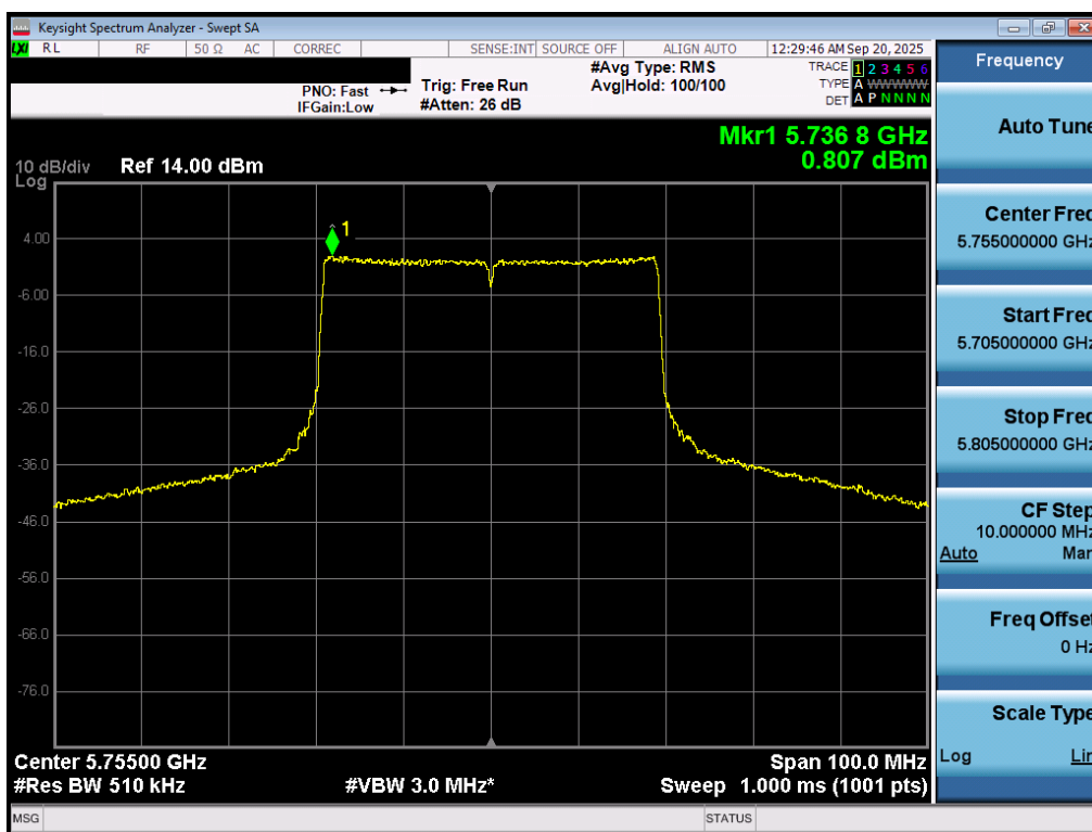
Plot 7-76. Power Spectral Density Plot MIMO ANT1 (40MHz BW 802.11be (UNII Band 3) – Ch. 151)
