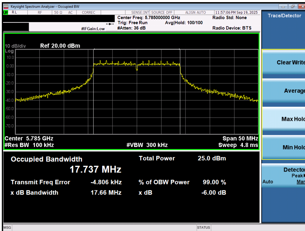
Plot 7-24. 6dB Bandwidth Plot MIMO ANT1 (20MHz BW 802.11n (UNII Band 3) – Ch. 157)
