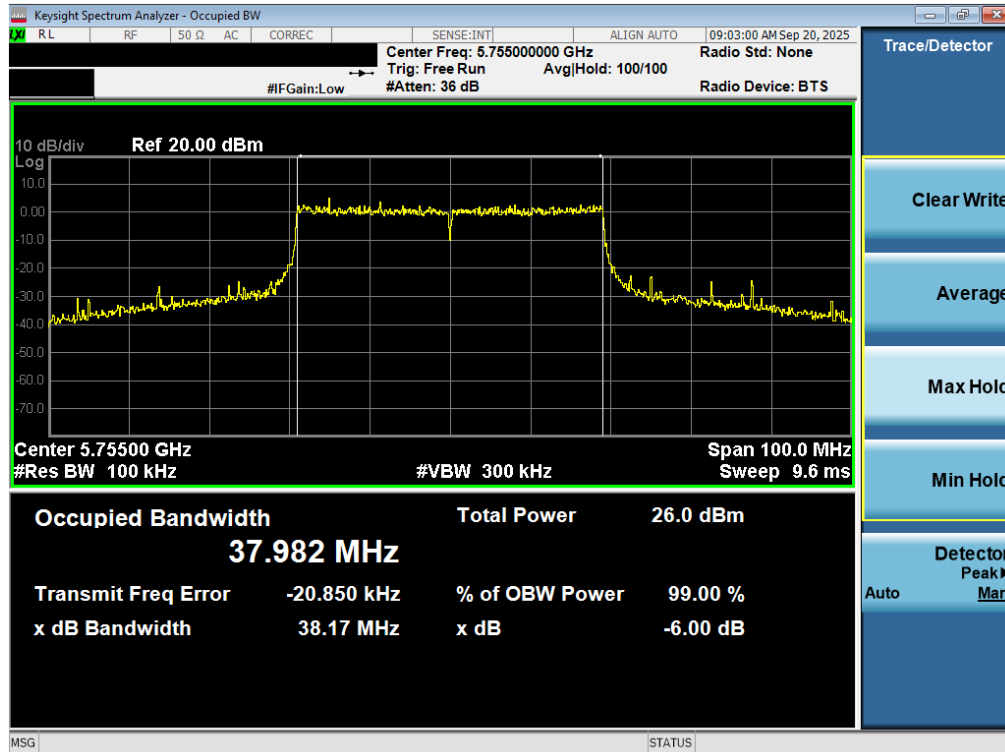
Plot 7-46. 6dB Bandwidth Plot MIMO ANT2 (40MHz BW 802.11be (UNII Band 3) – Ch. 151)
