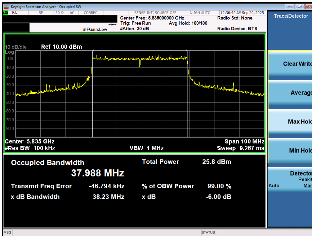
Plot 7-34. 6dB Bandwidth Plot MIMO ANT1 (40MHz BW 802.11be (UNII Band 3/4) – Ch. 167)
