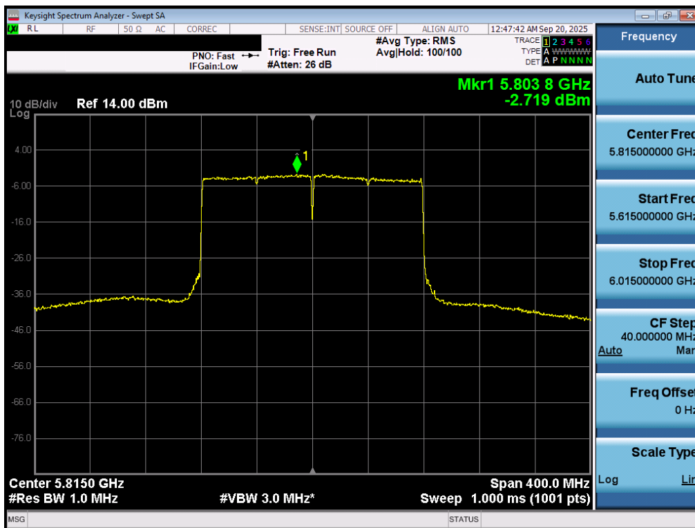
Plot 7-88. Power Spectral Density Plot MIMO ANT1 (160MHz BW 802.11be (UNII Band 3/4) – Ch. 163)
