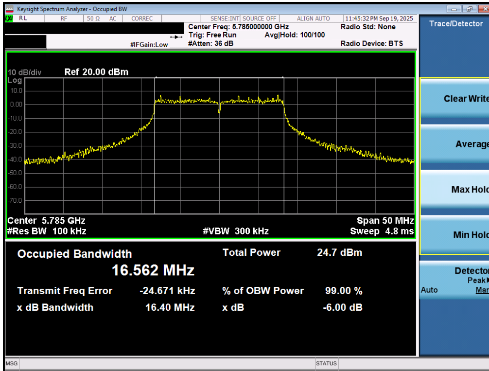
Plot 7-23. 6dB Bandwidth Plot MIMO ANT1 (802.11a (UNII Band 3) – Ch. 157)
