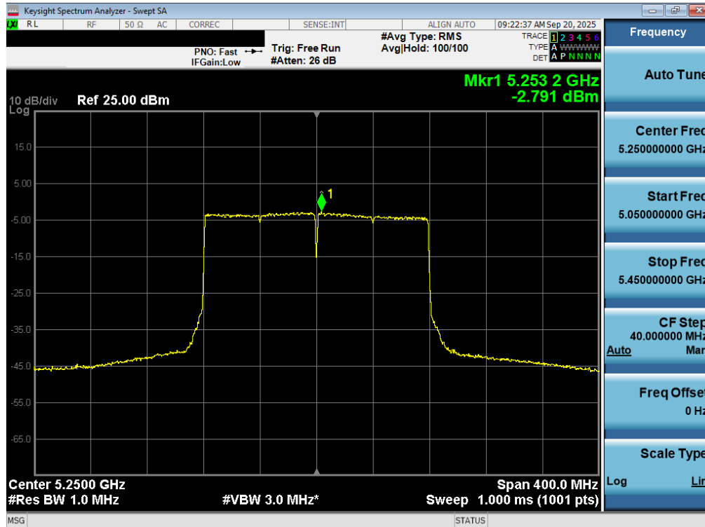
Plot 7-99. Power Spectral Density Plot MIMO ANT2 (160MHz BW 802.11be (UNII Band 1/2A) – Ch. 50)
