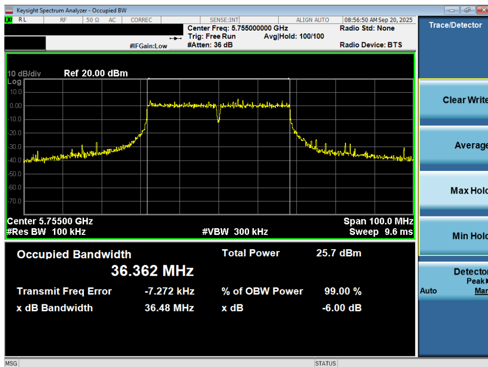
Plot 7-45. 6dB Bandwidth Plot MIMO ANT2 (40MHz BW 802.11n (UNII Band 3) – Ch. 151)
