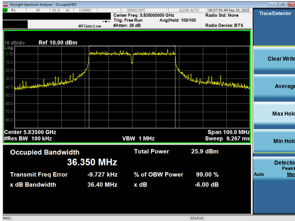
Plot 7-52. 6dB Bandwidth Plot MIMO ANT2 (40MHz BW 802.11n (UNII Band 3/4) – Ch. 167)
