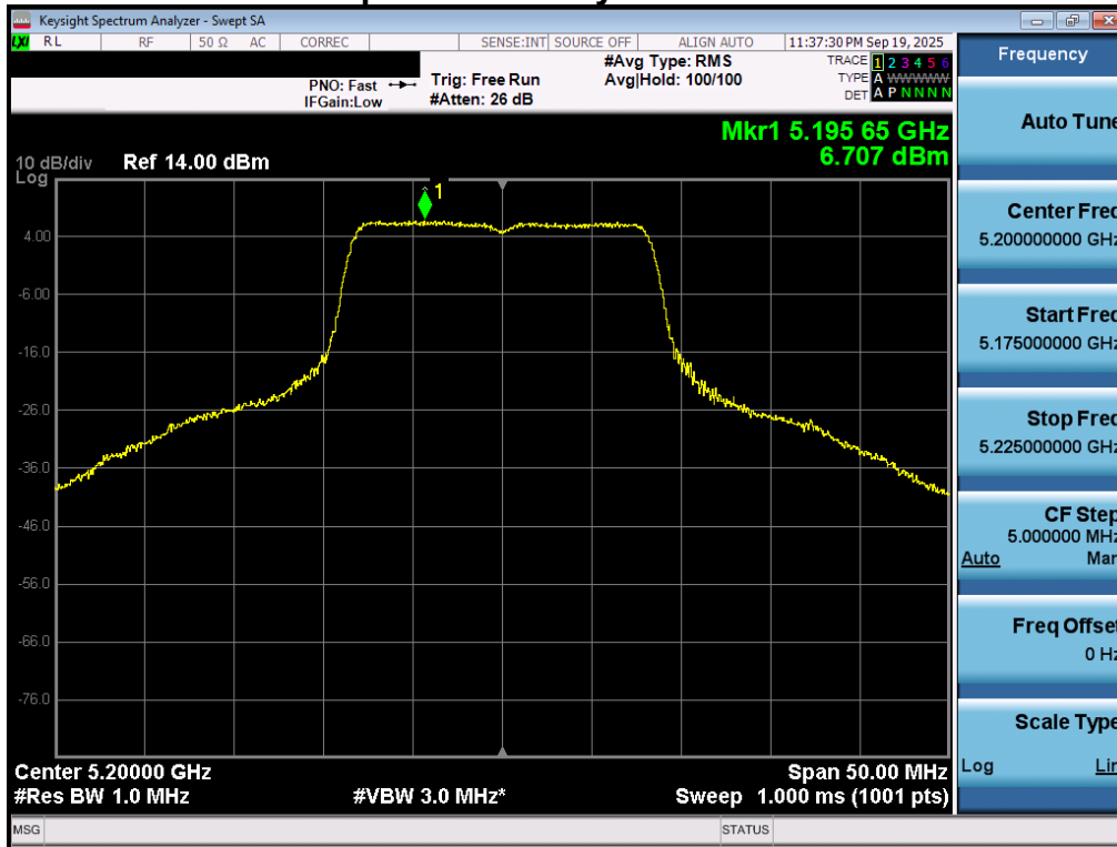
Plot 7-61. Power Spectral Density Plot MIMO ANT1 (802.11a (UNII Band 1) – Ch. 40)
