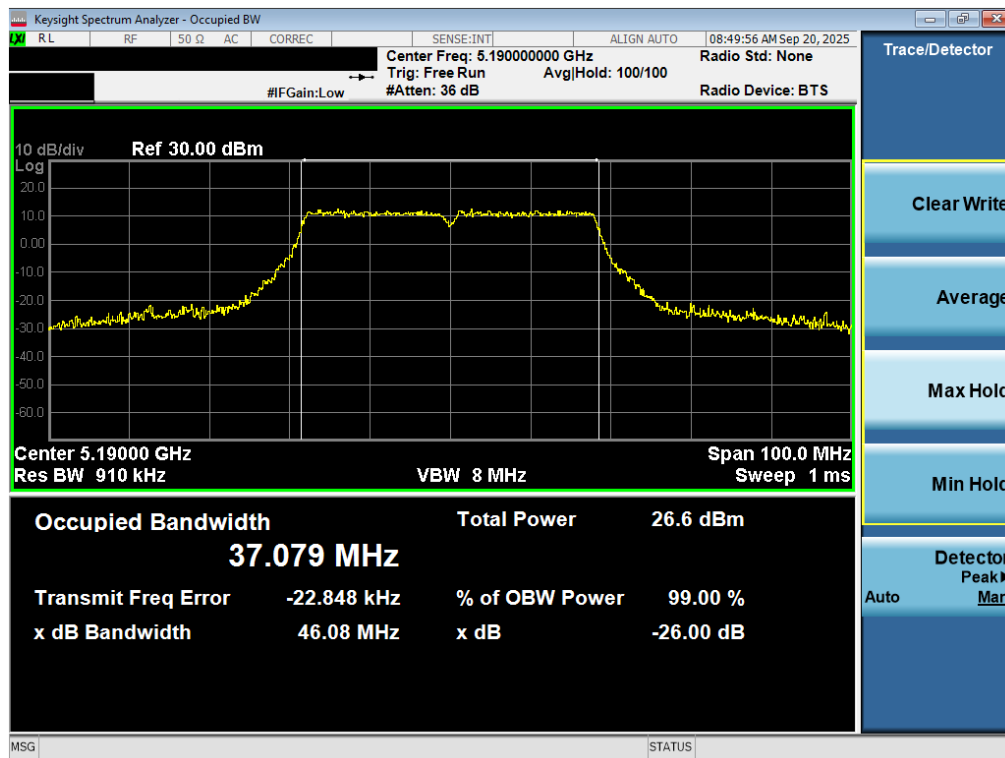
Plot 7-15. 26dB Bandwidth Plot MIMO ANT2 (40MHz BW 802.11n (UNII Band 1) – Ch. 38)
