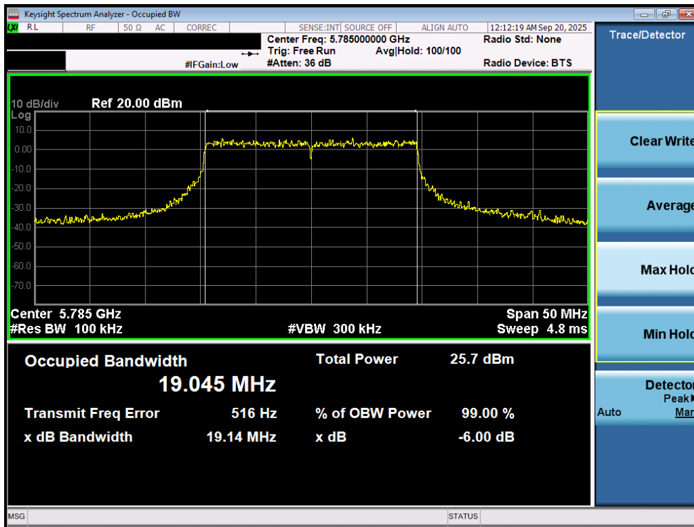
Plot 7-25. 6dB Bandwidth Plot MIMO ANT1 (20MHz BW 802.11be (UNII Band 3) – Ch. 157)
