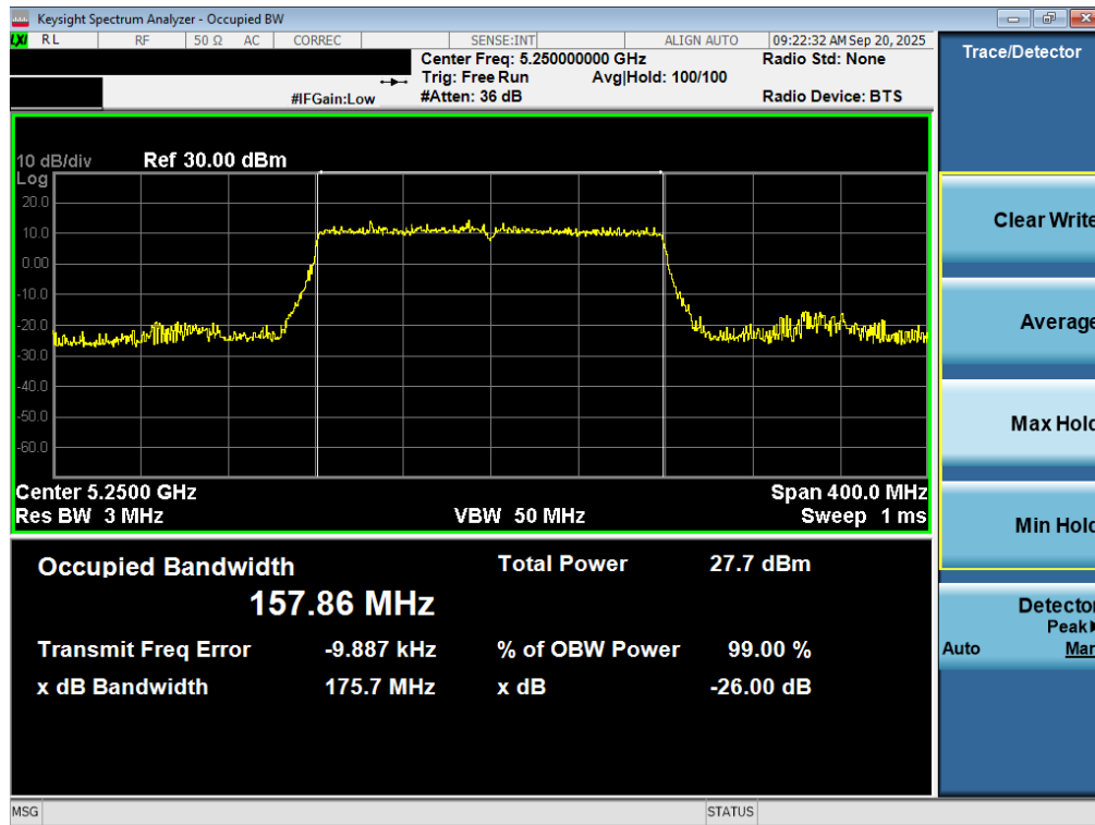
Plot 7-20. 26dB Bandwidth Plot MIMO ANT2 (160MHz BW 802.11be (UNII Band 1/2A) – Ch. 50)
