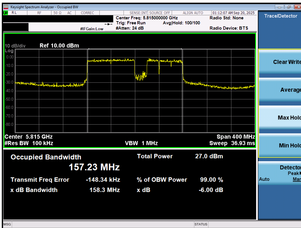
Plot 7-41. 6dB Bandwidth Plot MIMO ANT1 (160MHz BW 802.11be – 20MHz Puncture (UNII Band 3/4) – Ch. 163)
