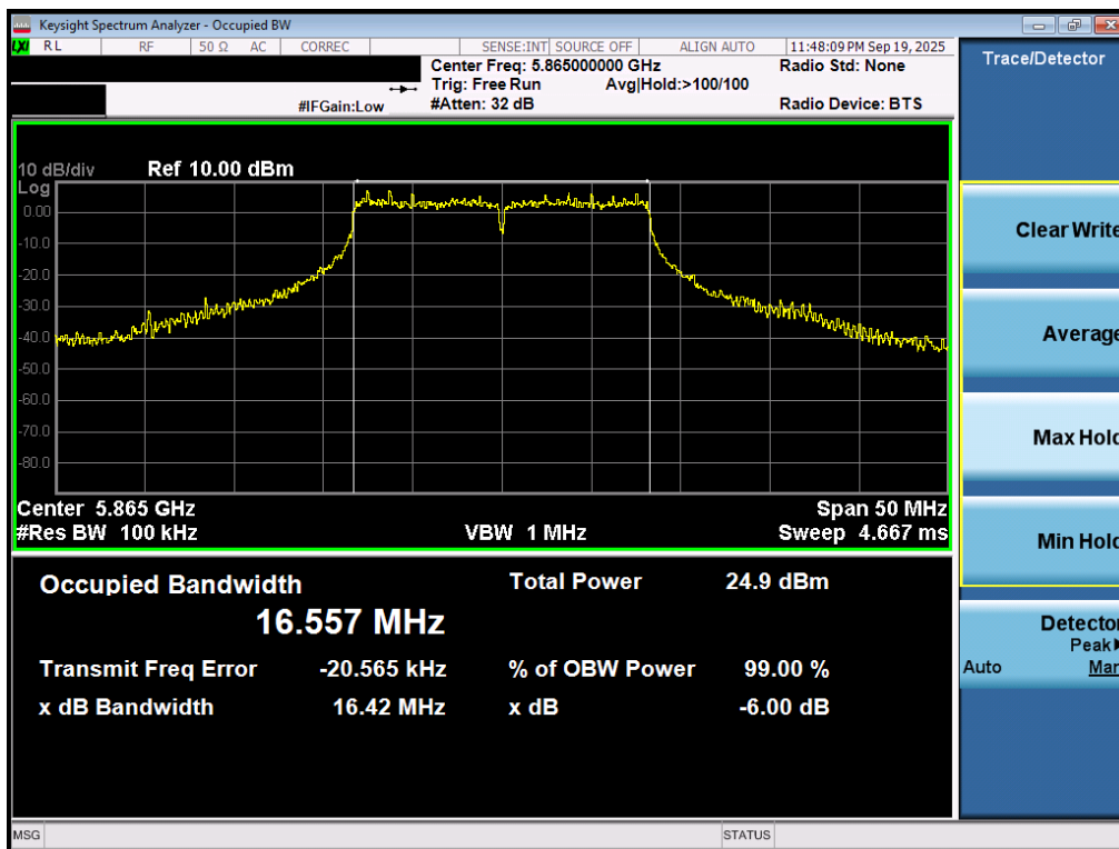
Plot 7-30. 6dB Bandwidth Plot MIMO ANT1 (802.11a (UNII Band 4) – Ch. 173)
