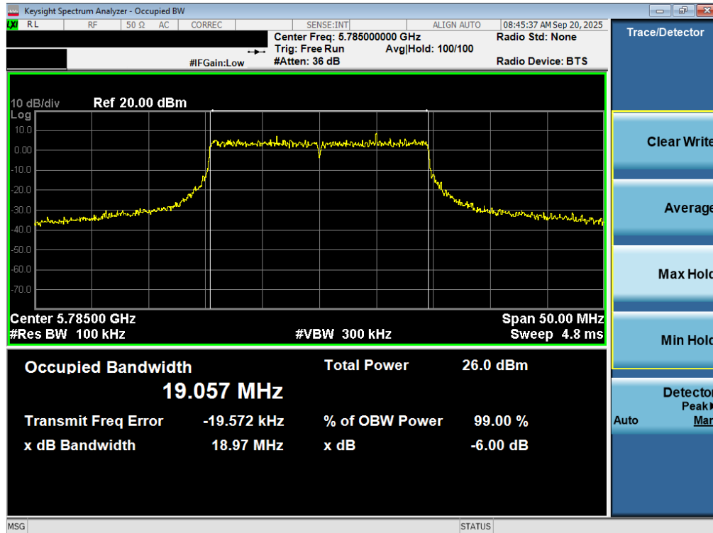
Plot 7-44. 6dB Bandwidth Plot MIMO ANT2 (20MHz BW 802.11be (UNII Band 3) – Ch. 157)
