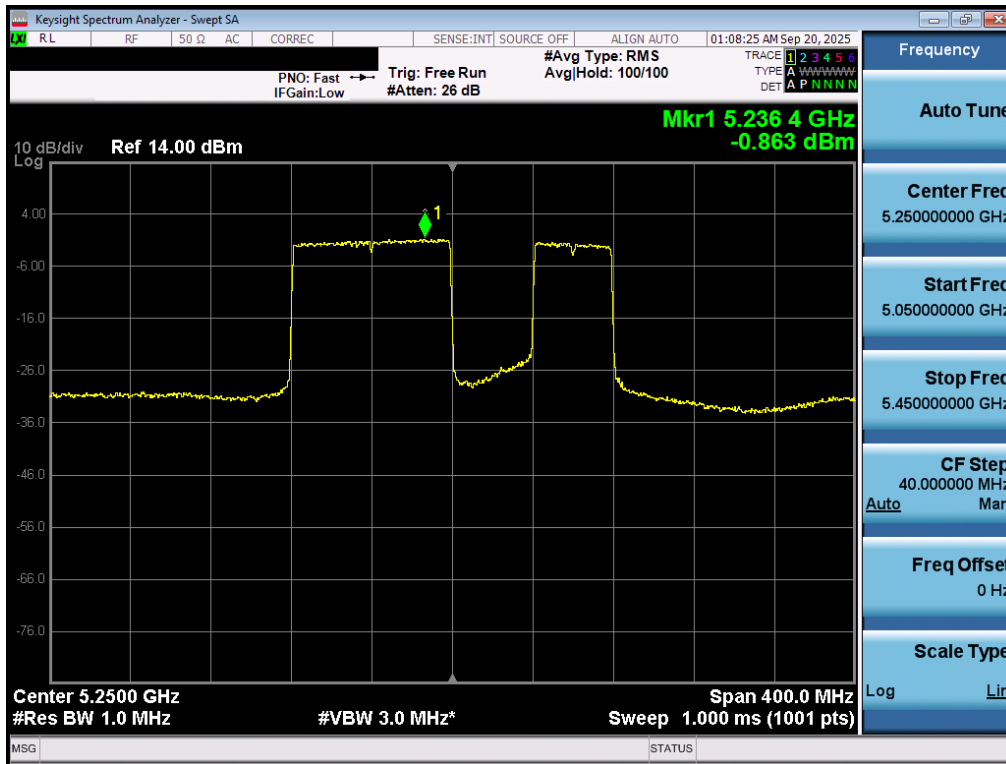
Plot 7-71. Power Spectral Density Plot MIMO ANT1 (160MHz BW 802.11be – 40MHz Puncture (UNII Band 1/2A) – Ch. 50)
