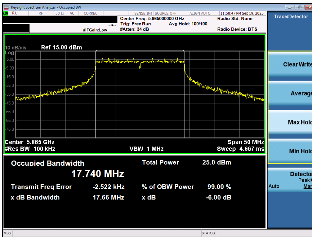
Plot 7-31. 6dB Bandwidth Plot MIMO ANT1 (20MHz BW 802.11n (UNII Band 4) – Ch. 173)
