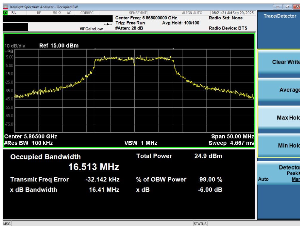
Plot 7-49. 6dB Bandwidth Plot MIMO ANT2 (802.11a (UNII Band 3/4) – Ch. 173)
