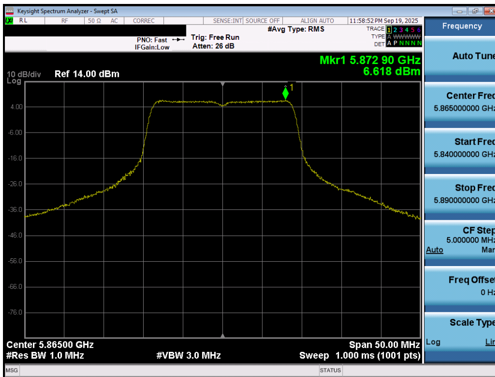
Plot 7-81. Power Spectral Density Plot MIMO ANT1 (20MHz BW 802.11n (UNII Band 4) – Ch. 173)
