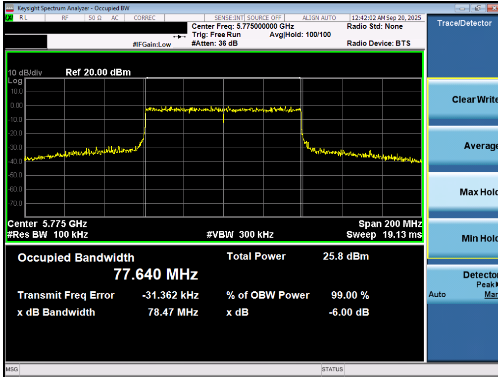
Plot 7-29. 6dB Bandwidth Plot MIMO ANT1 (80MHz BW 802.11be (UNII Band 3) – Ch. 155)
