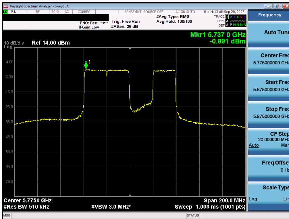
Plot 7-79. Power Spectral Density Plot MIMO ANT1 (80MHz BW 802.11be - 20MHz Puncture (UNII Band 3) - Ch. 155)
