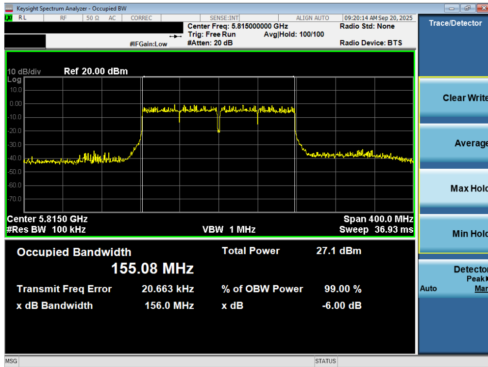
Plot 7-56. 6dB Bandwidth Plot MIMO ANT2 (160MHz BW 802.11ac (UNII Band 3/4) – Ch. 163)
