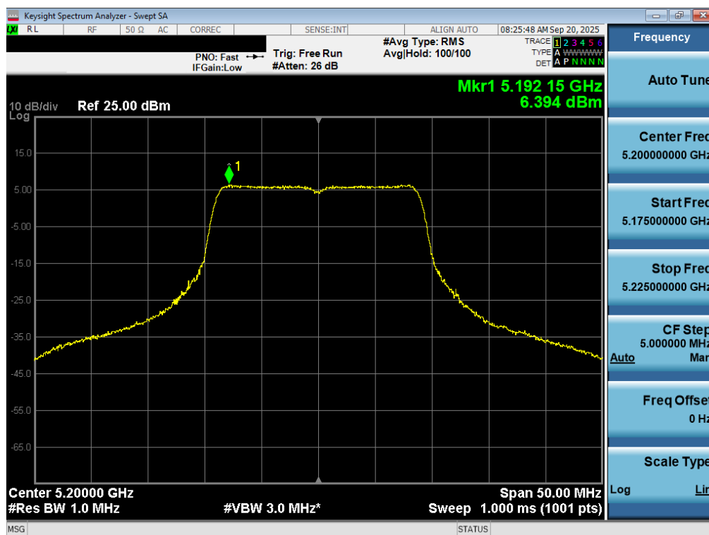
Plot 7-92. Power Spectral Density Plot MIMO ANT2 (20MHz BW 802.11n (UNII Band 1) – Ch. 40)
