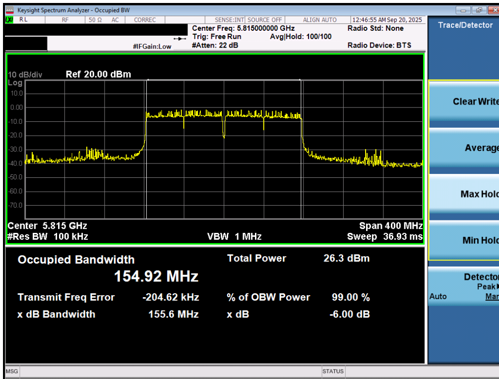
Plot 7-37. 6dB Bandwidth Plot MIMO ANT1 (160MHz BW 802.11ac (UNII Band 3/4) – Ch. 163)
