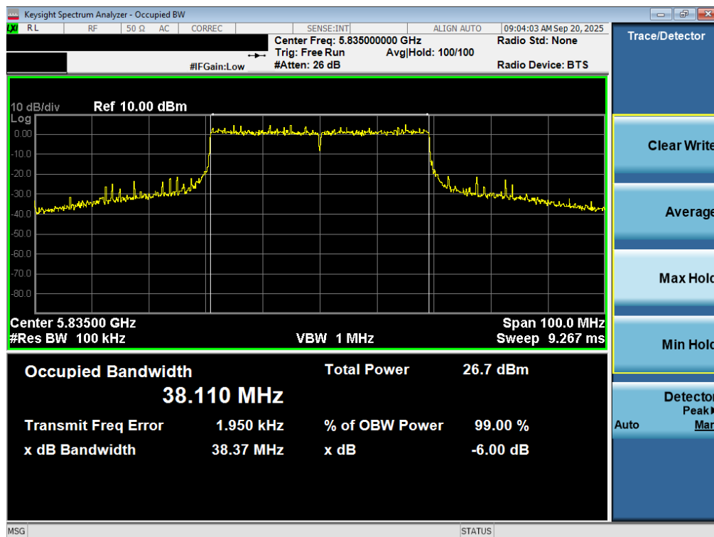
Plot 7-53. 6dB Bandwidth Plot MIMO ANT2 (40MHz BW 802.11be (UNII Band 3/4) – Ch. 167)
