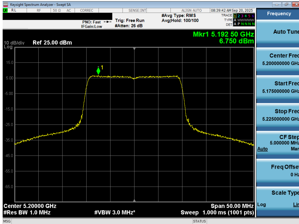
Plot 7-93. Power Spectral Density Plot MIMO ANT2 (20MHz BW 802.11be (UNII Band 1) – Ch. 40)
