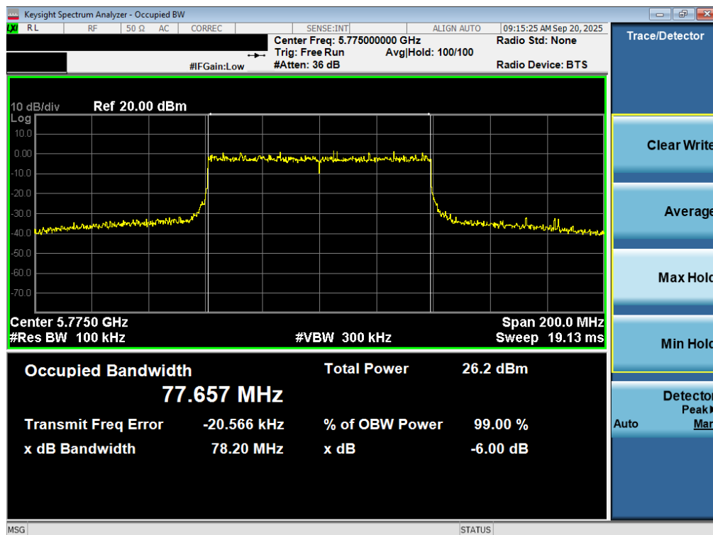
Plot 7-48. 6dB Bandwidth Plot MIMO ANT2 (80MHz BW 802.11be (UNII Band 3) – Ch. 155)
