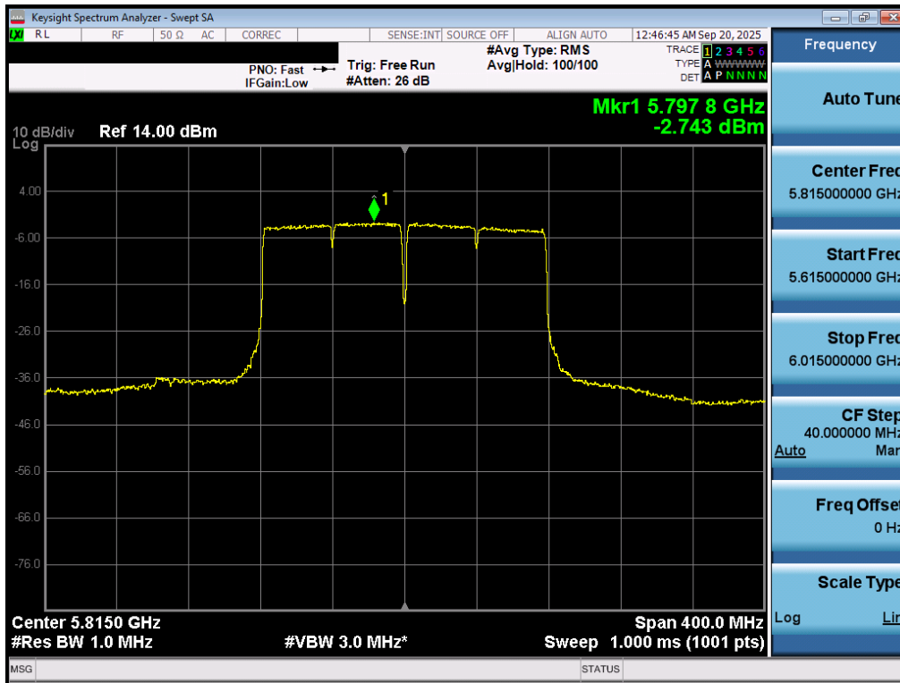
Plot 7-87. Power Spectral Density Plot MIMO ANT1 (160MHz BW 802.11ac (UNII Band 3/4) – Ch. 163)
