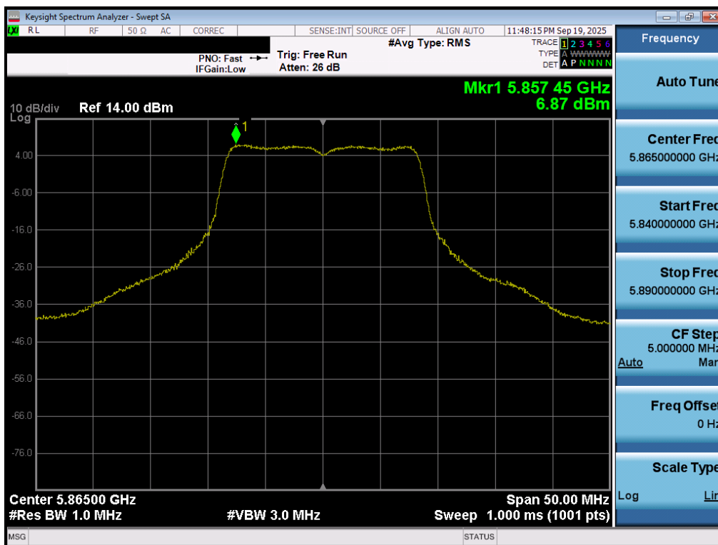
Plot 7-80. Power Spectral Density Plot MIMO ANT1 (802.11a (UNII Band 4) - Ch. 173)
