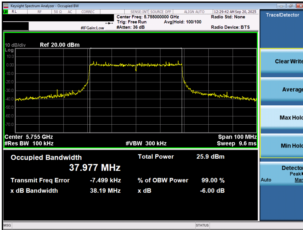
Plot 7-27. 6dB Bandwidth Plot MIMO ANT1 (40MHz BW 802.11be (UNII Band 3) – Ch. 151)
