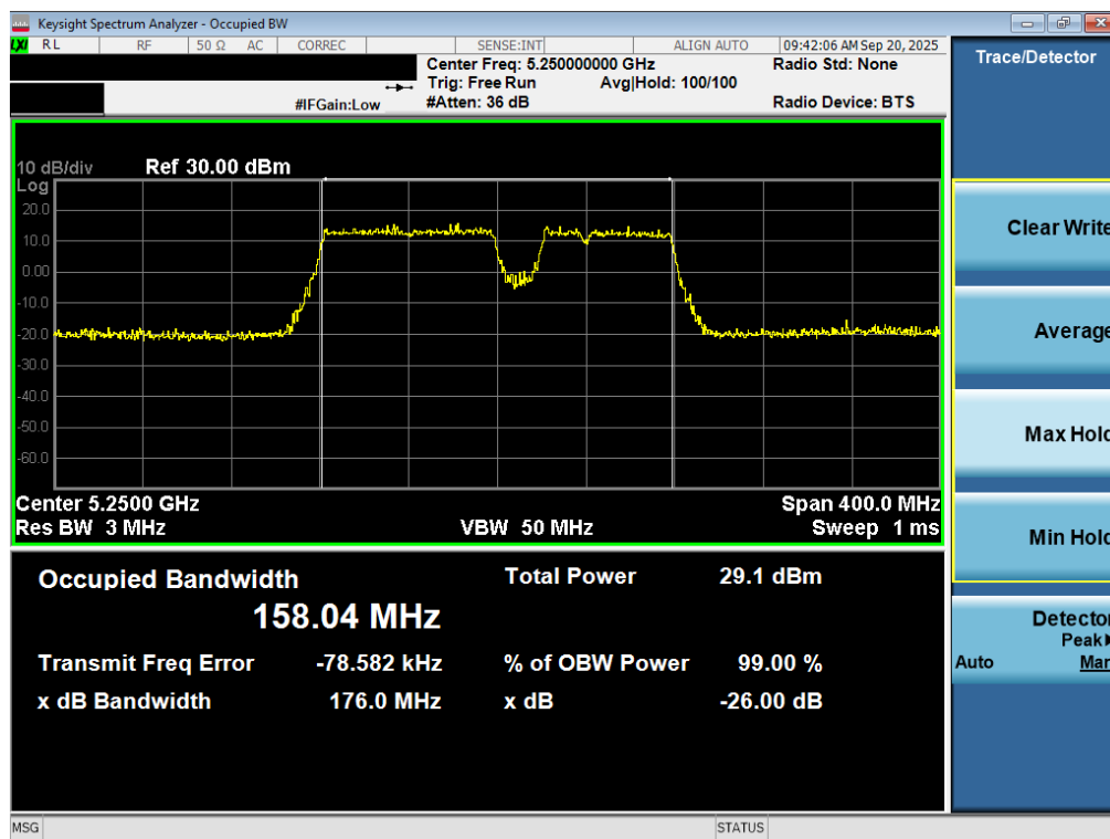
Plot 7-22. 26dB Bandwidth Plot MIMO ANT2 (160MHz BW 802.11be – 20MHz Puncture (UNII Band 1/2A) – Ch. 50)
