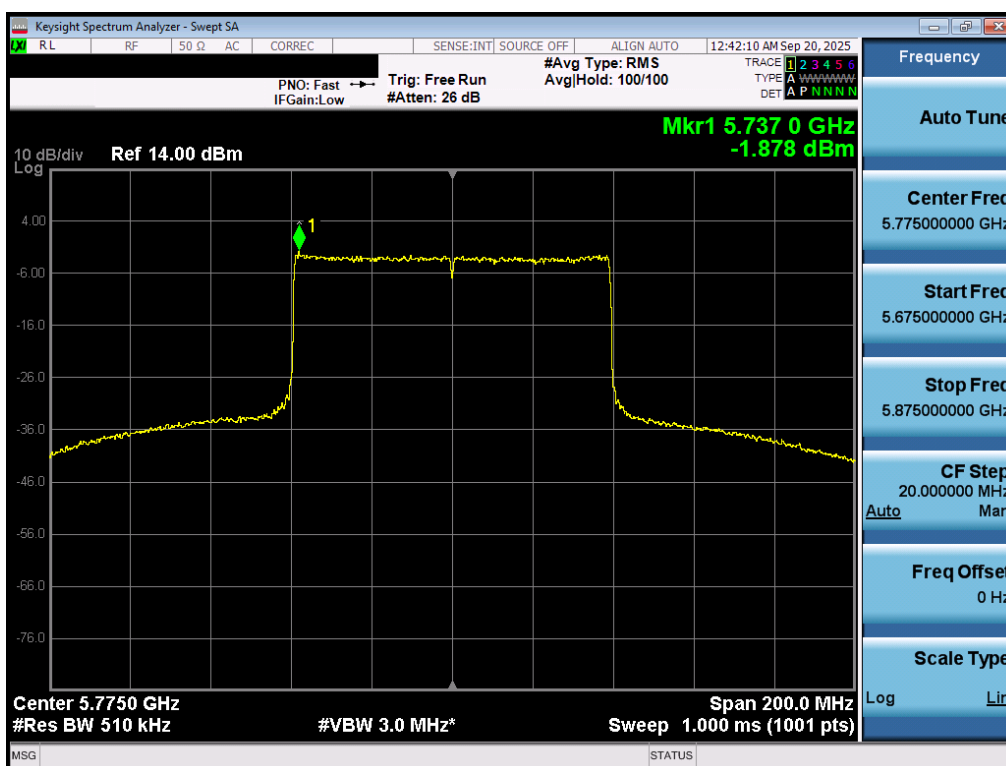
Plot 7-78. Power Spectral Density Plot MIMO ANT1 (80MHz BW 802.11be (UNII Band 3) – Ch. 155)
