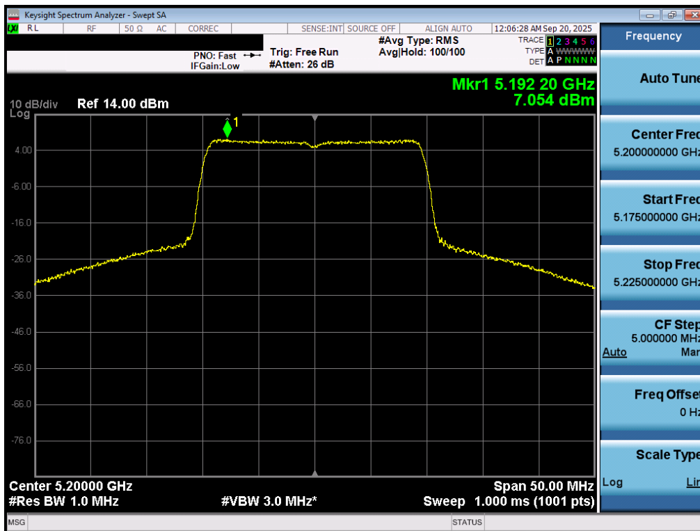
Plot 7-63. Power Spectral Density Plot MIMO ANT1 (20MHz BW 802.11be (UNII Band 1) – Ch. 40)
