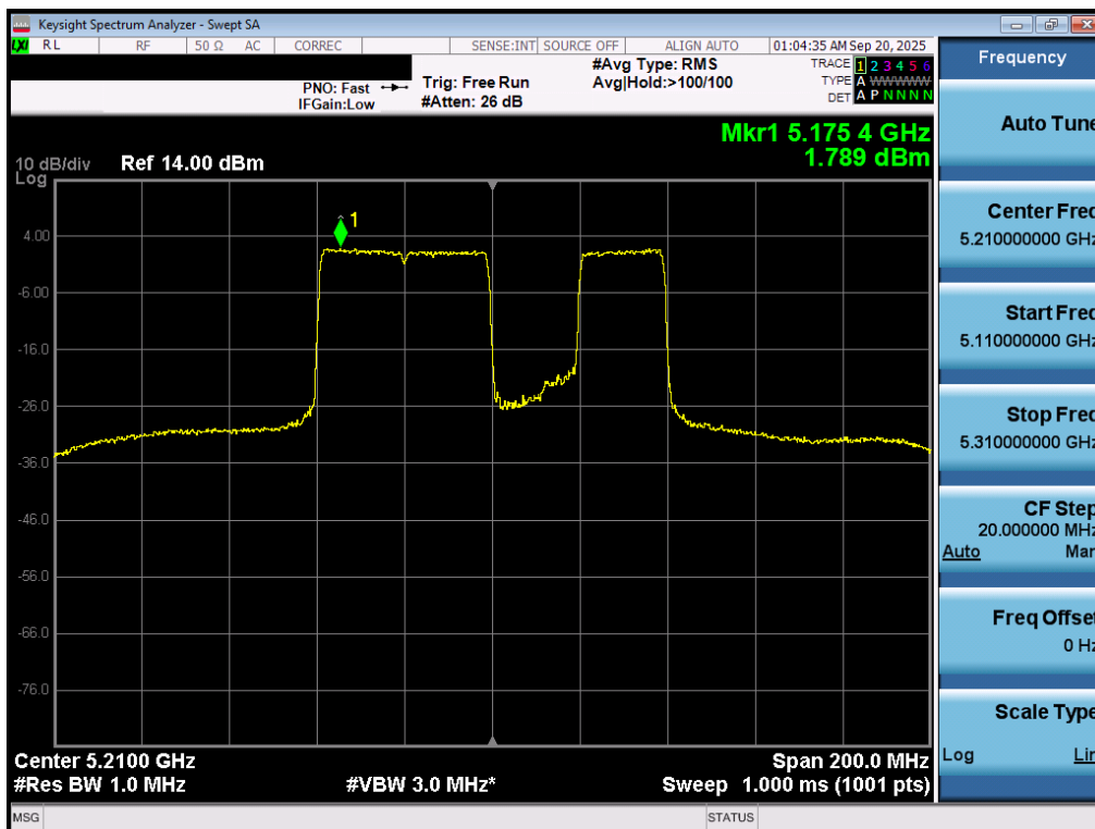
Plot 7-70. Power Spectral Density Plot MIMO ANT1 (80MHz BW 802.11be – 20MHz Puncture (UNII Band 1) – Ch. 42)
