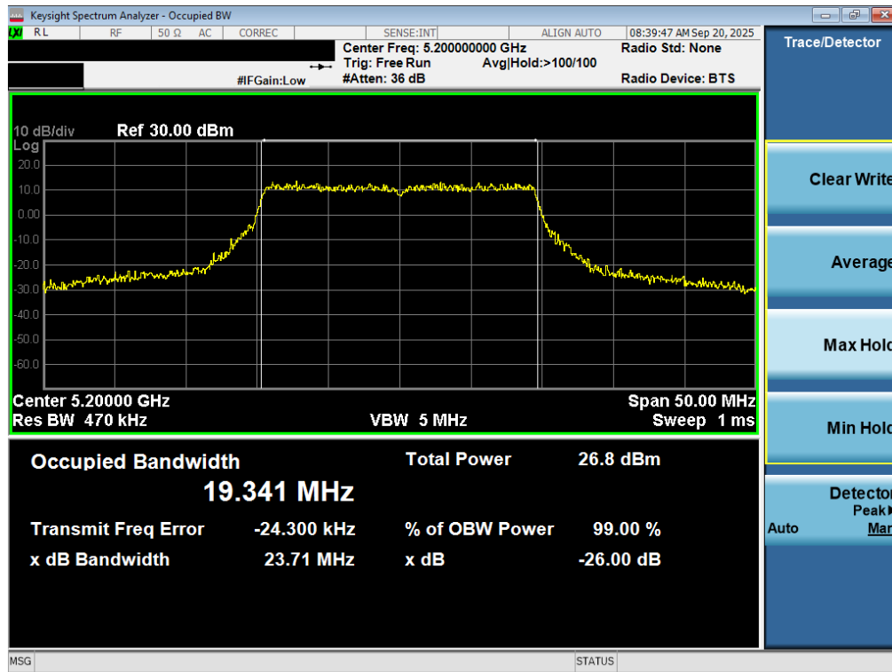
Plot 7-14. 26dB Bandwidth Plot MIMO ANT2 (20MHz BW 802.11be (UNII Band 1) – Ch. 40)
