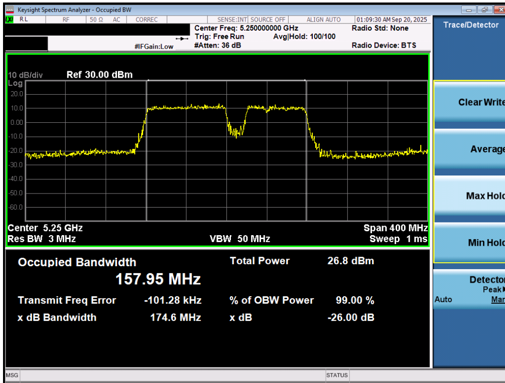
Plot 7-11. 26dB Bandwidth Plot MIMO ANT1 (160MHz BW 802.11be – 20MHz Puncture (UNII Band 1/2A) – Ch. 50)
