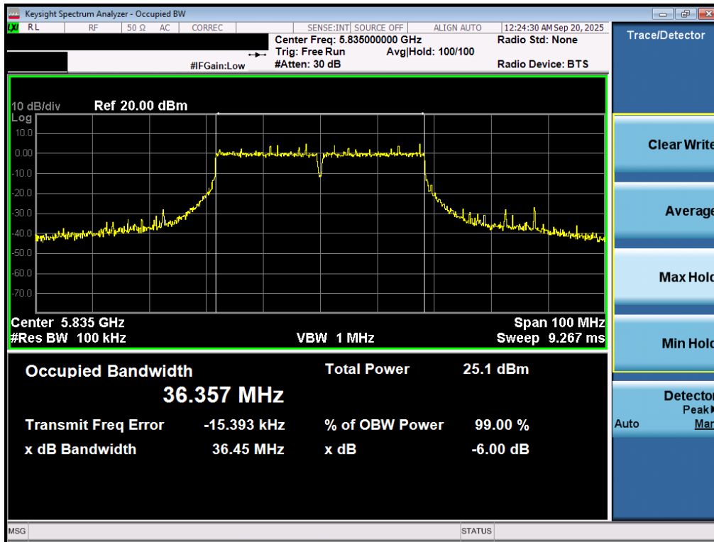
Plot 7-33. 6dB Bandwidth Plot MIMO ANT1 (40MHz BW 802.11n (UNII Band 3/4) – Ch. 167)
