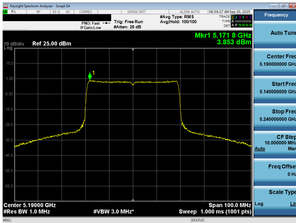
Plot 7-95. Power Spectral Density Plot MIMO ANT2 (40MHz BW 802.11be (UNII Band 1) – Ch. 38)
