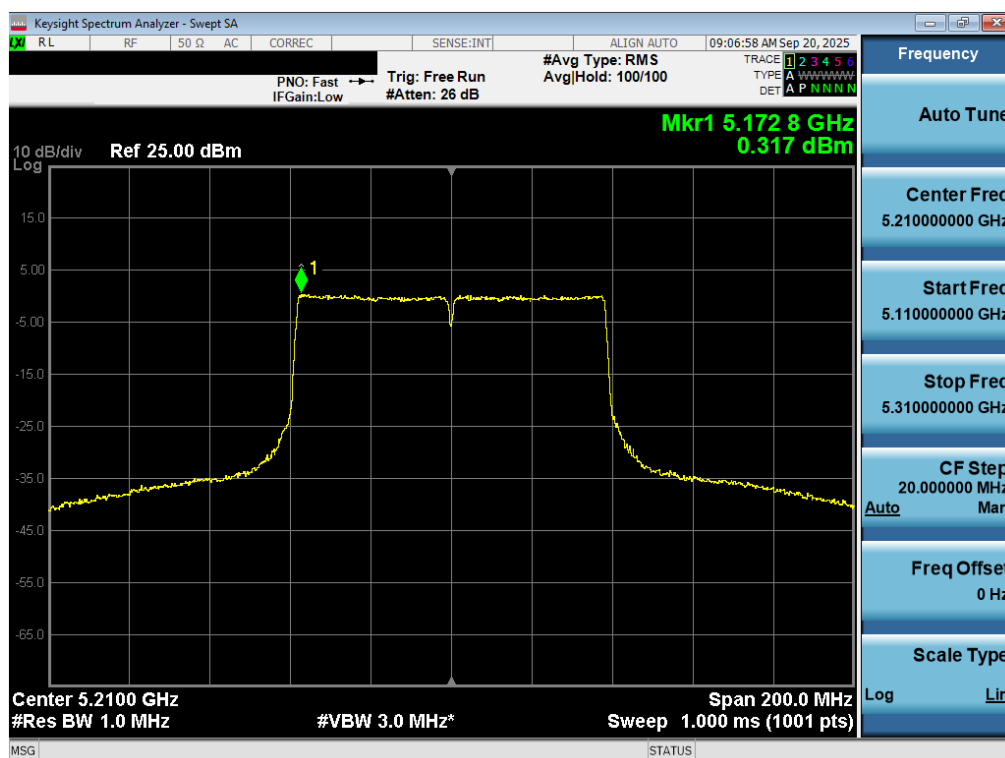
Plot 7-96. Power Spectral Density Plot MIMO ANT2 (80MHz BW 802.11ac (UNII Band 1) – Ch. 42)
