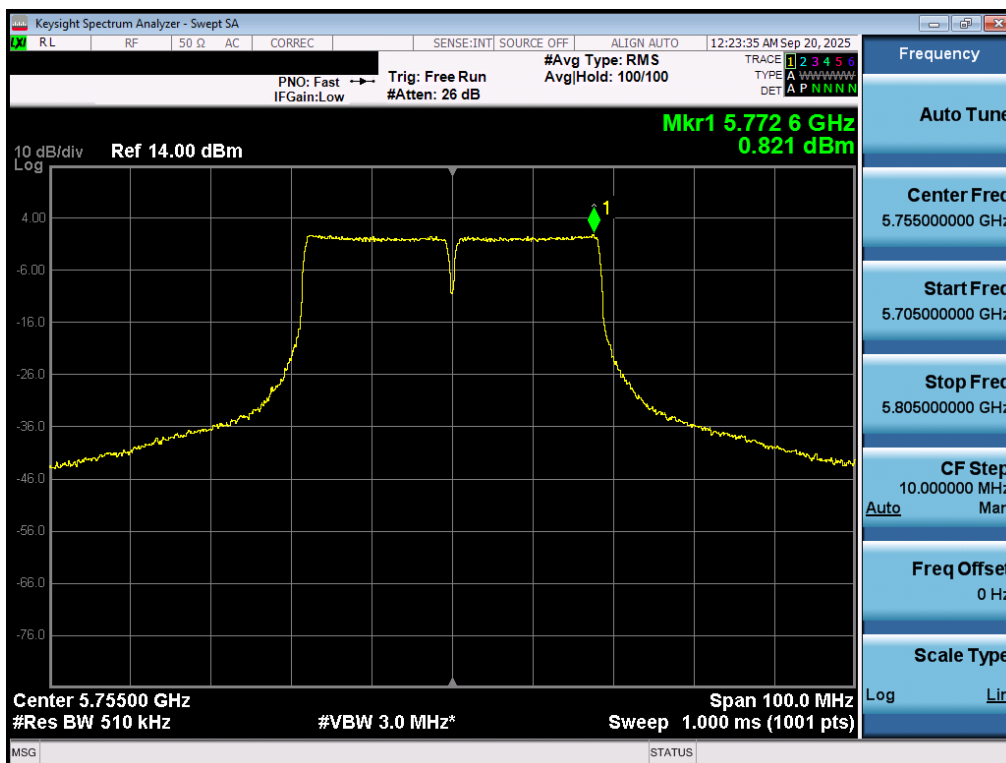
Plot 7-75. Power Spectral Density Plot MIMO ANT1 (40MHz BW 802.11n (UNII Band 3) – Ch. 151)
