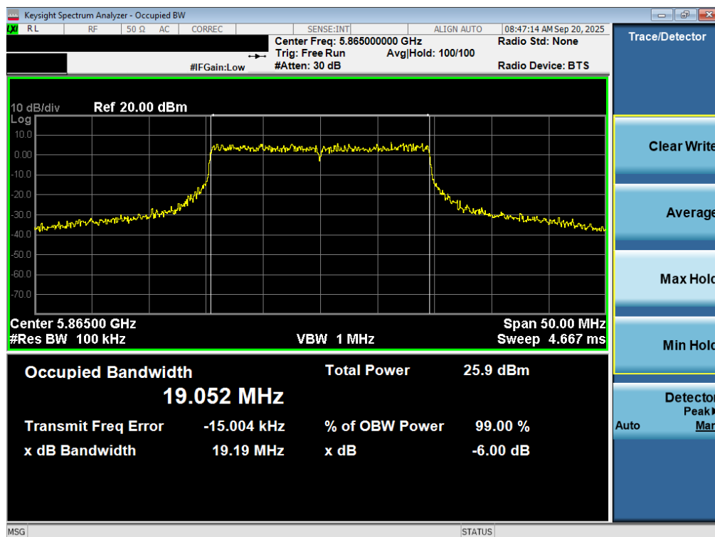
Plot 7-51. 6dB Bandwidth Plot MIMO ANT2 (20MHz BW 802.11be (UNII Band 3/4) – Ch. 173)
