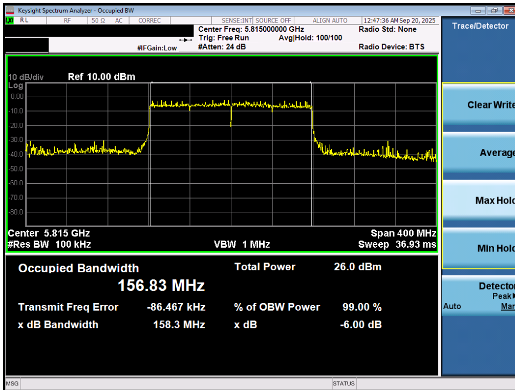
Plot 7-38. 6dB Bandwidth Plot MIMO ANT1 (160MHz BW 802.11be (UNII Band 3/4) – Ch. 163)
