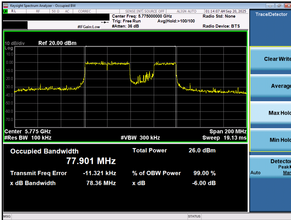
Plot 7-39. 6dB Bandwidth Plot MIMO ANT1 (80MHz BW 802.11be – 20MHz Puncture (UNII Band 3) – Ch. 155)
