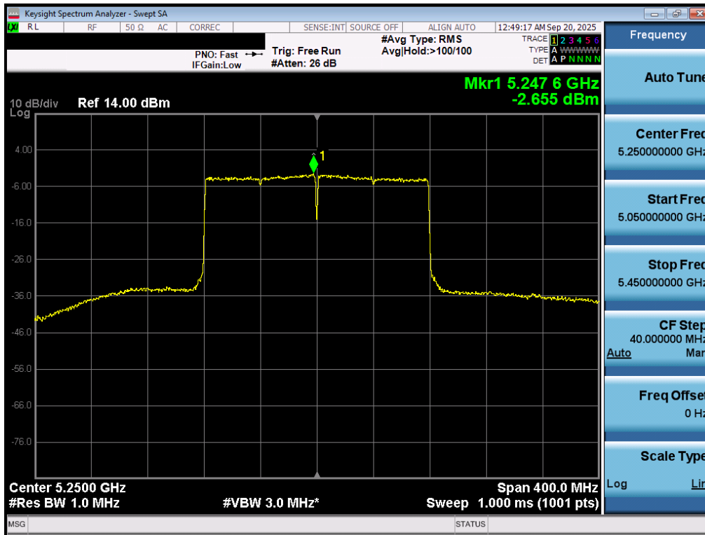
Plot 7-69. Power Spectral Density Plot MIMO ANT1 (160MHz BW 802.11be (UNII Band 1/2A) – Ch. 50)
