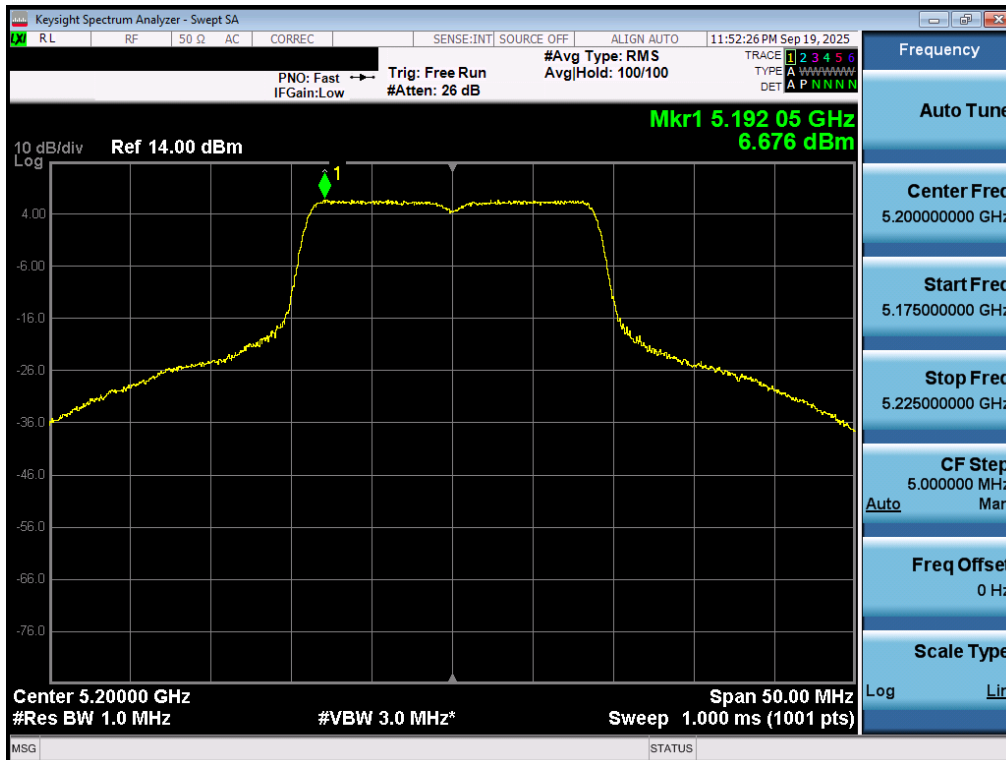
Plot 7-62. Power Spectral Density Plot MIMO ANT1 (20MHz BW 802.11n (UNII Band 1) – Ch. 40)
