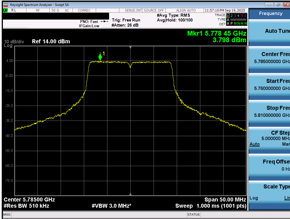
Plot 7-73. Power Spectral Density Plot MIMO ANT1 (20MHz BW 802.11n (UNII Band 3) – Ch. 157)
