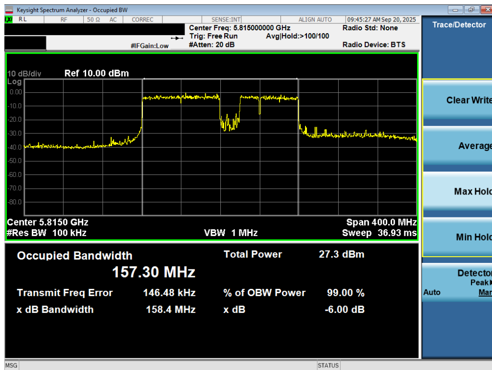
Plot 7-60. 6dB Bandwidth Plot MIMO ANT2 (160MHz BW 802.11be – 20MHz Puncture (UNII Band 3/4) – Ch. 163)
