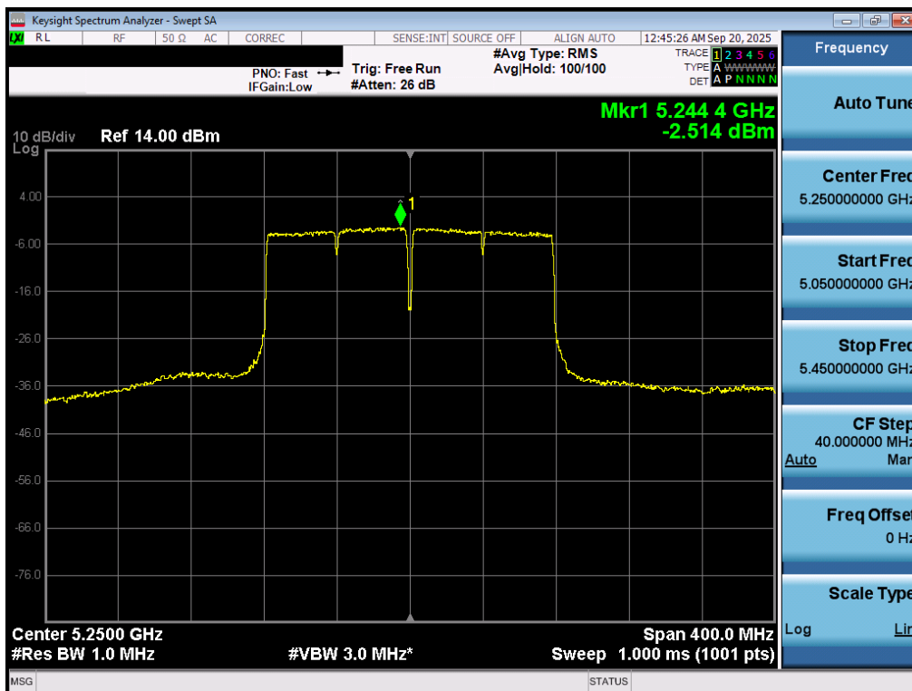
Plot 7-68. Power Spectral Density Plot MIMO ANT1 (160MHz BW 802.11ac (UNII Band 1/2A) – Ch. 50)
