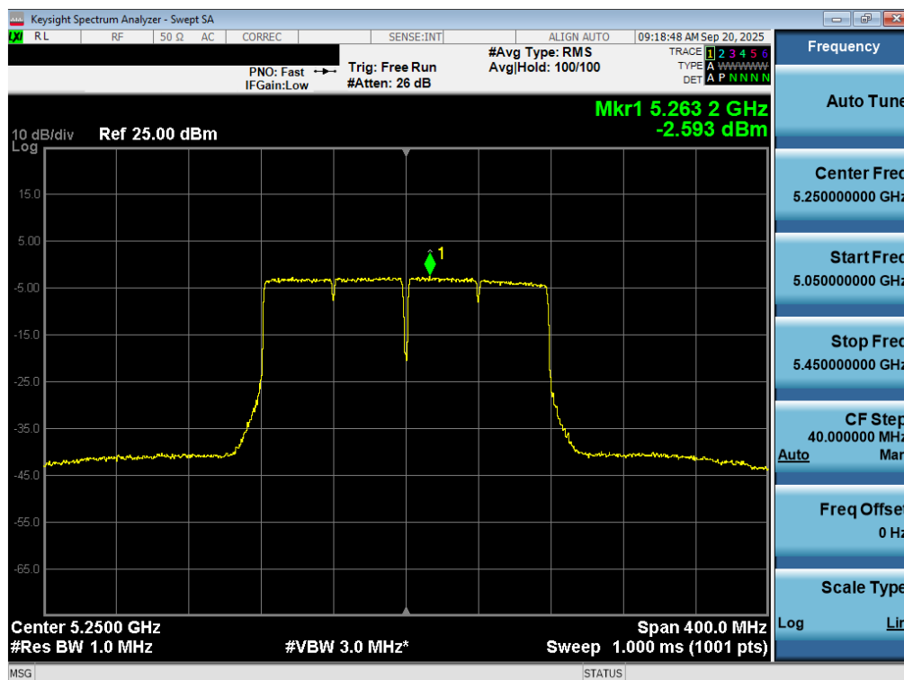
Plot 7-98. Power Spectral Density Plot MIMO ANT2 (160MHz BW 802.11ac (UNII Band 1/2A) – Ch. 50)
