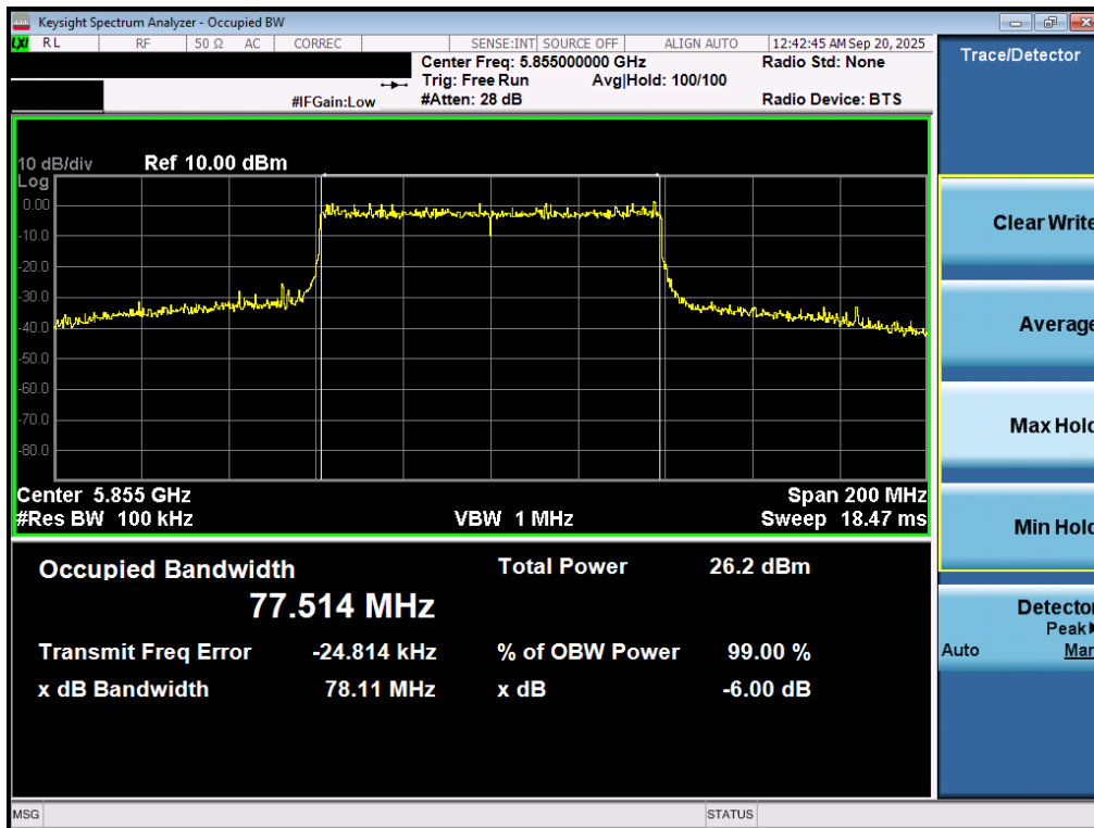
Plot 7-36. 6dB Bandwidth Plot MIMO ANT1 (80MHz BW 802.11be (UNII Band 3/4) – Ch. 171)
