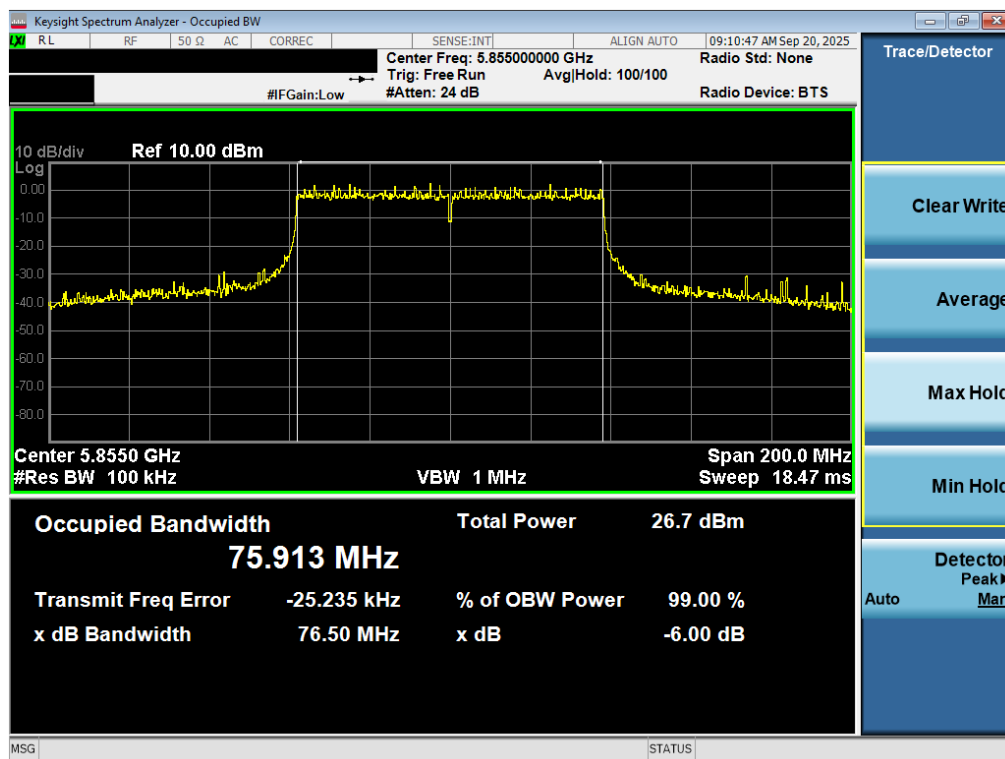
Plot 7-54. 6dB Bandwidth Plot MIMO ANT2 (80MHz BW 802.11ac (UNII Band 3/4) – Ch. 171)
