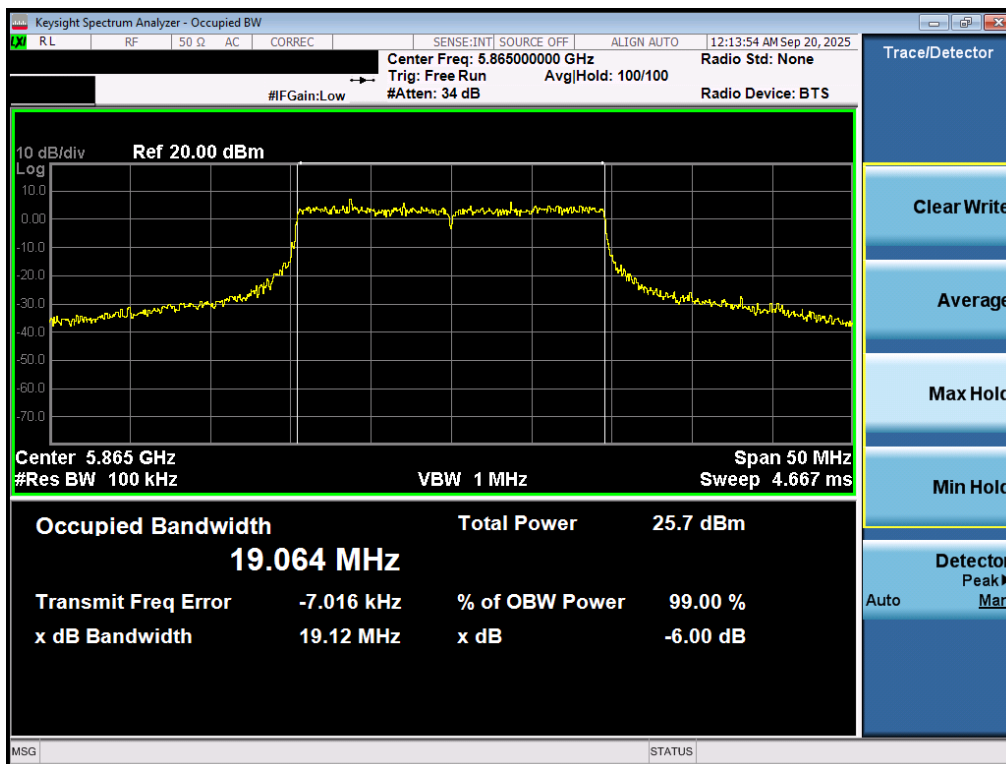
Plot 7-32. 6dB Bandwidth Plot MIMO ANT1 (20MHz BW 802.11be (UNII Band 4) – Ch. 173)
