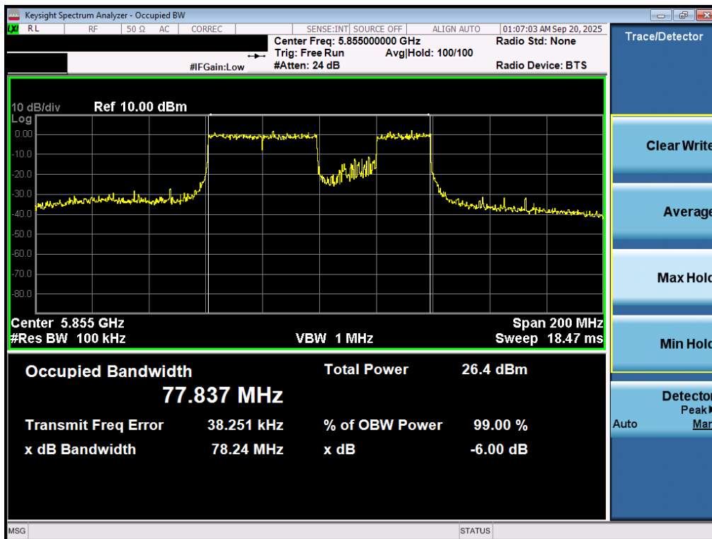
Plot 7-40. 6dB Bandwidth Plot MIMO ANT1 (80MHz BW 802.11be – 20MHz Puncture (UNII Band 3/4) – Ch. 171)
