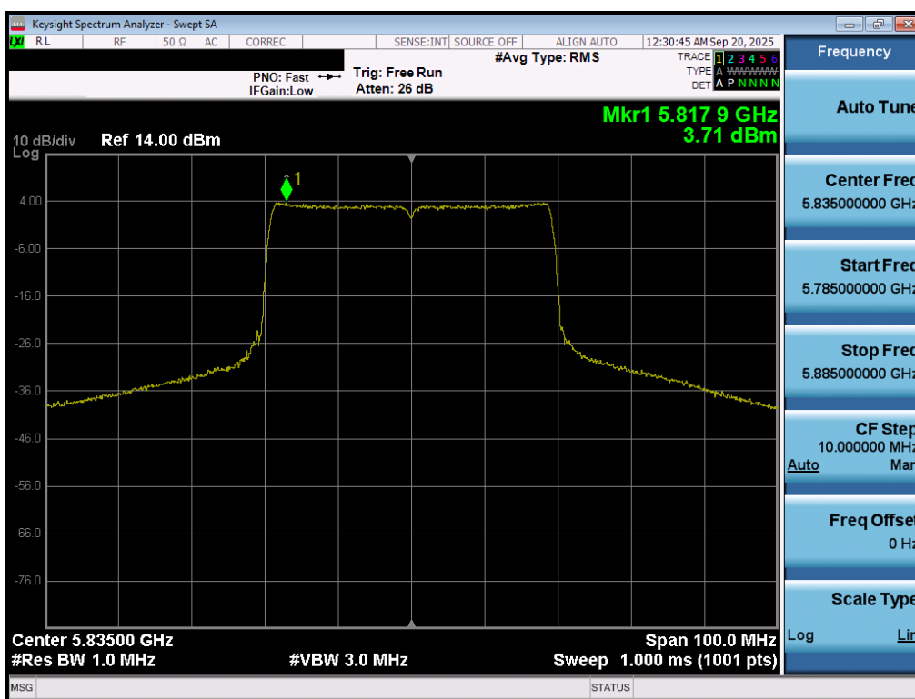
Plot 7-84. Power Spectral Density Plot MIMO ANT1 (40MHz BW 802.11be (UNII Band 3/4) – Ch. 167)
