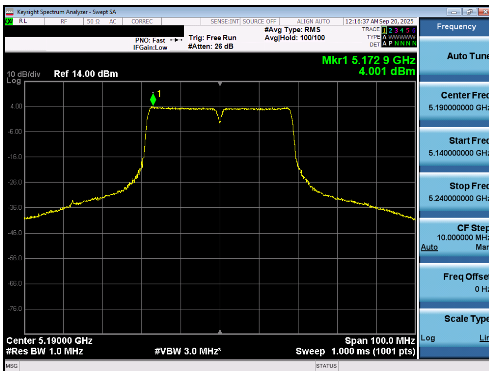
Plot 7-64. Power Spectral Density Plot MIMO ANT1 (40MHz BW 802.11n (UNII Band 1) – Ch. 38)
