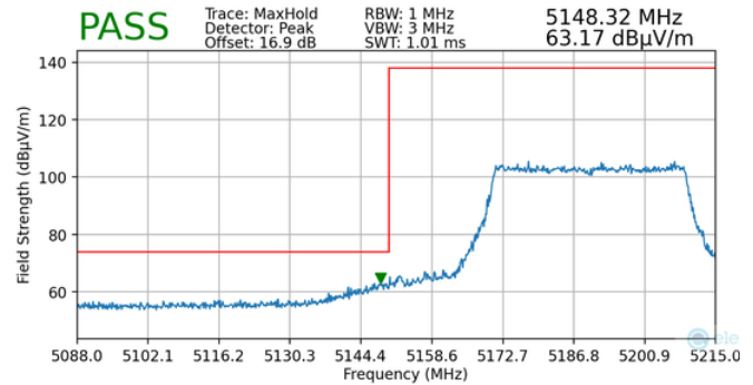
Plot 7-145. Radiated Lower Band Edge Plot MIMO (Peak – UNII Band 1)
