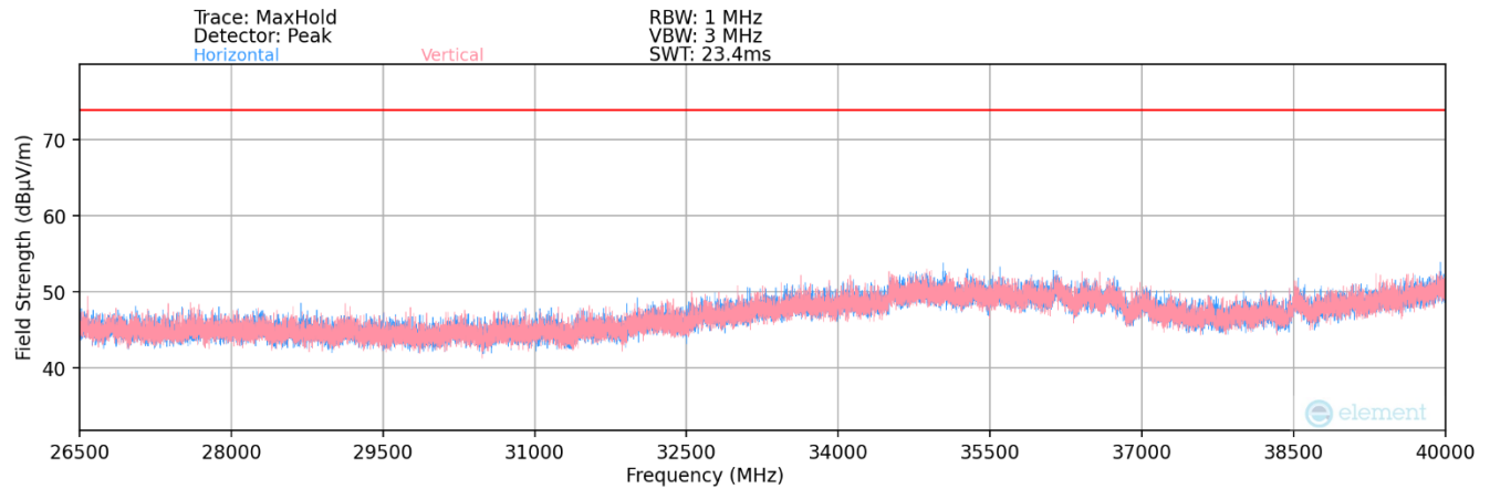
Plot 7-133. Radiated Spurious Plot below 26.5-40GHz MIMO 802.11g (2.4GHz – Ch.6) + MIMO 802.11a (5GHz – Ch. 120)
