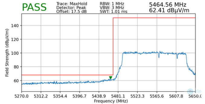
Plot 7-190. Radiated Lower Band Edge Plot MIMO (Peak – UNII Band 2C)
