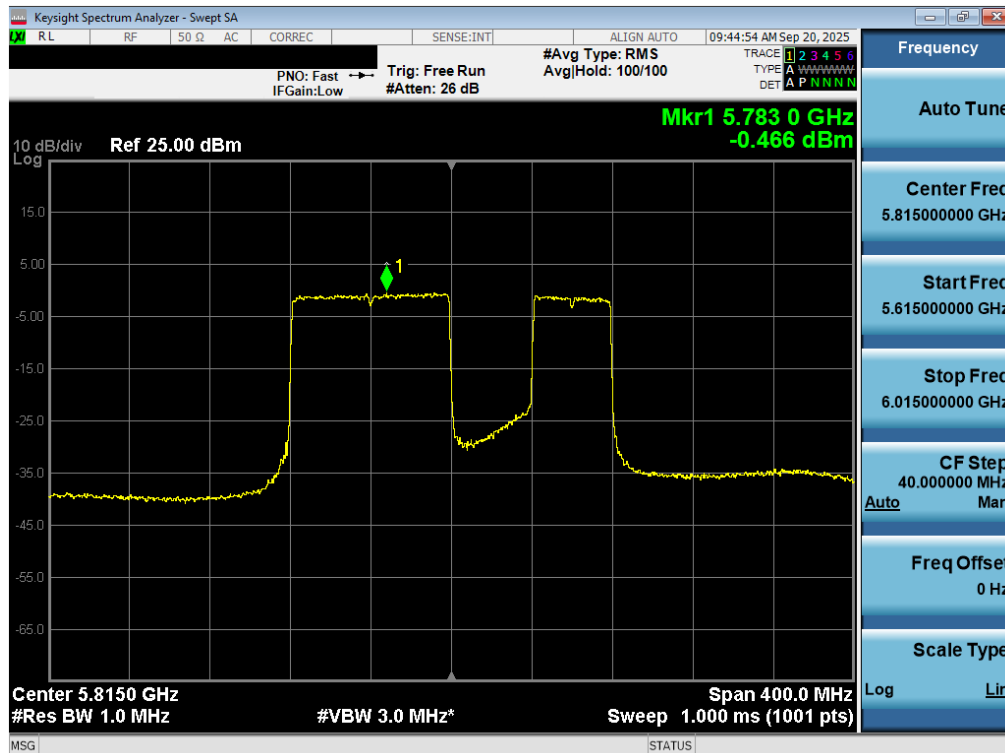
Plot 7-120. Power Spectral Density Plot MIMO ANT2 (160MHz BW 802.11be – 40MHz Puncture (UNII Band 3/4) – Ch. 163)
