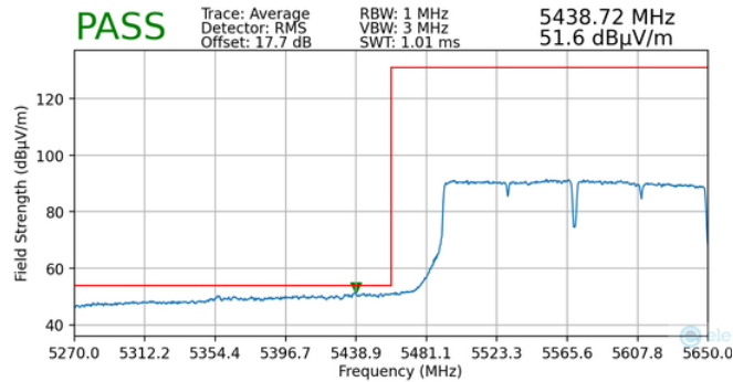
Plot 7-180. Radiated Lower Band Edge Plot MIMO (Average – UNII Band 2C)
