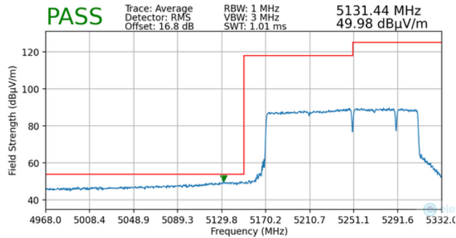
Plot 7-185. Radiated Lower Band Edge Plot MIMO (Average – UNII Band 1)
