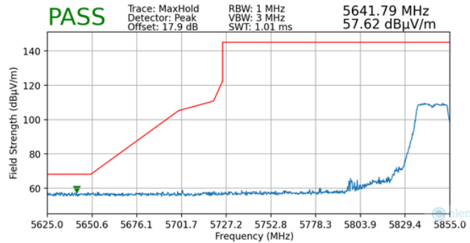
Plot 7-141. Radiated Lower Band Edge Plot MIMO (Peak – UNII Band 4)
