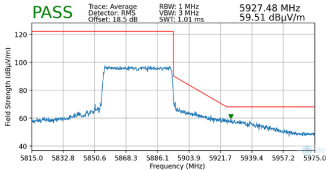
Plot 7-152. Radiated Upper Band Edge Plot MIMO (Average – UNII Band 4)
