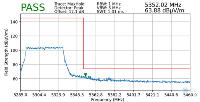
Plot 7-147. Radiated Upper Band Edge Plot MIMO (Peak – UNII Band 2A)
