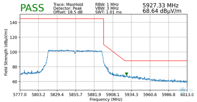
Plot 7-163. Radiated Upper Band Edge Plot MIMO (Peak – UNII Band 4)
