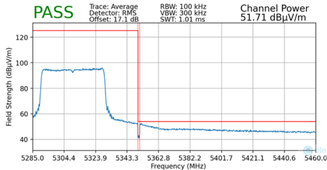
Plot 7-146. Radiated Upper Band Edge Plot MIMO (Average – UNII Band 2A)
