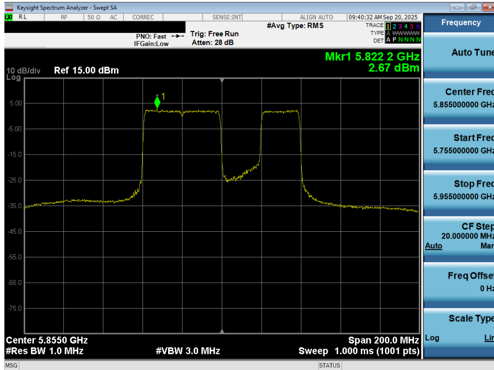
Plot 7-119. Power Spectral Density Plot MIMO ANT2 (80MHz BW 802.11be – 20MHz Puncture (UNII Band 3/4) – Ch. 171)
