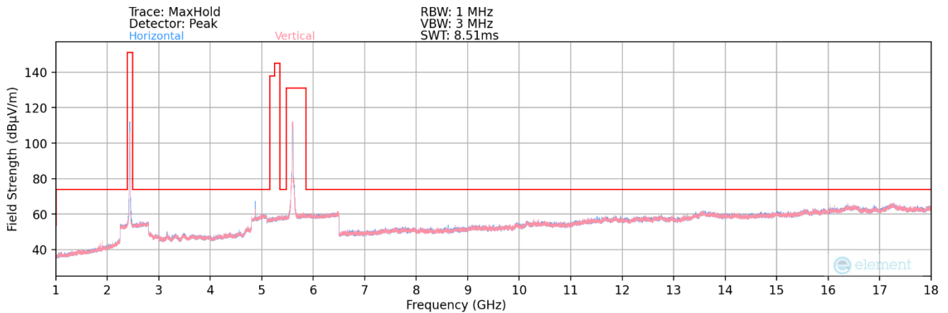
Plot 7-131. Radiated Spurious Plot below 1-18GHz MIMO 802.11g (2.4GHz – Ch.6) + MIMO 802.11a (5GHz – Ch. 120)
