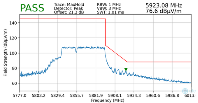
Plot 7-173. Radiated Upper Band Edge Plot MIMO (Peak – UNII Band 4)
