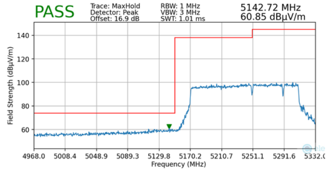
Plot 7-186. Radiated Lower Band Edge Plot MIMO (Peak – UNII Band 1)
