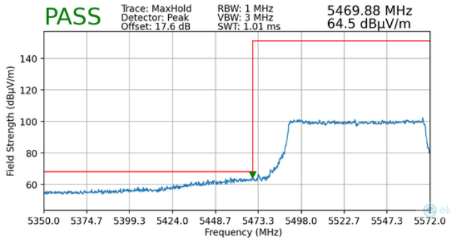
Plot 7-175. Radiated Lower Band Edge Plot MIMO (Peak – UNII Band 2C) – WCP
