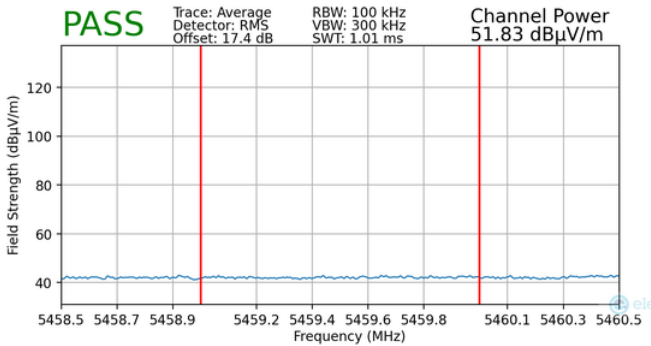
Plot 7-174. Radiated Lower Band Edge Plot MIMO (Average – UNII Band 2C) – WCP
