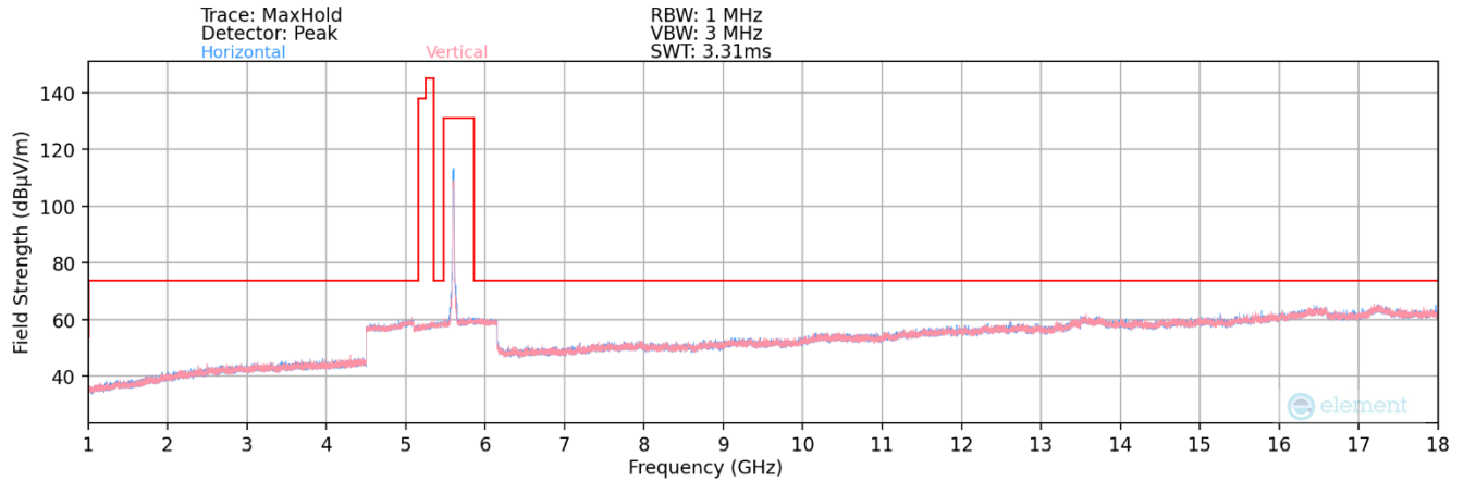
Plot 7-124. Radiated Spurious Plot above 1GHz MIMO (802.11a – UNII Band 2C Ch. 120)
