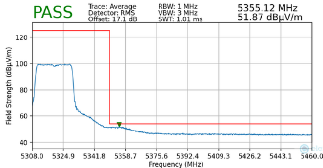
Plot 7-136. Radiated Upper Band Edge Plot MIMO (Average – UNII Band 2A)
