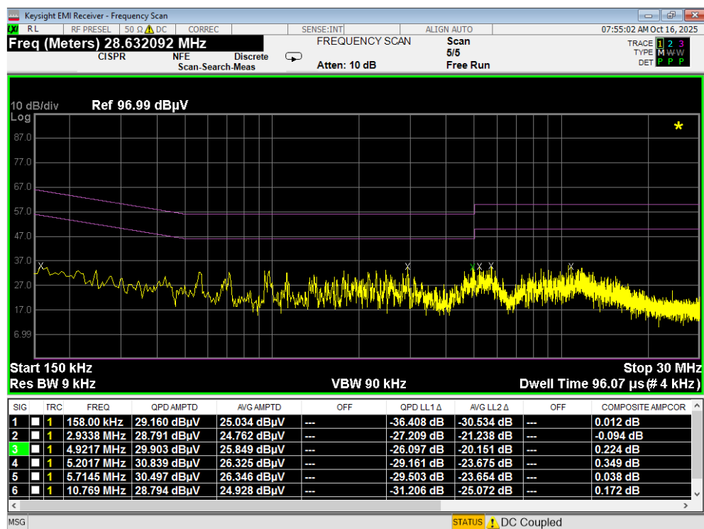
Plot 7-198. Line Conducted Plot with 802.11a UNII Band 2C (L1)
