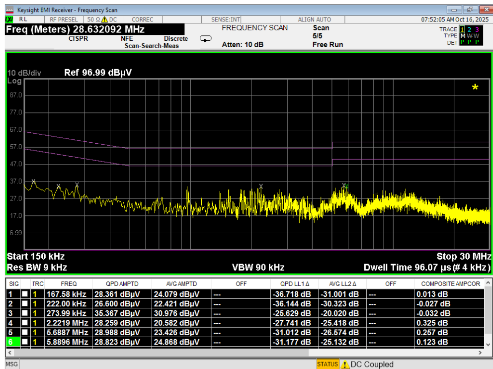
Plot 7-199. Line Conducted Plot with 802.11a UNII Band 2C (N)
