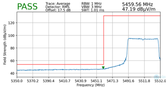
Plot 7-148. Radiated Lower Band Edge Plot MIMO (Average – UNII Band 2C)
