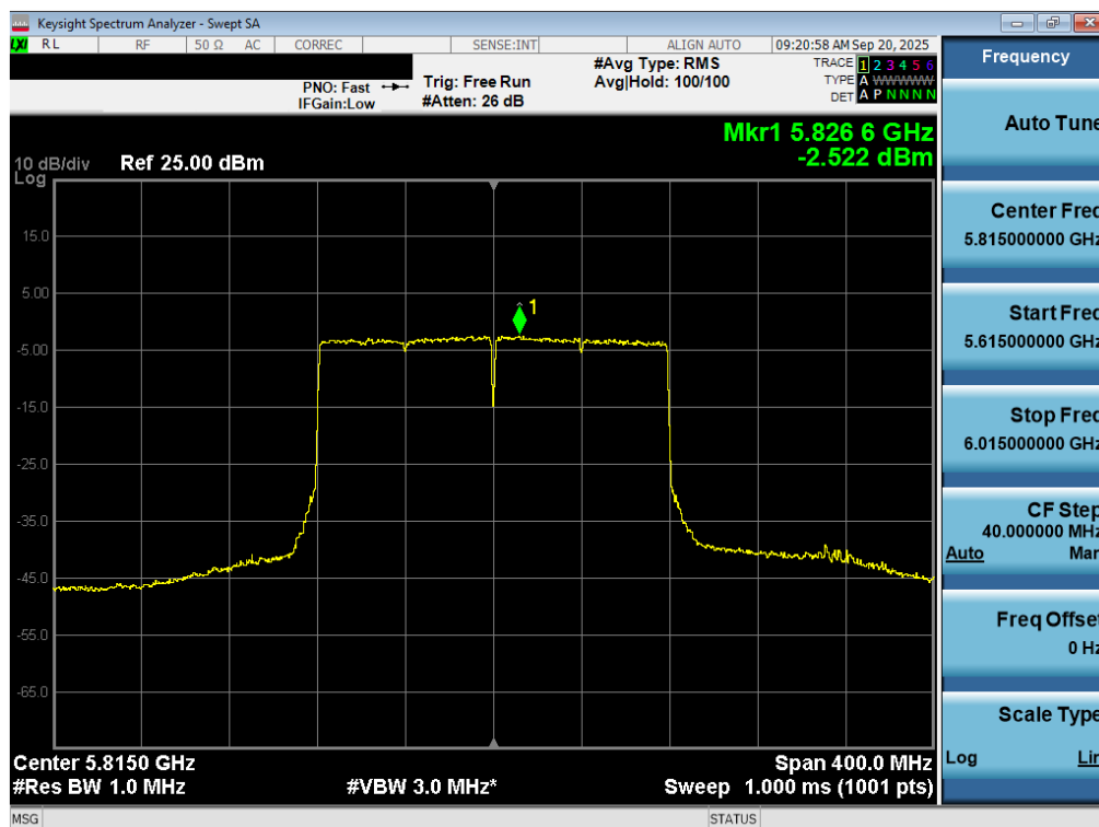
Plot 7-118. Power Spectral Density Plot MIMO ANT2 (160MHz BW 802.11be (UNII Band 3/4) – Ch. 163)
