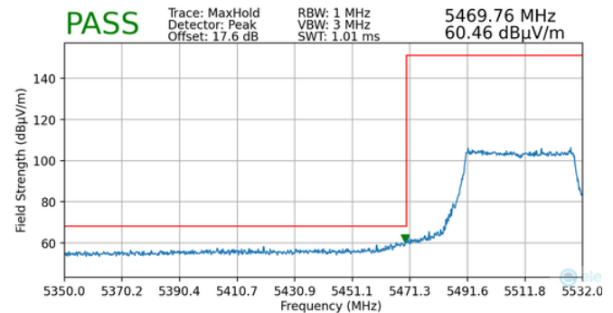
Plot 7-149. Radiated Lower Band Edge Plot MIMO (Peak – UNII Band 2C)
