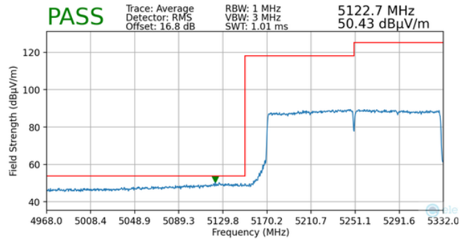
Plot 7-176. Radiated Lower Band Edge Plot MIMO (Average – UNII Band 1)
