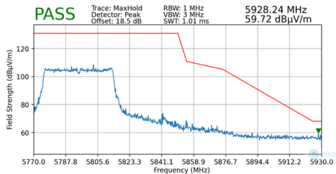
Plot 7-150. Radiated Upper Band Edge Plot MIMO (Peak – UNII Band 3)
