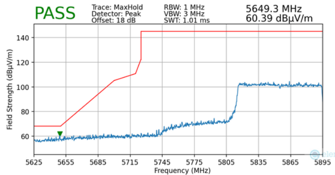
Plot 7-161. Radiated Lower Band Edge Plot MIMO (Peak – UNII Band 4)
