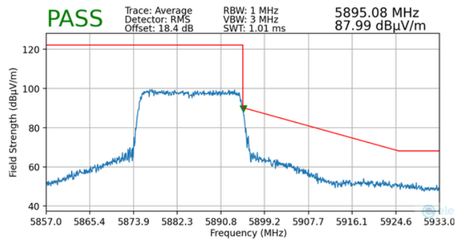
Plot 7-142. Radiated Upper Band Edge Plot MIMO (Average – UNII Band 4)
