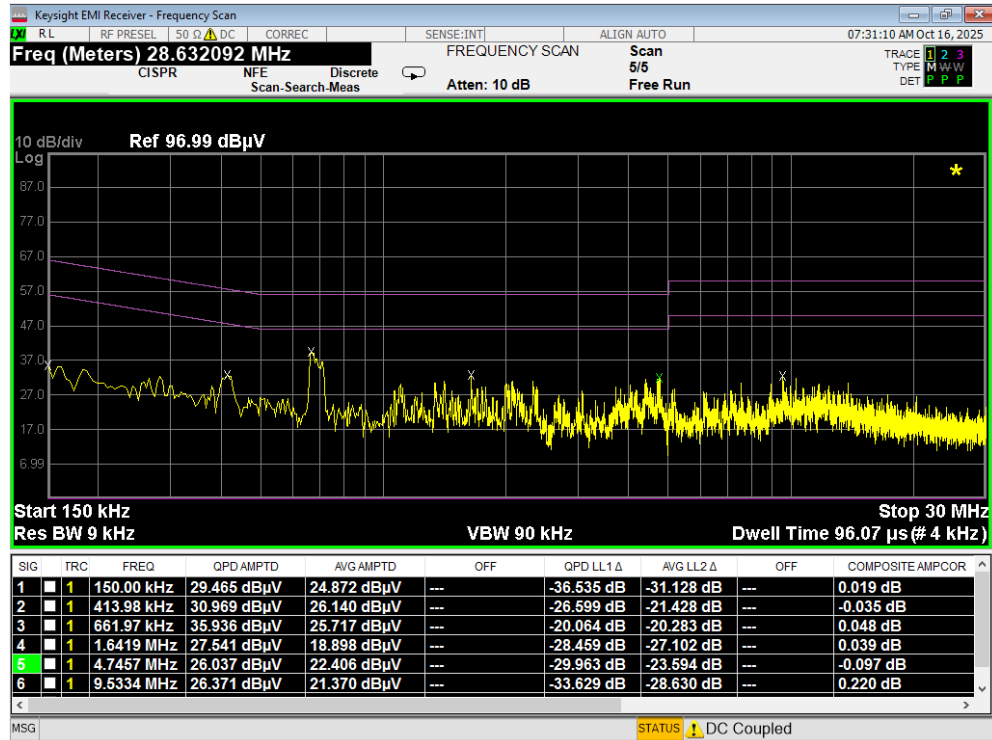
Plot 7-196. Line Conducted Plot with 802.11a UNII Band 2A (L1)
