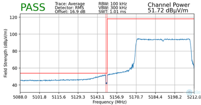
Plot 7-144. Radiated Lower Band Edge Plot MIMO (Average – UNII Band 1)
