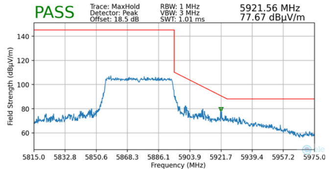
Plot 7-153. Radiated Upper Band Edge Plot MIMO (Peak – UNII Band 4)
