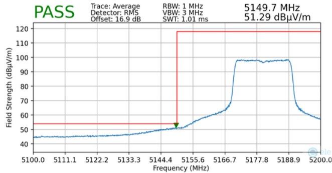
Plot 7-134. Radiated Lower Band Edge Plot MIMO (Average – UNII Band 1)
