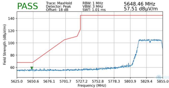
Plot 7-151. Radiated Lower Band Edge Plot MIMO (Peak – UNII Band 4)
