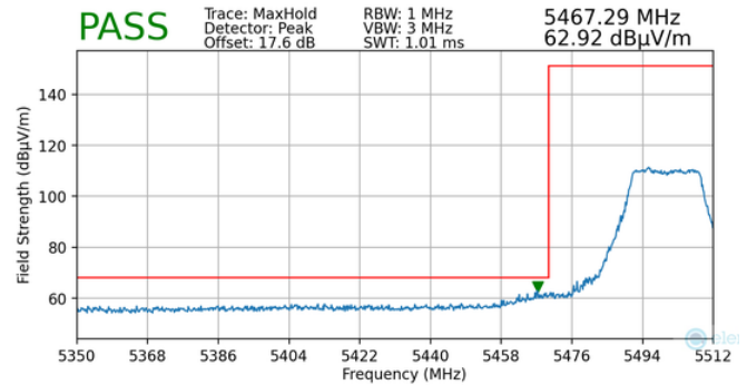
Plot 7-139. Radiated Lower Band Edge Plot MIMO (Peak – UNII Band 2C)
