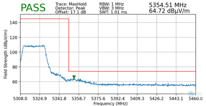
Plot 7-137. Radiated Upper Band Edge Plot MIMO (Peak – UNII Band 2A)
