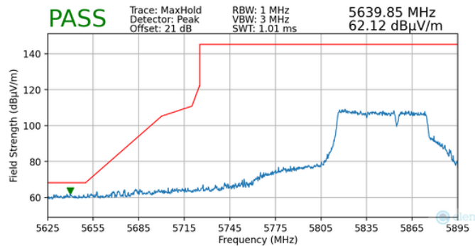
Plot 7-171. Radiated Lower Band Edge Plot MIMO (Peak – UNII Band 4)
