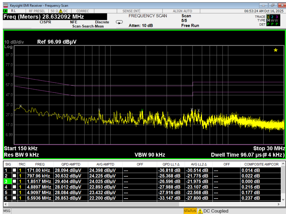
Plot 7-195. Line Conducted Plot with 802.11a UNII Band 1 (N)
