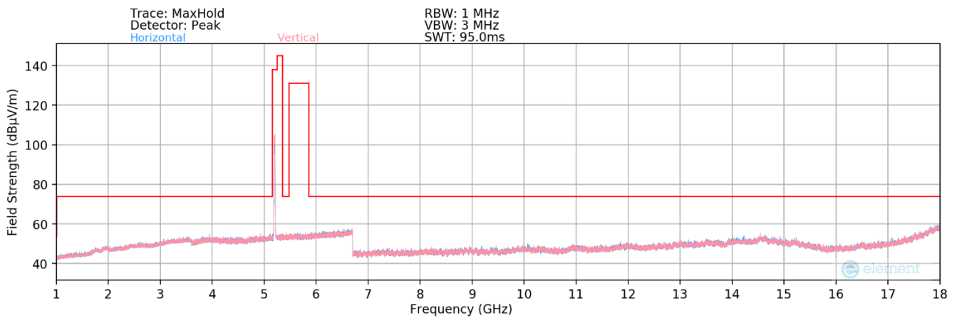
Plot 7-122. Radiated Spurious Plot above 1GHz MIMO (802.11a – UNII Band 1 Ch. 40)
