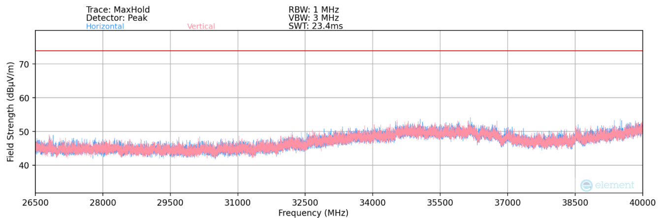
Plot 7-129. Radiated Spurious Plot 26.5GHz – 40GHz MIMO (802.11a)
