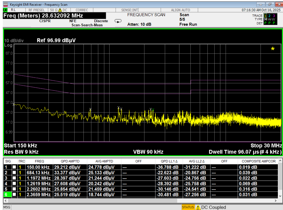
Plot 7-197. Line Conducted Plot with 802.11a UNII Band 2A (N)
