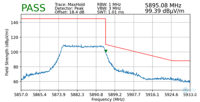
Plot 7-143. Radiated Upper Band Edge Plot MIMO (Peak – UNII Band 4)
