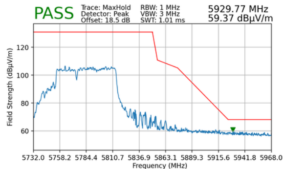
Plot 7-170. Radiated Upper Band Edge Plot MIMO (Peak – UNII Band 3)
