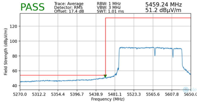
Plot 7-189. Radiated Lower Band Edge Plot MIMO (Average – UNII Band 2C)
