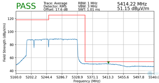
Plot 7-187. Radiated Upper Band Edge Plot MIMO (Average – UNII Band 2A)
