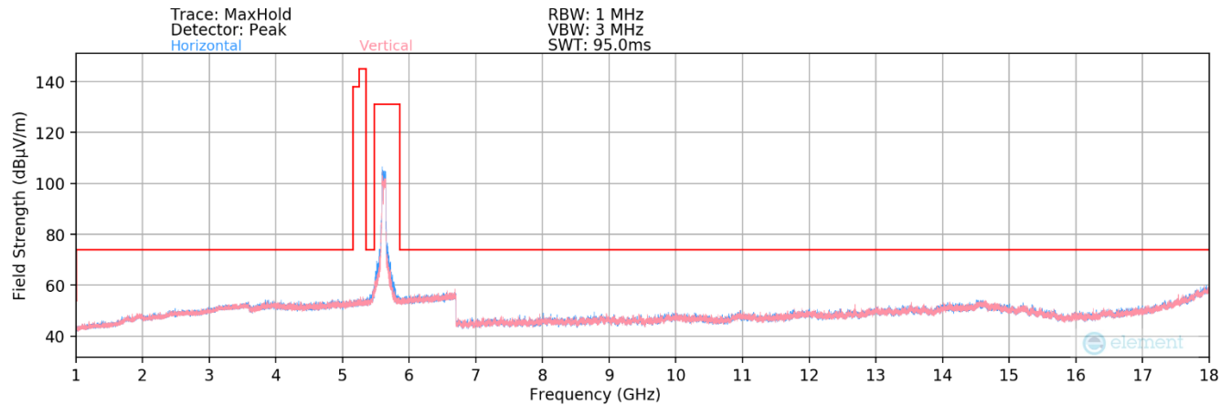
Plot 7-127. Radiated Spurious Plot above 1GHz MIMO (802.11be – UNII Band 2C Ch. 122 – Punctured)
