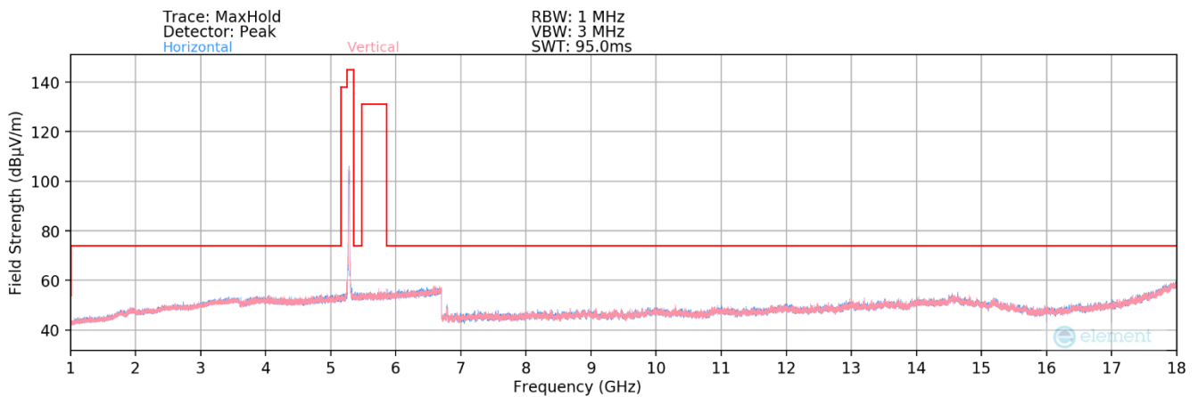
Plot 7-123. Radiated Spurious Plot above 1GHz MIMO (802.11a – UNII Band 2A Ch. 56)
