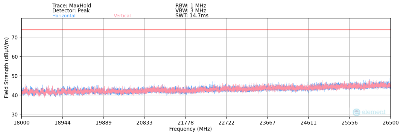
Plot 7-128. Radiated Spurious Plot 18GHz – 26.5GHz MIMO (802.11a)
