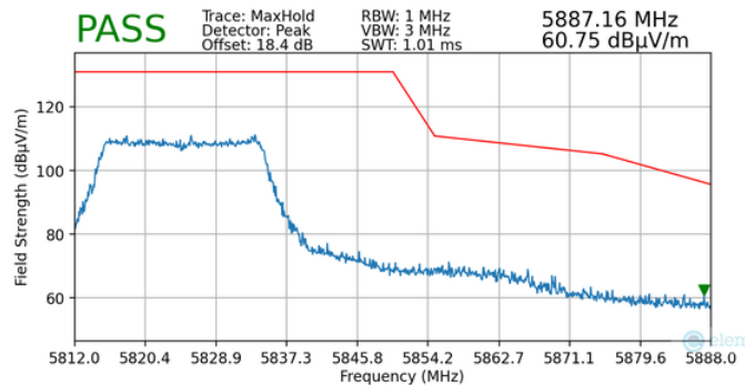
Plot 7-140. Radiated Upper Band Edge Plot MIMO (Peak – UNII Band 3)
