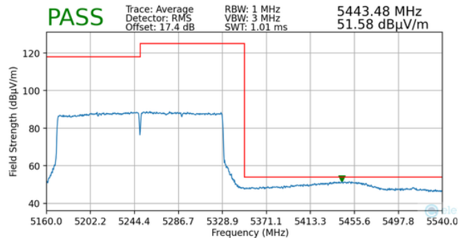
Plot 7-178. Radiated Upper Band Edge Plot MIMO (Average – UNII Band 2A)
