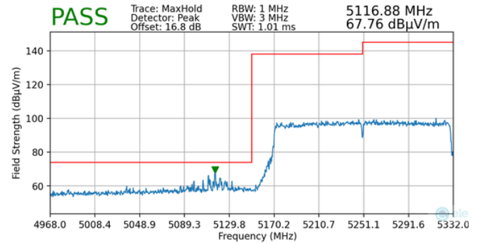
Plot 7-177. Radiated Lower Band Edge Plot MIMO (Peak – UNII Band 1)
