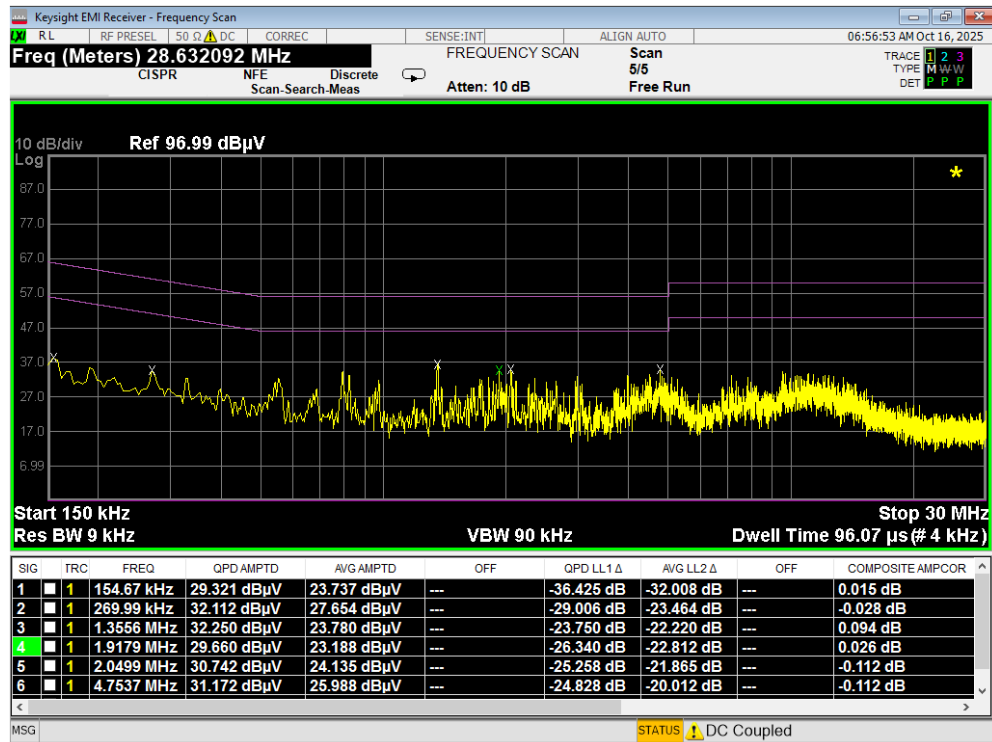
Plot 7-194. Line Conducted Plot with 802.11a UNII Band 1 (L1)
