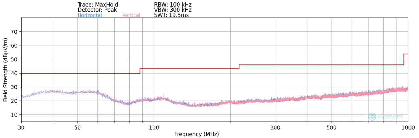
Plot 7-130. Radiated Spurious Plot below 1GHz MIMO 802.11g (2.4GHz – Ch. 6) + MIMO 802.11a (5GHz – Ch. 120)
