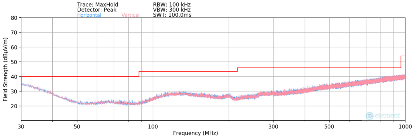
Plot 7-121. Radiated Spurious Plot below 1GHz MIMO (802.11a)
