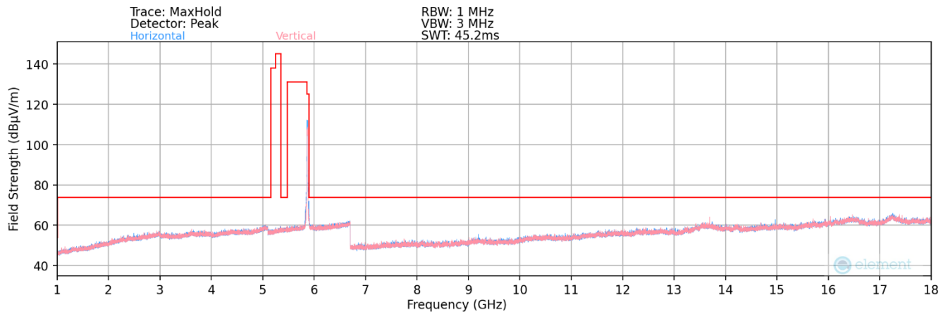
Plot 7-126. Radiated Spurious Plot above 1GHz MIMO (802.11a – UNII Band 4 Ch. 173)
