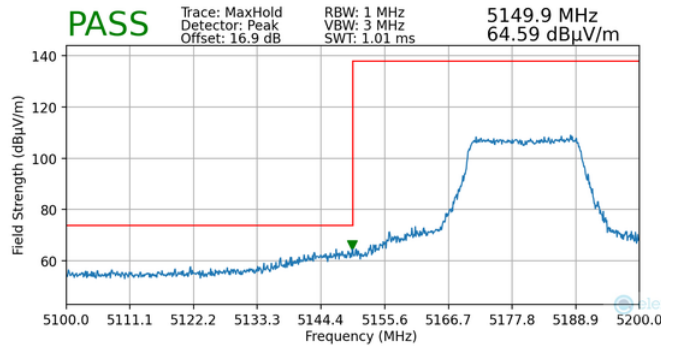
Plot 7-135. Radiated Lower Band Edge Plot MIMO (Peak – UNII Band 1)
