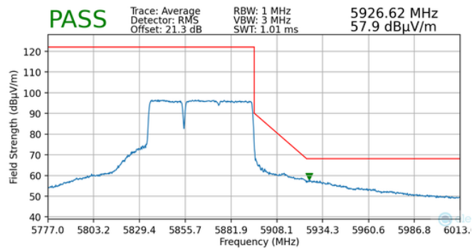
Plot 7-172. Radiated Upper Band Edge Plot MIMO (Average – UNII Band 4)
