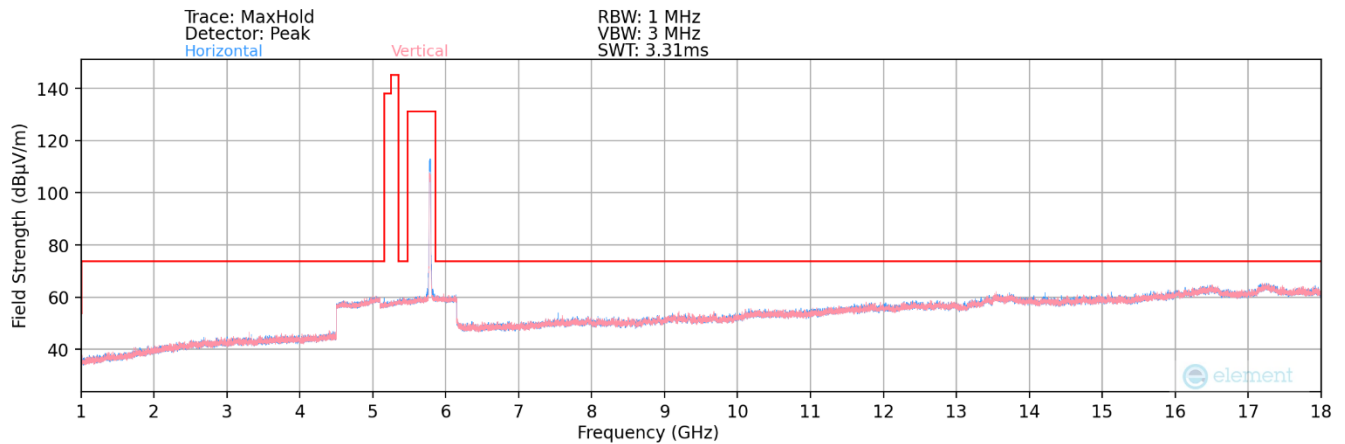
Plot 7-125. Radiated Spurious Plot above 1GHz MIMO (802.11a – UNII Band 3 Ch. 157)
