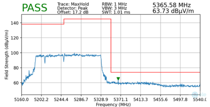
Plot 7-188. Radiated Upper Band Edge Plot MIMO (Peak – UNII Band 2A)
