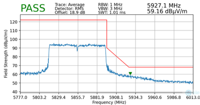
Plot 7-162. Radiated Upper Band Edge Plot MIMO (Average – UNII Band 4)
