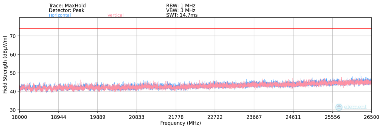
Plot 7-132. Radiated Spurious Plot below 18-26.5GHz MIMO 802.11g (2.4GHz – Ch.6) + MIMO 802.11a (5GHz – Ch. 120)
