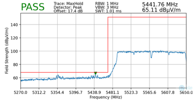
Plot 7-181. Radiated Lower Band Edge Plot MIMO (Peak – UNII Band 2C)
