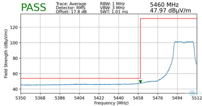
Plot 7-138. Radiated Lower Band Edge Plot MIMO (Average – UNII Band 2C)
