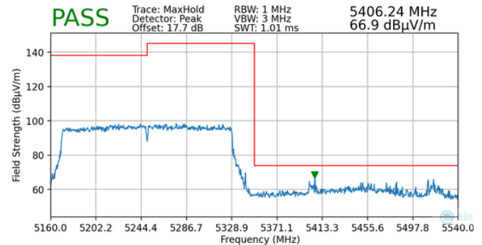
Plot 7-179. Radiated Upper Band Edge Plot MIMO (Peak – UNII Band 2A)
