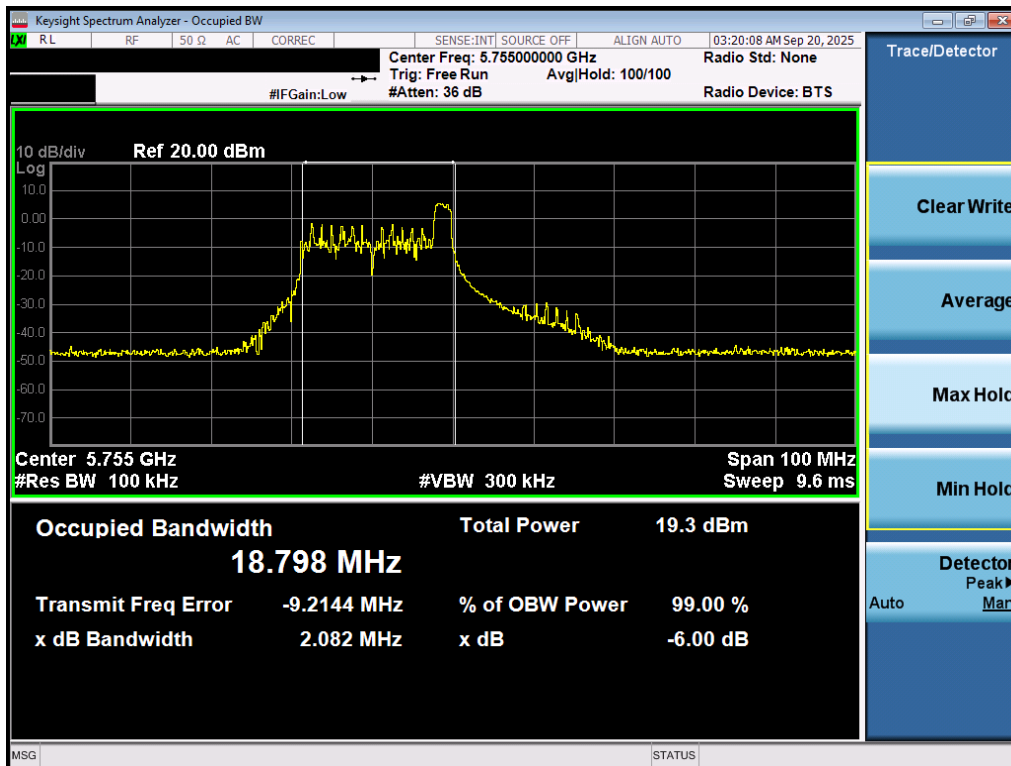
Plot 7-22. 6dB Bandwidth Plot MIMO ANT1 (40MHz BW 802.11be – 26 Tones (UNII Band 3) – Ch. 151)
