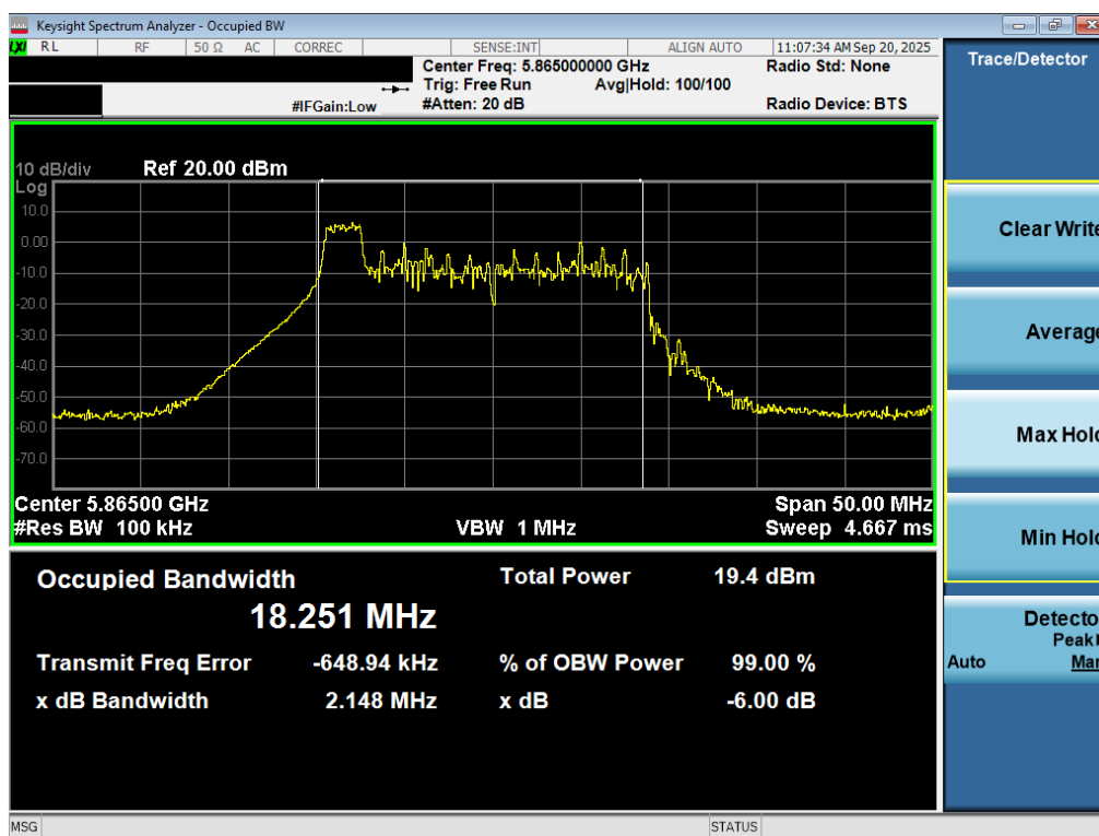
Plot 7-41. 6dB Bandwidth Plot MIMO ANT2 (20MHz BW 802.11be – 26 Tones (UNII Band 4) – Ch. 173)
