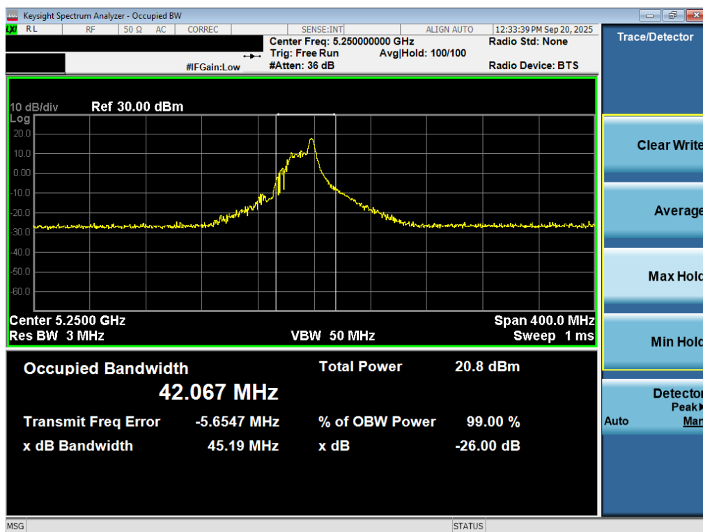
Plot 7-14. 26dB Bandwidth Plot MIMO ANT2 (160MHz(U) BW 802.11be – 26 Tones (UNII Band 1/2A) – Ch. 50)
