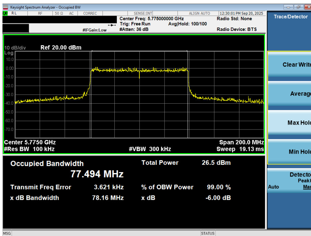
Plot 7-47. 6dB Bandwidth Plot MIMO ANT2 (80MHz BW 802.11be – 996 Tones (UNII Band 3) – Ch. 155)
