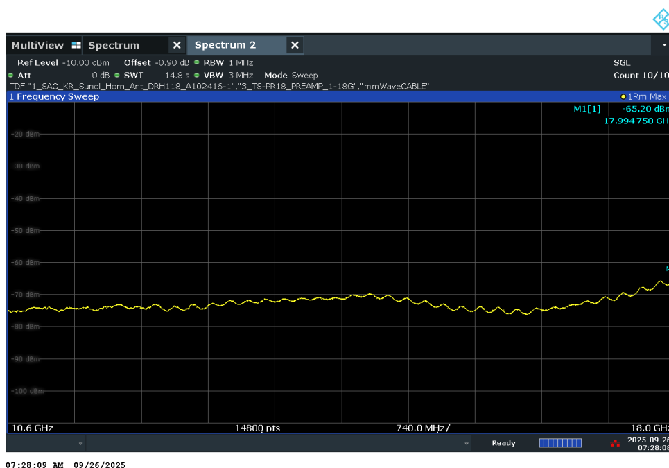
Plot 7-46. Radiated Spurious Pre-Scan 10600 - 18000 MHz - CH.9
