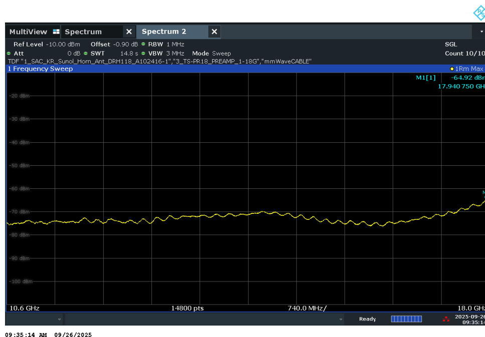
Plot 7-41. Radiated Spurious Pre-Scan 10600 - 18000 MHz - CH.5
