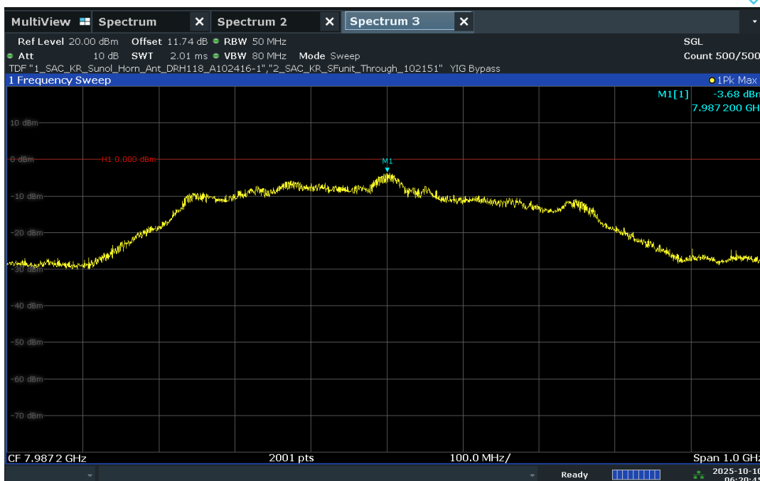
Plot 7-33. UWB Peak Power Measurement - CH.9 – BPRF
