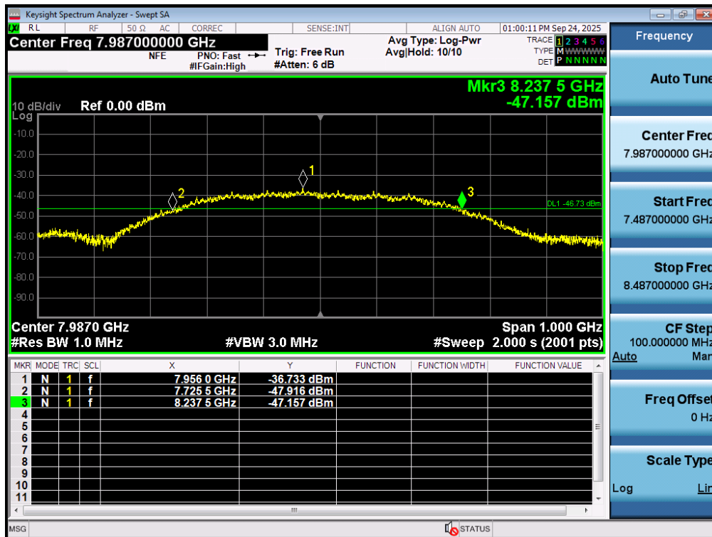
Plot 7-24. 10dBc Bandwidth – CH.9 – SP3 – Preamble 11
