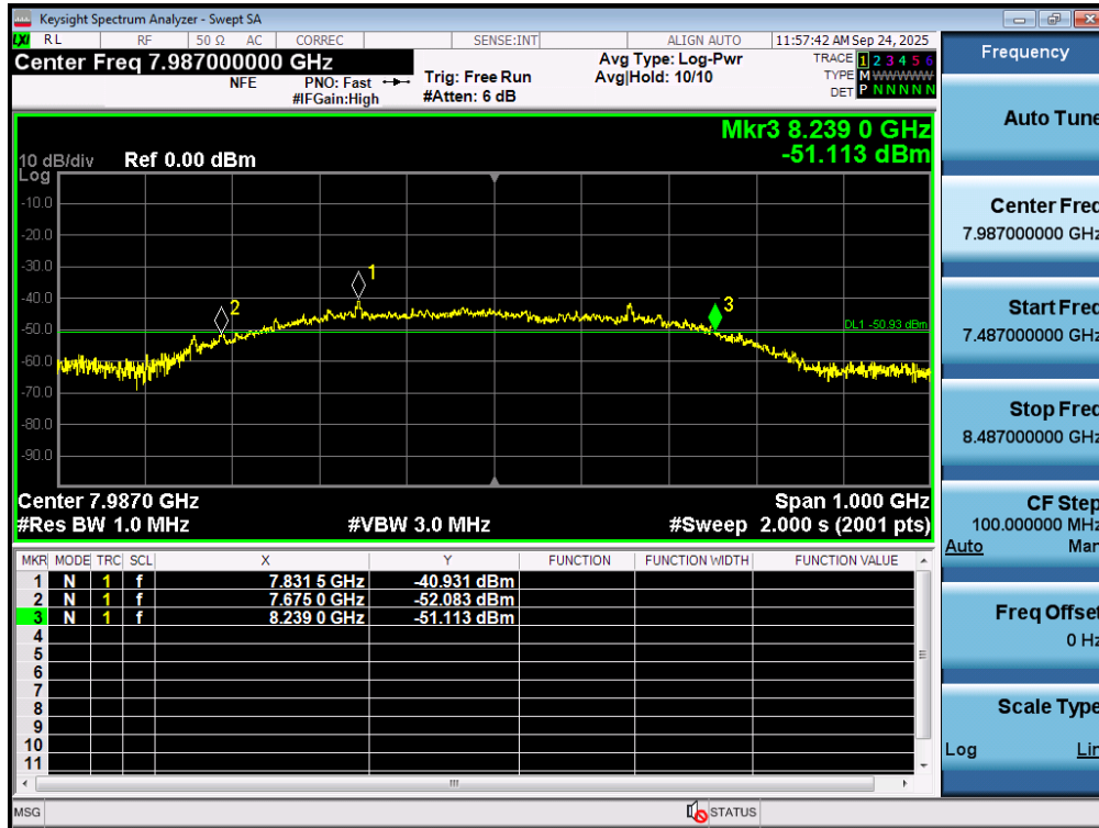
Plot 7-17. 10dBc Bandwidth – CH.9 – SP1 – Preamble 9
