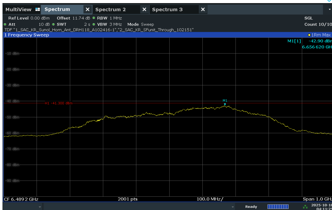
Plot 7-34. UWB Average Power Measurement - CH.5 – BPRF
