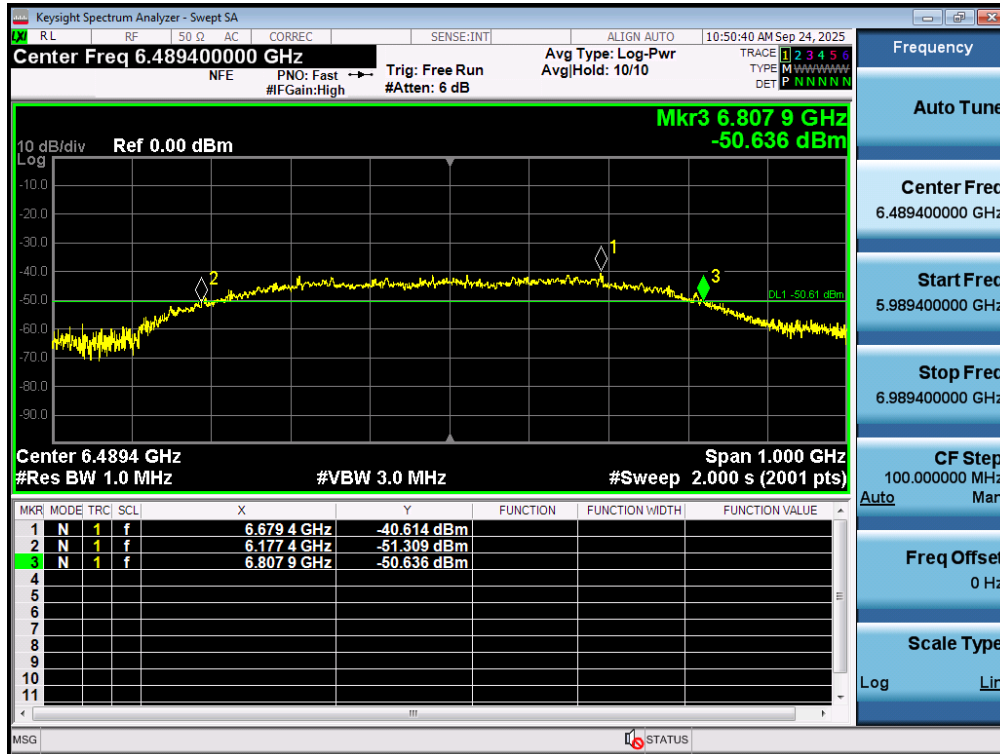
Plot 7-11. 10dBc Bandwidth – CH.5 – SP1 – Preamble 12
