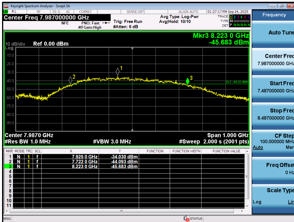
Plot 7-30. 10dBc Bandwidth - CH.9 - SP3 - Preamble 27
