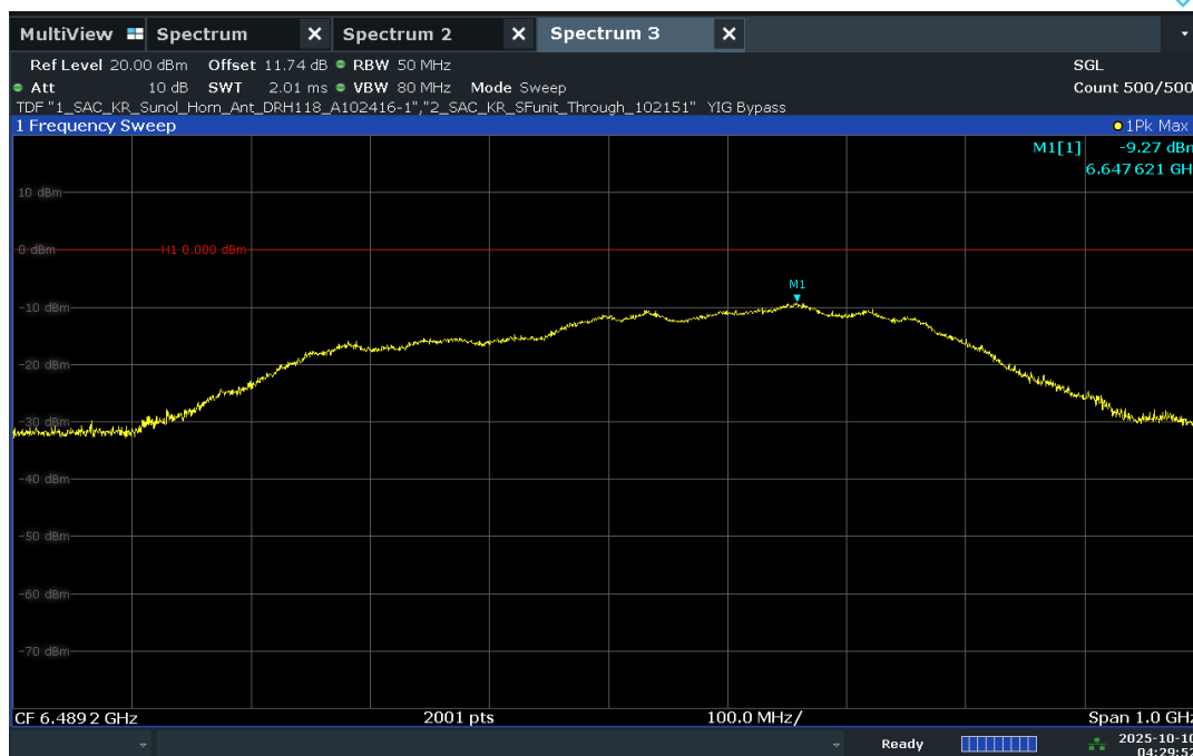
Plot 7-36. UWB Peak Power Measurement - CH.5 – HPRF
