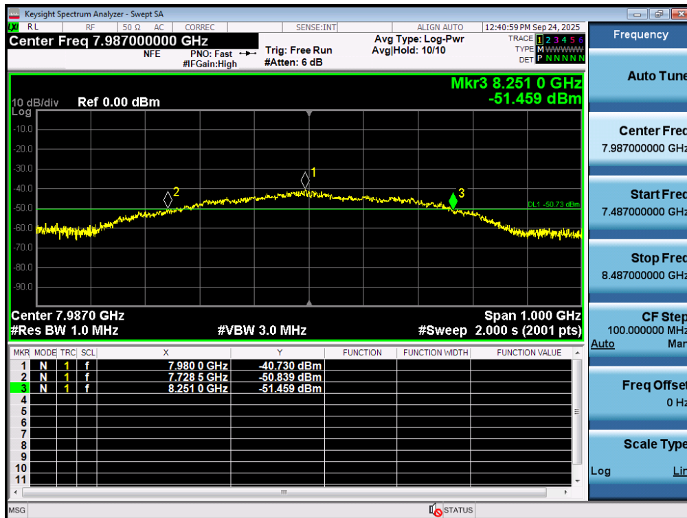
Plot 7-22. 10dBc Bandwidth – CH.9 - SP0 – Preamble 11
