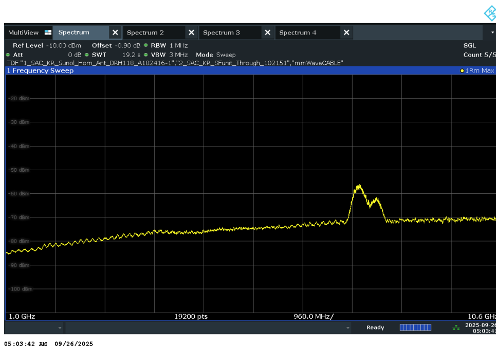
Plot 7-45. Radiated Spurious Pre-Scan 1000 - 10600 MHz - CH.9
