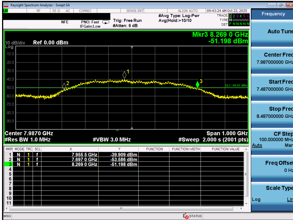
Plot 7-21. 10dBc Bandwidth – CH.9 – SP3 – Preamble 10
