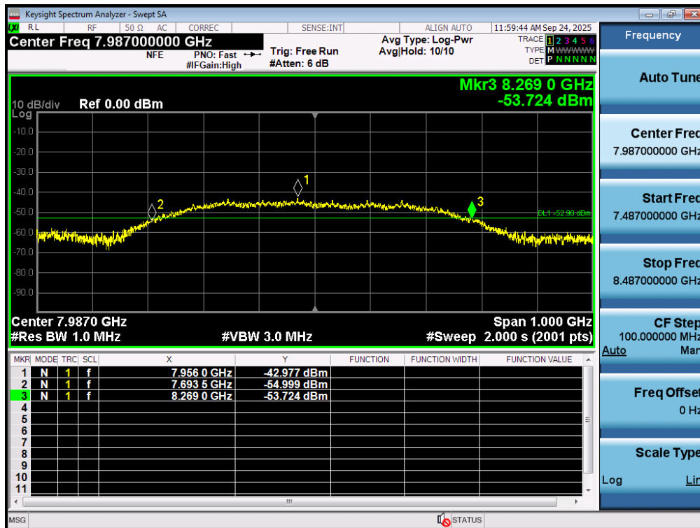
Plot 7-18. 10dBc Bandwidth – CH.9 – SP3 – Preamble 9
