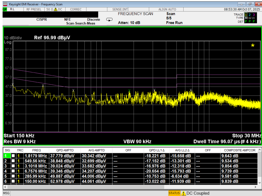
Plot 7-55. Line Conducted Plot (N) – CH 9
