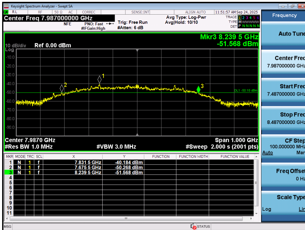
Plot 7-16. 10dBc Bandwidth – CH.9 - SP0 – Preamble 9
