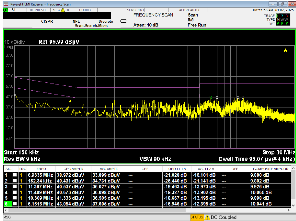
Plot 7-52. Line Conducted Plot (L1) – CH 5
