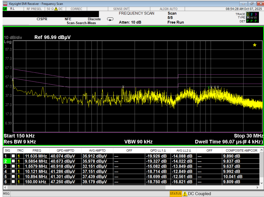
Plot 7-54. Line Conducted Plot (L1) – CH 9
