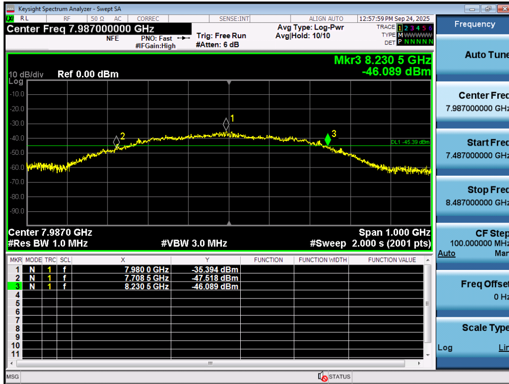
Plot 7-23. 10dBc Bandwidth – CH.9 – SP1 – Preamble 11
