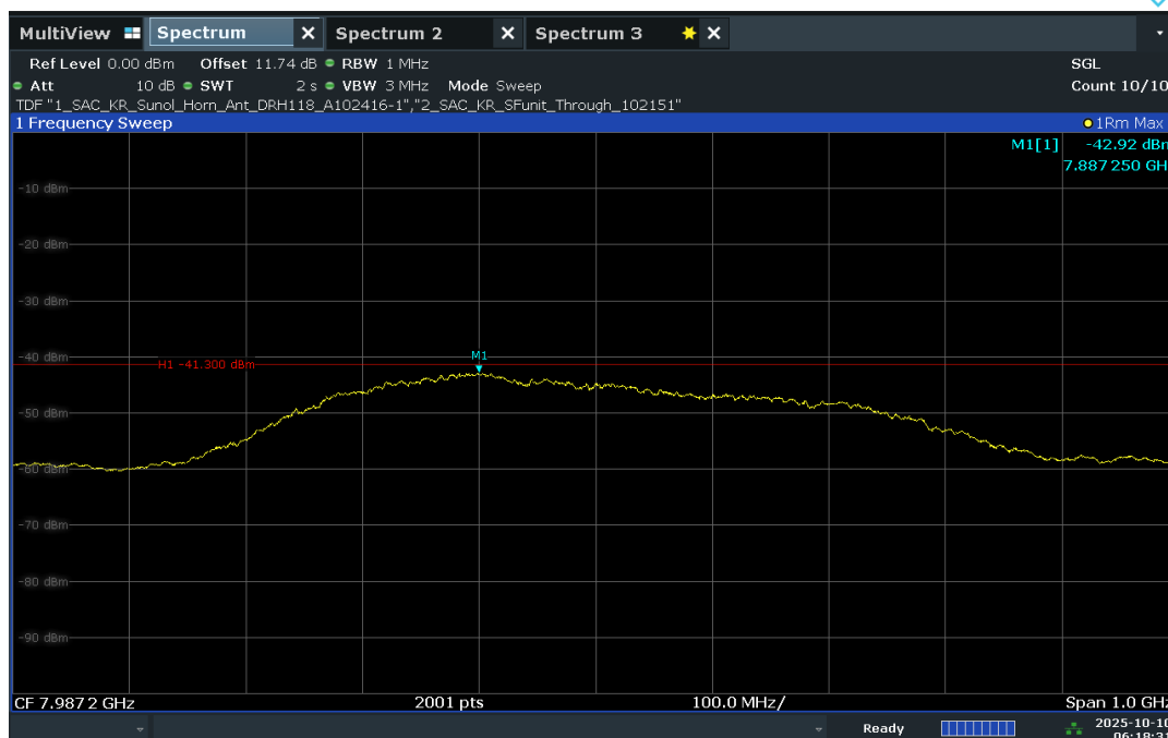
Plot 7-35. UWB Average Power Measurement - CH.9 – BPRF
