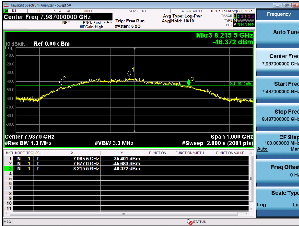
Plot 7-25. 10dBc Bandwidth – CH.9 - SP0 – Preamble 12
