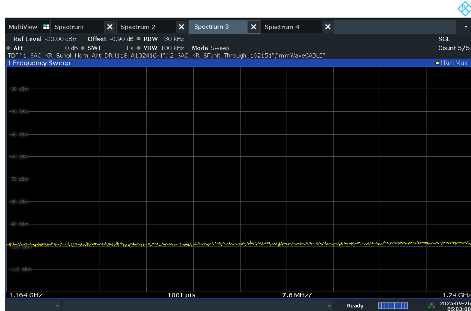
Plot 7-47. Radiated Spurious Pre-Scan 1164 - 1240 MHz - CH.9 – GPS band
