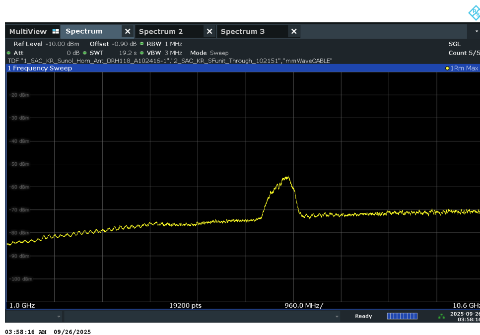
Plot 7-40. Radiated Spurious Pre-Scan 1000 - 10600 MHz - CH.5
