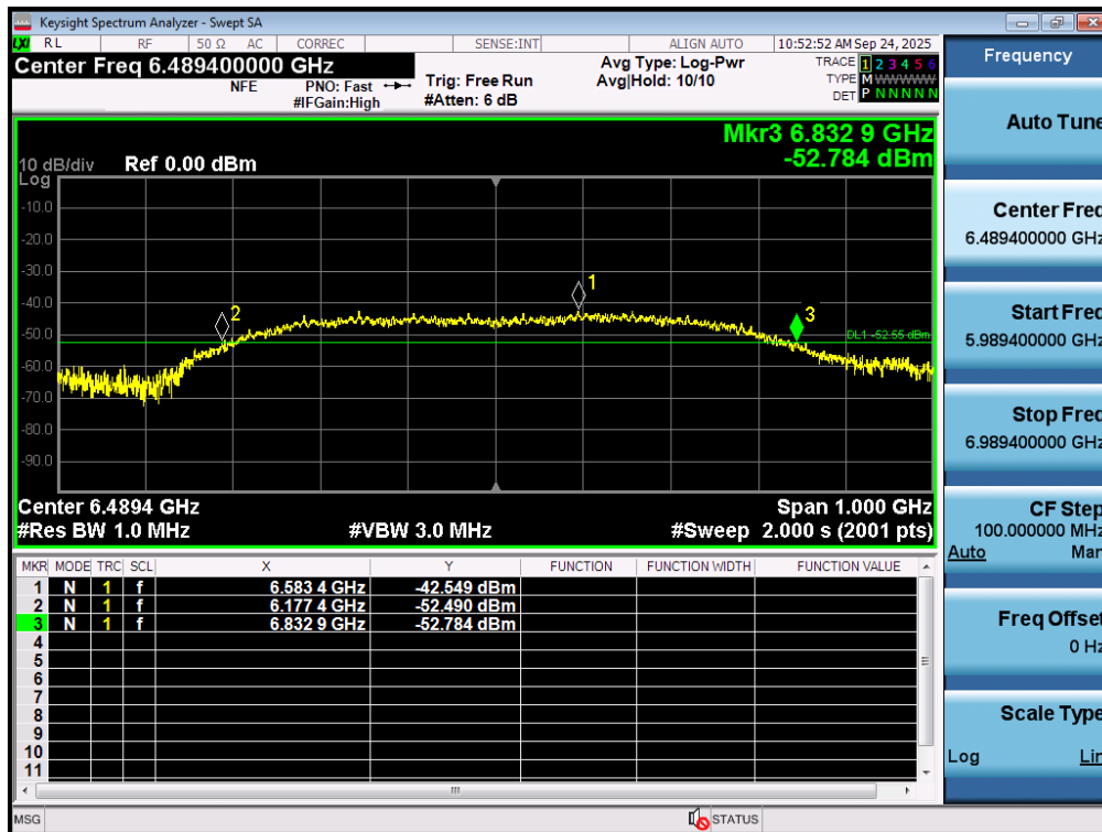
Plot 7-12. 10dBc Bandwidth – CH.5 – SP3 – Preamble 12
