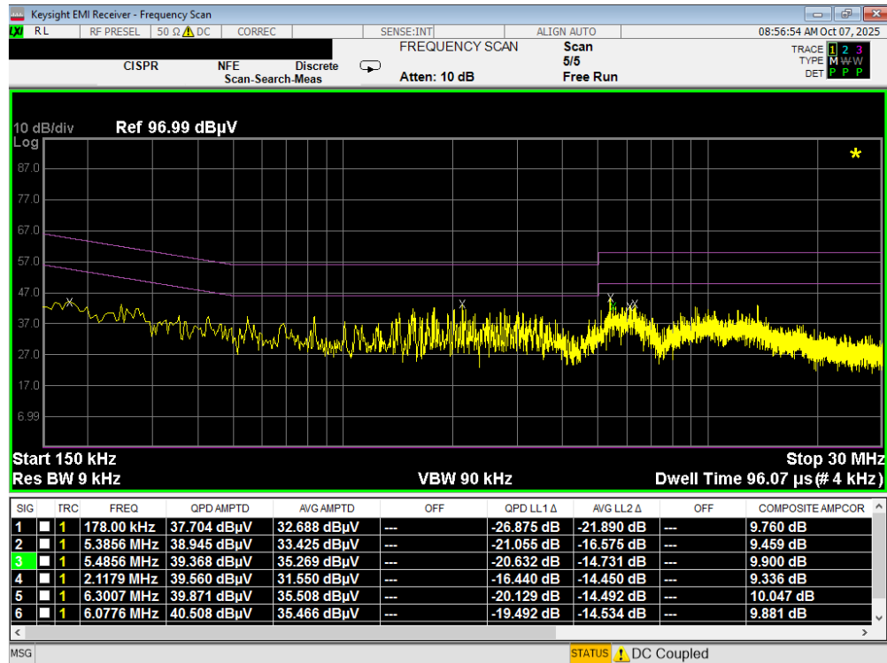
Plot 7-53. Line Conducted Plot (N) – CH 5
