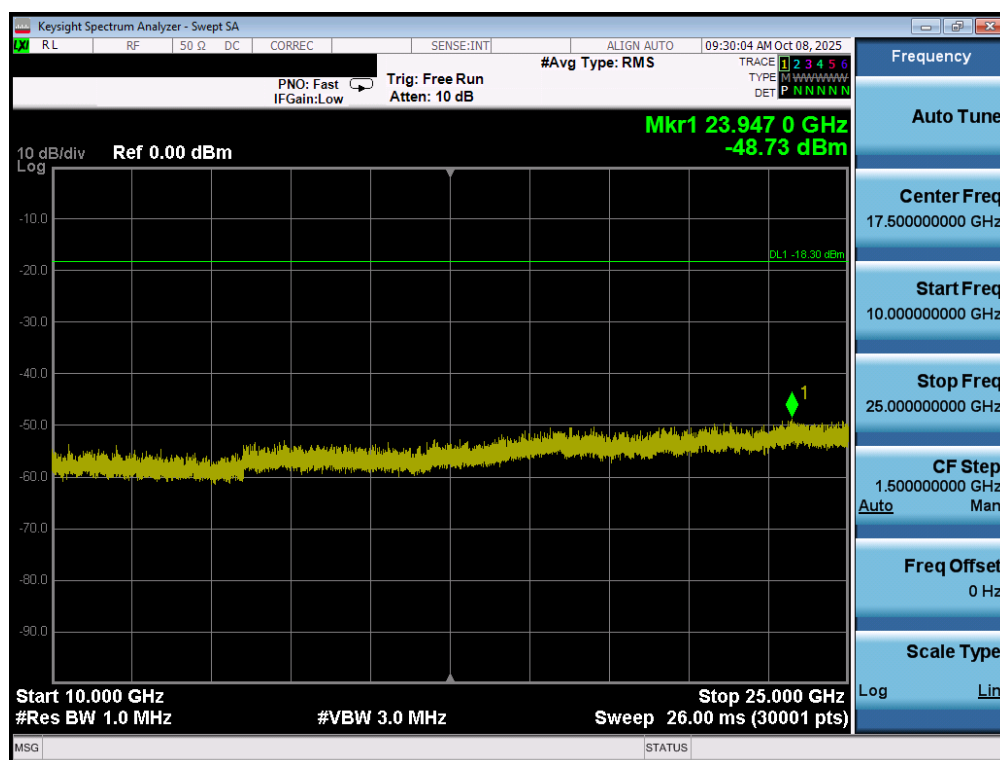
Plot 7-98. Conducted Spurious Plot SISO ANT2 (802.11b – Ch. 1)
