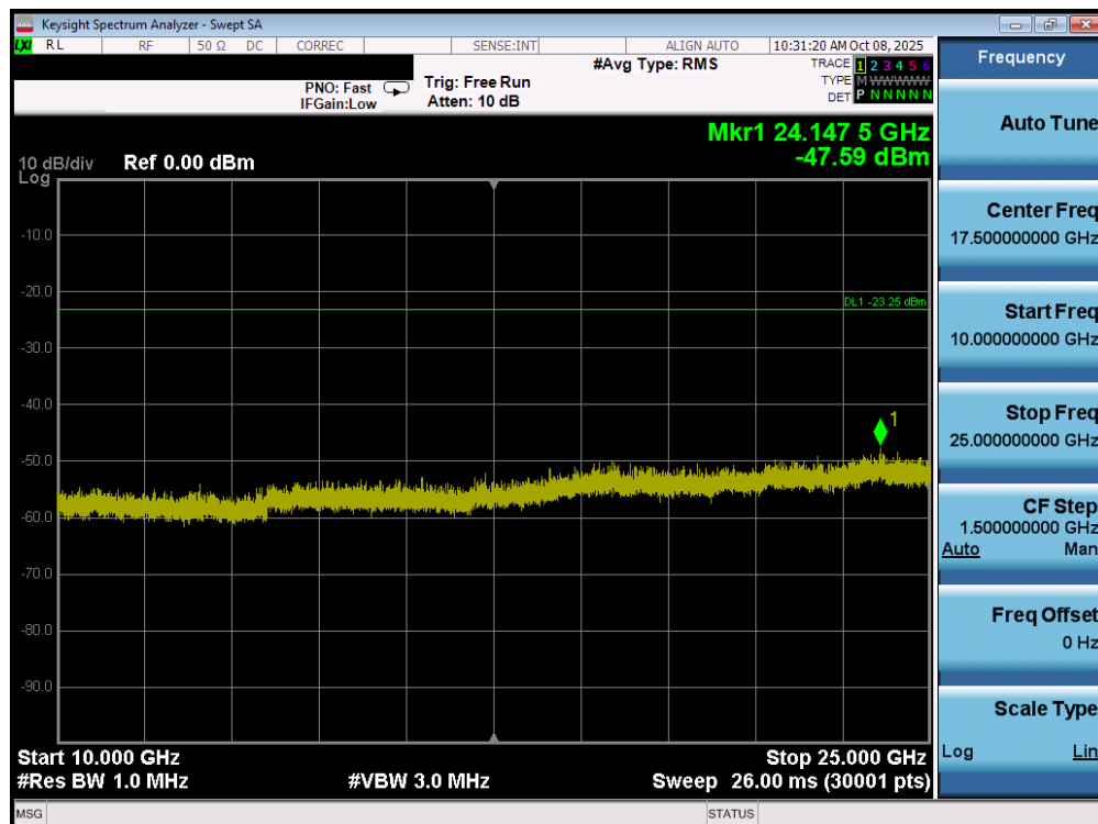
Plot 7-56. Conducted Spurious Plot MIMO ANT1 (802.11ax/be OFDMA – 242 Tones – Ch. 1)
