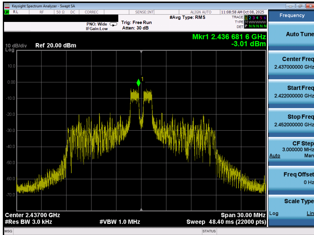
Plot 7-20. Power Spectral Density Plot MIMO ANT2 (802.11ax/be OFDMA – 26 Tones – Ch. 6)
