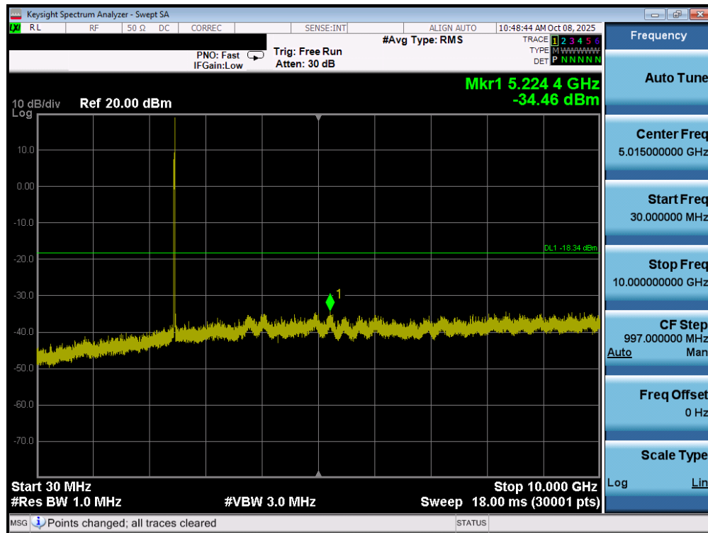
Plot 7-53. Conducted Spurious Plot MIMO ANT1 (802.11ax/be OFDMA – 26 Tones – Ch. 11)
