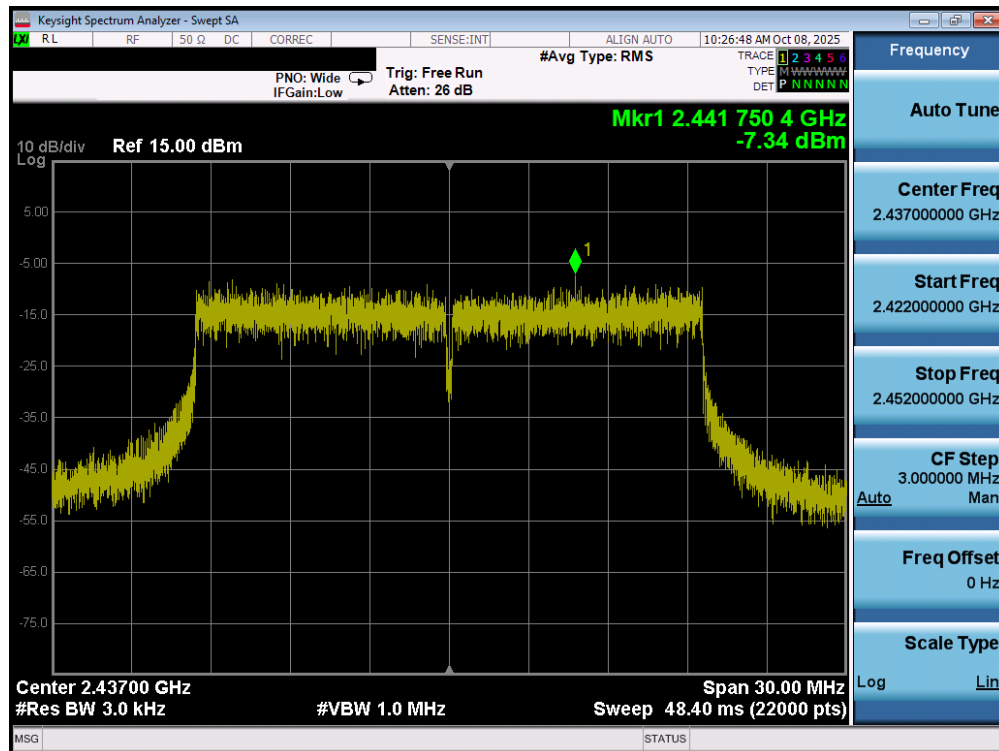
Plot 7-17. Power Spectral Density Plot MIMO ANT1 (802.11ax/be OFDMA – 242 Tones – Ch. 6)
