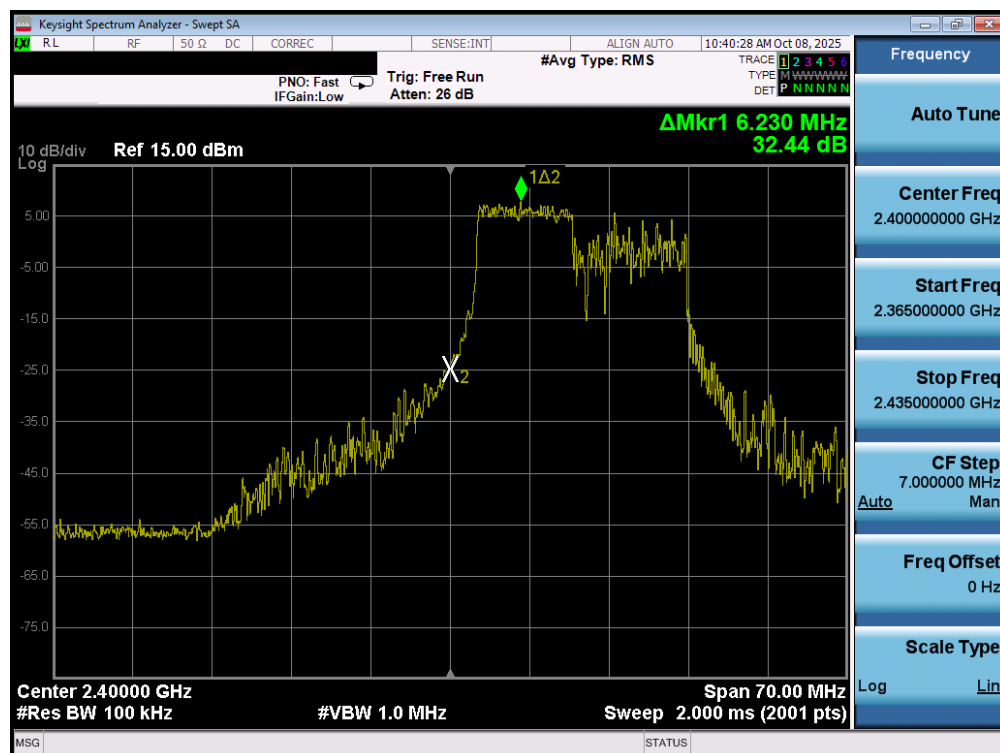
Plot 7-29. Band Edge Plot MIMO ANT1 (802.11be OFDMA – 106+26 Tones – Ch. 1)
