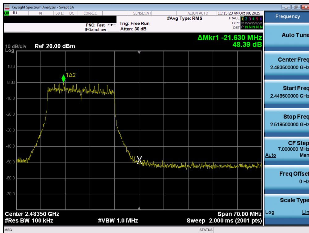
Plot 7-47. Band Edge Plot MIMO ANT2 (802.11ax/be OFDMA – 242 Tones – Ch. 12)
