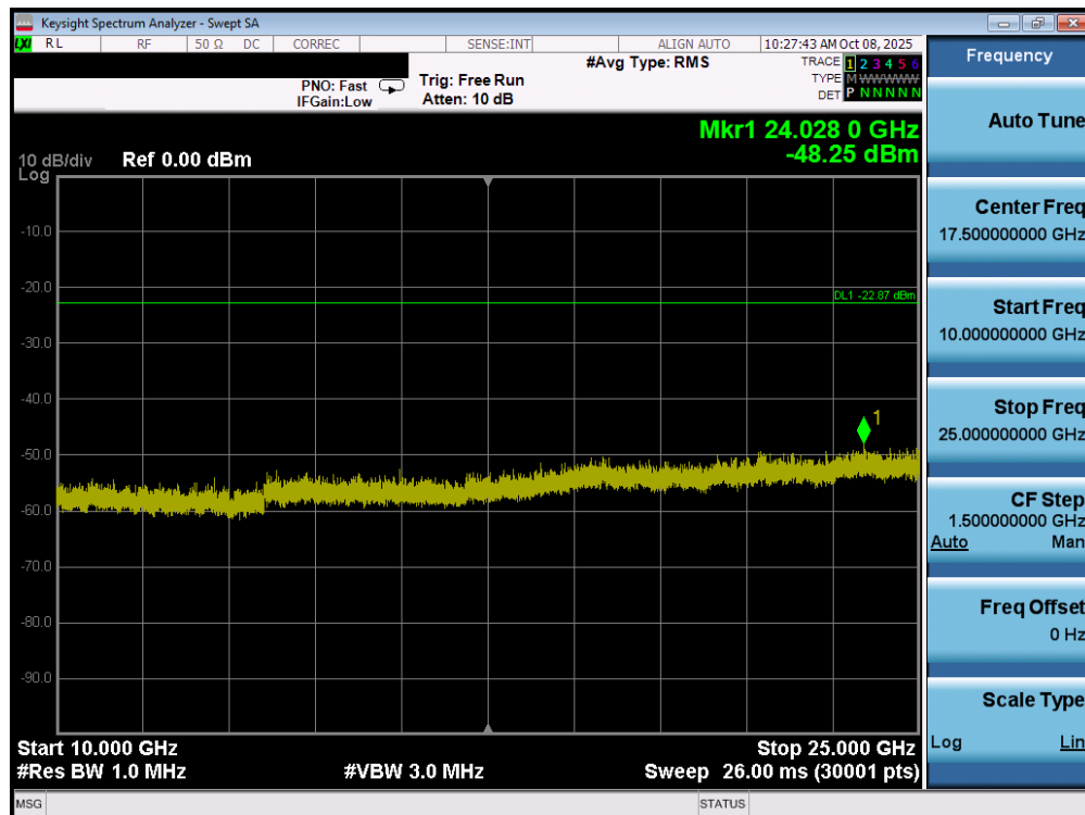
Plot 7-58. Conducted Spurious Plot MIMO ANT1 (802.11ax/be OFDMA – 242 Tones – Ch. 6)
