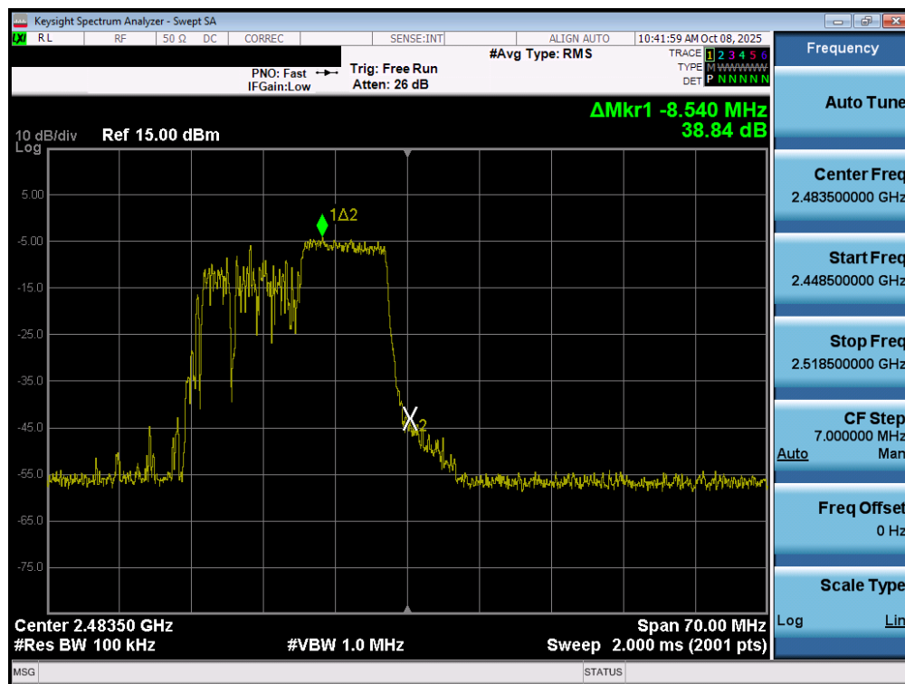
Plot 7-28. Band Edge Plot MIMO ANT1 (802.11ax/be OFDMA – 106 Tones – Ch. 13)
