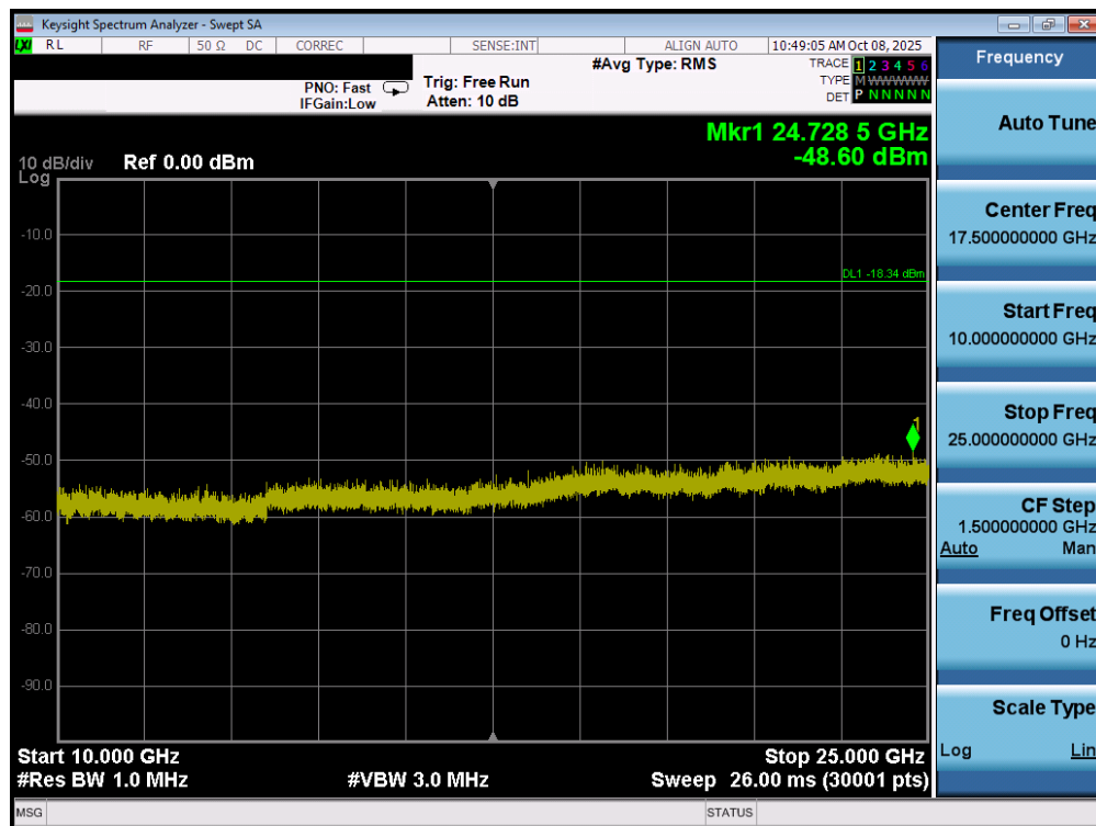
Plot 7-54. Conducted Spurious Plot MIMO ANT1 (802.11ax/be OFDMA – 26 Tones – Ch. 11)
