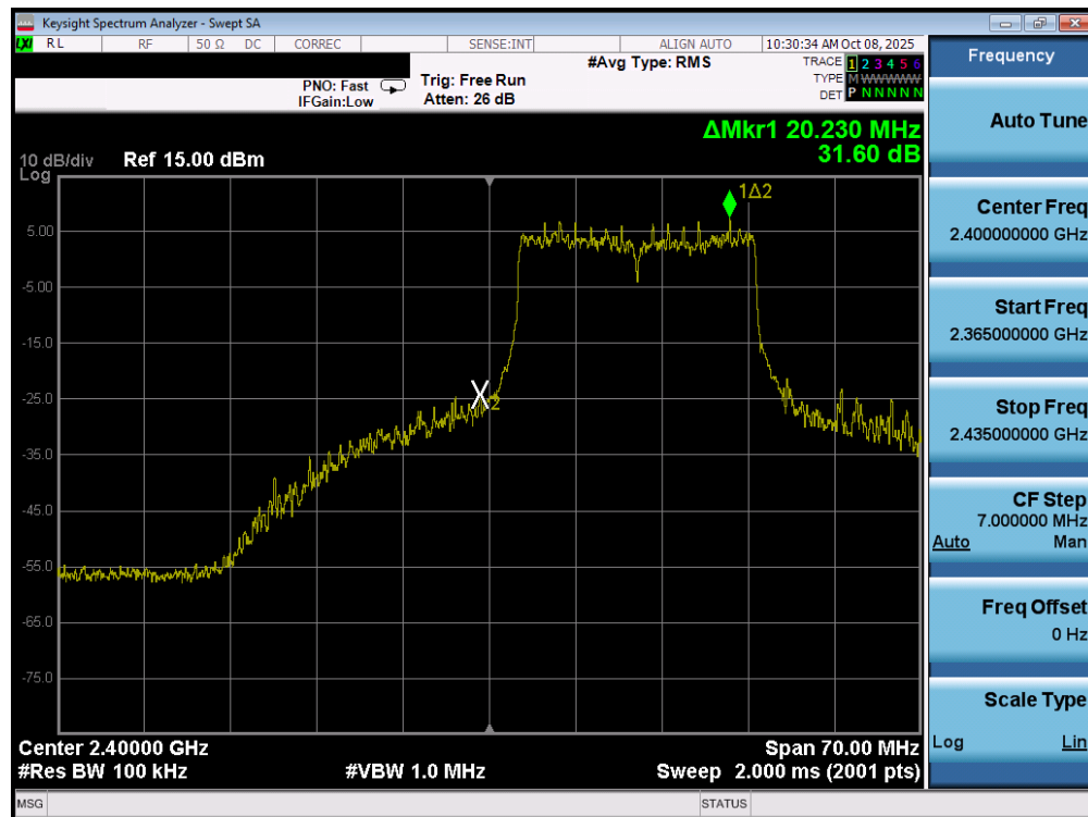
Plot 7-33. Band Edge Plot MIMO ANT1 (802.11ax/be OFDMA – 242 Tones – Ch. 1)
