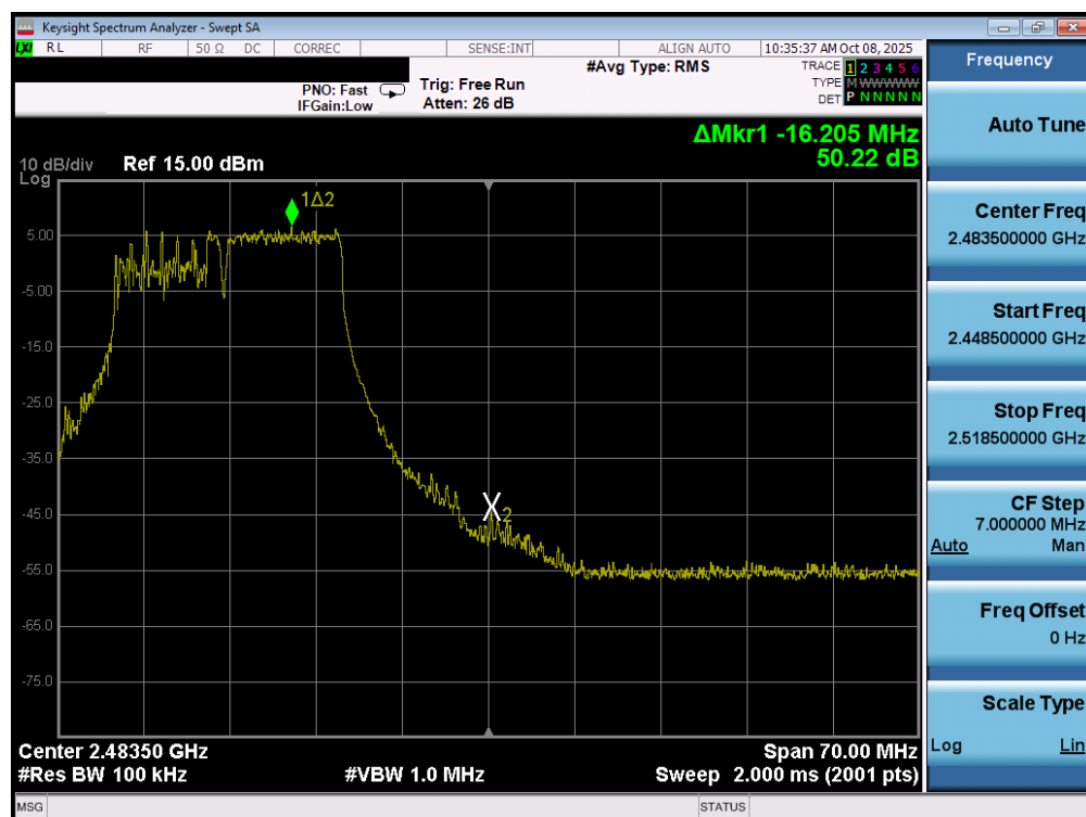
Plot 7-30. Band Edge Plot MIMO ANT1 (802.11be OFDMA – 106+26 Tones – Ch. 11)
