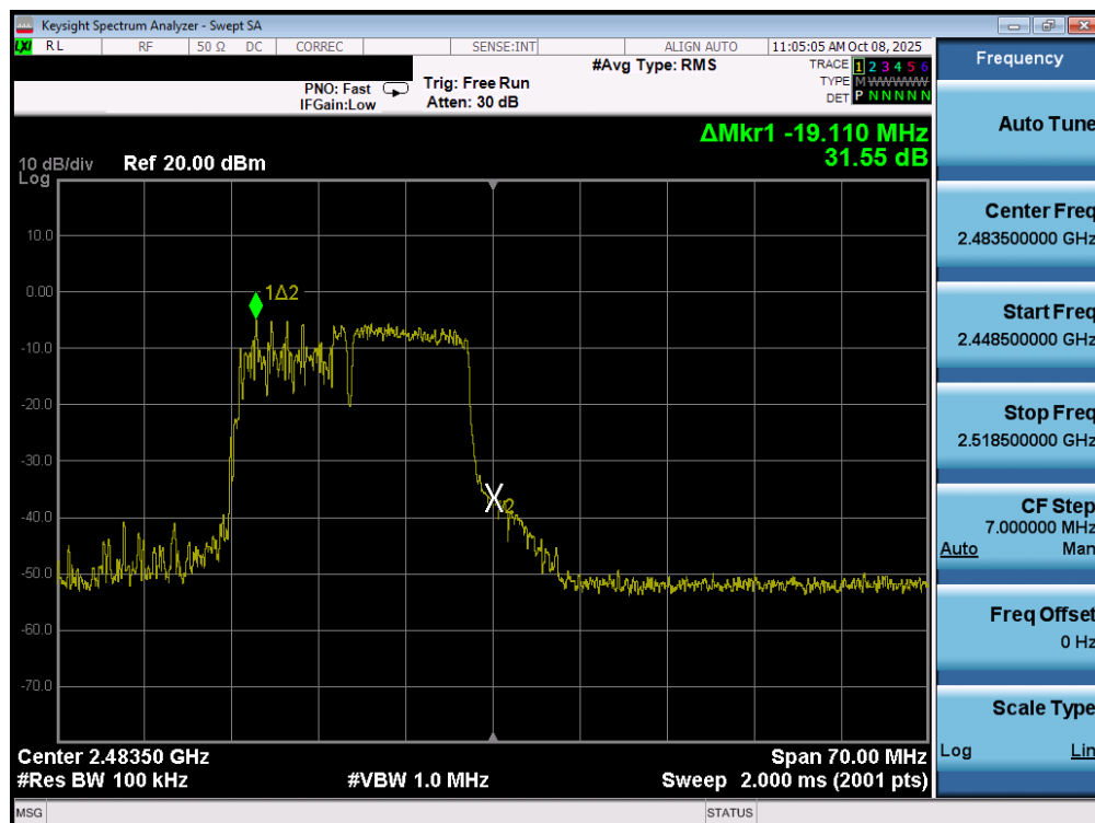
Plot 7-44. Band Edge Plot MIMO ANT2 (802.11be OFDMA – 106+26 Tones – Ch. 11)
