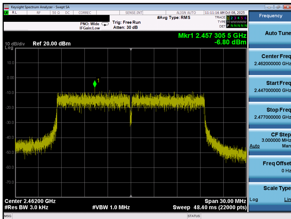
Plot 7-24. Power Spectral Density Plot MIMO ANT2 (802.11ax/be OFDMA – 242 Tones – Ch. 11)
