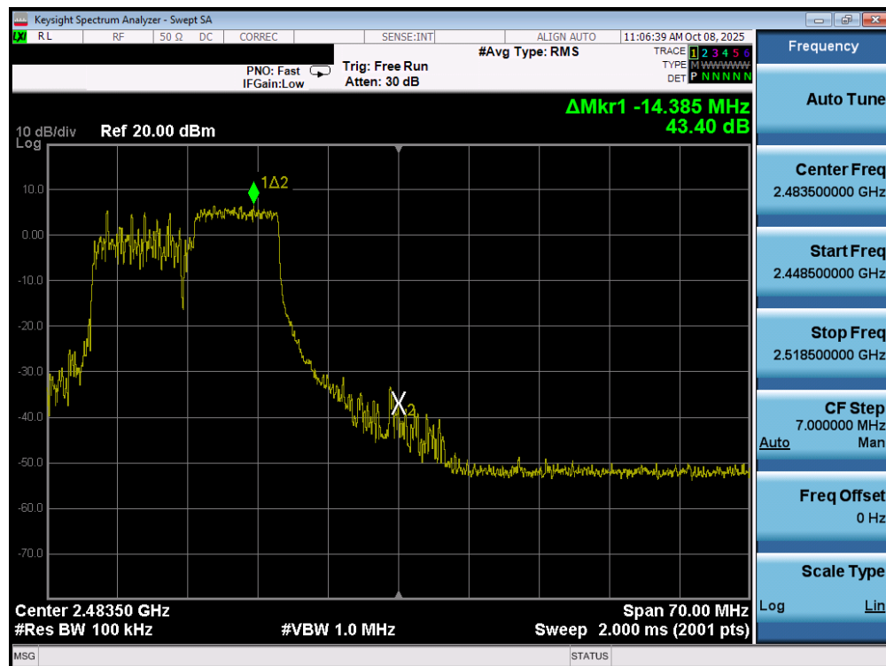
Plot 7-38. Band Edge Plot MIMO ANT2 (802.11ax/be OFDMA – 106 Tones – Ch. 11)
