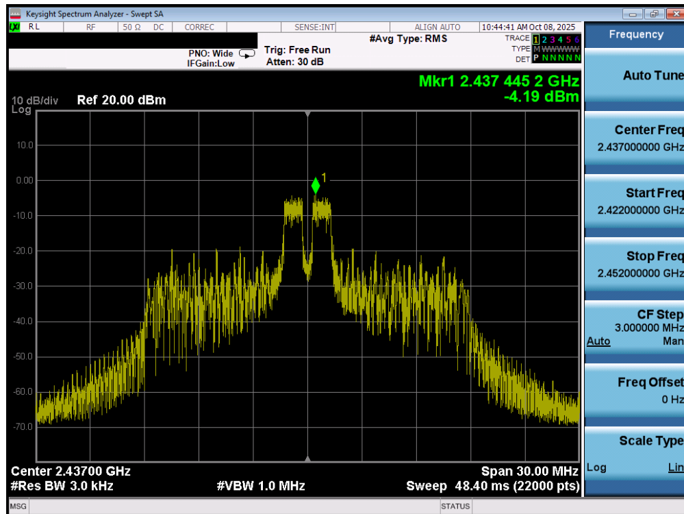
Plot 7-14. Power Spectral Density Plot MIMO ANT1 (802.11ax/be OFDMA – 26 Tones – Ch. 6)
