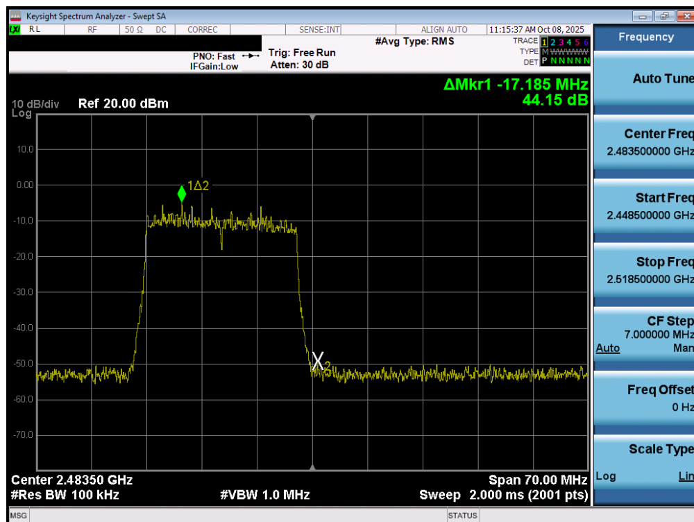
Plot 7-48. Band Edge Plot MIMO ANT2 (802.11ax/be OFDMA – 242 Tones – Ch. 13)
