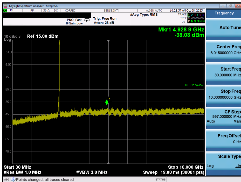
Plot 7-59. Conducted Spurious Plot MIMO ANT1 (802.11ax/be OFDMA – 242 Tones – Ch. 11)
