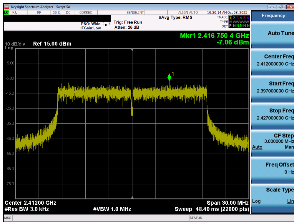
Plot 7-16. Power Spectral Density Plot MIMO ANT1 (802.11ax/be OFDMA – 242 Tones – Ch. 1)
