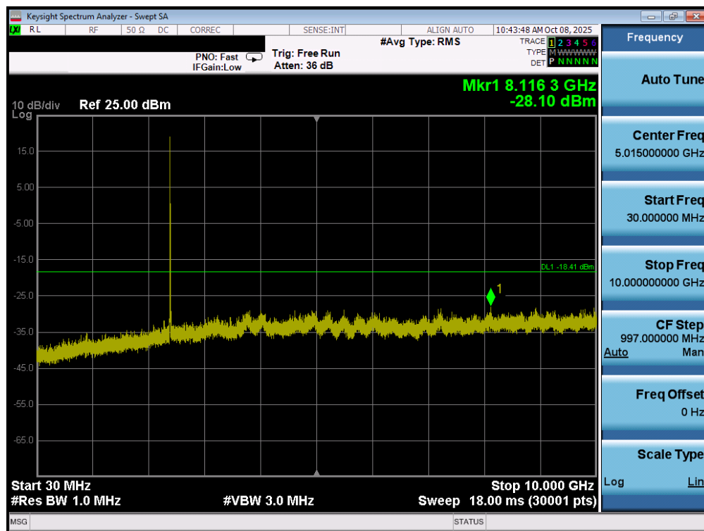
Plot 7-49. Conducted Spurious Plot MIMO ANT1 (802.11ax/be OFDMA – 26 Tones – Ch. 1)
