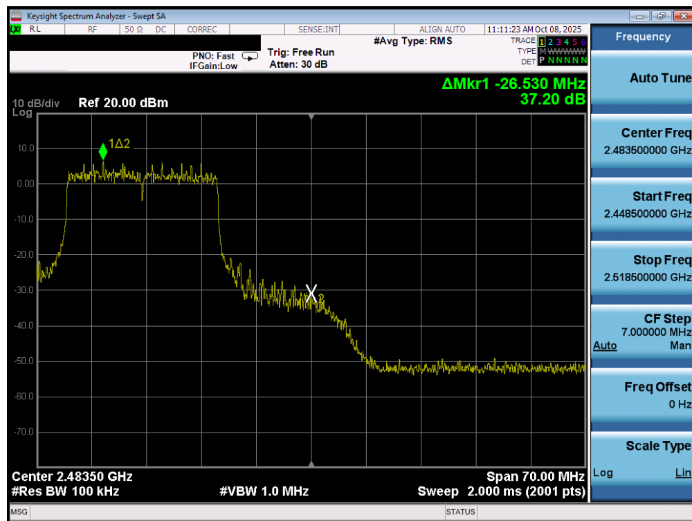
Plot 7-46. Band Edge Plot MIMO ANT2 (802.11ax/be OFDMA – 242 Tones – Ch. 11)
