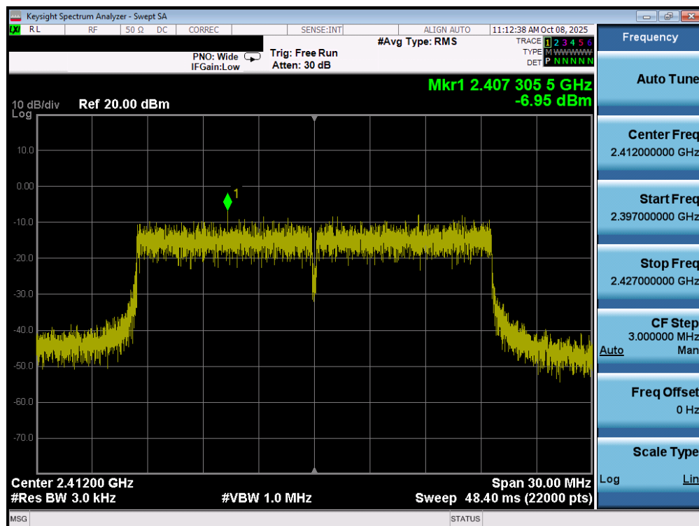
Plot 7-22. Power Spectral Density Plot MIMO ANT2 (802.11ax/be OFDMA – 242 Tones – Ch. 1)
