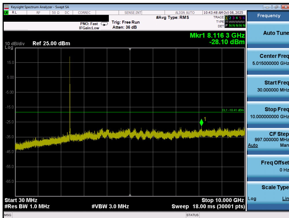
Plot 7-61. Conducted Spurious Plot MIMO ANT1 (802.11ax/be OFDMA – 26 Tones – Ch. 1)
