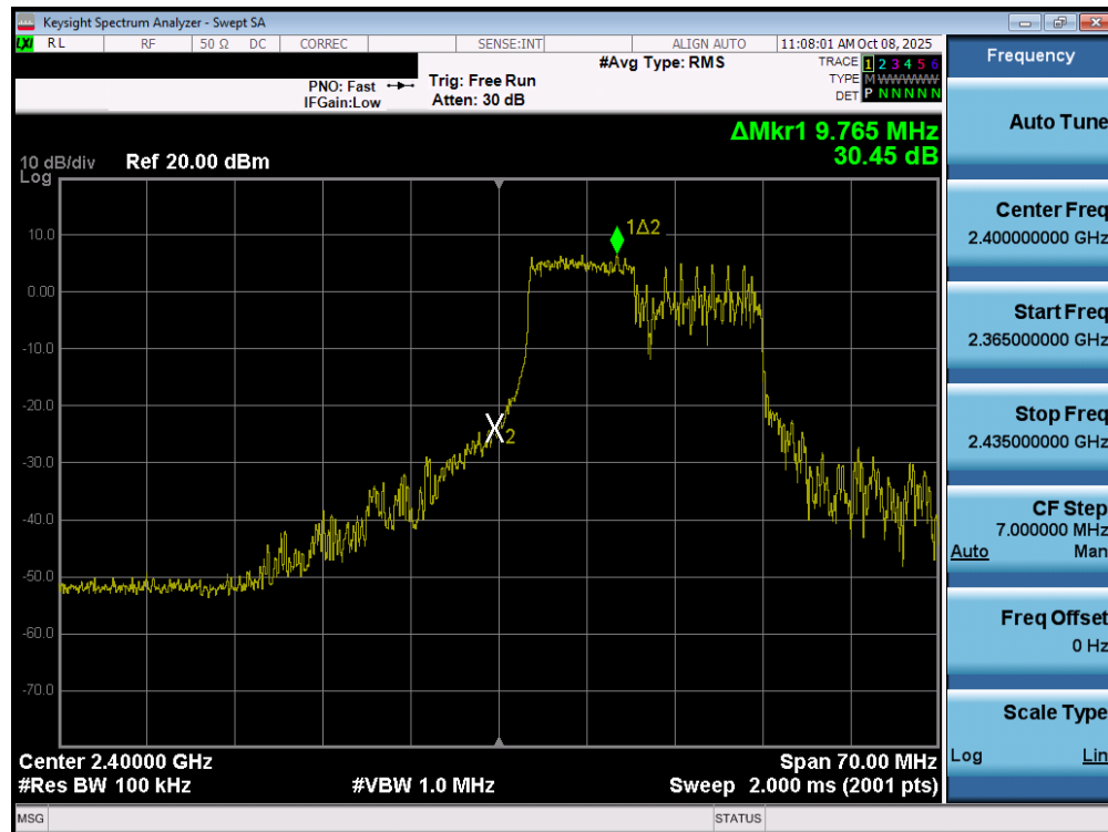
Plot 7-37. Band Edge Plot MIMO ANT2 (802.11ax/be OFDMA – 106 Tones – Ch. 1)
