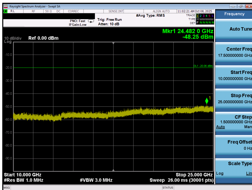
Plot 7-62. Conducted Spurious Plot MIMO ANT2 (802.11ax/be OFDMA – 26 Tones – Ch. 1)
