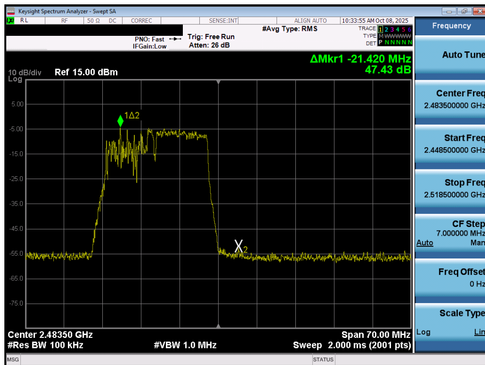
Plot 7-32. Band Edge Plot MIMO ANT1 (802.11be OFDMA – 106+26 Tones – Ch. 13)
