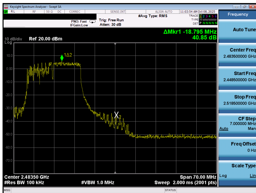
Plot 7-42. Band Edge Plot MIMO ANT2 (802.11be OFDMA – 106+26 Tones – Ch. 11)
