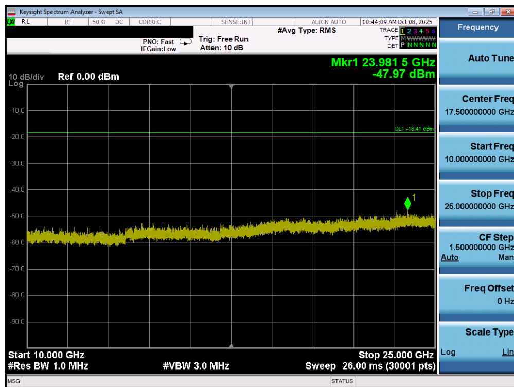
Plot 7-50. Conducted Spurious Plot MIMO ANT1 (802.11ax/be OFDMA – 26 Tones – Ch. 1)
