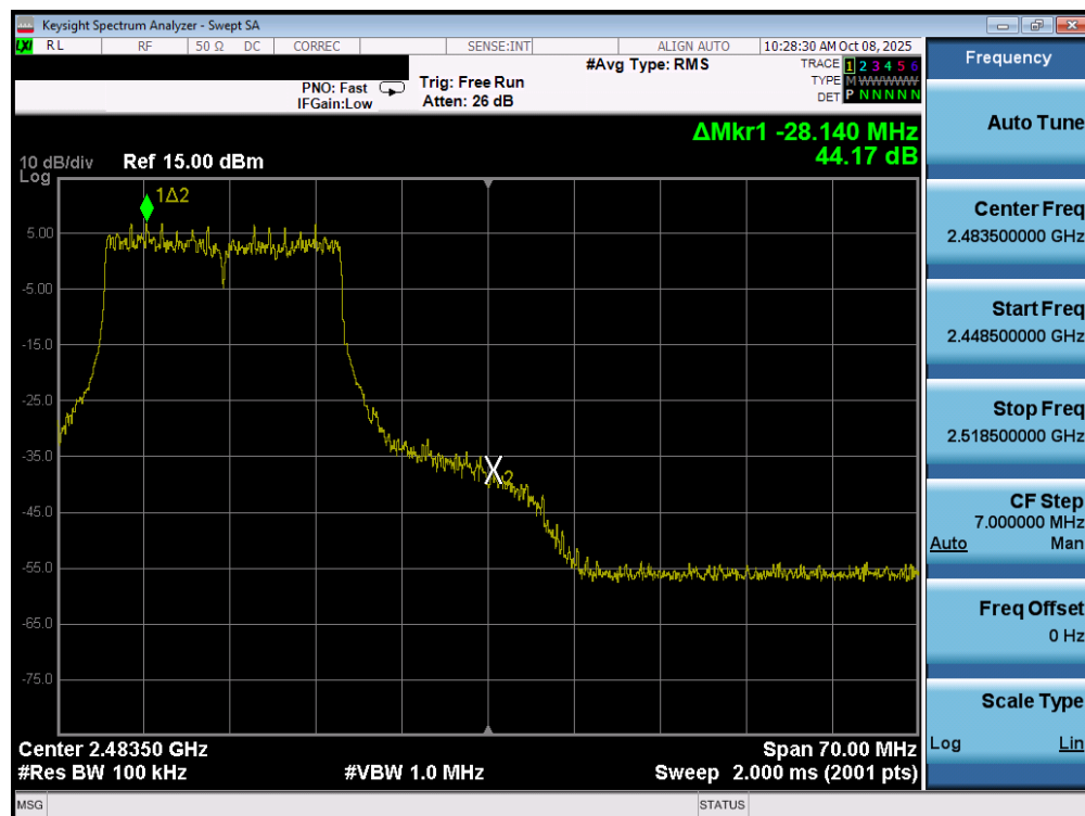
Plot 7-34. Band Edge Plot MIMO ANT1 (802.11ax/be OFDMA – 242 Tones – Ch. 11)
