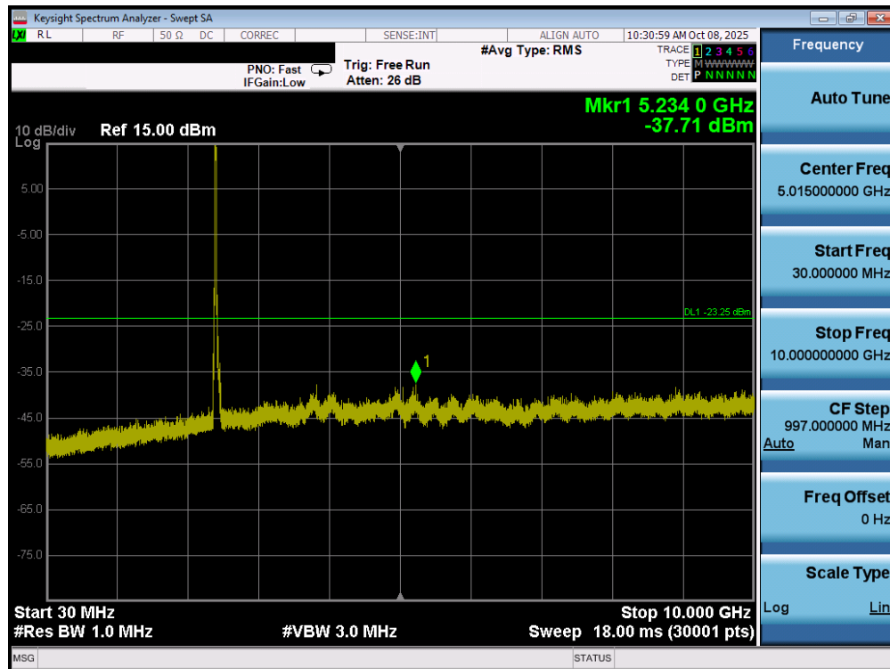
Plot 7-55. Conducted Spurious Plot MIMO ANT1 (802.11ax/be OFDMA – 242 Tones – Ch. 1)
