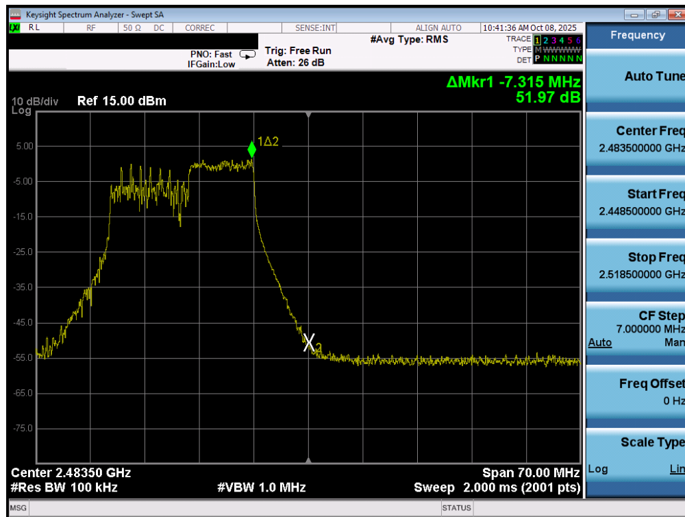
Plot 7-27. Band Edge Plot MIMO ANT1 (802.11ax/be OFDMA – 106 Tones – Ch. 12)
