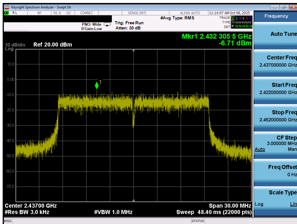
Plot 7-23. Power Spectral Density Plot MIMO ANT2 (802.11ax/be OFDMA – 242 Tones – Ch. 6)
