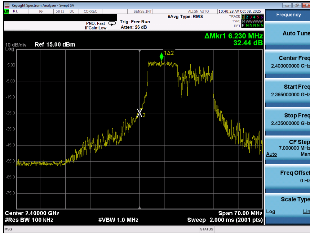
Plot 7-25. Band Edge Plot MIMO ANT1 (802.11ax/be OFDMA – 106 Tones – Ch. 1)
