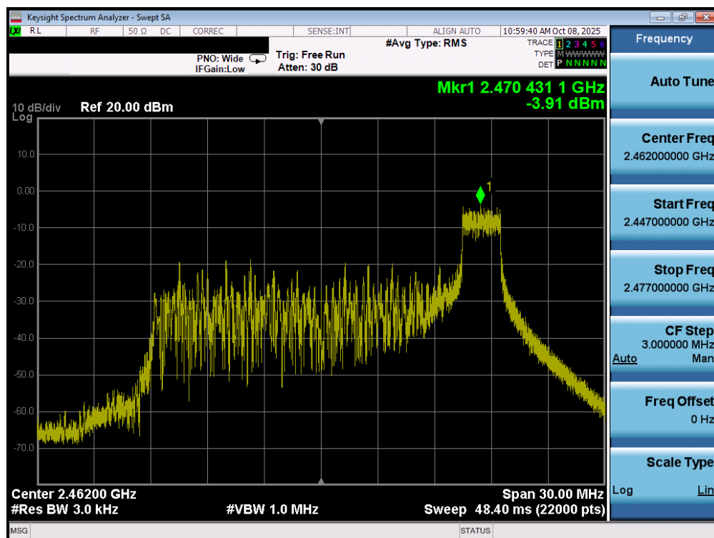
Plot 7-21. Power Spectral Density Plot MIMO ANT2 (802.11ax/be OFDMA – 26 Tones – Ch. 11)
