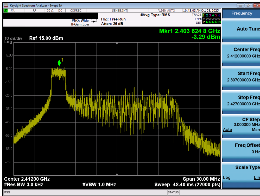
Plot 7-13. Power Spectral Density Plot MIMO ANT1 (802.11ax/be OFDMA – 26 Tones – Ch. 1)
