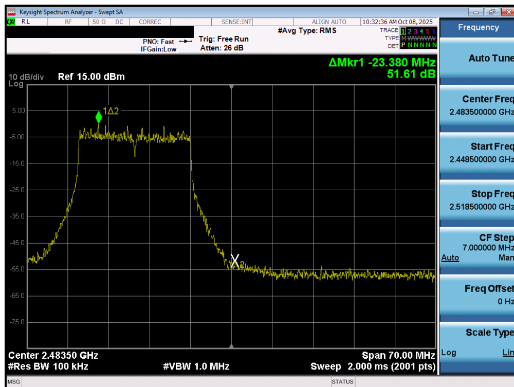
Plot 7-35. Band Edge Plot MIMO ANT1 (802.11ax/be OFDMA – 242 Tones – Ch. 12)
