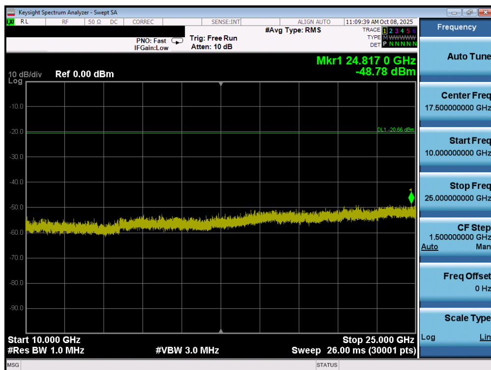
Plot 7-64. Conducted Spurious Plot MIMO ANT2 (802.11ax/be OFDMA – 26 Tones – Ch. 6)
