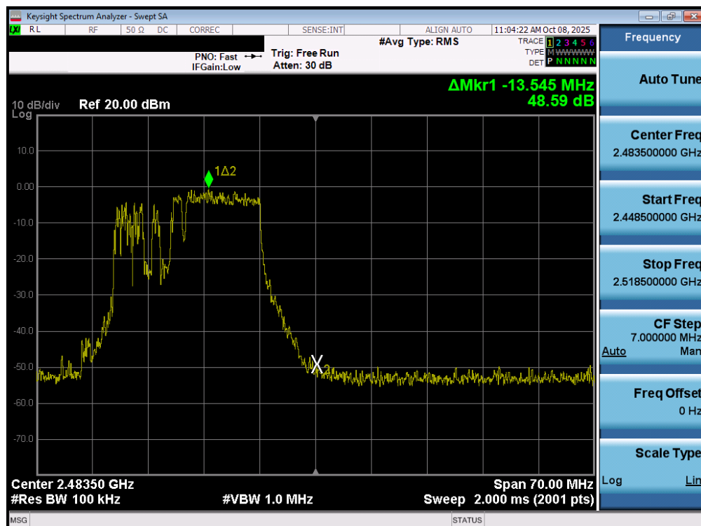
Plot 7-43. Band Edge Plot MIMO ANT2 (802.11be OFDMA – 106+26 Tones – Ch. 11)
