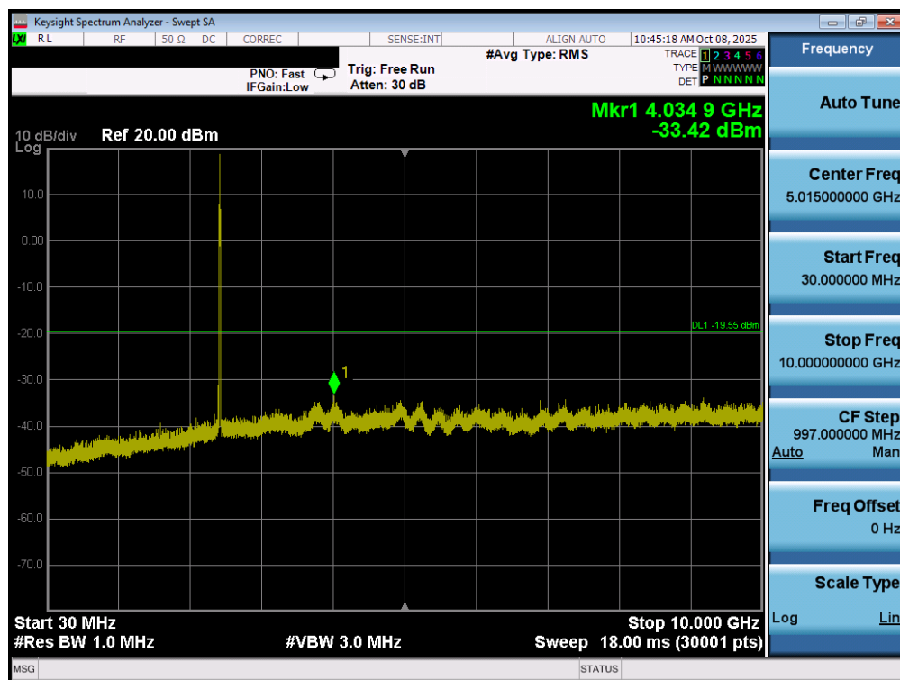
Plot 7-51. Conducted Spurious Plot MIMO ANT1 (802.11ax/be OFDMA – 26 Tones – Ch. 6)
