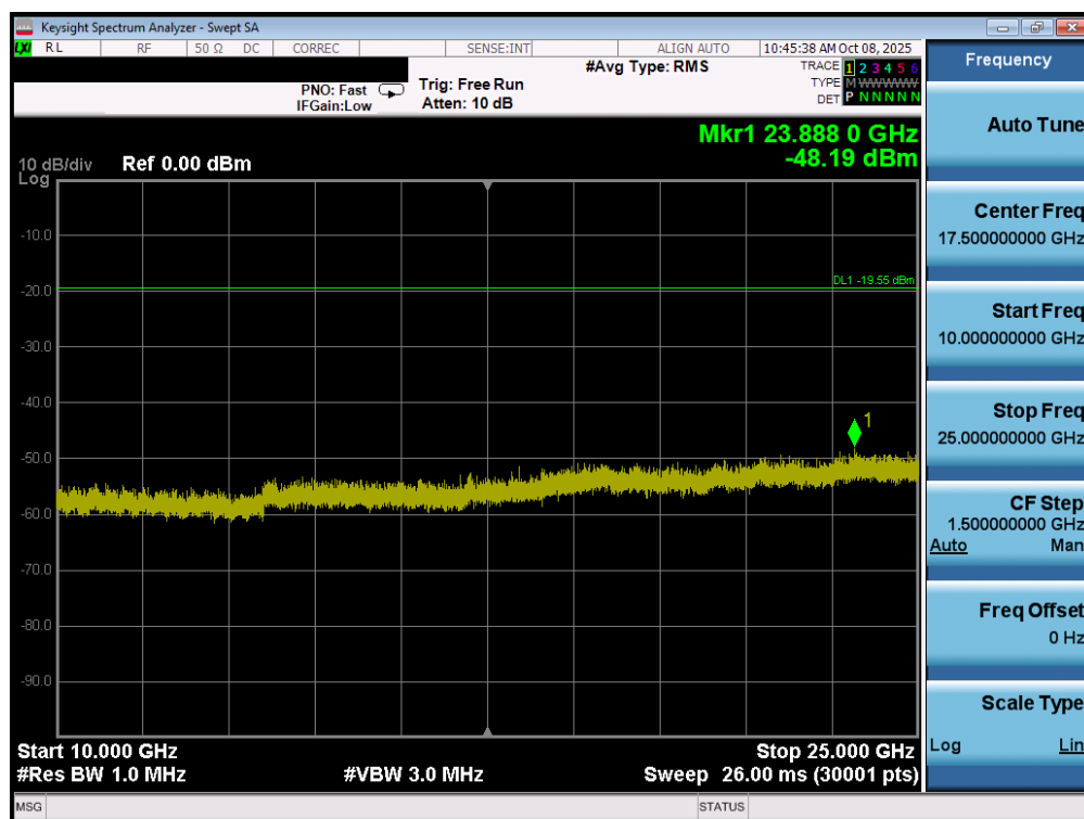
Plot 7-52. Conducted Spurious Plot MIMO ANT1 (802.11ax/be OFDMA – 26 Tones – Ch. 6)
