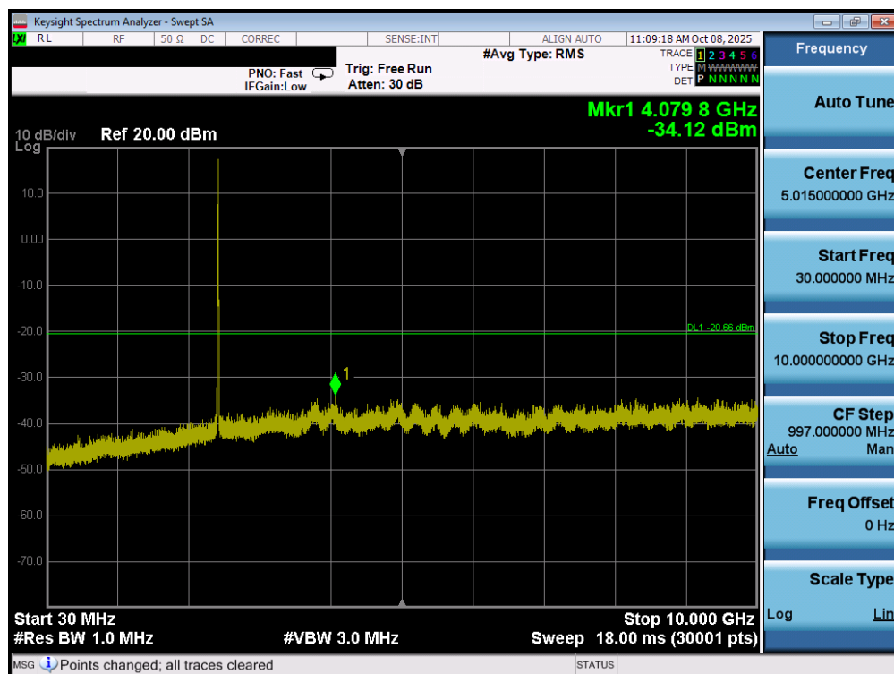
Plot 7-63. Conducted Spurious Plot MIMO ANT2 (802.11ax/be OFDMA – 26 Tones – Ch. 6)
