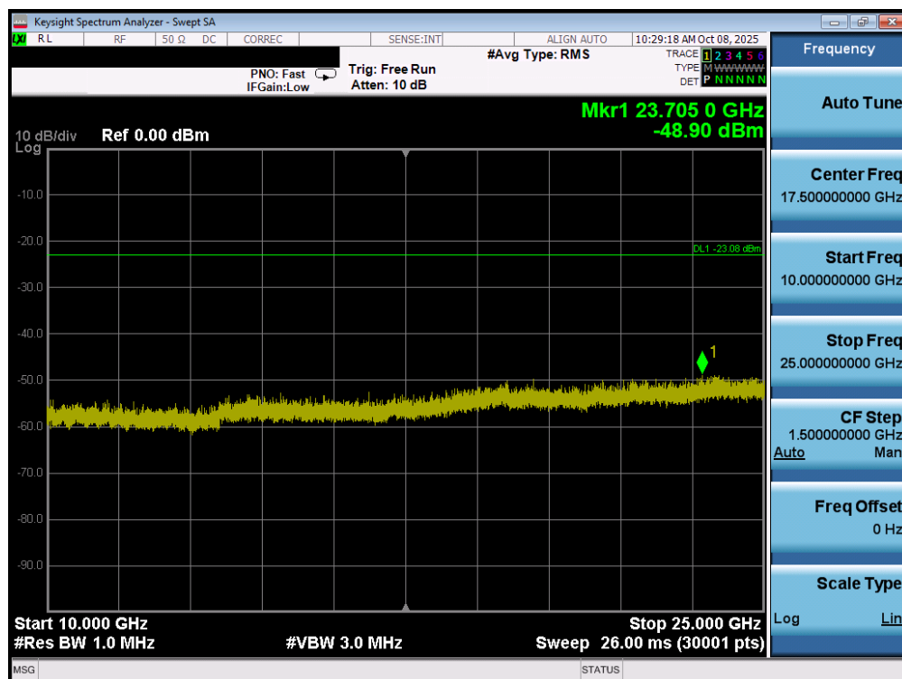
Plot 7-60. Conducted Spurious Plot MIMO ANT1 (802.11ax/be OFDMA – 242 Tones – Ch. 11)
