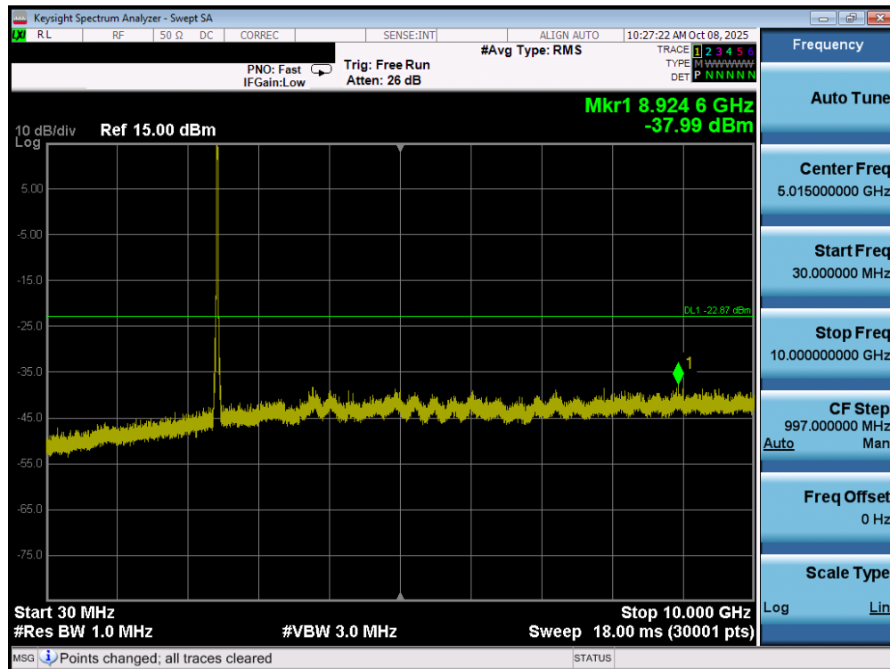
Plot 7-57. Conducted Spurious Plot MIMO ANT1 (802.11ax/be OFDMA – 242 Tones – Ch. 6)
