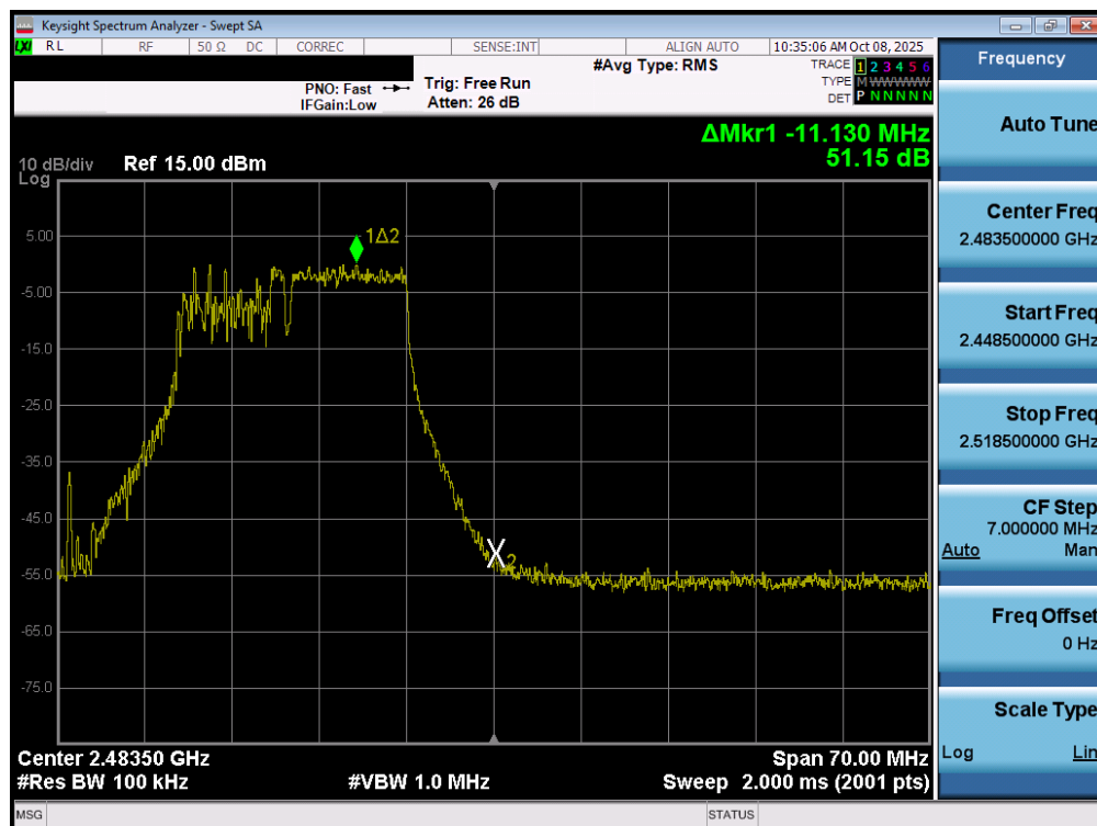
Plot 7-31. Band Edge Plot MIMO ANT1 (802.11be OFDMA – 106+26 Tones – Ch. 12)
