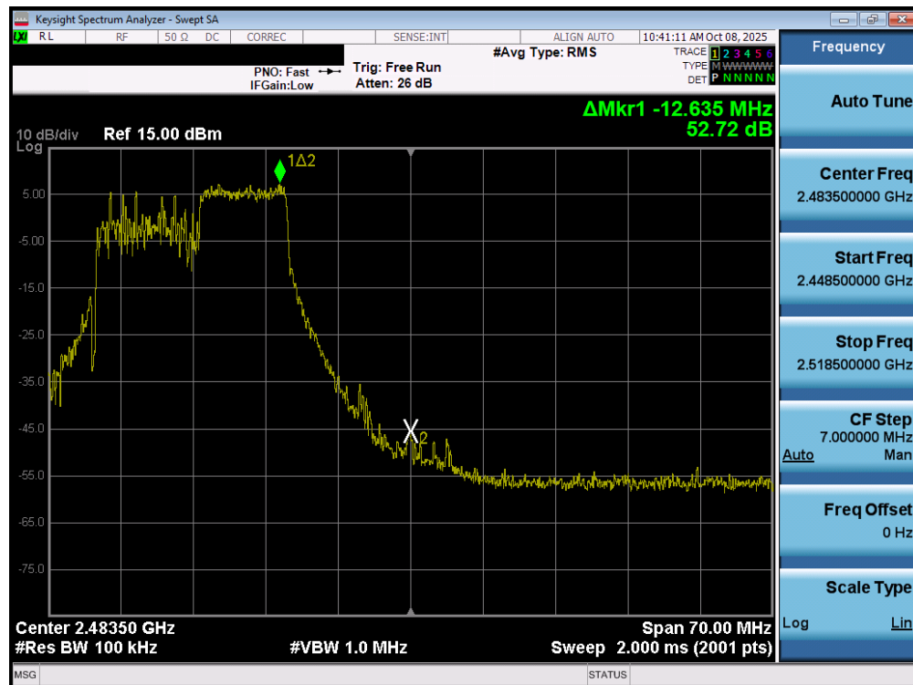
Plot 7-26. Band Edge Plot MIMO ANT1 (802.11ax/be OFDMA – 106 Tones – Ch. 11)
