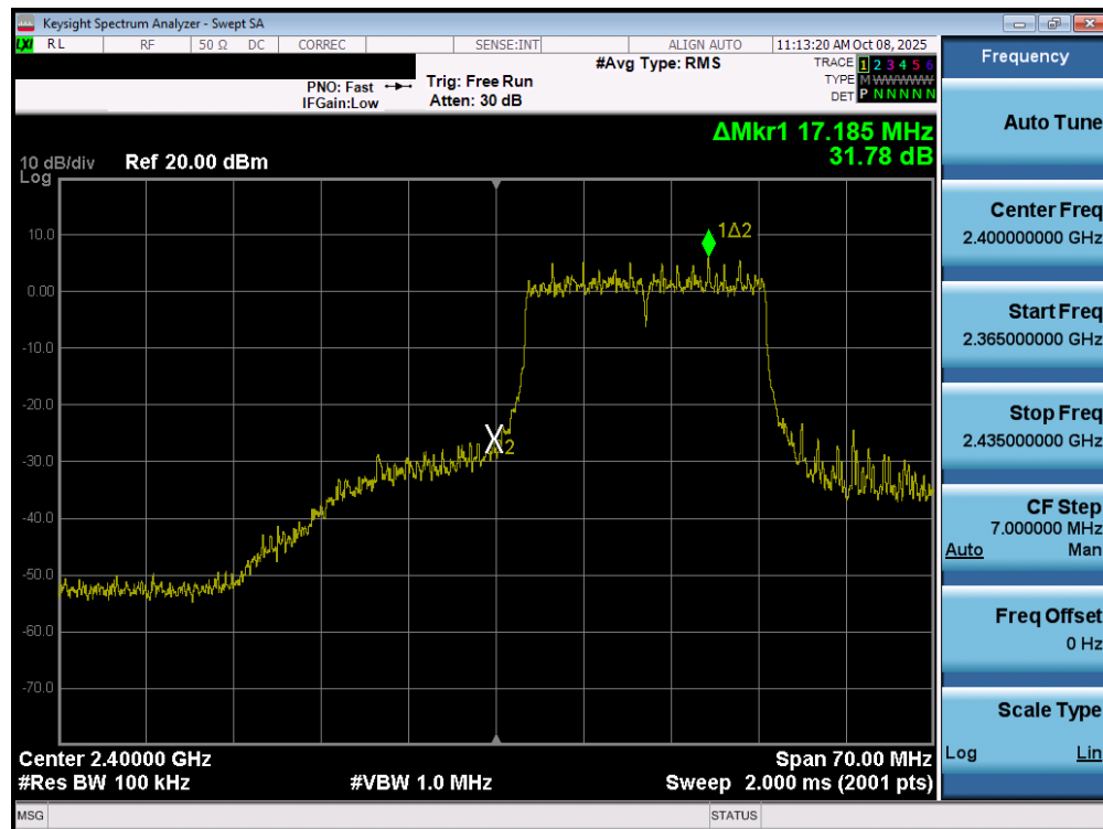
Plot 7-45. Band Edge Plot MIMO ANT2 (802.11ax/be OFDMA – 242 Tones – Ch. 1)
