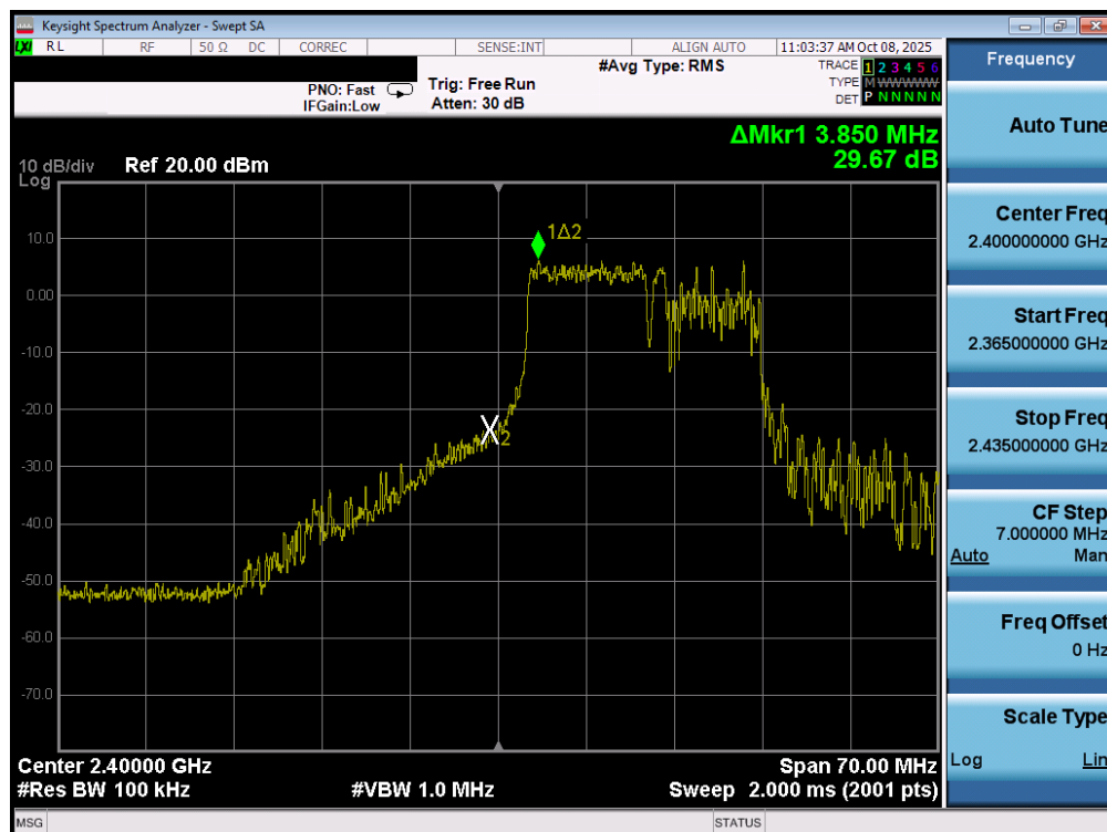
Plot 7-41. Band Edge Plot MIMO ANT2 (802.11be OFDMA – 106+26 Tones – Ch. 1)
