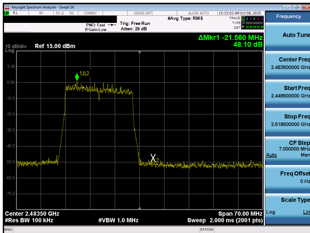
Plot 7-36. Band Edge Plot MIMO ANT1 (802.11ax/be OFDMA – 242 Tones – Ch. 13)
