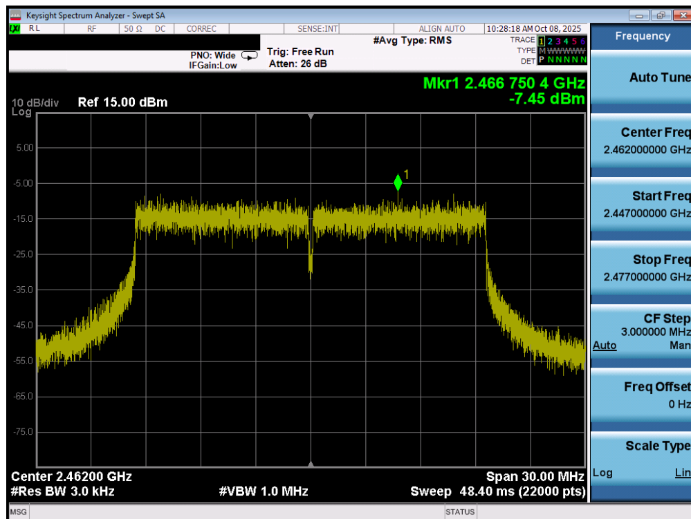
Plot 7-18. Power Spectral Density Plot MIMO ANT1 (802.11ax/be OFDMA – 242 Tones – Ch. 11)
