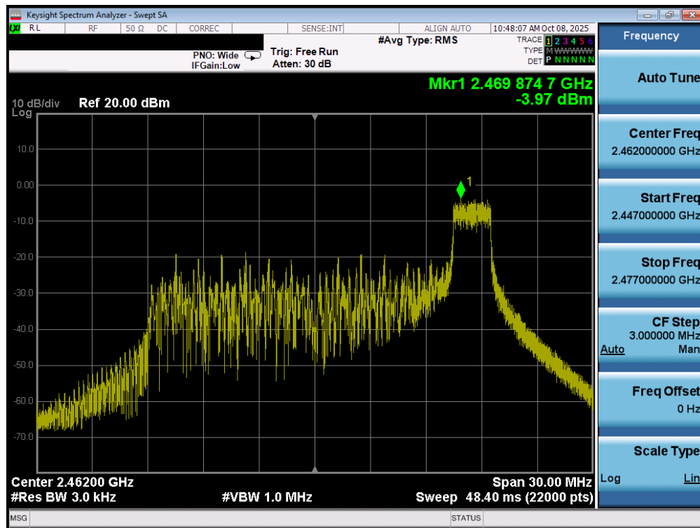
Plot 7-15. Power Spectral Density Plot MIMO ANT1 (802.11ax/be OFDMA – 26 Tones – Ch. 11)
