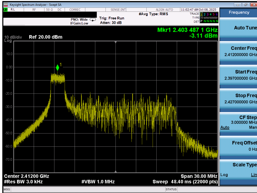
Plot 7-19. Power Spectral Density Plot MIMO ANT2 (802.11ax/be OFDMA – 26 Tones – Ch. 1)
