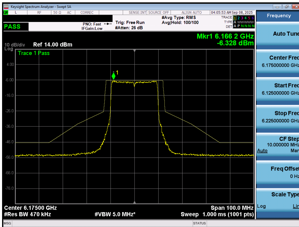
Plot 7-62. In Band Emissions Plot MIMO ANT1 (20MHz 802.11ax/be (UNII Band 5) – Ch. 45) - LPI
