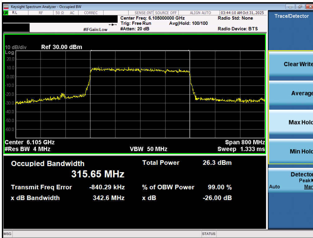
Plot 7-21. 26dB Bandwidth Plot MIMO ANT2 (320MHz 802.11ax/be (UNII Band 5) – Ch. 31) - LPI/SP
