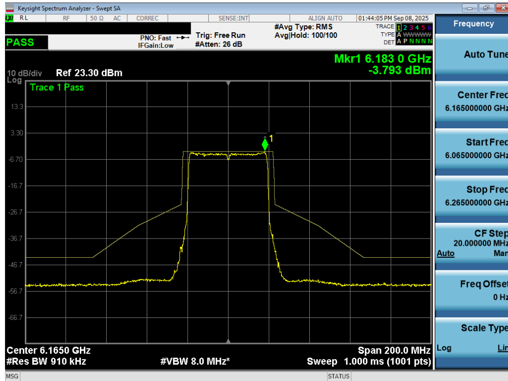
Plot 7-78. In Band Emissions Plot MIMO ANT2 (40MHz 802.11ax/be (UNII Band 5) – Ch. 43) - LPI
