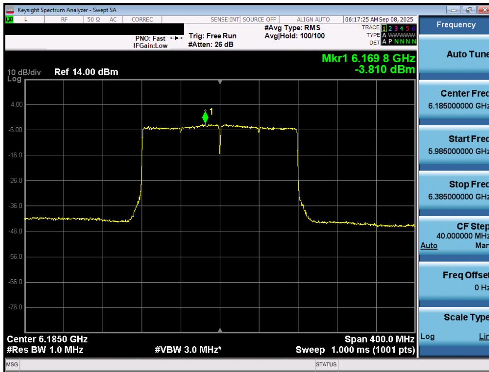
Plot 7-35. Power Spectral Density Plot MIMO ANT1 (160MHz 802.11ax/be (UNII Band 5) – Ch. 47) - LPI/SP
