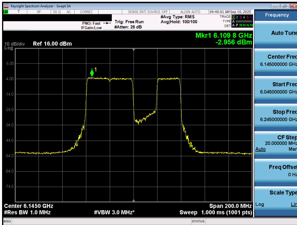
Plot 7-37. Power Spectral Density Plot MIMO ANT1 (80MHz 802.11be (UNII Band 5) – Ch. 39) – 20MHz Punctured - LPI
