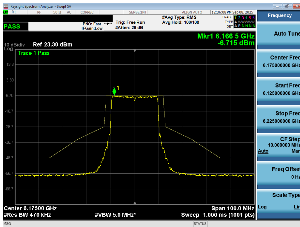
Plot 7-77. In Band Emissions Plot MIMO ANT2 (20MHz 802.11ax/be (UNII Band 5) – Ch. 45) - LPI
