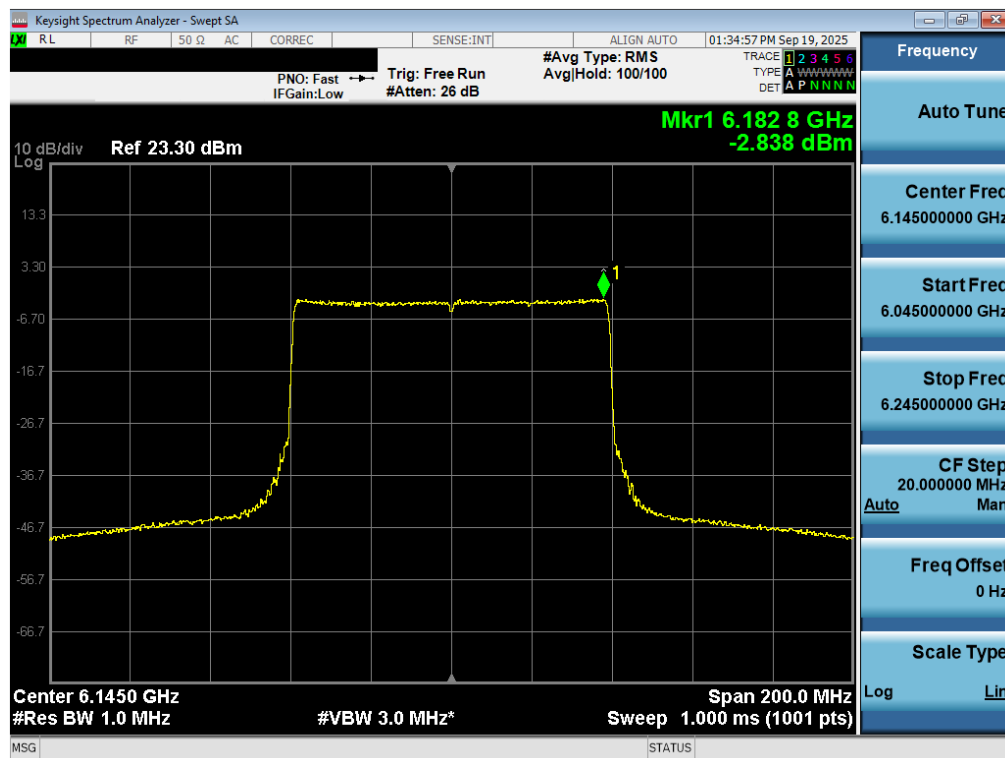
Plot 7-49. Power Spectral Density Plot MIMO ANT2 (80MHz 802.11ax/be (UNII Band 5) – Ch. 39) - LPI
