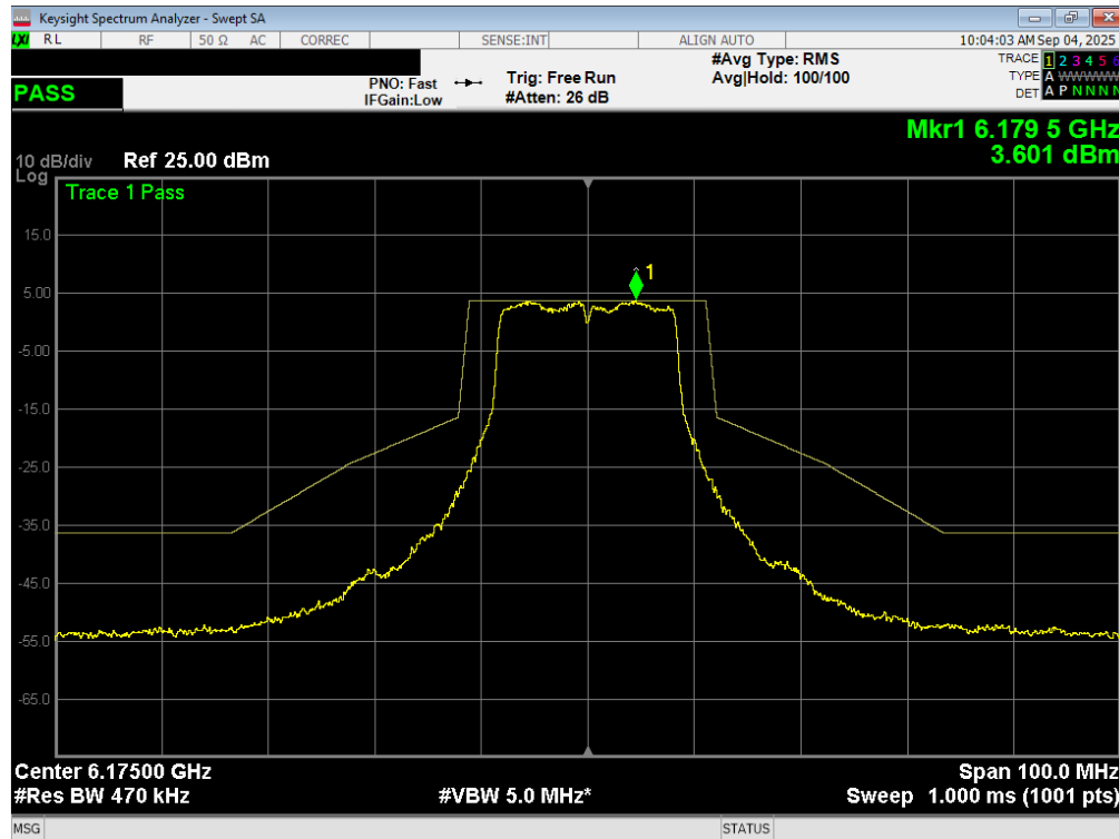
Plot 7-85. In Band Emissions Plot MIMO ANT2 (20MHz 802.11a (UNII Band 5) – Ch. 45) - SP
