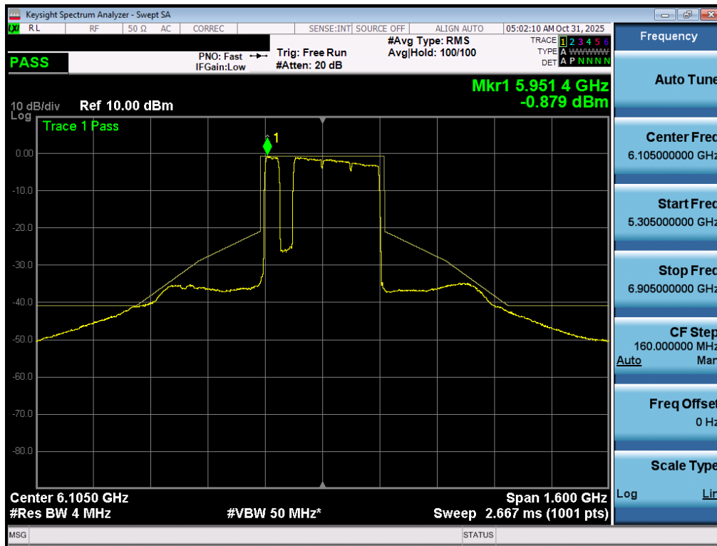
Plot 7-69. In Band Emissions Plot MIMO ANT1 (320MHz 802.11be (UNII Band 5) – Ch. 31) – 40MHz Punctured – LPI/SP
