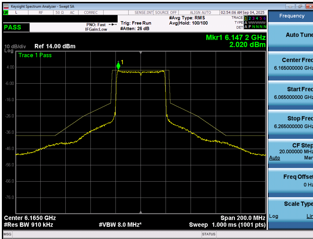
Plot 7-72. In Band Emissions Plot MIMO ANT1 (40MHz 802.11ax/be (UNII Band 5) – Ch. 43) – SP
