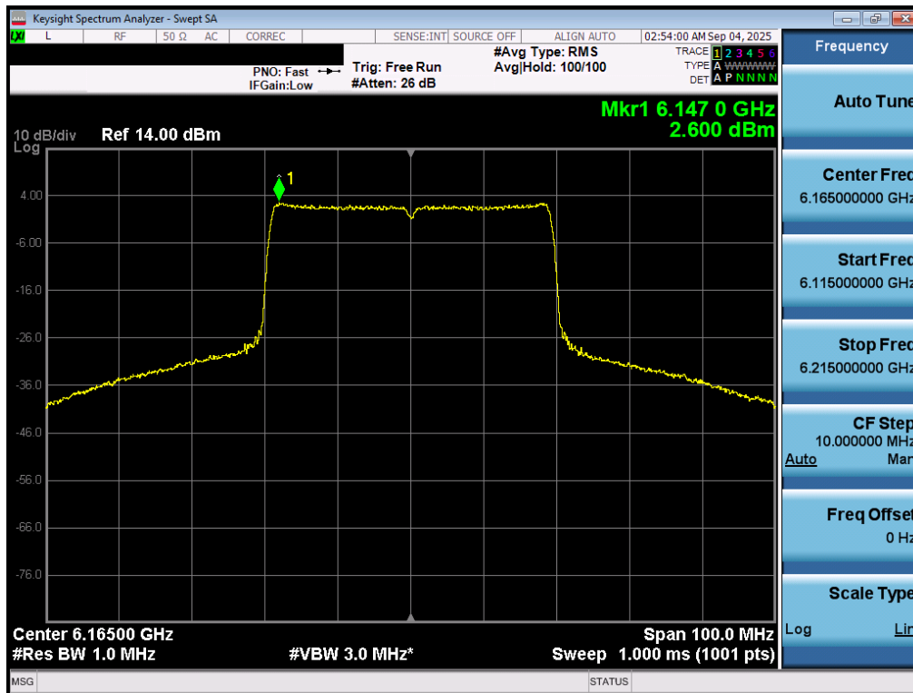
Plot 7-42. Power Spectral Density Plot MIMO ANT1 (40MHz 802.11ax/be (UNII Band 5) – Ch. 43) – SP
