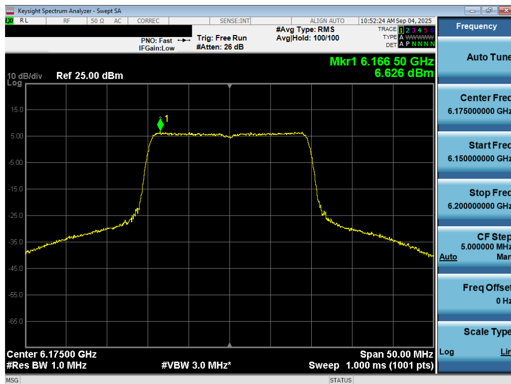
Plot 7-56. Power Spectral Density Plot MIMO ANT2 (20MHz 802.11ax/be (UNII Band 5) – Ch. 45) - SP
