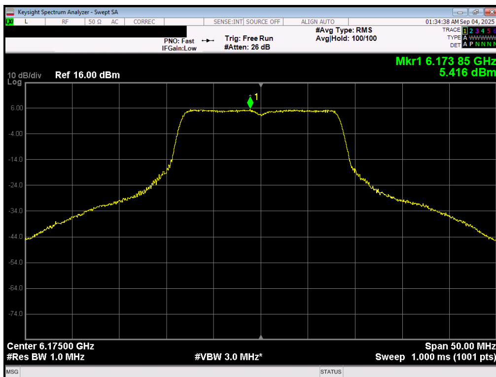
Plot 7-40. Power Spectral Density Plot MIMO ANT1 (20MHz 802.11a (UNII Band 5) – Ch. 45) - SP
