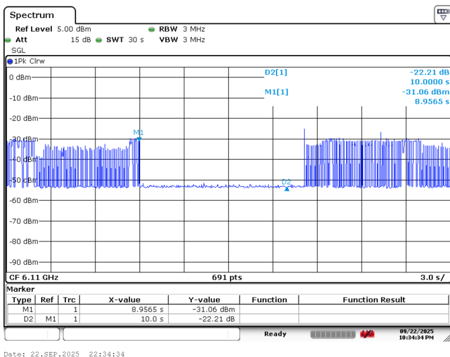
Plot 7-93. Contention Based Protocol Timing Plot (320MHz (UNII Band 5) – Ch. 31 Low)
