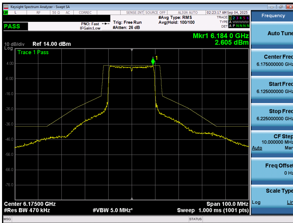
Plot 7-71. In Band Emissions Plot MIMO ANT1 (20MHz 802.11ax/be (UNII Band 5) – Ch. 45) - SP
