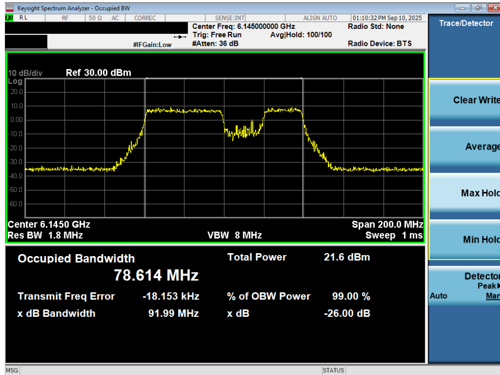
Plot 7-22. 26dB Bandwidth Plot MIMO ANT2 (80MHz 802.11be (UNII Band 5) – Ch. 39) – 20MHz Punctured - LPI
