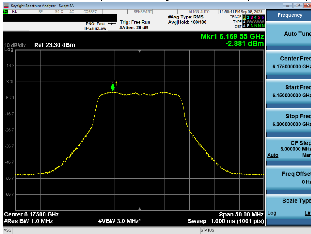
Plot 7-46. Power Spectral Density Plot MIMO ANT2 (20MHz 802.11a (UNII Band 5) – Ch. 45) - LPI
