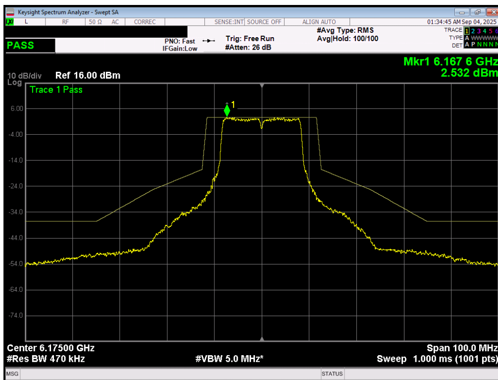
Plot 7-70. In Band Emissions Plot MIMO ANT1 (20MHz 802.11a (UNII Band 5) – Ch. 45) - SP
