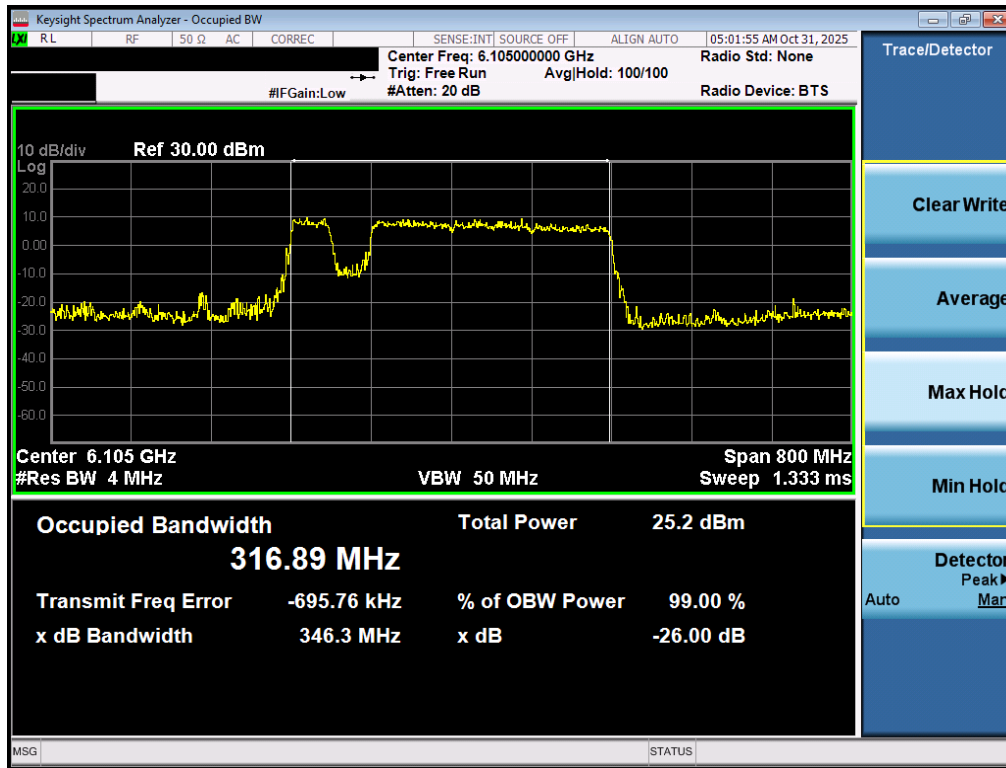
Plot 7-9. 26dB Bandwidth Plot MIMO ANT1 (320MHz 802.11be (UNII Band 5) – Ch. 31) – 40MHz Punctured – LPI/SP
