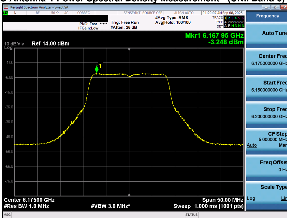
Plot 7-31. Power Spectral Density Plot MIMO ANT1 (20MHz 802.11a (UNII Band 5) – Ch. 45) - LPI
