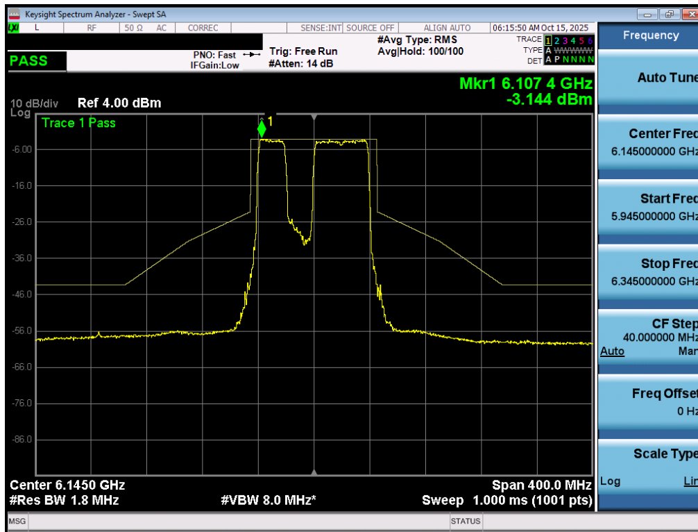
Plot 7-67. In Band Emissions Plot MIMO ANT1 (80MHz 802.11be (UNII Band 5) – Ch. 39) – 20MHz Punctured - LPI
