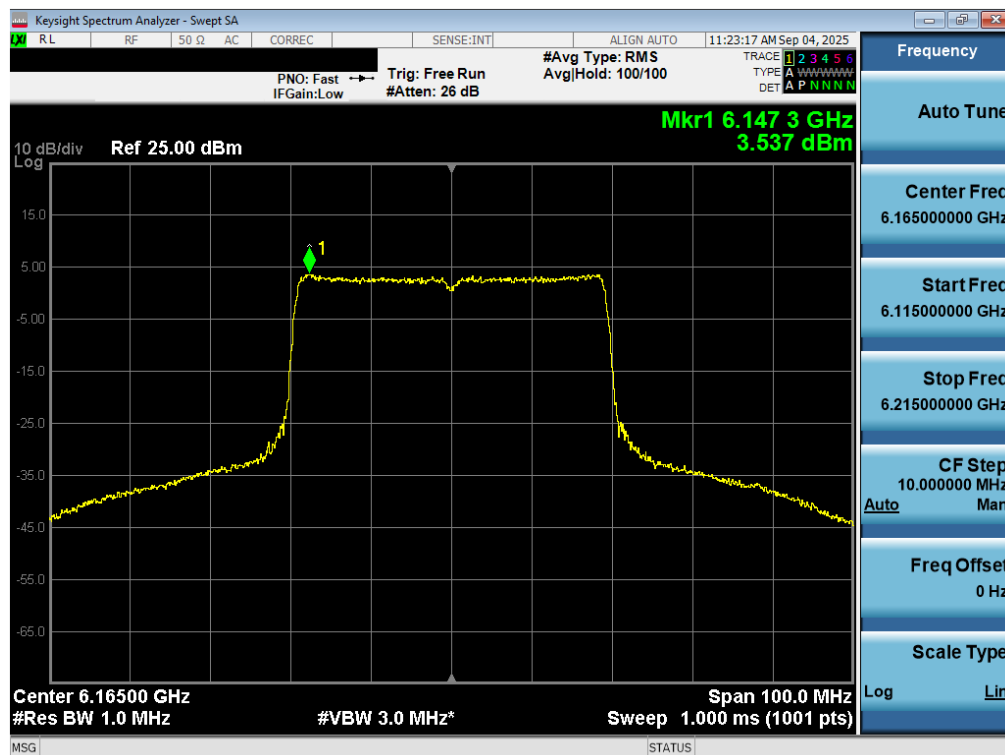
Plot 7-57. Power Spectral Density Plot MIMO ANT2 (40MHz 802.11ax/be (UNII Band 5) – Ch. 43) – SP
