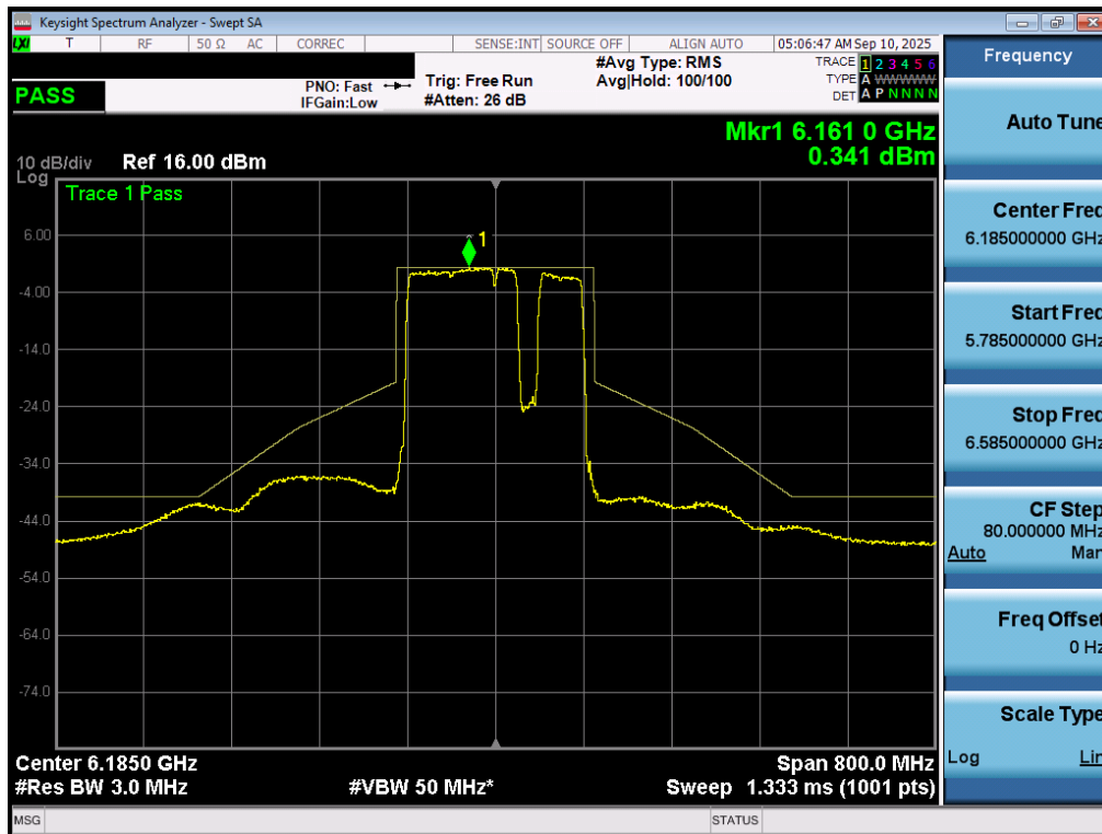
Plot 7-68. In Band Emissions Plot MIMO ANT1 (160MHz 802.11be (UNII Band 5) – Ch. 47) – 20MHz Punctured - LPI
