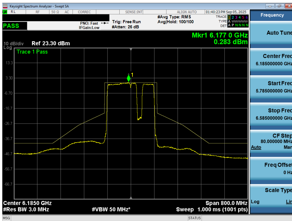
Plot 7-90. In Band Emissions Plot MIMO ANT2 (160MHz 802.11be (UNII Band 5) – Ch. 47) – 20MHz Punctured - SP
