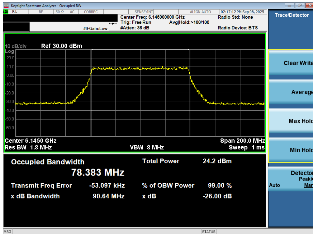
Plot 7-19. 26dB Bandwidth Plot MIMO ANT2 (80MHz 802.11ax/be (UNII Band 5) – Ch. 39) - LPI
