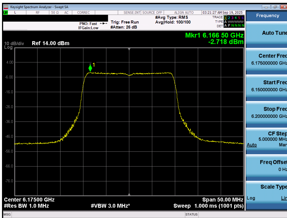
Plot 7-32. Power Spectral Density Plot MIMO ANT1 (20MHz 802.11ax/be (UNII Band 5) – Ch. 45) - LPI
