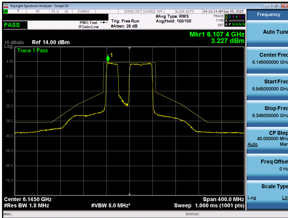
Plot 7-74. In Band Emissions Plot MIMO ANT1 (80MHz 802.11be (UNII Band 5) – Ch. 39) – 20MHz Punctured - SP
