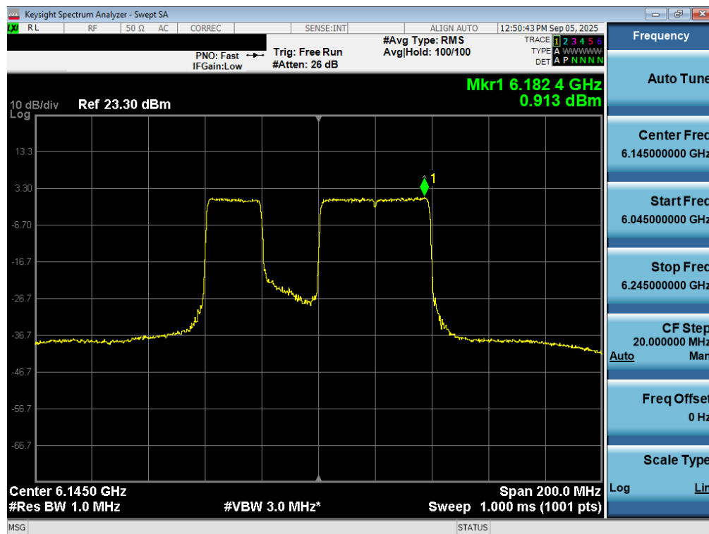
Plot 7-59. Power Spectral Density Plot MIMO ANT2 (80MHz 802.11be (UNII Band 5) – Ch. 39) – 20MHz Punctured - SP
