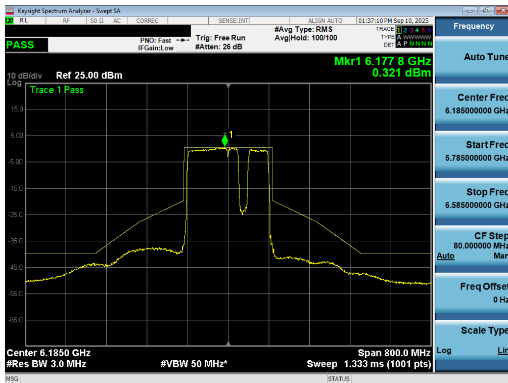
Plot 7-83. In Band Emissions Plot MIMO ANT2 (160MHz 802.11be (UNII Band 5) – Ch. 47) – 20MHz Punctured - LPI
