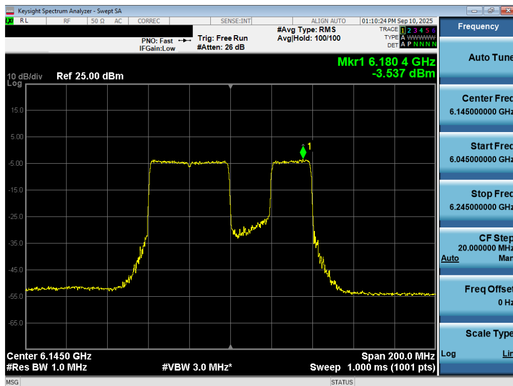
Plot 7-52. Power Spectral Density Plot MIMO ANT2 (80MHz 802.11be (UNII Band 5) – Ch. 39) – 20MHz Punctured - LPI
