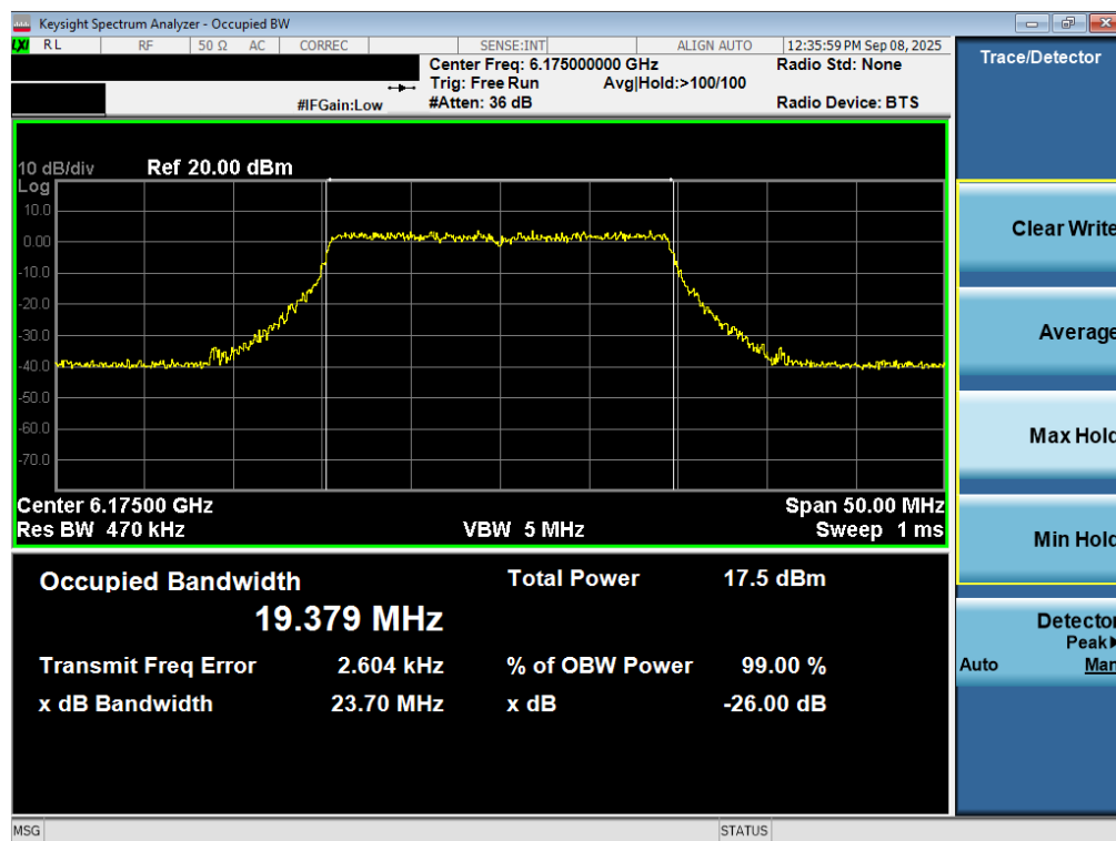
Plot 7-17. 26dB Bandwidth Plot MIMO ANT2 (20MHz 802.11ax/be (UNII Band 5) – Ch. 45) - LPI
