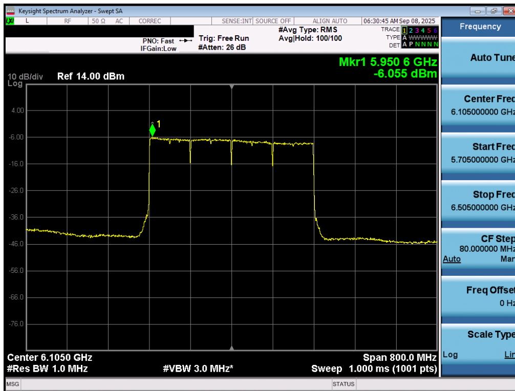
Plot 7-36. Power Spectral Density Plot MIMO ANT1 (320MHz 802.11ax/be (UNII Band 5) – Ch. 31) - LPI/SP
