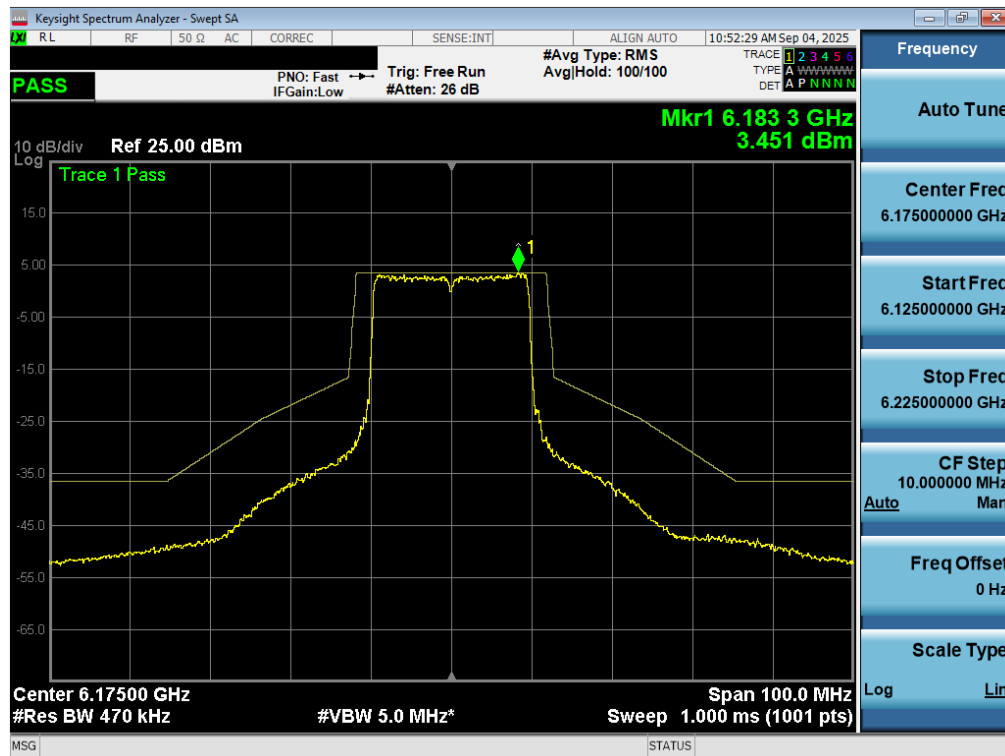
Plot 7-86. In Band Emissions Plot MIMO ANT2 (20MHz 802.11ax/be (UNII Band 5) – Ch. 45) - SP
