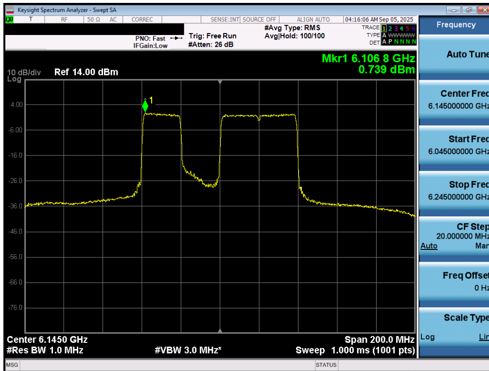
Plot 7-44. Power Spectral Density Plot MIMO ANT1 (80MHz 802.11be (UNII Band 5) – Ch. 39) – 20MHz Punctured - SP
