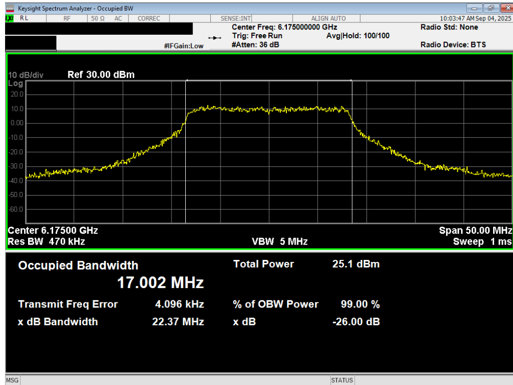
Plot 7-25. 26dB Bandwidth Plot MIMO ANT2 (20MHz 802.11a (UNII Band 5) – Ch. 45) - SP
