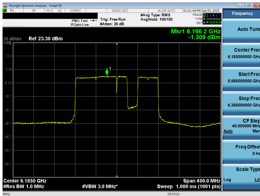
Plot 7-60. Power Spectral Density Plot MIMO ANT2 (160MHz 802.11be (UNII Band 5) – Ch. 47) – 40MHz Punctured - SP
