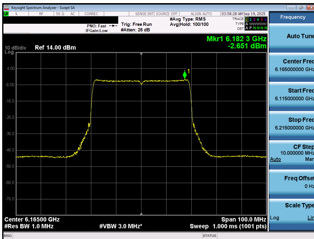
Plot 7-33. Power Spectral Density Plot MIMO ANT1 (40MHz 802.11ax/be (UNII Band 5) – Ch. 43) - LPI
