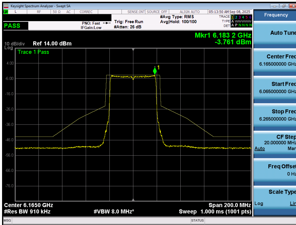
Plot 7-63. In Band Emissions Plot MIMO ANT1 (40MHz 802.11ax/be (UNII Band 5) – Ch. 43) - LPI
