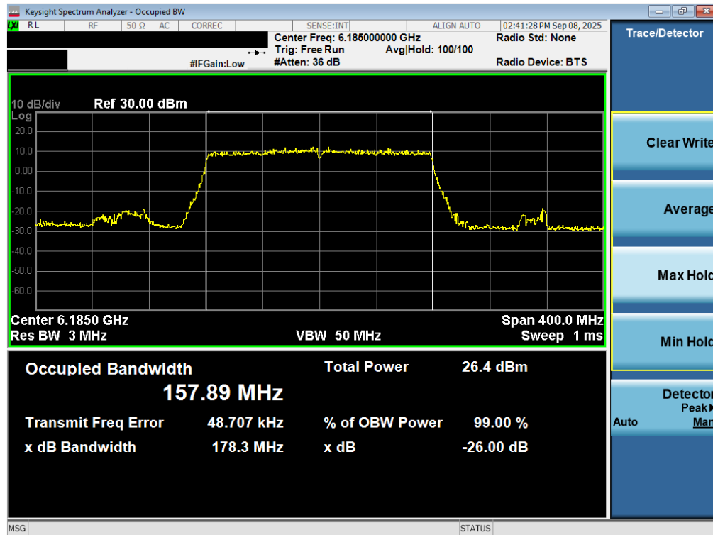
Plot 7-20. 26dB Bandwidth Plot MIMO ANT2 (160MHz 802.11ax/be (UNII Band 5) – Ch. 47) - LPI/SP
