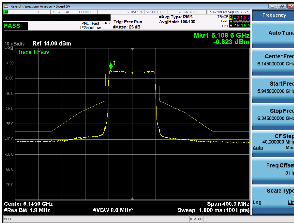
Plot 7-64. In Band Emissions Plot MIMO ANT1 (80MHz 802.11ax/be (UNII Band 5) – Ch. 39) - LPI
