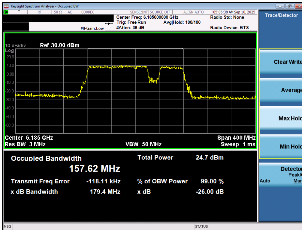
Plot 7-8. 26dB Bandwidth Plot MIMO ANT1 (160MHz 802.11be (UNII Band 5) – Ch. 47) – 20MHz Punctured - LPI
