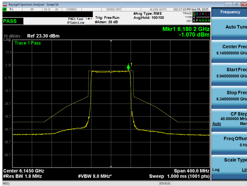
Plot 7-79. In Band Emissions Plot MIMO ANT2 (80MHz 802.11ax/be (UNII Band 5) – Ch. 39) – LPI
