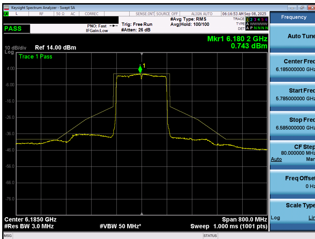
Plot 7-65. In Band Emissions Plot MIMO ANT1 (160MHz 802.11ax/be (UNII Band 5) – Ch. 47) - LPI/SP
