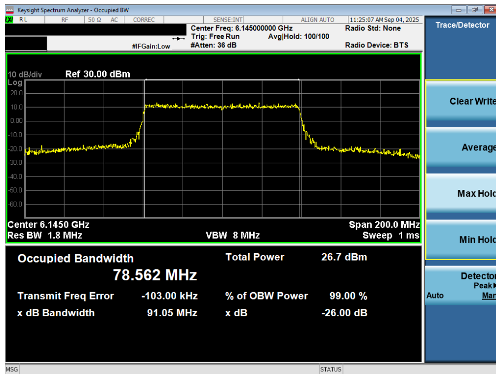
Plot 7-28. 26dB Bandwidth Plot MIMO ANT2 (80MHz 802.11ax/be (UNII Band 5) – Ch. 39) – SP
