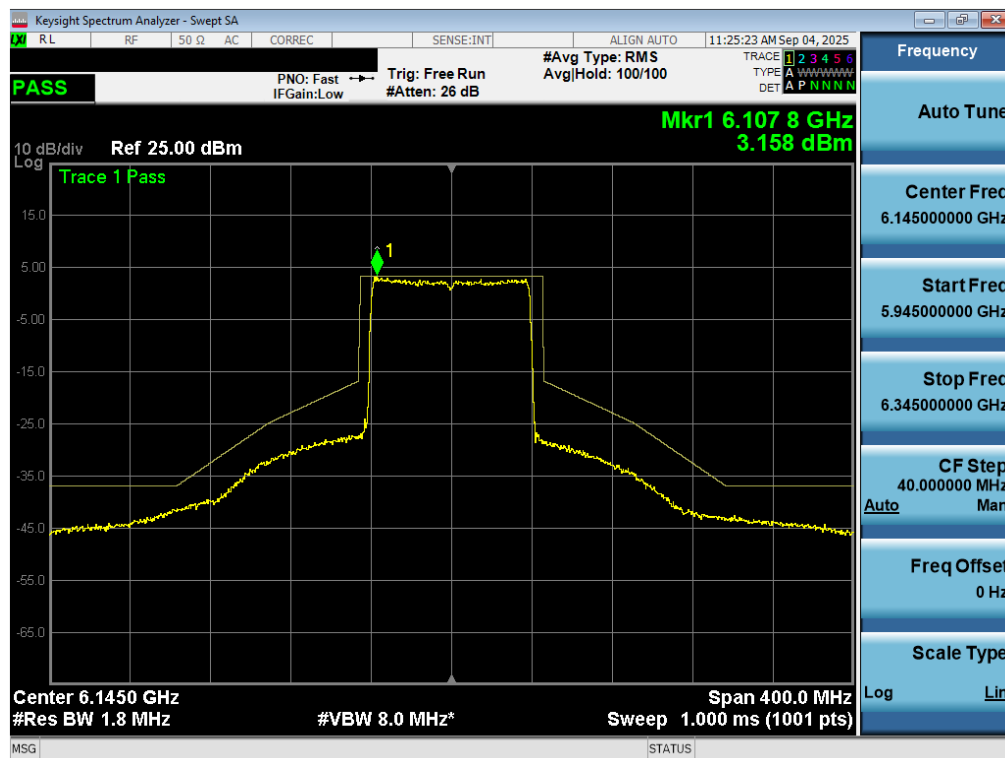
Plot 7-88. In Band Emissions Plot MIMO ANT2 (80MHz 802.11ax/be (UNII Band 5) – Ch. 39) – SP
