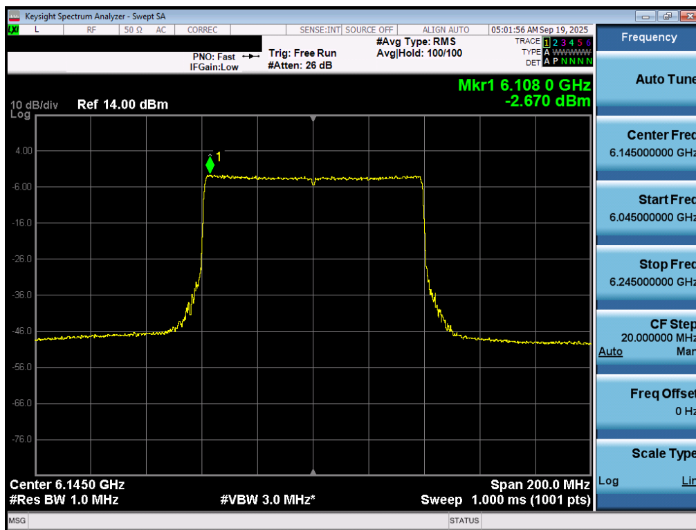
Plot 7-34. Power Spectral Density Plot MIMO ANT1 (80MHz 802.11ax/be (UNII Band 5) – Ch. 39) - LPI
