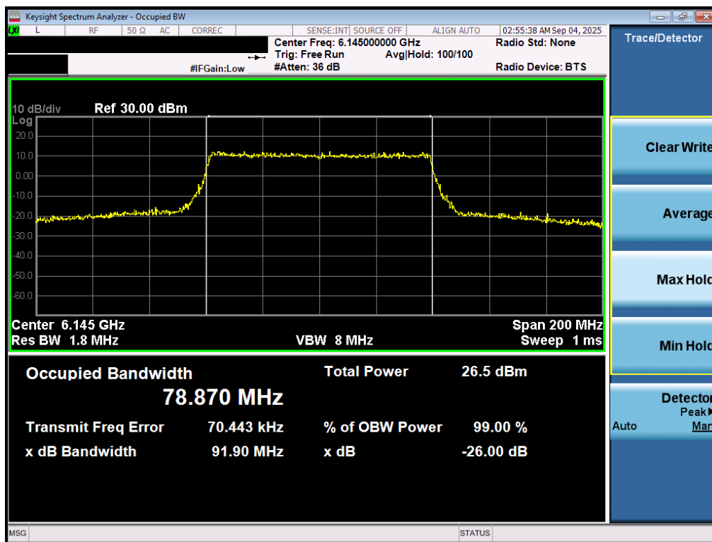
Plot 7-13. 26dB Bandwidth Plot MIMO ANT1 (80MHz 802.11ax/be (UNII Band 5) – Ch. 39) – SP
