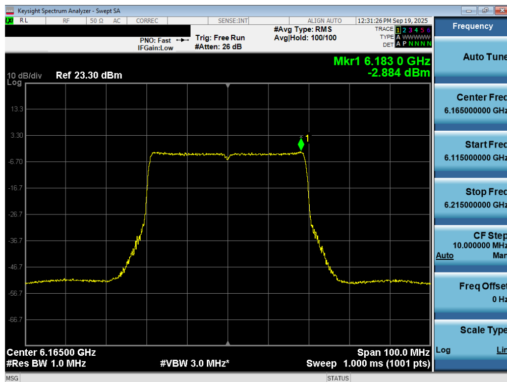
Plot 7-48. Power Spectral Density Plot MIMO ANT2 (40MHz 802.11ax/be (UNII Band 5) – Ch. 43) - LPI
