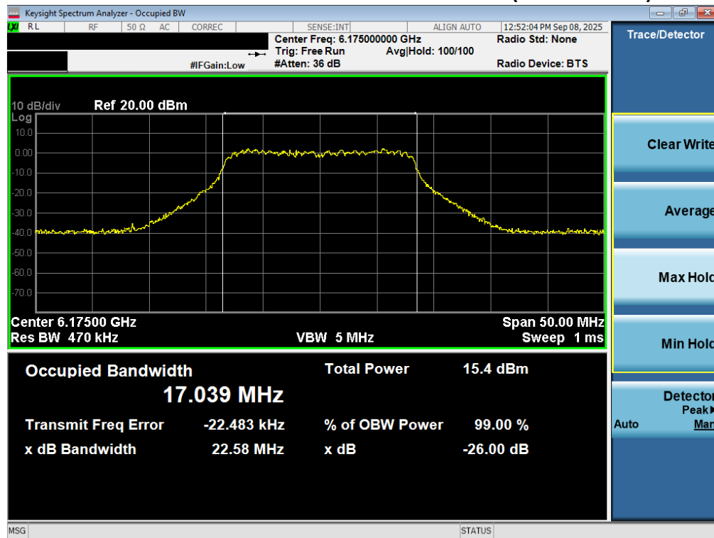
Plot 7-16. 26dB Bandwidth Plot MIMO ANT2 (20MHz 802.11a (UNII Band 5) – Ch. 45) - LPI
