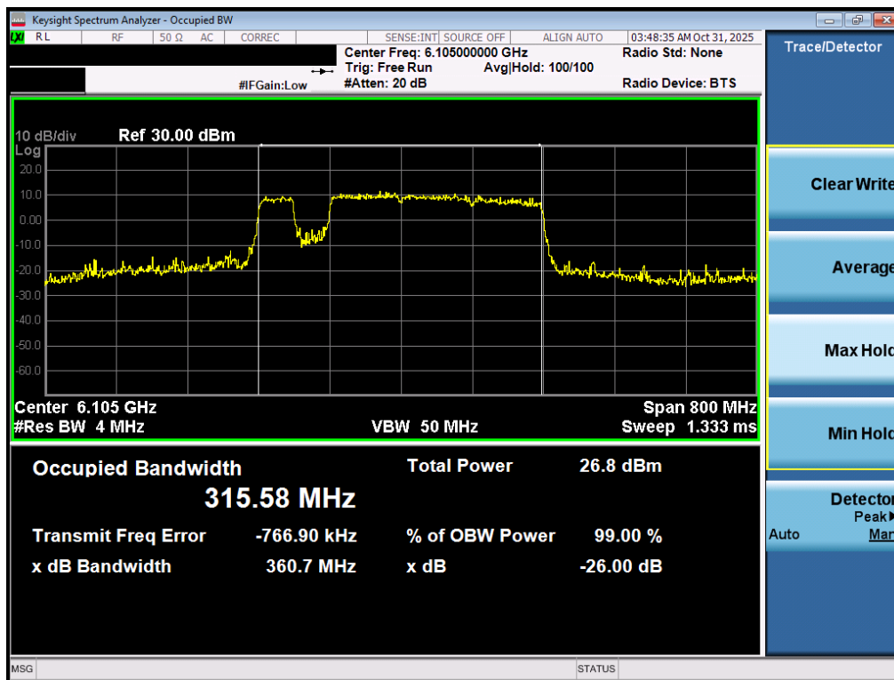
Plot 7-24. 26dB Bandwidth Plot MIMO ANT2 (320MHz 802.11be (UNII Band 5) – Ch. 31) – 40MHz Punctured – LPI/SP
