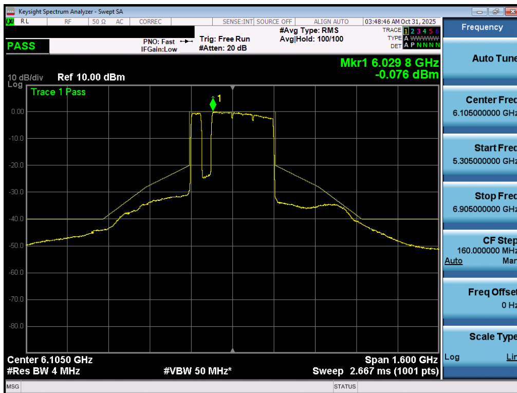
Plot 7-84. In Band Emissions Plot MIMO ANT2 (320MHz 802.11be (UNII Band 5) – Ch. 31) – 40MHz Punctured – LPI/SP
