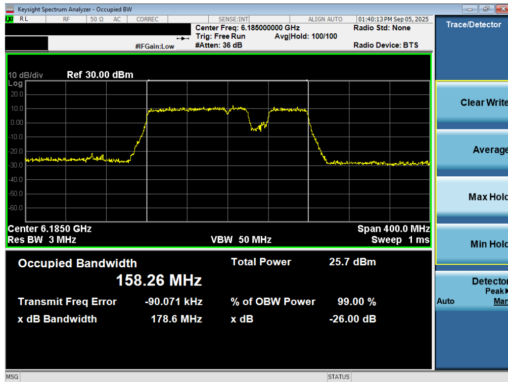
Plot 7-30. 26dB Bandwidth Plot MIMO ANT2 (160MHz 802.11be (UNII Band 5) – Ch. 47) – 20MHz Punctured - SP
