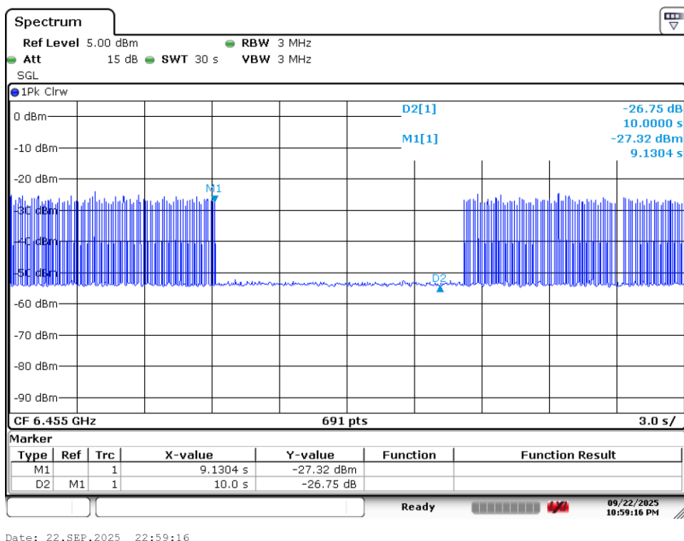
Plot 7-96. Contention Based Protocol Timing Plot (20MHz (UNII Band 6) – Ch. 101)
