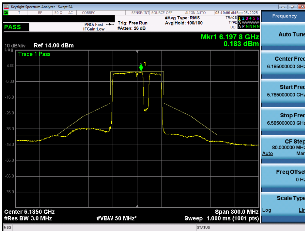
Plot 7-75. In Band Emissions Plot MIMO ANT1 (160MHz 802.11be (UNII Band 5) – Ch. 47) – 20MHz Punctured - SP
