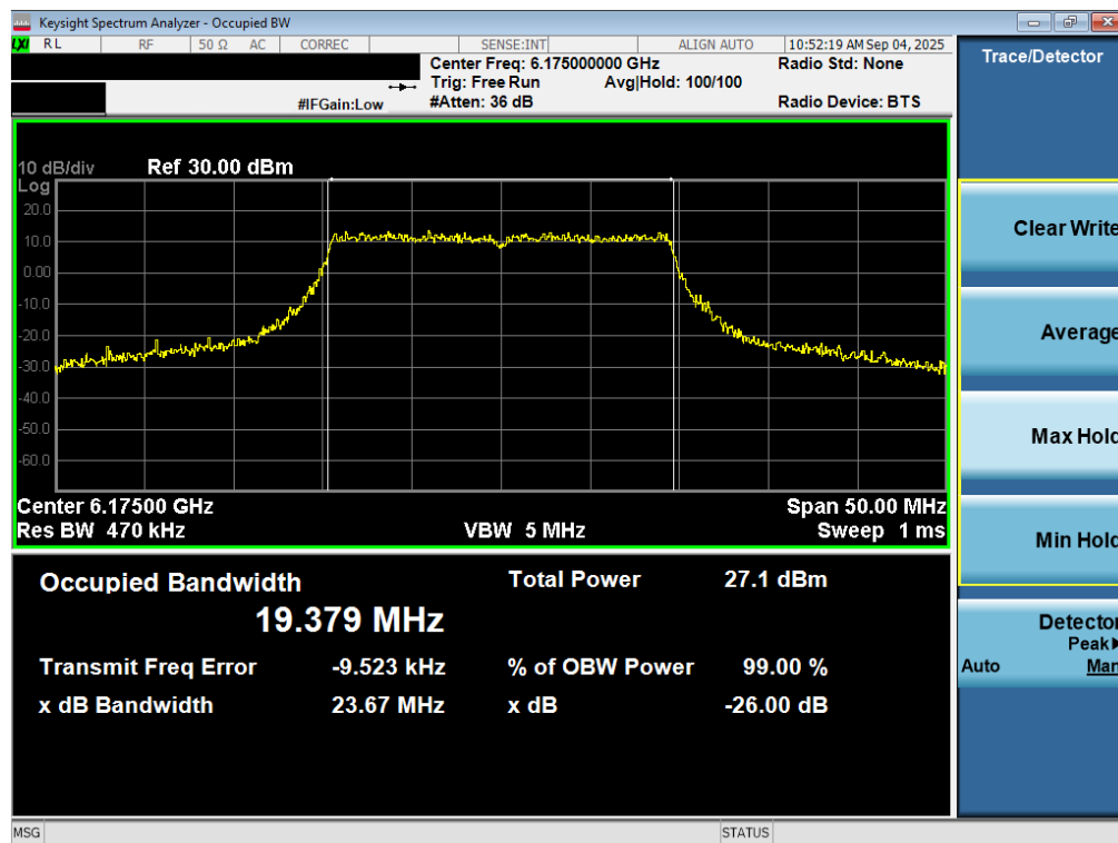
Plot 7-26. 26dB Bandwidth Plot MIMO ANT2 (20MHz 802.11ax/be (UNII Band 5) – Ch. 45) - SP
