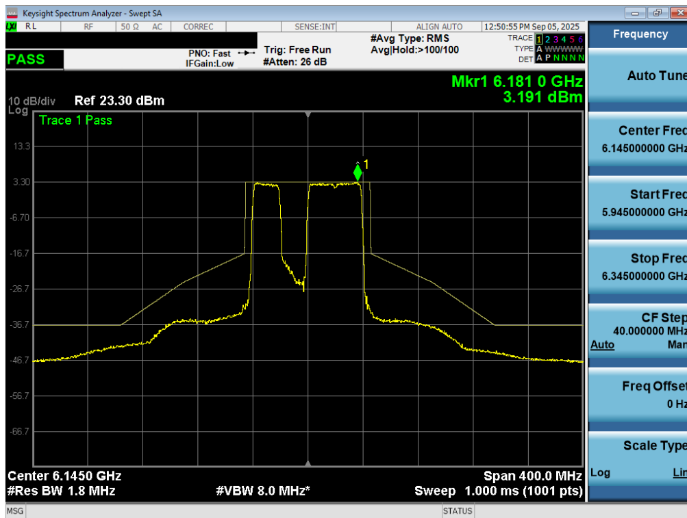
Plot 7-89. In Band Emissions Plot MIMO ANT2 (80MHz 802.11be (UNII Band 5) – Ch. 39) – 20MHz Punctured - SP
