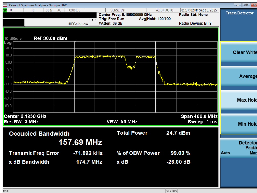
Plot 7-23. 26dB Bandwidth Plot MIMO ANT2 (160MHz 802.11be (UNII Band 5) – Ch. 47) – 20MHz Punctured - LPI
