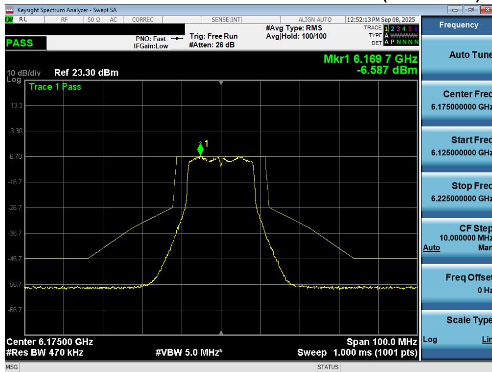
Plot 7-76. In Band Emissions Plot MIMO ANT2 (20MHz 802.11a (UNII Band 5) – Ch. 45) - LPI
