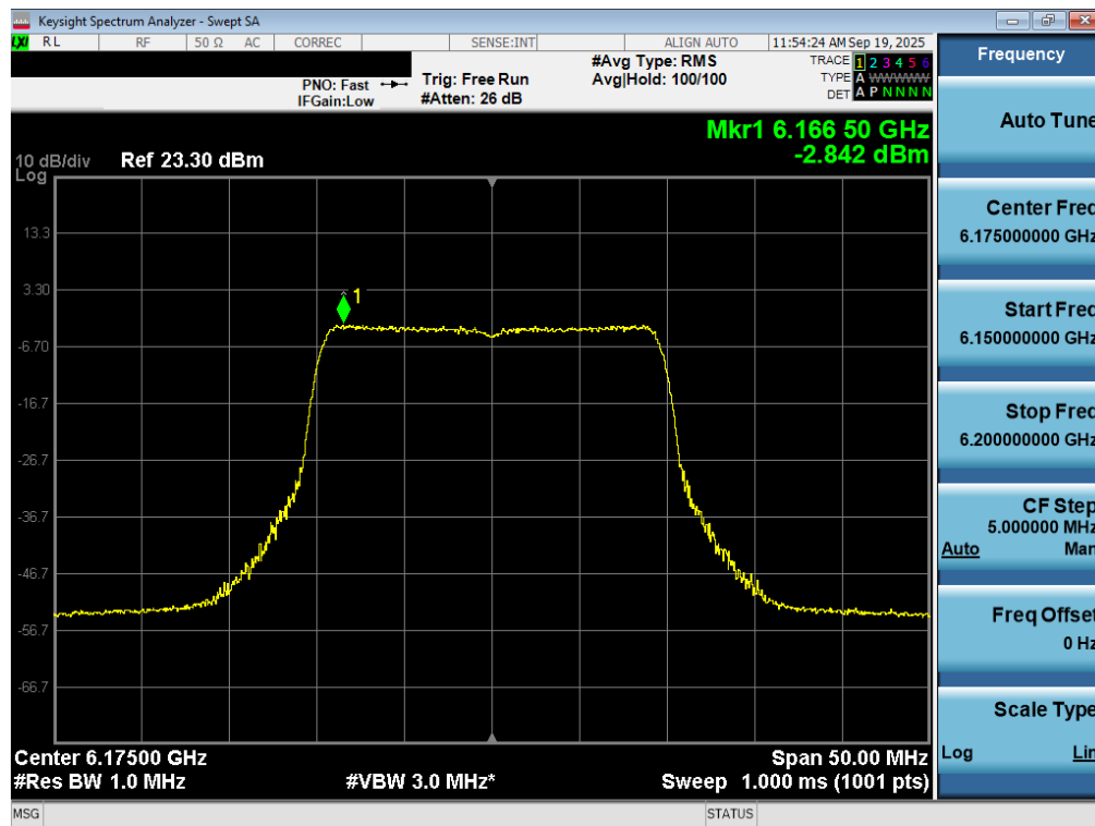
Plot 7-47. Power Spectral Density Plot MIMO ANT2 (20MHz 802.11ax/be (UNII Band 5) – Ch. 45) - LPI
