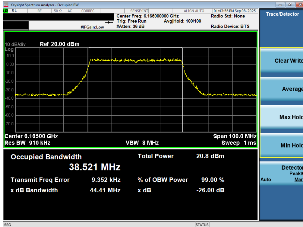
Plot 7-18. 26dB Bandwidth Plot MIMO ANT2 (40MHz 802.11ax/be (UNII Band 5) – Ch. 43) - LPI
