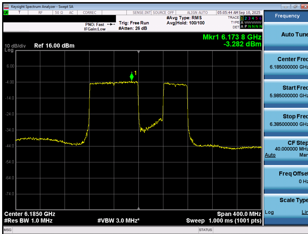
Plot 7-38. Power Spectral Density Plot MIMO ANT1 (160MHz 802.11be (UNII Band 5) – Ch. 47) – 40MHz Punctured - LPI
