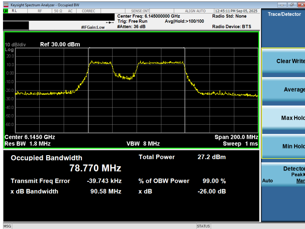
Plot 7-29. 26dB Bandwidth Plot MIMO ANT2 (80MHz 802.11be (UNII Band 5) – Ch. 39) – 20MHz Punctured - SP
