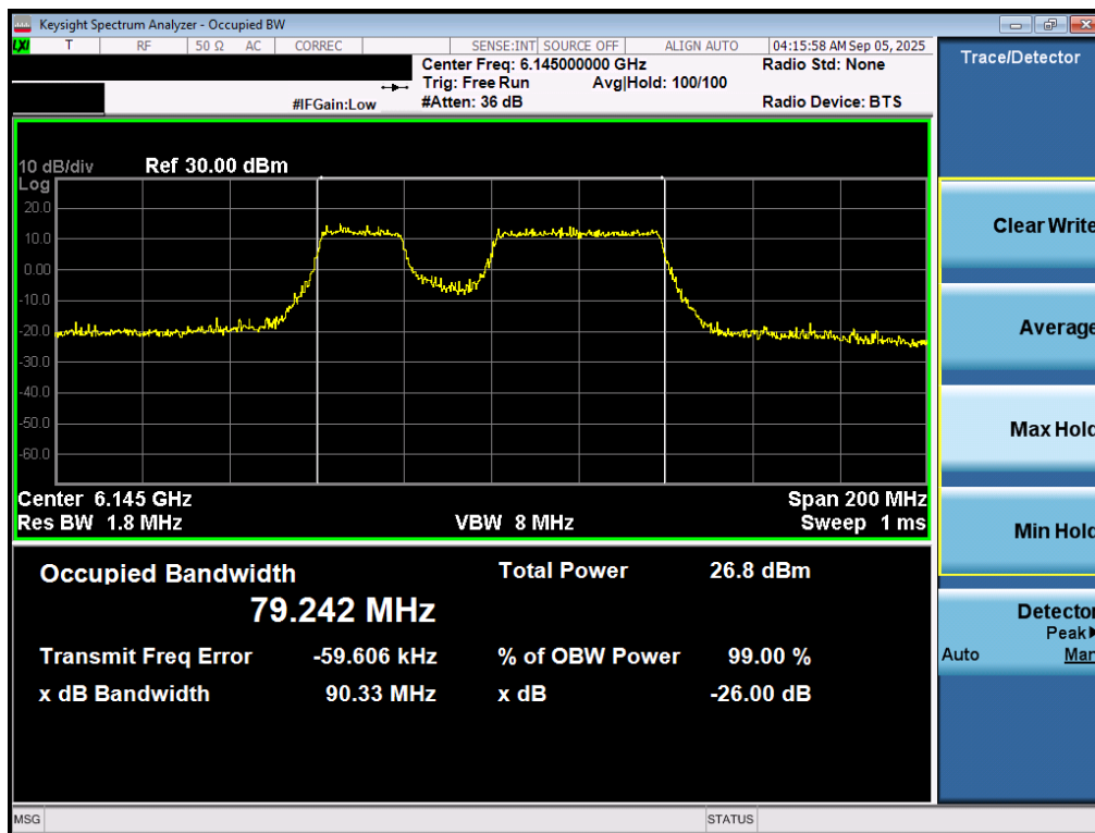
Plot 7-14. 26dB Bandwidth Plot MIMO ANT1 (80MHz 802.11be (UNII Band 5) – Ch. 39) – 20MHz Punctured - SP
