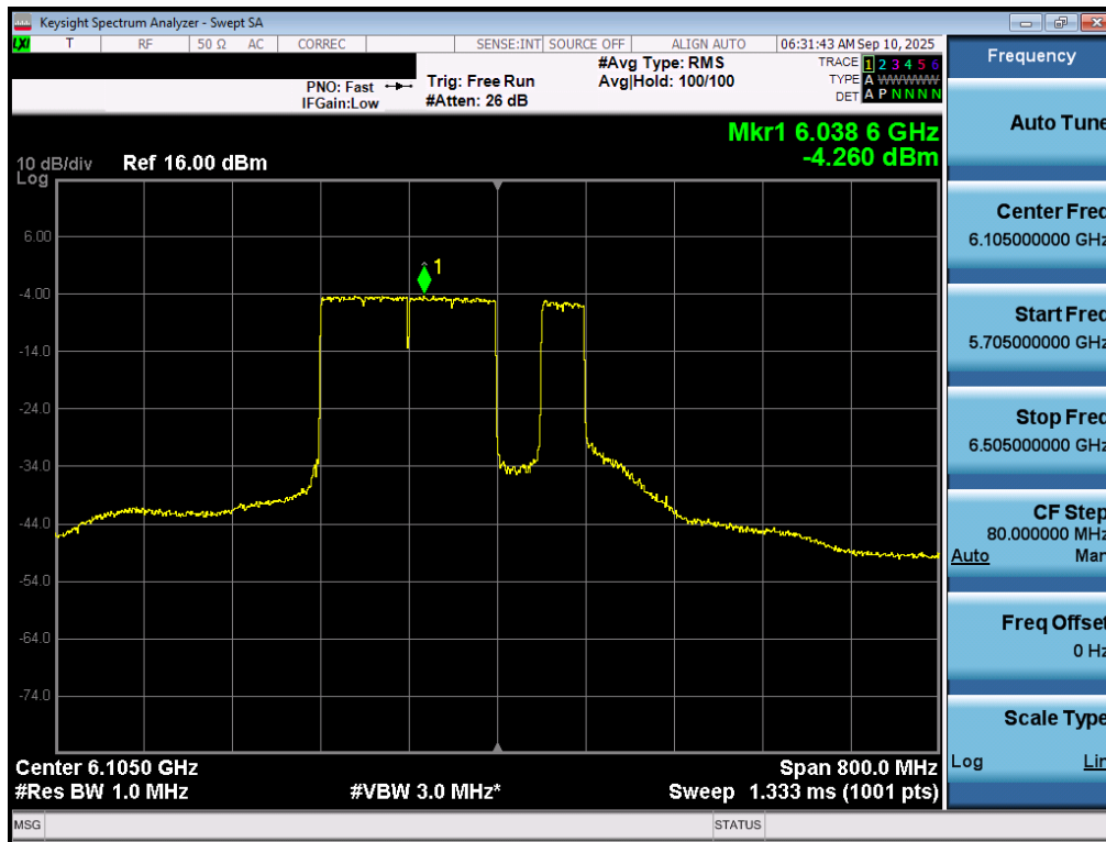
Plot 7-39. Power Spectral Density Plot MIMO ANT1 (320MHz 802.11be (UNII Band 5) – Ch. 31) – 120MHz Punctured – LPI/SP
