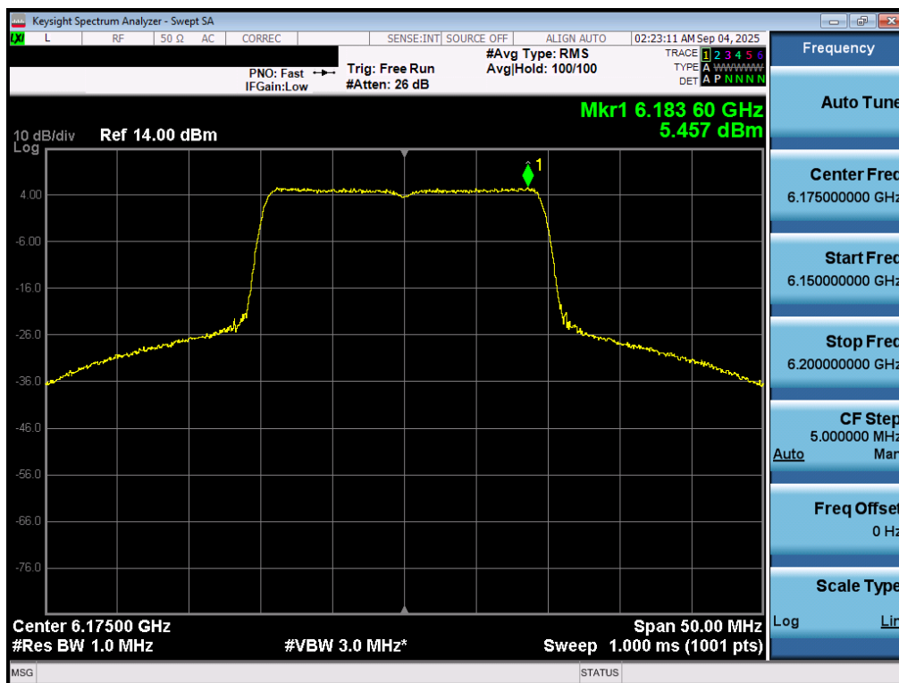
Plot 7-41. Power Spectral Density Plot MIMO ANT1 (20MHz 802.11ax/be (UNII Band 5) – Ch. 45) - SP
