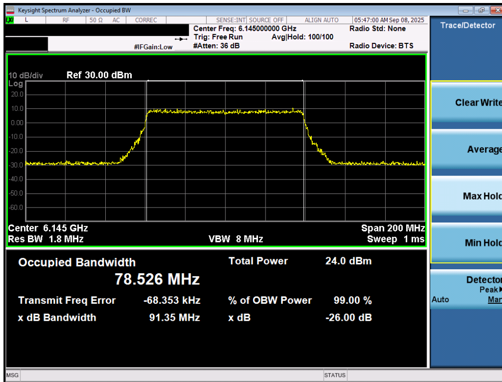
Plot 7-4. 26dB Bandwidth Plot MIMO ANT1 (80MHz 802.11ax/be (UNII Band 5) – Ch. 39) - LPI
