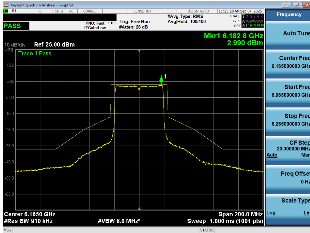
Plot 7-87. In Band Emissions Plot MIMO ANT2 (40MHz 802.11ax/be (UNII Band 5) – Ch. 43) – SP
