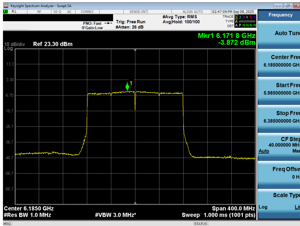
Plot 7-50. Power Spectral Density Plot MIMO ANT2 (160MHz 802.11ax/be (UNII Band 5) - Ch. 47) - LPI/SP
