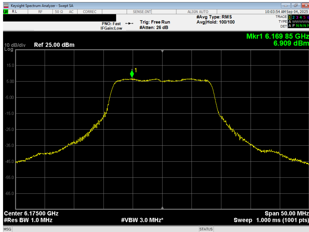
Plot 7-55. Power Spectral Density Plot MIMO ANT2 (20MHz 802.11a (UNII Band 5) – Ch. 45) – SP
