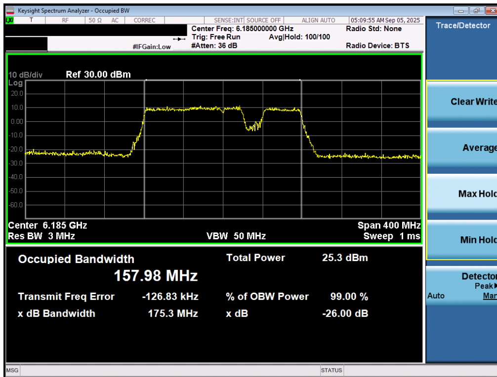
Plot 7-15. 26dB Bandwidth Plot MIMO ANT1 (160MHz 802.11be (UNII Band 5) – Ch. 47) – 20MHz Punctured - SP
