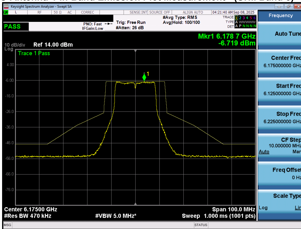
Plot 7-61. In Band Emissions Plot MIMO ANT1 (20MHz 802.11a (UNII Band 5) – Ch. 45) - LPI
