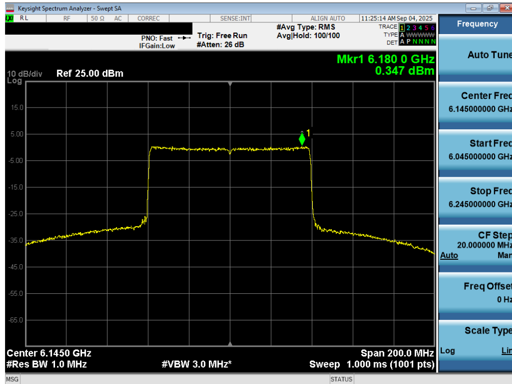
Plot 7-58. Power Spectral Density Plot MIMO ANT2 (80MHz 802.11ax/be (UNII Band 5) – Ch. 39) – SP
