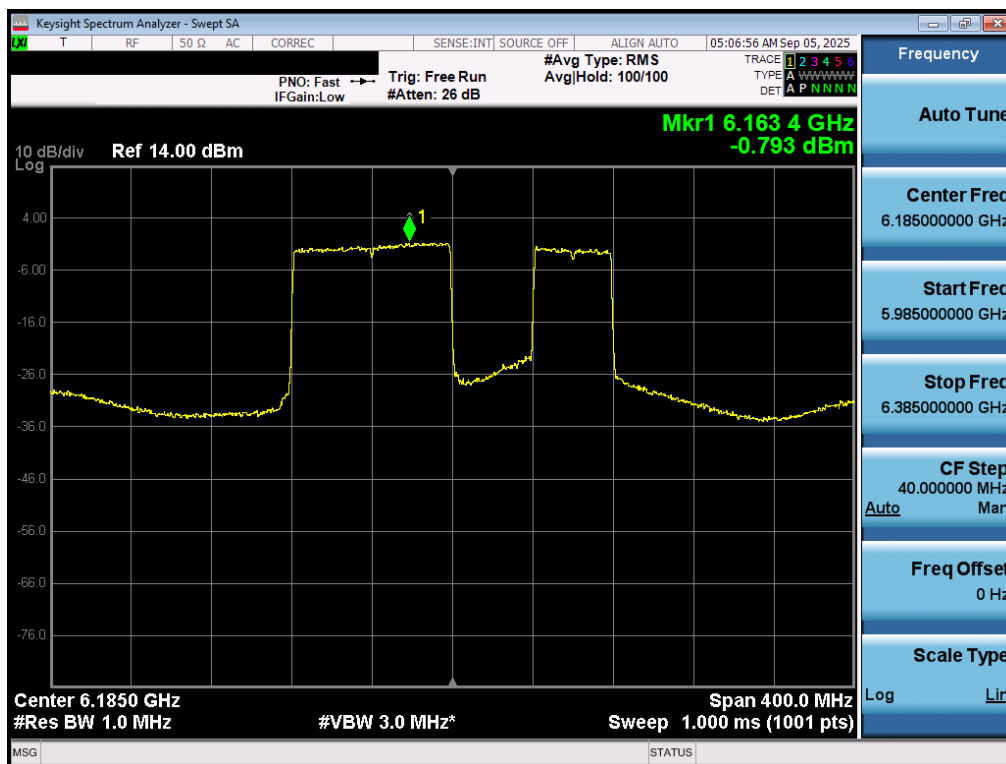
Plot 7-45. Power Spectral Density Plot MIMO ANT1 (160MHz 802.11be (UNII Band 5) – Ch. 47) – 40MHz Punctured - SP
