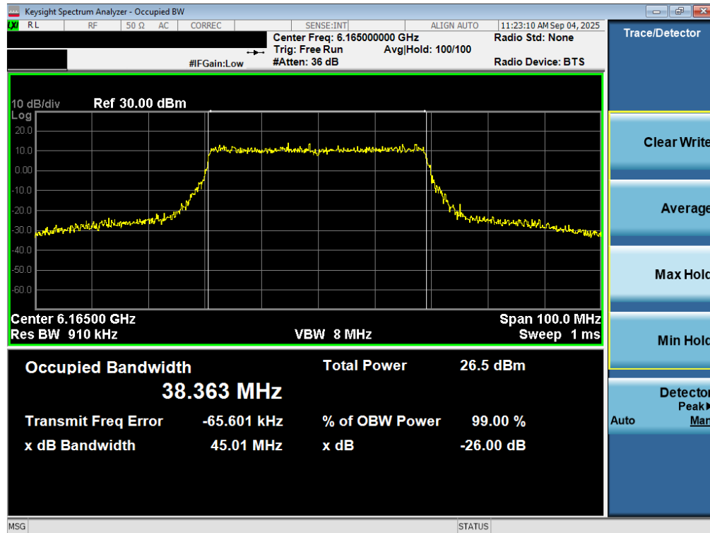
Plot 7-27. 26dB Bandwidth Plot MIMO ANT2 (40MHz 802.11ax/be (UNII Band 5) – Ch. 43) – SP
