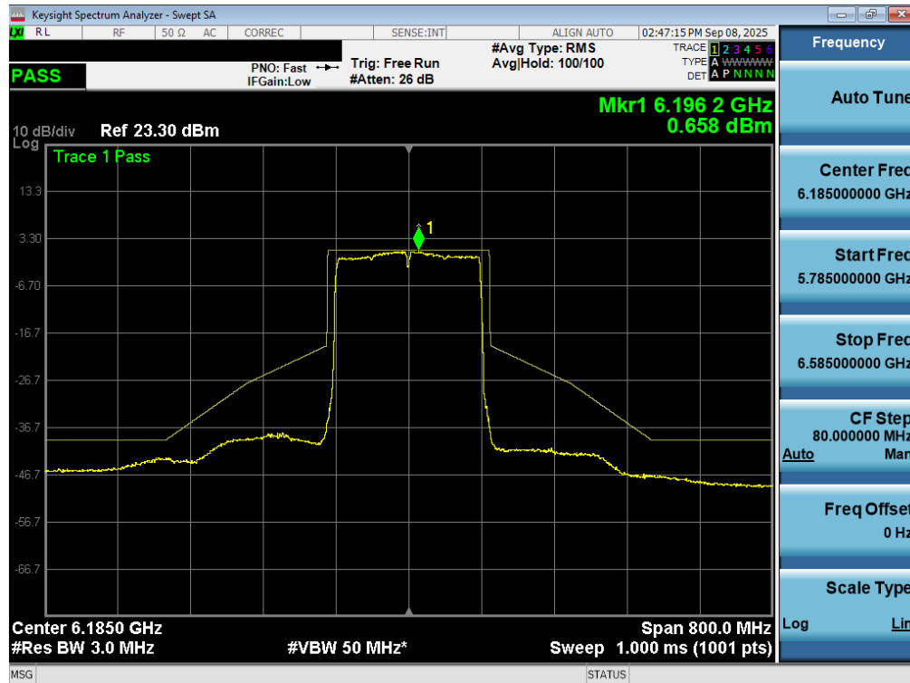
Plot 7-80. In Band Emissions Plot MIMO ANT2 (160MHz 802.11ax/be (UNII Band 5) – Ch. 47) - LPI/SP
