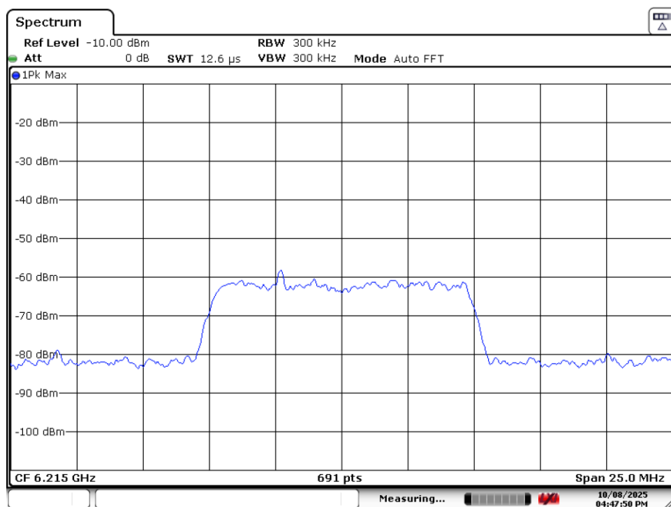
Plot 7-91. AWGN Signal (Demonstration)
