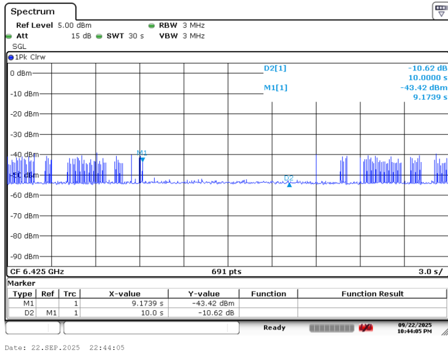
Plot 7-98. Contention Based Protocol Timing Plot (320MHz (UNII Band 6) – Ch. 95 Mid)
