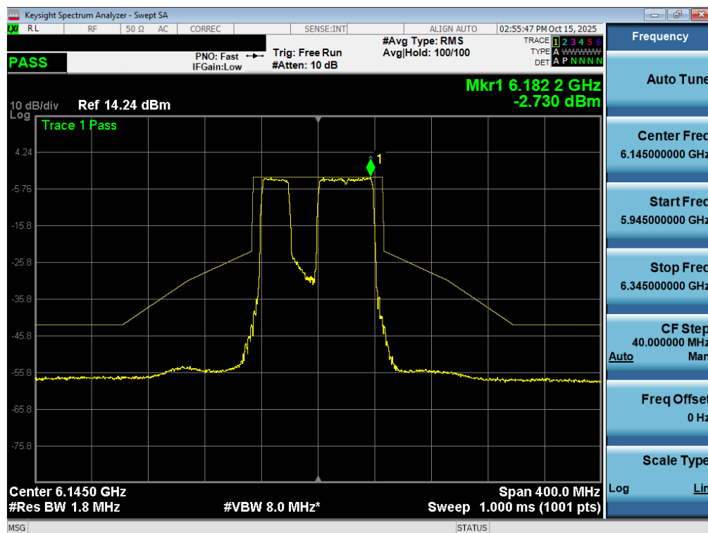
Plot 7-82. In Band Emissions Plot MIMO ANT2 (80MHz 802.11be (UNII Band 5) – Ch. 39) – 20MHz Punctured - LPI
