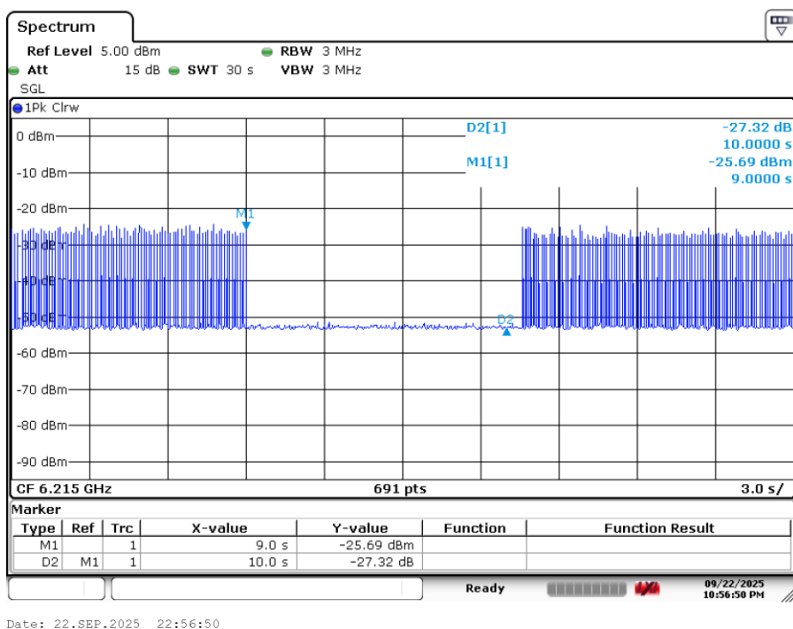
Plot 7-92. Contention Based Protocol Timing Plot (20MHz (UNII Band 5) – Ch. 53)
