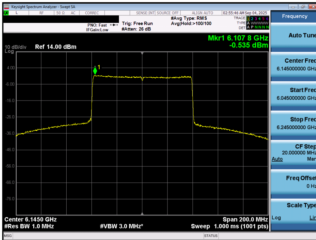
Plot 7-43. Power Spectral Density Plot MIMO ANT1 (80MHz 802.11ax/be (UNII Band 5) – Ch. 39) – SP
