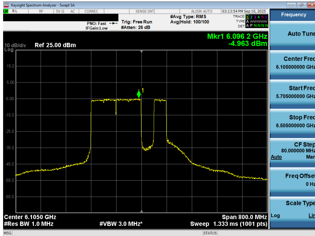
Plot 7-54. Power Spectral Density Plot MIMO ANT2 (320MHz 802.11be (UNII Band 5) – Ch. 31) – 120MHz Punctured – LPI/SP
