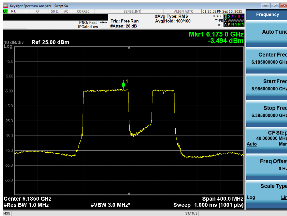
Plot 7-53. Power Spectral Density Plot MIMO ANT2 (160MHz 802.11be (UNII Band 5) – Ch. 47) – 40MHz Punctured - LPI
