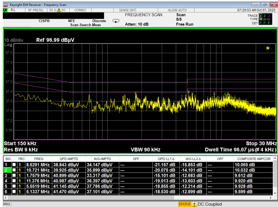
Plot 7-18. Line-Conducted Test Plot (L1) – Device to Device
