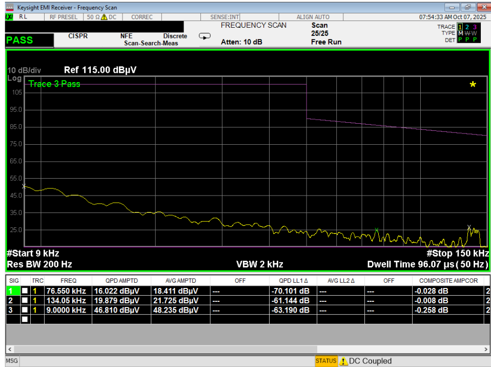
Plot 7-21. Line-Conducted Test Plot (L1) – Digitizer (Click)
