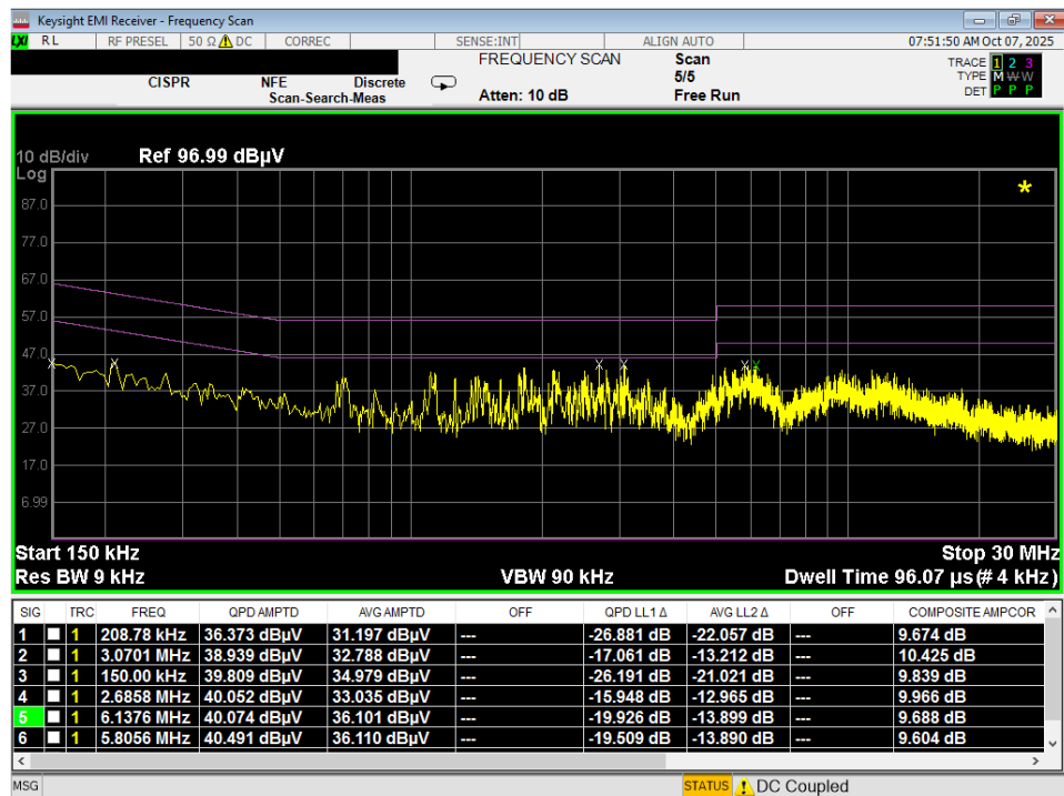
Plot 7-24. Line-Conducted Test Plot (N) – Digitizer (Click)
