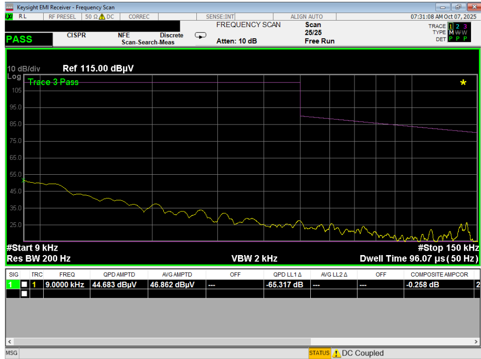
Plot 7-17. Line-Conducted Test Plot (L1) – Device to Device
