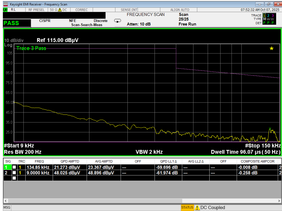
Plot 7-23. Line-Conducted Test Plot (N) – Digitizer (Click)
