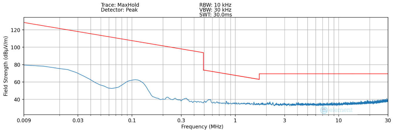
Plot 7-6 Radiated Spurious Plot 9kHz – 30MHz (Pol. Y – Device to Device)
