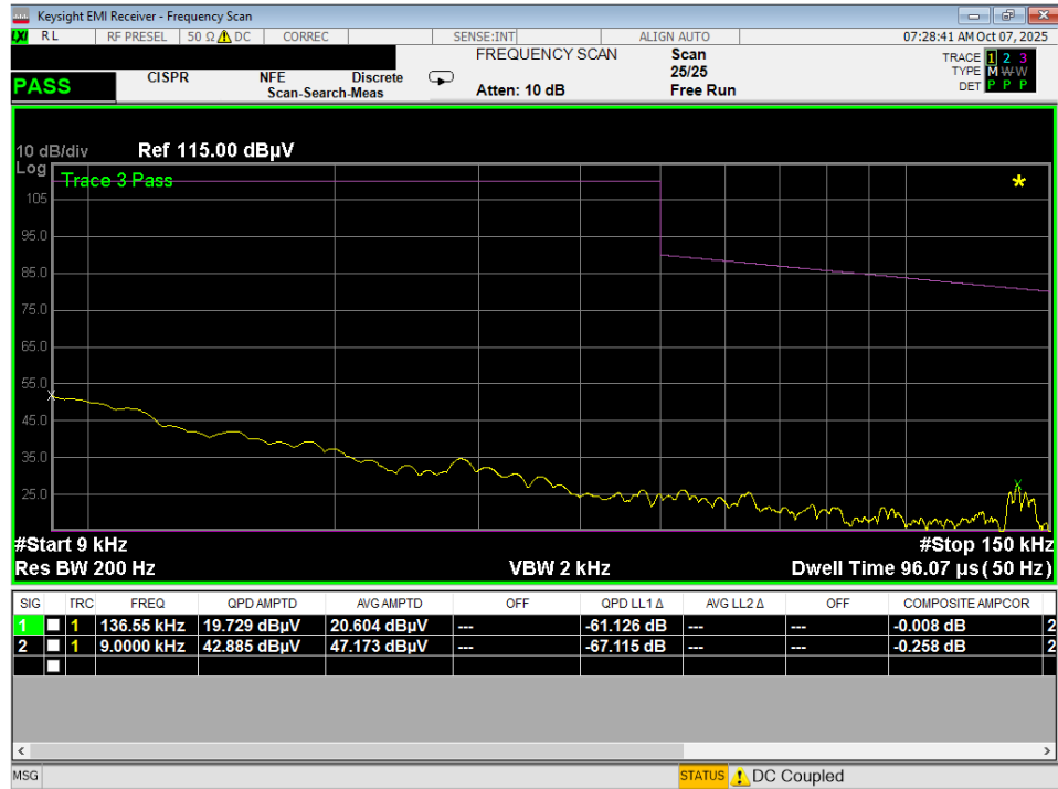
Plot 7-19. Line-Conducted Test Plot (N) – Device to Device
