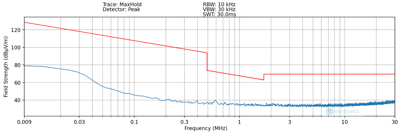
Plot 7-15Radiated Spurious Plot 9kHz – 30MHz (Pol. Y – Digitizer – Eraser)
