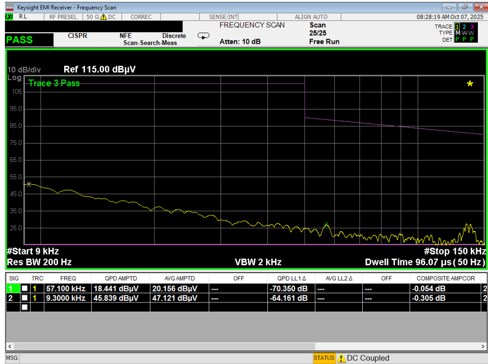
Plot 7-31. Line-Conducted Test Plot (N) – Digitizer (Eraser)
