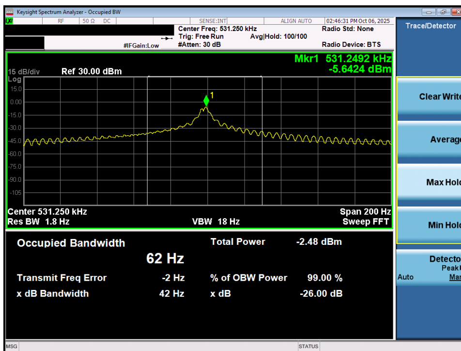
Plot 7-2. Occupied Bandwidth Measurement – Click
