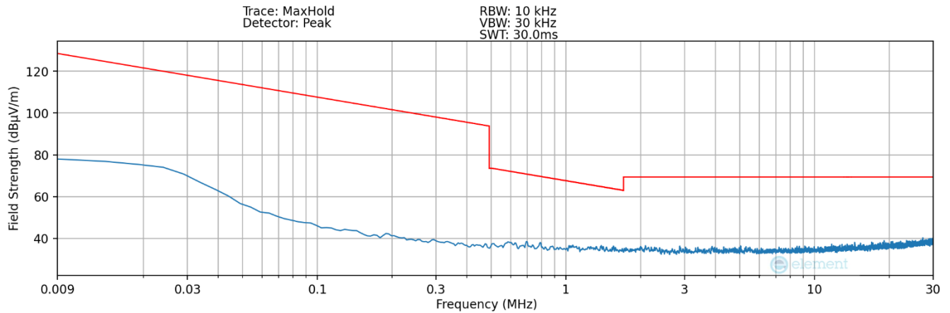
Plot 7-16. Radiated Spurious Plot 9kHz – 30MHz (Pol. Z– Digitizer – Eraser)
