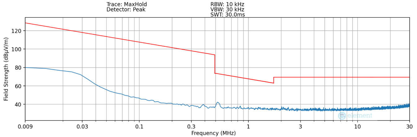
Plot 7-8. Radiated Spurious Plot 9kHz – 30MHz (Pol. X – Digitizer – Click)
