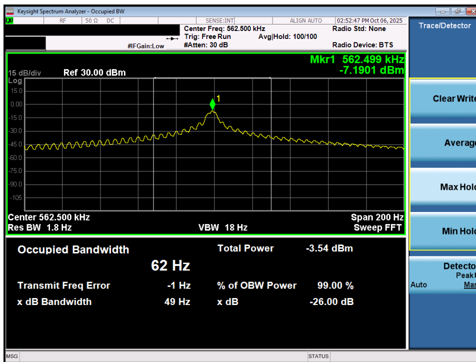
Plot 7-3. Occupied Bandwidth Measurement – Hover
