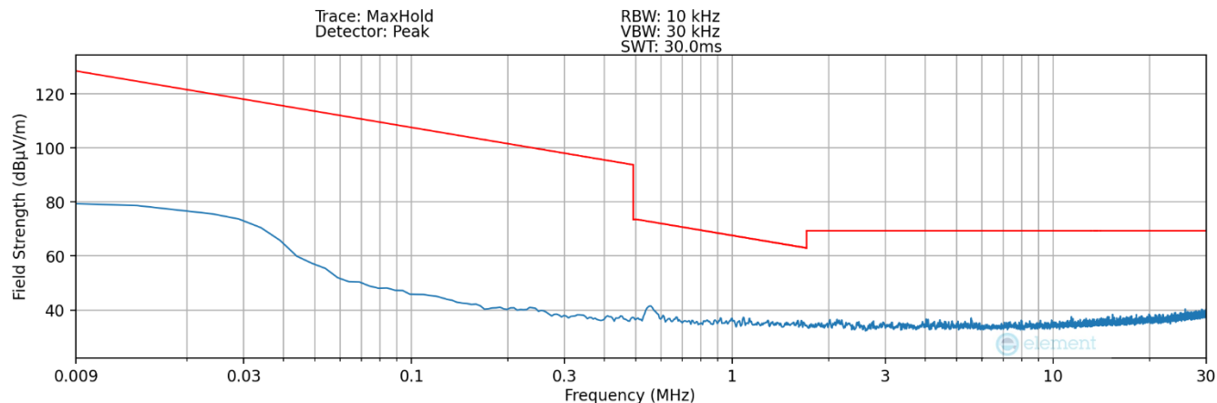
Plot 7-11. Radiated Spurious Plot 9kHz – 30MHz (Pol. X – Digitizer – Hover)
