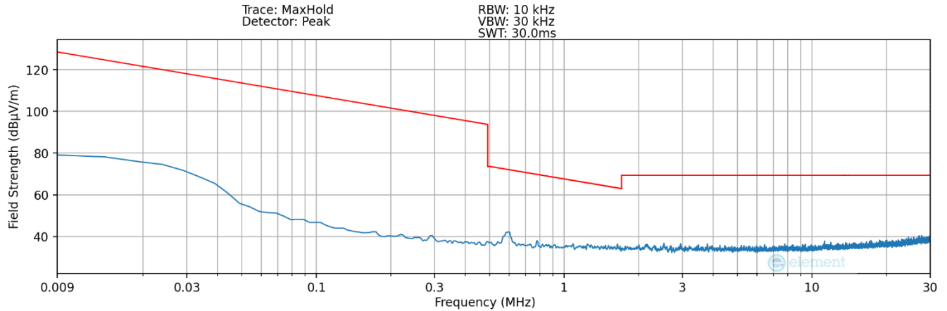
Plot 7-14. Radiated Spurious Plot 9kHz – 30MHz (Pol. X – Digitizer – Eraser)
