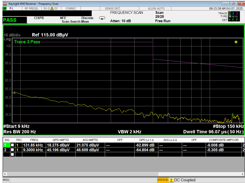
Plot 7-25. Line-Conducted Test Plot (L1) – Digitizer (Hover)
