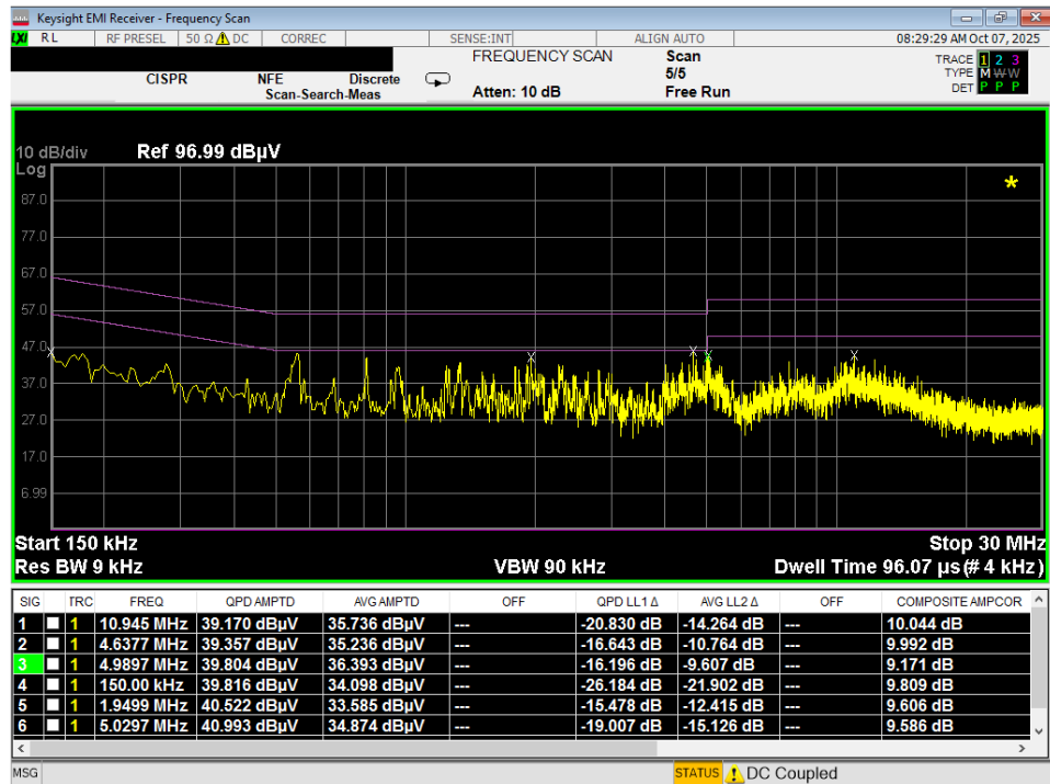
Plot 7-30. Line-Conducted Test Plot (L1) – Digitizer (Eraser)
