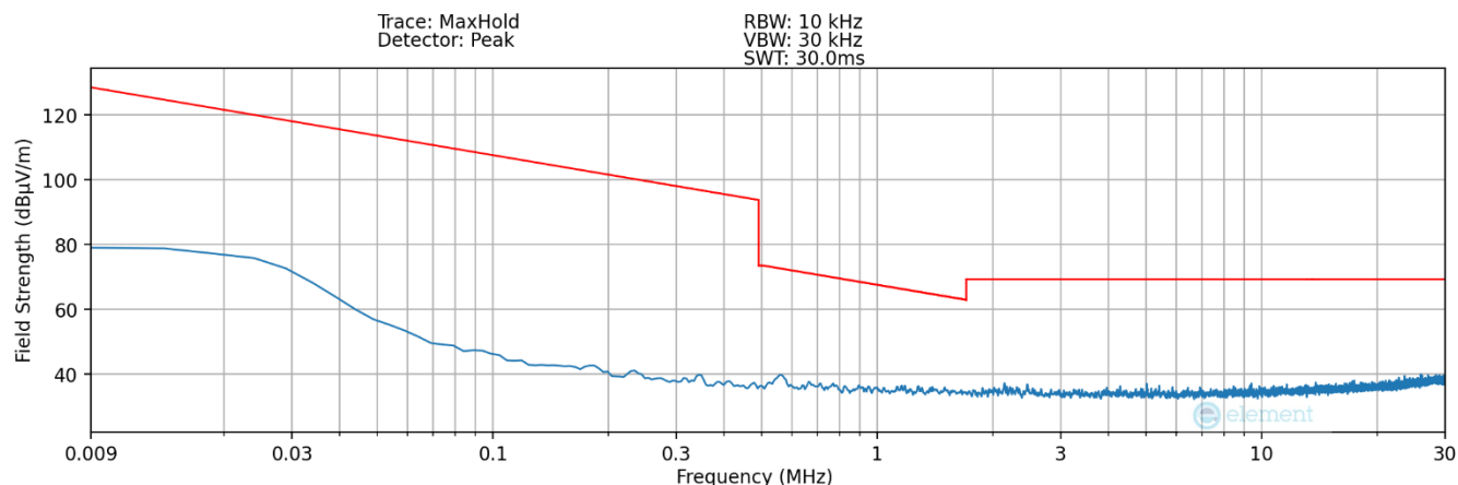
Plot 7-12Radiated Spurious Plot 9kHz – 30MHz (Pol. Y – Digitizer – Hover)
