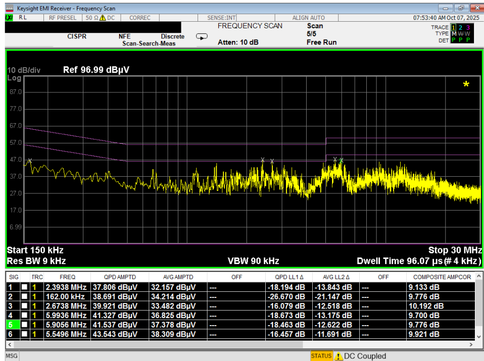
Plot 7-22. Line-Conducted Test Plot (L1) – Digitizer (Click)
