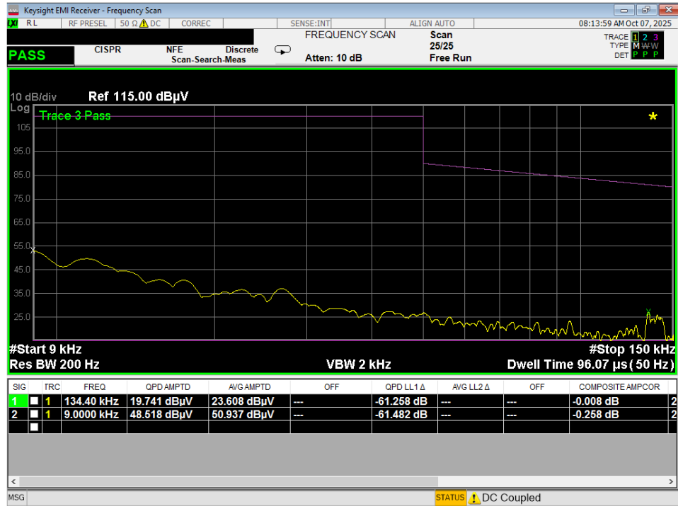
Plot 7-27. Line-Conducted Test Plot (N) – Digitizer (Hover)
