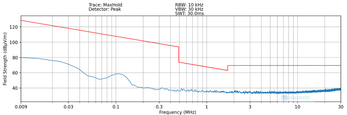
Plot 7-7. Radiated Spurious Plot 9kHz – 30MHz (Pol. Z – Device to Device)
