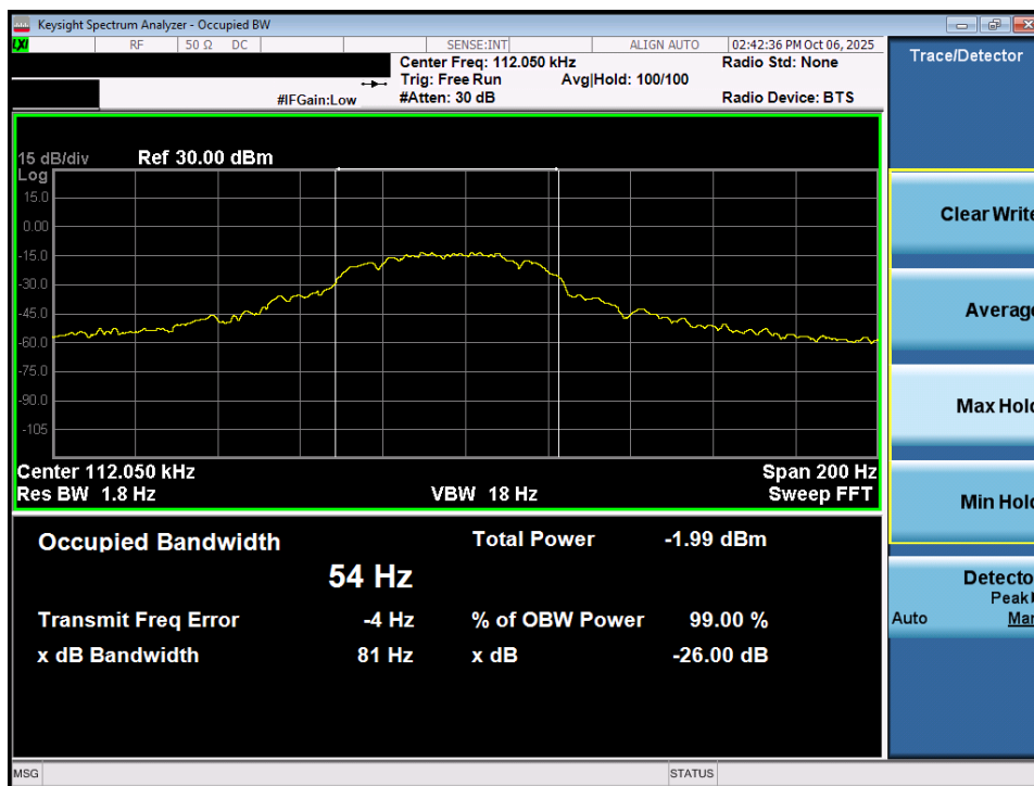
Plot 7-1. Occupied Bandwidth Measurement – Device to Device
