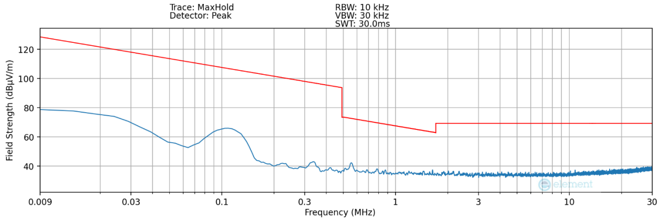
Plot 7-5. Radiated Spurious Plot 9kHz – 30MHz (Pol. X – Device to Device)
