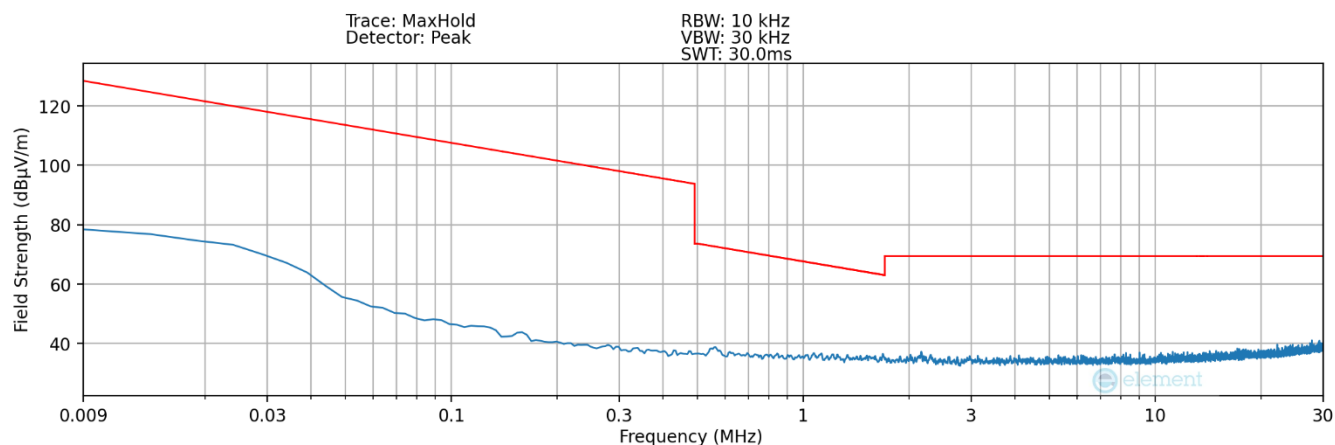
Plot 7-13. Radiated Spurious Plot 9kHz – 30MHz (Pol. Z – Digitizer – Hover)
