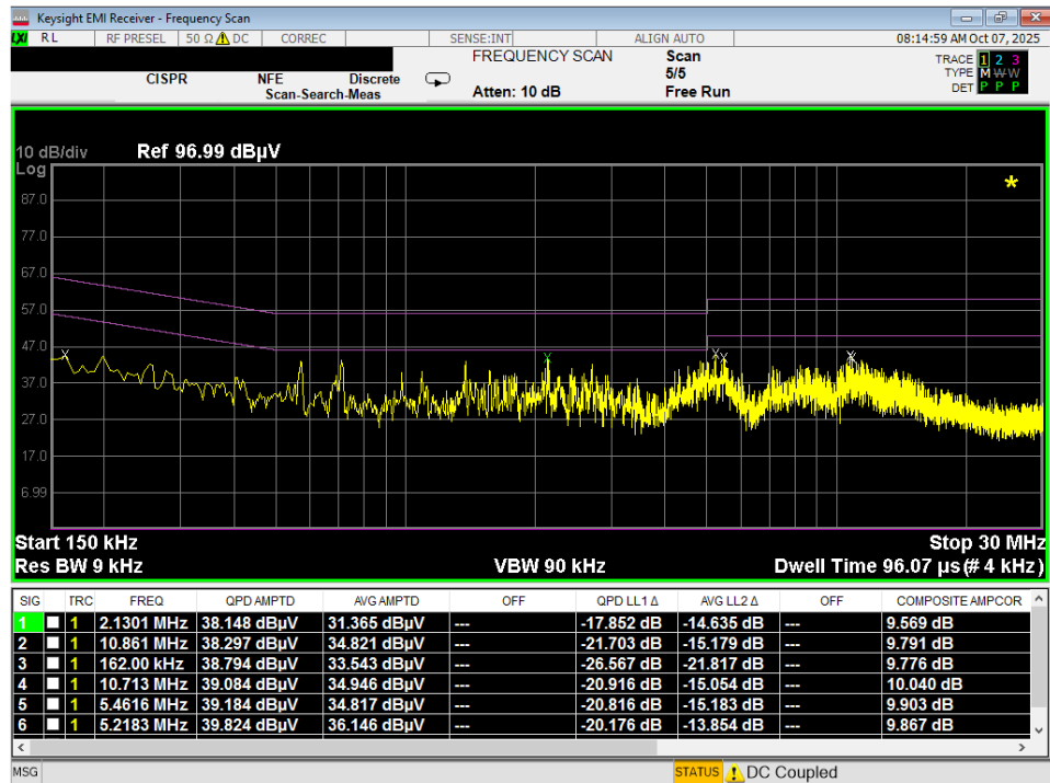
Plot 7-26. Line-Conducted Test Plot (L1) – Digitizer (Hover)
