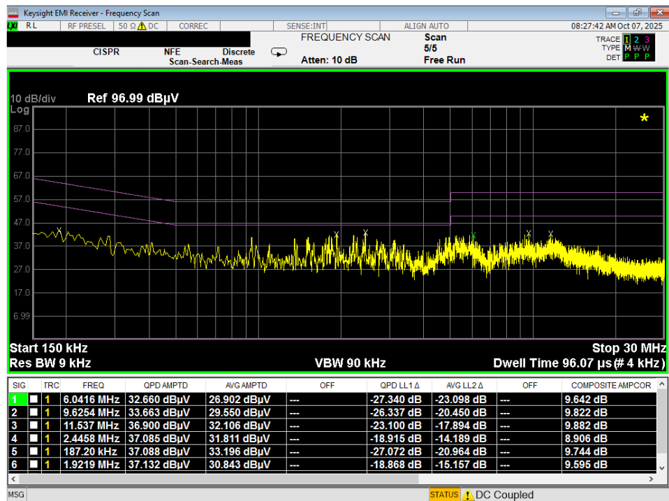
Plot 7-32. Line-Conducted Test Plot (N) – Digitizer (Eraser)
