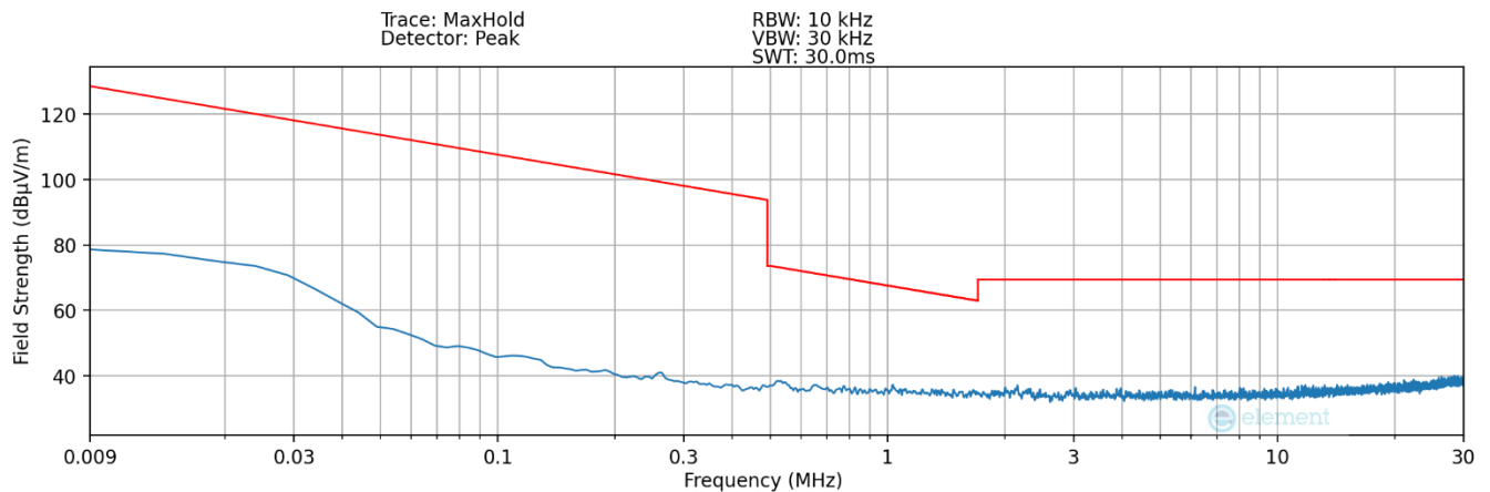
Plot 7-10. Radiated Spurious Plot 9kHz – 30MHz (Pol. Z– Digitizer – Click)
