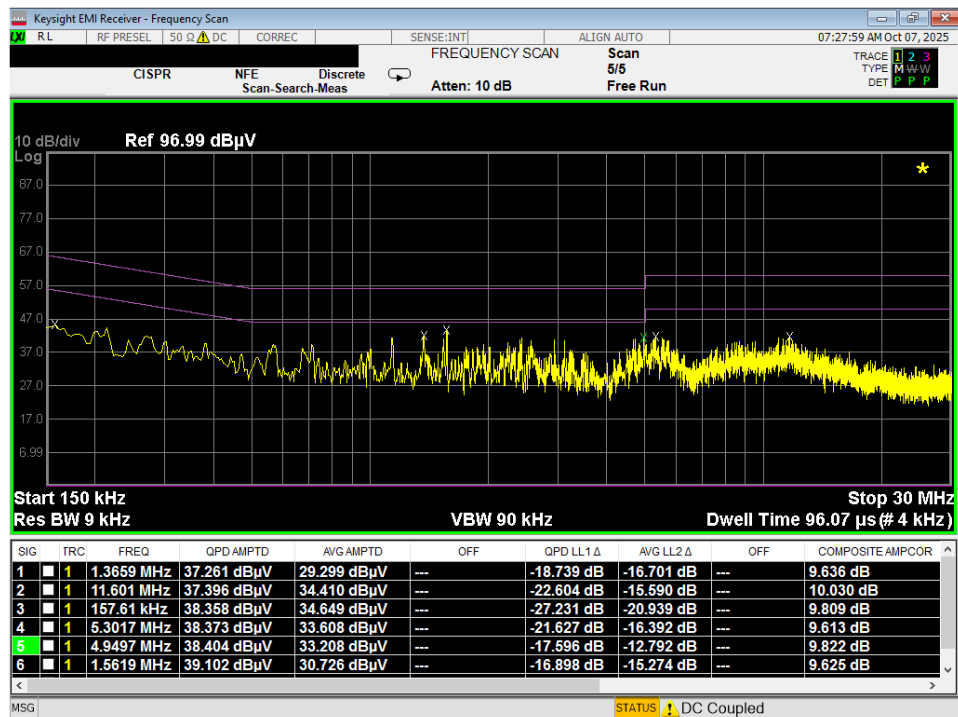
Plot 7-20. Line-Conducted Test Plot (N) – Device to Device
