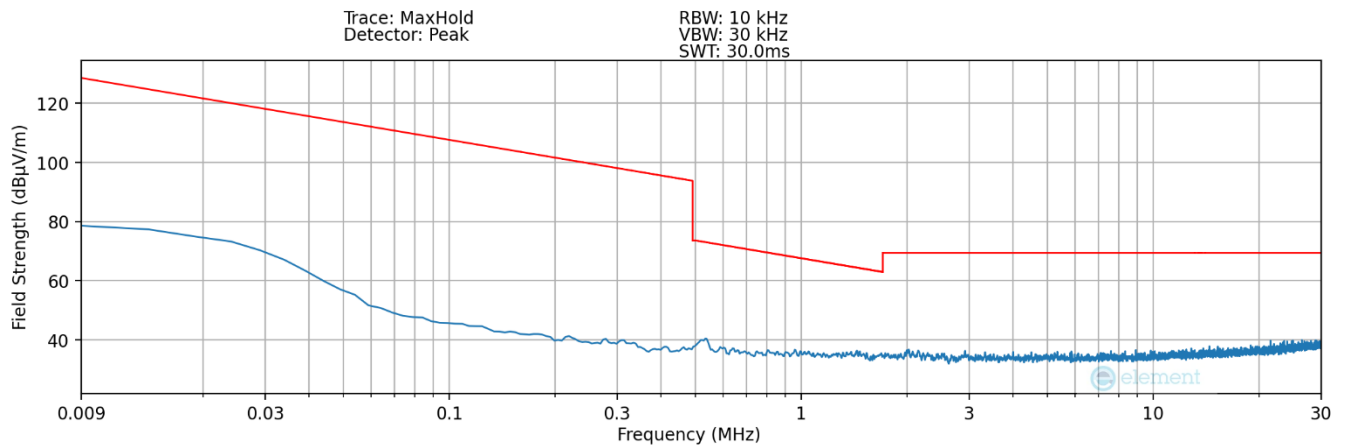
Plot 7-9Radiated Spurious Plot 9kHz – 30MHz (Pol. Y – Digitizer – Click)
