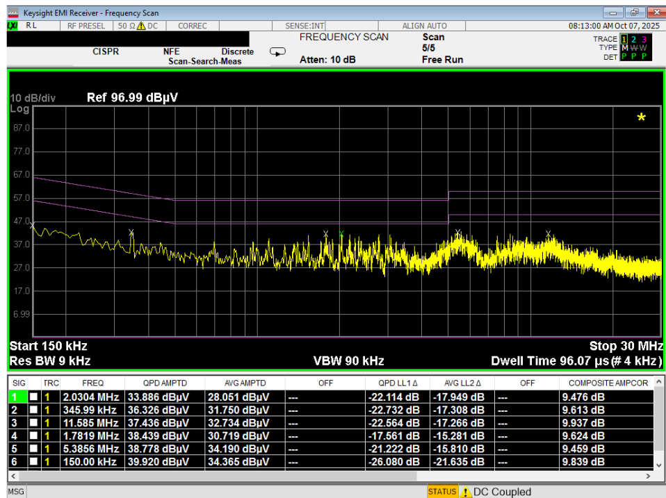
Plot 7-28. Line-Conducted Test Plot (N) – Digitizer (Hover)
