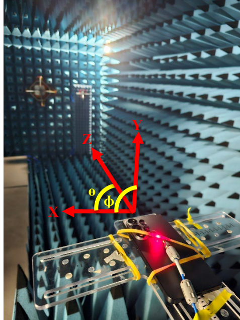
Figure 1: Geometry for SM-S948B/DS for Radiation patterns.
