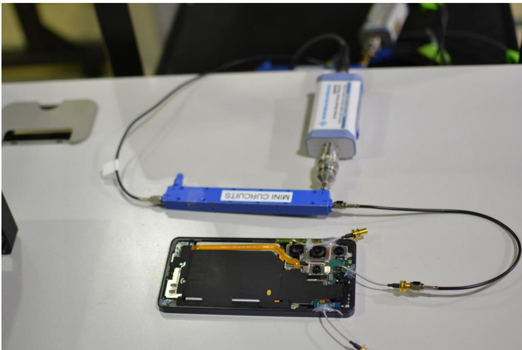
Test Setup Photo 6 – Conducted Test Setup (Figure 6-1g)
