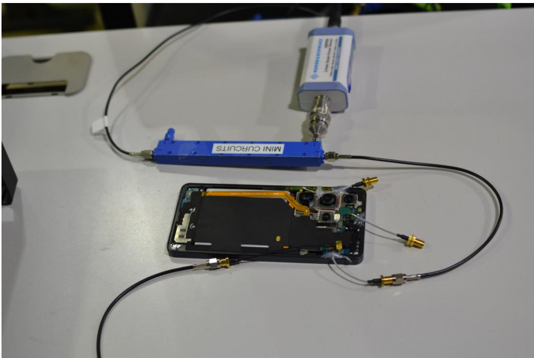
Test Setup Photo 4 – Conducted Test Setup (Figure 6-1d)
