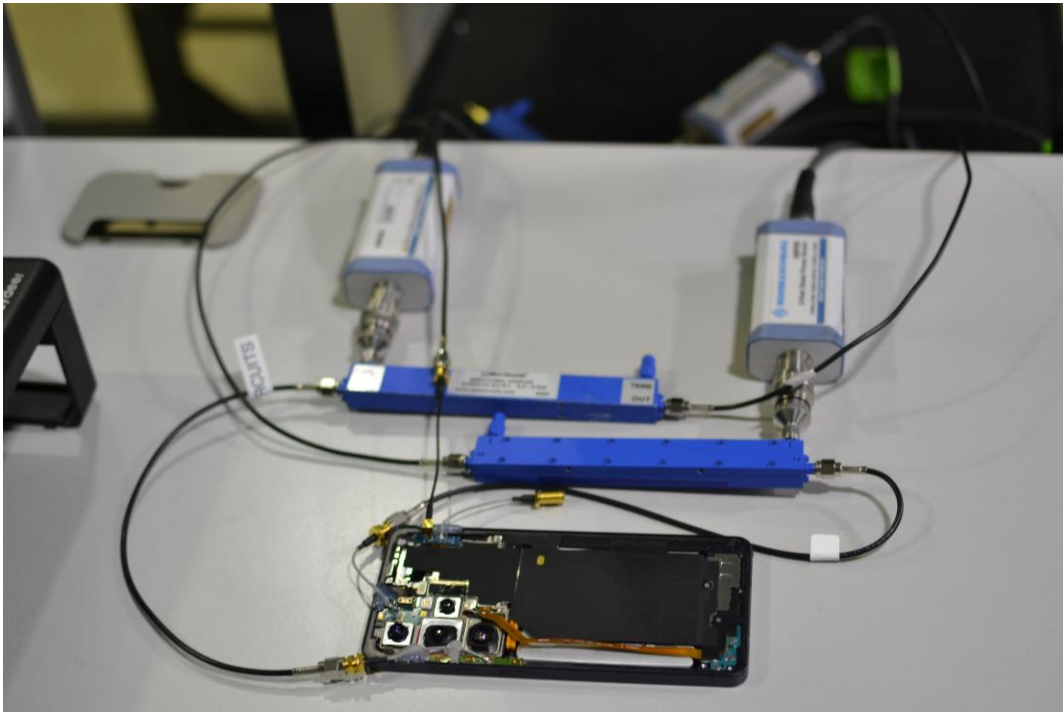
Test Setup Photo 8 – Conducted Test Setup (Figure 6-1e)
