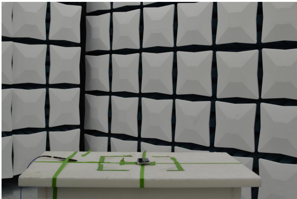
Figure 8. Test Setup – WCP – 30MHz-1GHz
