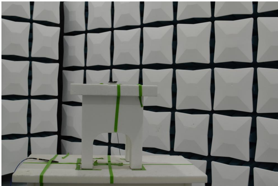
Figure 4. Test Setup – WCP
