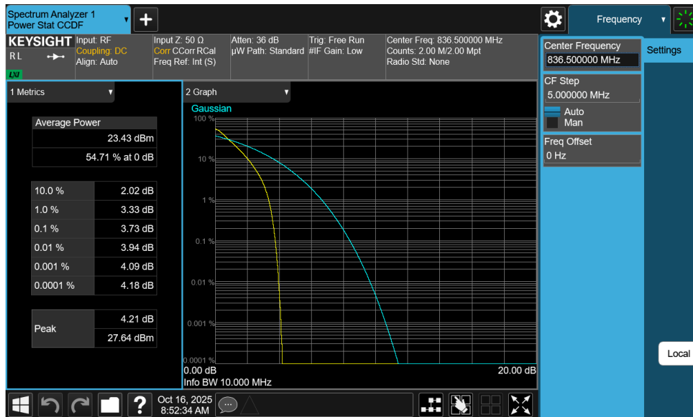
Plot 7-162. Peak-Average Ratio Plot (LTE Band 5 - 10MHz QPSK - Full RB - Ant1)
