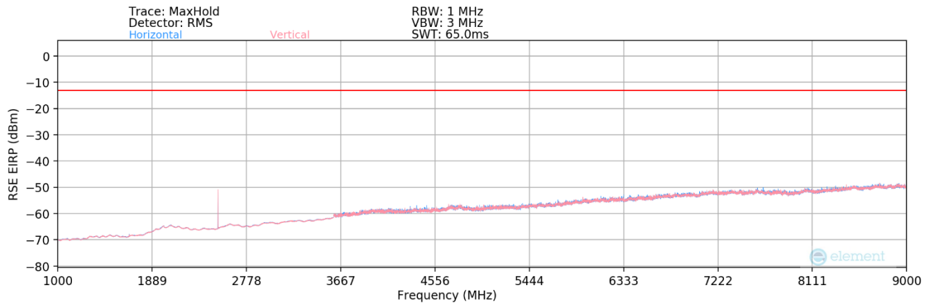
Plot 7-186. Radiated Spurious Plot (NR Band n5 – Ant2)
