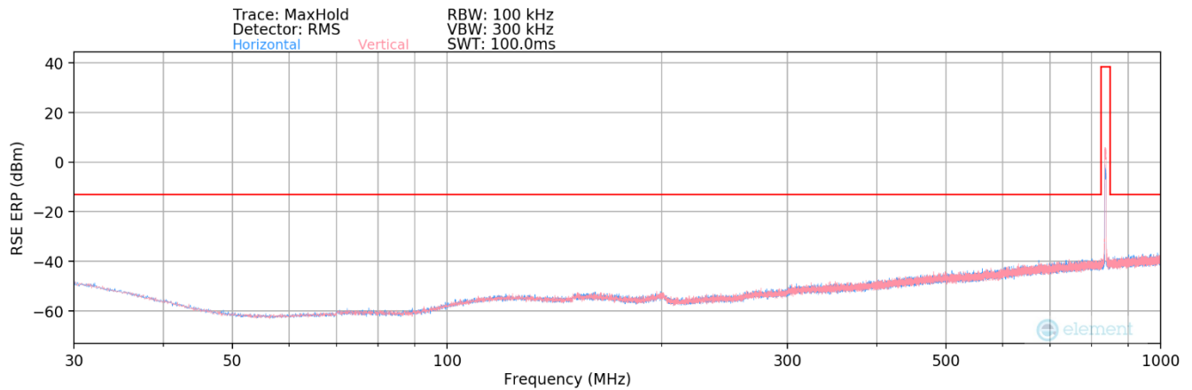
Plot 7-181. Radiated Spurious Plot (WCDMA Cell – Ant1)
