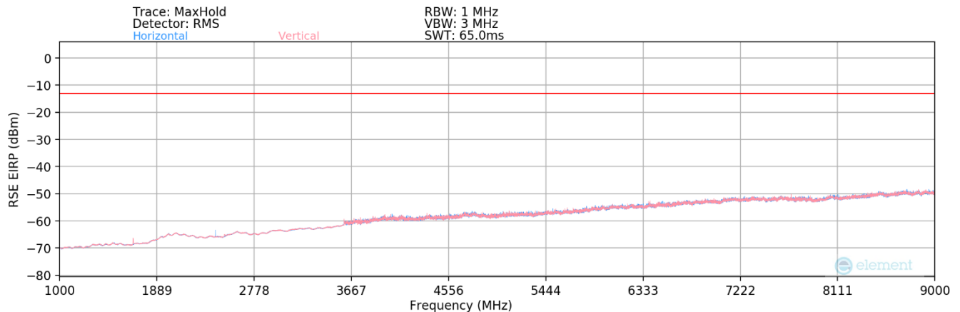
Plot 7-182. Radiated Spurious Plot (WCDMA Cell – Ant1)
