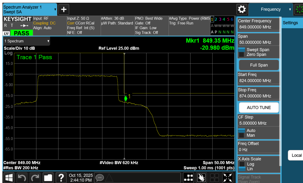
Plot 7-148. Upper Band Edge Plot (NR Band n5 – 20.0MHz - Full RB - Ant2)
