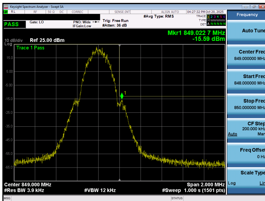
Plot 7-156. Upper Band Edge Plot (GPRS Cell – Ch. 251 – Ant2)
