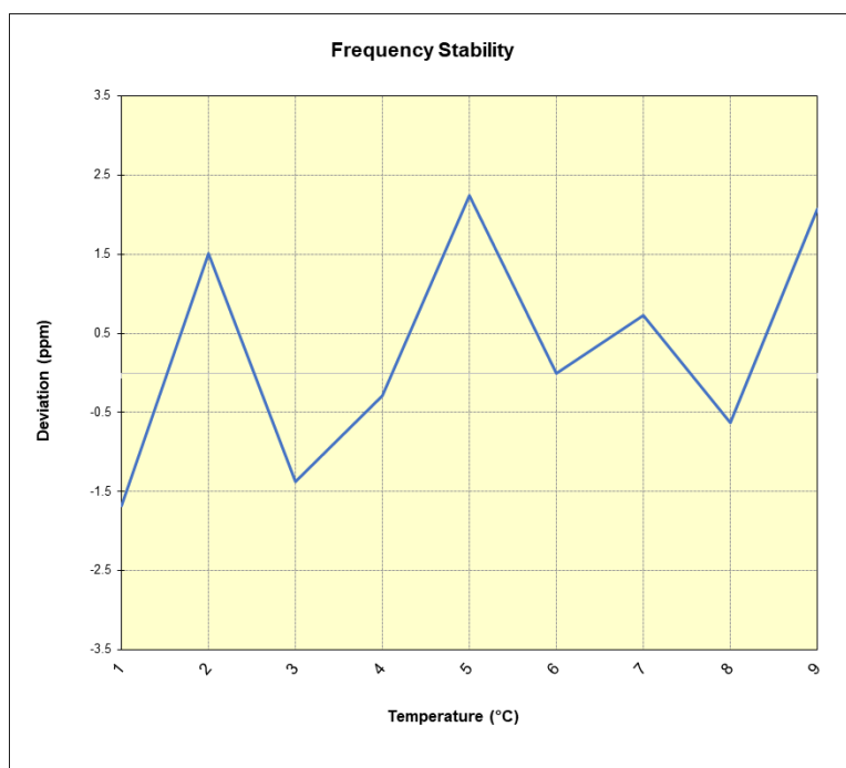
Plot 7-191. LTE Band 5 Frequency Stability Chart
