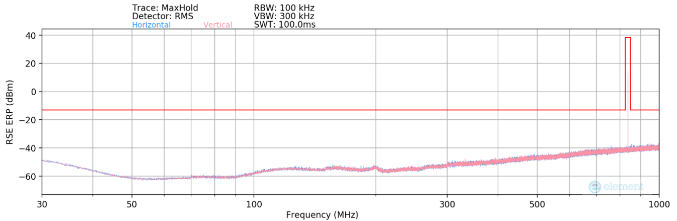
Plot 7-187. Radiated Spurious Plot (GPRS Cell – Ant2)
