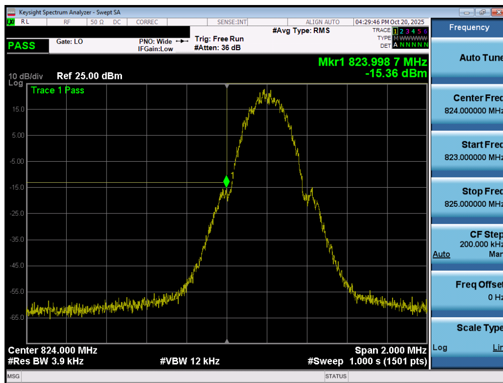
Plot 7-155. Lower Band Edge Plot (GPRS Cell – Ch. 128 – Ant2)
