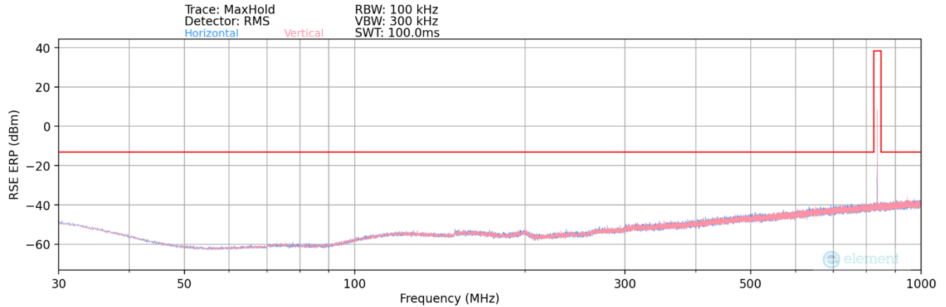
Plot 7-185. Radiated Spurious Plot (NR Band n5 – Ant2)
