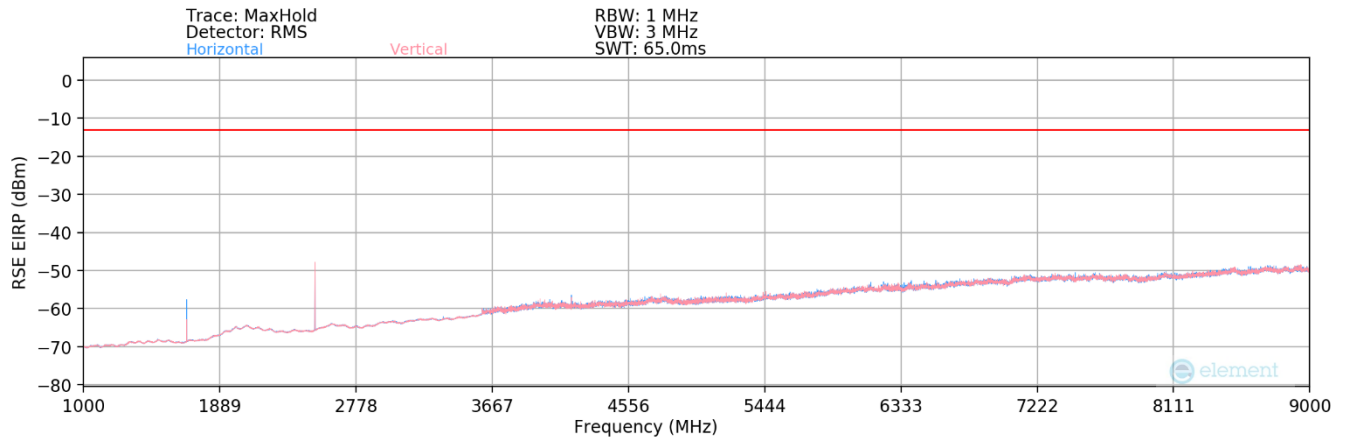
Plot 7-180. Radiated Spurious Plot (GPRS Cell – Ant1)
