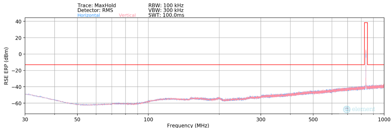
Plot 7-189. Radiated Spurious Plot (WCDMA Cell – Ant2)
