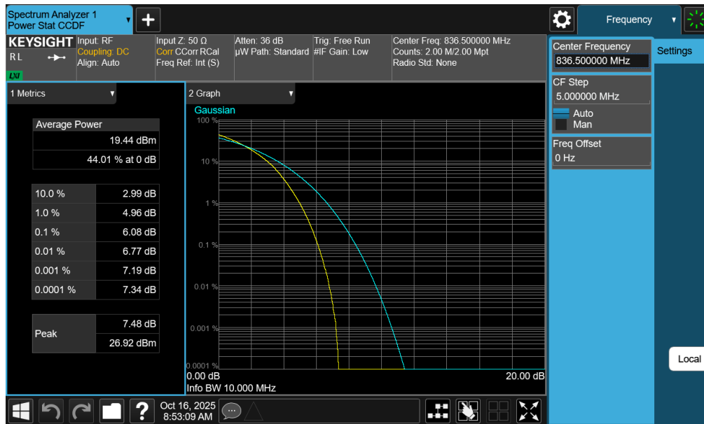
Plot 7-163. Peak-Average Ratio Plot (LTE Band 5 - 10MHz 256-QAM - Full RB - Ant1)
