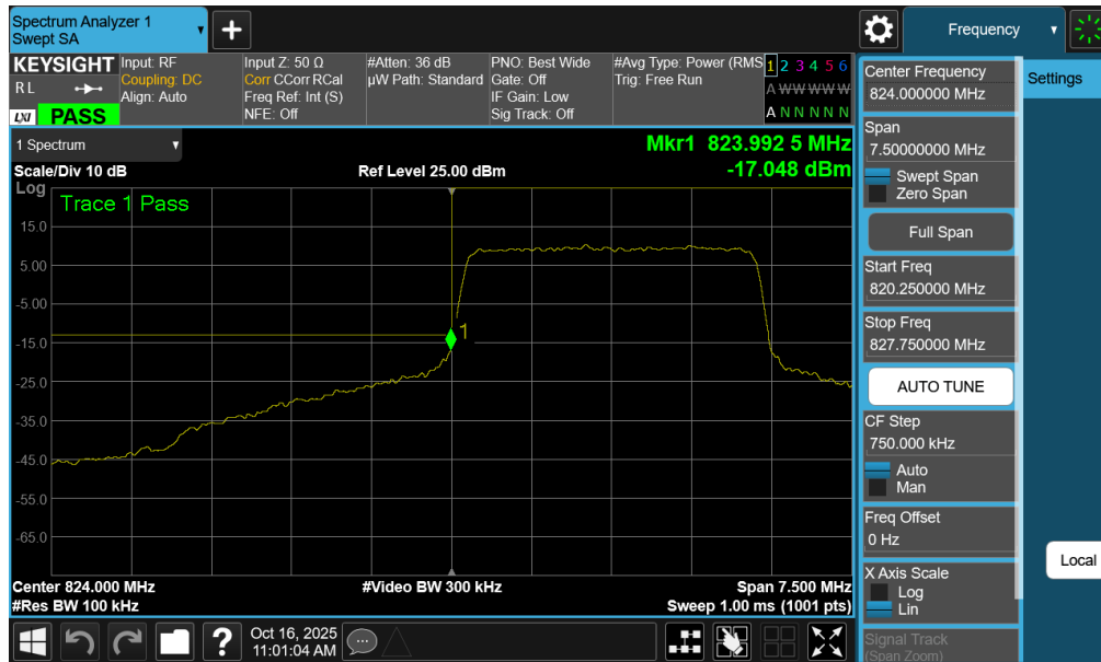
Plot 7-143. Lower Band Edge Plot (LTE Band 5 - 3MHz QPSK – Full RB - Ant2)
