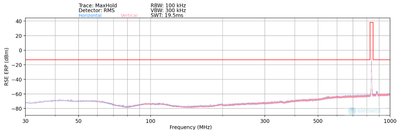
Plot 7-183. Radiated Spurious Plot (LTE Band 5 – Ant2)
