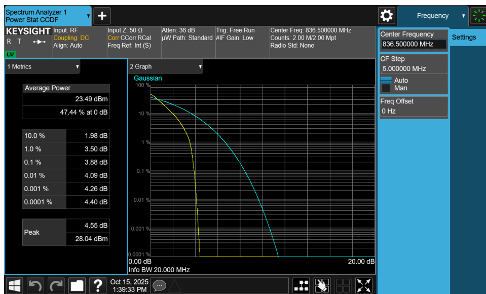
Plot 7-172. Peak-Average Ratio Plot (NR Band n5 - 20MHz \pi/2 BPSK - Full RB - Ant2)
