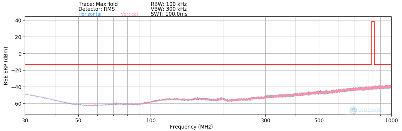
Plot 7-179. Radiated Spurious Plot (GPRS Cell – Ant1)
