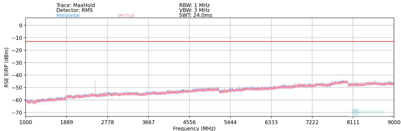
Plot 7-184. Radiated Spurious Plot (LTE Band 5 – Ant2)
