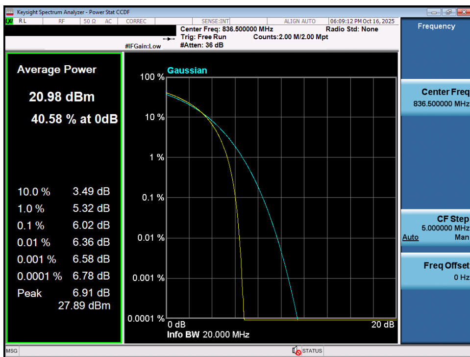
Plot 7-173. Peak-Average Ratio Plot (NR Band n5 - 20MHz QPSK - Full RB - Ant2)
