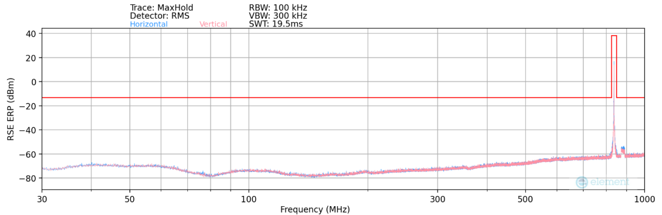
Plot 7-177. Radiated Spurious Plot (NR Band n5 – Ant1)
