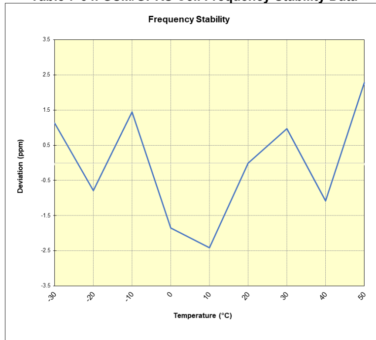
Plot 7-193. GSM/GPRS Cell Frequency Stability Chart
