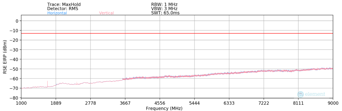
Plot 7-188. Radiated Spurious Plot (GPRS Cell – Ant2)
