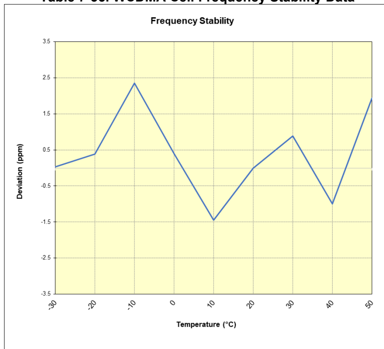
Plot 7-194. WCDMA Cell Frequency Stability Chart
