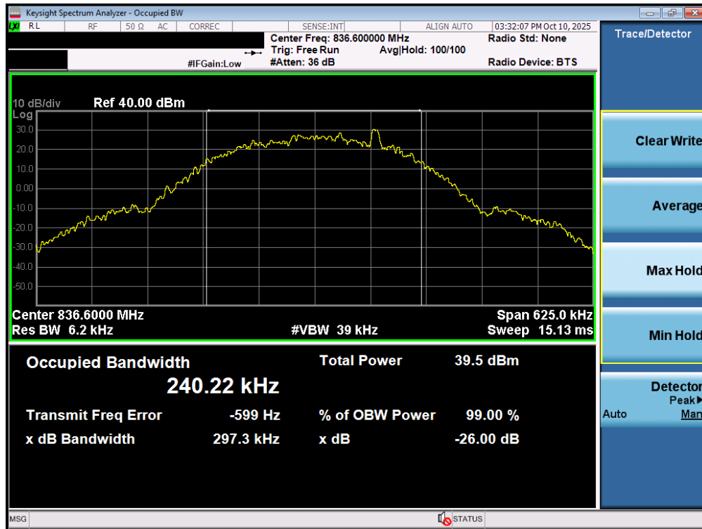
Plot 9-1. Occupied Bandwidth (Spot-check) – GPRS850 (Spot-check)
