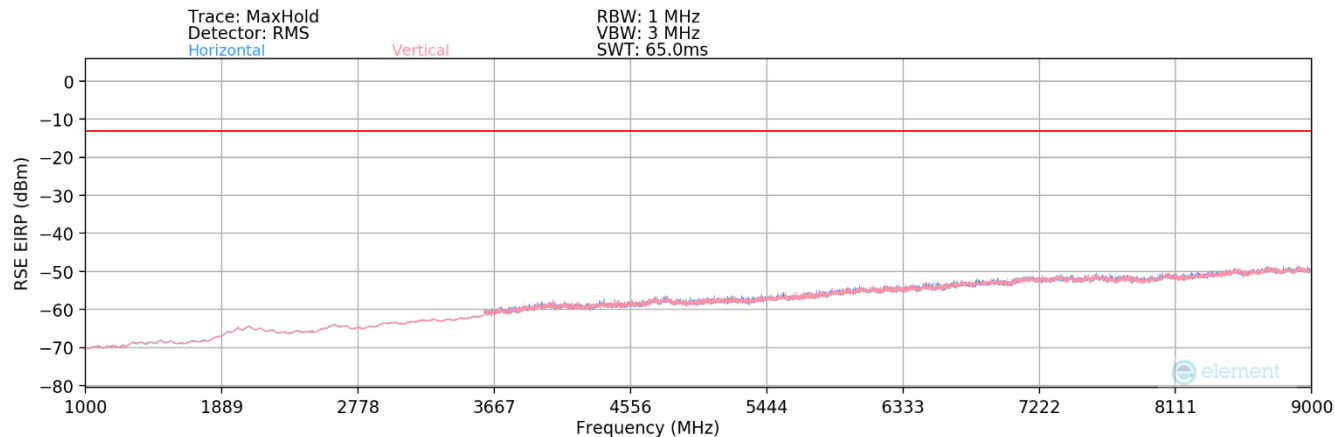
Plot 7-190. Radiated Spurious Plot (WCDMA Cell – Ant2)
