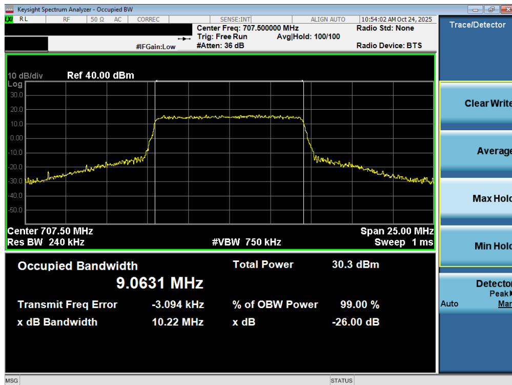
Plot 7-53. Occupied Bandwidth Plot (LTE Band 12 - 10MHz 16-QAM - Full RB – ANT2)
