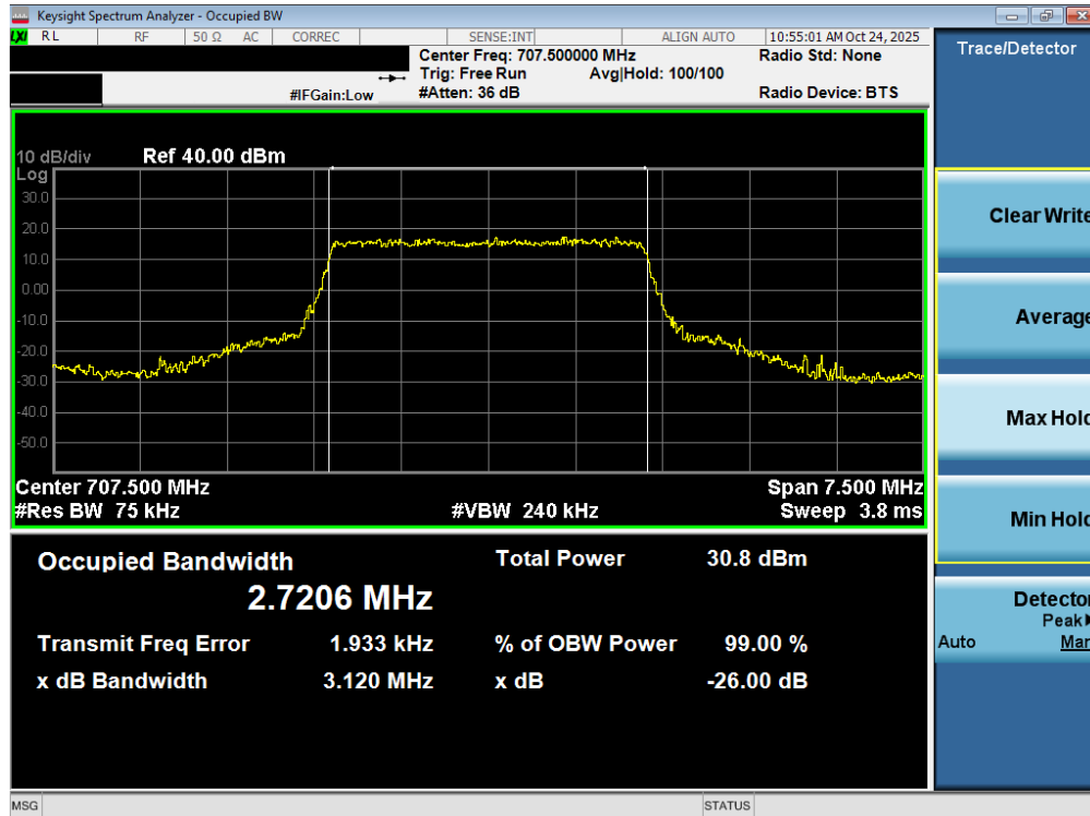
Plot 7-56. Occupied Bandwidth Plot (LTE Band 12 - 3MHz QPSK - Full RB – ANT2)
