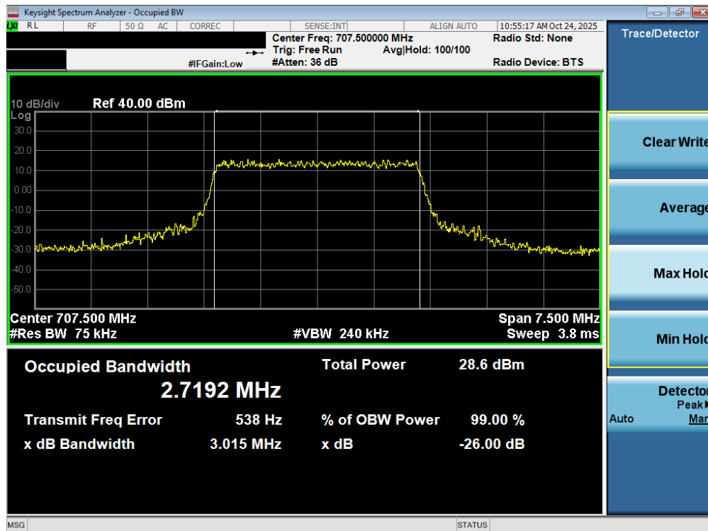
Plot 7-57. Occupied Bandwidth Plot (LTE Band 12 - 3MHz 16-QAM - Full RB – ANT2)
