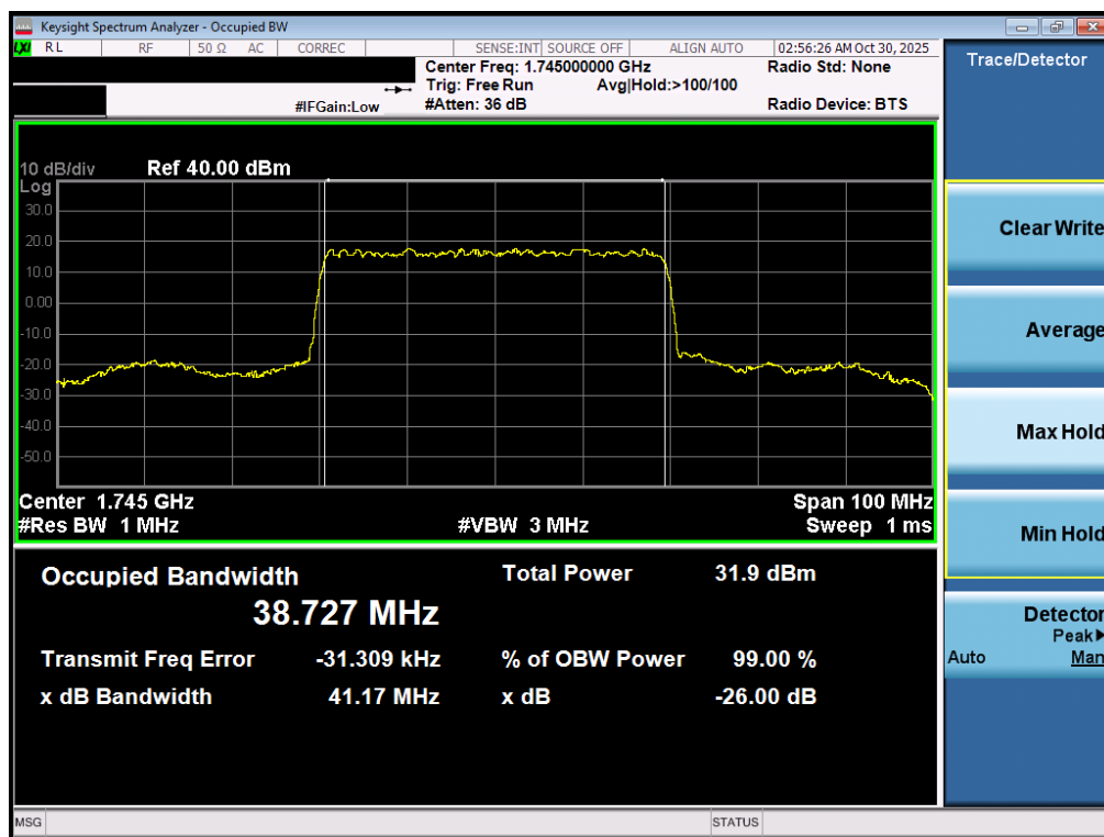
Plot 7-28. Occupied Bandwidth Plot (NR Band n66 - 40.0MHz DFT-s-OFDM BPSK - Full RB – ANT1)
