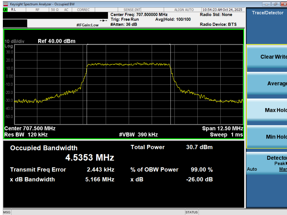
Plot 7-54. Occupied Bandwidth Plot (LTE Band 12 - 5MHz QPSK - Full RB – ANT2)
