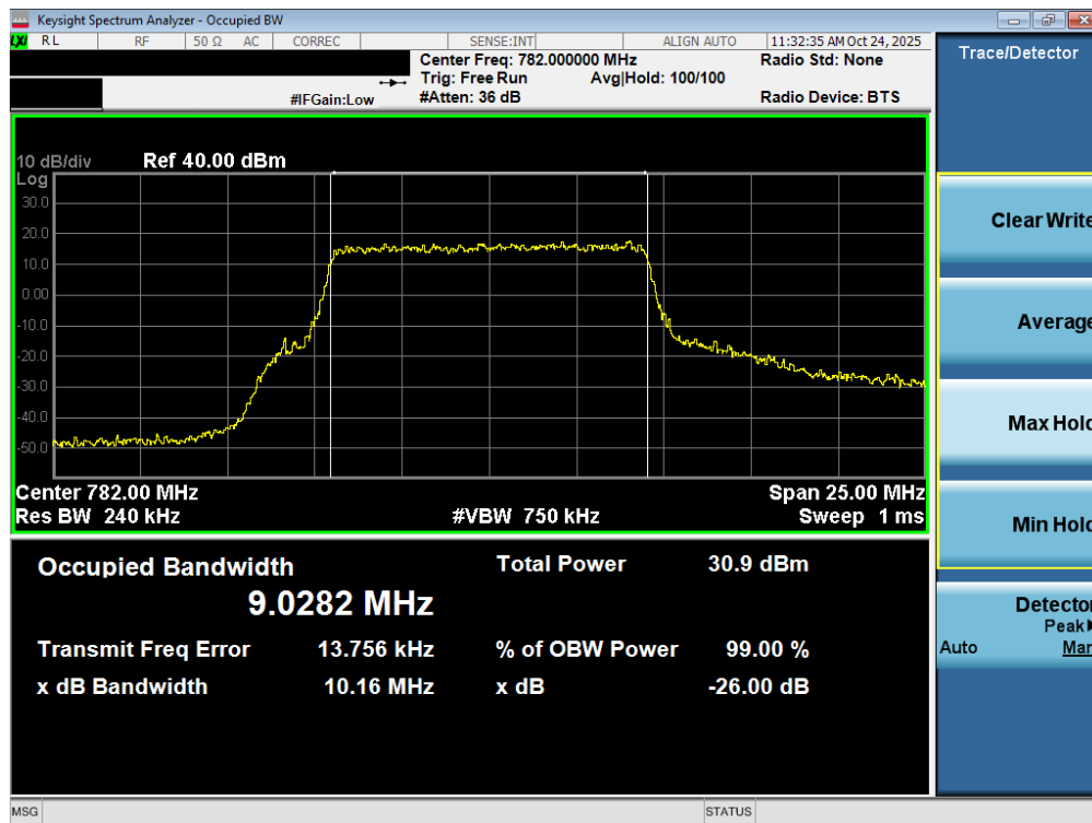
Plot 7-60. Occupied Bandwidth Plot (LTE Band 13 - 10MHz QPSK - Full RB – ANT2)
