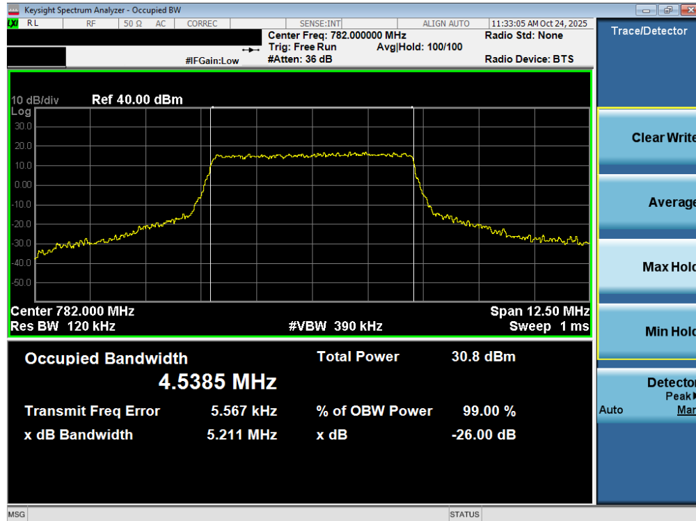
Plot 7-62. Occupied Bandwidth Plot (LTE Band 13 - 5MHz QPSK - Full RB – ANT2)
