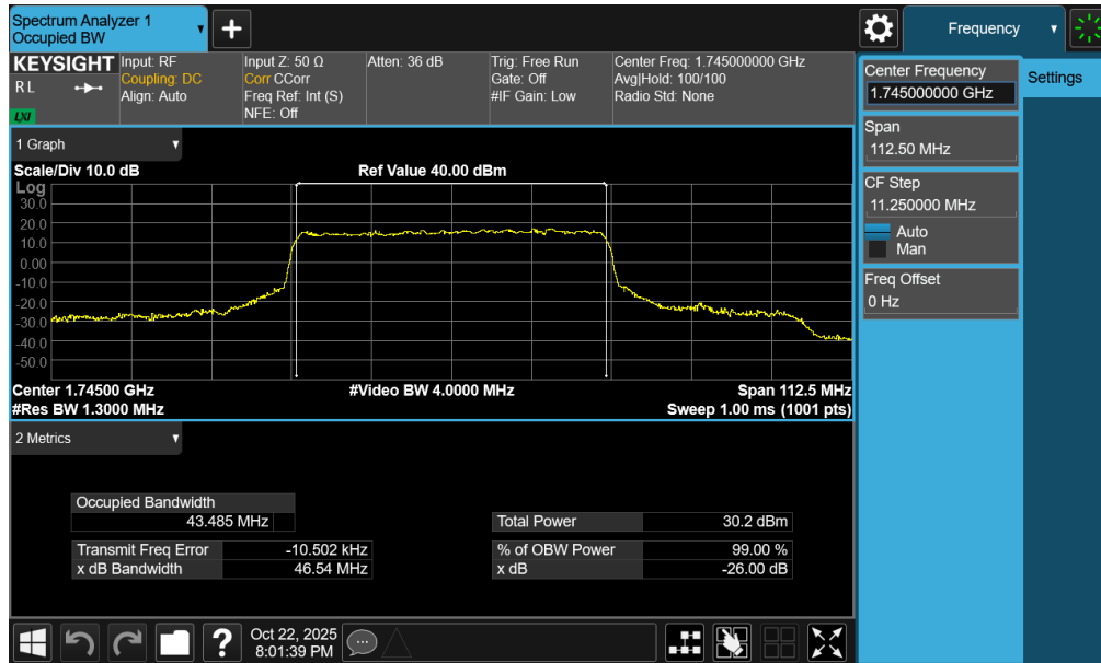
Plot 7-66. Occupied Bandwidth Plot (NR Band n66 - 45.0MHz CP-OFDM 16QAM - Full RB – ANT2)
