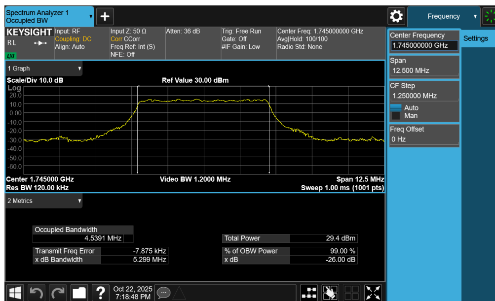
Plot 7-51. Occupied Bandwidth Plot (NR Band n66 - 5.0MHz CP-OFDM 16QAM - Full RB – ANT1)
