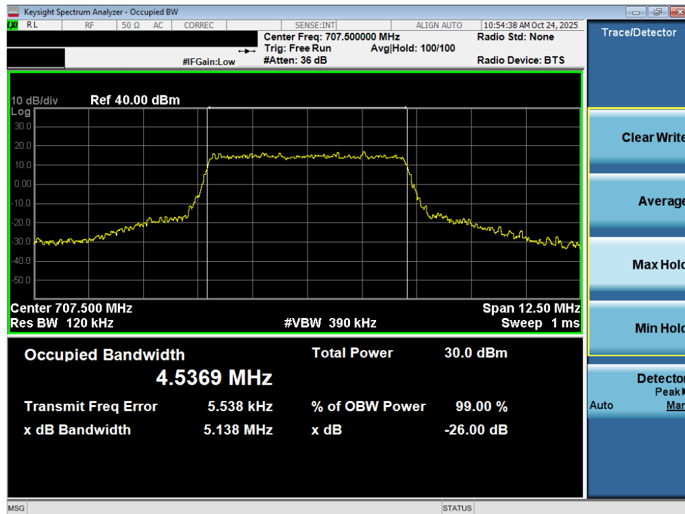
Plot 7-55. Occupied Bandwidth Plot (LTE Band 12 - 5MHz 16-QAM - Full RB – ANT2)
