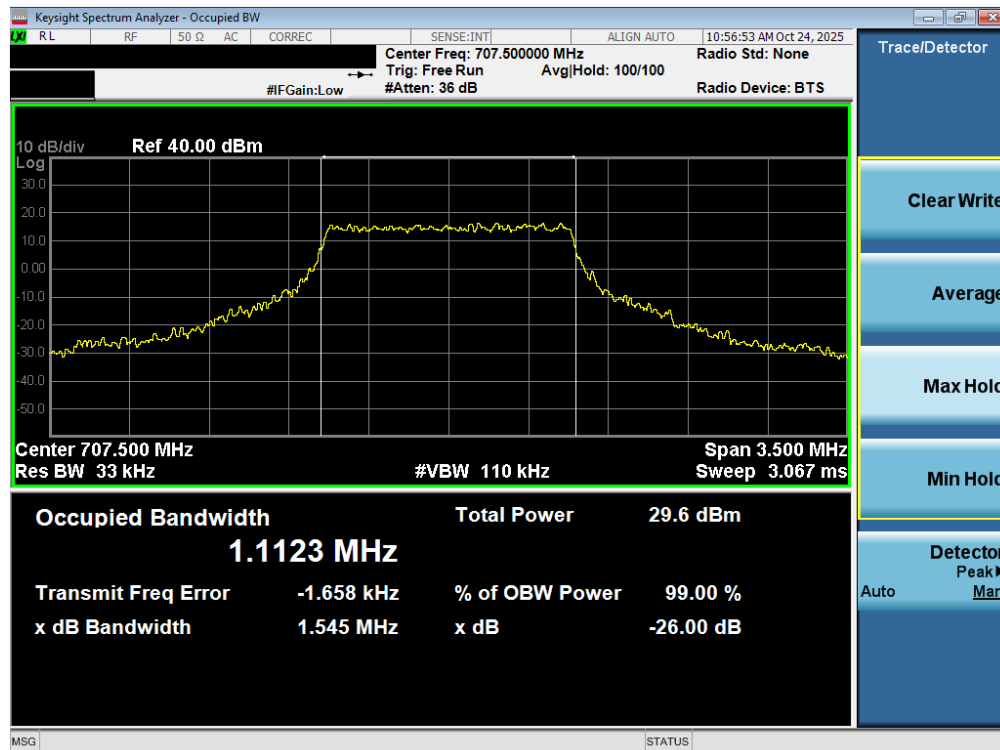
Plot 7-59. Occupied Bandwidth Plot (LTE Band 12 – 1.4MHz 16-QAM - Full RB – ANT2)
