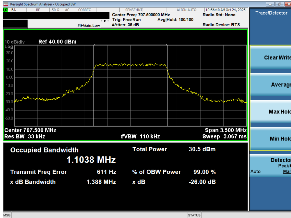
Plot 7-58. Occupied Bandwidth Plot (LTE Band 12 – 1.4MHz QPSK - Full RB – ANT2)
