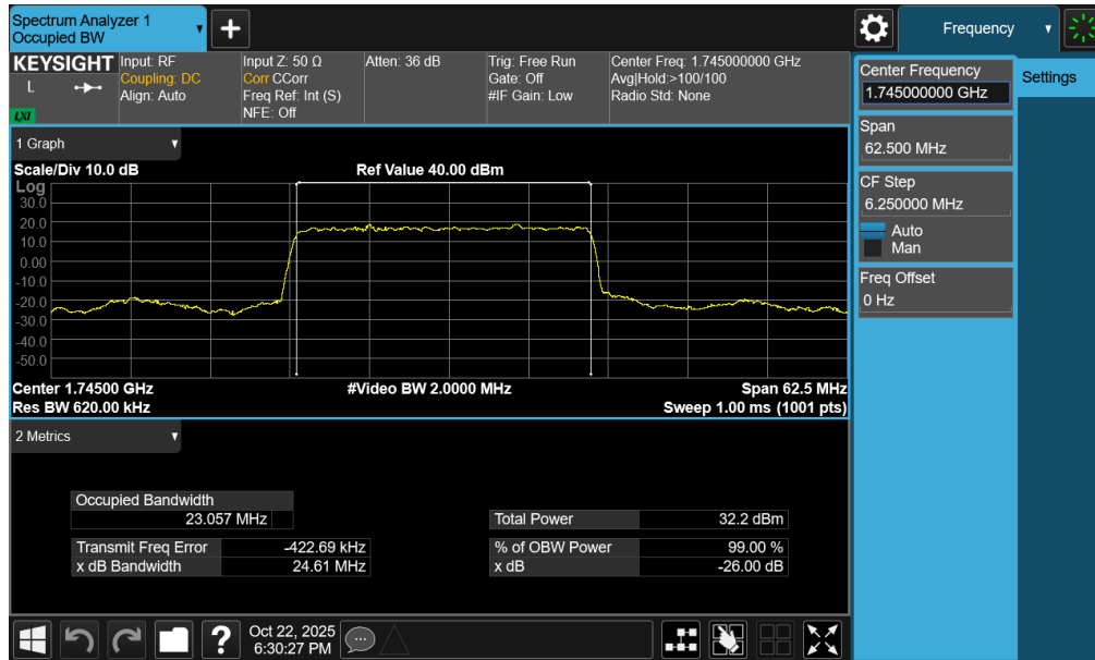
Plot 7-37. Occupied Bandwidth Plot (NR Band n66 - 25.0MHz DFT-s-OFDM BPSK - Full RB – ANT1)
