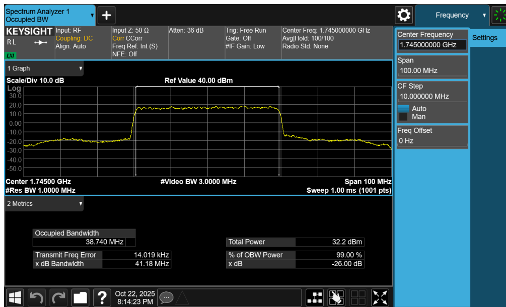
Plot 7-67. Occupied Bandwidth Plot (NR Band n66 - 40.0MHz DFT-s-OFDM BPSK - Full RB – ANT2)
