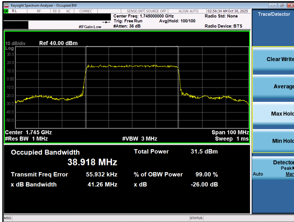
Plot 7-29. Occupied Bandwidth Plot (NR Band n66 - 40.0MHz CP-OFDM QPSK - Full RB – ANT1)
