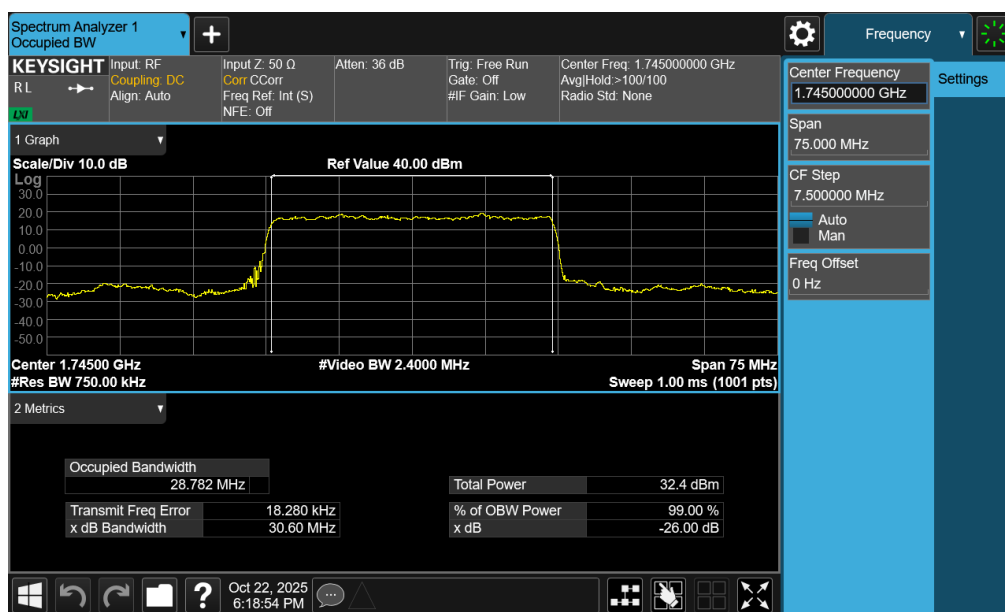
Plot 7-34. Occupied Bandwidth Plot (NR Band n66 - 30.0MHz DFT-s-OFDM BPSK - Full RB – ANT1)
