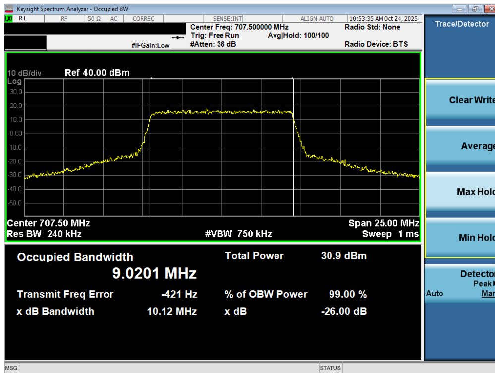
Plot 7-52. Occupied Bandwidth Plot (LTE Band 12 - 10MHz QPSK - Full RB – ANT2)
