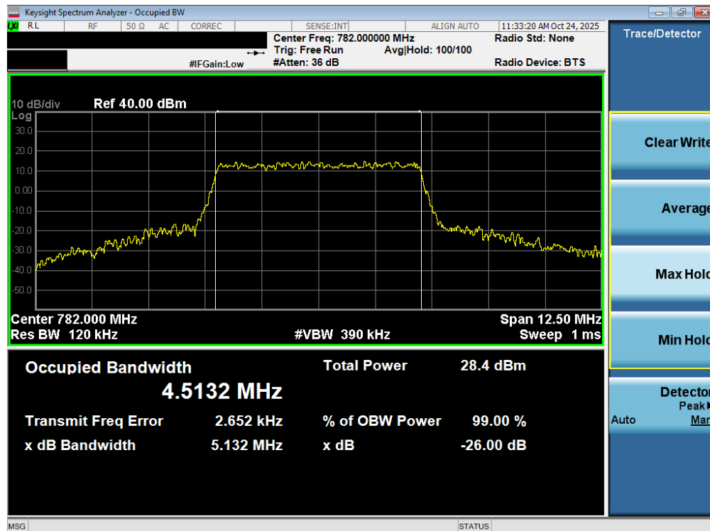
Plot 7-63. Occupied Bandwidth Plot (LTE Band 13 - 5MHz 16-QAM - Full RB – ANT2)
