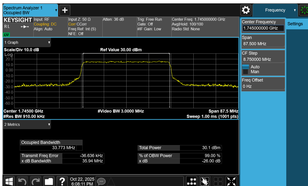
Plot 7-33. Occupied Bandwidth Plot (NR Band n66 - 35.0MHz CP-OFDM 16QAM - Full RB – ANT1)
