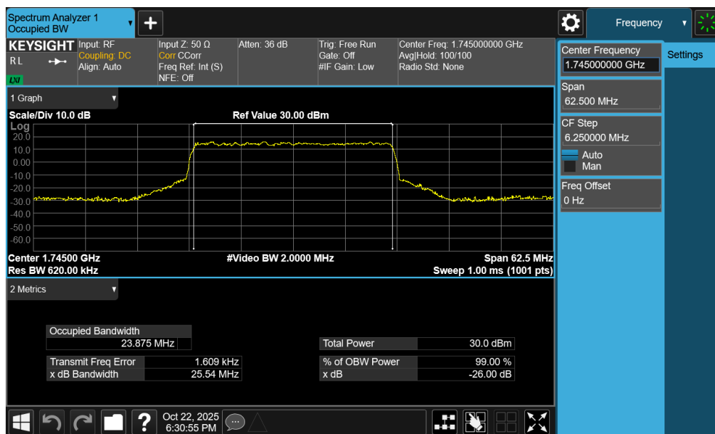
Plot 7-38. Occupied Bandwidth Plot (NR Band n66 - 25.0MHz CP-OFDM QPSK - Full RB – ANT1)
