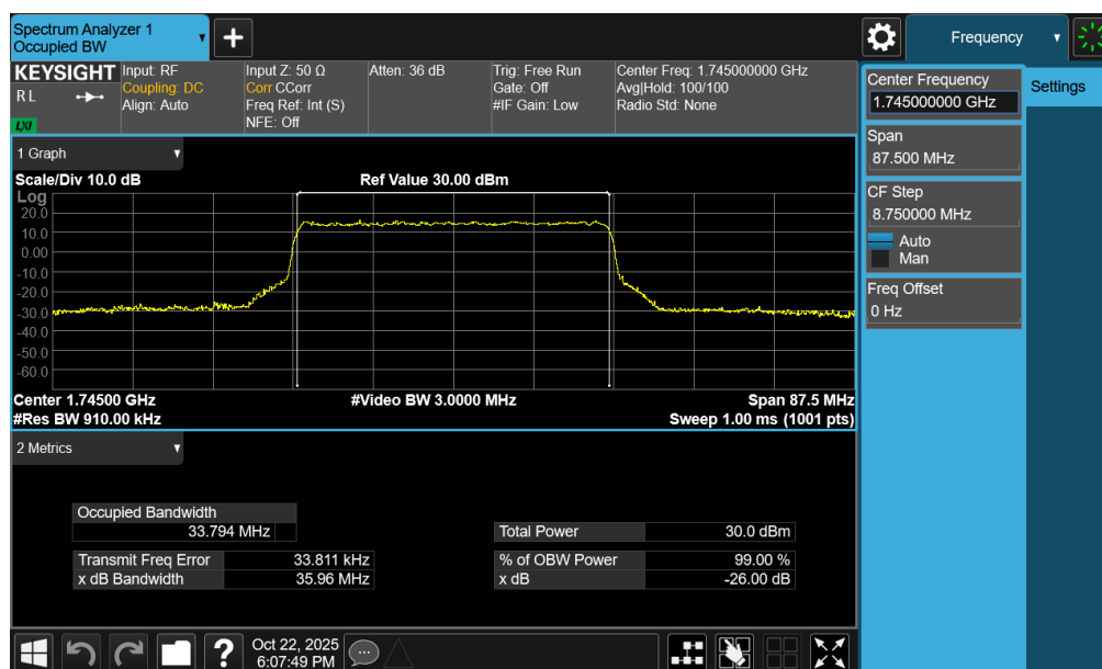
Plot 7-32. Occupied Bandwidth Plot (NR Band n66 - 35.0MHz CP-OFDM QPSK - Full RB – ANT1)
