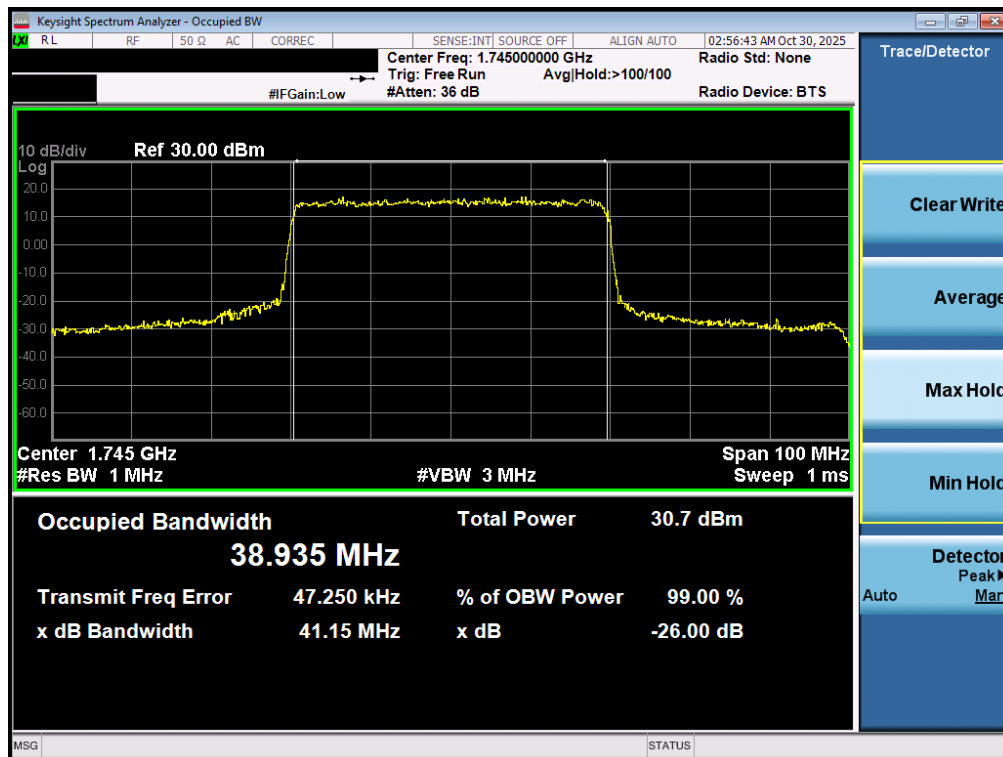
Plot 7-30. Occupied Bandwidth Plot (NR Band n66 - 40.0MHz CP-OFDM 16QAM - Full RB – ANT1)
