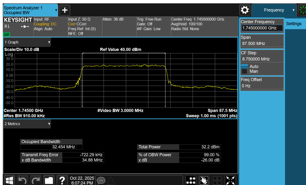
Plot 7-31. Occupied Bandwidth Plot (NR Band n66 - 35.0MHz DFT-s-OFDM BPSK - Full RB – ANT1)
