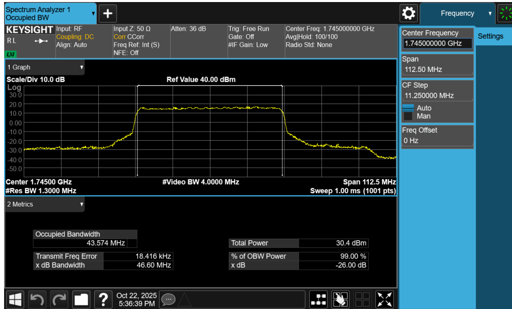
Plot 7-27. Occupied Bandwidth Plot (NR Band n66 - 45.0MHz CP-OFDM 16QAM - Full RB – ANT1)
