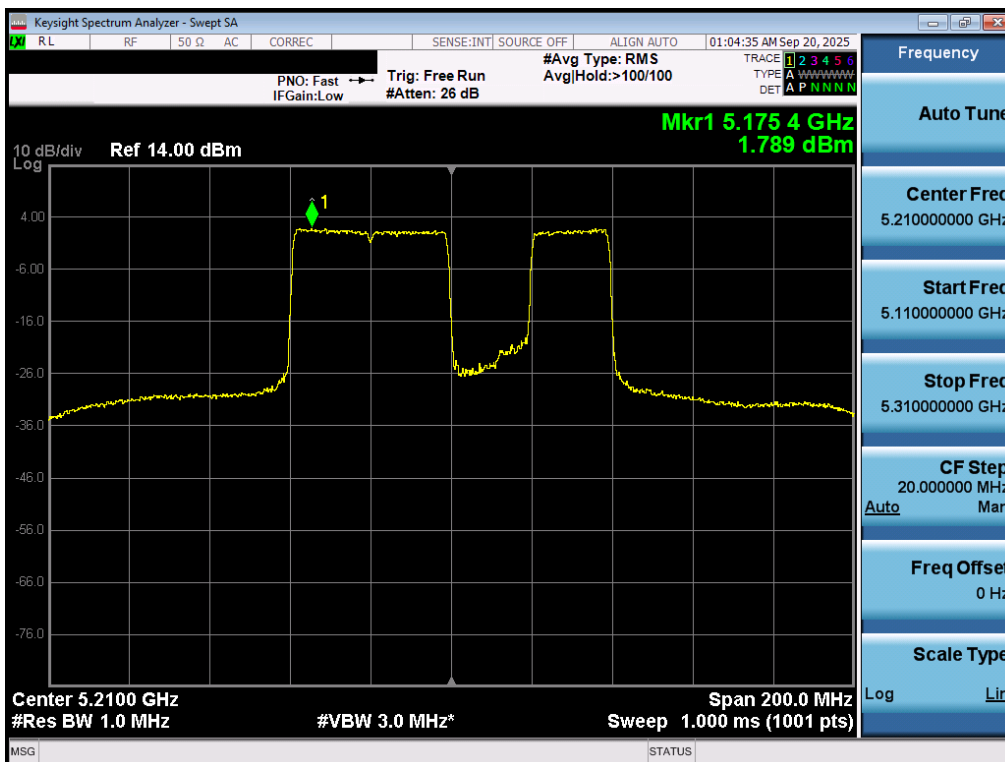
Plot 7-100. Power Spectral Density Plot MIMO ANT2 (80MHz BW 802.11be – 20MHz Puncture (UNII Band 1) – Ch. 42)
