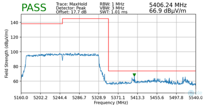
Plot 7-179. Radiated Upper Band Edge Plot MIMO (Peak – UNII Band 2A)
