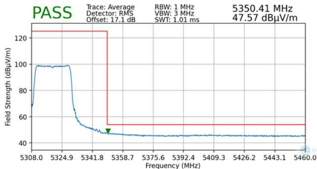
Plot 7-147. Radiated Upper Band Edge Plot MIMO (Average – UNII Band 2A – 242 Tones)
