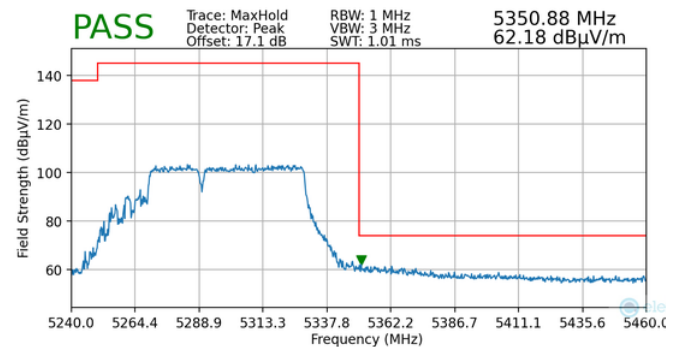
Plot 7-168. Radiated Upper Band Edge Plot MIMO (Peak – UNII Band 2A – 484+242 Tones)
