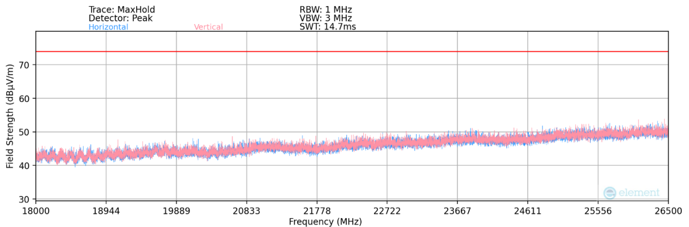
Plot 7-114. Radiated Spurious Plot 18GHz - 26.5GHz (802.11be)
