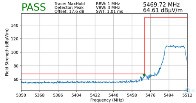
Plot 7-150. Radiated Lower Band Edge Plot MIMO (Peak – UNII Band 2C – 242 Tones)
