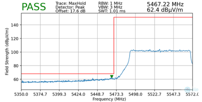
Plot 7-180. Radiated Lower Band Edge Plot MIMO (Peak – UNII Band 2C – 996 Tones)
