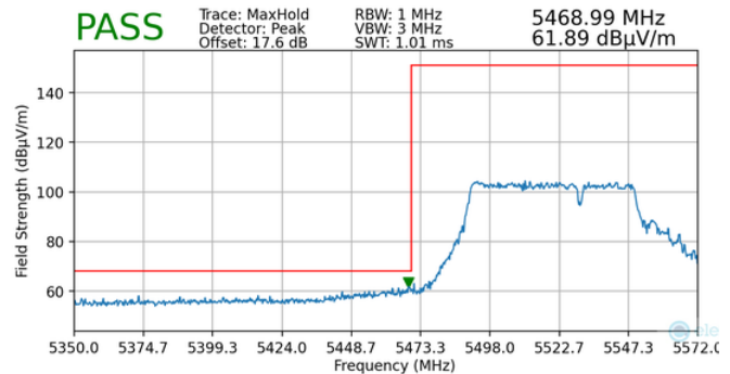
Plot 7-170. Radiated Lower Band Edge Plot MIMO (Peak – UNII Band 2C – 484+242 Tones)
