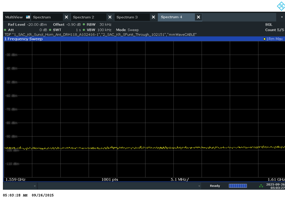
Plot 7-48. Radiated Spurious Pre-Scan 1559 - 1610 MHz - CH.9 – GPS band
