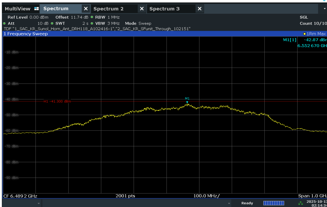
Plot 7-38. UWB Average Power Measurement - CH.5 – HPRF
