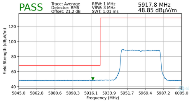
Plot 7-91. Radiated Lower Band Edge Plot MIMO (Average – UNII Band 5)
