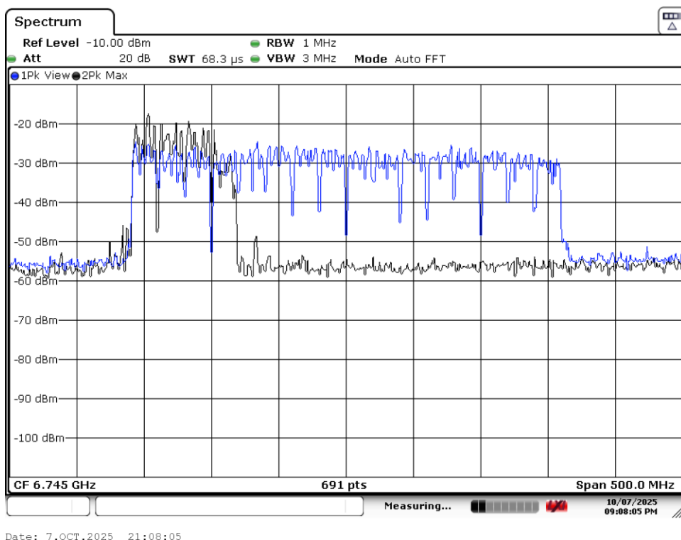
Plot 9-3. CBP 320MHz Channel - Injection Center – 6745 MHz]
