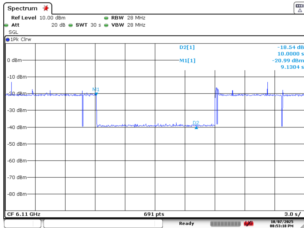
Plot 9-1. Contention Based Protocol Timing Plot (320MHz (UNII Band 5) – Ch.31 Low)
