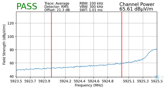
Plot 7-85. Radiated Lower Band Edge Plot MIMO (Average – UNII Band 5)
