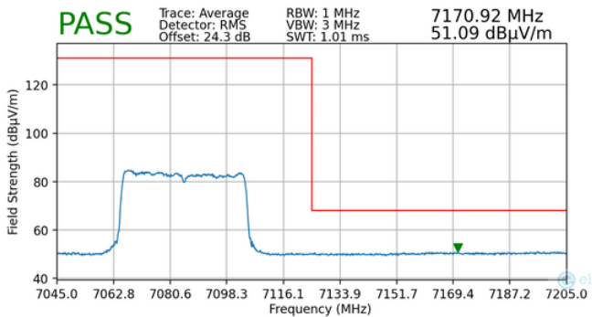
Plot 7-93. Radiated Upper Band Edge Plot MIMO (Average – UNII Band 8)
