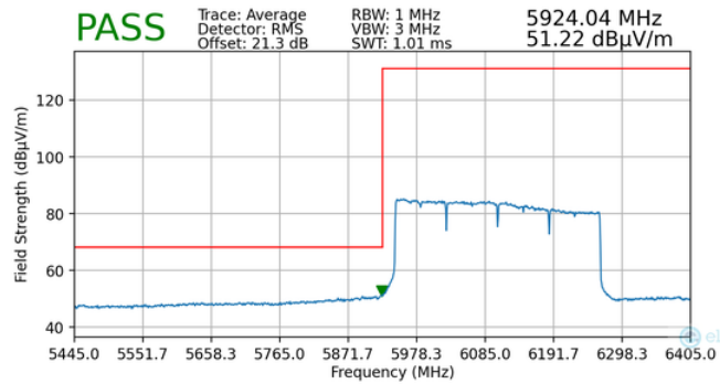
Plot 7-111. Radiated Lower Band Edge Plot MIMO (Average – UNII Band 5)
