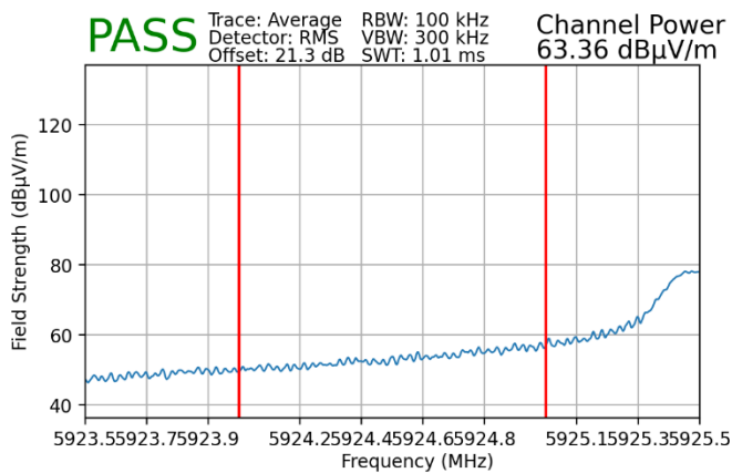
Plot 9-5. Radiated Lower Band Edge Plot MIMO (Average – UNII Band 5)
