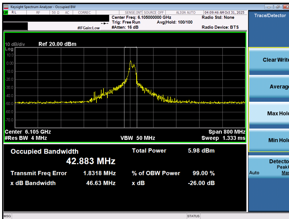
Plot 7-5. 26dB Bandwidth Plot MIMO ANT1 (320MHz 802.11be (26 Tones) (UNII Band 5) – Ch. 31) - VLP
