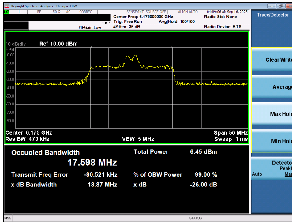
Plot 7-1. 26dB Bandwidth Plot MIMO ANT1 (20MHz 802.11ax/be (26 Tones) (UNII Band 5) – Ch. 45) - VLP
