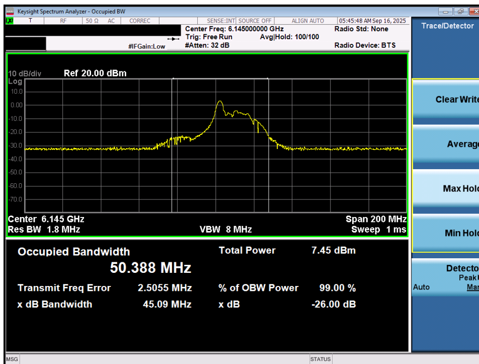
Plot 7-3. 26dB Bandwidth Plot MIMO ANT1 (80MHz 802.11ax/be (26 Tones) (UNII Band 5) – Ch. 39) - VLP
