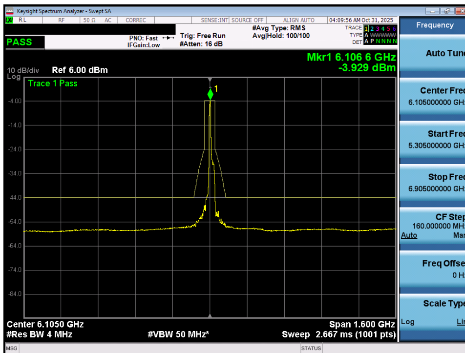
Plot 7-61. In Band Emissions Plot MIMO ANT1 (320MHz 802.11be (26 Tones) (UNII Band 5) – Ch. 31) - VLP
