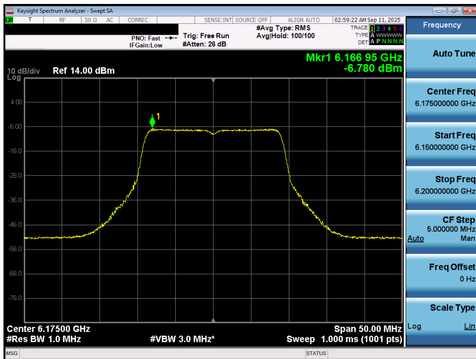
Plot 7-38. Power Spectral Density Plot MIMO ANT1 (20MHz 802.11ax/be (Full Tones) (UNII Band 5) – Ch. 45) - VLP
