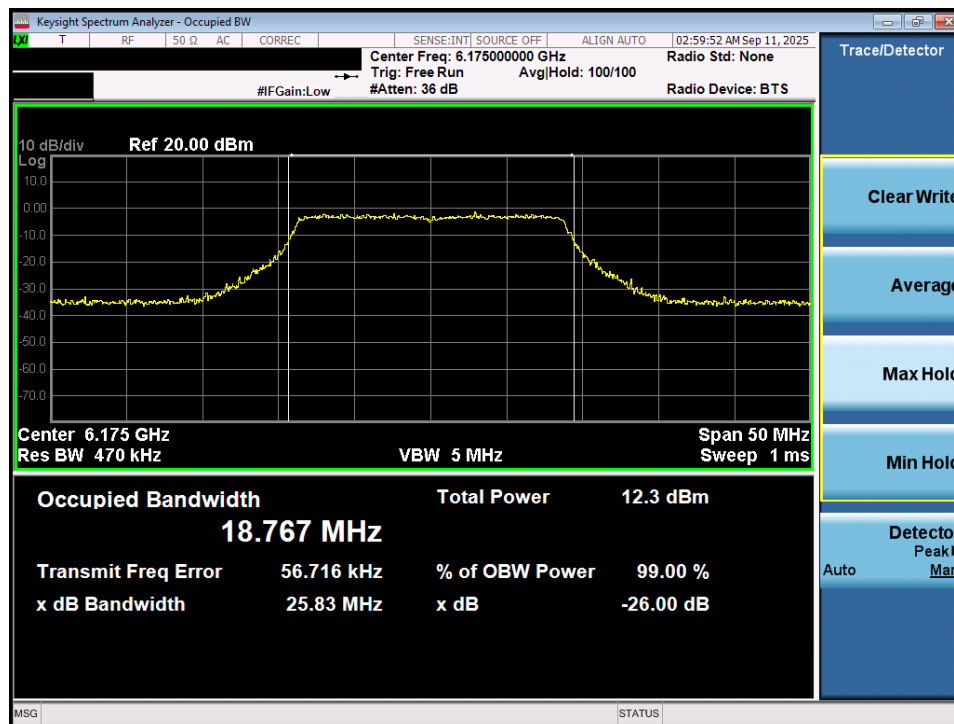
Plot 7-10. 26dB Bandwidth Plot MIMO ANT1 (20MHz 802.11ax/be (Full Tones) (UNII Band 5) – Ch. 45) - VLP
