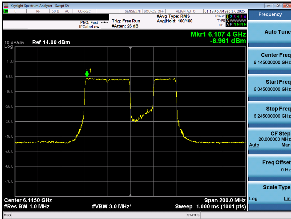
Plot 7-35. Power Spectral Density Plot MIMO ANT1 (80MHz 802.11be (484+242 Tones) (UNII Band 5) – Ch. 39) VLP
