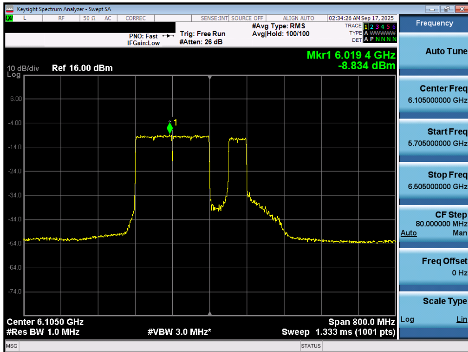
Plot 7-37. Power Spectral Density Plot MIMO ANT1 (320MHz 802.11be (2*996+484 Tones) (UNII Band 5) – Ch. 31) VLP
