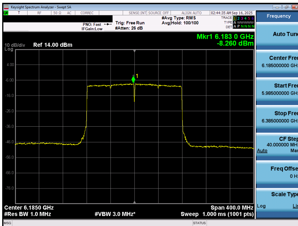
Plot 7-41. Power Spectral Density Plot MIMO ANT1 (160MHz 802.11ax/be (Full Tones) (UNII Band 5) – Ch. 47) - VLP
