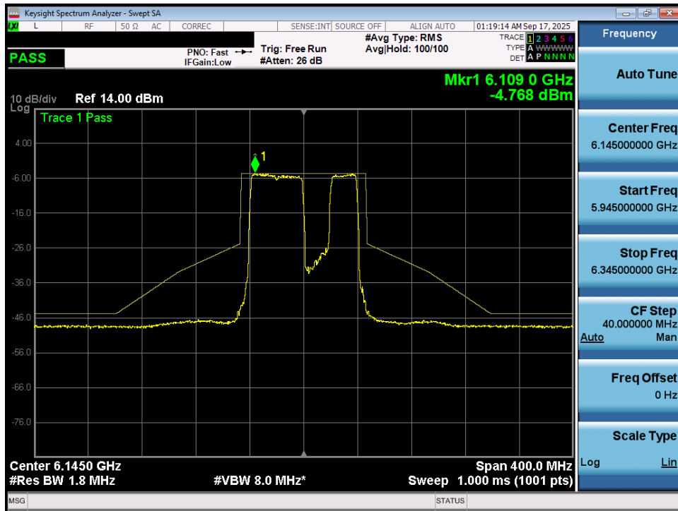
Plot 7-63. In Band Emissions Plot MIMO ANT1 (80MHz 802.11be (484+242 Tones) (UNII Band 5) – Ch. 39) VLP
