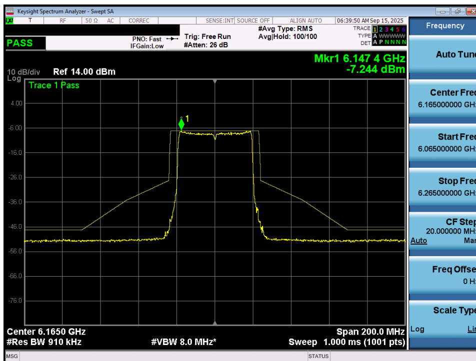
Plot 7-67. In Band Emissions Plot MIMO ANT1 (40MHz 802.11ax/be (Full Tones) (UNII Band 5) – Ch. 43) - VLP
