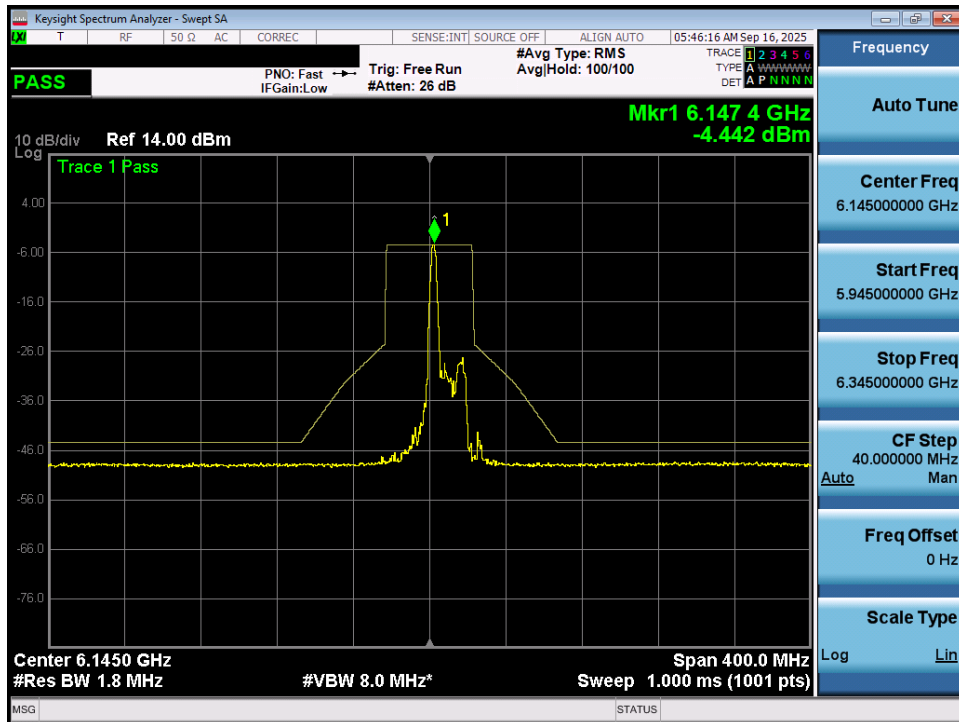
Plot 7-59. In Band Emissions Plot MIMO ANT1 (80MHz 802.11ax/be (26 Tones) (UNII Band 5) – Ch. 39) - VLP
