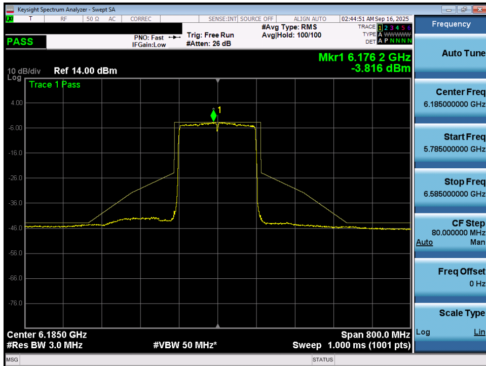
Plot 7-69. In Band Emissions Plot MIMO ANT1 (160MHz 802.11ax/be (Full Tones) (UNII Band 5) – Ch. 47) - VLP
