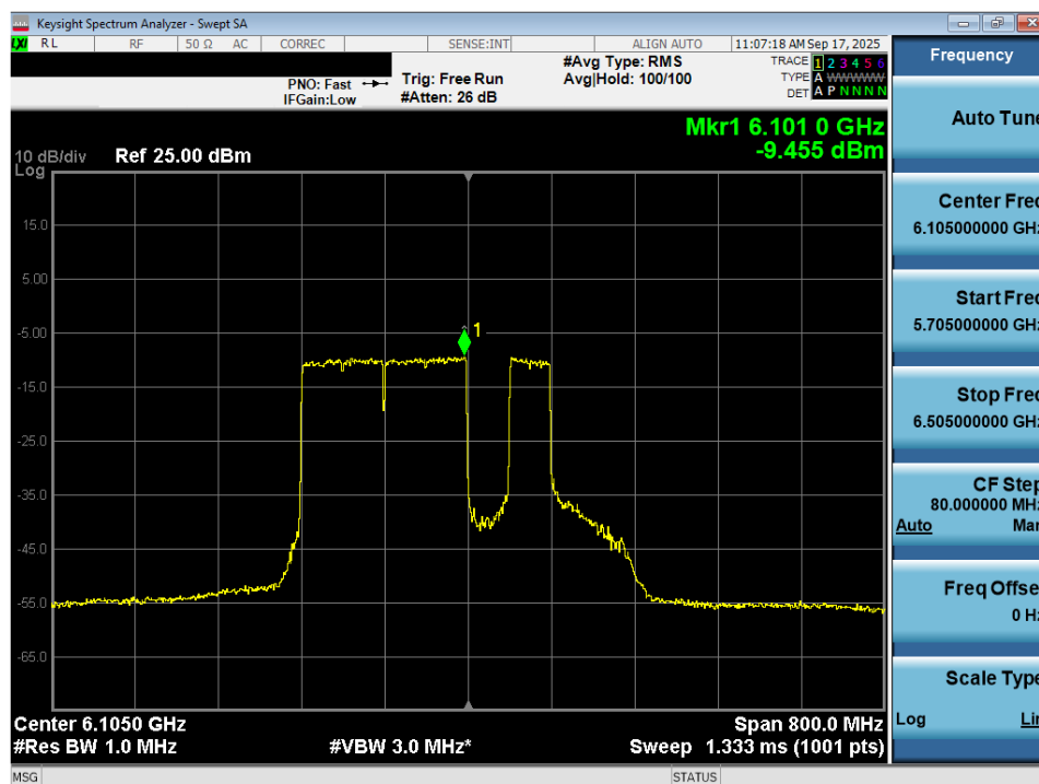
Plot 7-51. Power Spectral Density Plot MIMO ANT2 (320MHz 802.11be (2*996+484 Tones) (UNII Band 5) – Ch. 31) VLP
