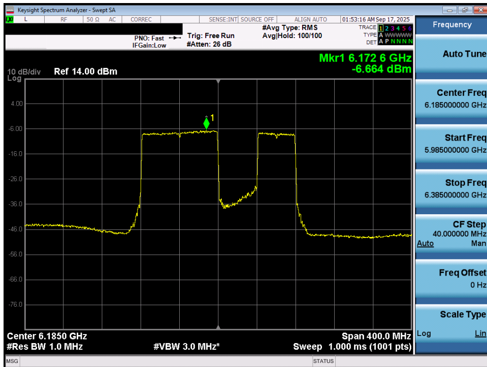
Plot 7-36. Power Spectral Density Plot MIMO ANT1 (160MHz 802.11be (996+484 Tones) (UNII Band 5) – Ch. 47) VLP
