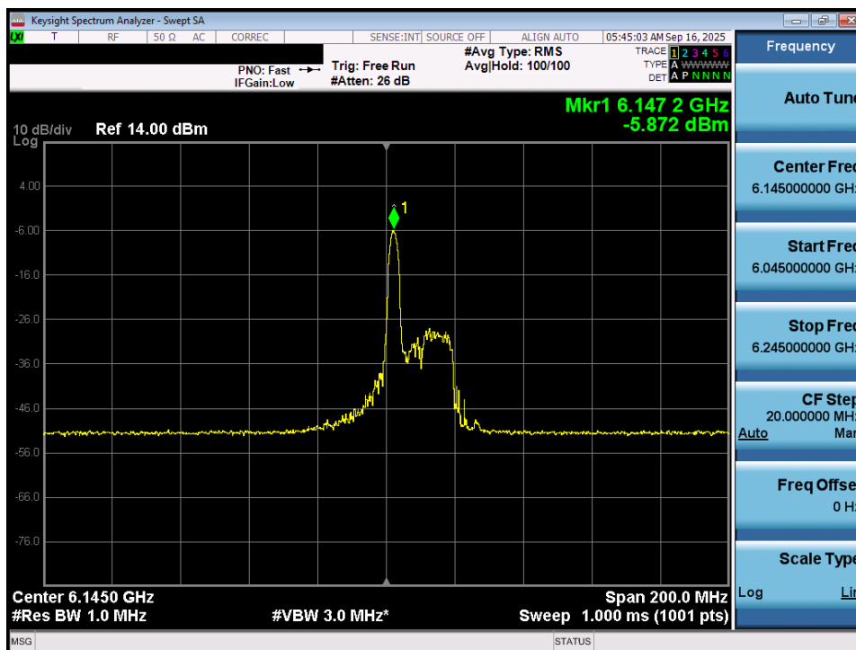
Plot 7-31. Power Spectral Density Plot MIMO ANT1 (80MHz 802.11ax/be (26 Tones) (UNII Band 5) – Ch. 39) - VLP
