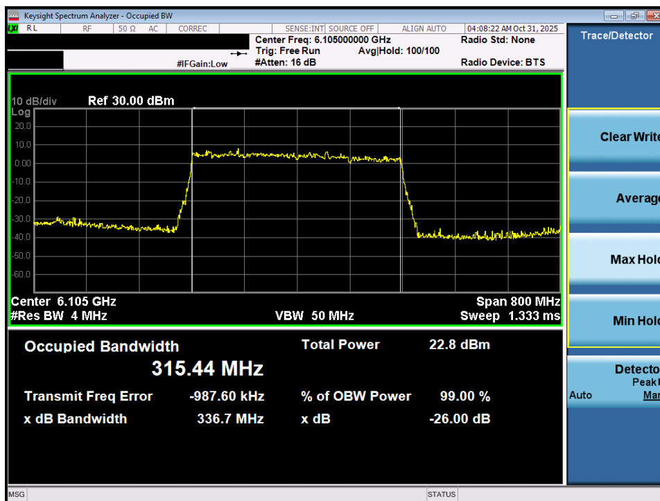
Plot 7-14. 26dB Bandwidth Plot MIMO ANT1 (320MHz 802.11be (Full Tones) (UNII Band 5) – Ch. 31) - VLP
