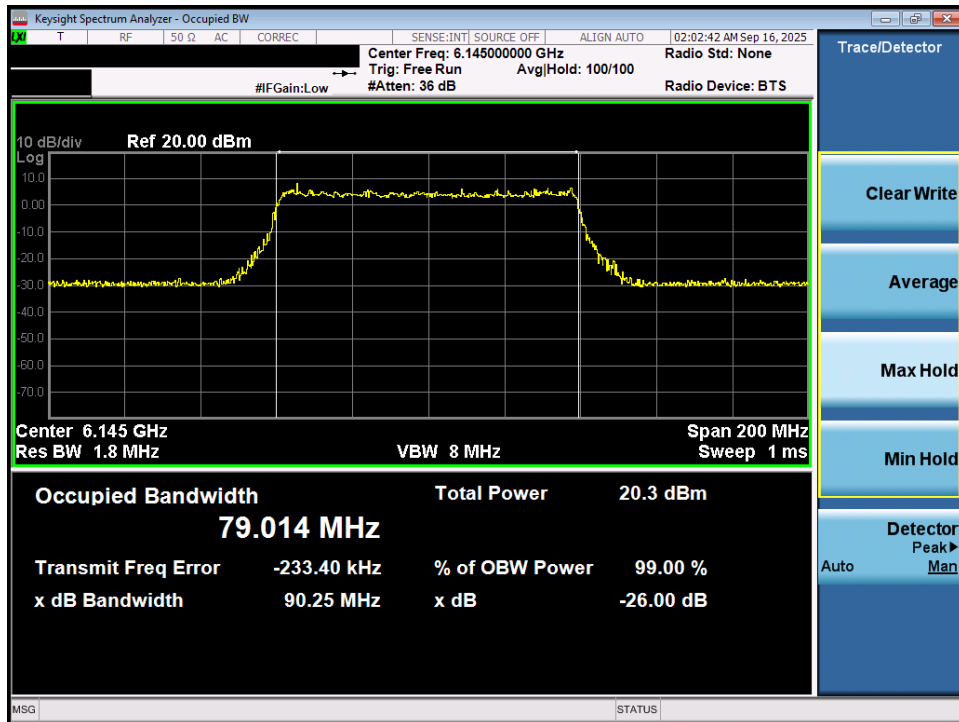
Plot 7-12. 26dB Bandwidth Plot MIMO ANT1 (80MHz 802.11ax/be (Full Tones) (UNII Band 5) – Ch. 39) - VLP
