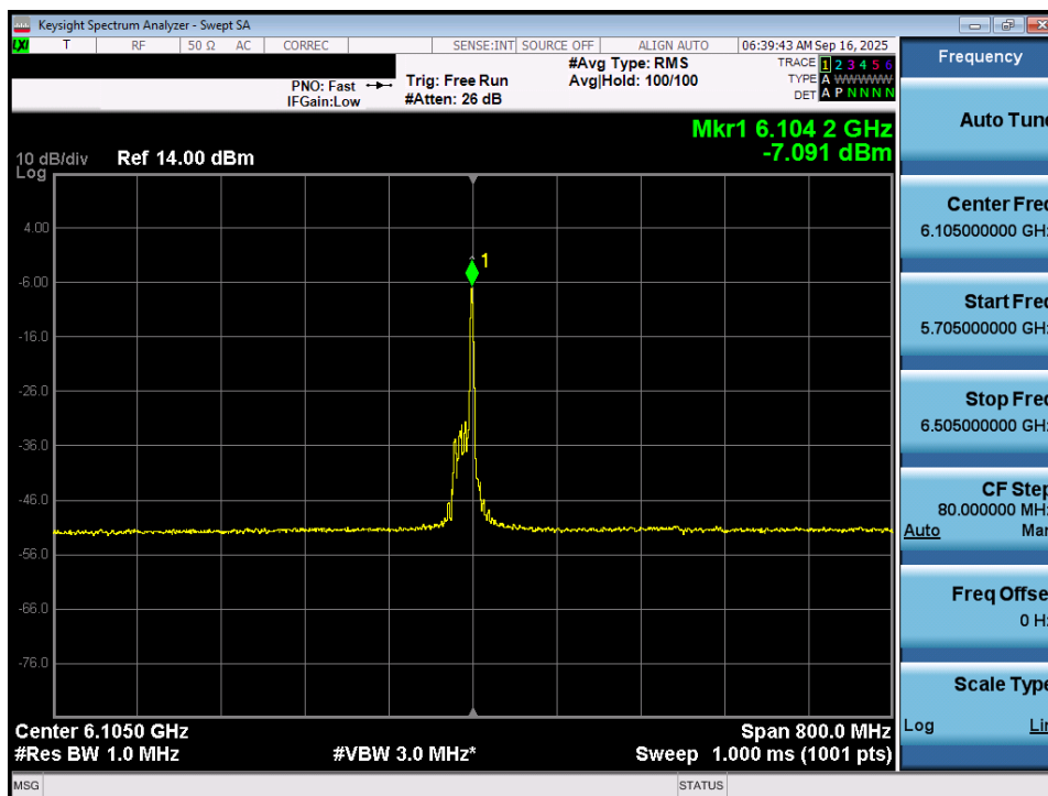
Plot 7-33. Power Spectral Density Plot MIMO ANT1 (320MHz 802.11be (26 Tones) (UNII Band 5) – Ch. 31) - VLP
