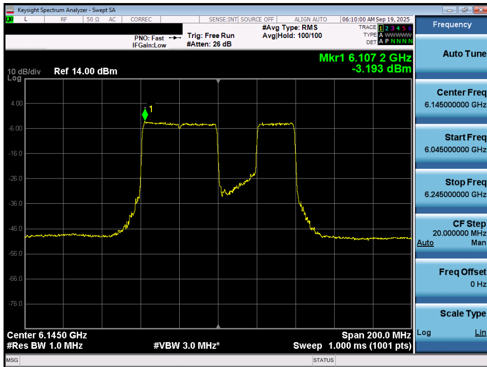
Plot 7-57. Power Spectral Density Plot MIMO ANT1 (80MHz 802.11be (484+242 Tones) (UNII Band 5) – Ch. 39) - LPI
