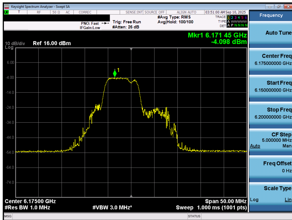
Plot 7-56. Power Spectral Density Plot MIMO ANT1 (20MHz 802.11be (52+26 Tones) (UNII Band 5) – Ch. 45) - LPI
