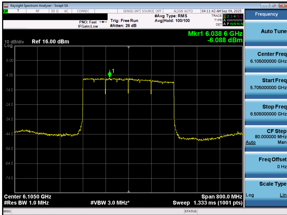
Plot 7-72. Power Spectral Density Plot MIMO ANT1 (320MHz 802.11be (Full Tones) (UNII Band 5) – Ch. 31) - LPI/SP
