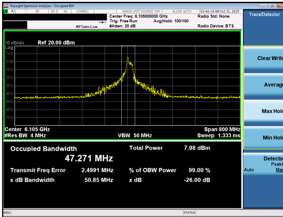
Plot 7-30. 26dB Bandwidth Plot MIMO ANT2 (320MHz 802.11be (26 Tones) (UNII Band 5) – Ch. 31) - LPI
