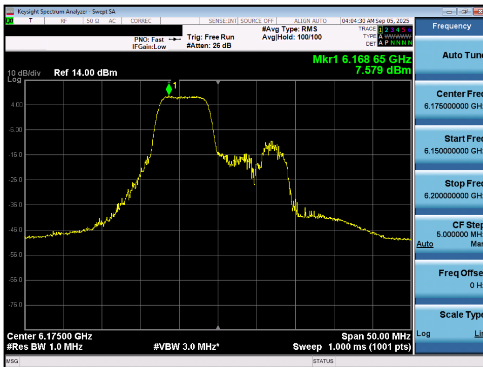
Plot 7-65. Power Spectral Density Plot MIMO ANT1 (20MHz 802.11be (52+26 Tones) (UNII Band 5) – Ch. 45) – SP
