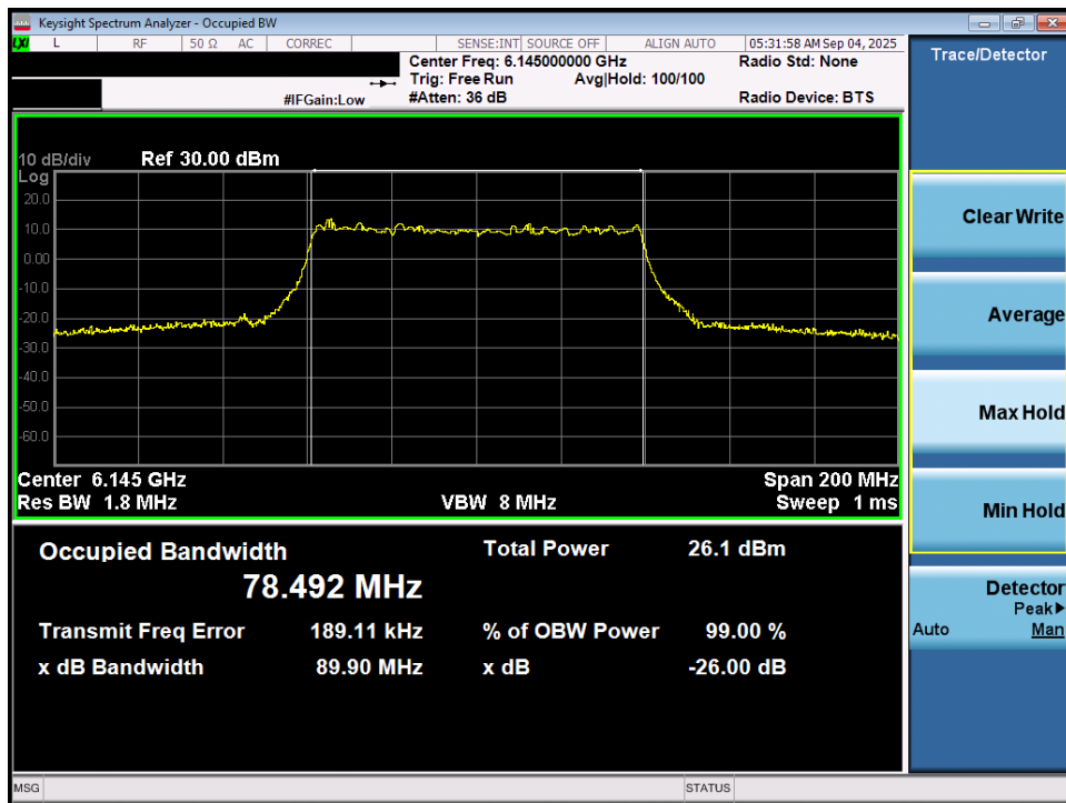
Plot 7-25. 26dB Bandwidth Plot MIMO ANT1 (80MHz 802.11ax/be (Full Tones) (UNII Band 5) – Ch. 39) - SP
