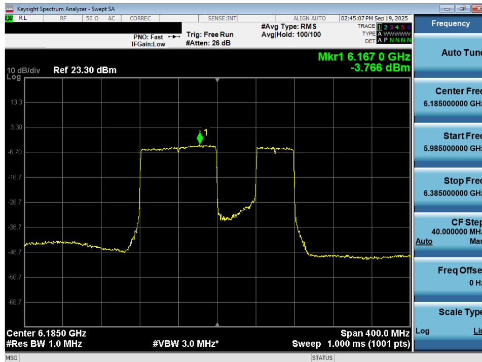
Plot 7-83. Power Spectral Density Plot MIMO ANT2 (160MHz 802.11be (996+484 Tones) (UNII Band 5) – Ch. 47) - LPI
