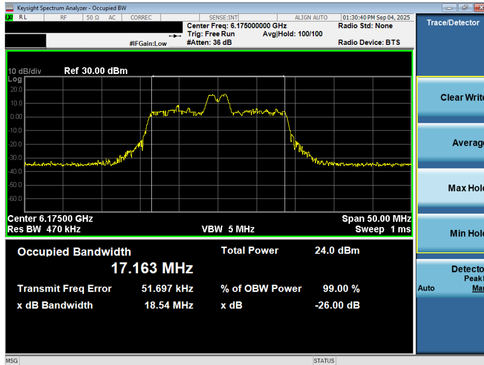
Plot 7-35. 26dB Bandwidth Plot MIMO ANT2 (20MHz 802.11ax/be (26 Tones) (UNII Band 5) – Ch. 45) - SP
