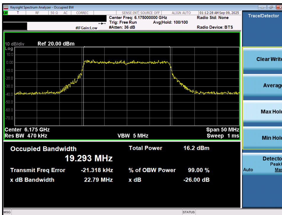
Plot 7-18. 26dB Bandwidth Plot MIMO ANT1 (20MHz 802.11ax/be (Full Tones) (UNII Band 5) – Ch. 45) – LPI
