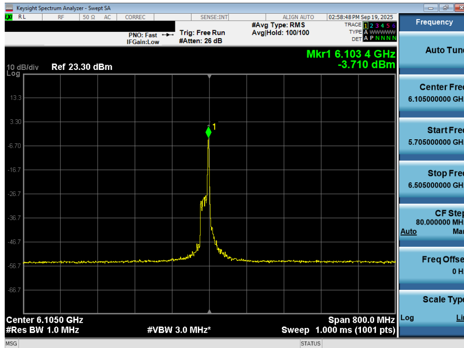
Plot 7-80. Power Spectral Density Plot MIMO ANT2 (320MHz 802.11be (26 Tones) (UNII Band 5) – Ch. 31) - LPI
