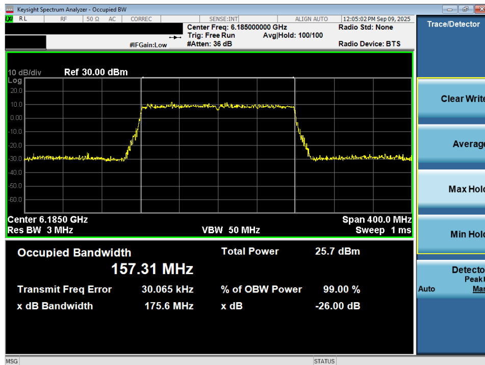
Plot 7-46. 26dB Bandwidth Plot MIMO ANT2 (160MHz 802.11ax/be (Full Tones) (UNII Band 5) – Ch. 47) - LPI/SP
