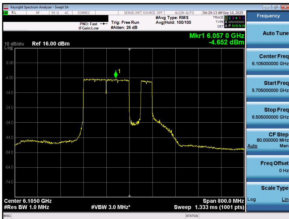
Plot 7-59. Power Spectral Density Plot MIMO ANT1 (320MHz 802.11be (UNII Band 5) – Ch. 31) LPI/SP
