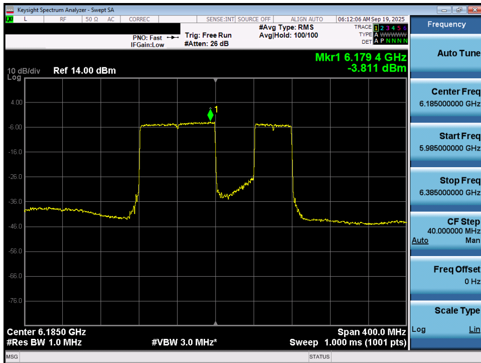
Plot 7-58. Power Spectral Density Plot MIMO ANT1 (160MHz 802.11be (996+484 Tones) (UNII Band 5) – Ch. 47) - LPI
