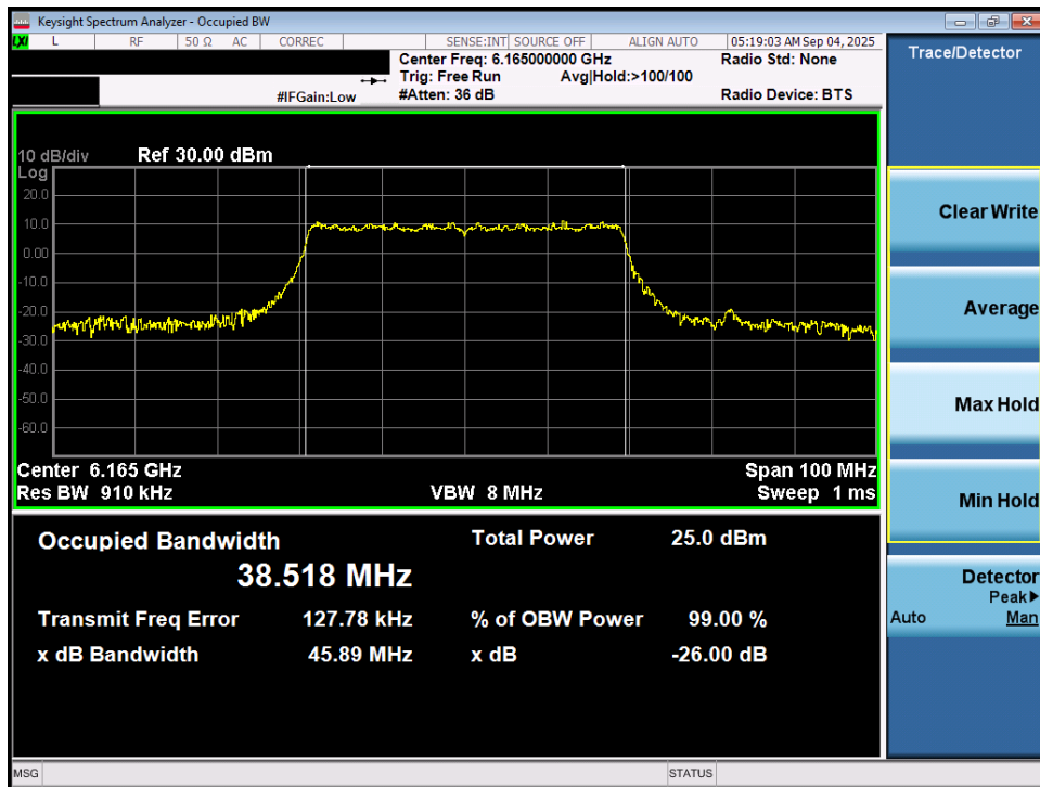
Plot 7-24. 26dB Bandwidth Plot MIMO ANT1 (40MHz 802.11ax/be (Full Tones) (UNII Band 5) – Ch. 43) – SP
