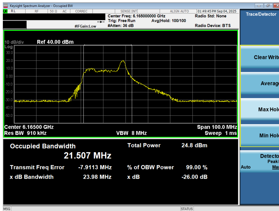
Plot 7-36. 26dB Bandwidth Plot MIMO ANT2 (40MHz 802.11ax/be (26 Tones) (UNII Band 5) – Ch. 43) - SP
