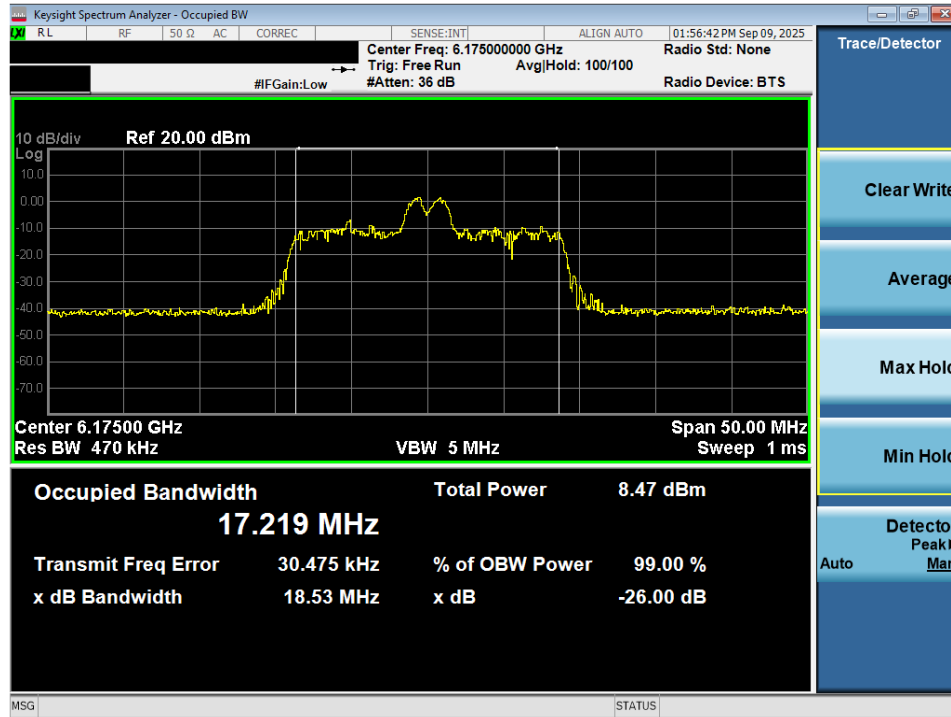
Plot 7-26. 26dB Bandwidth Plot MIMO ANT2 (20MHz 802.11ax/be (26 Tones) (UNII Band 5) – Ch. 45) - LPI
