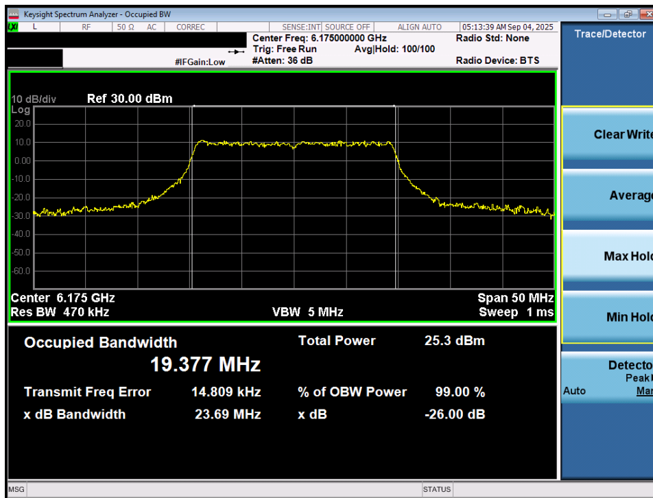
Plot 7-23. 26dB Bandwidth Plot MIMO ANT1 (20MHz 802.11ax/be (Full Tones) (UNII Band 5) – Ch. 45) - SP
