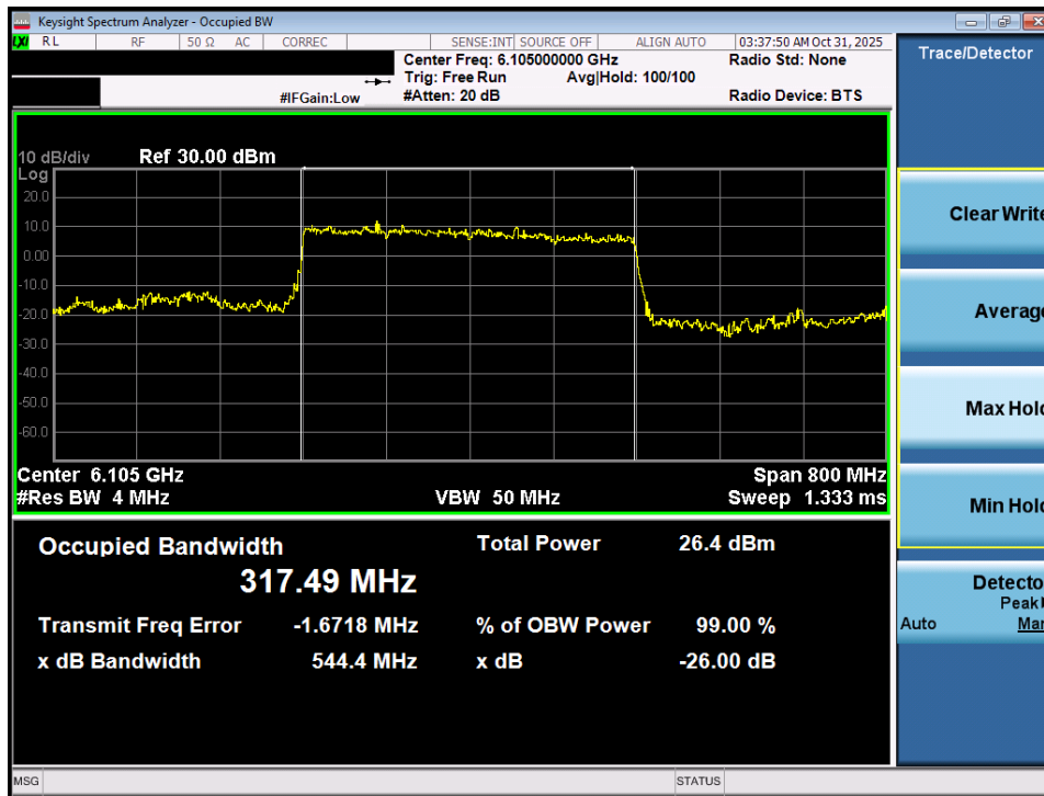
Plot 7-22. 26dB Bandwidth Plot MIMO ANT1 (320MHz 802.11be (Full Tones) (UNII Band 5) – Ch. 31) - LPI/SP
