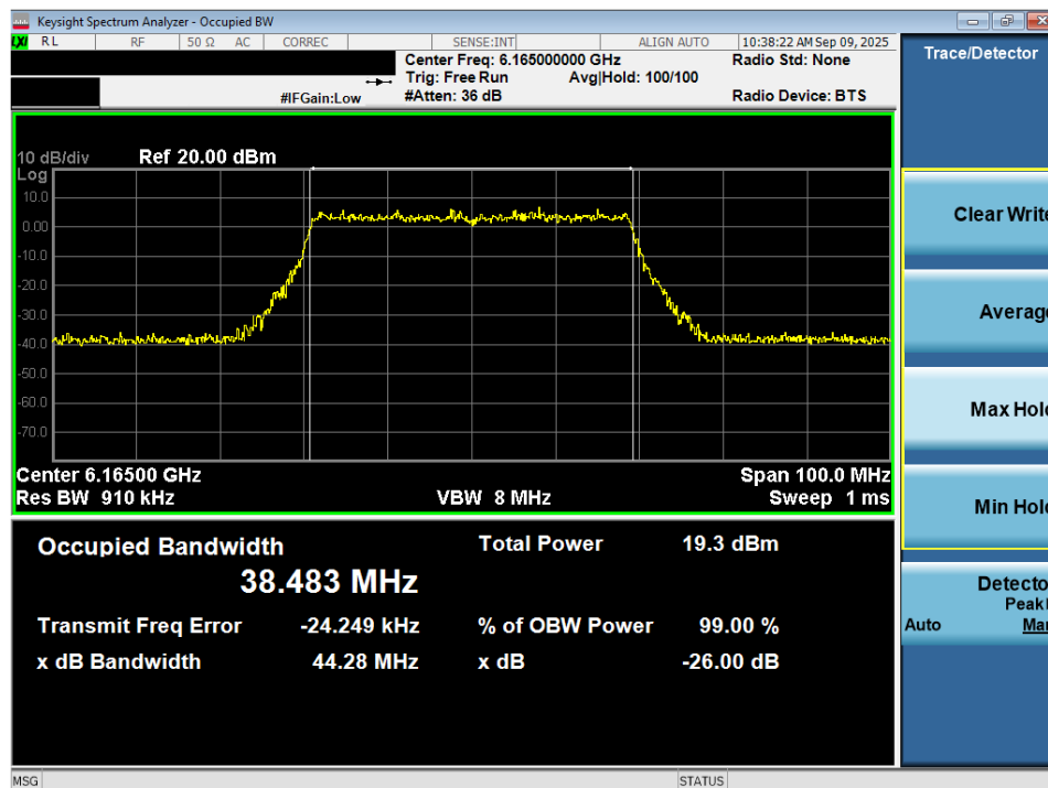
Plot 7-44. 26dB Bandwidth Plot MIMO ANT2 (40MHz 802.11ax/be (Full Tones) (UNII Band 5) – Ch. 43) - LPI
