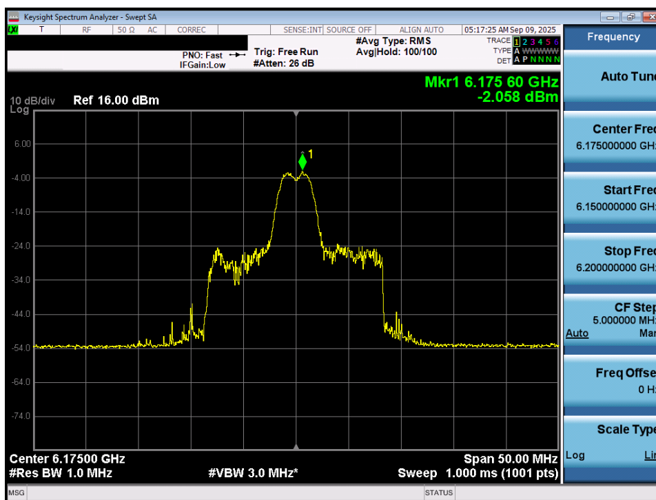
Plot 7-51. Power Spectral Density Plot MIMO ANT1 (20MHz 802.11ax/be (26 Tones) (UNII Band 5) – Ch. 45) - LPI
