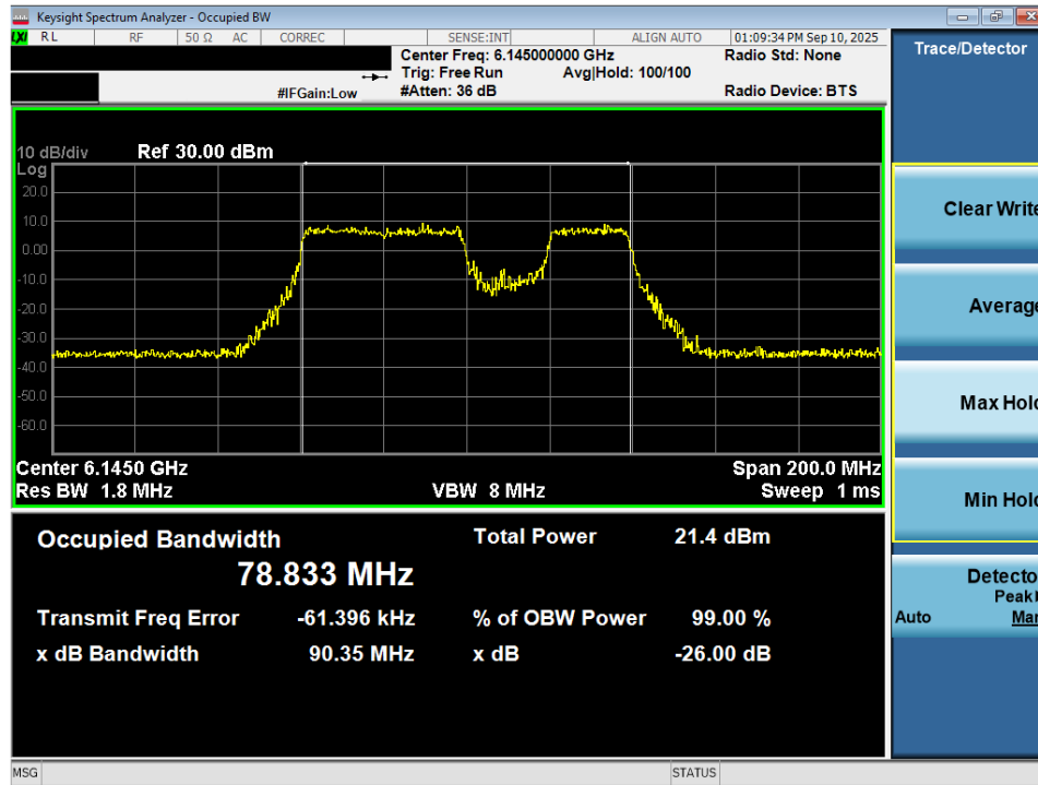
Plot 7-32. 26dB Bandwidth Plot MIMO ANT2 (80MHz 802.11be (484+242 Tones) (UNII Band 5) – Ch. 39) - LPI
