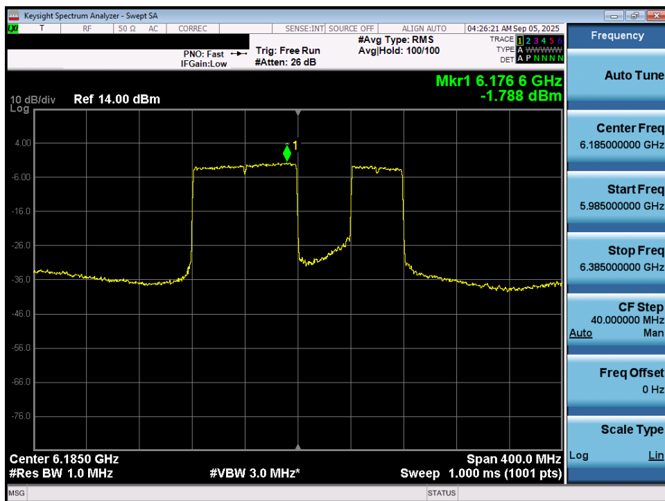
Plot 7-67. Power Spectral Density Plot MIMO ANT1 (160MHz 802.11be (996+484 Tones) (UNII Band 5) – Ch. 47) - SP
