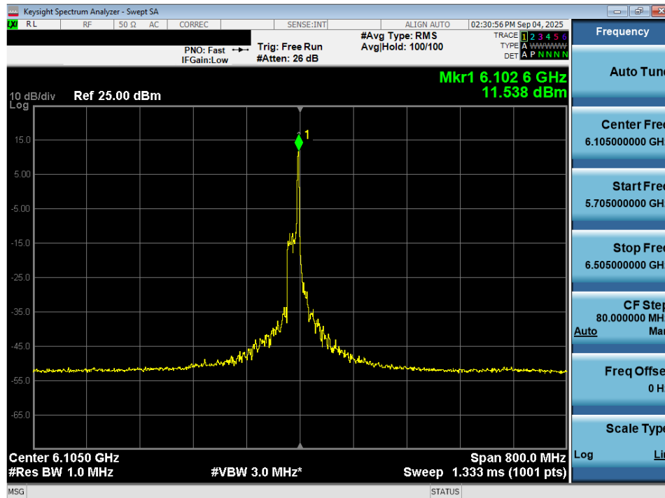
Plot 7-89. Power Spectral Density Plot MIMO ANT2 (320MHz 802.11be (26 Tones) (UNII Band 5) – Ch. 31) - SP
