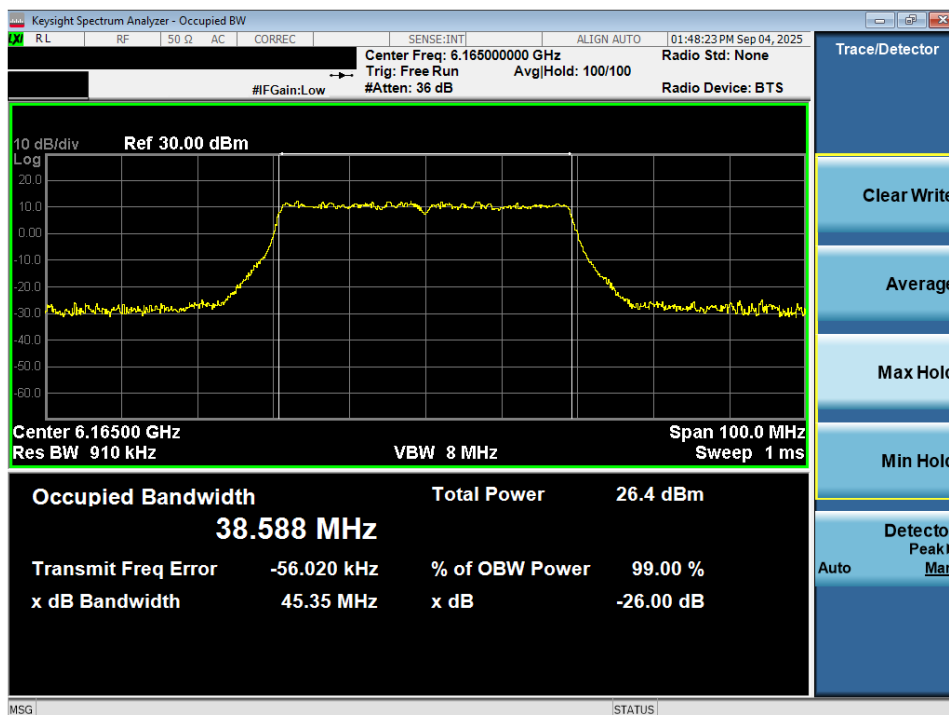
Plot 7-49. 26dB Bandwidth Plot MIMO ANT2 (40MHz 802.11ax/be (Full Tones) (UNII Band 5) – Ch. 43) - SP
