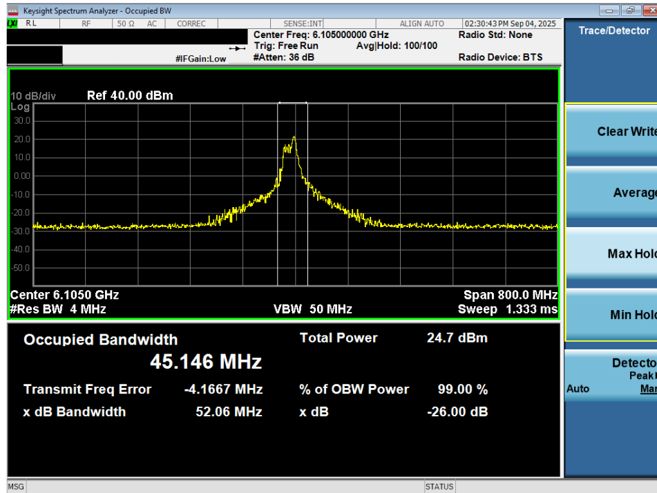
Plot 7-39. 26dB Bandwidth Plot MIMO ANT2 (320MHz 802.11be (26 Tones) (UNII Band 5) – Ch. 31) - SP
