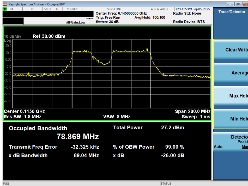
Plot 7-41. 26dB Bandwidth Plot MIMO ANT2 (80MHz 802.11be (484+242 Tones) (UNII Band 5) – Ch. 39) - SP
