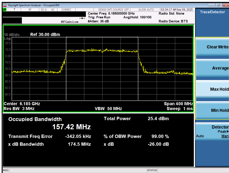
Plot 7-21. 26dB Bandwidth Plot MIMO ANT1 (160MHz 802.11ax/be (Full Tones) (UNII Band 5) – Ch. 47) - LPI/SP
