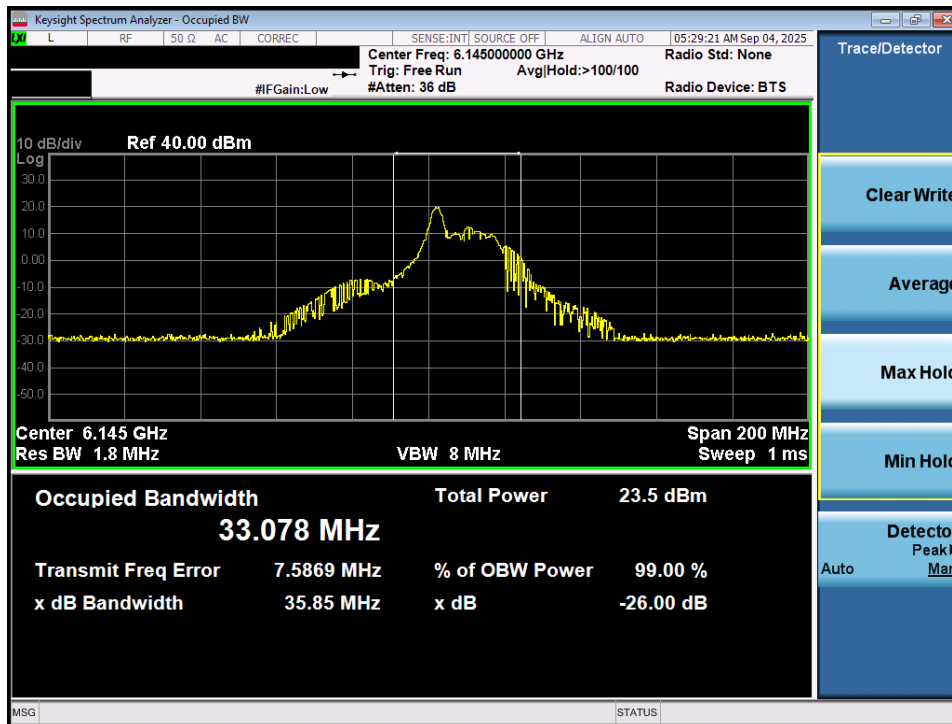
Plot 7-12. 26dB Bandwidth Plot MIMO ANT1 (80MHz 802.11ax/be (26 Tones) (UNII Band 5) – Ch. 39) - SP
