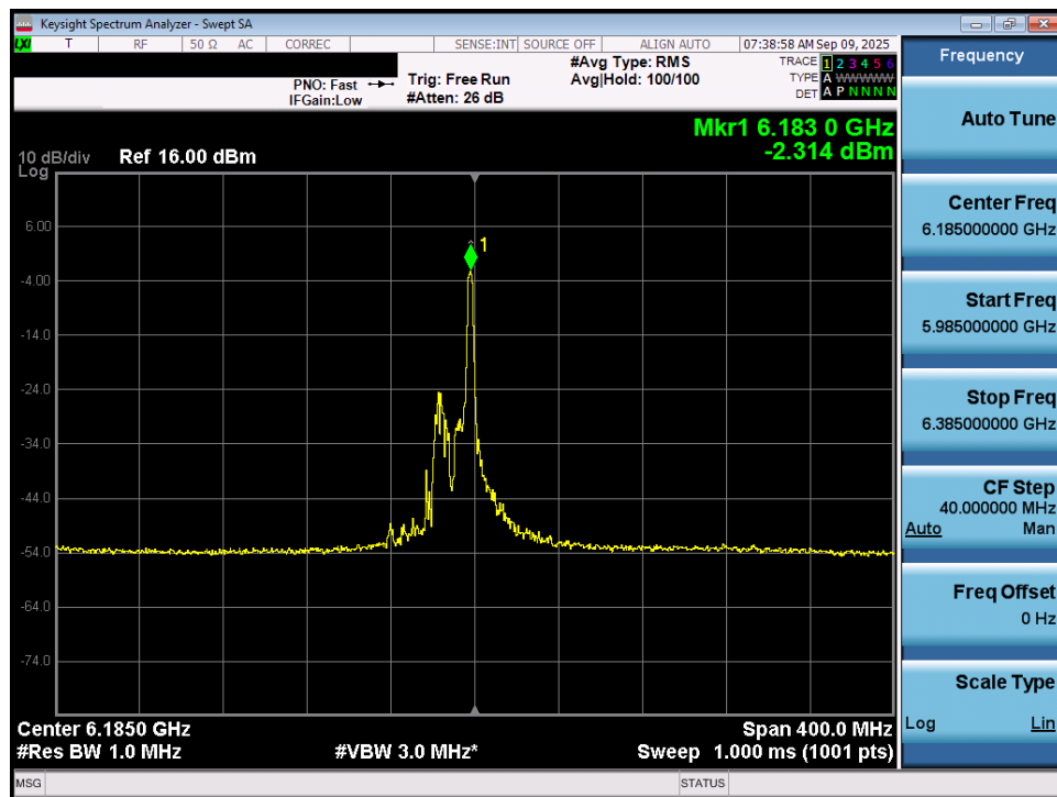
Plot 7-54. Power Spectral Density Plot MIMO ANT1 (160MHz 802.11ax/be (26 Tones) (UNII Band 5) – Ch. 47) - LPI
