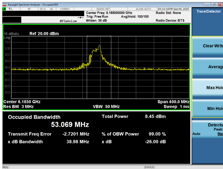
Plot 7-29. 26dB Bandwidth Plot MIMO ANT2 (160MHz 802.11ax/be (26 Tones) (UNII Band 5) – Ch. 47) - LPI
