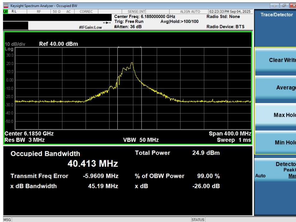
Plot 7-38. 26dB Bandwidth Plot MIMO ANT2 (160MHz 802.11ax/be (26 Tones) (UNII Band 5) – Ch. 47) - SP
