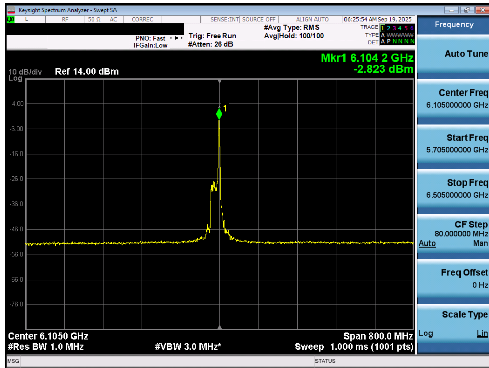
Plot 7-55. Power Spectral Density Plot MIMO ANT1 (320MHz 802.11be (26 Tones) (UNII Band 5) – Ch. 31) - LPI
