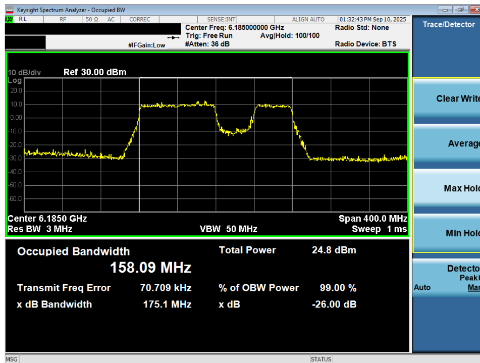
Plot 7-33. 26dB Bandwidth Plot MIMO ANT2 (160MHz 802.11be (996+484 Tones) (UNII Band 5) – Ch. 47) - LPI
