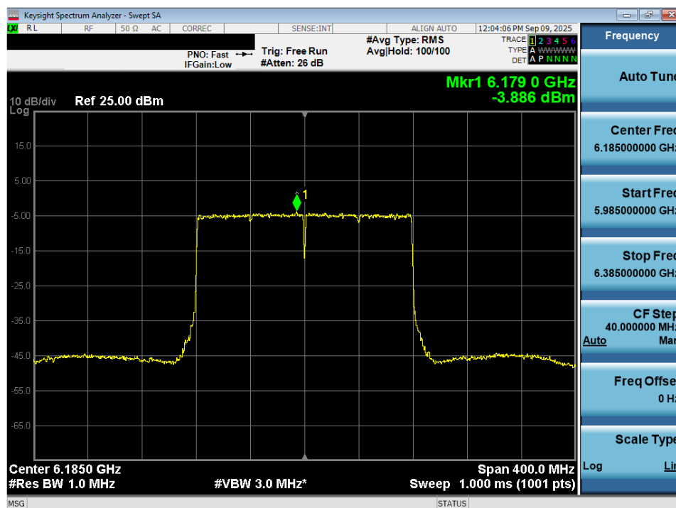
Plot 7-96. Power Spectral Density Plot MIMO ANT2 (160MHz 802.11ax/be (Full Tones) (UNII Band 5) – Ch. 47) - LPI/SP
