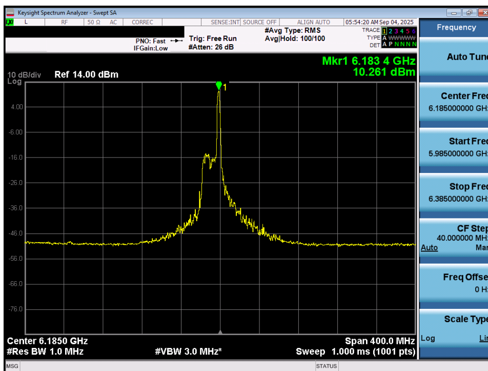
Plot 7-63. Power Spectral Density Plot MIMO ANT1 (160MHz 802.11ax/be (26 Tones) (UNII Band 5) – Ch. 47) - SP
