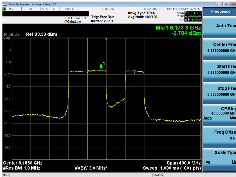
Plot 7-92. Power Spectral Density Plot MIMO ANT2 (160MHz 802.11be (996+484 Tones) (UNII Band 5) – Ch. 47) - SP
