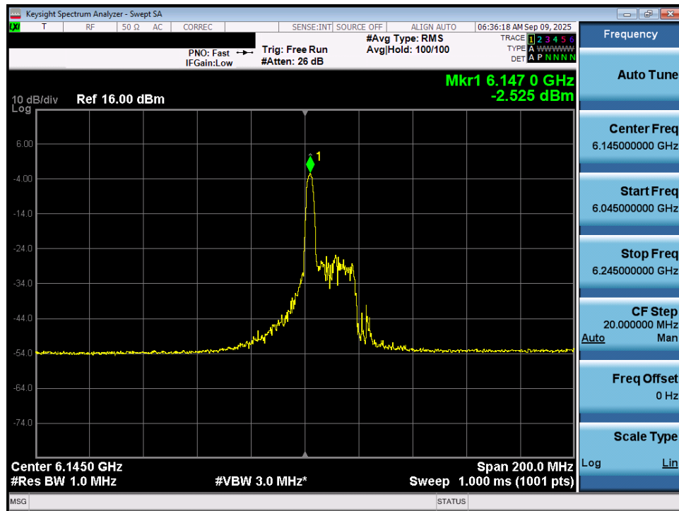
Plot 7-53. Power Spectral Density Plot MIMO ANT1 (80MHz 802.11ax/be (26 Tones) (UNII Band 5) – Ch. 39) - LPI
