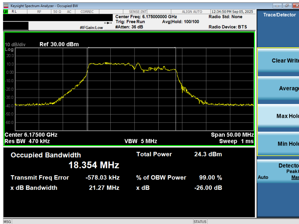
Plot 7-40. 26dB Bandwidth Plot MIMO ANT2 (20MHz 802.11be (106+26 Tones) (UNII Band 5) – Ch. 45) – SP
