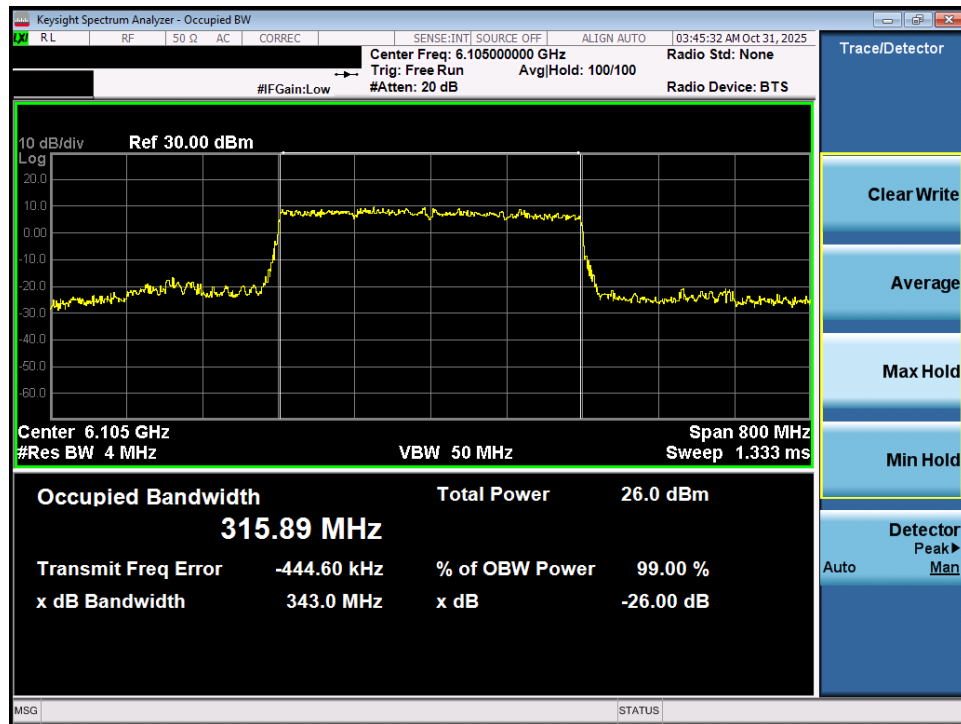
Plot 7-47. 26dB Bandwidth Plot MIMO ANT2 (320MHz 802.11be (Full Tones) (UNII Band 5) – Ch. 31) - LPI/SP
