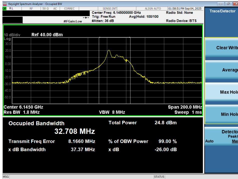
Plot 7-37. 26dB Bandwidth Plot MIMO ANT2 (80MHz 802.11ax/be (26 Tones) (UNII Band 5) – Ch. 39) - SP
