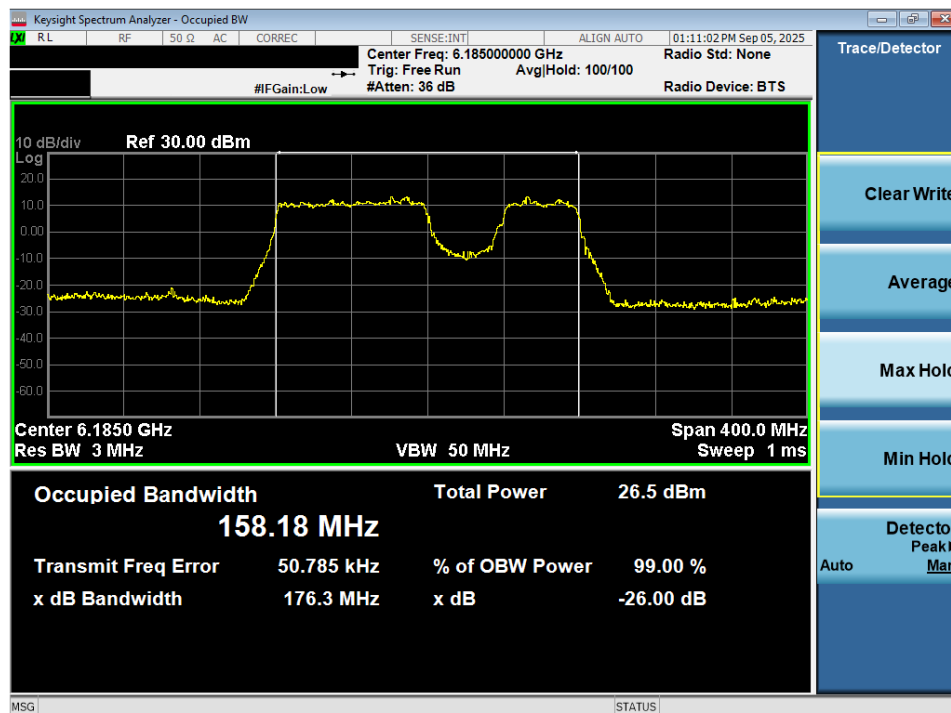
Plot 7-42. 26dB Bandwidth Plot MIMO ANT2 (160MHz 802.11be (996+484 Tones) (UNII Band 5) – Ch. 47) - SP
