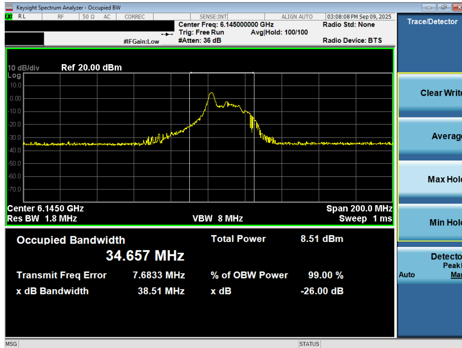
Plot 7-28. 26dB Bandwidth Plot MIMO ANT2 (80MHz 802.11ax/be (26 Tones) (UNII Band 5) – Ch. 39) - LPI
