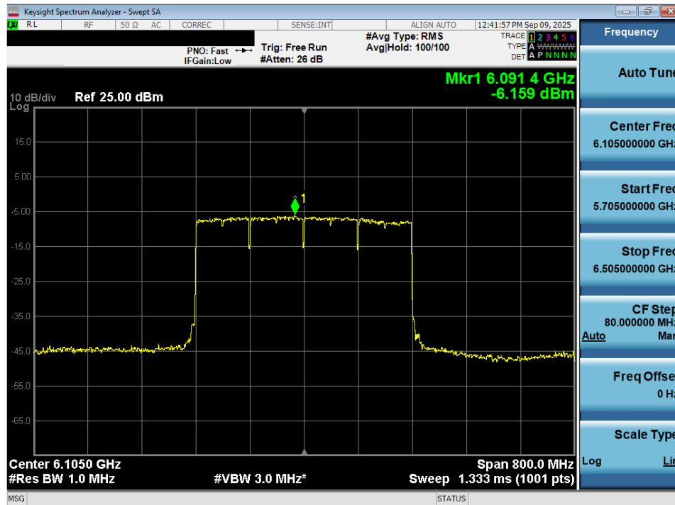
Plot 7-97. Power Spectral Density Plot MIMO ANT2 (320MHz 802.11be (Full Tones) (UNII Band 5) – Ch. 31) - LPI/SP
