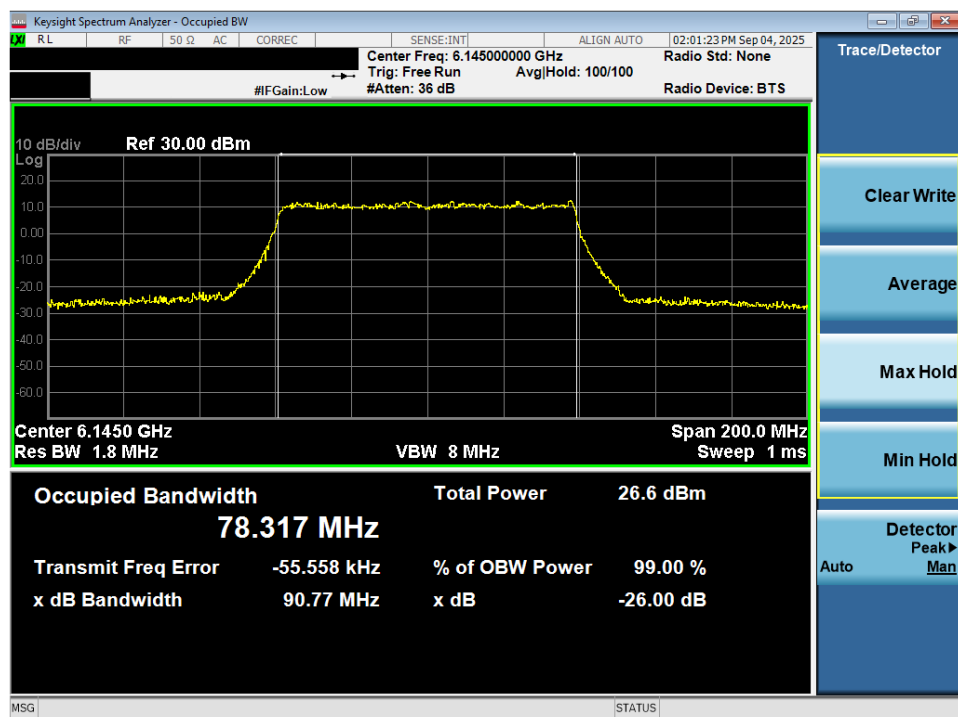
Plot 7-50. 26dB Bandwidth Plot MIMO ANT2 (80MHz 802.11ax/be (Full Tones) (UNII Band 5) – Ch. 39) - SP
