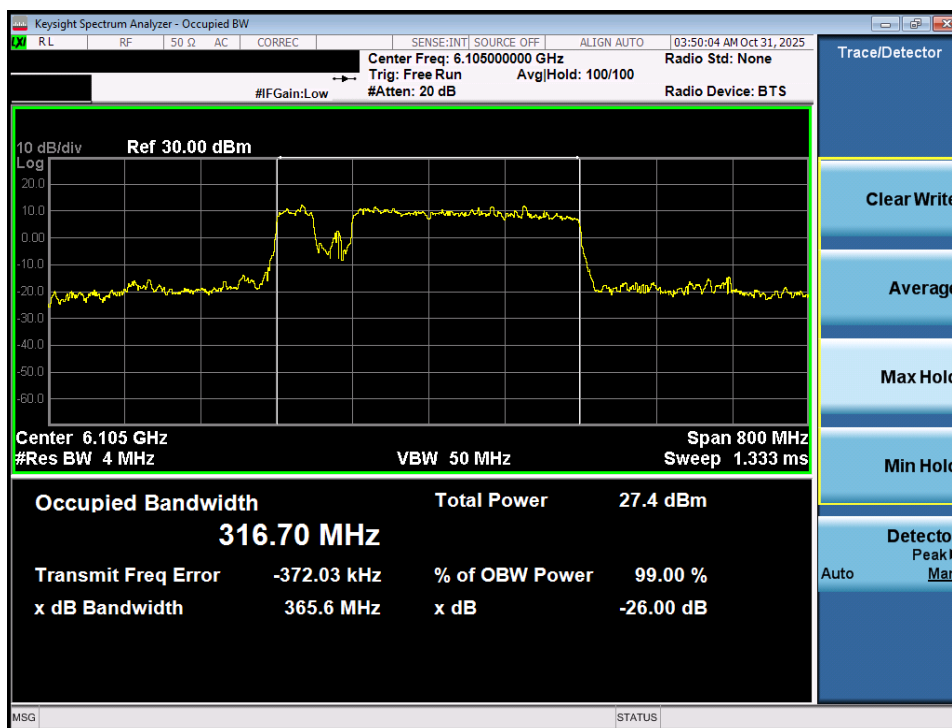
Plot 7-34. 26dB Bandwidth Plot MIMO ANT2 (320MHz 802.11be (3*996+484 Tones) (UNII Band 5) – Ch. 31) LPI/SP
