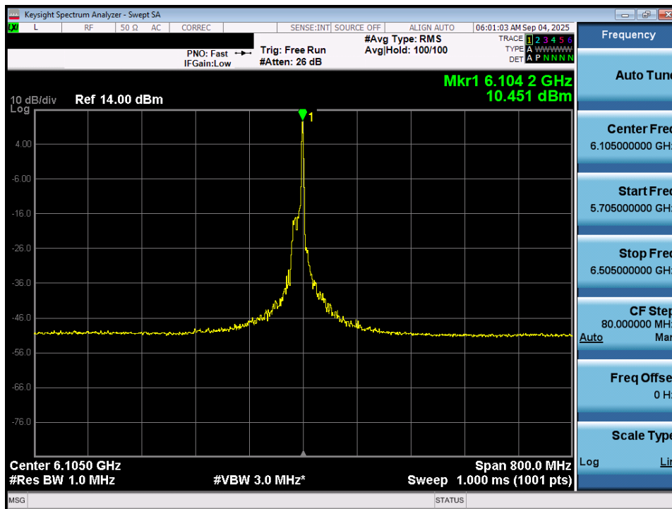
Plot 7-64. Power Spectral Density Plot MIMO ANT1 (320MHz 802.11be (26 Tones) (UNII Band 5) – Ch. 31) - SP
