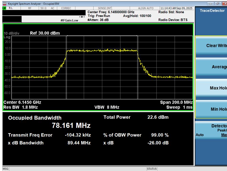
Plot 7-45. 26dB Bandwidth Plot MIMO ANT2 (80MHz 802.11ax/be (Full Tones) (UNII Band 5) – Ch. 39) - LPI
