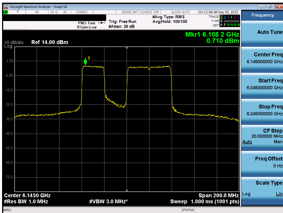
Plot 7-66. Power Spectral Density Plot MIMO ANT1 (80MHz 802.11be (484+242 Tones) (UNII Band 5) – Ch. 39) - SP
