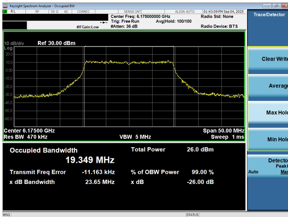
Plot 7-48. 26dB Bandwidth Plot MIMO ANT2 (20MHz 802.11ax/be (Full Tones) (UNII Band 5) – Ch. 45) - SP
