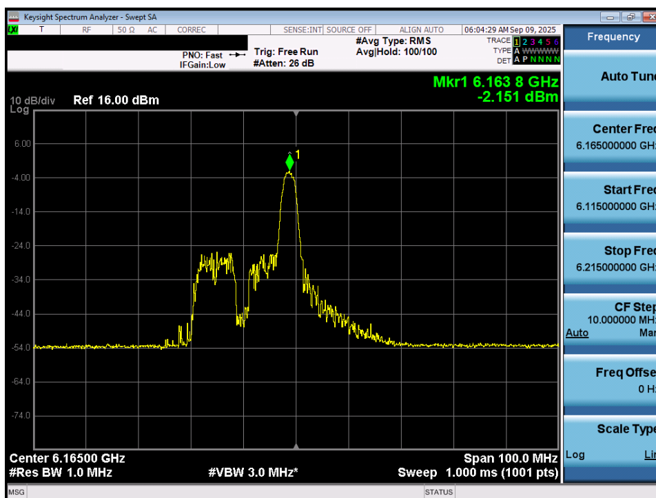
Plot 7-52. Power Spectral Density Plot MIMO ANT1 (40MHz 802.11ax/be (26 Tones) (UNII Band 5) – Ch. 43) - LPI
