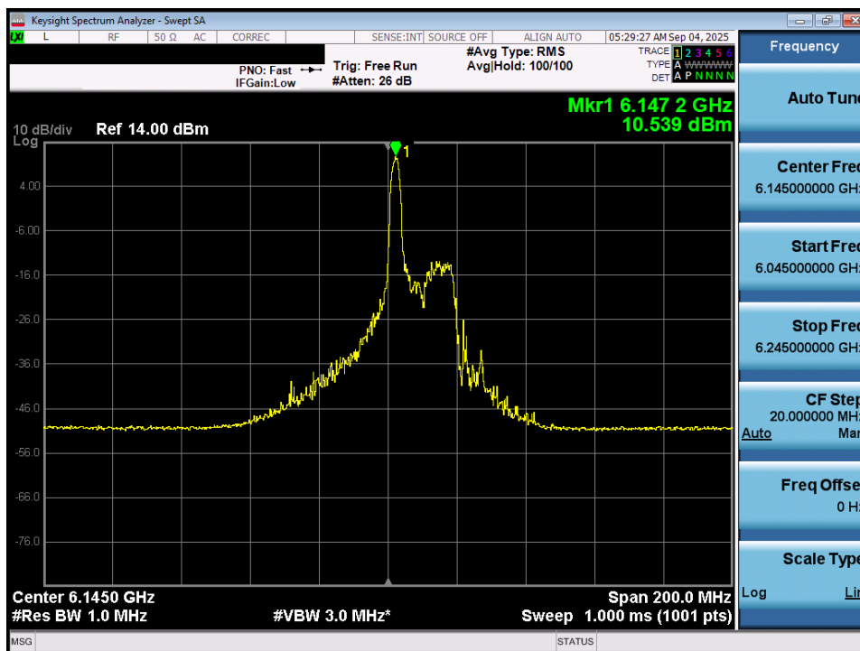
Plot 7-62. Power Spectral Density Plot MIMO ANT1 (80MHz 802.11ax/be (26 Tones) (UNII Band 5) – Ch. 39) - SP
