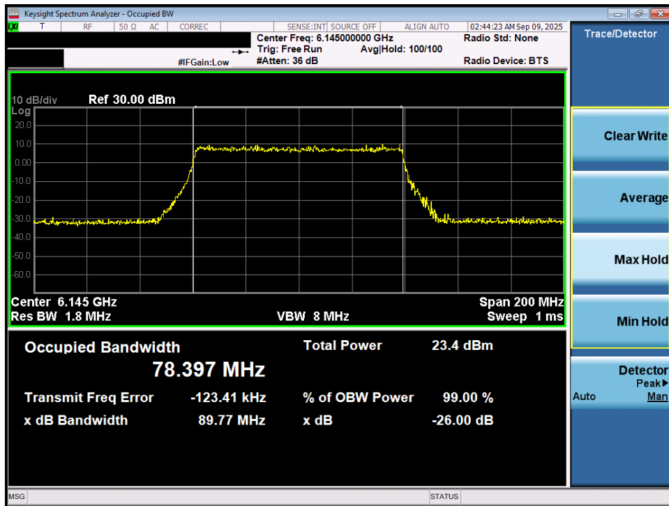
Plot 7-20. 26dB Bandwidth Plot MIMO ANT1 (80MHz 802.11ax/be (Full Tones) (UNII Band 5) – Ch. 39) - LPI
