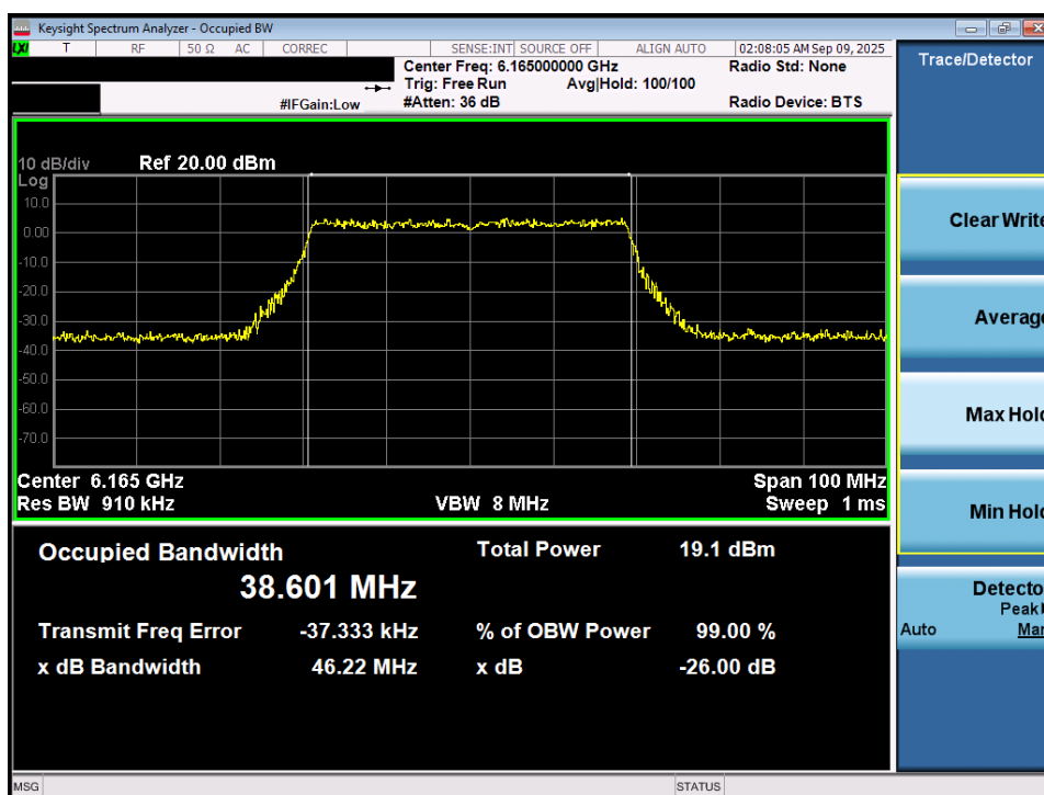
Plot 7-19. 26dB Bandwidth Plot MIMO ANT1 (40MHz 802.11ax/be (Full Tones) (UNII Band 5) – Ch. 43) - LPI
