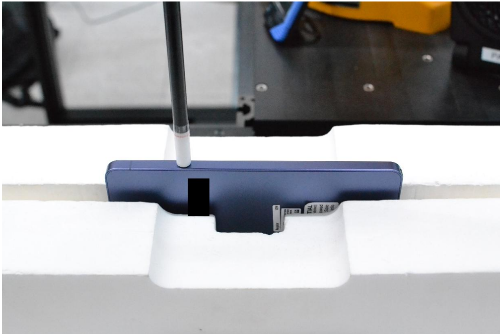
PD Test Setup Photo 36 – PD, Left Edge at 2mm (Antenna H)
