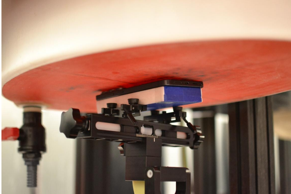
SAR Test Setup Photo 9 – NFC Phablet, Back Side at 0mm
