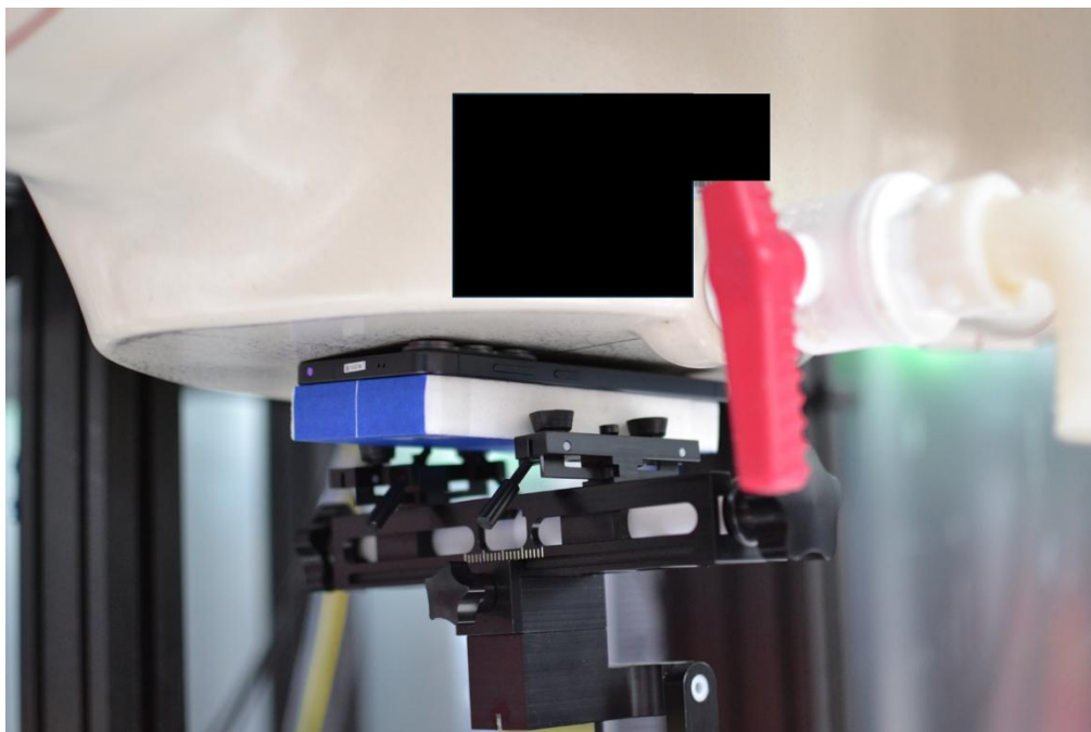
SAR Test Setup Photo 7 – Phablet, Back Side at 0mm (for Antenna G, H, F, I, MIMO)
