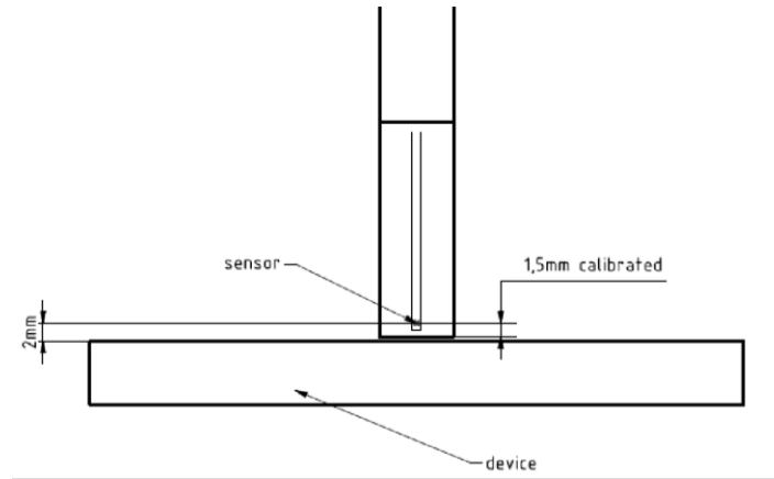
Figure J-3 EUmWVx Probe
