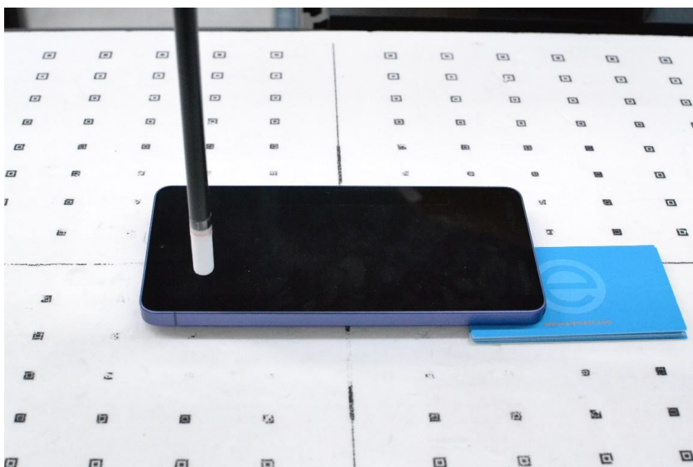
PD Test Setup Photo 32 – PD, Front Side at 9.95mm (Antenna G)
