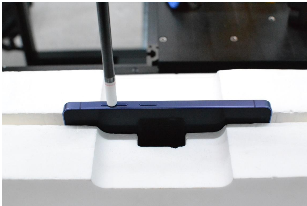
PD Test Setup Photo 38 – PD, Right Edge at 2mm (Antenna H)
