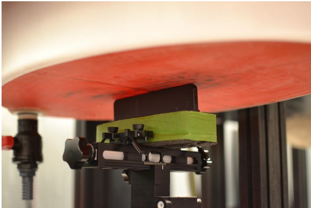
SAR Test Setup Photo 22 – NFC Phablet, Left Edge at 0mm
