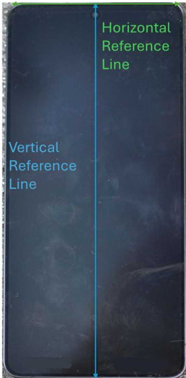
SAR Test Setup Photo 23 –Reference Lines
