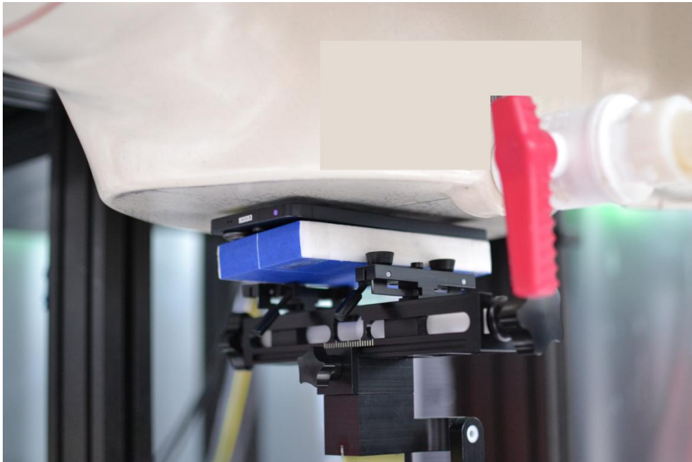
SAR Test Setup Photo 10 – Hotspot, Front Side at 5mm
