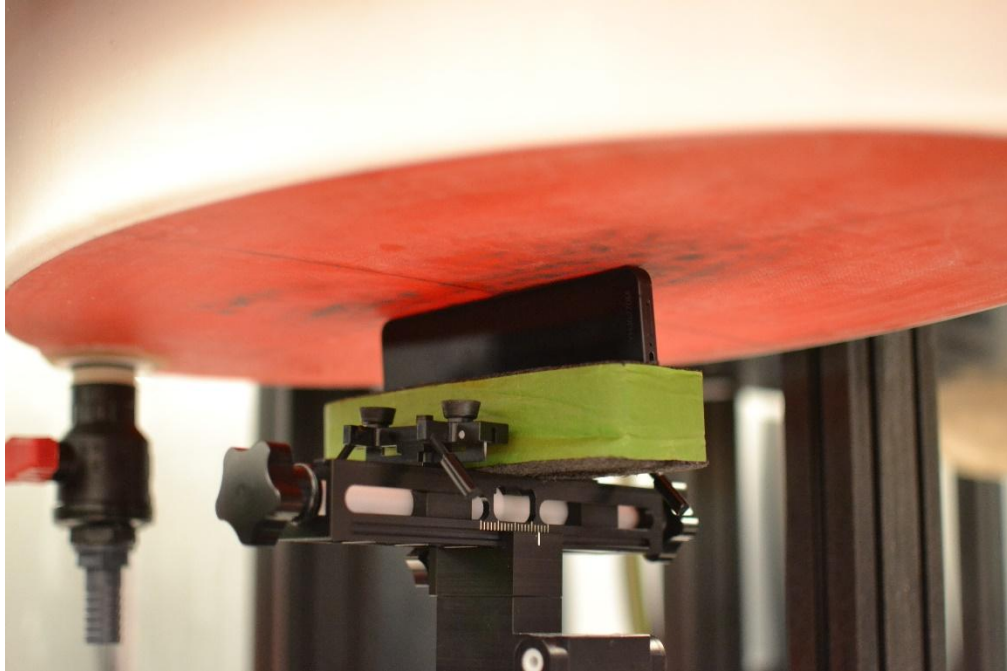
SAR Test Setup Photo 19 – NFC Phablet, Right Edge at 0mm
