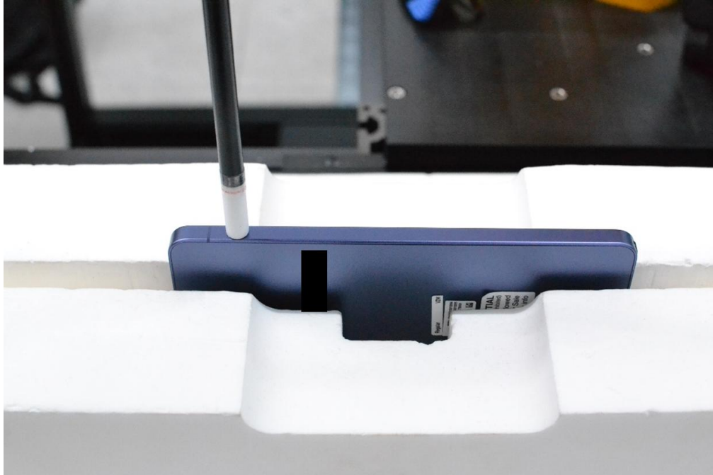
PD Test Setup Photo 35 – PD, Left Edge at 2mm (Antenna G, MIMO)
