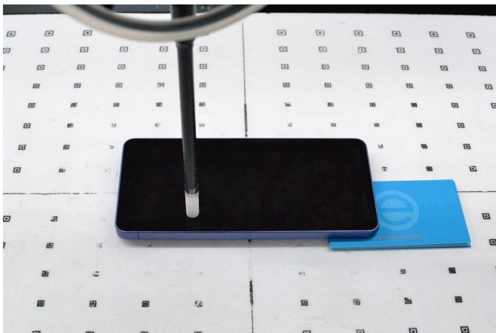
PD Test Setup Photo 31 – PD, Front Side at 2mm (Antenna H)
