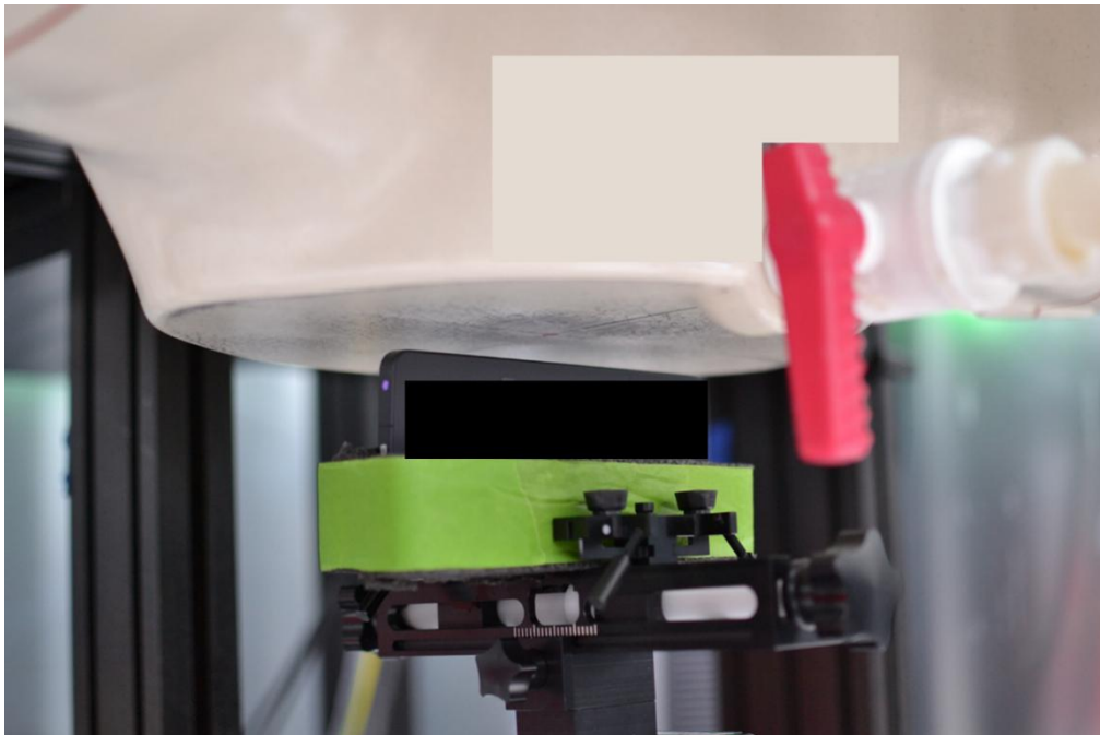
SAR Test Setup Photo 20 – Hotspot, Left Edge at 10mm
