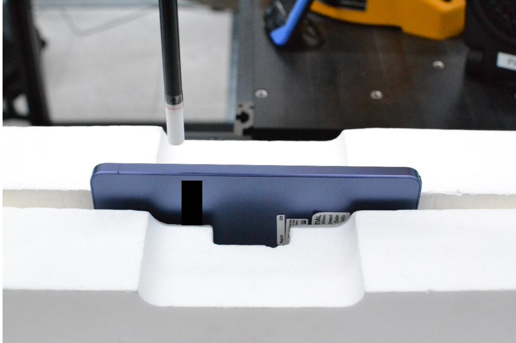
PD Test Setup Photo 37 – PD, Left Edge at 9.24mm (Antenna H)
