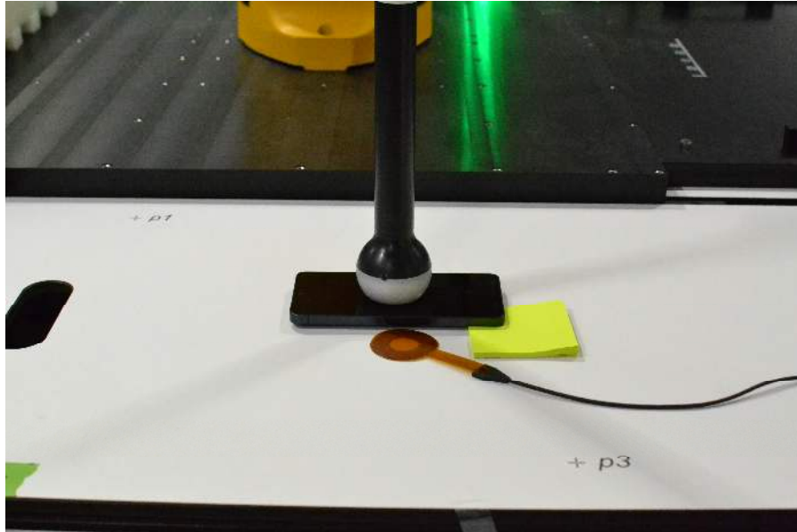
Test Setup Photo 1 Standby (Ping) Signal, Front side, 0mm
