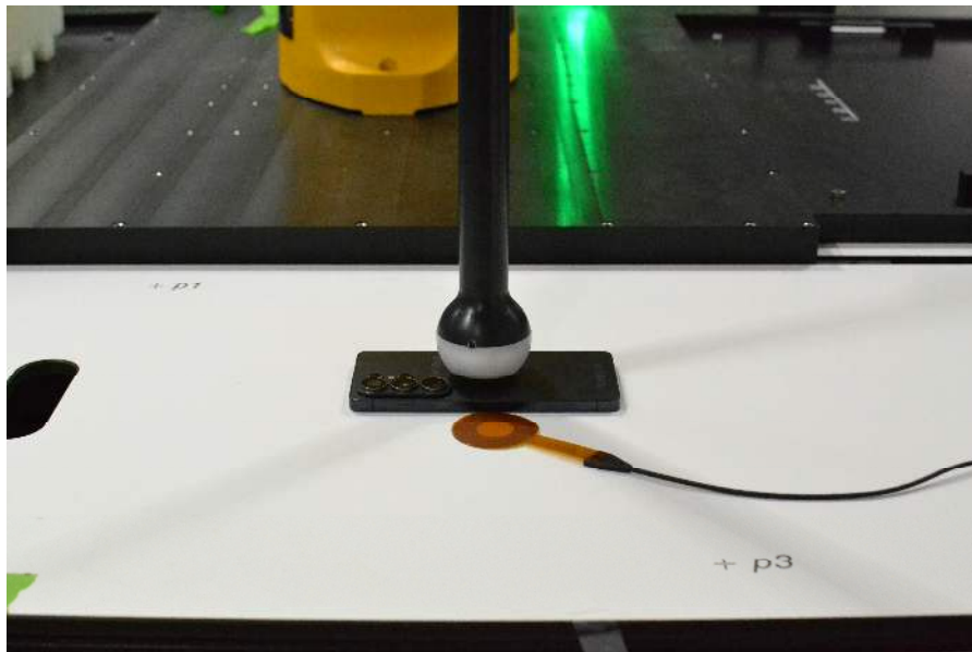
Test Setup Photo 2 Standby (Ping) Signal, Back side, 0mm
