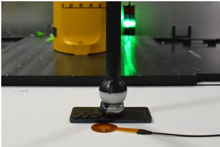
Test Setup Photo 10 Device to Earbuds, Back Side, 0mm
