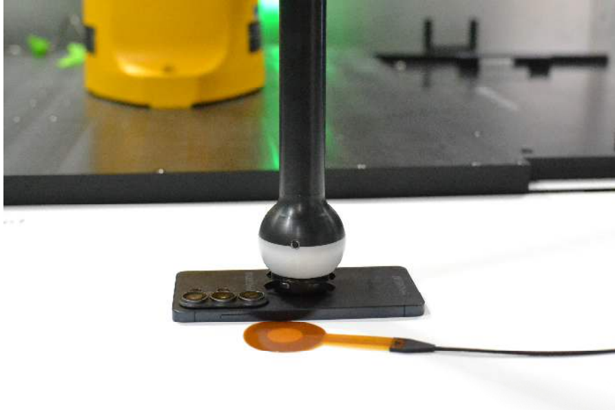
Test Setup Photo 9 Device to Watch, Back Side, 0mm
