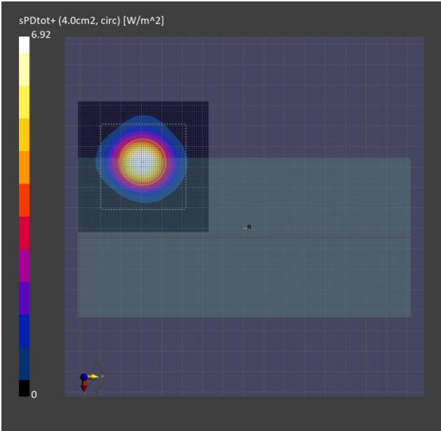
Figure 10-3 4cm 2 psPD distribution measured at input.power.limit of 3.0 dBm on the Back Side at 2mm for n258 beam 270
