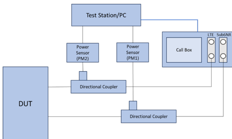
(c) Appendix D – Test Setup Photo 9
