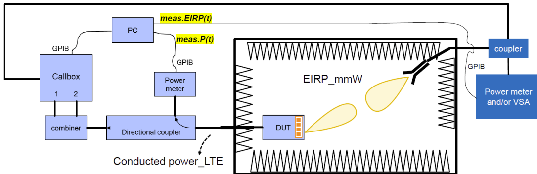
Figure 10-1 mmW NR radiated power measurement setup – Test Setup Photos 13
