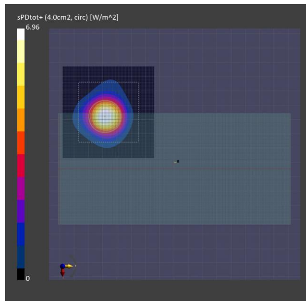
Figure 10-2 4cm 2 psPD distribution measured at input.power.limit of 2.5 dBm on the Back Side at 2mm for n261 beam 275
