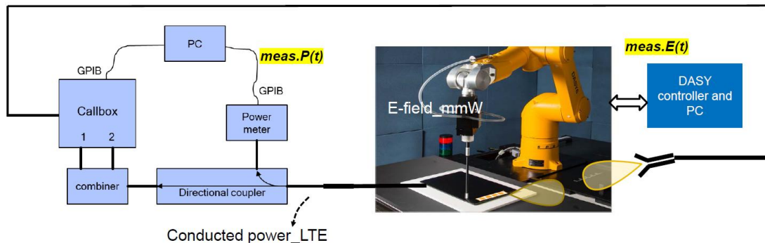
Figure 12-1 Power Density Measurement Setup – Test Setup Photos 14
