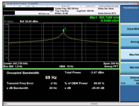
Figure 1-3 Digitizer Occupied Bandwidth
