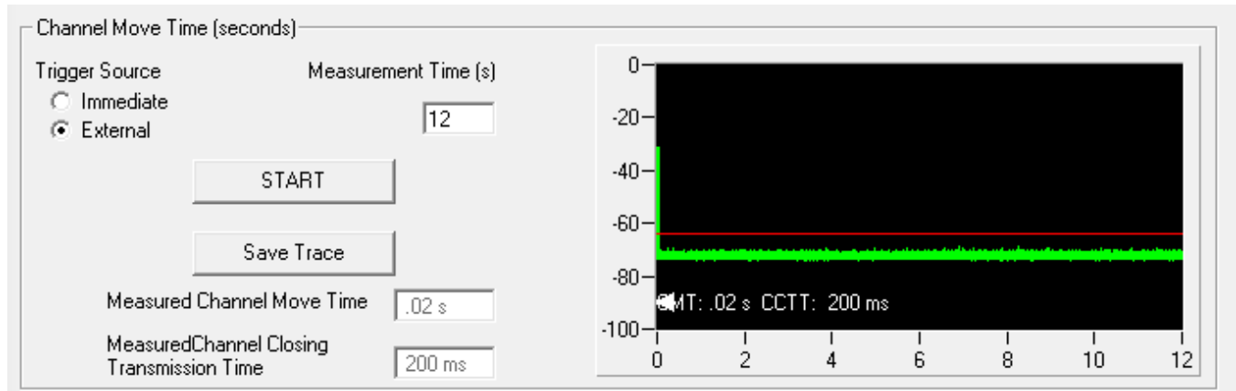
Figure 9-7. Band 2C CMT and CCTT – 20MHz
