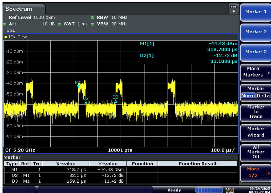
Figure 9-1. Band 2A Period – 20MHz
