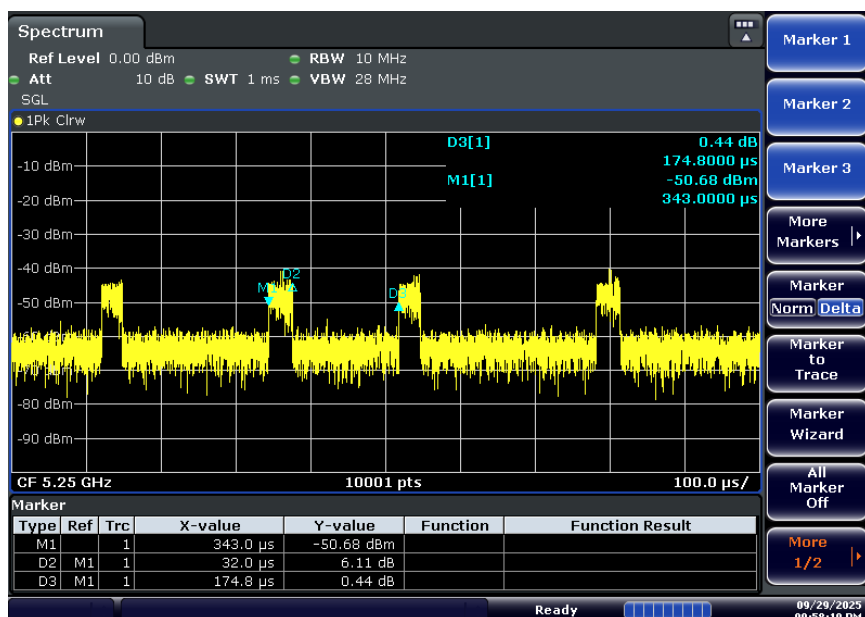
Figure 9-2. Band 2A Period – 160MHz
