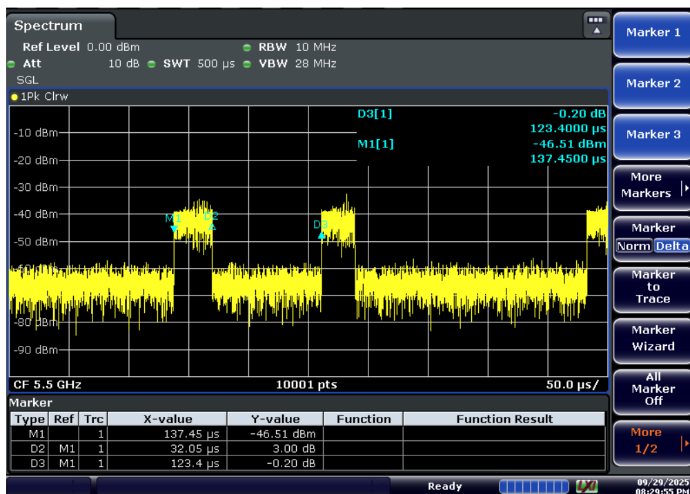
Figure 9-3. Band 2C Period – 20MHz
