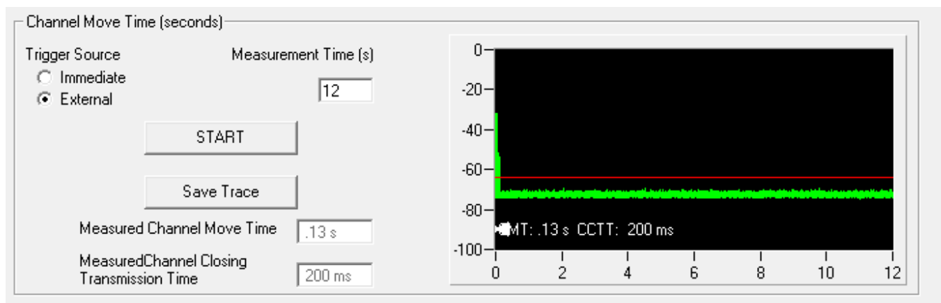
Figure 9-8. Band 2C CMT and CCTT – 160MHz
