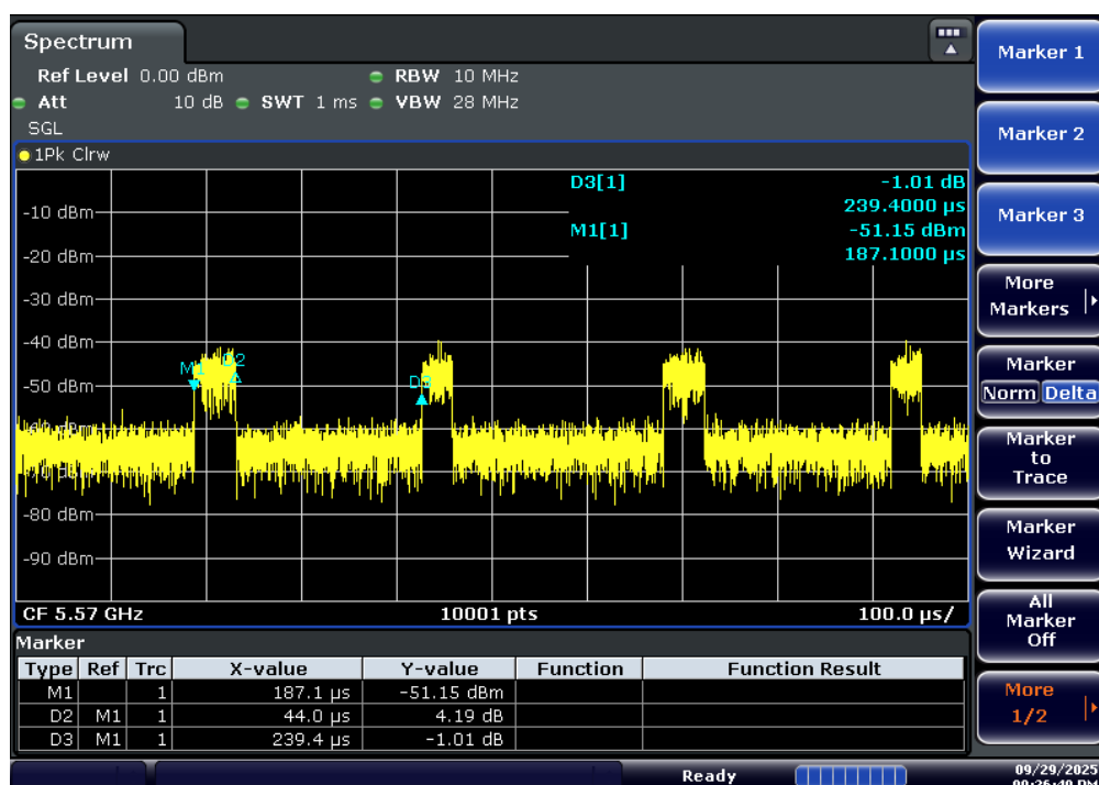
Figure 9-4. Band 2C Period – 160MHz
