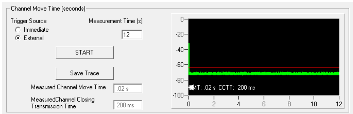
Figure 9-5. Band 2A CMT and CCTT – 20MHz
