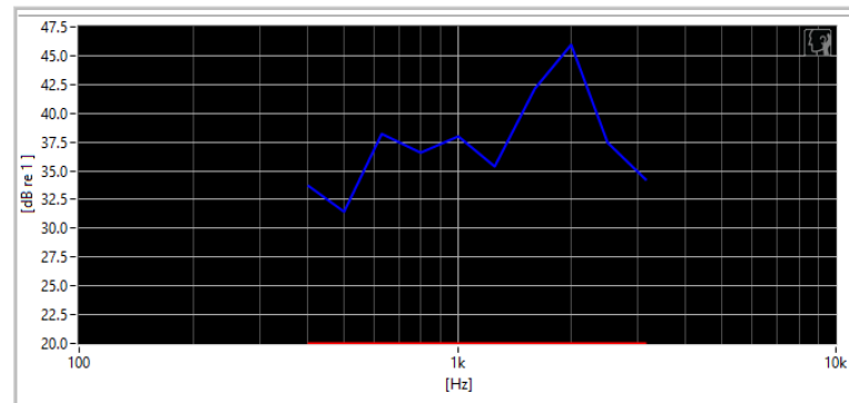
Results DF
