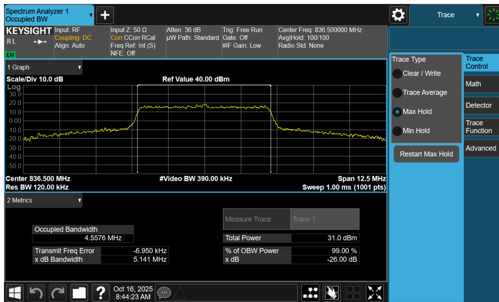
Plot 7-6. Occupied Bandwidth Plot (LTE Band 26/5 - 5MHz 16-QAM - Full RB - Ant1)
