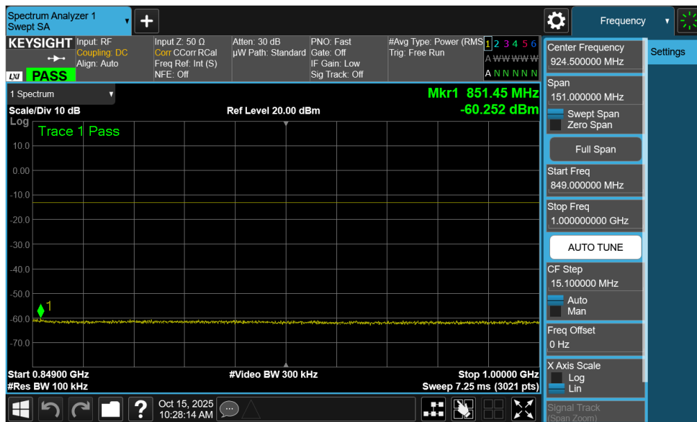
Plot 7-64. Conducted Spurious Plot (NR Band n26/5 - 20.0MHz - 1 RB - Mid Channel - Ant1)
