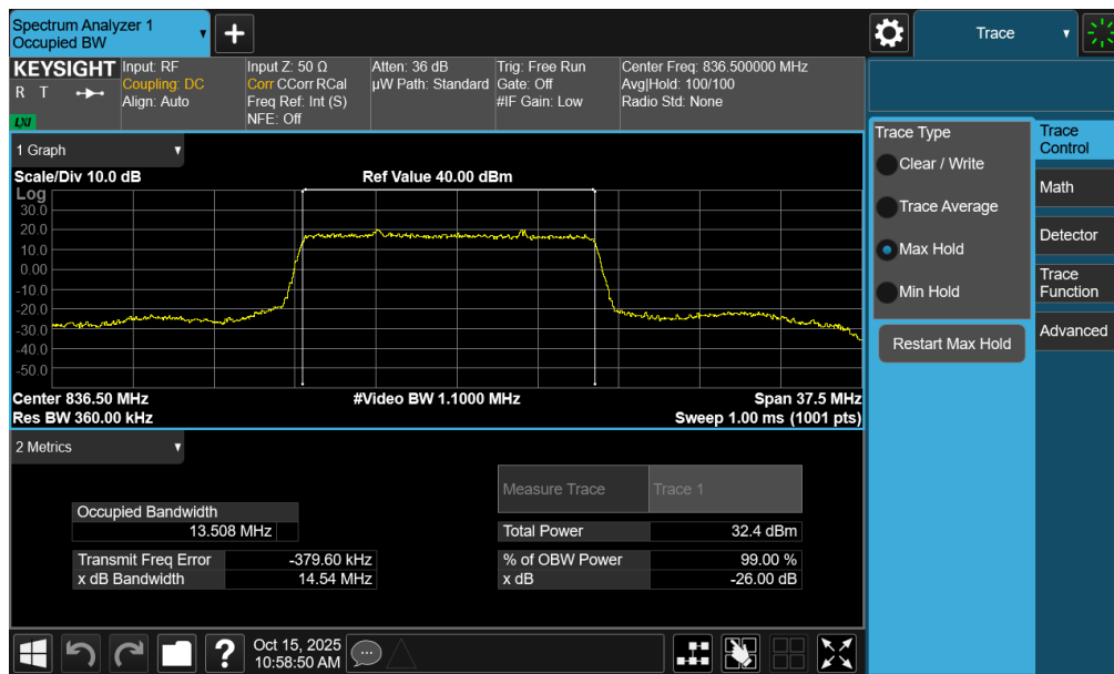
Plot 7-14. Occupied Bandwidth Plot (NR Band n26/5 - 15MHz \pi/2 BPSK - Full RB - Ant1)
