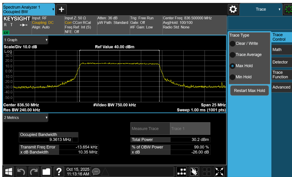
Plot 7-18. Occupied Bandwidth Plot (NR Band n26/5 - 10MHz QPSK - Full RB - Ant1)
