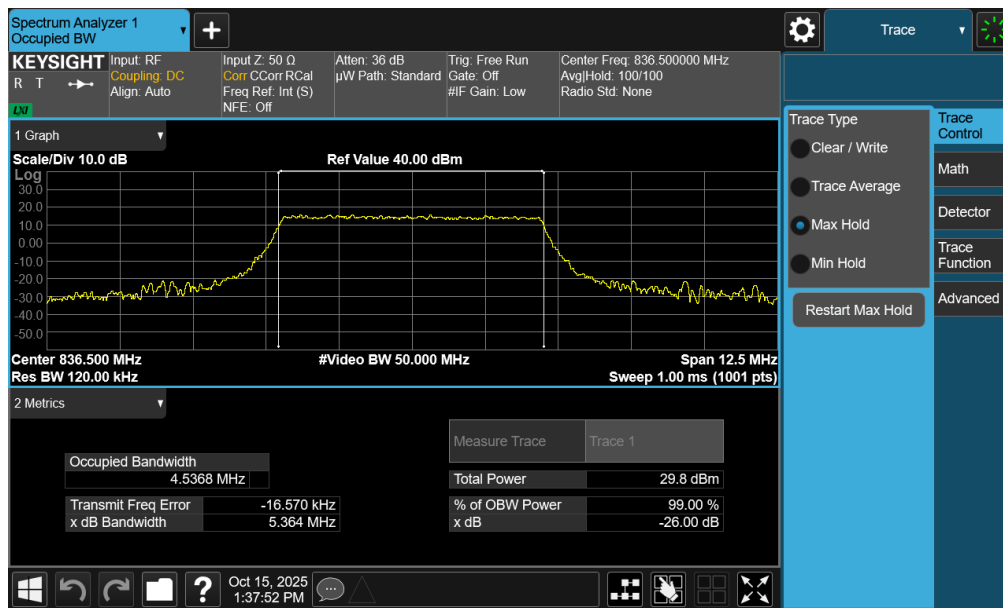
Plot 7-47. Occupied Bandwidth Plot (NR Band n26/5 - 5MHz 16-QAM - Full RB - Ant2)
