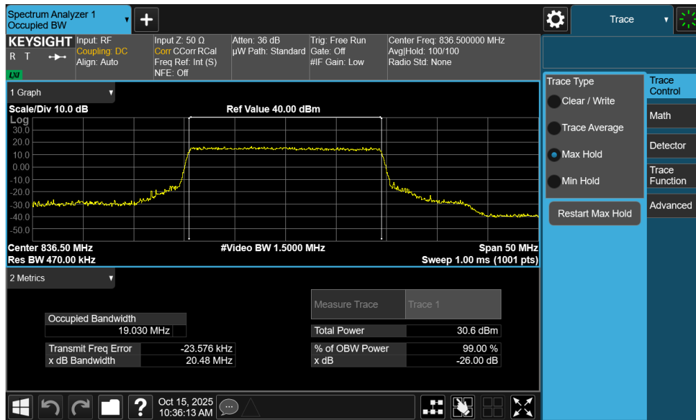
Plot 7-13. Occupied Bandwidth Plot (NR Band n26/5 - 20MHz 16-QAM - Full RB - Ant1)
