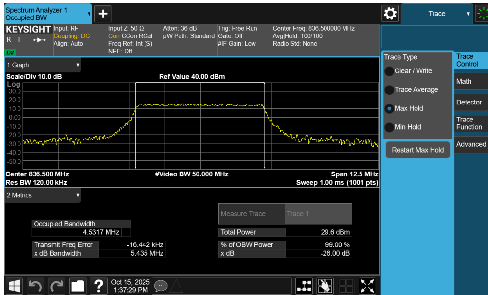
Plot 7-46. Occupied Bandwidth Plot (NR Band n26/5 - 5MHz QPSK - Full RB - Ant2)
