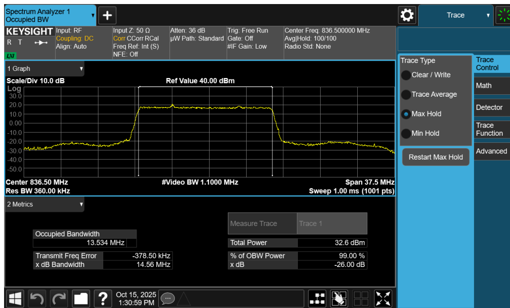
Plot 7-39. Occupied Bandwidth Plot (NR Band n26/5 - 15MHz \pi/2 BPSK - Full RB - Ant2)
