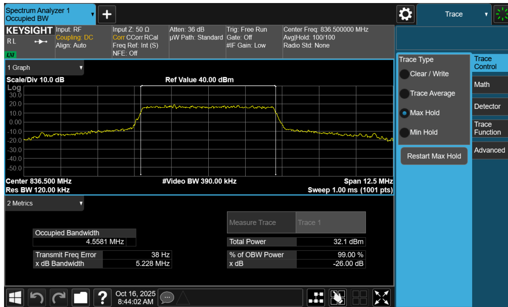
Plot 7-5. Occupied Bandwidth Plot (LTE Band 26/5 - 5MHz QPSK - Full RB - Ant1)
