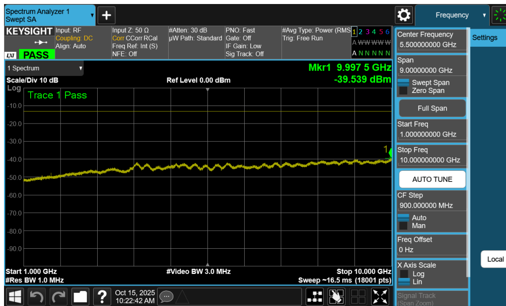
Plot 7-62. Conducted Spurious Plot (NR Band n26/5 - 20.0MHz - 1 RB - Low Channel - Ant1)
