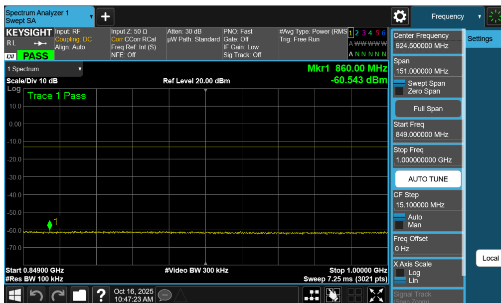
Plot 7-88. Conducted Spurious Plot (LTE Band 26/5 - 15MHz QPSK - 1 RB - Low Channel – Ant2)
