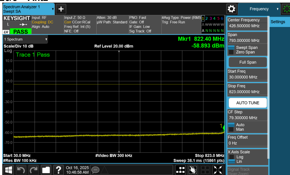
Plot 7-87. Conducted Spurious Plot (LTE Band 26/5 - 15MHz QPSK – 1 RB - Low Channel – Ant2)
