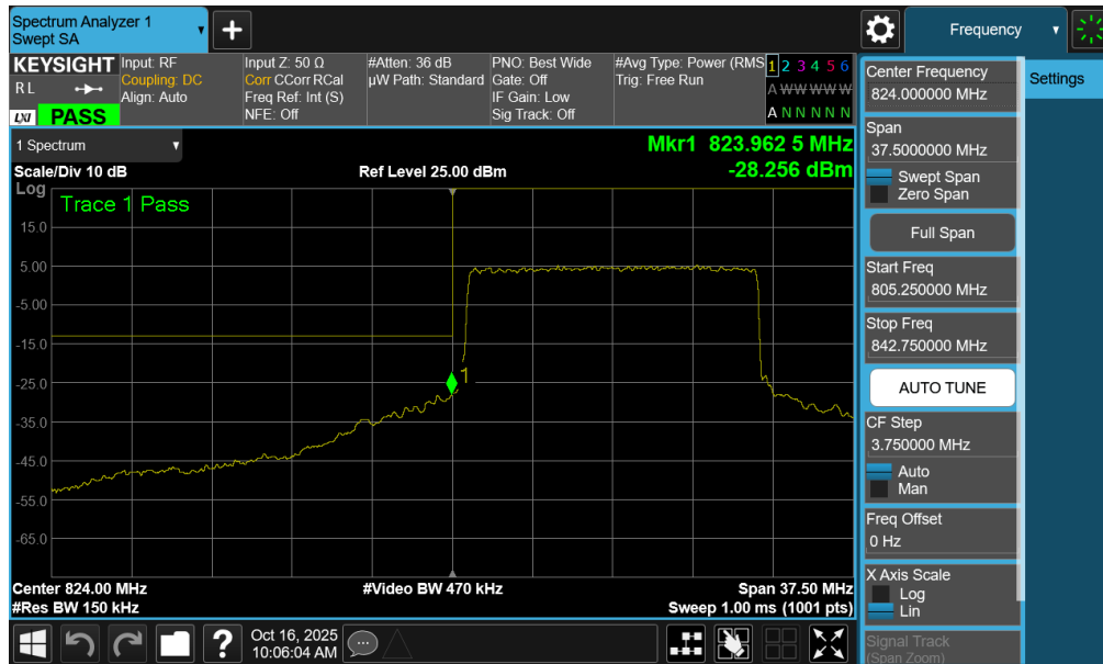
Plot 7-123. Lower Band Edge Plot (LTE Band 26 - 15MHz QPSK – Full RB - Ant1)
