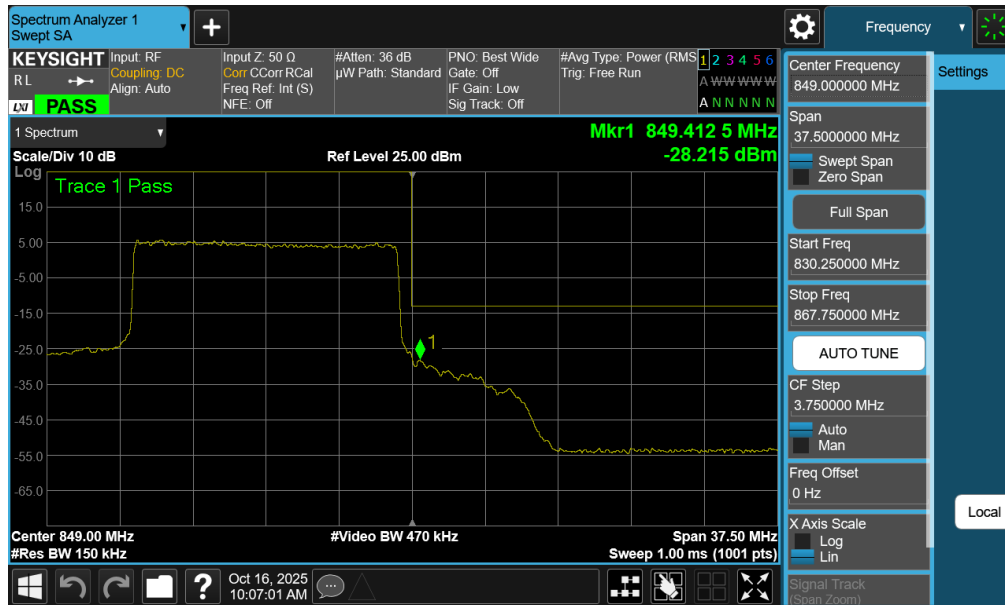
Plot 7-124. Upper Band Edge Plot (LTE Band 26 - 15MHz QPSK – Full RB - Ant1)
