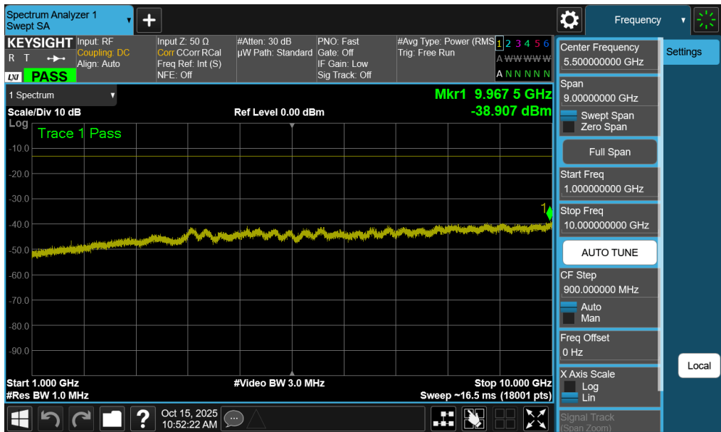
Plot 7-68. Conducted Spurious Plot (NR Band n26/5 - 20.0MHz - 1 RB - High Channel - Ant1)
