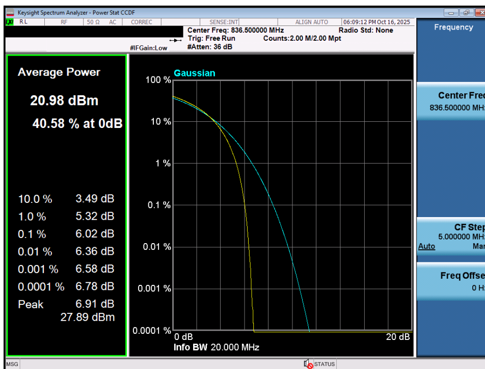
Plot 7-183. Peak-Average Ratio Plot (NR Band n26/5 - 20MHz QPSK - Full RB - Ant2)
