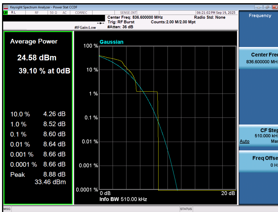
Plot 7-178. Peak-Average Ratio Plot (EDGE, Ch. 190 – Ant2)
