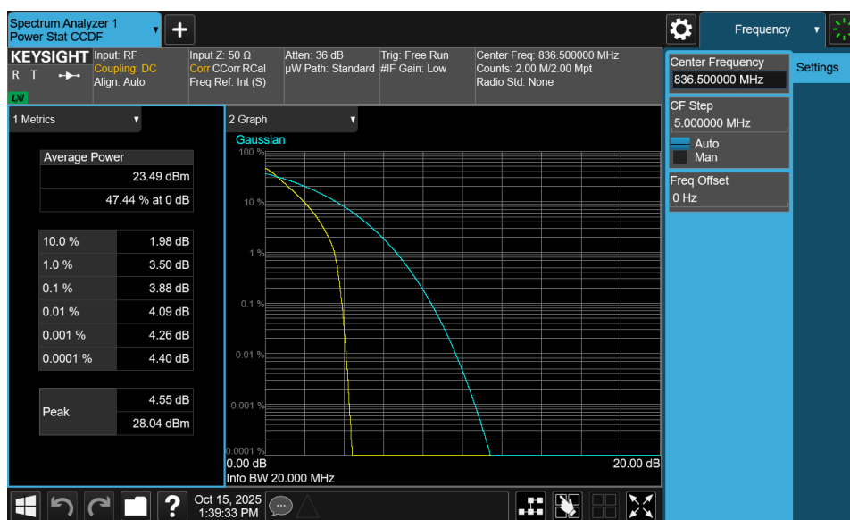
Plot 7-182. Peak-Average Ratio Plot (NR Band n26/5 - 20MHz \pi/2 BPSK - Full RB - Ant2)
