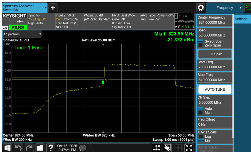
Plot 7-155. Lower Band Edge Plot (NR Band n26/5 – 20.0MHz - Full RB - Ant2)
