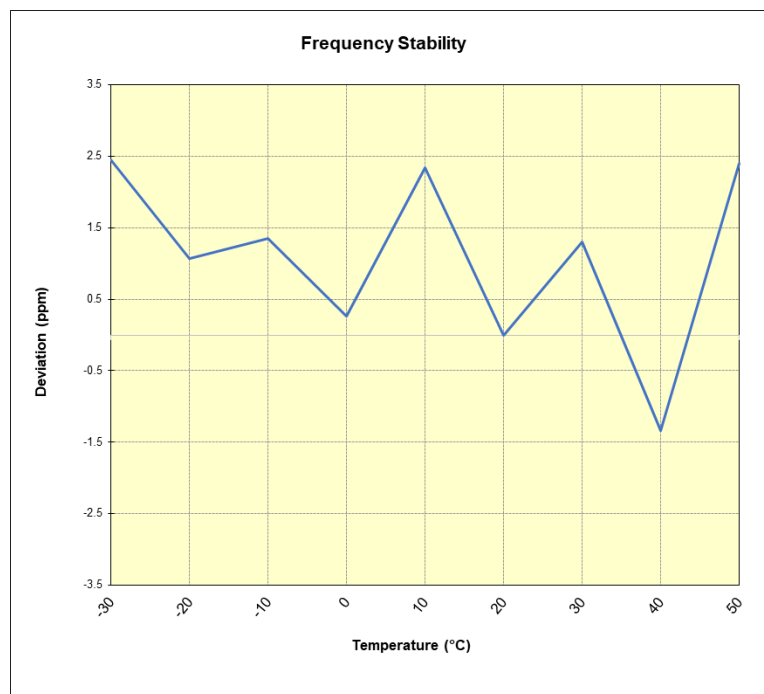
Plot 7-202. NR Band n26/5 Frequency Stability Chart
