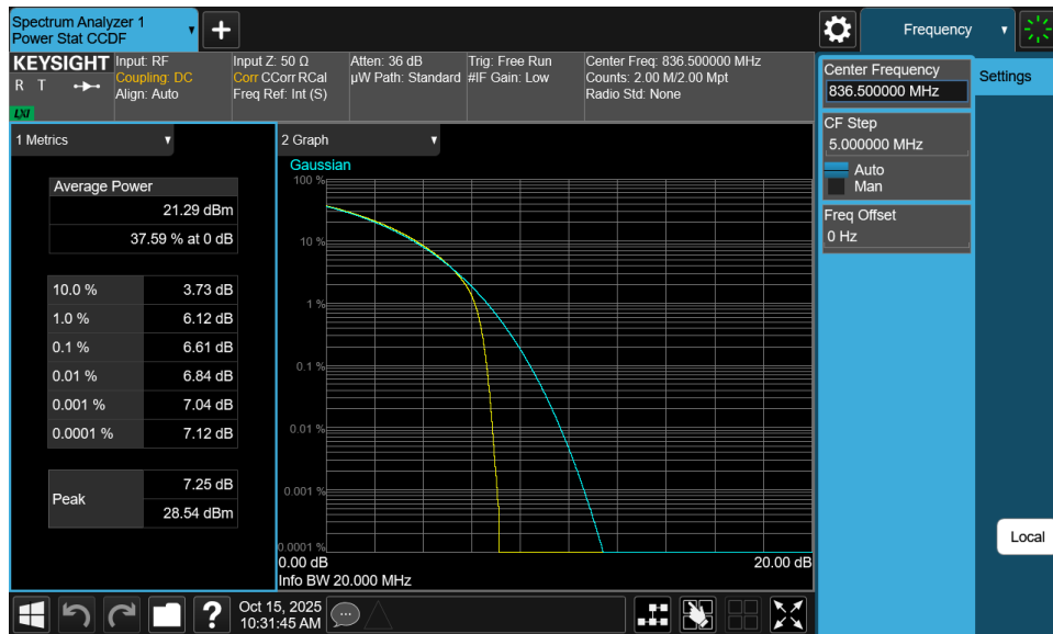
Plot 7-175. Peak-Average Ratio Plot (NR Band n26/5 - 20MHz QPSK - Full RB - Ant1)
