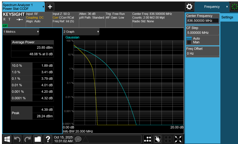
Plot 7-174. Peak-Average Ratio Plot (NR Band n26/5 - 20MHz \pi/2 BPSK - Full RB - Ant1)
