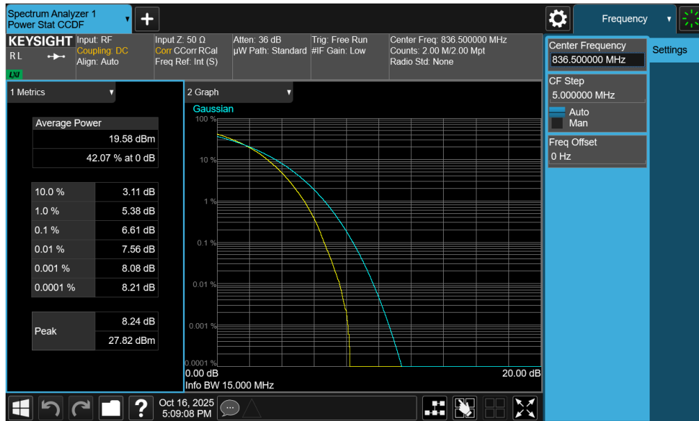
Plot 7-171. Peak-Average Ratio Plot (LTE Band 26 - 15MHz 256-QAM - Full RB - Ant1)
