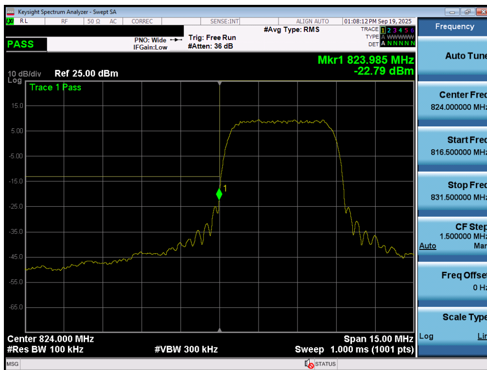
Plot 7-165. Lower Band Edge Plot (WCDMA Cell – Ch. 4132 – Ant2)
