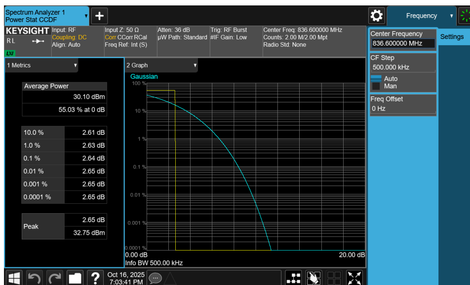
Plot 7-177. Peak-Average Ratio Plot (GPRS, Ch. 190 – Ant2)
