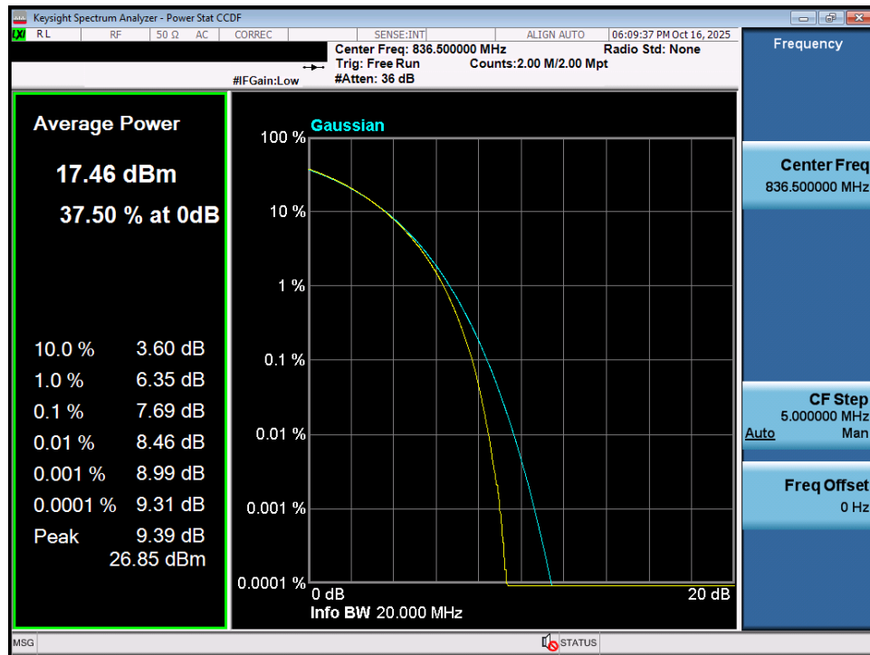
Plot 7-184. Peak-Average Ratio Plot (NR Band n26/5 - 20MHz 256-QAM - Full RB - Ant2)
