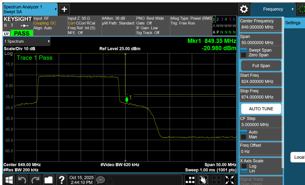
Plot 7-156. Upper Band Edge Plot (NR Band n26/5 – 20.0MHz - Full RB - Ant2)
