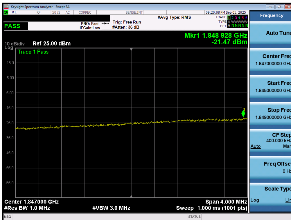
Plot 7-95. Extended Lower Band Edge Plot (LTE Band 25/2 - 15MHz QPSK – Full RB - Ant1)
