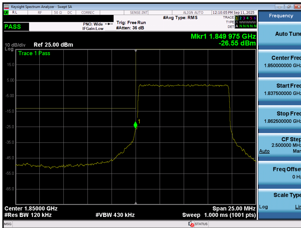
Plot 7-100. Lower Band Edge Plot (NR Band n25/2 - 10MHz QPSK – Full RB - Ant1)
