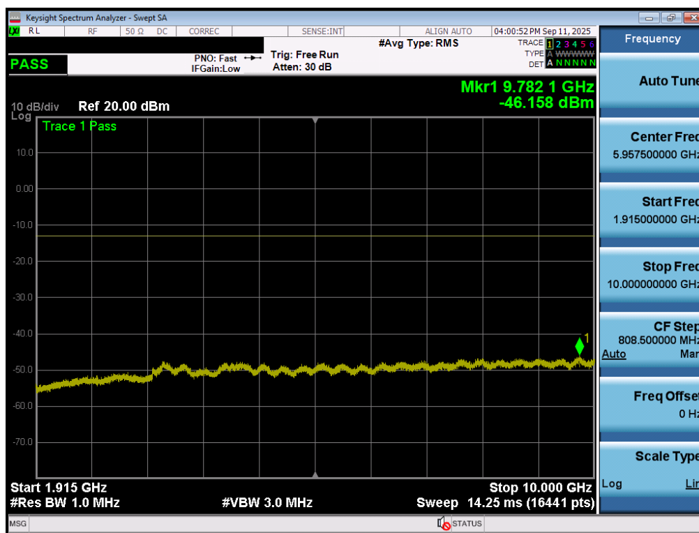
Plot 7-92. Conducted Spurious Plot (NR Band n25/2 - 40.0MHz - 1RB - High Channel - Ant2)
