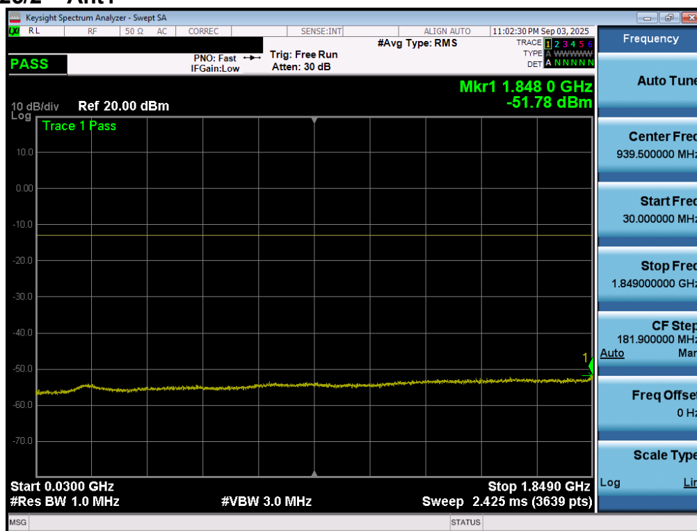
Plot 7-76. Conducted Spurious Plot (LTE Band 25/2 - 20MHz QPSK - 1RB - Low Channel - Ant1)
