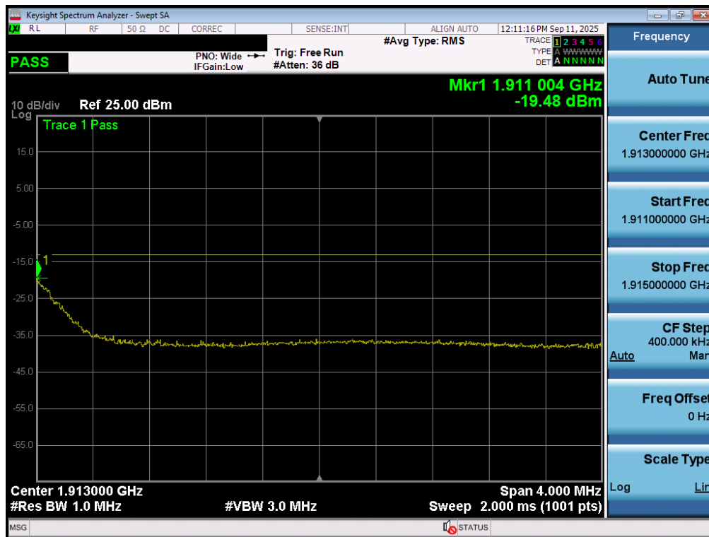
Plot 7-103. Extended Upper Band Edge Plot (NR Band n2 - 10MHz QPSK – Full RB - Ant1)
