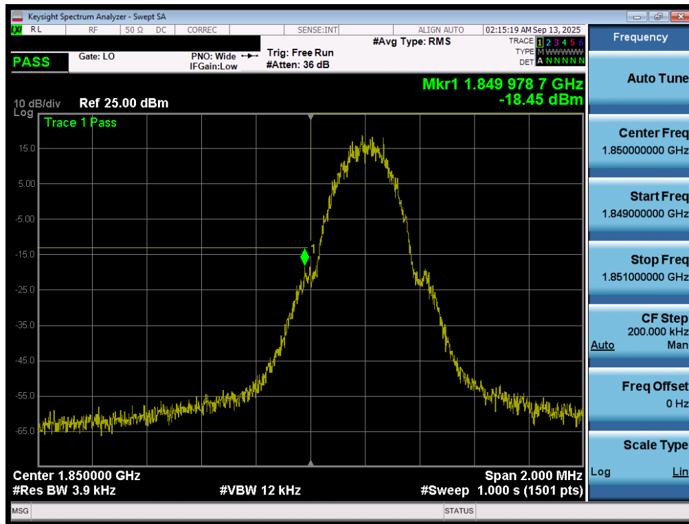
Plot 7-106. Lower Band Edge Plot (GPRS PCS – Ch. 512 - Ant1)
