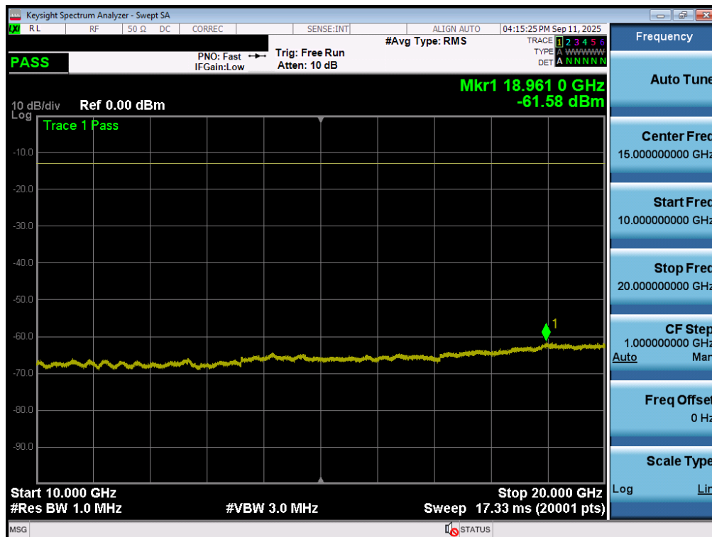
Plot 7-81. Conducted Spurious Plot (NR Band n25/2 - 40.0MHz - 1RB - Mid Channel - Ant1)
