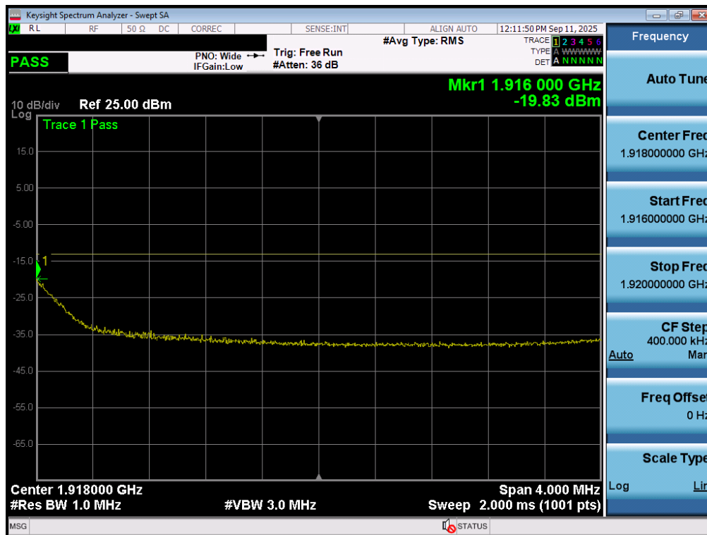
Plot 7-105. Extended Upper Band Edge Plot (NR Band n25 - 10MHz QPSK – Full RB - Ant1)
