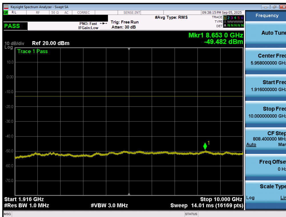
Plot 7-89. Conducted Spurious Plot (LTE Band 25/2 - 20MHz QPSK - 1RB - High Channel - Ant2)
