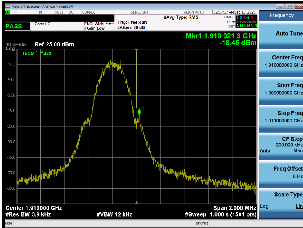
Plot 7-107. Upper Band Edge Plot (GPRS PCS – Ch. 810 - Ant1)
