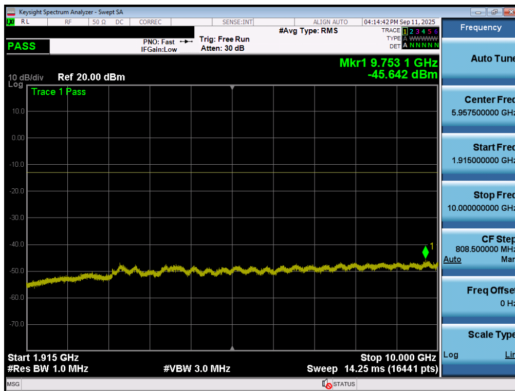
Plot 7-80. Conducted Spurious Plot (NR Band n25/2 - 40.0MHz - 1RB - Mid Channel - Ant1)
