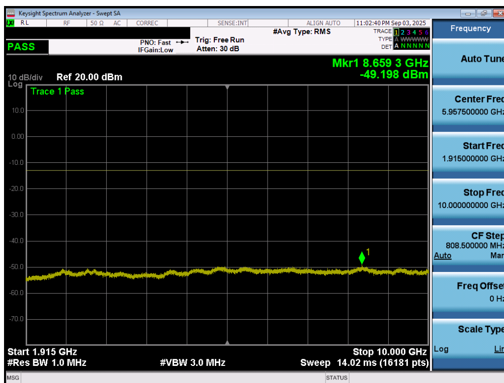
Plot 7-77. Conducted Spurious Plot (LTE Band 25/2 - 20MHz QPSK - 1RB - Low Channel - Ant1)
