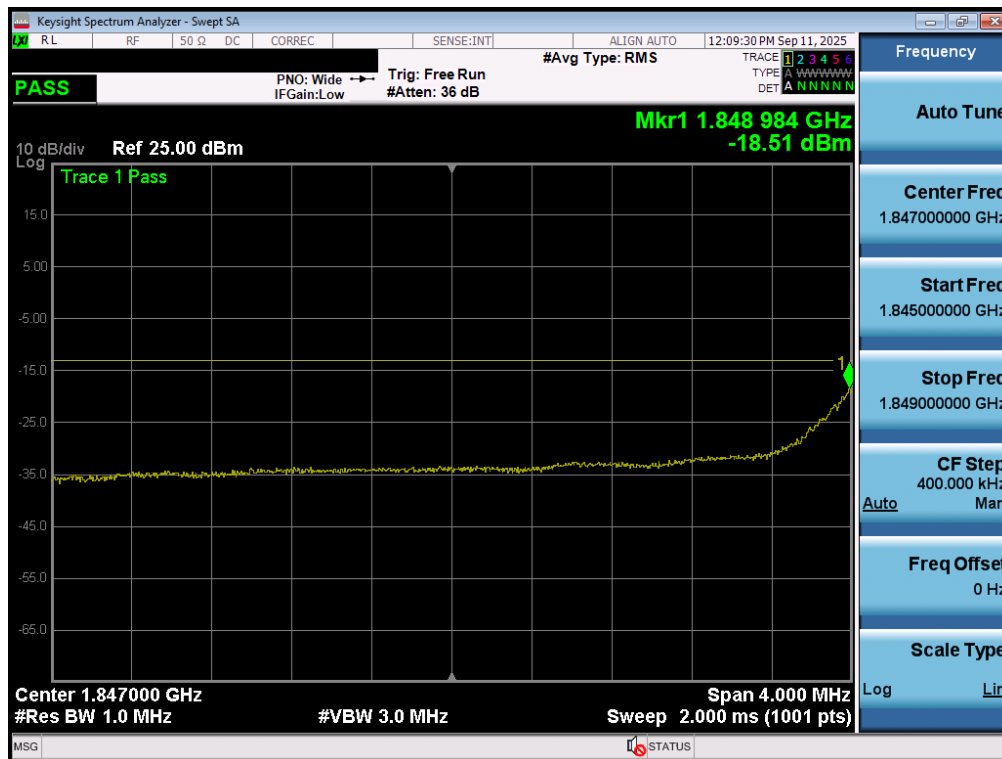
Plot 7-101. Extended Lower Band Edge Plot (NR Band n25/2 - 10MHz QPSK – Full RB - Ant1)
