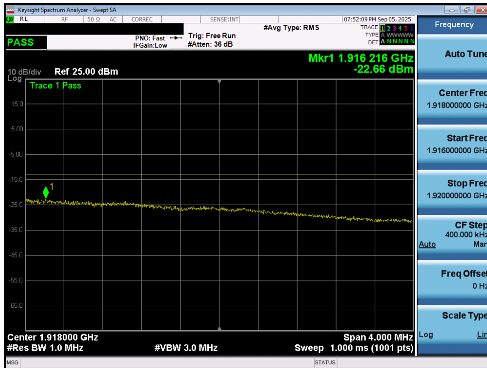
Plot 7-99. Extended Upper Band Edge Plot (LTE Band 25 - 15MHz QPSK – Full RB - Ant1)
