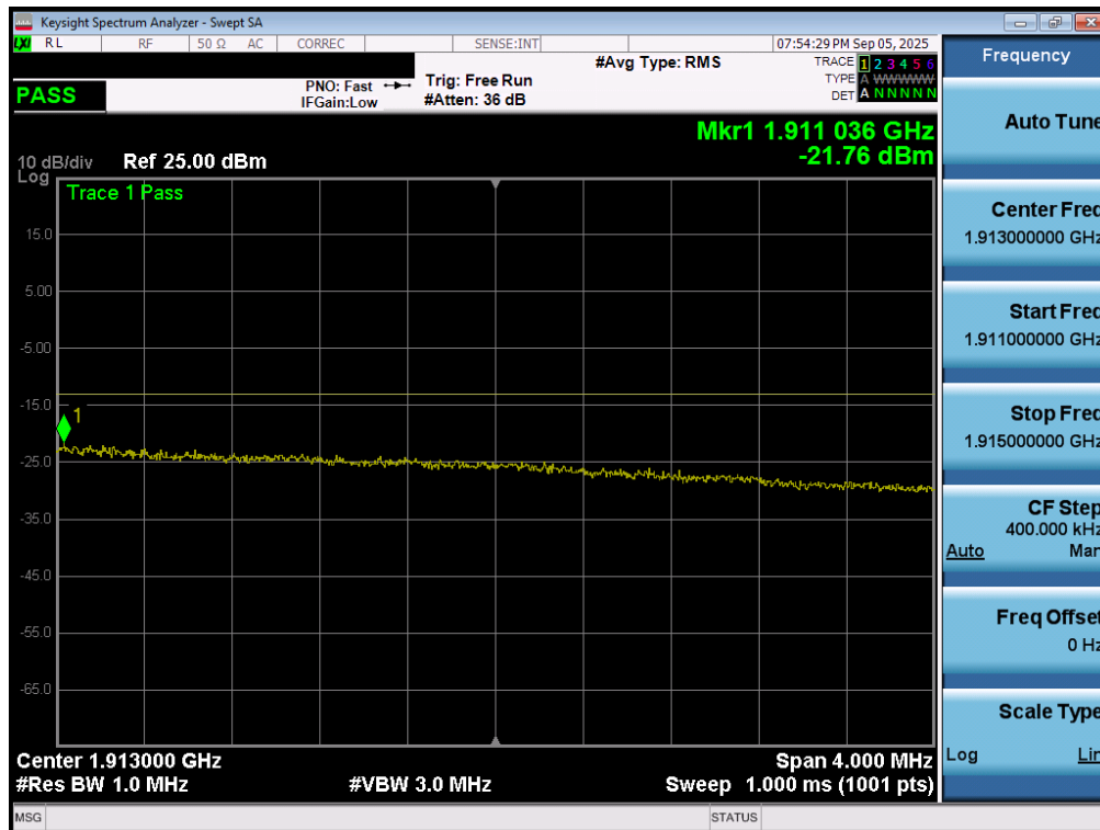
Plot 7-97. Extended Upper Band Edge Plot (LTE Band 2 - 15MHz QPSK – Full RB - Ant1)
