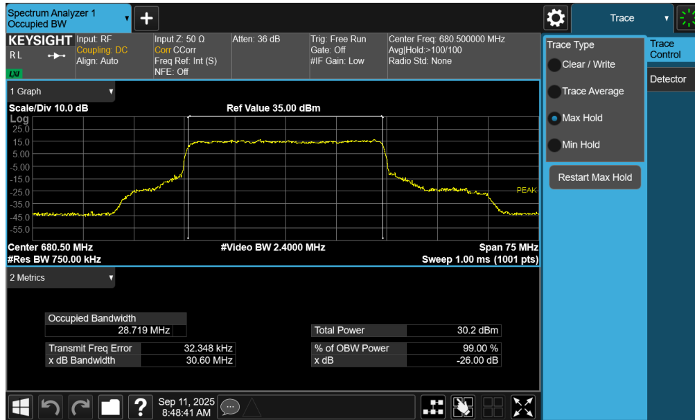
Plot 7-47. Occupied Bandwidth Plot (NR Band n71 – 30MHz CP-OFDM QPSK - Full RB – ANT1)
