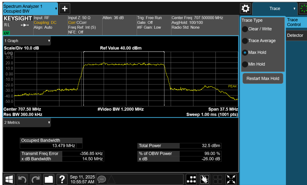
Plot 7-34. Occupied Bandwidth Plot (NR Band n12 - 15MHz DFT-s-OFDM BPSK - Full RB – ANT1)
