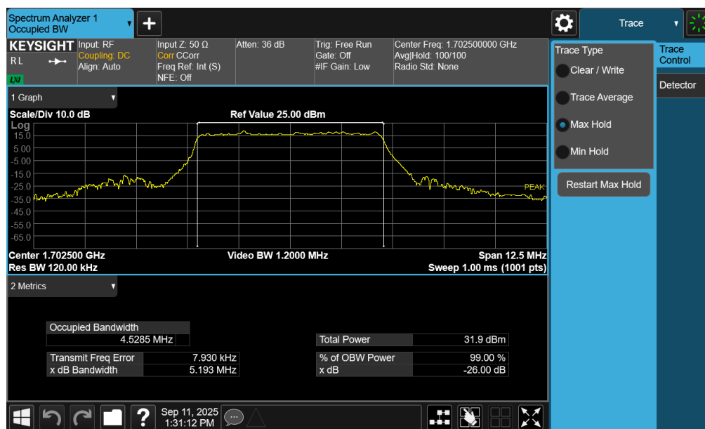
Plot 7-70. Occupied Bandwidth Plot (NR Band n70 - 5.0MHz DFT-s-OFDM BPSK - Full RB – ANT1)
