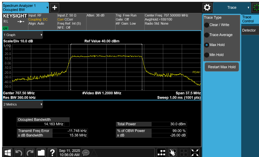
Plot 7-35. Occupied Bandwidth Plot (NR Band n12 - 15MHz QPSK - Full RB – ANT1)
