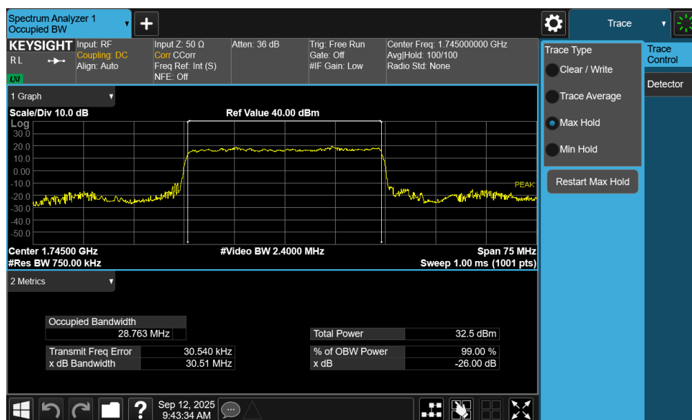
Plot 7-82. Occupied Bandwidth Plot (NR Band n66 - 30.0MHz DFT-s-OFDM BPSK - Full RB – ANT1)
