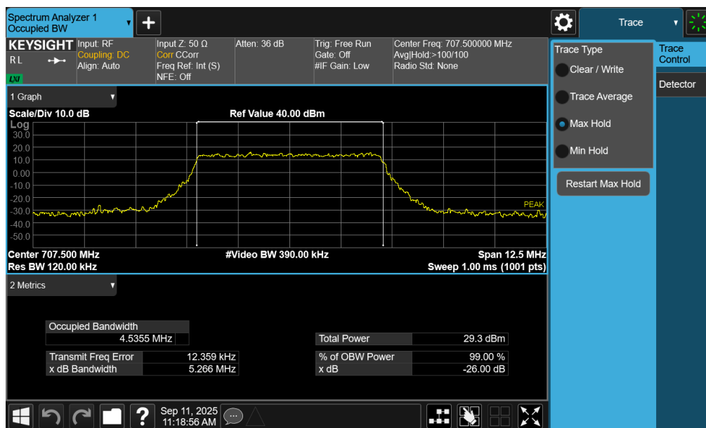
Plot 7-41. Occupied Bandwidth Plot (NR Band n12 - 5MHz CP-OFDM QPSK - Full RB – ANT1)
