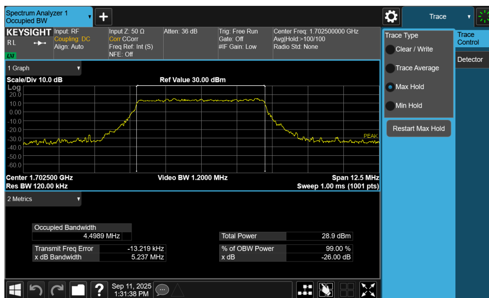
Plot 7-71. Occupied Bandwidth Plot (NR Band n70 - 5.0MHz CP-OFDM QPSK - Full RB – ANT1)
