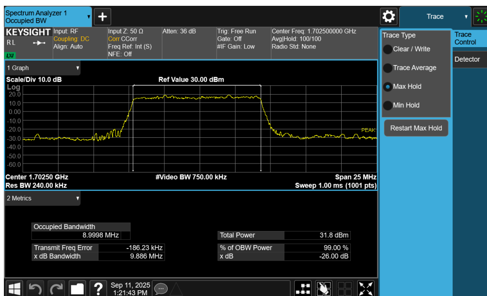
Plot 7-67. Occupied Bandwidth Plot (NR Band n70 - 10.0MHz DFT-s-OFDM BPSK - Full RB – ANT1)
