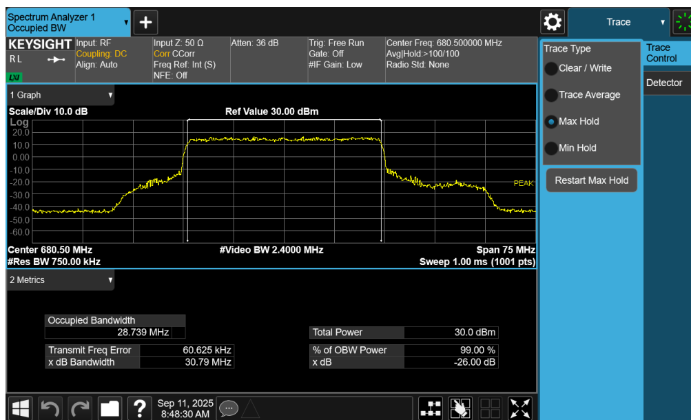
Plot 7-48. Occupied Bandwidth Plot (NR Band n71 - 30MHz CP-OFDM 16-QAM - Full RB – ANT1)
