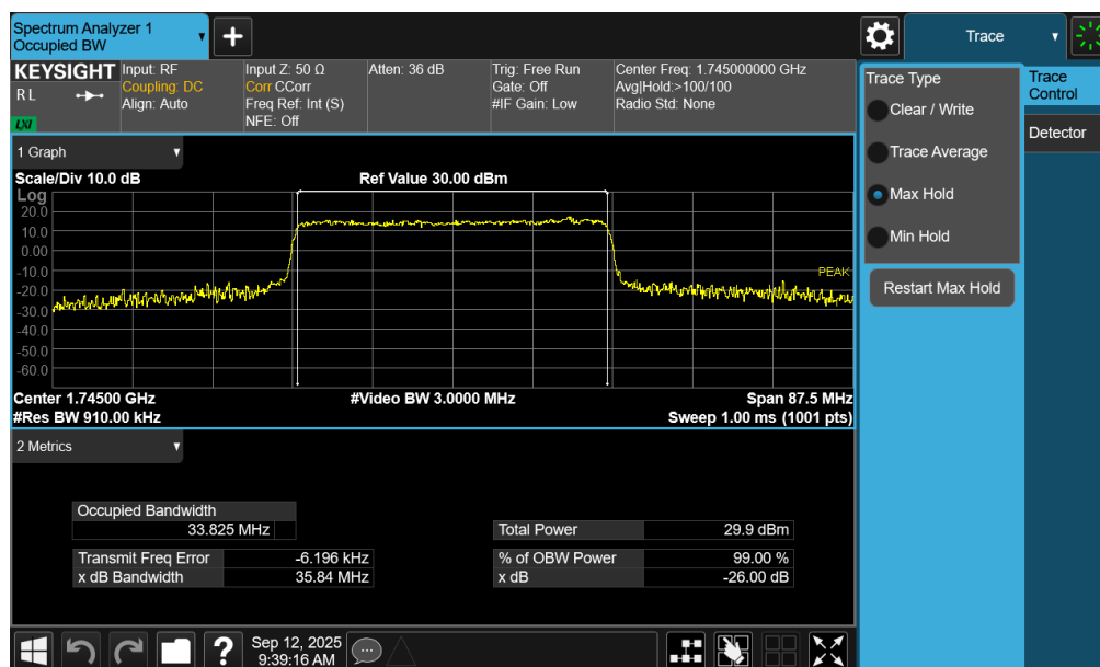
Plot 7-81. Occupied Bandwidth Plot (NR Band n66 - 35.0MHz CP-OFDM 16QAM - Full RB – ANT1)
