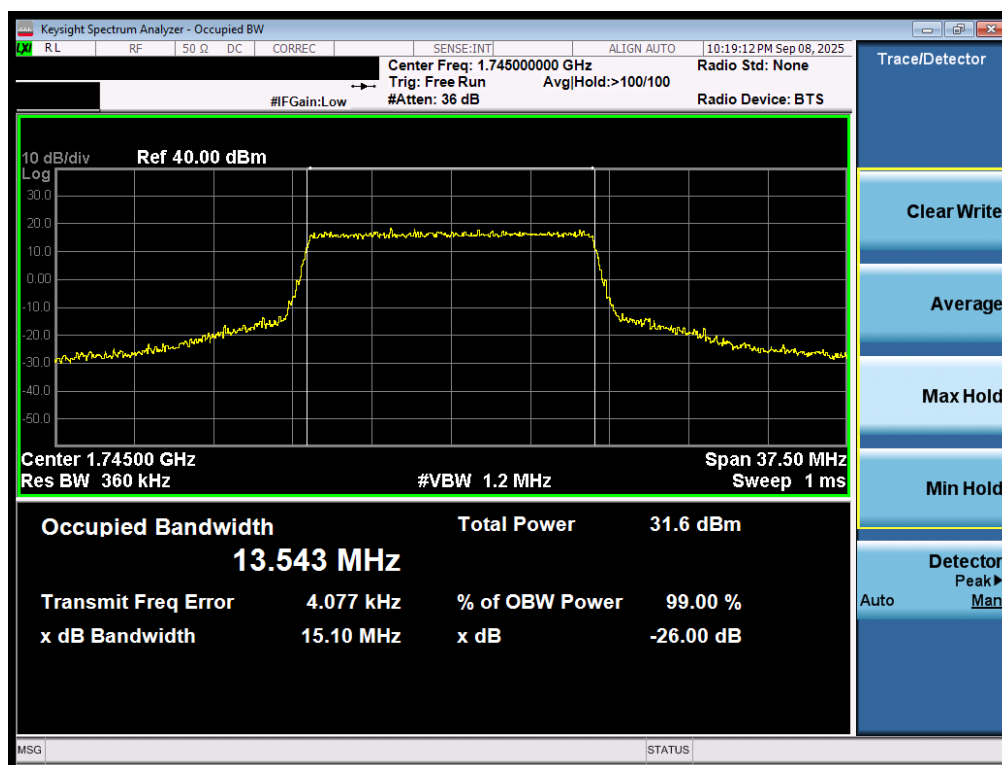
Plot 7-24. Occupied Bandwidth Plot (LTE Band 66/4 - 15MHz QPSK - Full RB - ANT1)
