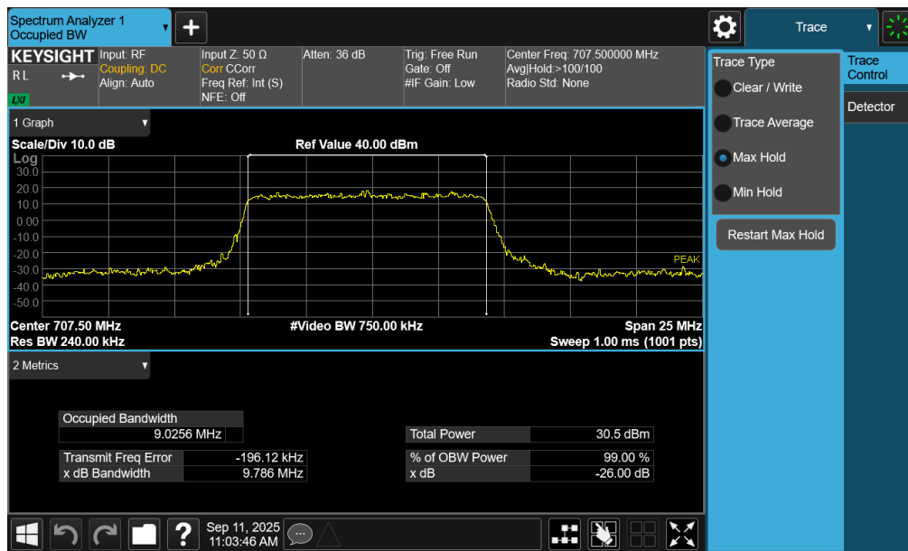
Plot 7-39. Occupied Bandwidth Plot (NR Band n12 - 10MHz CP-OFDM 16-QAM - Full RB – ANT1)
