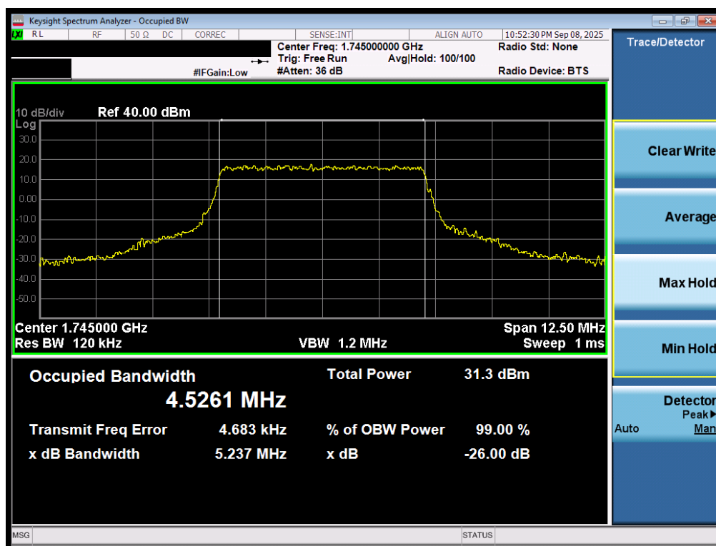
Plot 7-28. Occupied Bandwidth Plot (LTE Band 66/4 - 5MHz QPSK - Full RB - ANT1)
