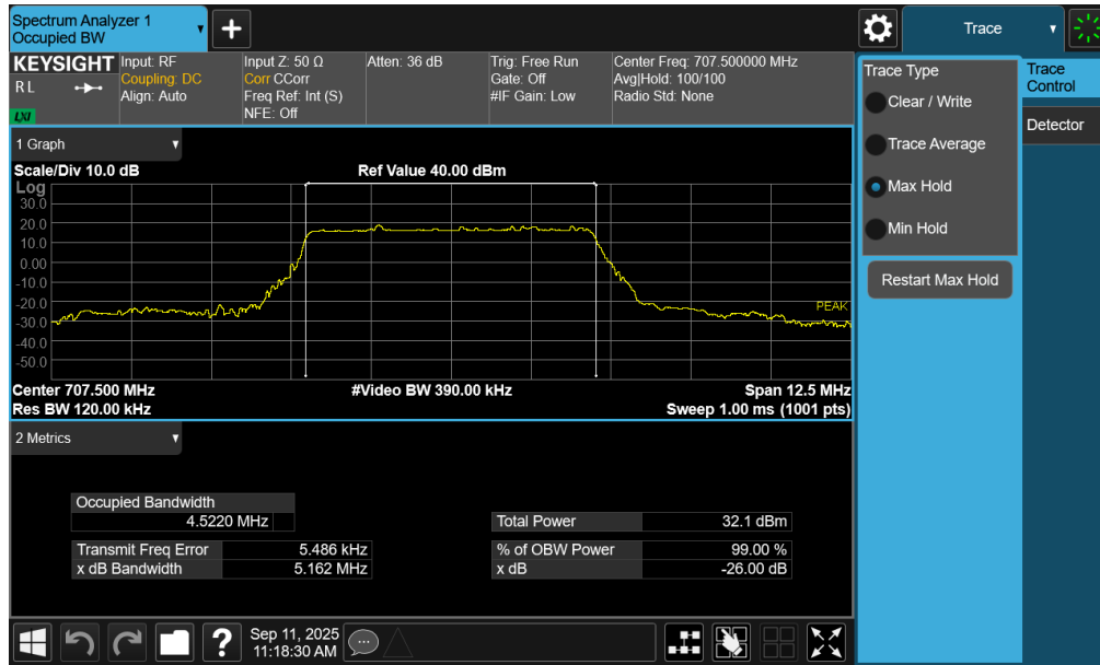
Plot 7-40. Occupied Bandwidth Plot (NR Band n12 - 5MHz DFT-s-OFDM BPSK - Full RB – ANT1)
