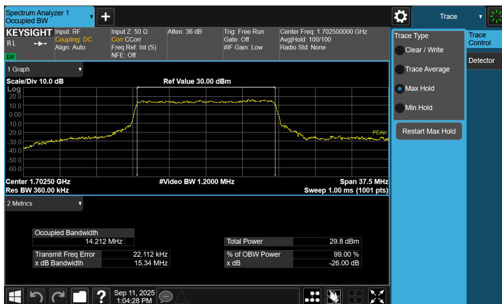
Plot 7-66. Occupied Bandwidth Plot (NR Band n70 - 15.0MHz CP-OFDM 16QAM - Full RB – ANT1)
