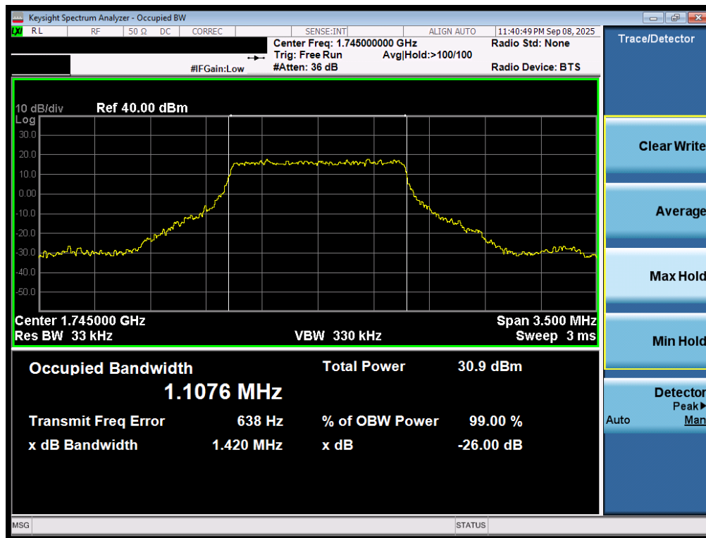
Plot 7-32. Occupied Bandwidth Plot (LTE Band 66/4 - 1.4MHz QPSK - Full RB - ANT1)
