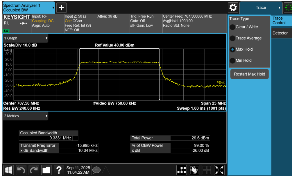
Plot 7-38. Occupied Bandwidth Plot (NR Band n12 - 10MHz CP-OFDM QPSK - Full RB – ANT1)
